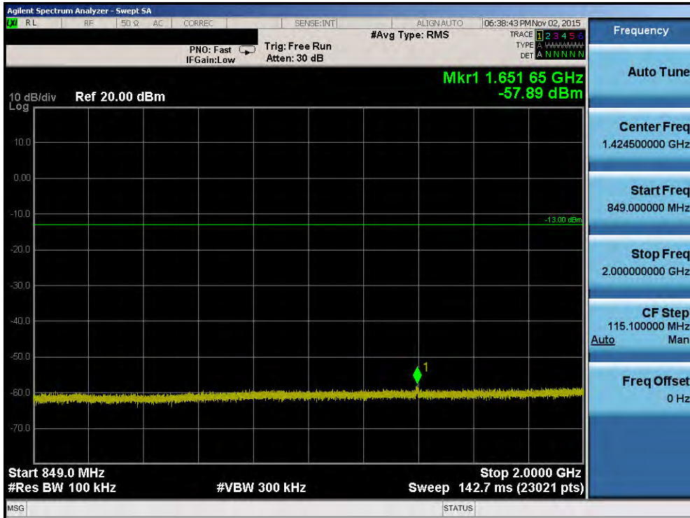
Plot 7-61. Conducted Spurious Plot (Band 5/26 – 3.0MHz QPSK – RB Size 1, RB Offset 0 – Low Channel)
