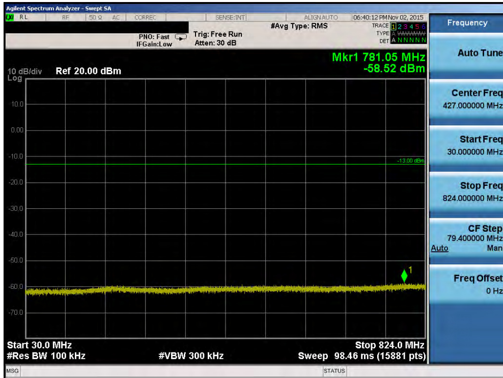
Plot 7-66. Conducted Spurious Plot (Band 5/26 – 3.0MHz QPSK – RB Size 1, RB Offset 0 – High Channel)
