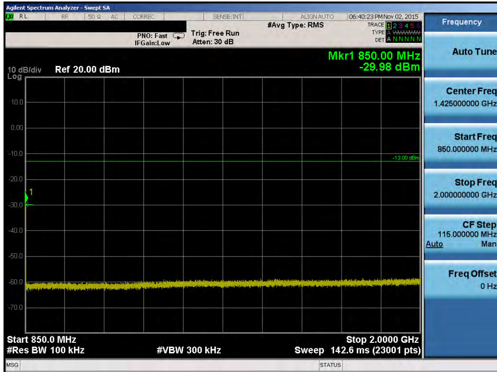
Plot 7-67. Conducted Spurious Plot (Band 5/26 – 3.0MHz QPSK – RB Size 1, RB Offset 0 – High Channel)
