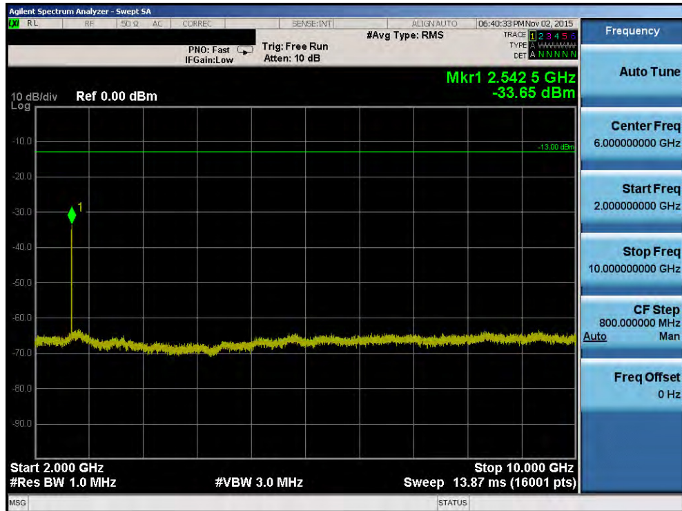
Plot 7-68. Conducted Spurious Plot (Band 5/26 – 3.0MHz QPSK – RB Size 1, RB Offset 0 – High Channel)
