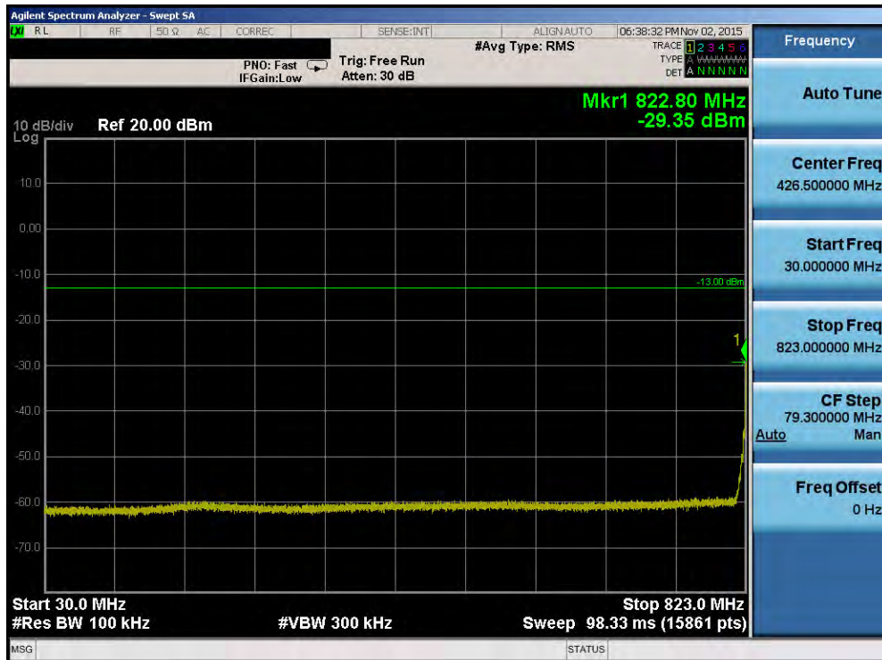
Plot 7-60. Conducted Spurious Plot (Band 5/26 – 3.0MHz QPSK – RB Size 1, RB Offset 0– Low Channel)
