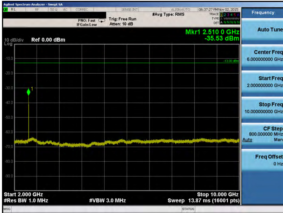
Plot 7-65. Conducted Spurious Plot (Band 5/26 – 3.0MHz QPSK – RB Size 1, RB Offset 0 – Mid Channel)
