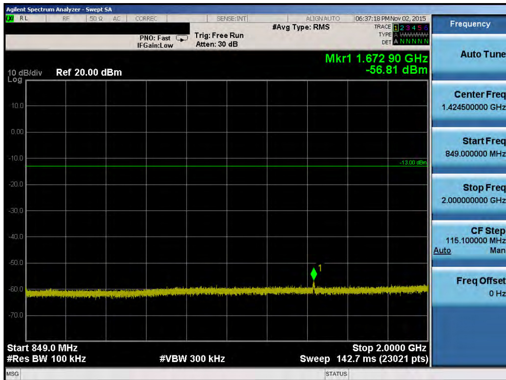
Plot 7-64. Conducted Spurious Plot (Band 5/26 – 3.0MHz QPSK – RB Size 1, RB Offset 0 – Mid Channel)
