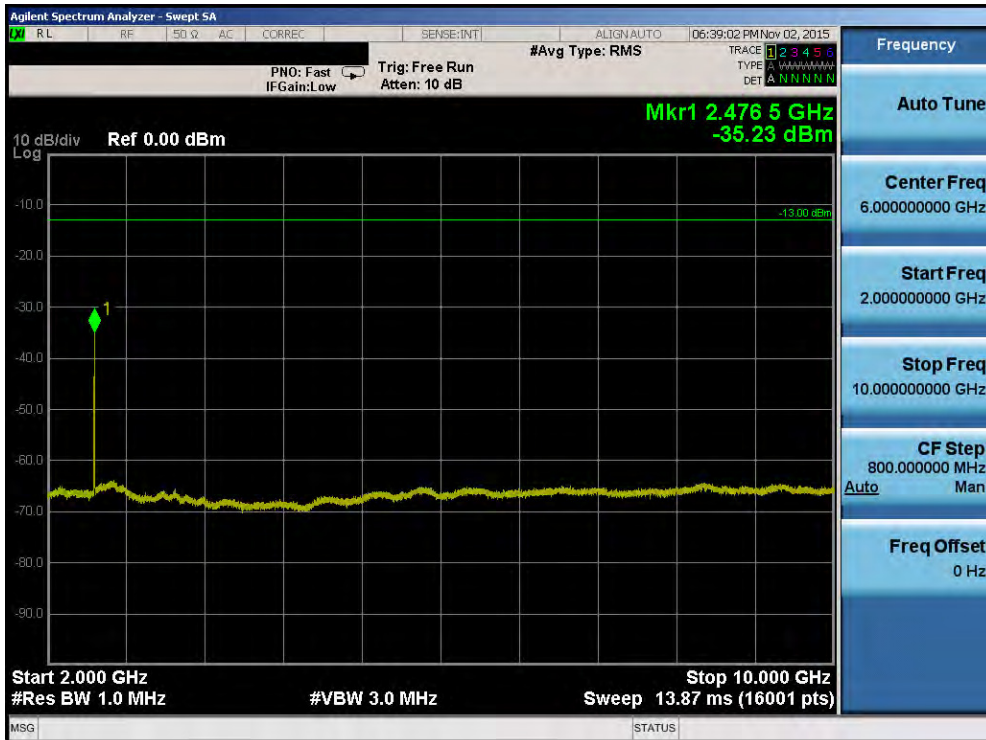
Plot 7-62. Conducted Spurious Plot (Band 5/26 – 3.0MHz QPSK – RB Size 1, RB Offset 0 – Low Channel)
