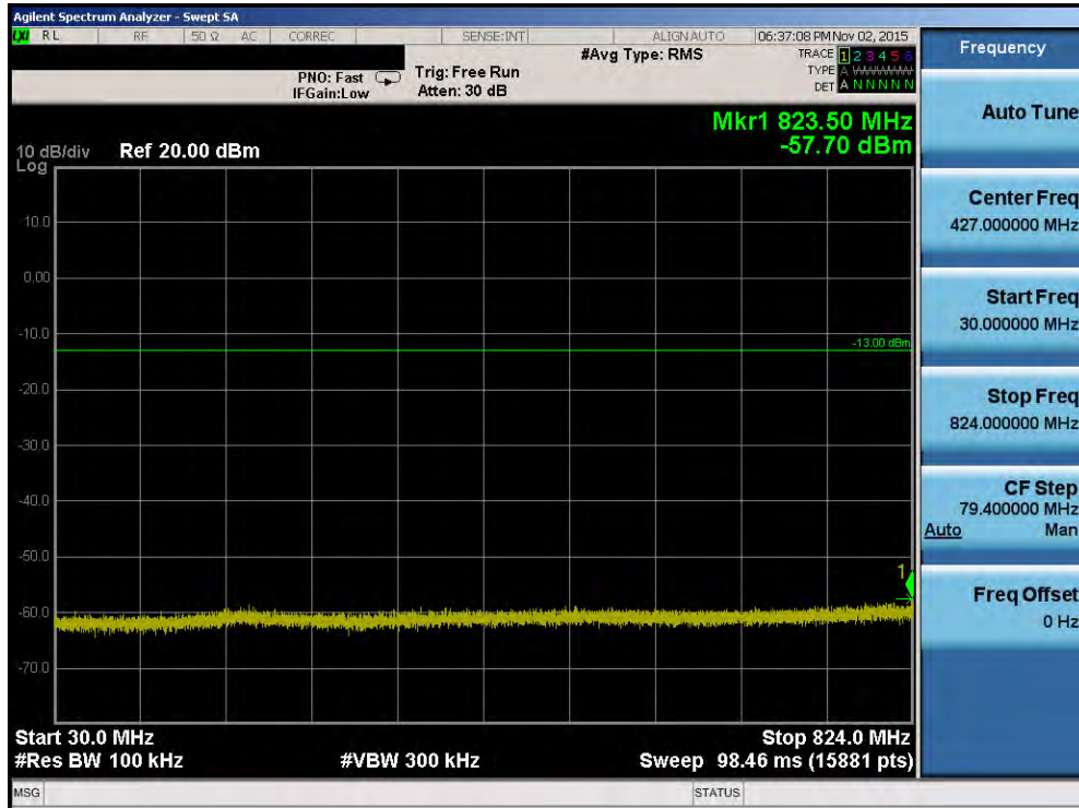
Plot 7-63. Conducted Spurious Plot (Band 5/26 –3.0MHz QPSK – RB Size 1, RB Offset 0 – Mid Channel)
