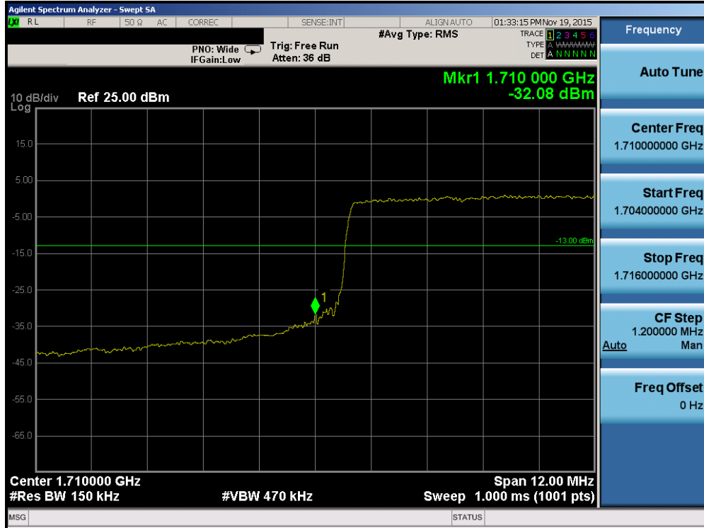
Plot 7-115. Lower Band Edge Plot (Band 4 – 15.0MHz QPSK – RB Size 75)
