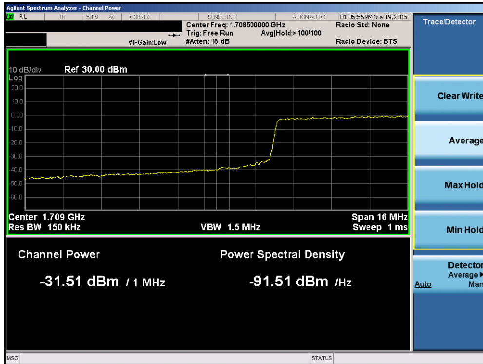
Plot 7-120. Lower Extended Band Edge Plot (Band 4 – 20.0MHz QPSK – RB Size 100)
