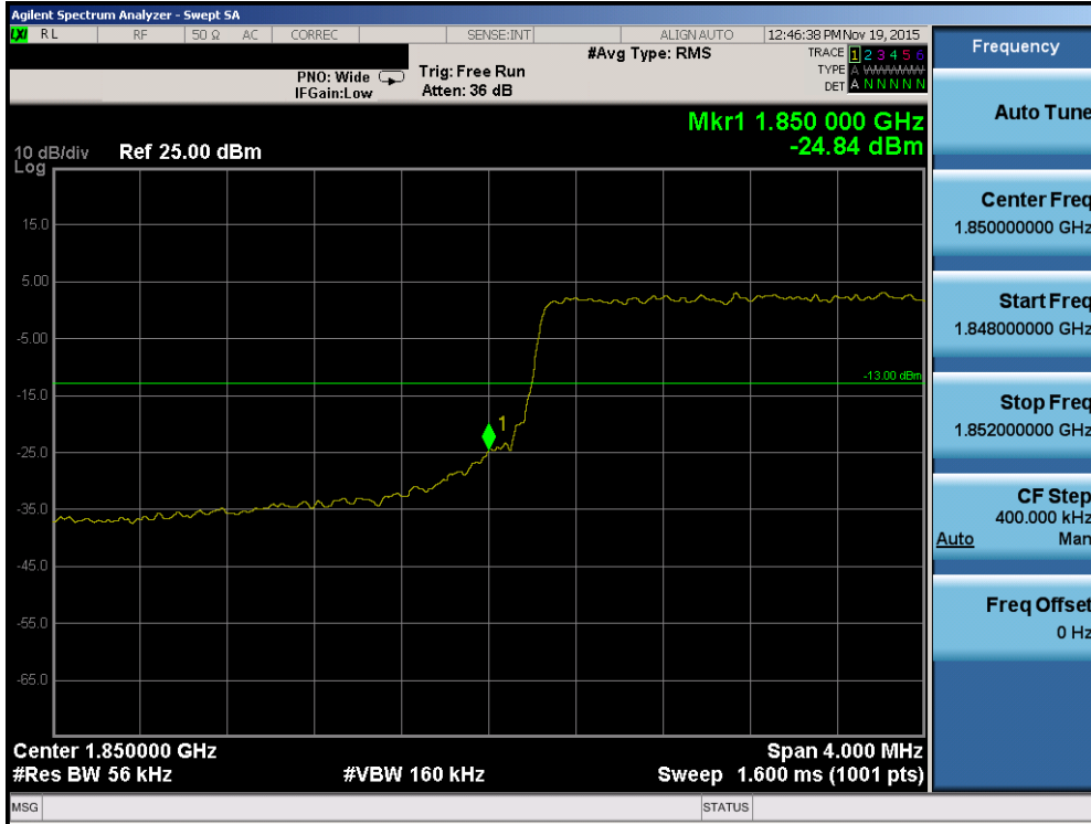
Plot 7-131. Lower Band Edge Plot (Band 2 – 5.0MHz QPSK – RB Size 25)
