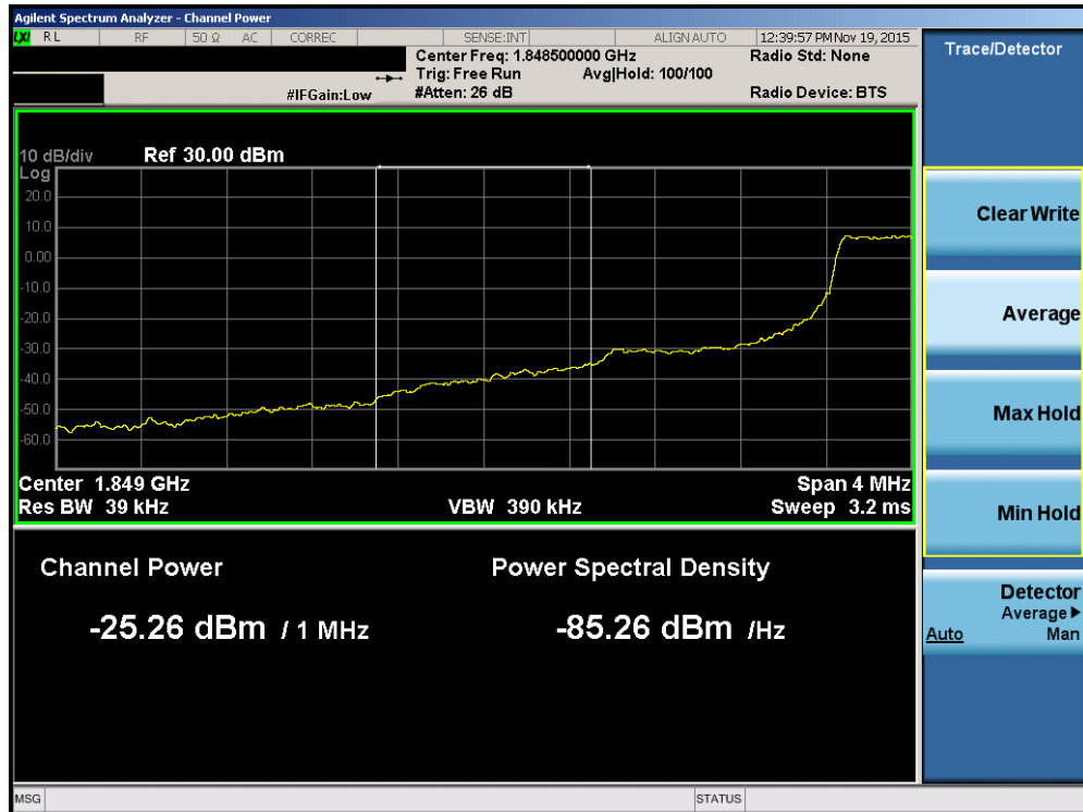
Plot 7-124. Lower Extended Band Edge Plot (Band 2 – 1.4MHz QPSK – RB Size 6)
