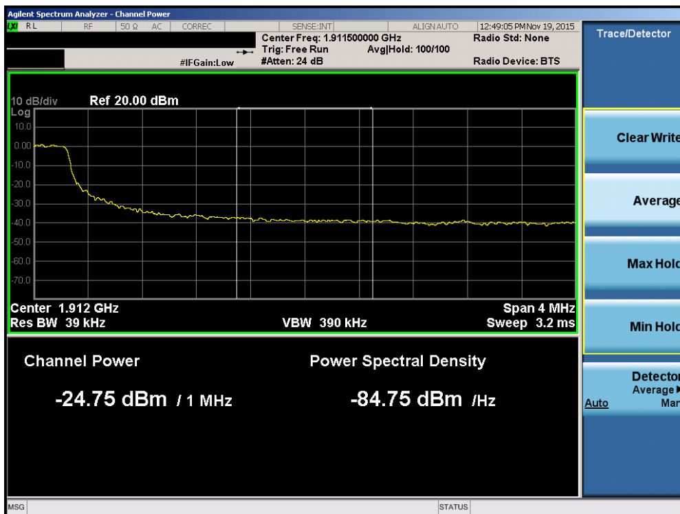
Plot 7-134. Upper Extended Band Edge Plot (Band 2 – 5.0MHz QPSK – RB Size 25)
