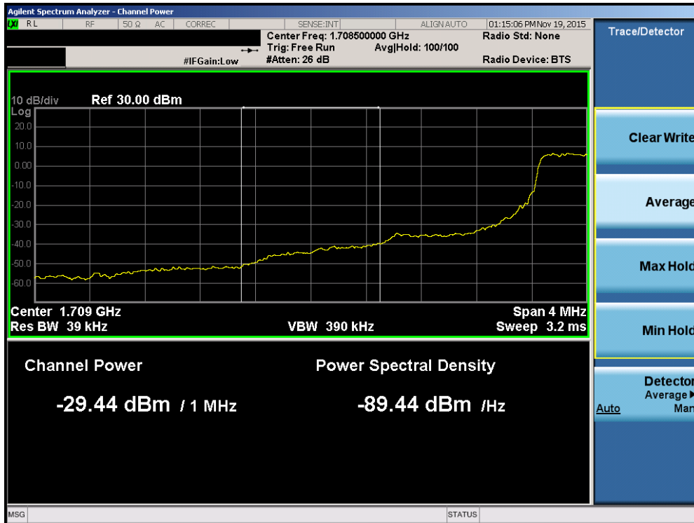
Plot 7-100. Lower Extended Band Edge Plot (Band 4 – 1.4MHz QPSK – RB Size 6)
