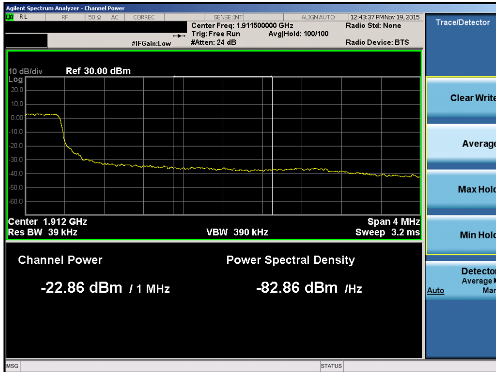
Plot 7-130. Upper Extended Band Edge Plot (Band 2 – 3.0MHz QPSK – RB Size 15)
