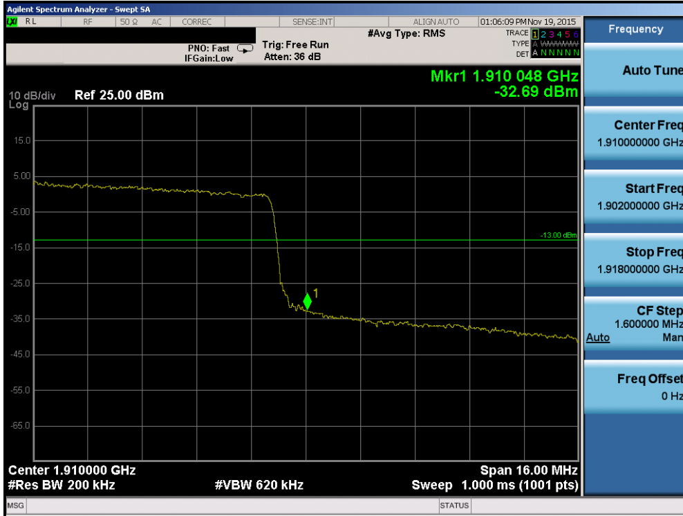
Plot 7-145. Upper Band Edge Plot (Band 2 – 20.0MHz QPSK – RB Size 100)
