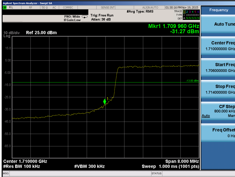
Plot 7-111. Lower Band Edge Plot (Band 4 – 10.0MHz QPSK – RB Size 50)
