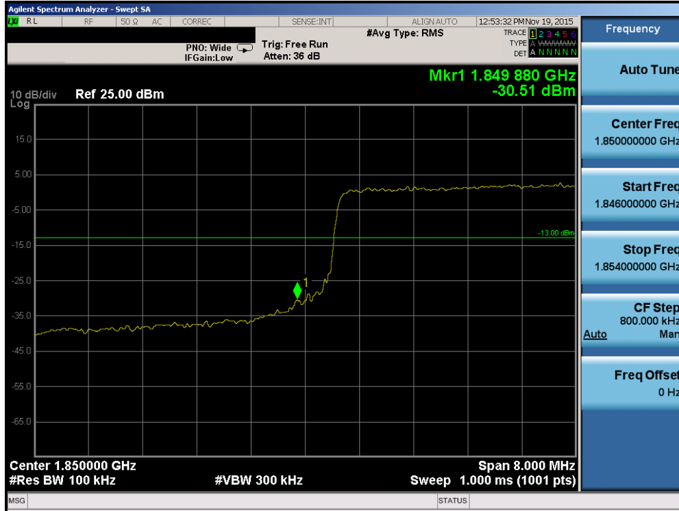
Plot 7-135. Lower Band Edge Plot (Band 2 – 10.0MHz QPSK – RB Size 50)
