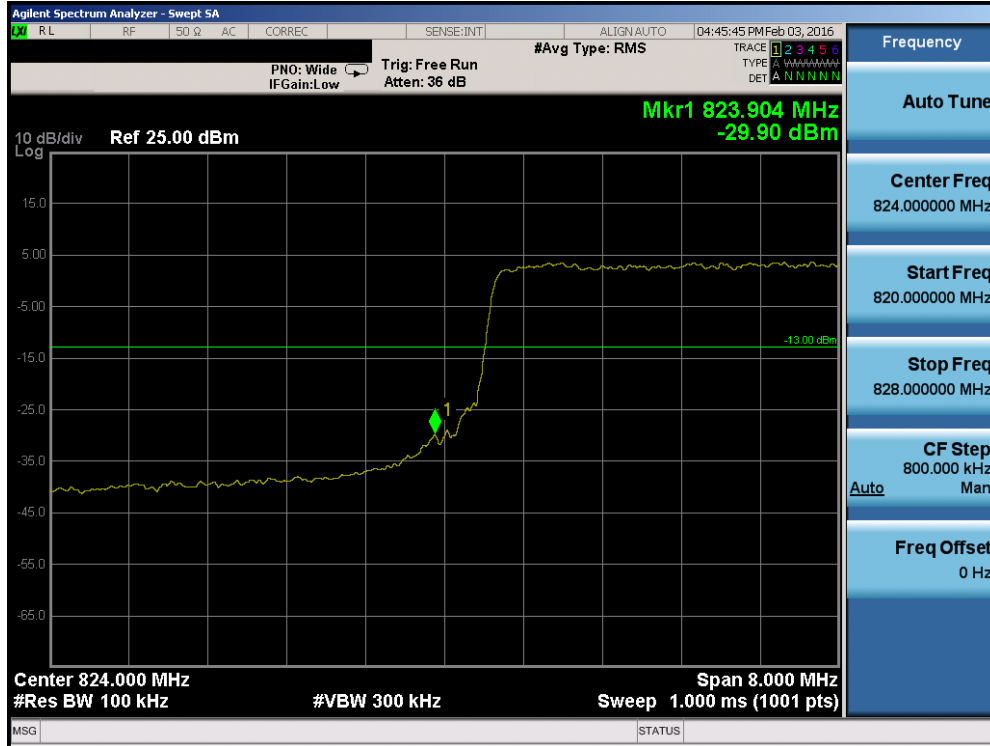
Plot 7-97. Lower Band Edge Plot (Band 5 – 10.0MHz QPSK – RB Size 50)
