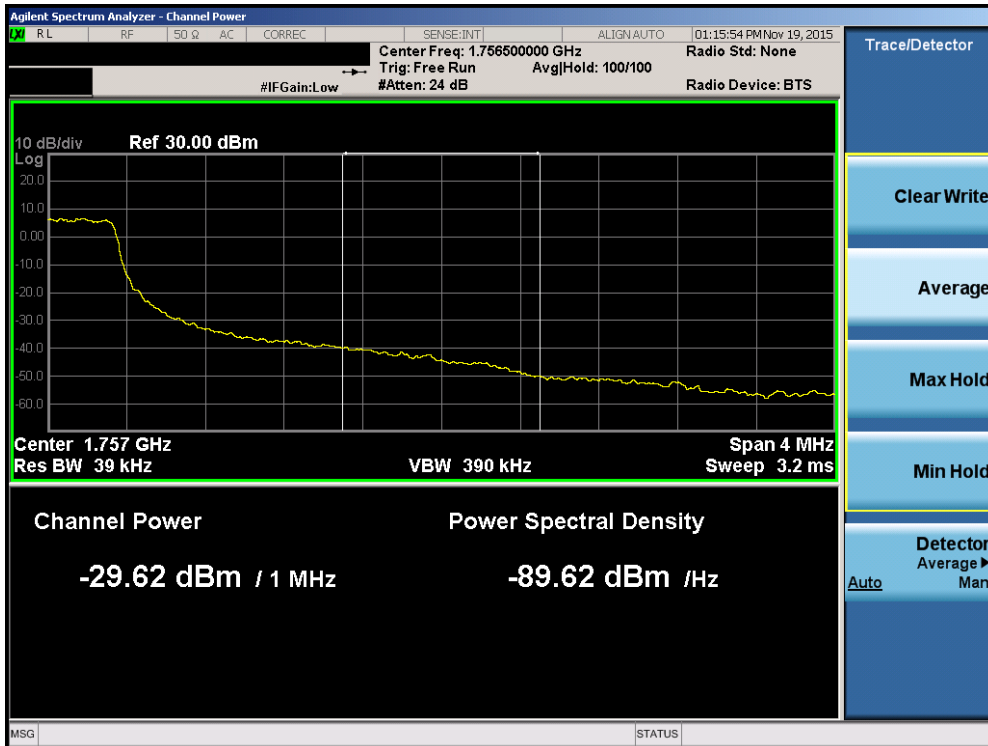
Plot 7-102. Upper Extended Band Edge Plot (Band 4 – 1.4MHz QPSK – RB Size 6)
