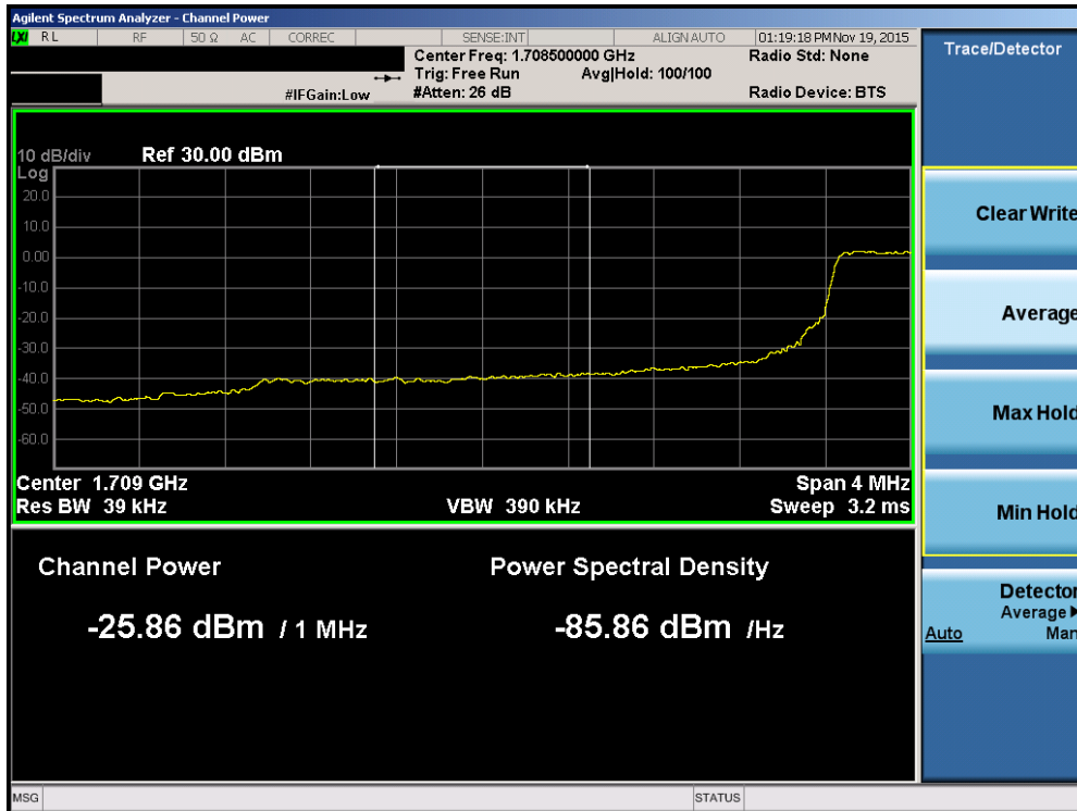
Plot 7-104. Lower Extended Band Edge Plot (Band 4 – 3.0MHz QPSK – RB Size 15)
