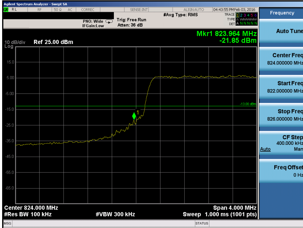
Plot 7-95. Lower Band Edge Plot (Band 5 – 5.0MHz QPSK – RB Size 25)
