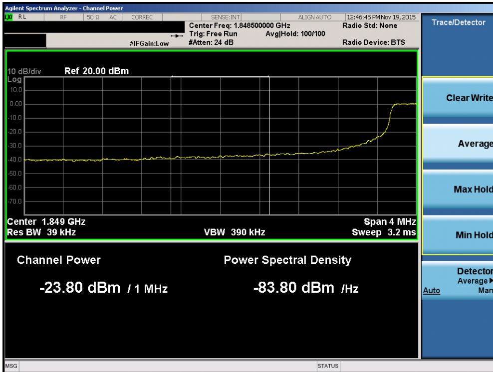
Plot 7-132. Lower Extended Band Edge Plot (Band 2 – 5.0MHz QPSK – RB Size 25)
