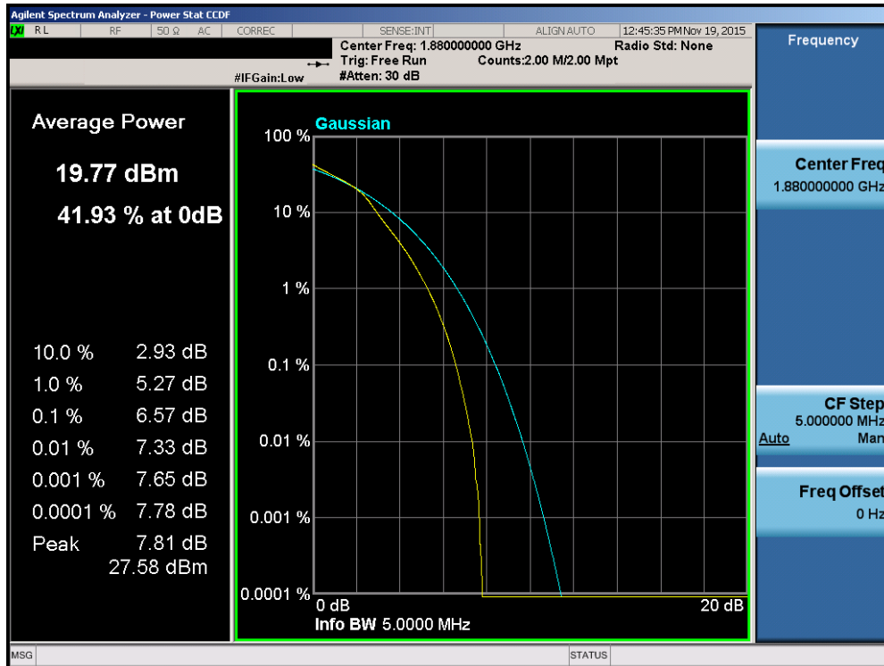
Plot 7-152. PAR Plot (Band 2 – 5.0MHz 16-QAM – RB Size 25)
