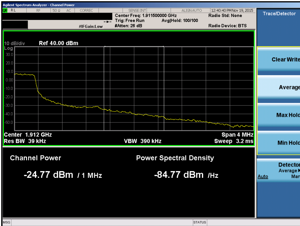
Plot 7-126. Upper Extended Band Edge Plot (Band 2 – 1.4MHz QPSK – RB Size 6)
