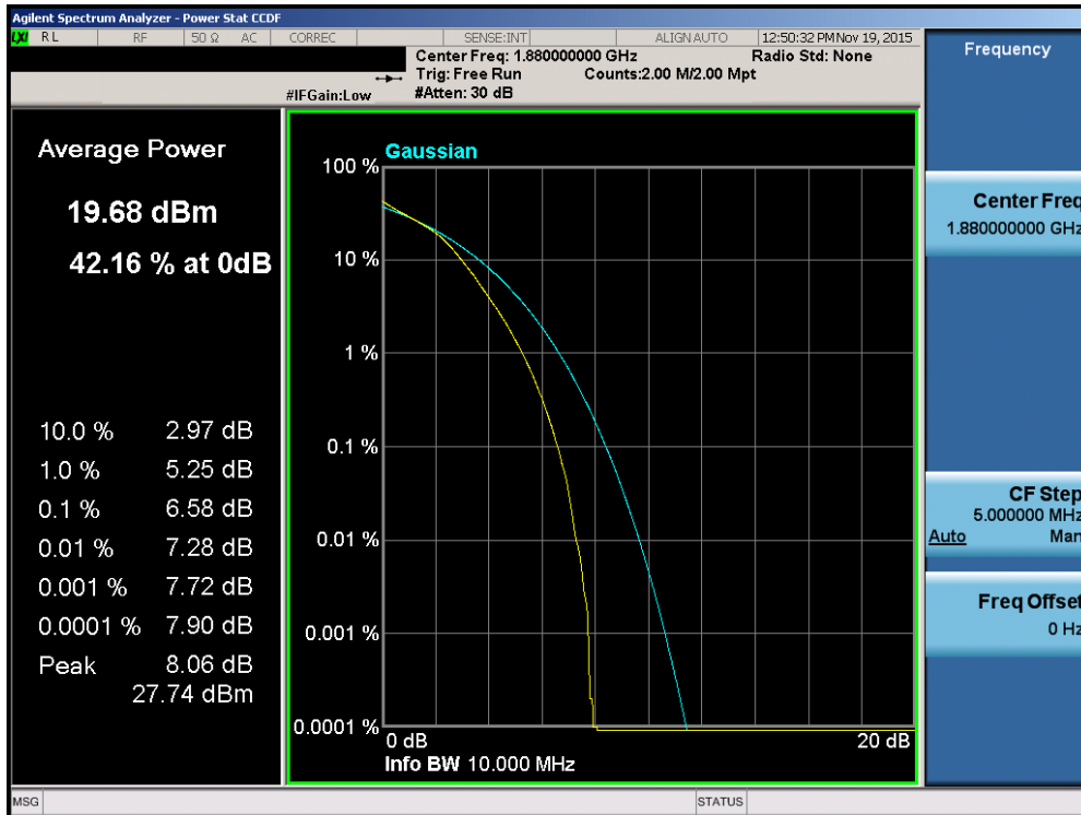
Plot 7-154. PAR Plot (Band 2 – 10.0MHz 16-QAM – RB Size 50)
