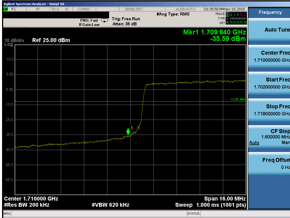
Plot 7-119. Lower Band Edge Plot (Band 4 – 20.0MHz QPSK – RB Size 100)
