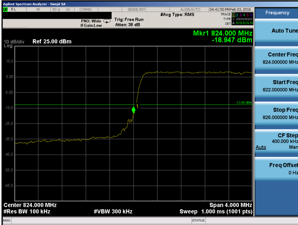
Plot 7-93. Lower Band Edge Plot (Band 5 – 3.0MHz QPSK – RB Size 15)
