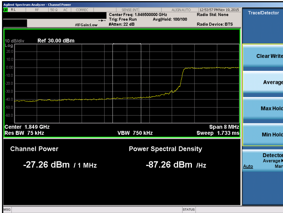
Plot 7-136. Lower Extended Band Edge Plot (Band 2 – 10.0MHz QPSK – RB Size 50)
