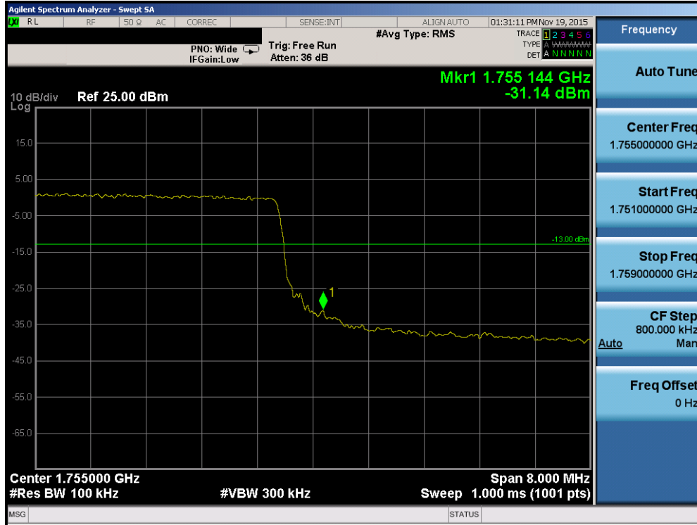
Plot 7-113. Upper Band Edge Plot (Band 4 – 10.0MHz QPSK – RB Size 50)
