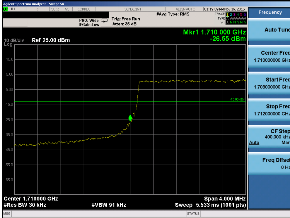
Plot 7-103. Lower Band Edge Plot (Band 4 – 3.0MHz QPSK – RB Size 15)
