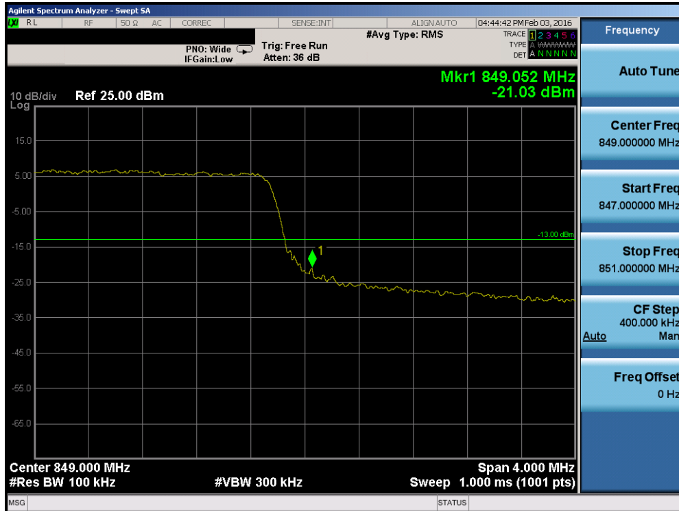
Plot 7-96. Upper Band Edge Plot (Band 5 – 5.0MHz QPSK – RB Size 25)
