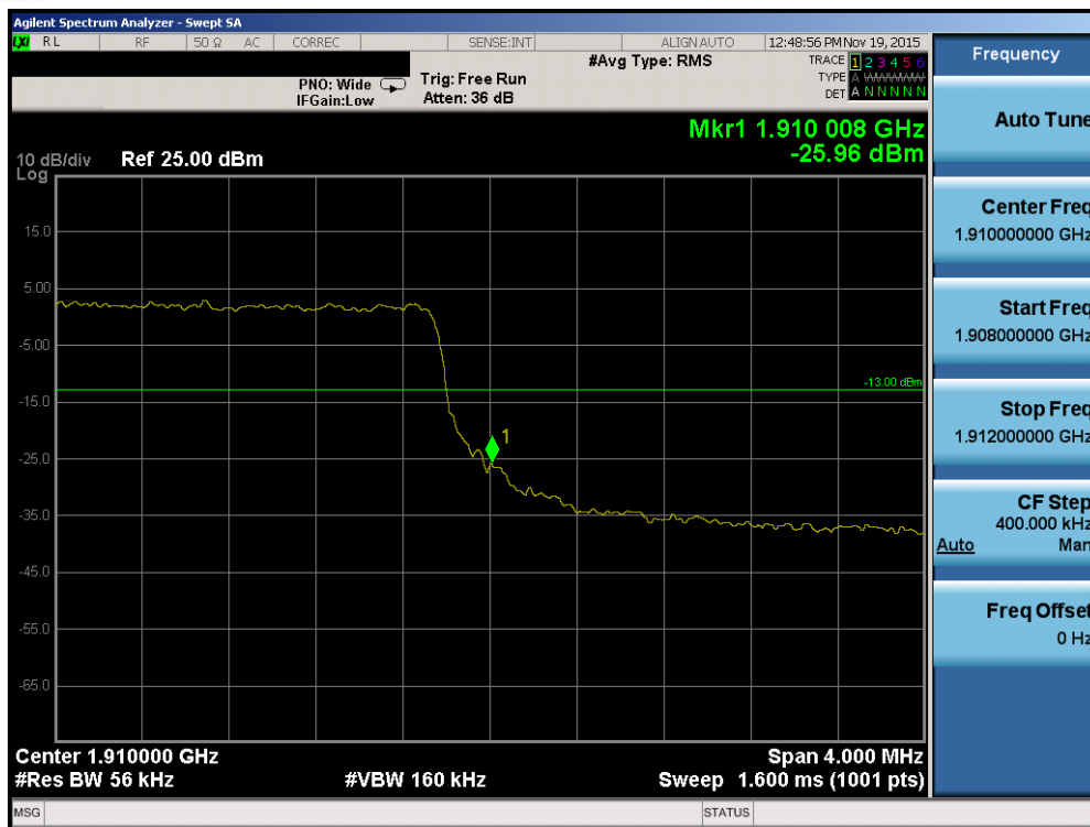
Plot 7-133. Upper Band Edge Plot (Band 2 – 5.0MHz QPSK – RB Size 25)
