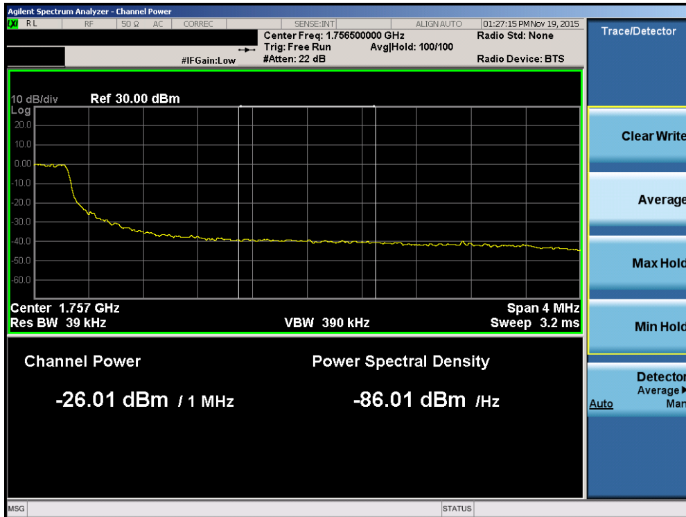
Plot 7-110. Upper Extended Band Edge Plot (Band 4 – 5.0MHz QPSK – RB Size 25)
