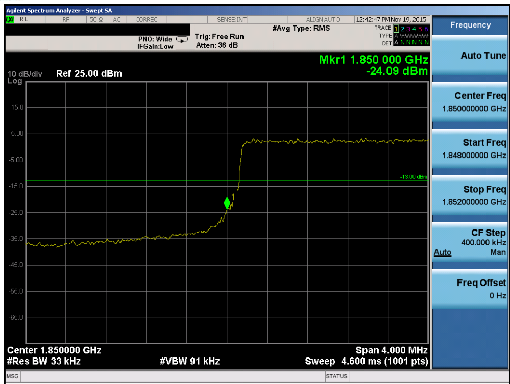
Plot 7-127. Lower Band Edge Plot (Band 2 – 3.0MHz QPSK – RB Size 15)
