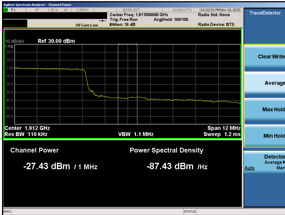
Plot 7-142. Upper Extended Band Edge Plot (Band 2 – 15.0MHz QPSK – RB Size 75)
