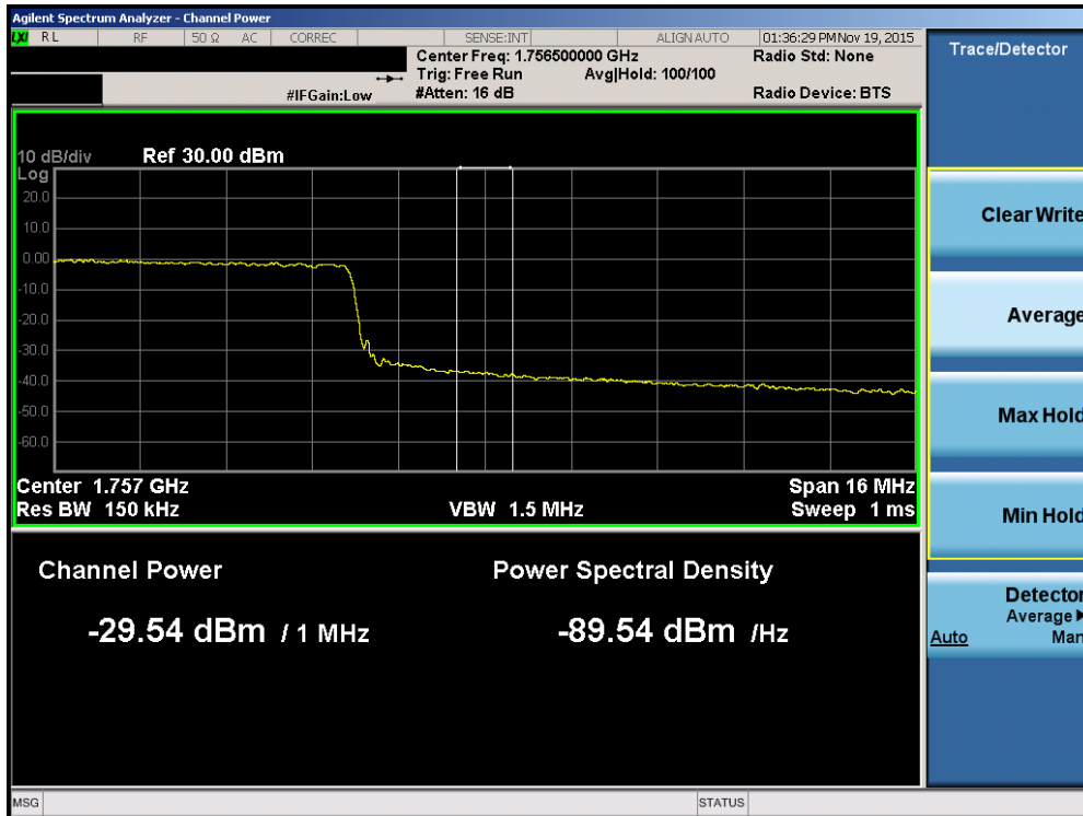
Plot 7-122. Upper Extended Band Edge Plot (Band 4 – 20.0MHz QPSK – RB Size 100)
