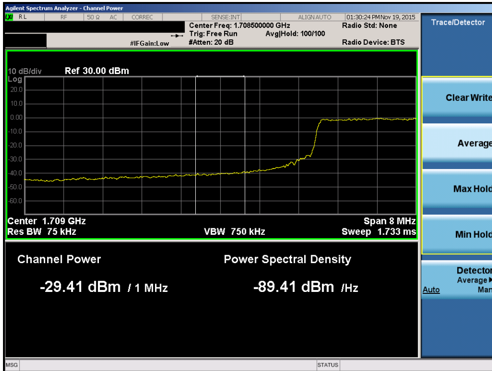
Plot 7-112. Lower Extended Band Edge Plot (Band 4 – 10.0MHz QPSK – RB Size 50)
