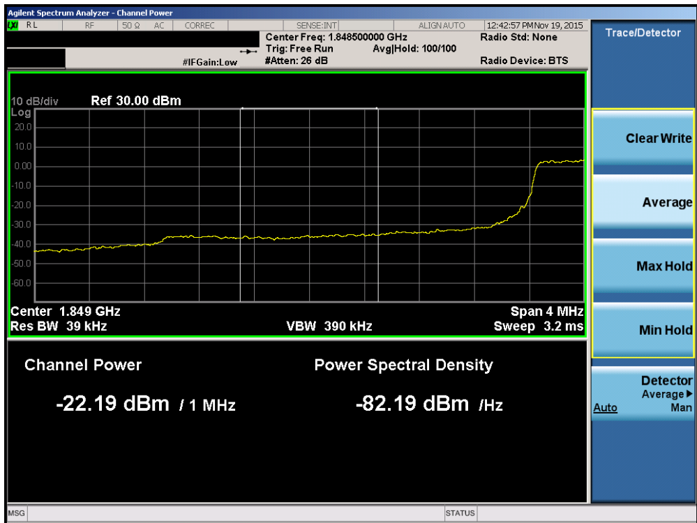
Plot 7-128. Lower Extended Band Edge Plot (Band 2 – 3.0MHz QPSK – RB Size 15)
