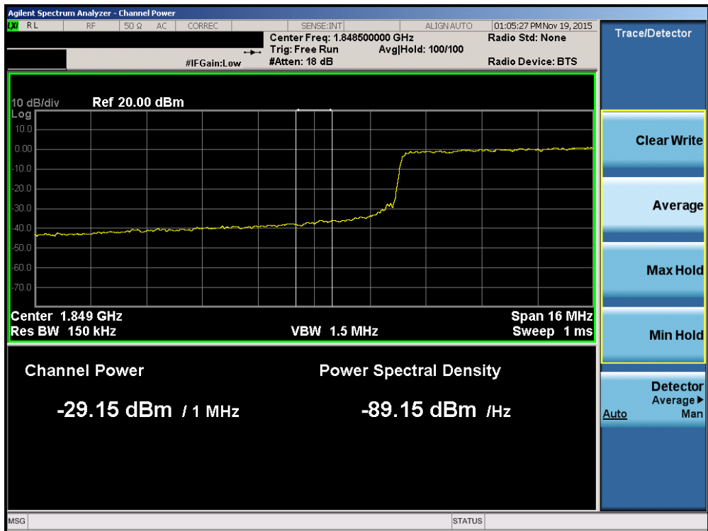
Plot 7-144. Lower Extended Band Edge Plot (Band 2 – 20.0MHz QPSK – RB Size 100)
