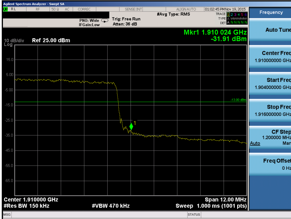
Plot 7-141. Upper Band Edge Plot (Band 2 – 15.0MHz QPSK – RB Size 75)
