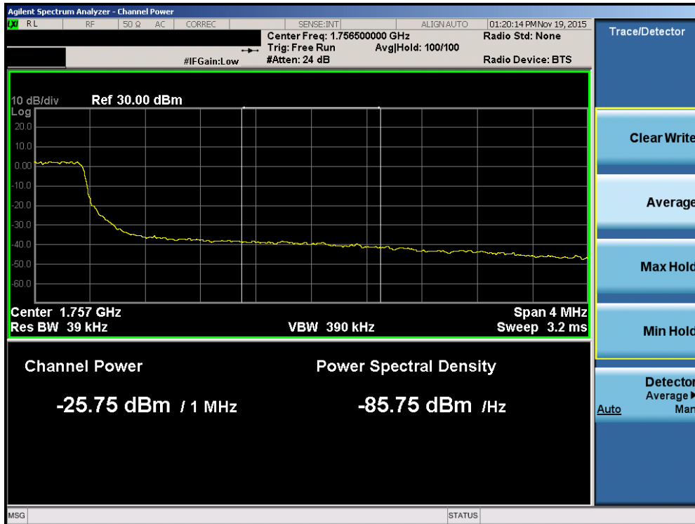
Plot 7-106. Upper Extended Band Edge Plot (Band 4 – 3.0MHz QPSK – RB Size 15)
