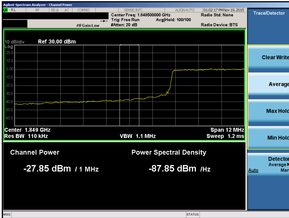
Plot 7-140. Lower Extended Band Edge Plot (Band 2 – 15.0MHz QPSK – RB Size 75)
