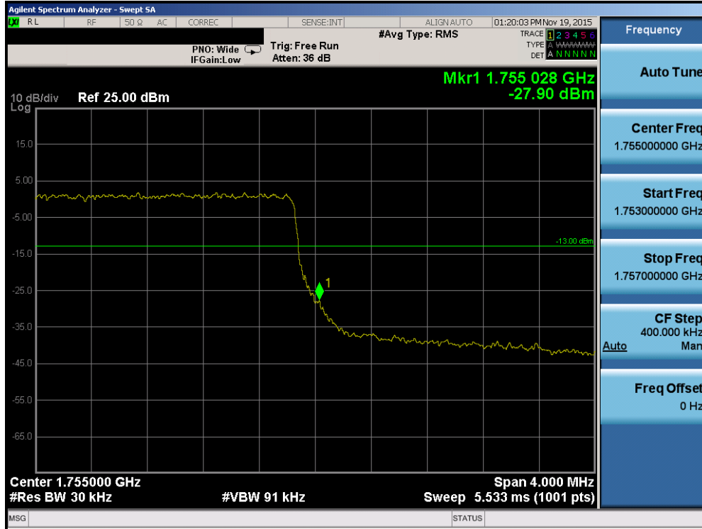
Plot 7-105. Upper Band Edge Plot (Band 4 – 3.0MHz QPSK – RB Size 15)
