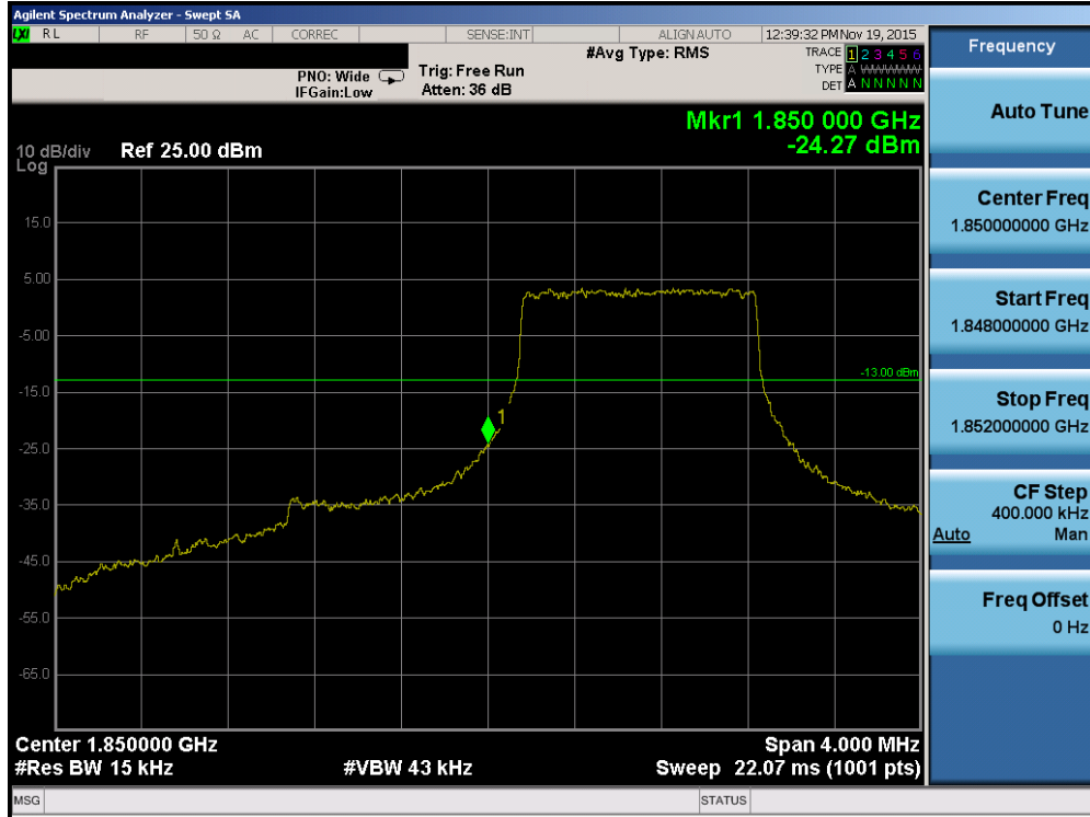
Plot 7-123. Lower Band Edge Plot (Band 2 – 1.4MHz QPSK – RB Size 6)
