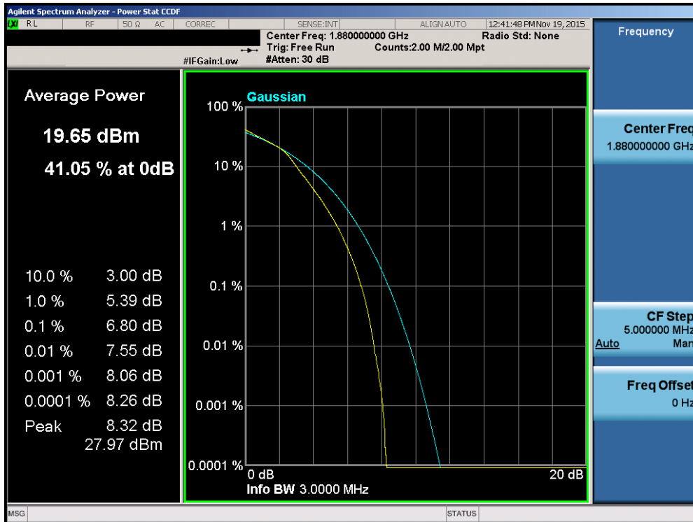
Plot 7-150. PAR Plot (Band 2 – 3.0MHz 16-QAM – RB Size 15)
