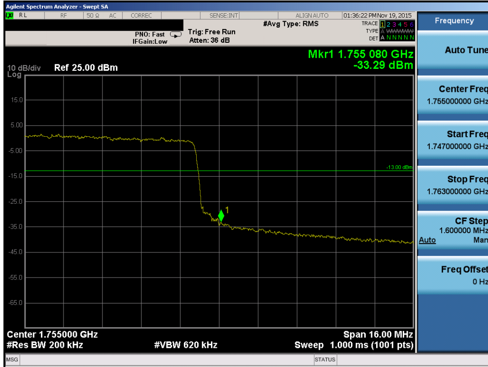
Plot 7-121. Upper Band Edge Plot (Band 4 – 20.0MHz QPSK – RB Size 100)
