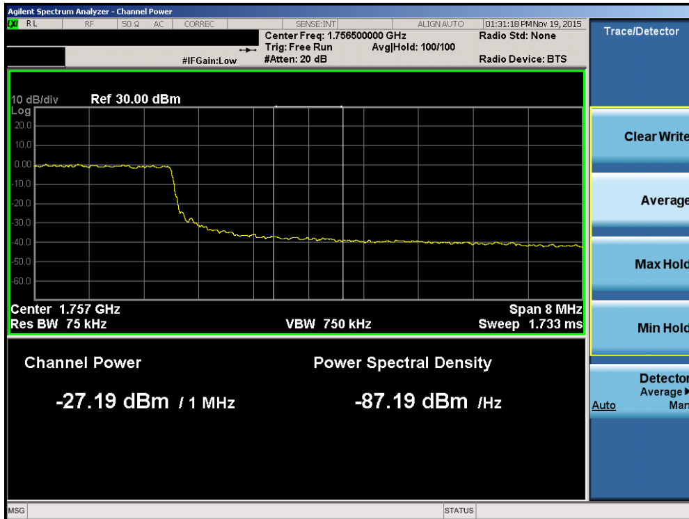
Plot 7-114. Upper Extended Band Edge Plot (Band 4 – 10.0MHz QPSK – RB Size 50)
