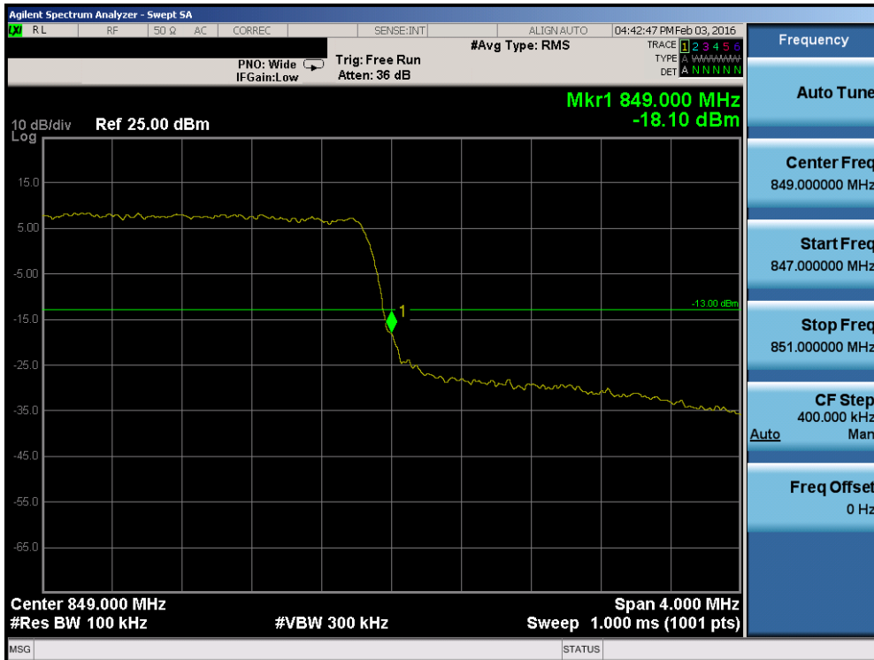
Plot 7-94. Upper Band Edge Plot (Band 5 – 3.0MHz QPSK – RB Size 15)
