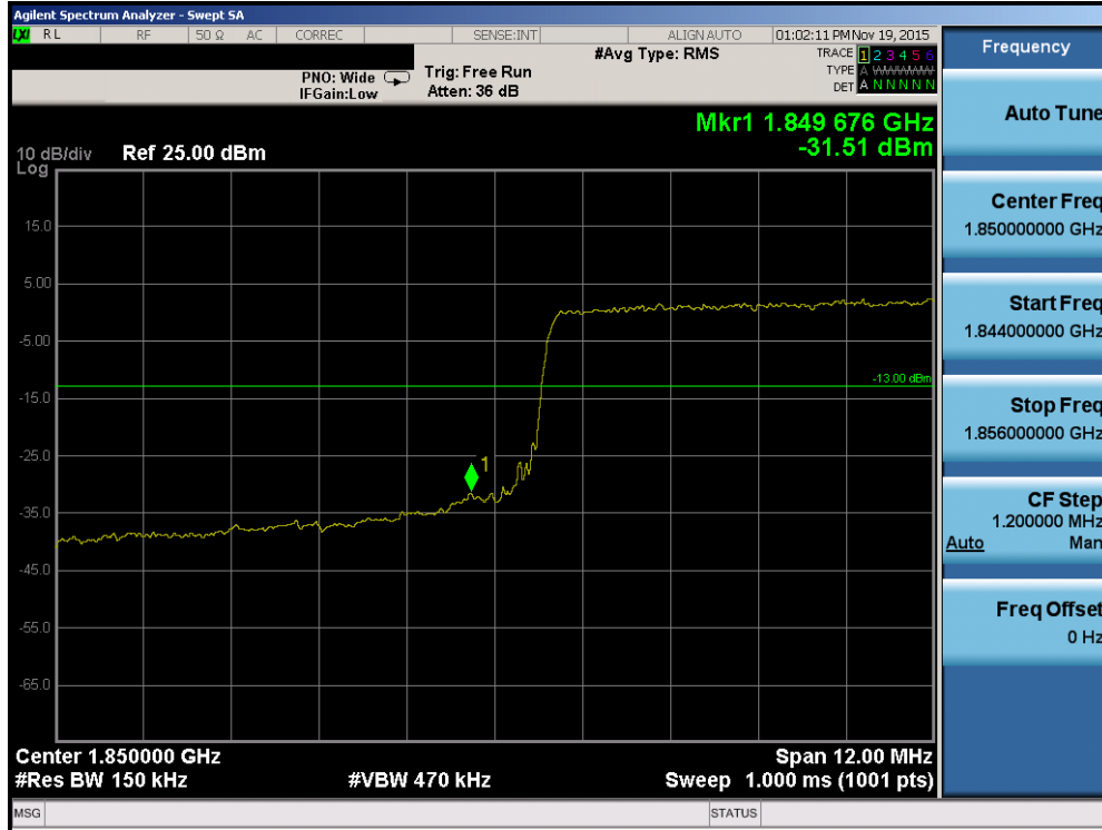
Plot 7-139. Lower Band Edge Plot (Band 2 – 15.0MHz QPSK – RB Size 75)
