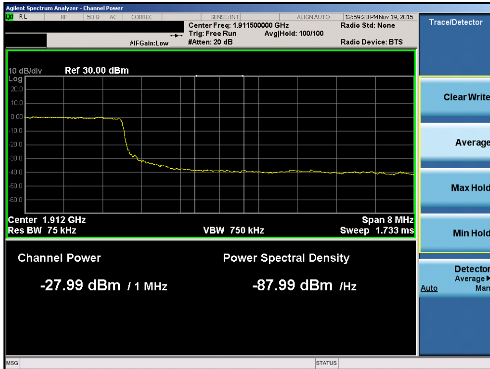
Plot 7-138. Upper Extended Band Edge Plot (Band 2 – 10.0MHz QPSK – RB Size 50)
