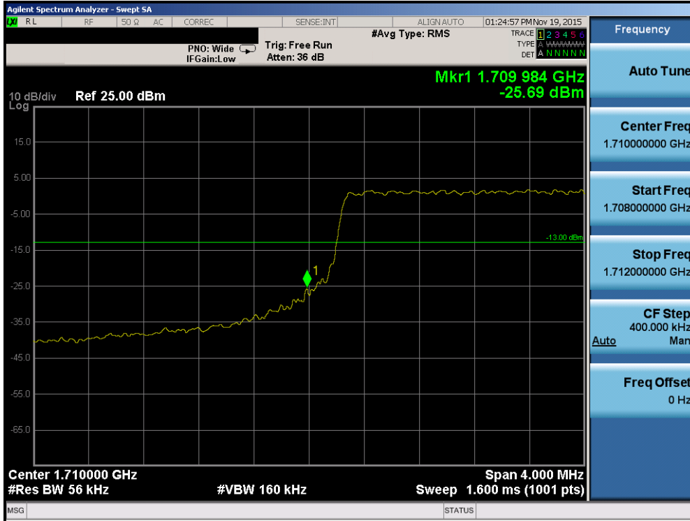
Plot 7-107. Lower Band Edge Plot (Band 4 – 5.0MHz QPSK – RB Size 25)
