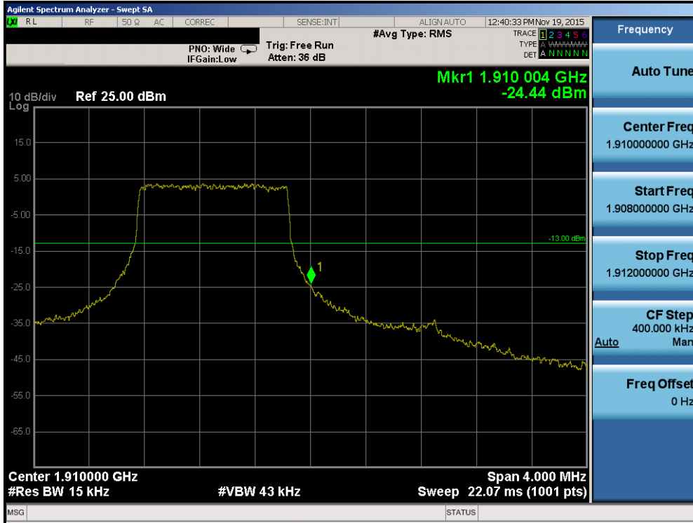
Plot 7-125. Upper Band Edge Plot (Band 2 – 1.4MHz QPSK – RB Size 6)
