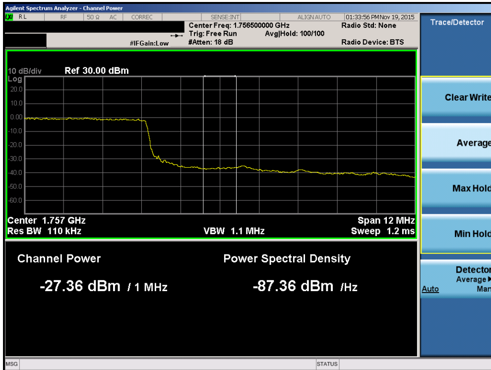
Plot 7-118. Upper Extended Band Edge Plot (Band 4 – 15.0MHz QPSK – RB Size 75)
