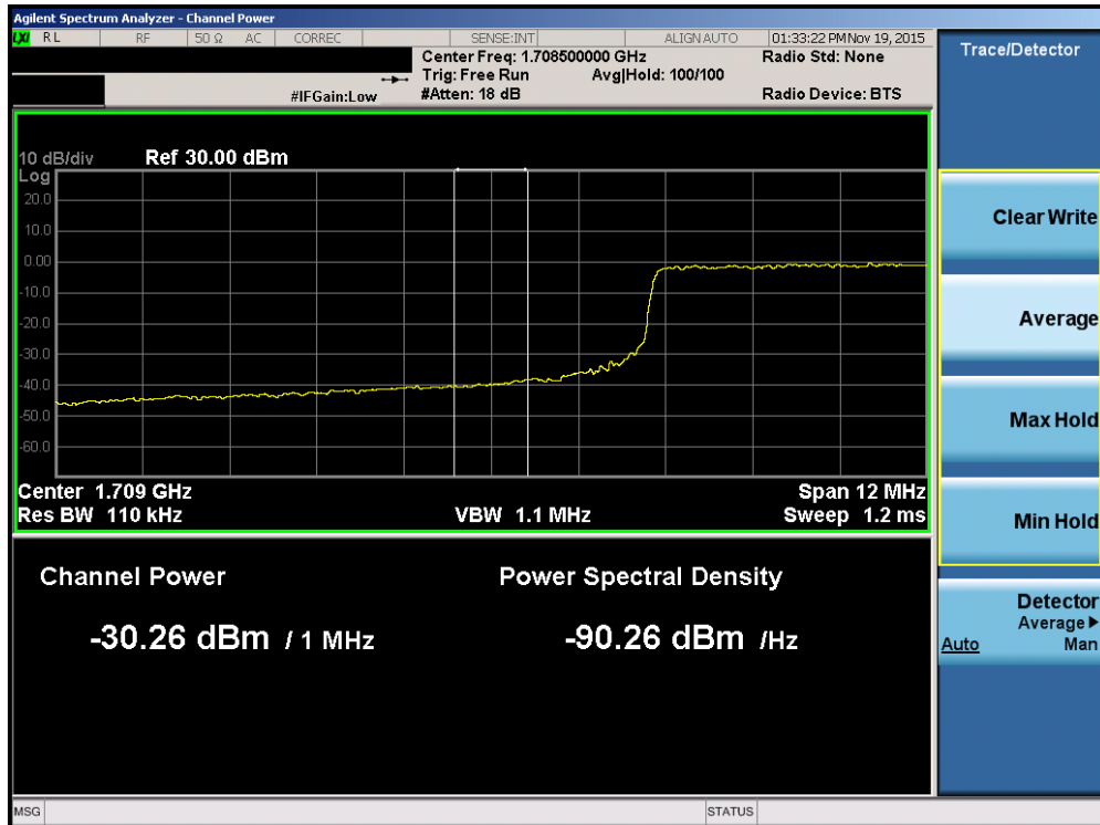
Plot 7-116. Lower Extended Band Edge Plot (Band 4 – 15.0MHz QPSK – RB Size 75)
