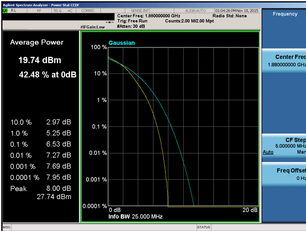
Plot 7-158. PAR Plot (Band 2 – 20.0MHz 16-QAM – RB Size 100)
