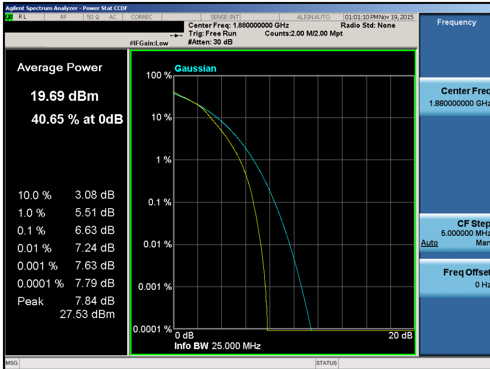
Plot 7-156. PAR Plot (Band 2 – 15.0MHz 16-QAM – RB Size 75)
