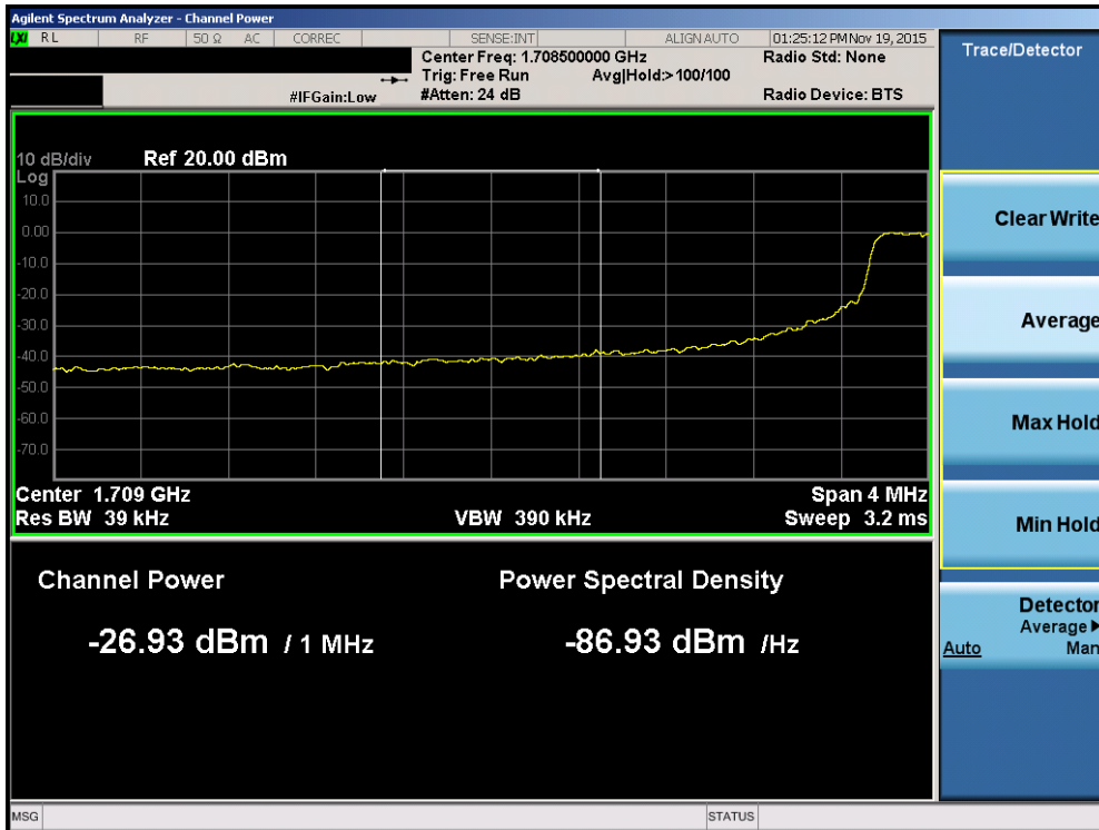
Plot 7-108. Lower Extended Band Edge Plot (Band 4 – 5.0MHz QPSK – RB Size 25)
