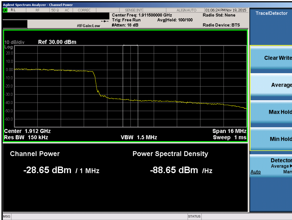
Plot 7-146. Upper Extended Band Edge Plot (Band 2 – 20.0MHz QPSK – RB Size 100)
