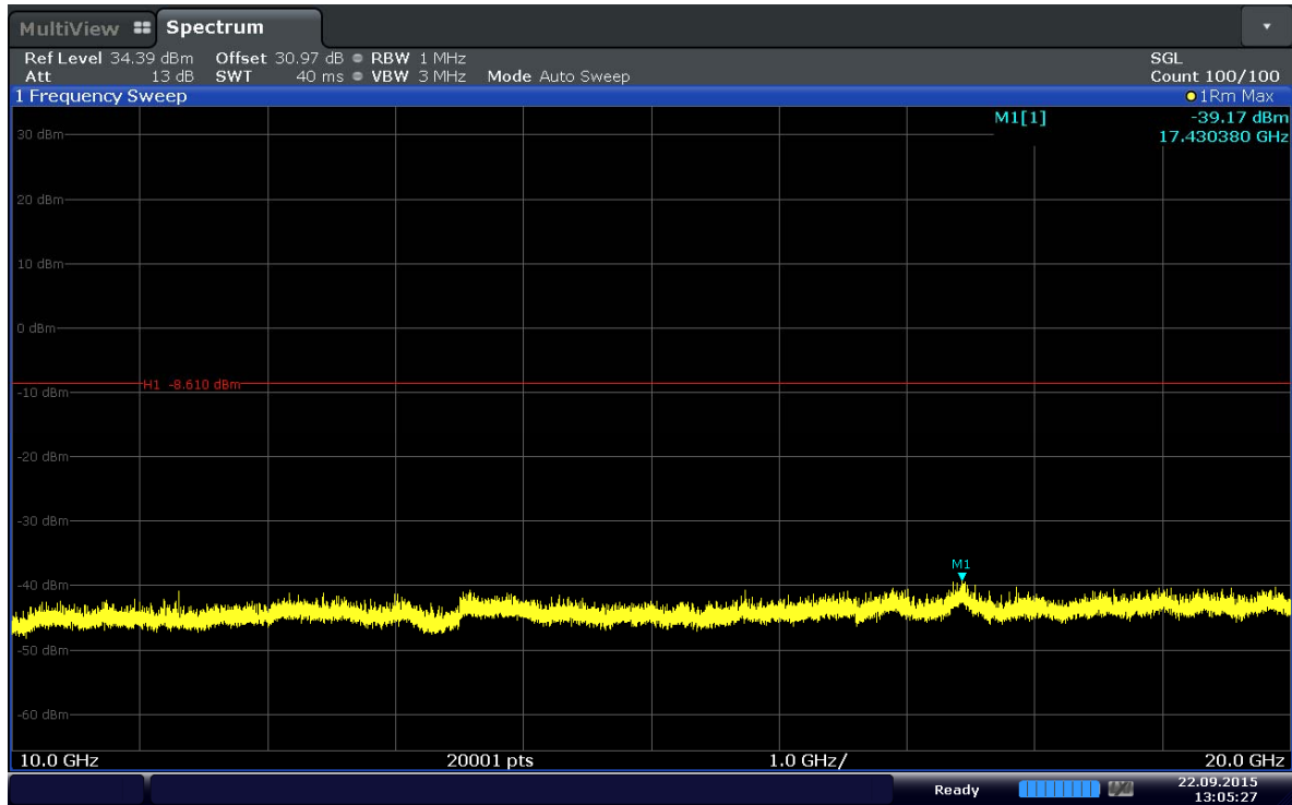
Plot 6-19. Conducted Spurious Plot (Band 41–10MHz–QPSK–RB Size 1–RB Offset 49–Ch.40290)
