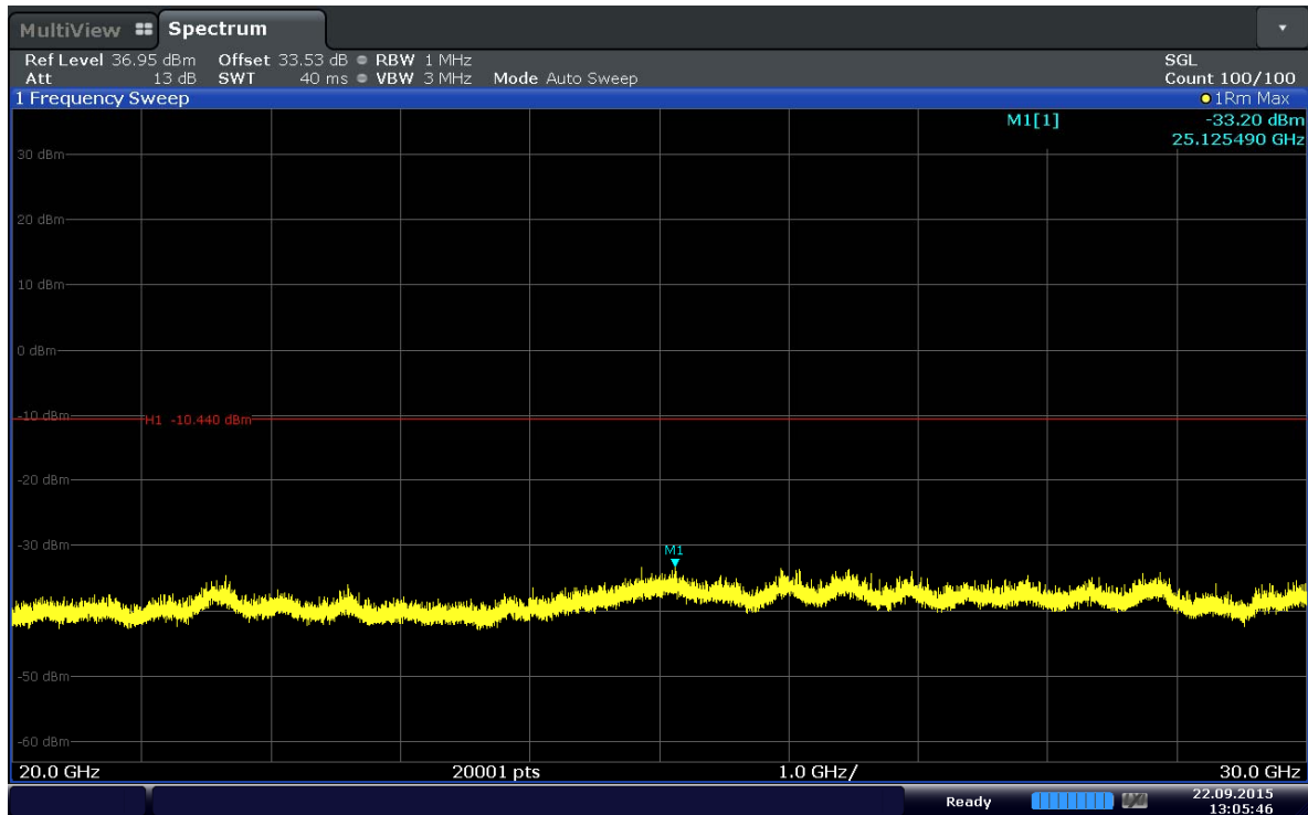
Plot 6-20. Conducted Spurious Plot (Band 41–10MHz–QPSK–RB Size 1–RB Offset 49–Ch.40290)
