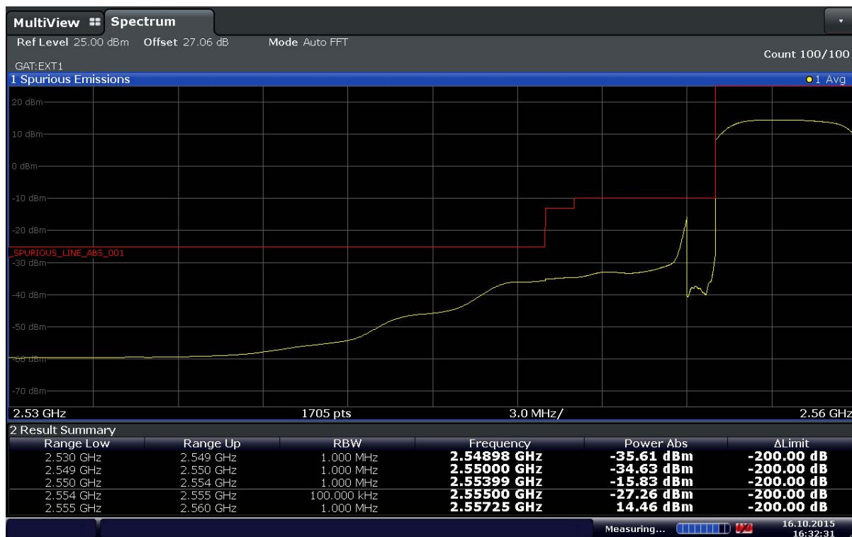
Plot 6-45. Lower Band Edge Plot (Band41 – 5MHz – QPSK – RB Size 25 – Ch.40265)
