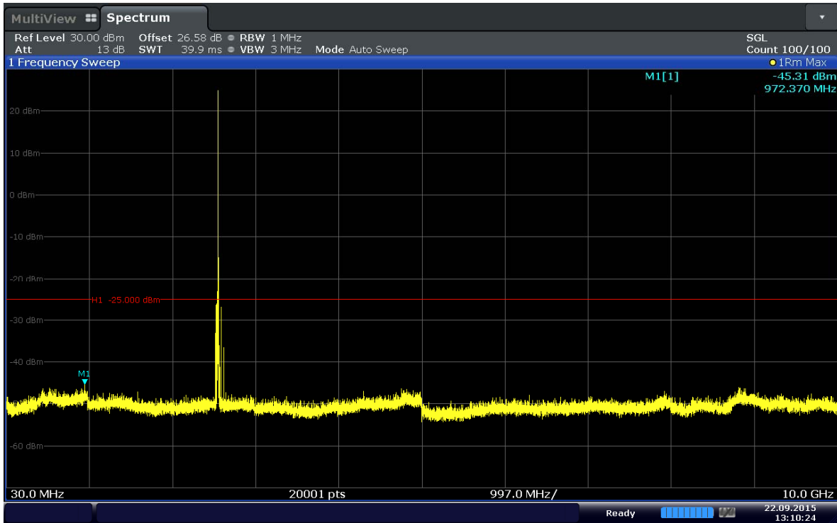
Plot 6-27. Conducted Spurious Plot (Band 41–15MHz–QPSK–RB Size 1–RB Offset 74–Ch.40315)
