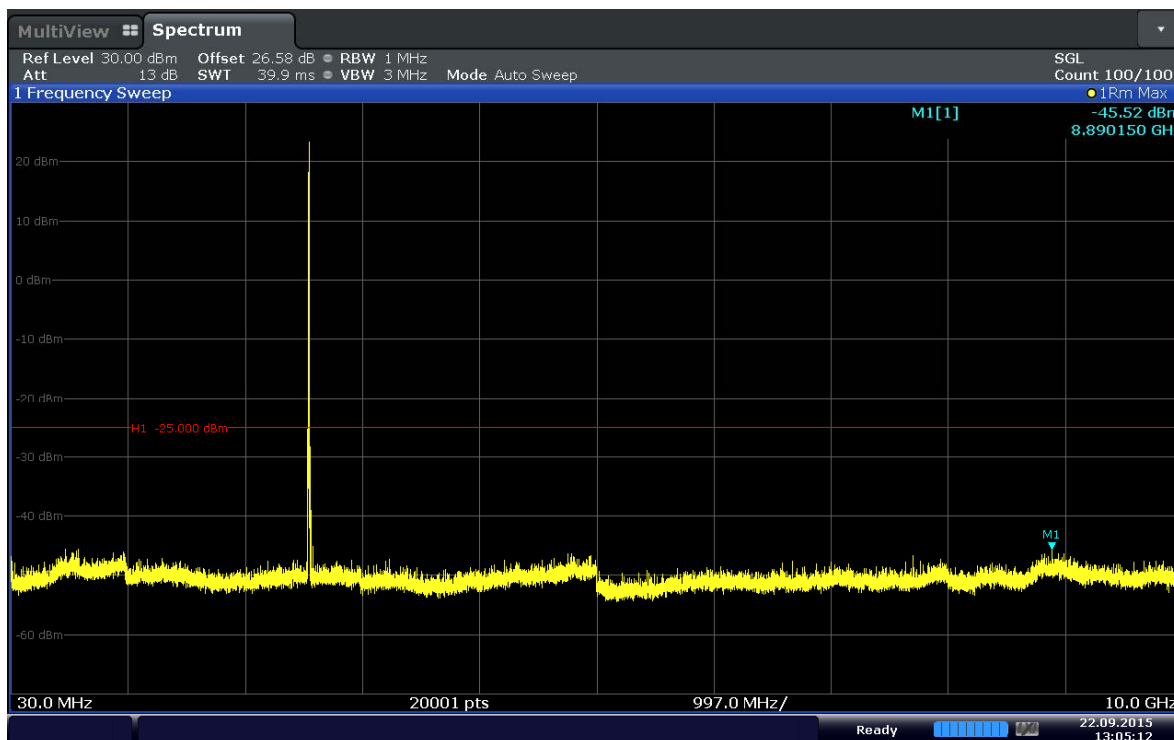
Plot 6-18. Conducted Spurious Plot (Band 41–10MHz–QPSK–RB Size 1–RB Offset 49–Ch.40290)
