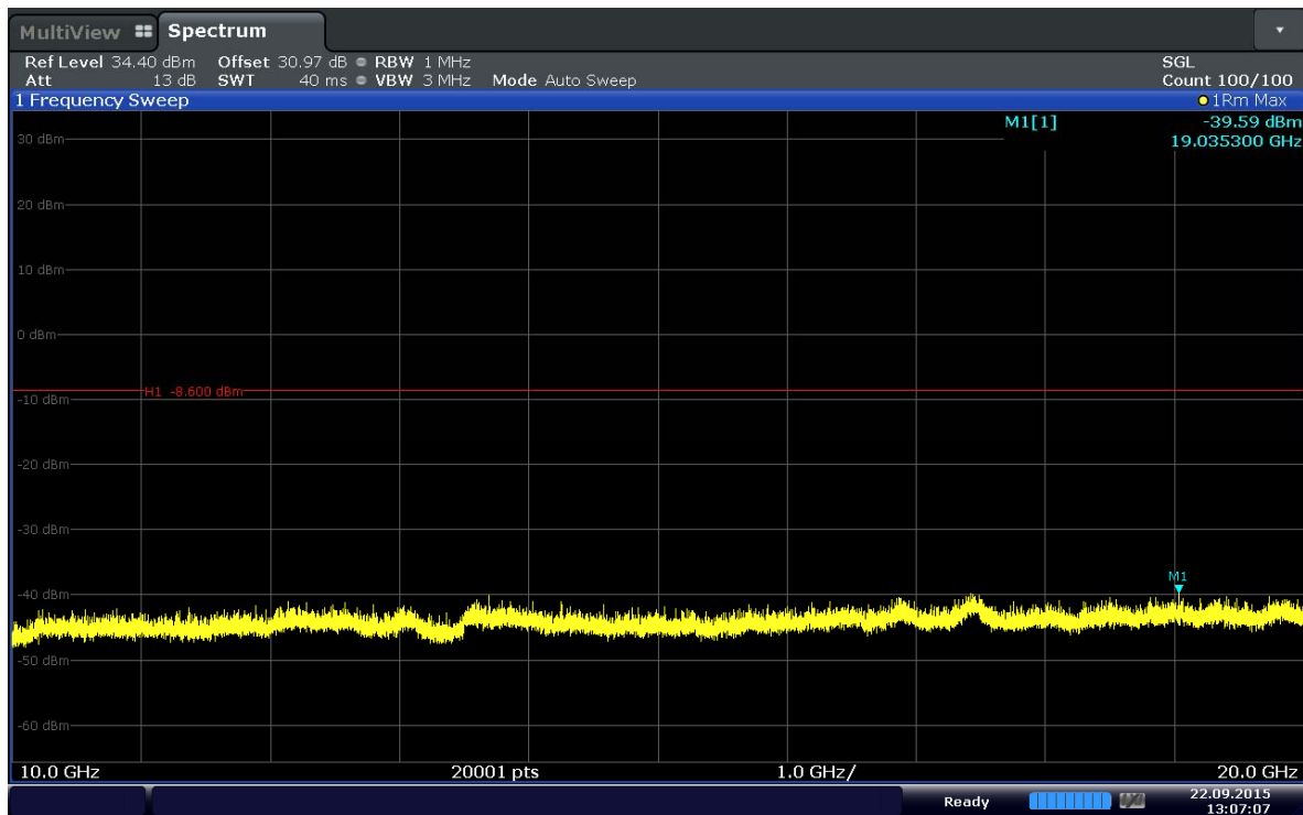
Plot 6-22. Conducted Spurious Plot (Band 41–10MHz–QPSK–RB Size 1–RB Offset 24–Ch.40740)
