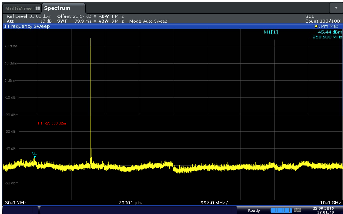
Plot 6-12. Conducted Spurious Plot (Band 41–5MHz–QPSK–RB Size 1–RB Offset 0–Ch.40740)
