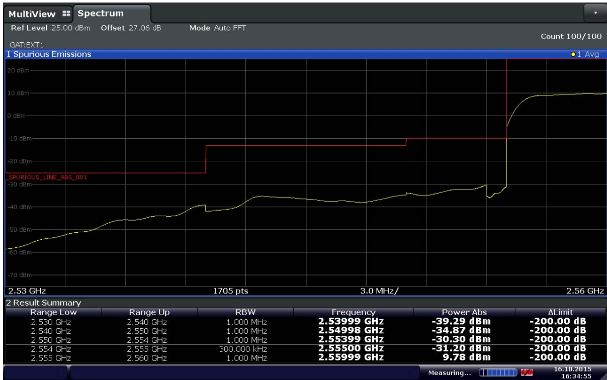
Plot 6-49. Lower Band Edge Plot (Band41 – 15MHz – QPSK – RB Size 75 – Ch.40315)
