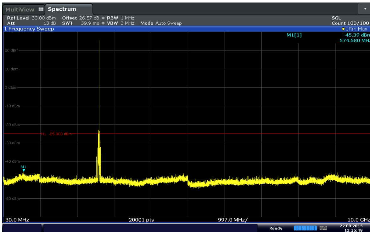
Plot 6-39. Conducted Spurious Plot (Band 41–20MHz–QPSK–RB Size 1–RB Offset 99–Ch.40740)
