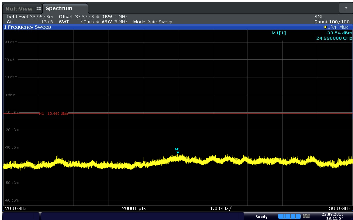
Plot 6-38. Conducted Spurious Plot (Band 41–20MHz–QPSK–RB Size 1–RB Offset 99–Ch.40340)
