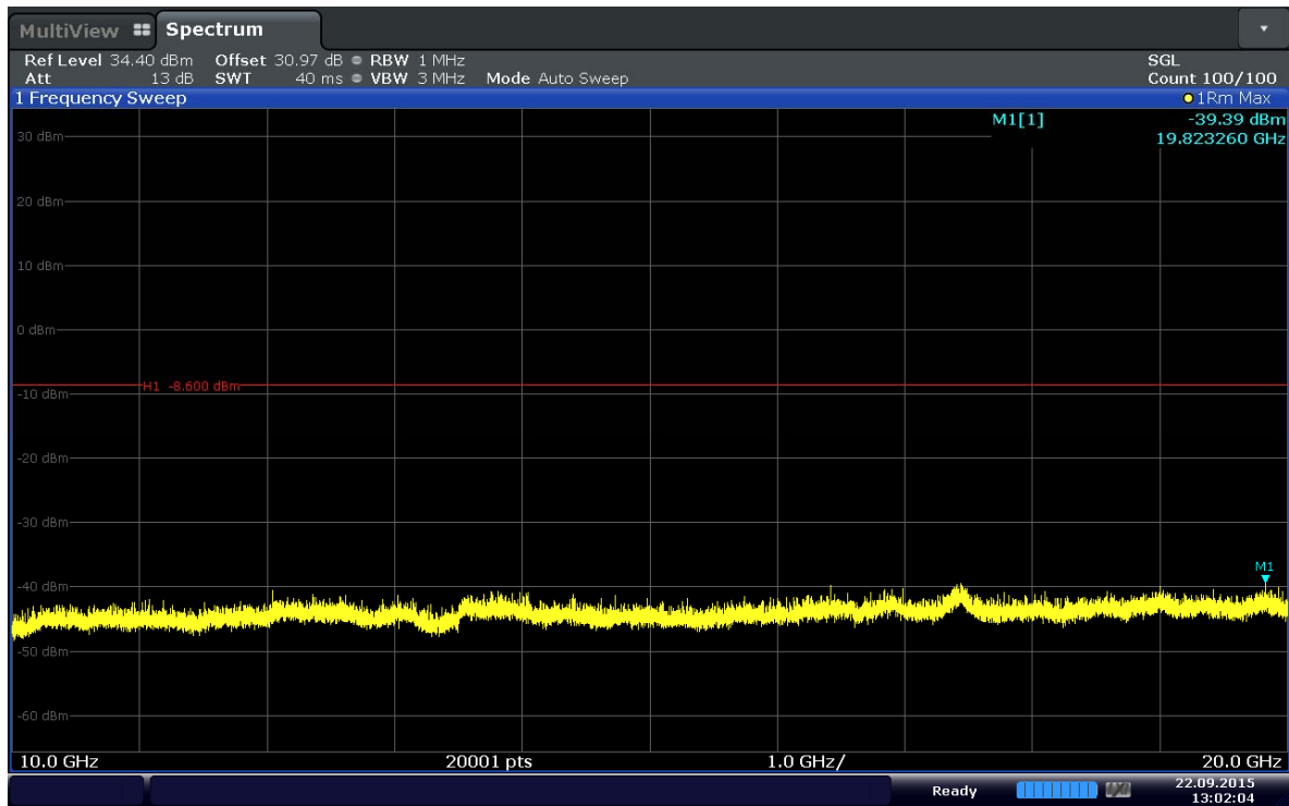
Plot 6-13. Conducted Spurious Plot (Band 41–5MHz–QPSK–RB Size 1–RB Offset 0–Ch.40740)
