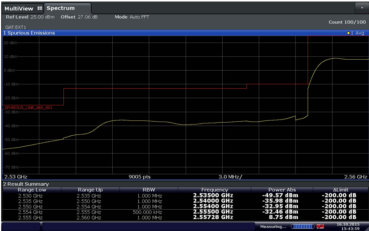
Plot 6-51. Lower Band Edge Plot (Band41 – 20MHz – QPSK – RB Size 100 – Ch.40340)
