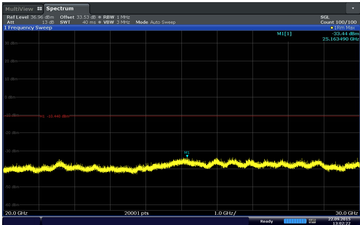
Plot 6-14. Conducted Spurious Plot (Band 41–5MHz–QPSK–RB Size 1–RB Offset 0–Ch.40740)
