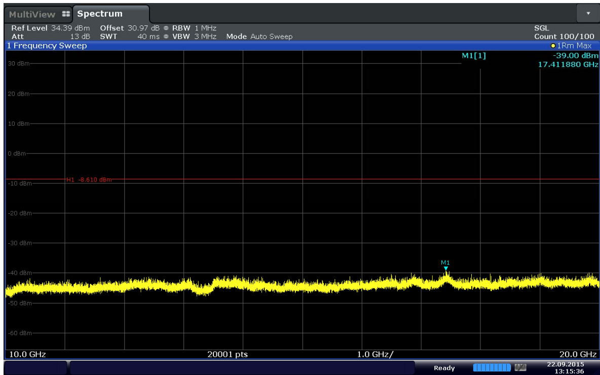
Plot 6-37. Conducted Spurious Plot (Band 41–20MHz–QPSK–RB Size 1–RB Offset 99–Ch.40340)
