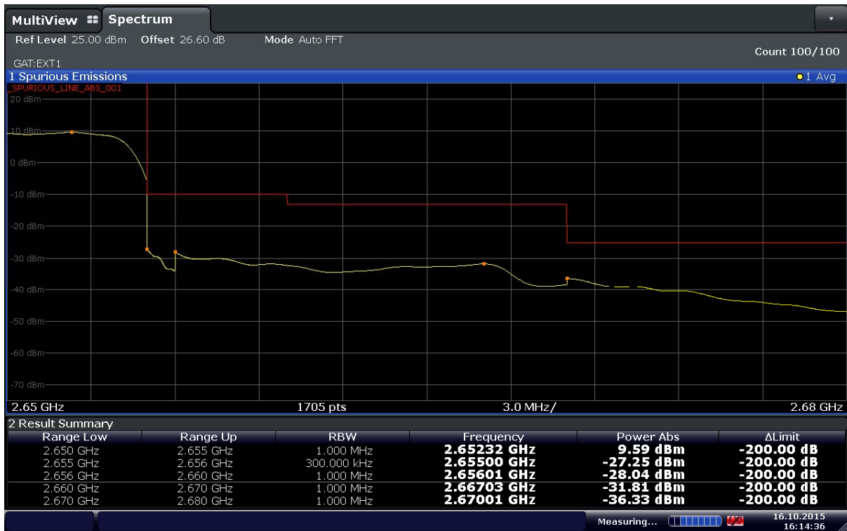
Plot 6-50. Upper Band Edge Plot (Band41 – 15MHz – QPSK – RB Size 75 – Ch.41165)
