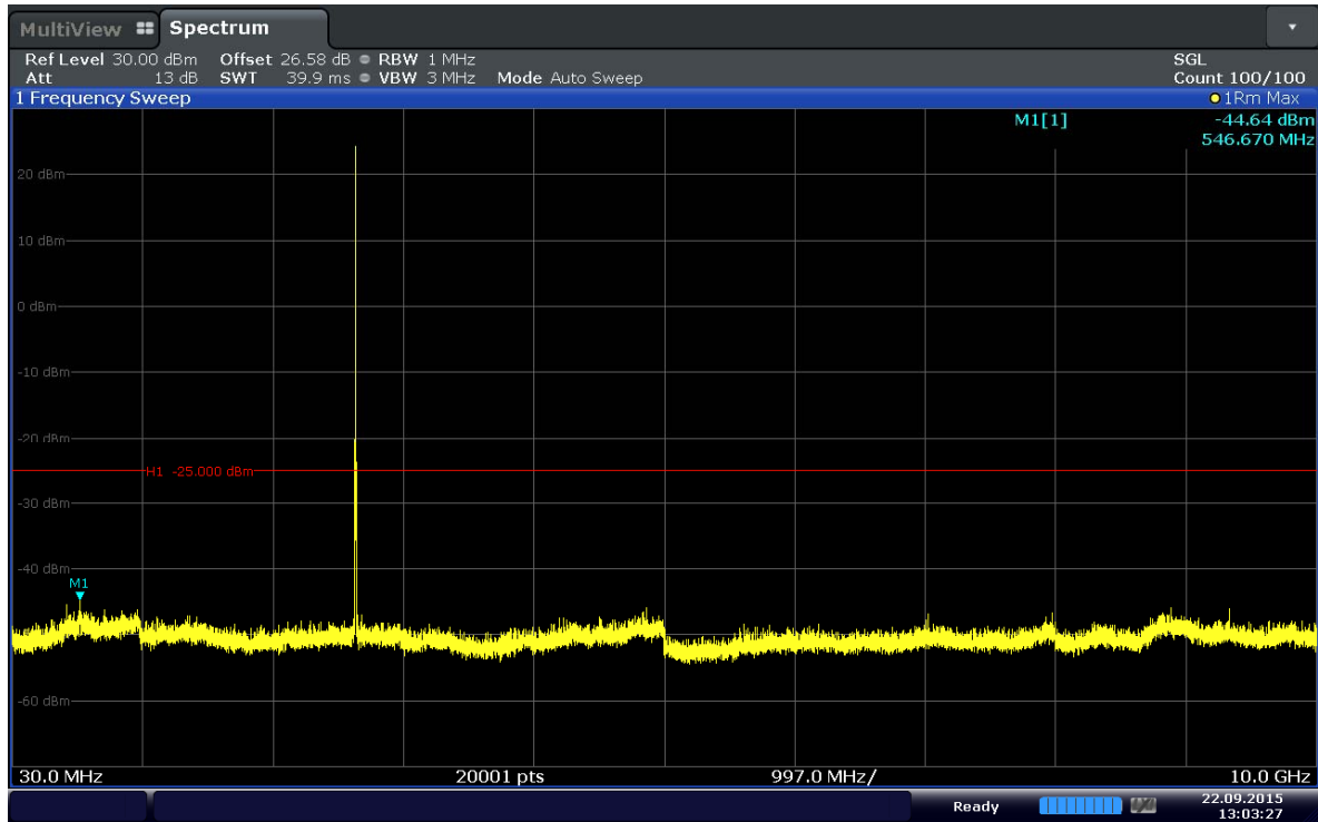
Plot 6-15. Conducted Spurious Plot (Band 41–5MHz–QPSK–RB Size 1–RB Offset 12–Ch.41215)
