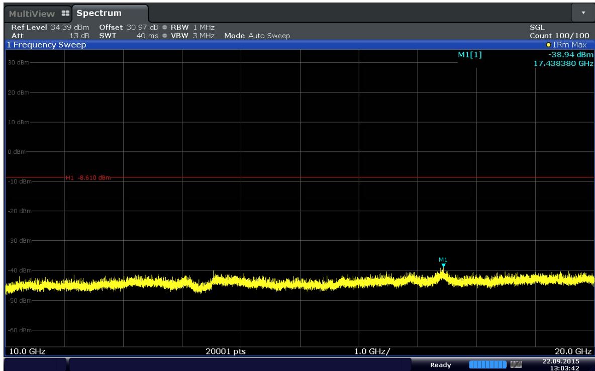
Plot 6-16. Conducted Spurious Plot (Band 41–5MHz–QPSK–RB Size 1–RB Offset 12–Ch.41215)
