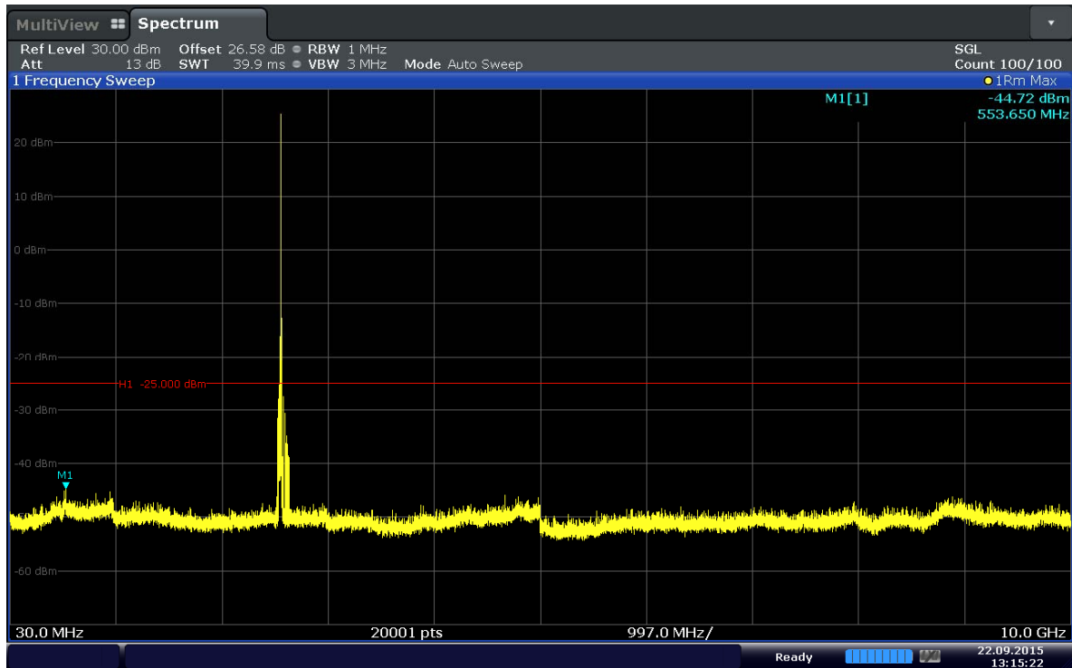
Plot 6-36. Conducted Spurious Plot (Band 41–20MHz–QPSK–RB Size 1–RB Offset 99–Ch.40340)
