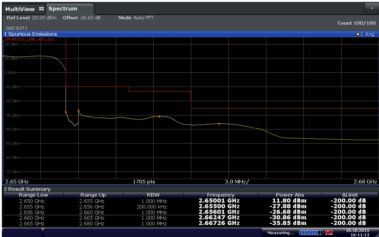
Plot 6-48. Upper Band Edge Plot (Band41 – 10MHz – QPSK – RB Size 50 – Ch.41190)
