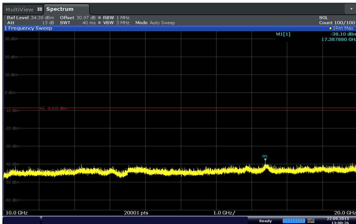
Plot 6-9. Conducted Spurious Plot (Band 41-5MHz-QPSK-RB Size 1-RB Offset 12-Ch.40265)
