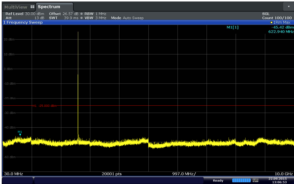
Plot 6-21. Conducted Spurious Plot (Band 41–10MHz–QPSK–RB Size 1–RB Offset 24–Ch.40740)
