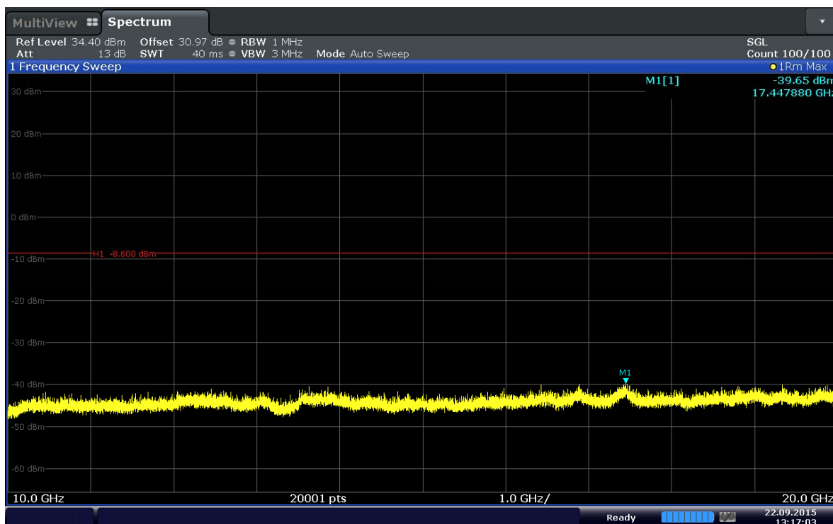
Plot 6-40. Conducted Spurious Plot (Band 41–20MHz–QPSK–RB Size 1–RB Offset 99–Ch.40740)
