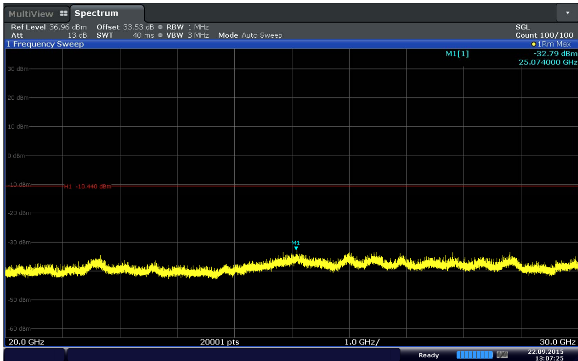
Plot 6-23. Conducted Spurious Plot (Band 41–10MHz–QPSK–RB Size 1–RB Offset 24–Ch.40740)
