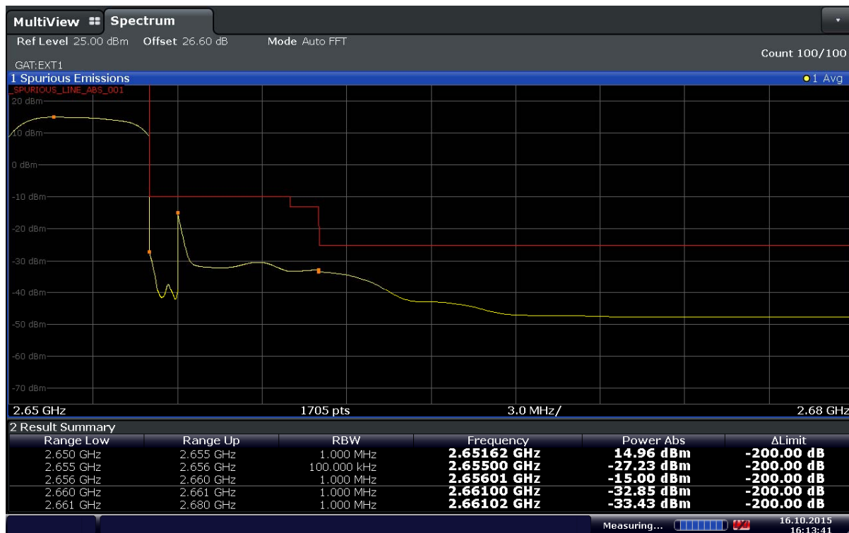
Plot 6-46. Upper Band Edge Plot (Band41 – 5MHz – QPSK – RB Size 25 – Ch.41215)
