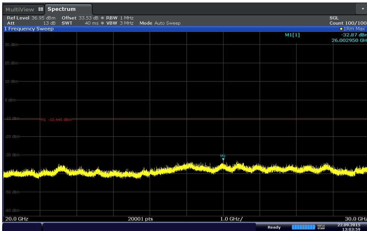
Plot 6-17. Conducted Spurious Plot (Band 41–5MHz–QPSK–RB Size 1–RB Offset 12–Ch.41215)
