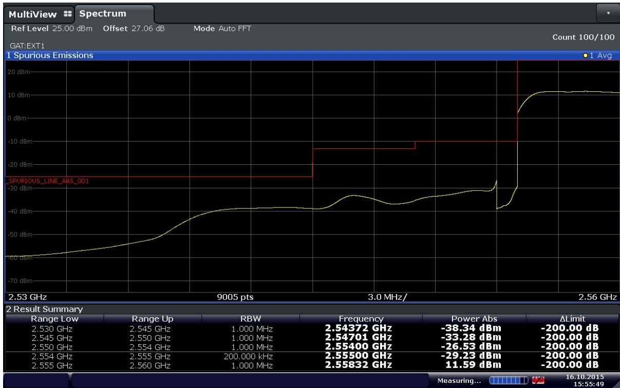
Plot 6-47. Lower Band Edge Plot (Band41 – 10MHz – QPSK – RB Size 50 – Ch.40290 )
