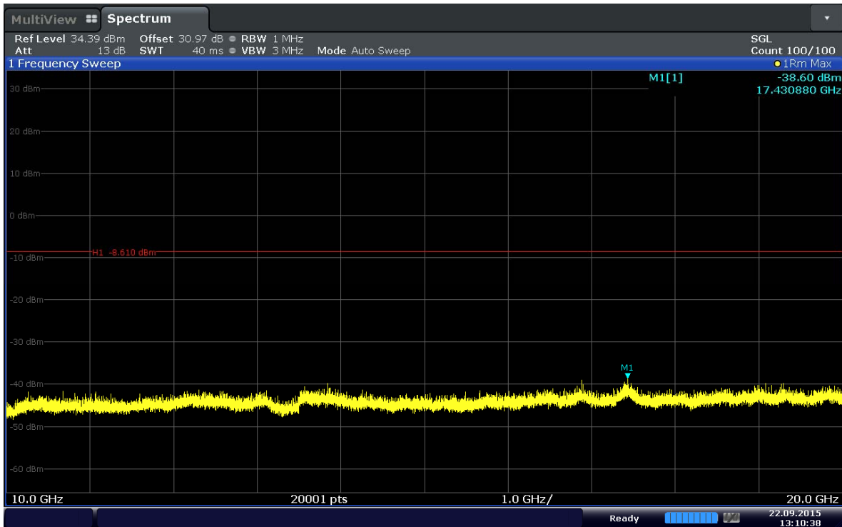
Plot 6-28. Conducted Spurious Plot (Band 41–15MHz–QPSK–RB Size 1–RB Offset 74–Ch.40315)
