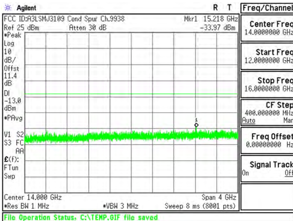
Plot 6-33. Conducted Spurious Plot (PCS WCDMA Mode - Ch.9538(DL9938))
