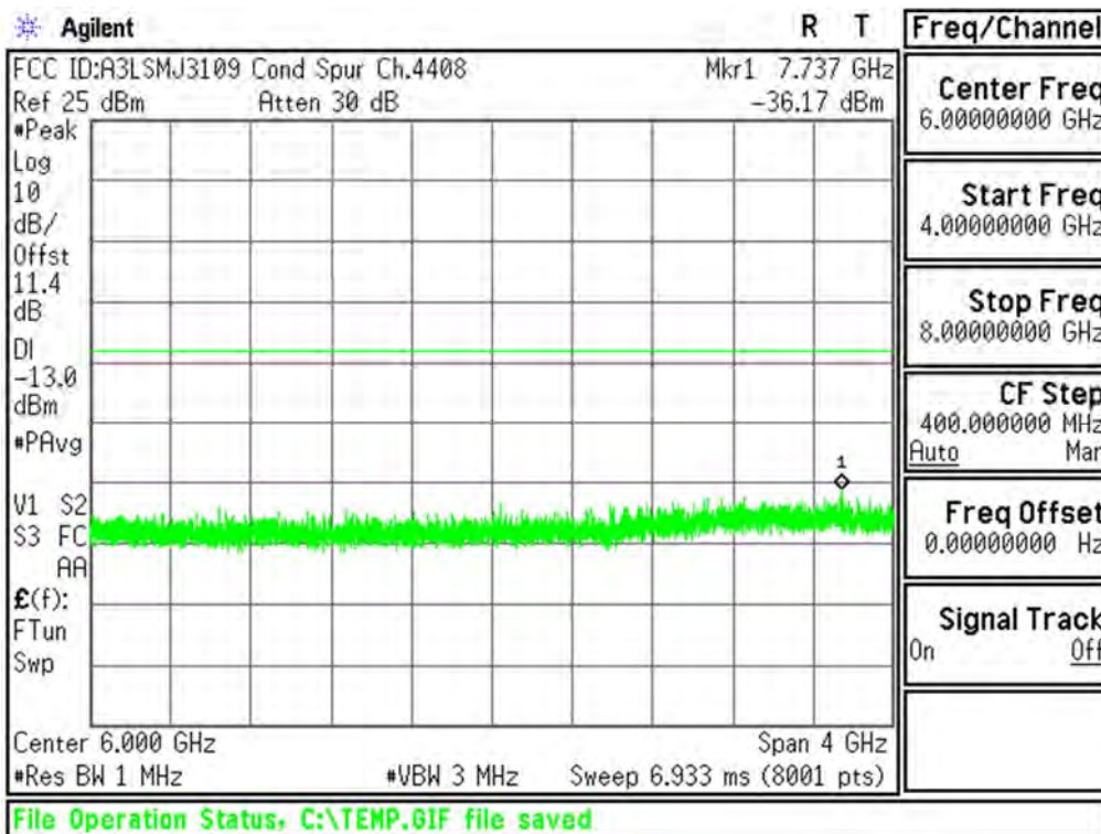
Plot 6-15. Conducted Spurious Plot (Cellular WCDMA Mode - Ch.4183(DL4408))
