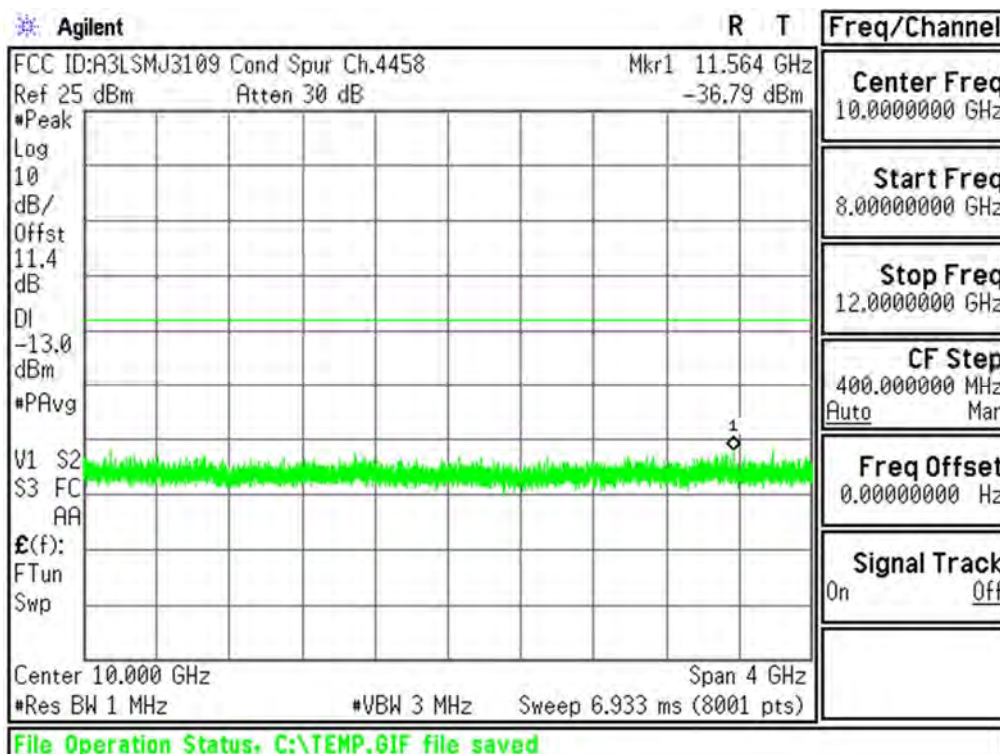
Plot 6-19. Conducted Spurious Plot (Cellular WCDMA Mode - Ch.4233(DL4458))
