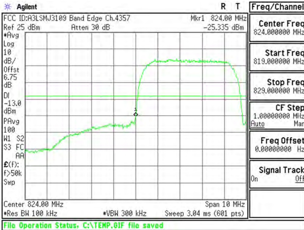
Plot 6-39. Lower Band Edge Plot (Cellular WCDMA Mode - Ch.4132(DL4357))
