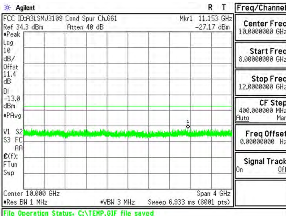
Plot 6-3. Conducted Spurious Plot (PCS GSM Mode - Ch.661)
