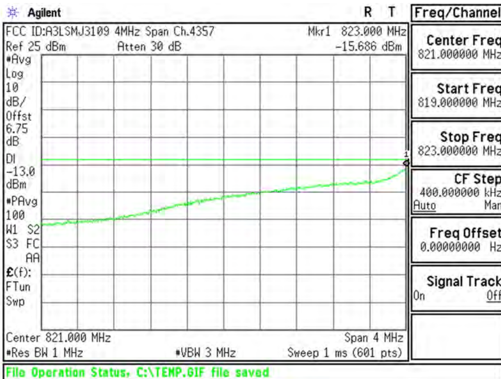
Plot 6-40. Extended Lower Band Edge Plot (Cellular WCDMA Mode - Ch.4132(DL4357))
