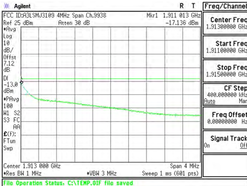
Plot 6-46. Extended Upper Band Edge Plot (PCS WCDMA Mode - Ch.9538(DL9938))
