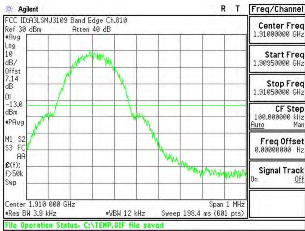
Plot 6-37. Upper Band Edge Plot (PCS GSM Mode – Ch.810)
