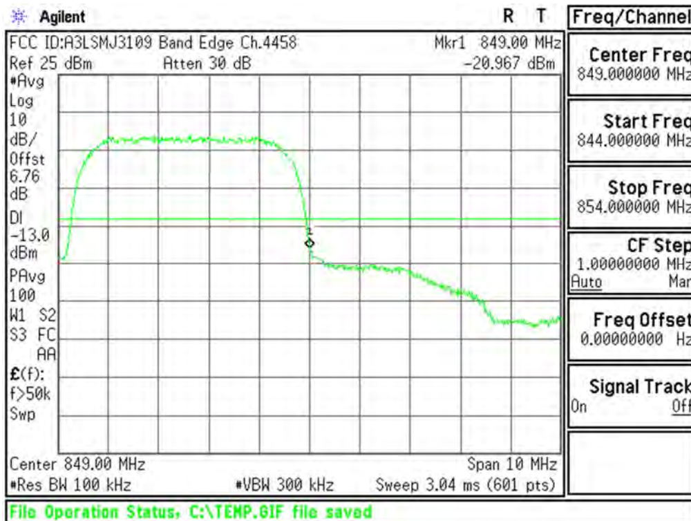
Plot 6-41. Upper Band Edge Plot (Cellular WCDMA Mode - Ch.4233(DL4458))
