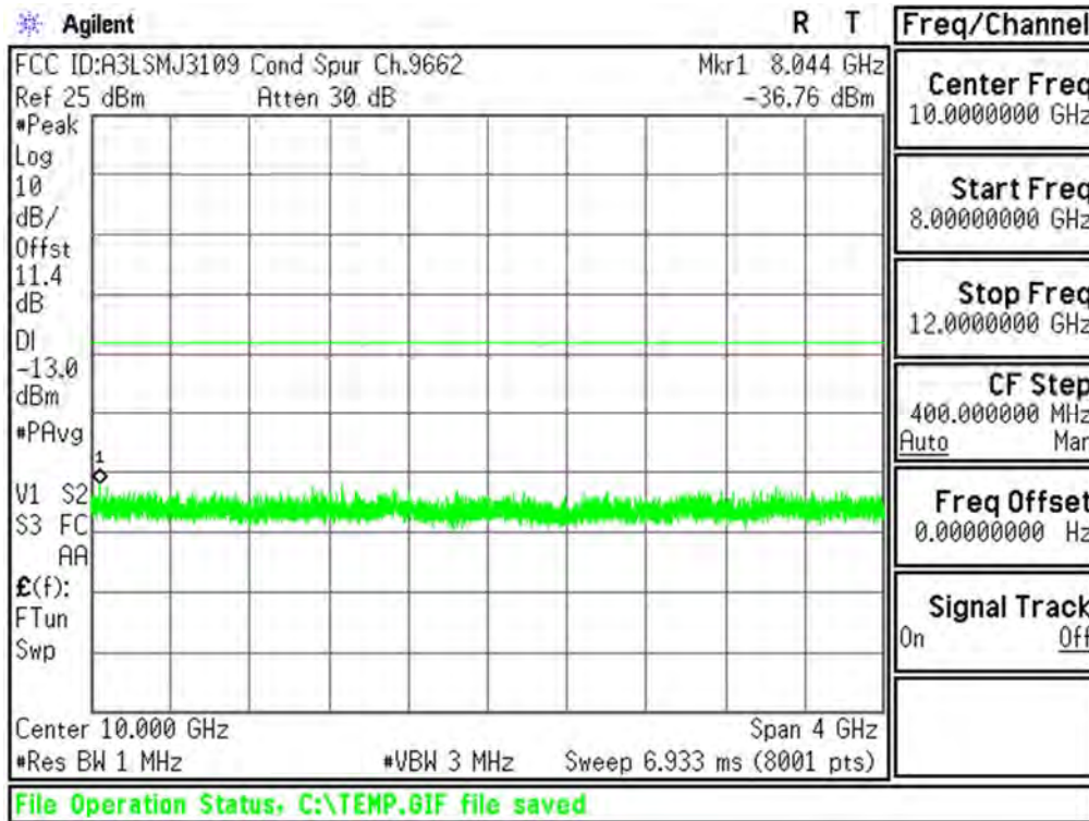
Plot 6-22. Conducted Spurious Plot (PCS WCDMA Mode - Ch.9262(DL9662))
