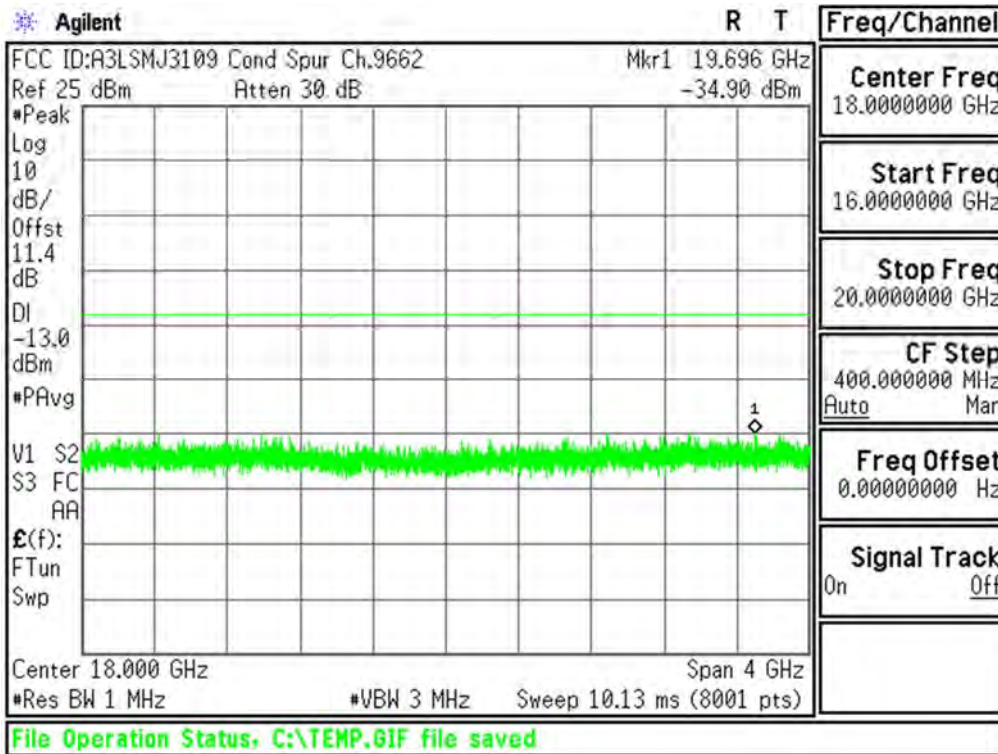
Plot 6-24. Conducted Spurious Plot (PCS WCDMA Mode - Ch.9262(DL9662))
