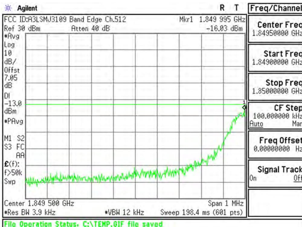
Plot 6-36. Lower Band Edge Plot (PCS GSM Mode – Ch.512)
