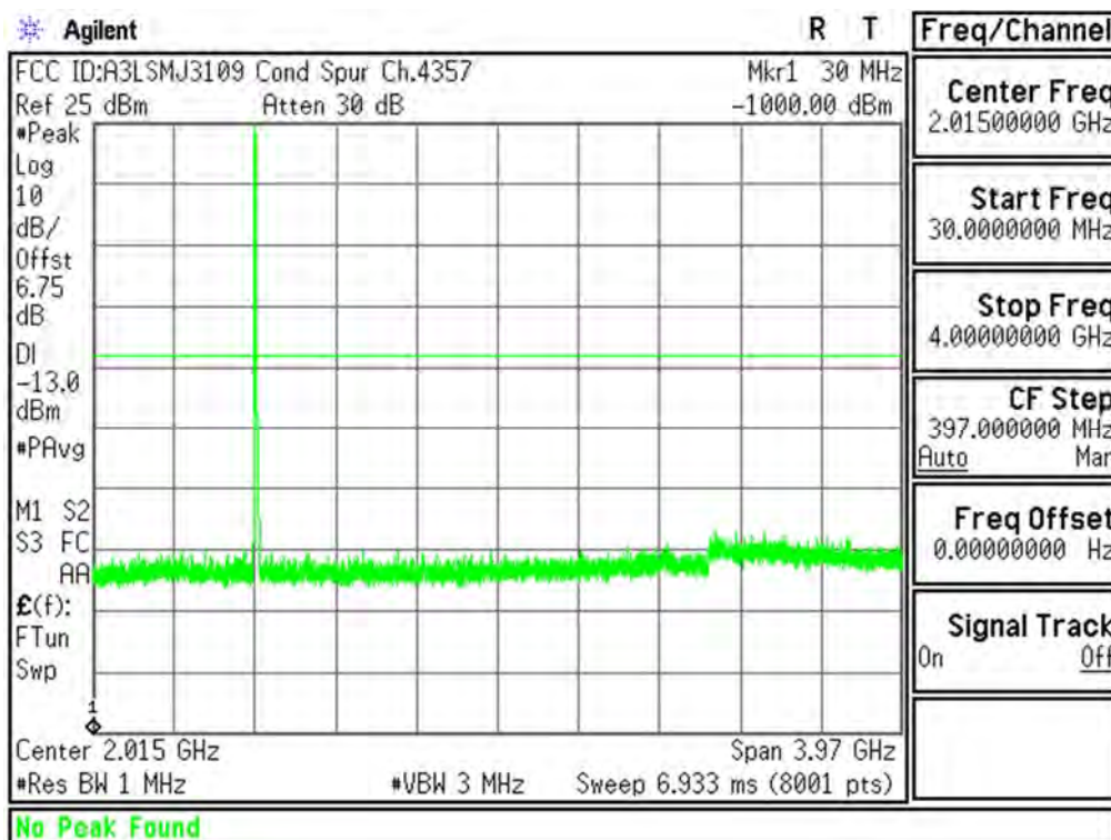
Plot 6-11. Conducted Spurious Plot (Cellular WCDMA Mode - Ch.4132(DL4357))
