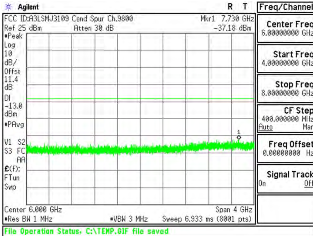
Plot 6-26. Conducted Spurious Plot (PCS WCDMA Mode - Ch.9400(DL9800))
