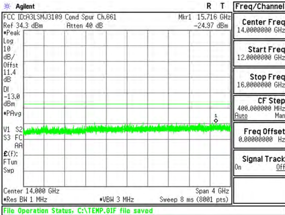
Plot 6-4. Conducted Spurious Plot (PCS GSM Mode - Ch.661)
