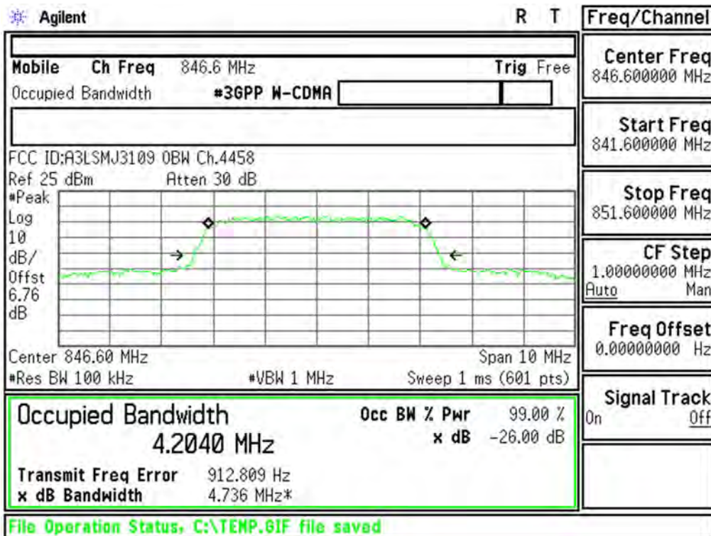
Plot 6-3. Occupied Bandwidth Plot (Cellular WCDMA Mode - Ch.4233(DL4458))
