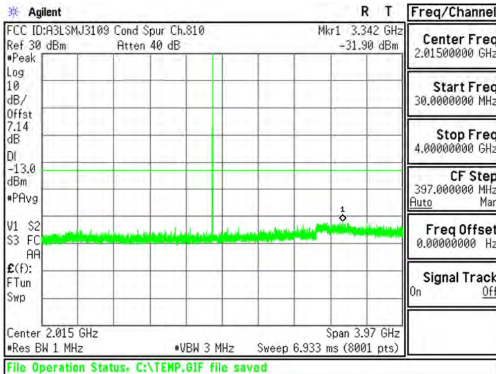
Plot 6-6. Conducted Spurious Plot (PCS GSM Mode - Ch.810)
