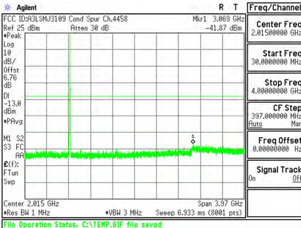
Plot 6-17. Conducted Spurious Plot (Cellular WCDMA Mode - Ch.4233(DL4458))
