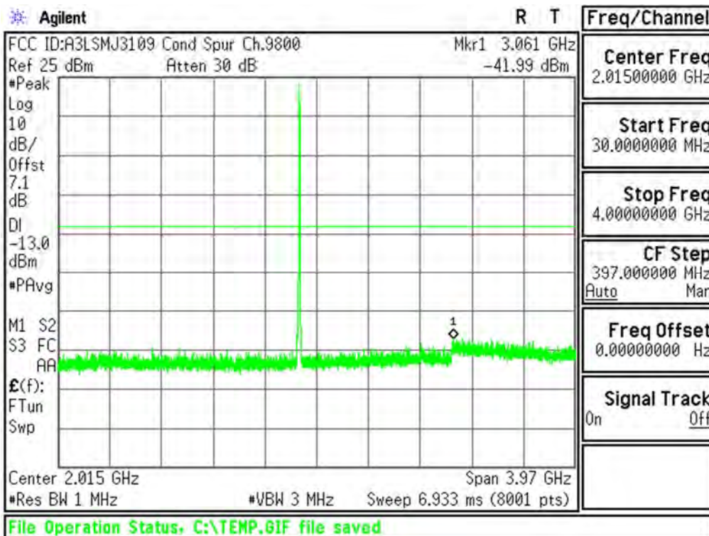
Plot 6-25. Conducted Spurious Plot (PCS WCDMA Mode - Ch.9400(DL9800))
