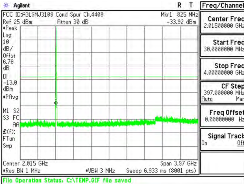
Plot 6-14. Conducted Spurious Plot (Cellular WCDMA Mode - Ch.4183(DL4408))
