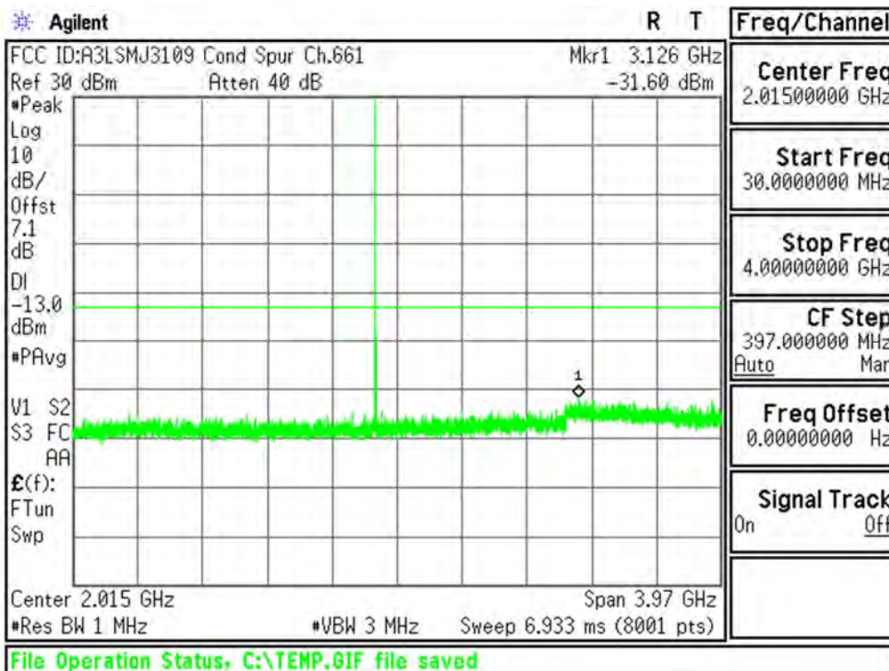
Plot 6-1. Conducted Spurious Plot (PCS GSM Mode - Ch.661)
