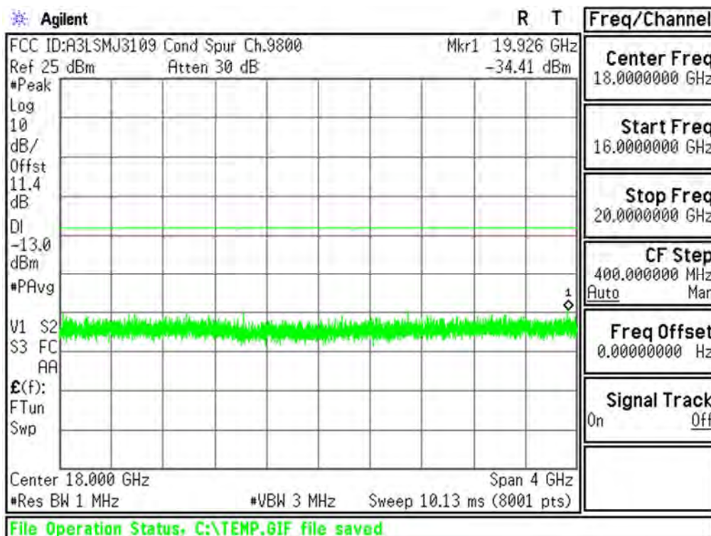
Plot 6-29. Conducted Spurious Plot (PCS WCDMA Mode - Ch.9400(DL9800))
