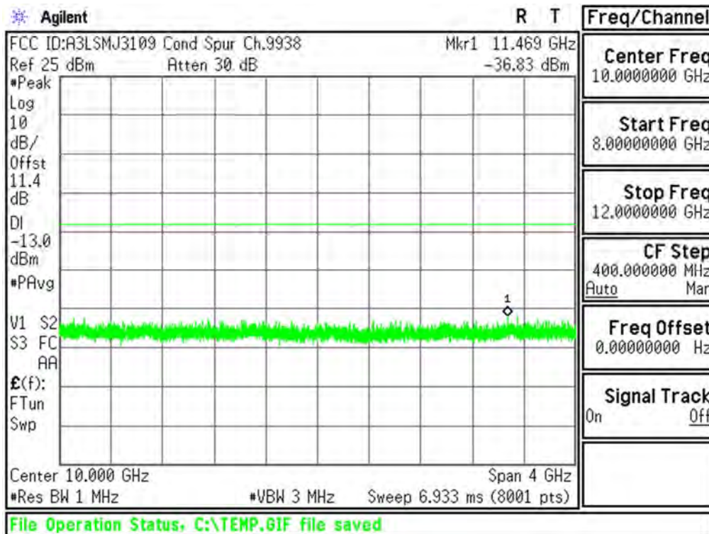
Plot 6-32. Conducted Spurious Plot (PCS WCDMA Mode - Ch.9538(DL9938))
