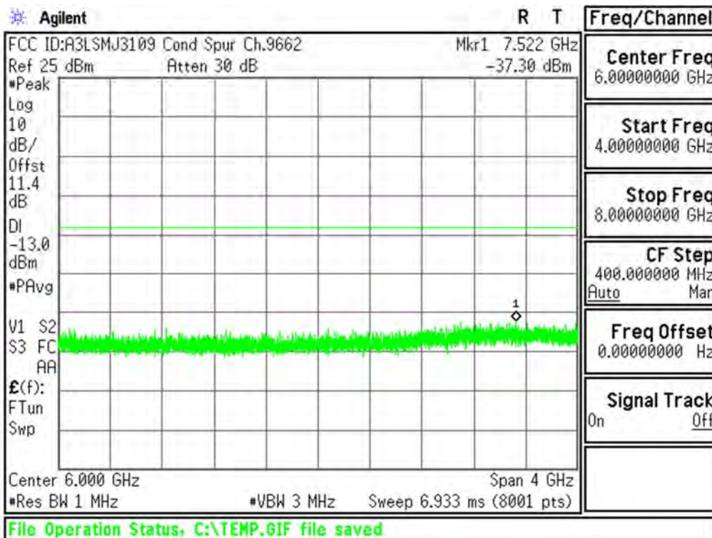
Plot 6-21. Conducted Spurious Plot (PCS WCDMA Mode - Ch.9262(DL9662))
