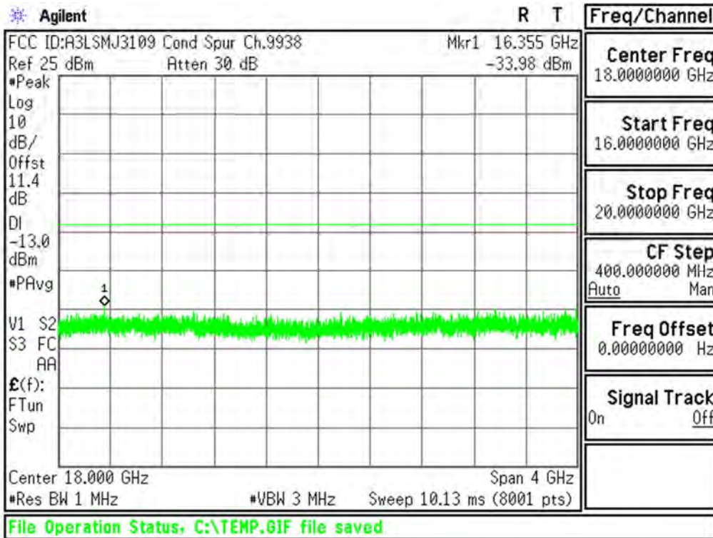
Plot 6-34. Conducted Spurious Plot (PCS WCDMA Mode - Ch.9538(DL9938))
