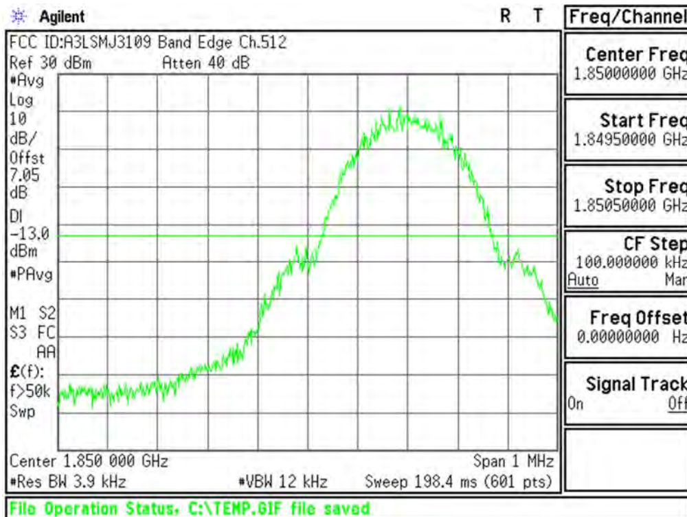
Plot 6-35. Lower Band Edge Plot (PCS GSM Mode – Ch.512)
