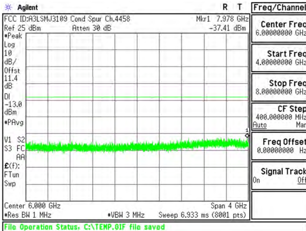
Plot 6-18. Conducted Spurious Plot (Cellular WCDMA Mode - Ch.4233(DL4458))
