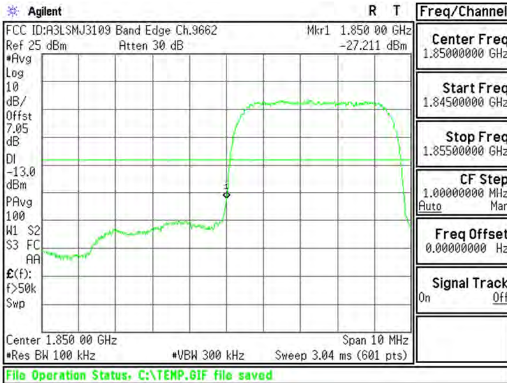
Plot 6-43. Lower Band Edge Plot (PCS WCDMA Mode - Ch.9262(DL9662))
