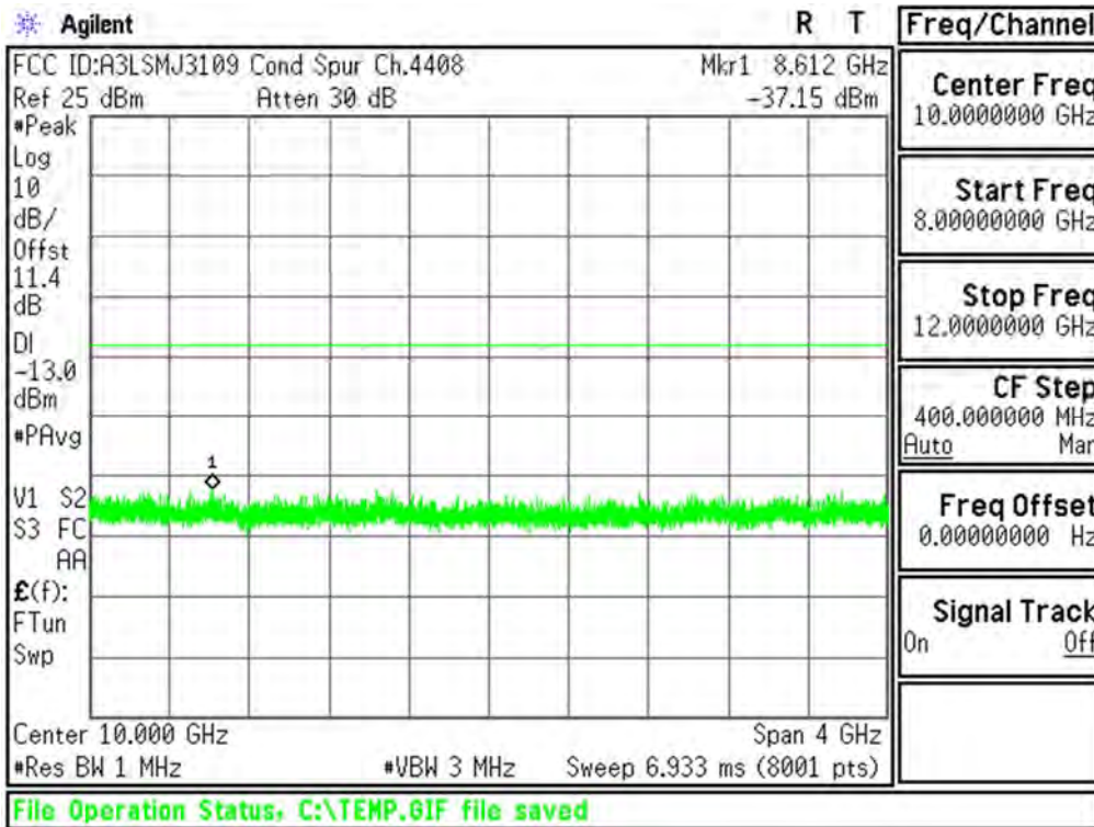
Plot 6-16. Conducted Spurious Plot (Cellular WCDMA Mode - Ch.4183(DL4408))
