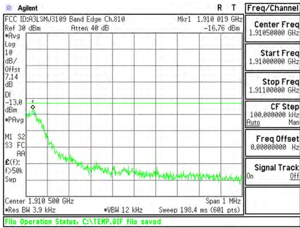
Plot 6-38. Upper Band Edge Plot (PCS GSM Mode – Ch.810)
