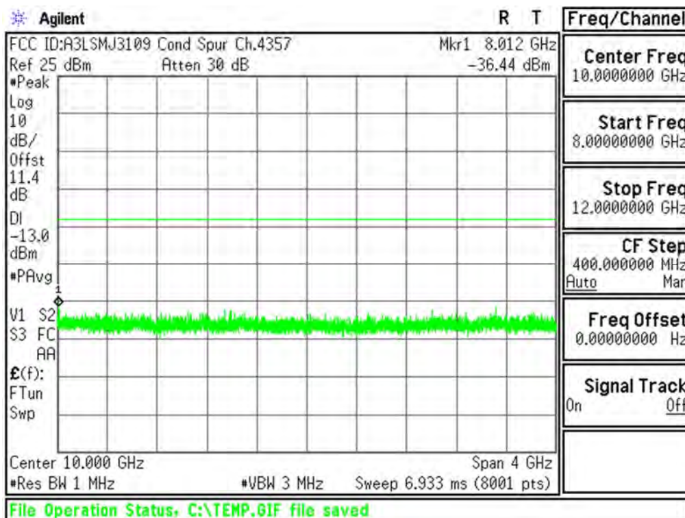
Plot 6-13. Conducted Spurious Plot (Cellular WCDMA Mode - Ch.4132(DL4357))
