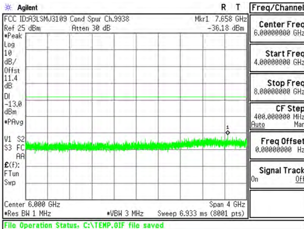
Plot 6-31. Conducted Spurious Plot (PCS WCDMA Mode - Ch.9538(DL9938))
