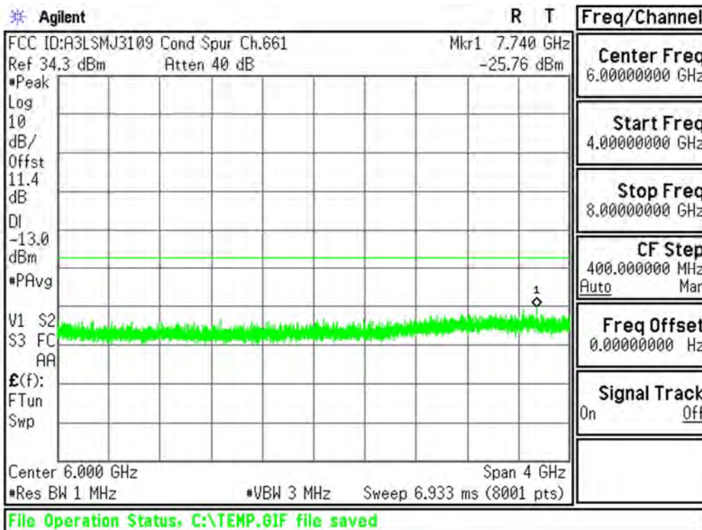
Plot 6-2. Conducted Spurious Plot (PCS GSM Mode - Ch.661)
