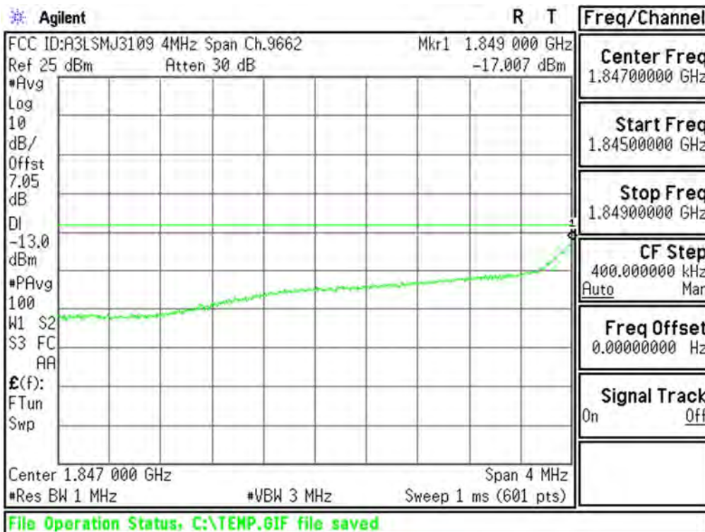
Plot 6-44. Extended Lower Band Edge Plot (PCS WCDMA Mode - Ch.9262(DL9662))
