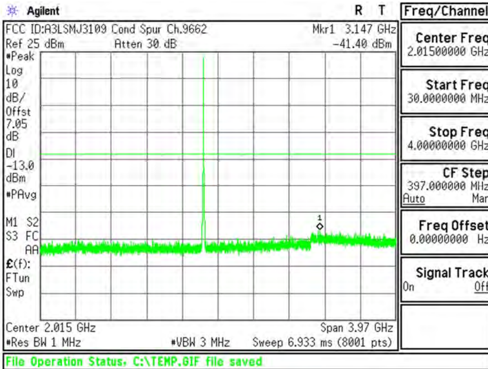
Plot 6-20. Conducted Spurious Plot (PCS WCDMA Mode - Ch.9262(DL9662))
