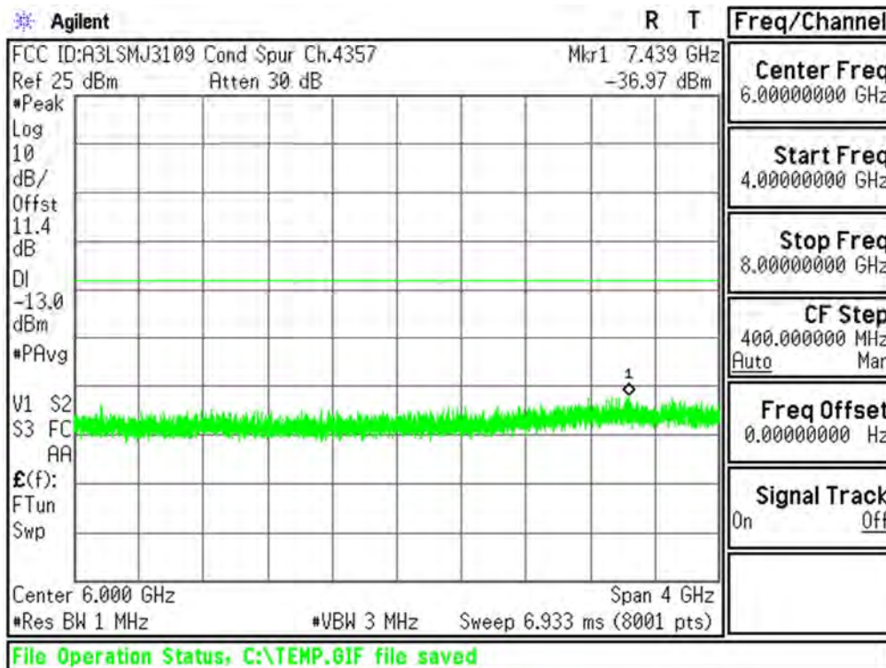
Plot 6-12. Conducted Spurious Plot (Cellular WCDMA Mode - Ch.4132(DL4357))
