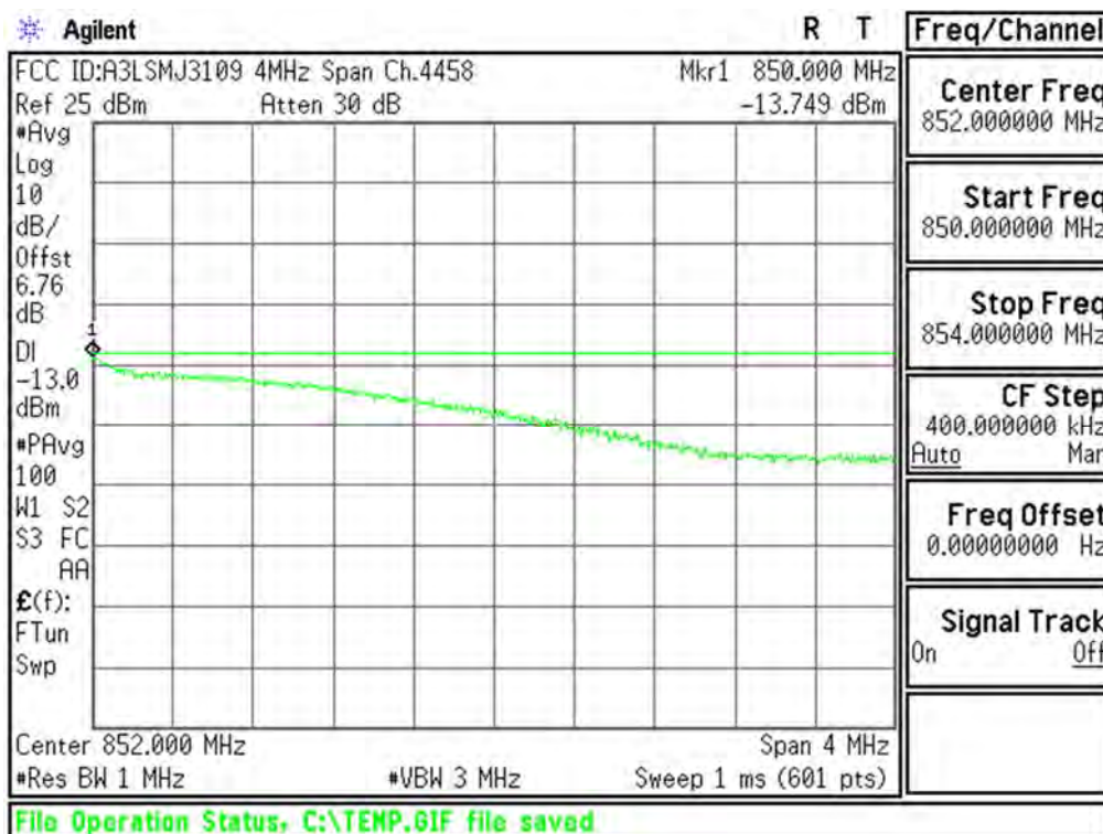
Plot 6-42. Extended Upper Band Edge Plot (Cellular WCDMA Mode - Ch.4233(DL4458))
