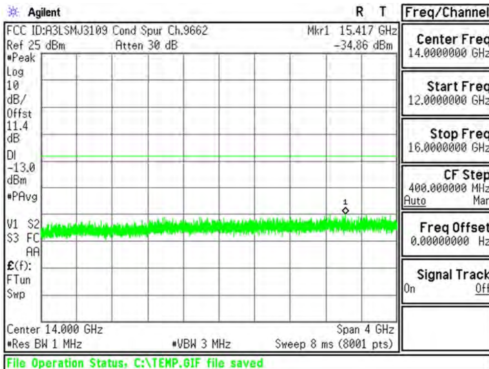
Plot 6-23. Conducted Spurious Plot (PCS WCDMA Mode - Ch.9262(DL9662))
