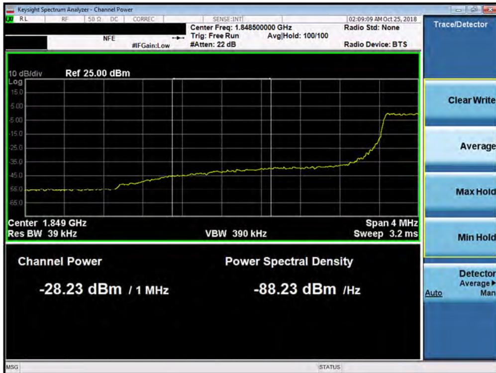
Plot 7-176. Lower Extended Band Edge Plot (Band 2 – 3.0MHz QPSK - Full RB Configuration)
