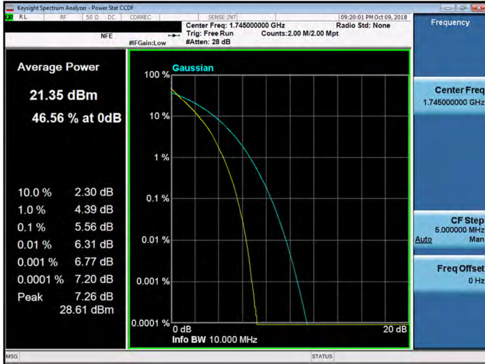
Plot 7-209. PAR Plot (Band 66/4 - 10.0MHz QPSK - Full RB Configuration)
