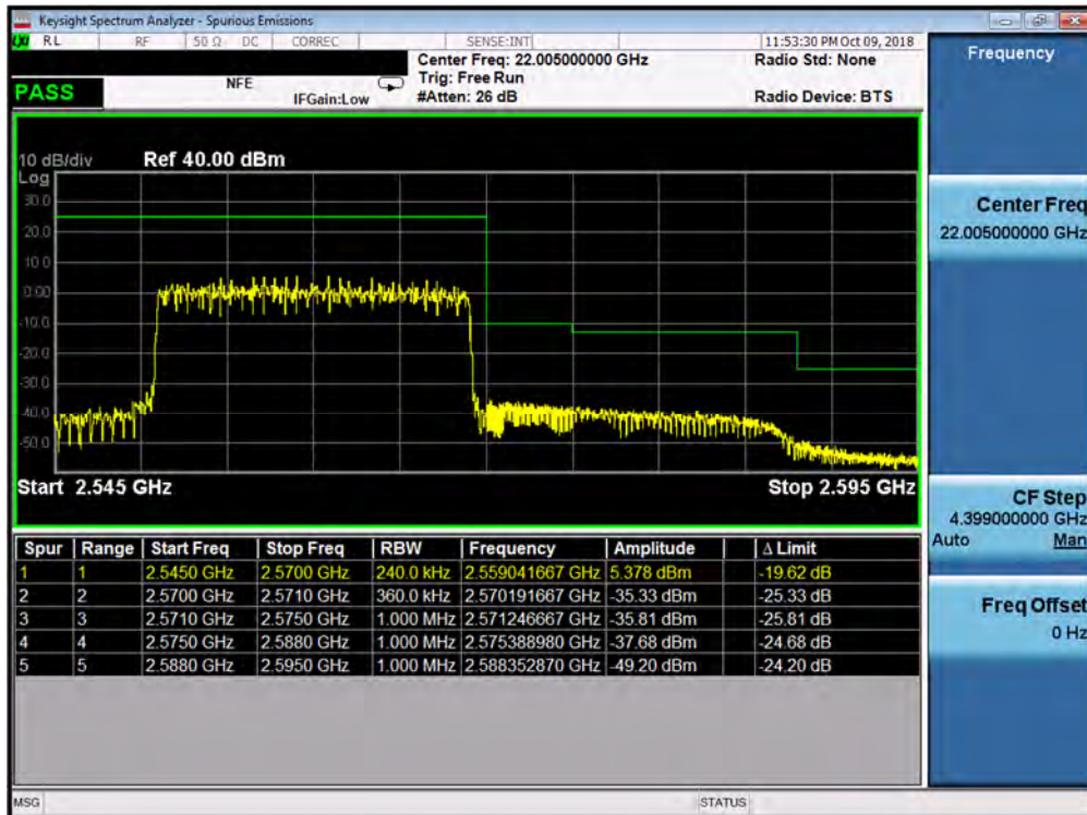
Plot 7-202. Upper ACP Plot (Band 7 - 20.0MHz QPSK - RB Size 100)
