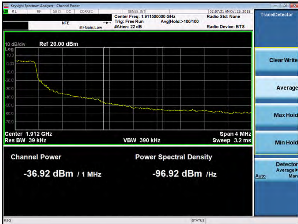
Plot 7-174. Upper Extended Band Edge Plot (Band 2 – 1.4MHz QPSK - Full RB Configuration)
