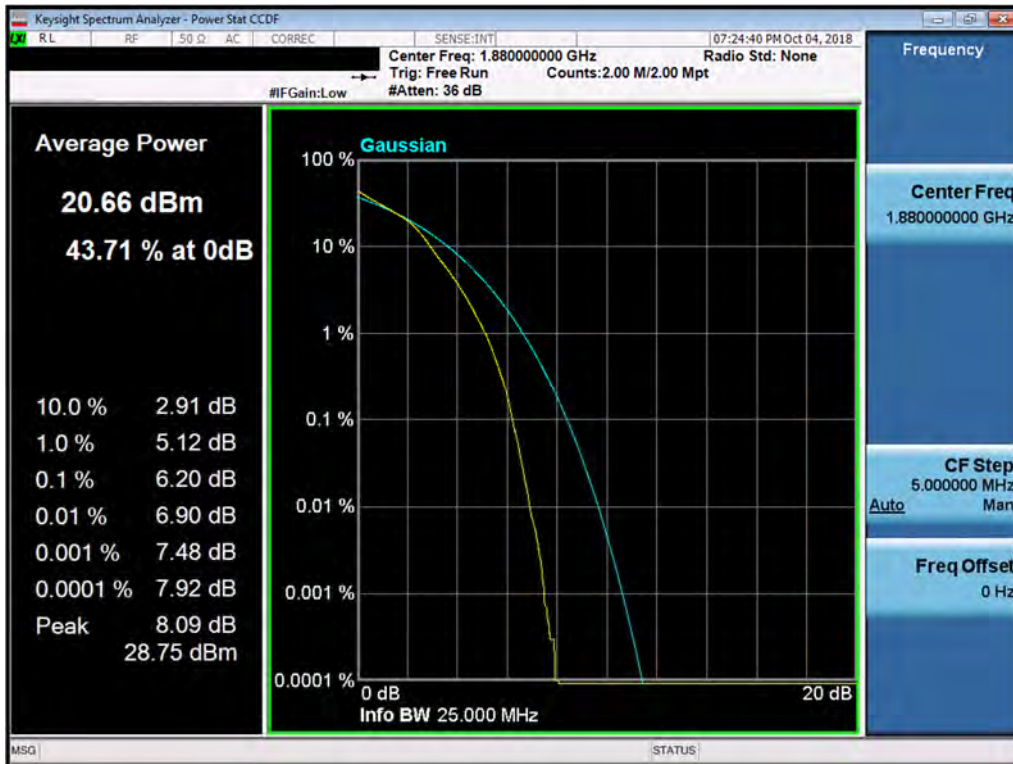
Plot 7-224. PAR Plot (Band 2 - 15.0MHz 16-QAM - Full RB Configuration)
