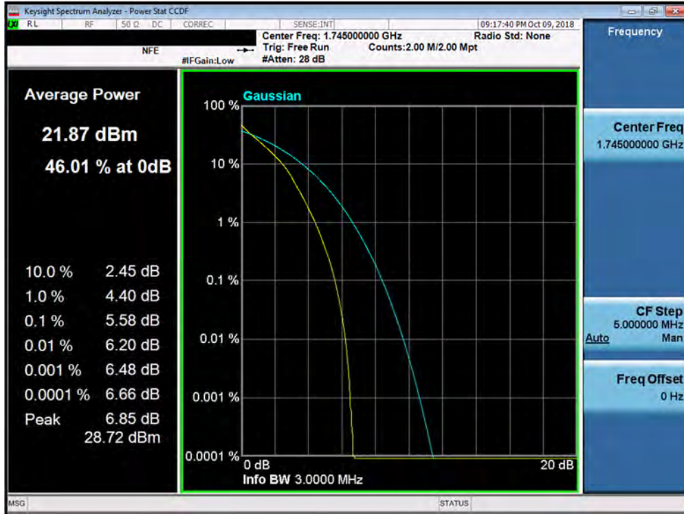
Plot 7-205. PAR Plot (Band 66/4 - 3.0MHz QPSK - Full RB Configuration)
