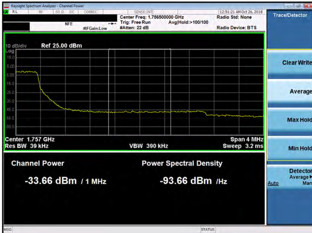
Plot 7-144. Upper Extended Band Edge Plot (Band 4 - 3.0MHz QPSK - Full RB Configuration)
