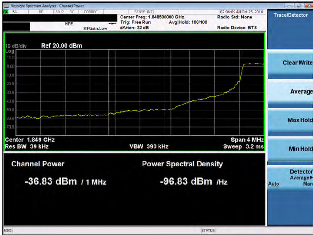
Plot 7-172. Lower Extended Band Edge Plot (Band 2 – 1.4MHz QPSK - Full RB Configuration)
