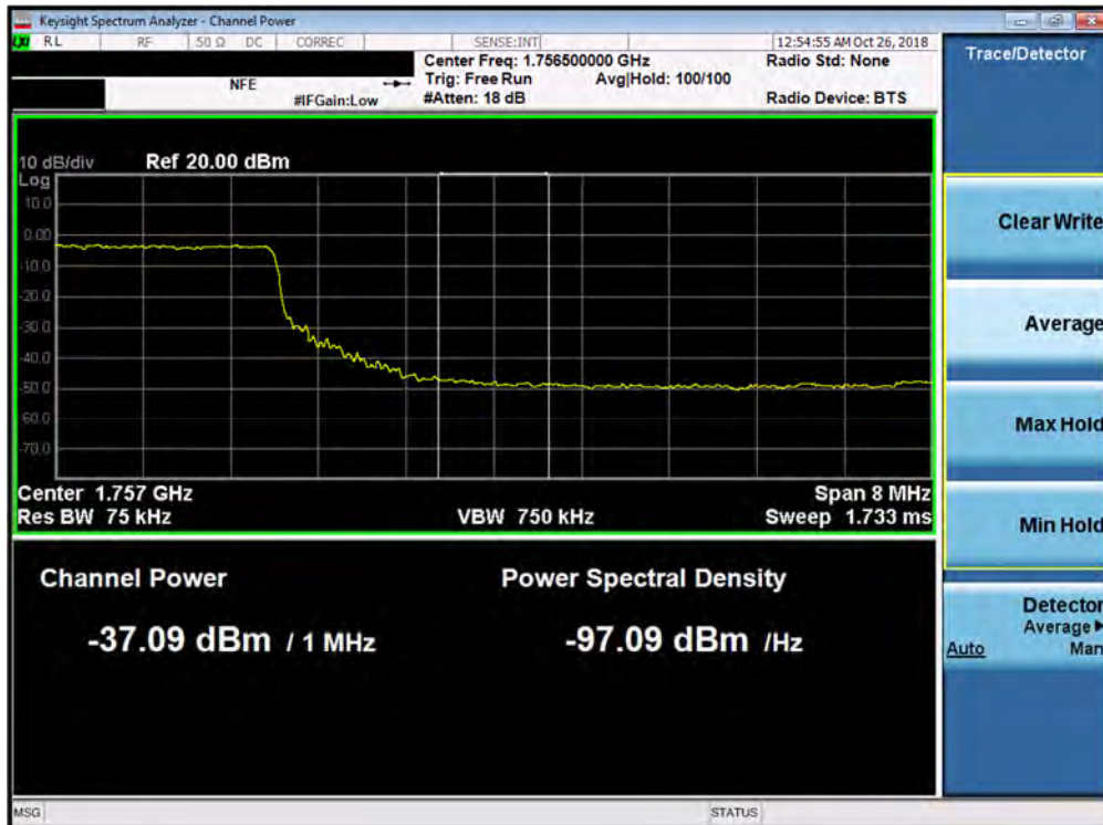
Plot 7-156. Upper Extended Band Edge Plot (Band 4 - 10.0MHz QPSK - Full RB Configuration)
