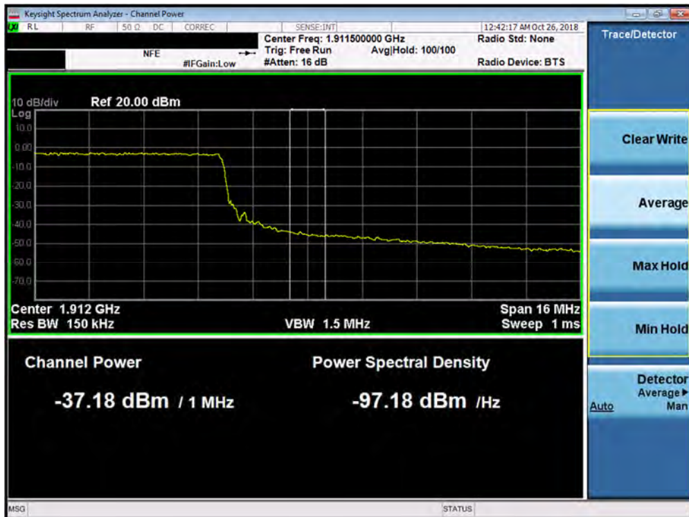
Plot 7-194. Upper Extended Band Edge Plot (Band 2 - 20.0MHz QPSK - Full RB Configuration)
