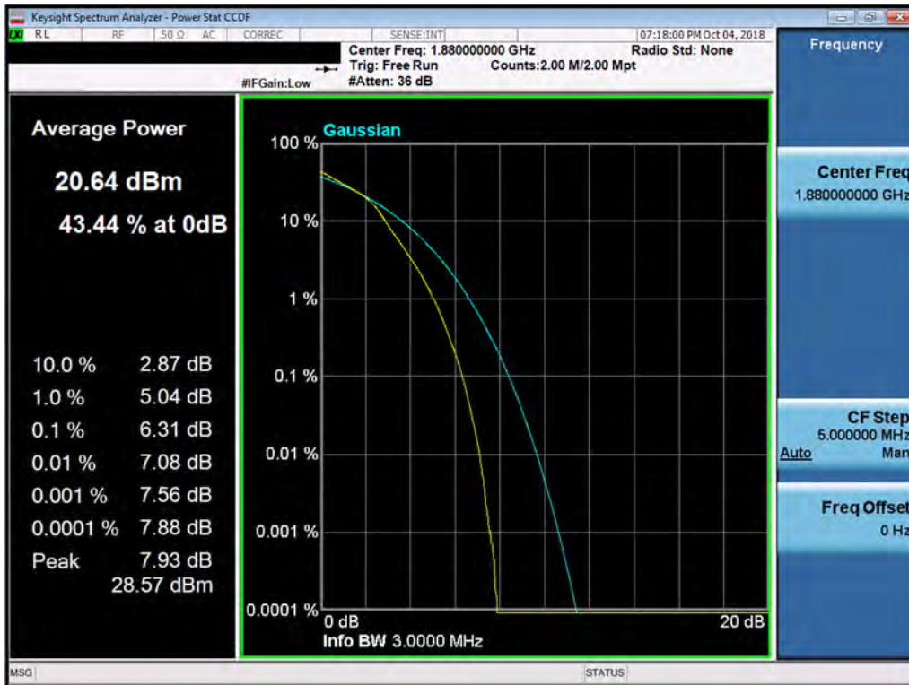
Plot 7-218. PAR Plot (Band 2 - 3.0MHz 16-QAM - Full RB Configuration)
