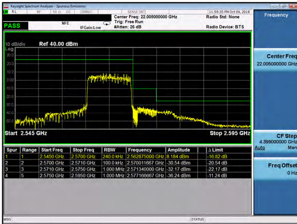
Plot 7-198. Upper ACP Plot (Band 7 - 10.0MHz QPSK - RB Size 50)
