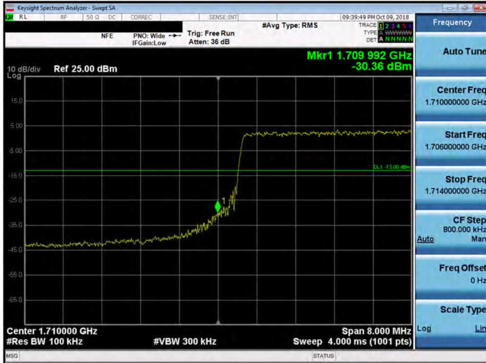
Plot 7-153. Lower Band Edge Plot (Band 66/4 - 10.0MHz QPSK - Full RB Configuration)
