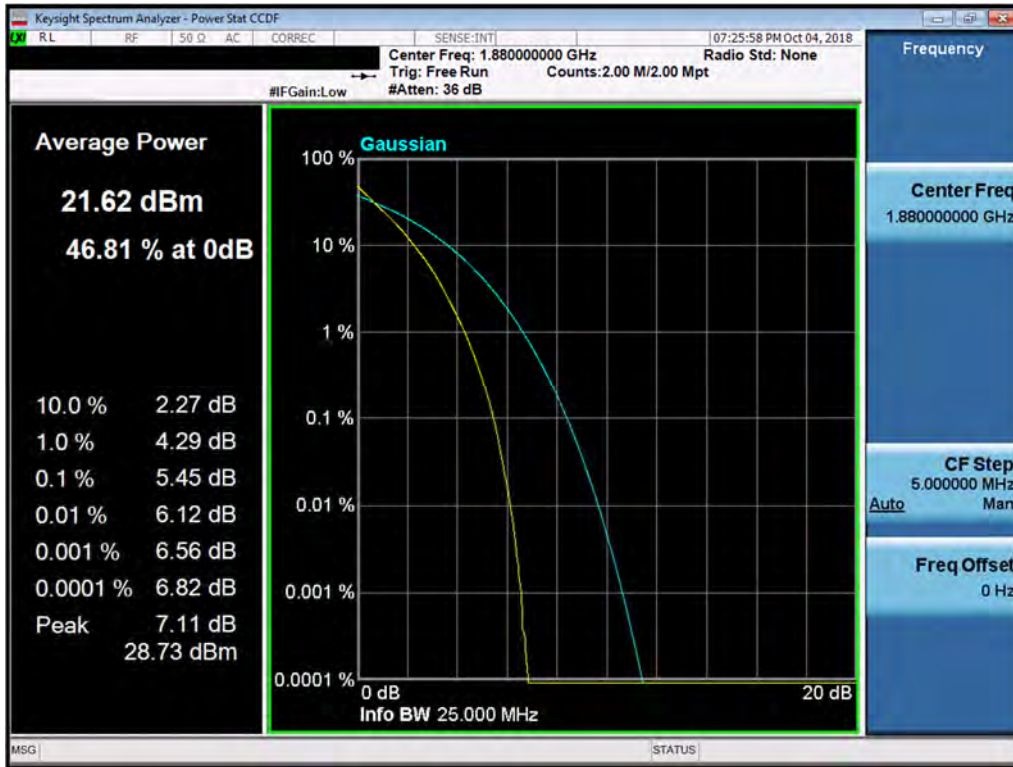
Plot 7-225. PAR Plot (Band 2 - 20.0MHz QPSK - Full RB Configuration)
