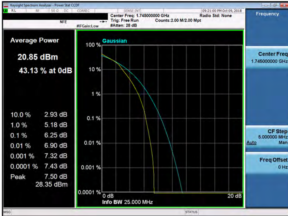
Plot 7-212. PAR Plot (Band 66/4 - 15.0MHz 16-QAM - Full RB Configuration)
