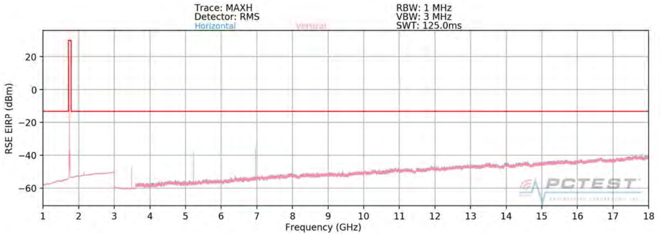
Plot 7-230. Radiated Spurious Plot above 1GHz (Band 66/4)
