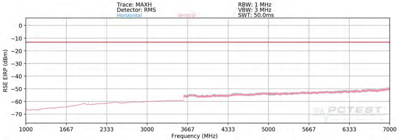
Plot 7-227. Radiated Spurious Plot above 1GHz (Band 71)
