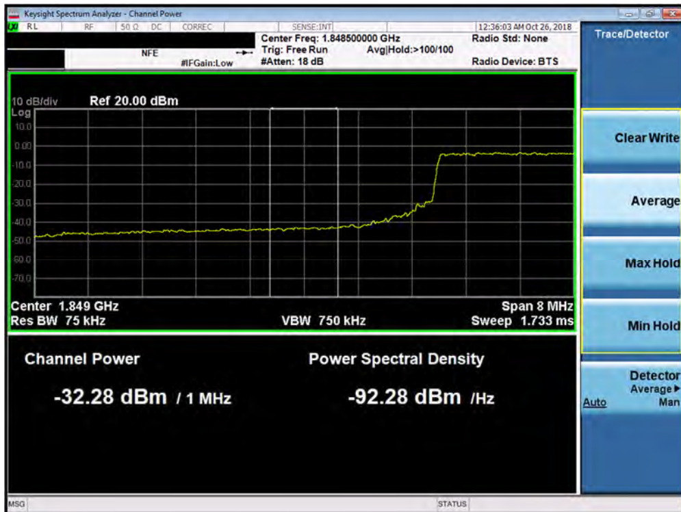
Plot 7-184. Lower Extended Band Edge Plot (Band 2 – 10.0MHz QPSK - Full RB Configuration)
