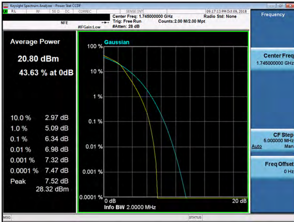
Plot 7-204. PAR Plot (Band 66/4 - 1.4MHz 16-QAM - Full RB Configuration)
