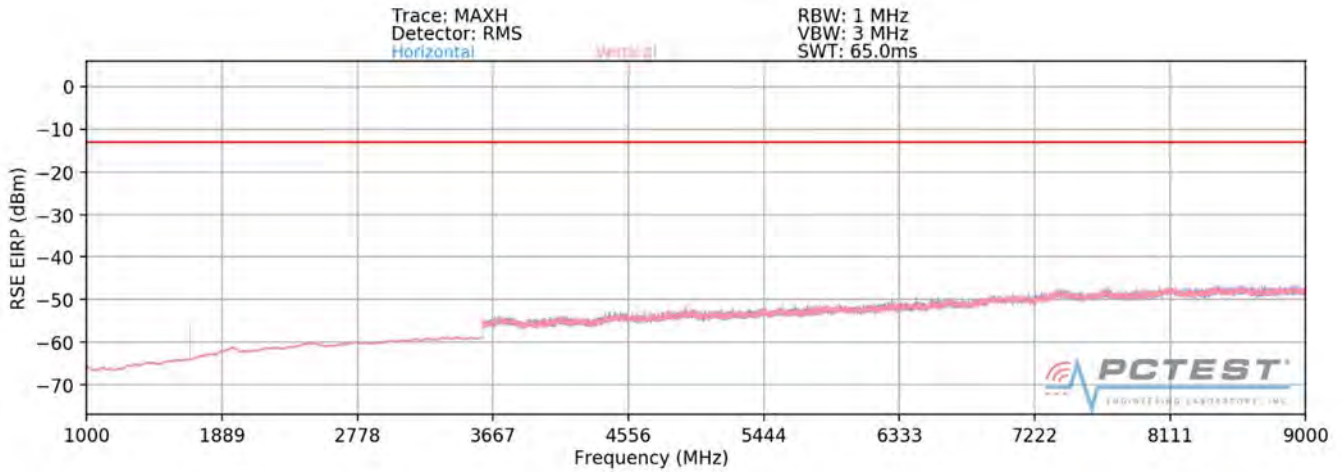
Plot 7-229. Radiated Spurious Plot above 1GHz (Band 5)
