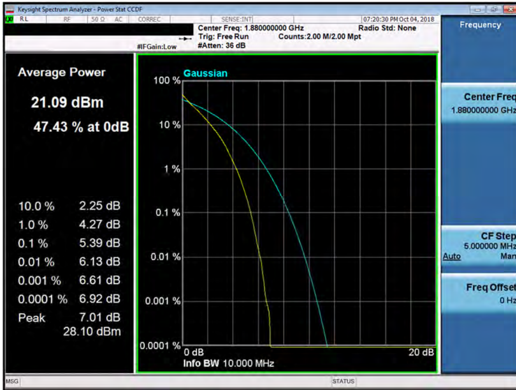
Plot 7-221. PAR Plot (Band 2 - 10.0MHz QPSK - Full RB Configuration)
