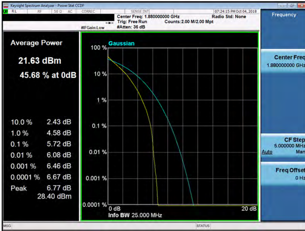
Plot 7-223. PAR Plot (Band 2 - 15.0MHz QPSK - Full RB Configuration)
