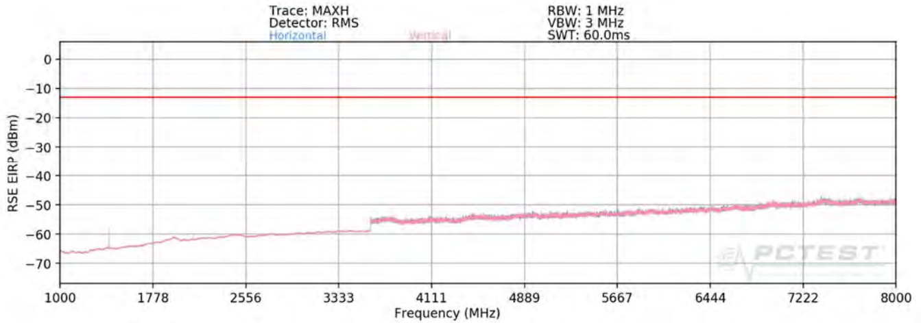
Plot 7-228. Radiated Spurious Plot above 1GHz (Band 12)
