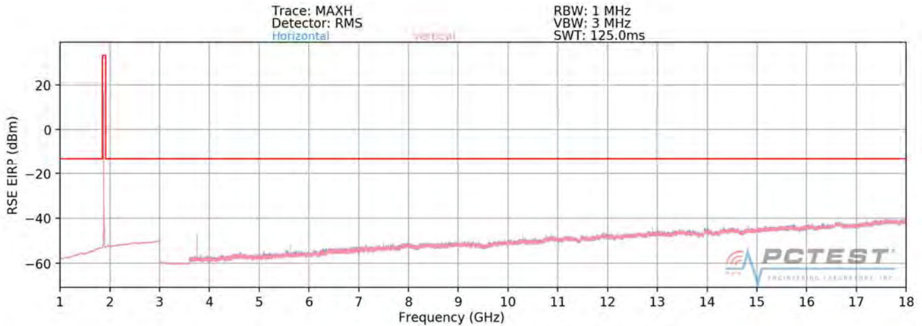
Plot 7-231. Radiated Spurious Plot above 1GHz (Band 2)
