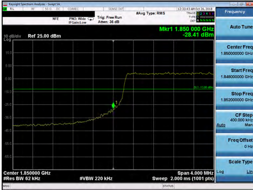
Plot 7-179. Lower Band Edge Plot (Band 2 – 5.0MHz QPSK - Full RB Configuration)
