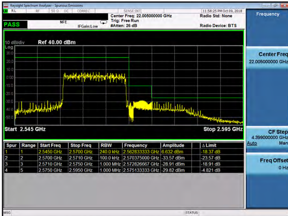
Plot 7-200. Upper ACP Plot (Band 7 - 15.0MHz QPSK - RB Size 75)
