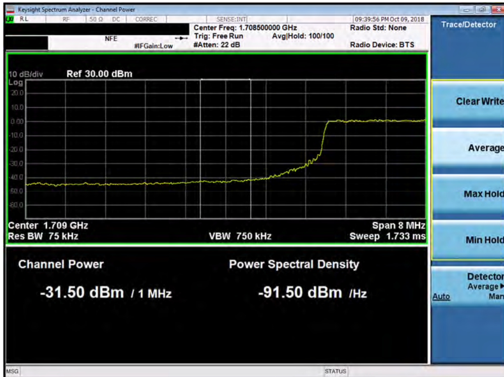
Plot 7-154. Lower Extended Band Edge Plot (Band 66/4 - 10.0MHz QPSK - Full RB Configuration)
