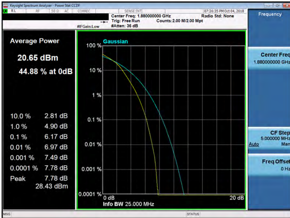
Plot 7-226. PAR Plot (Band 2 - 20.0MHz 16-QAM - Full RB Configuration)
