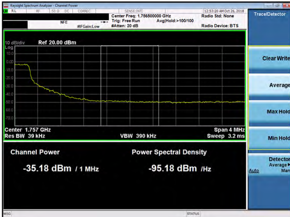
Plot 7-150. Upper Extended Band Edge Plot (Band 4 - 5.0MHz QPSK - Full RB Configuration)
