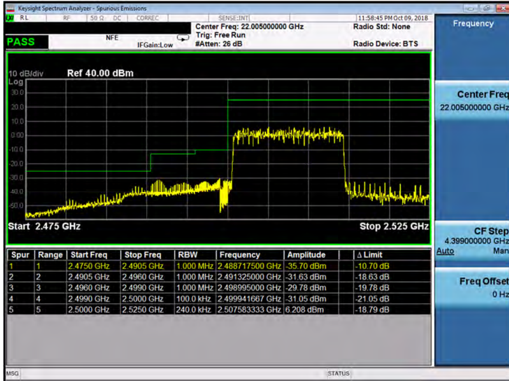
Plot 7-199. Lower ACP Plot (Band 7 - 15.0MHz QPSK - RB Size 75)
