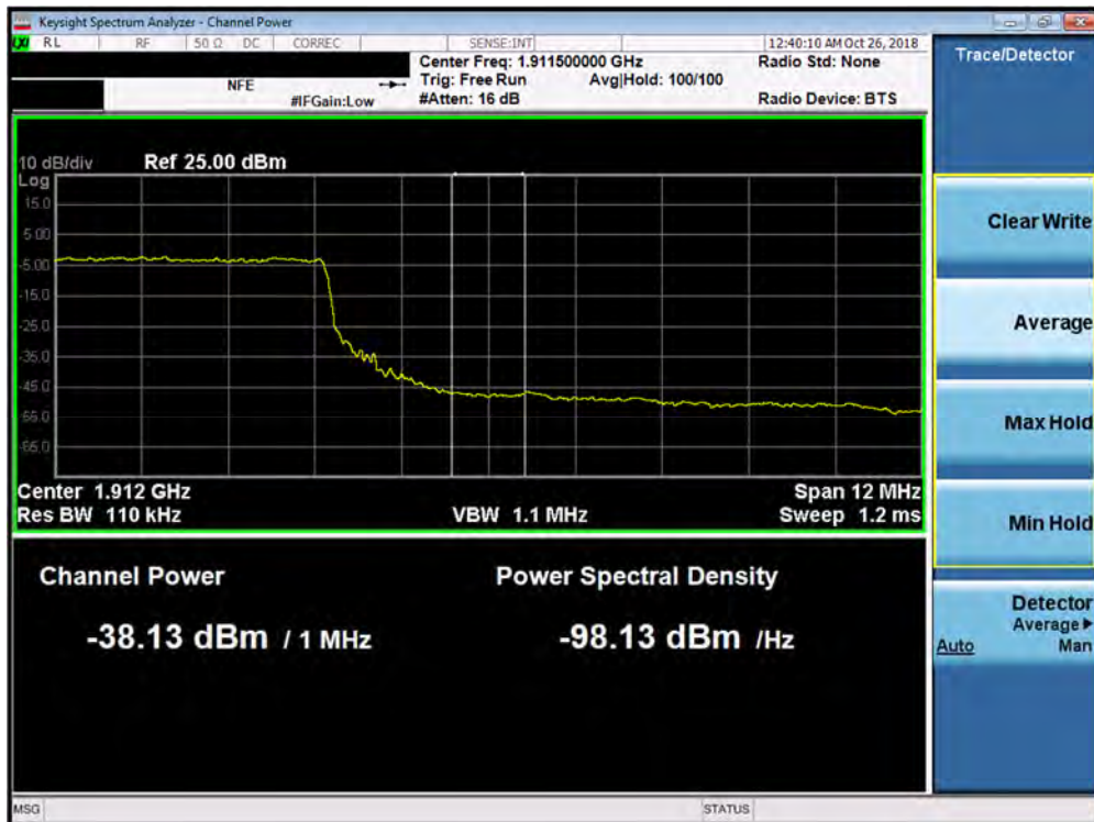
Plot 7-190. Upper Extended Band Edge Plot (Band 2 - 15.0MHz QPSK - Full RB Configuration)
