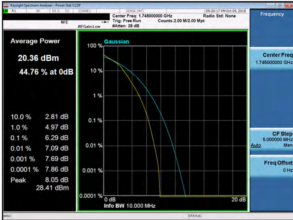
Plot 7-210. PAR Plot (Band 66/4 - 10.0MHz 16-QAM - Full RB Configuration)
