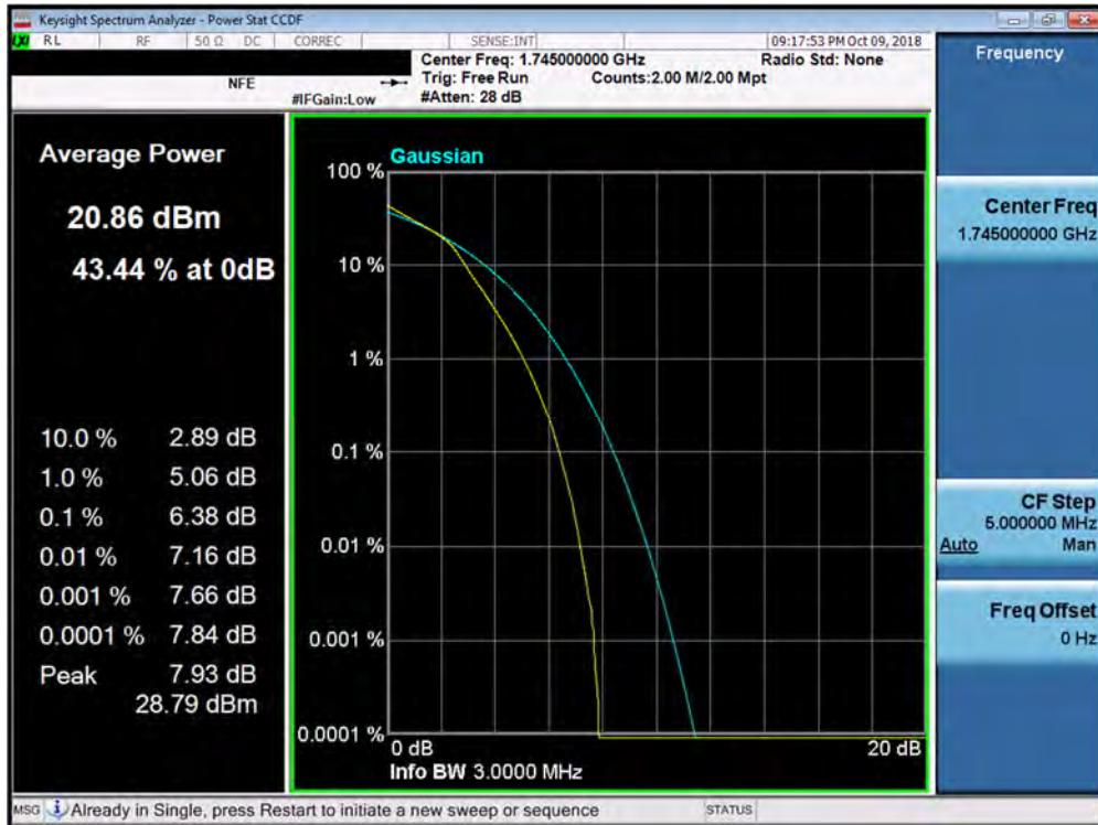
Plot 7-206. PAR Plot (Band 66/4 - 3.0MHz 16-QAM - Full RB Configuration)
