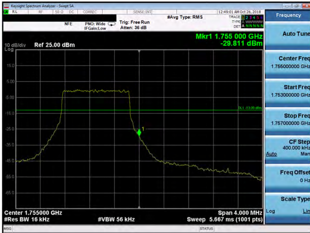
Plot 7-137. Upper Band Edge Plot (Band 4 - 1.4MHz QPSK - Full RB Configuration)
