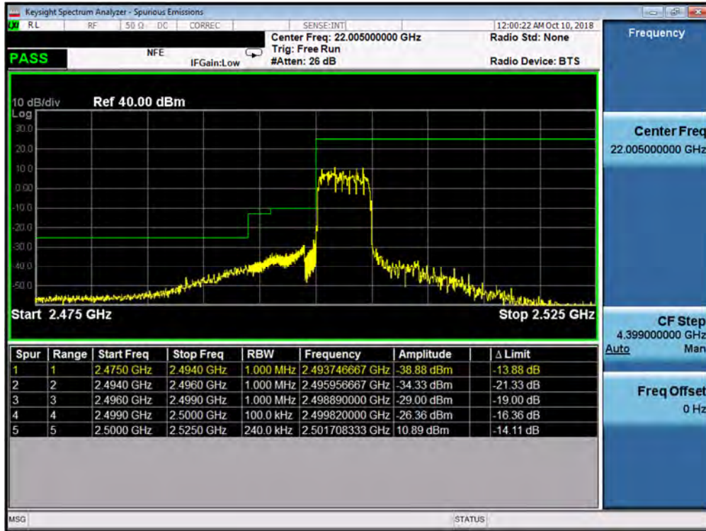
Plot 7-195. Lower ACP Plot (Band 7 - 5.0MHz QPSK - RB Size 25)
