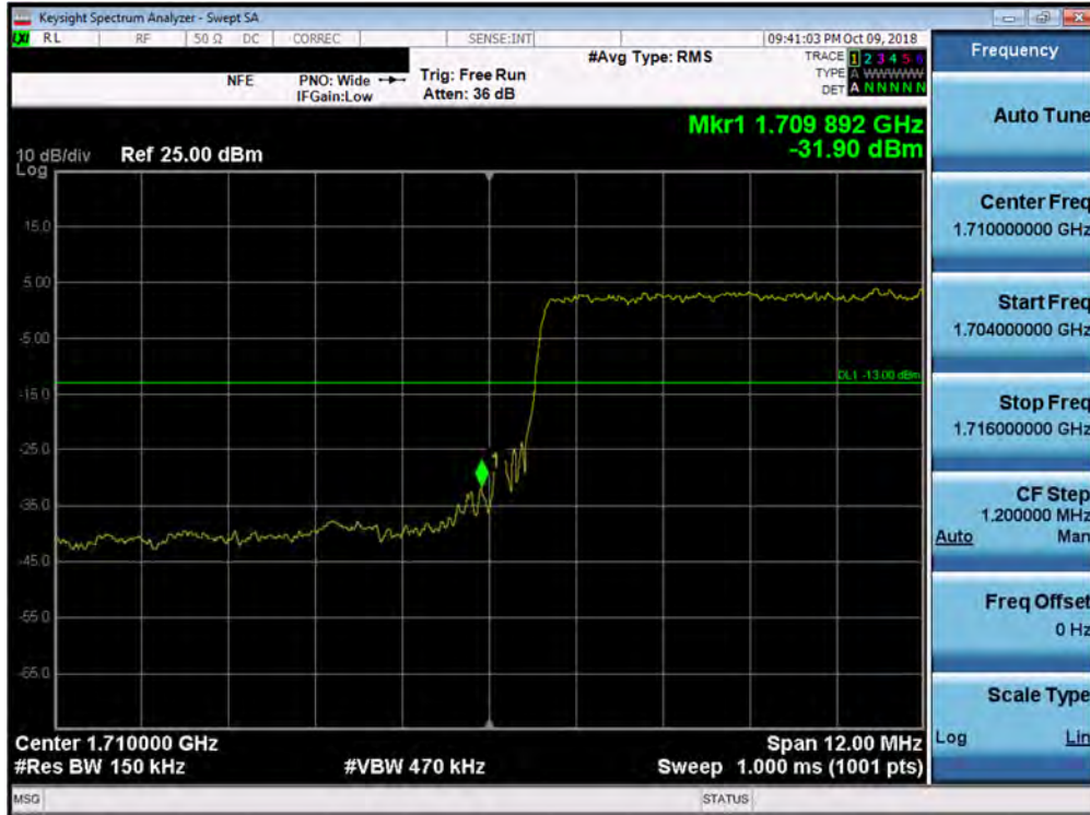
Plot 7-159. Lower Band Edge Plot (Band 66/4 - 15.0MHz QPSK - Full RB Configuration)
