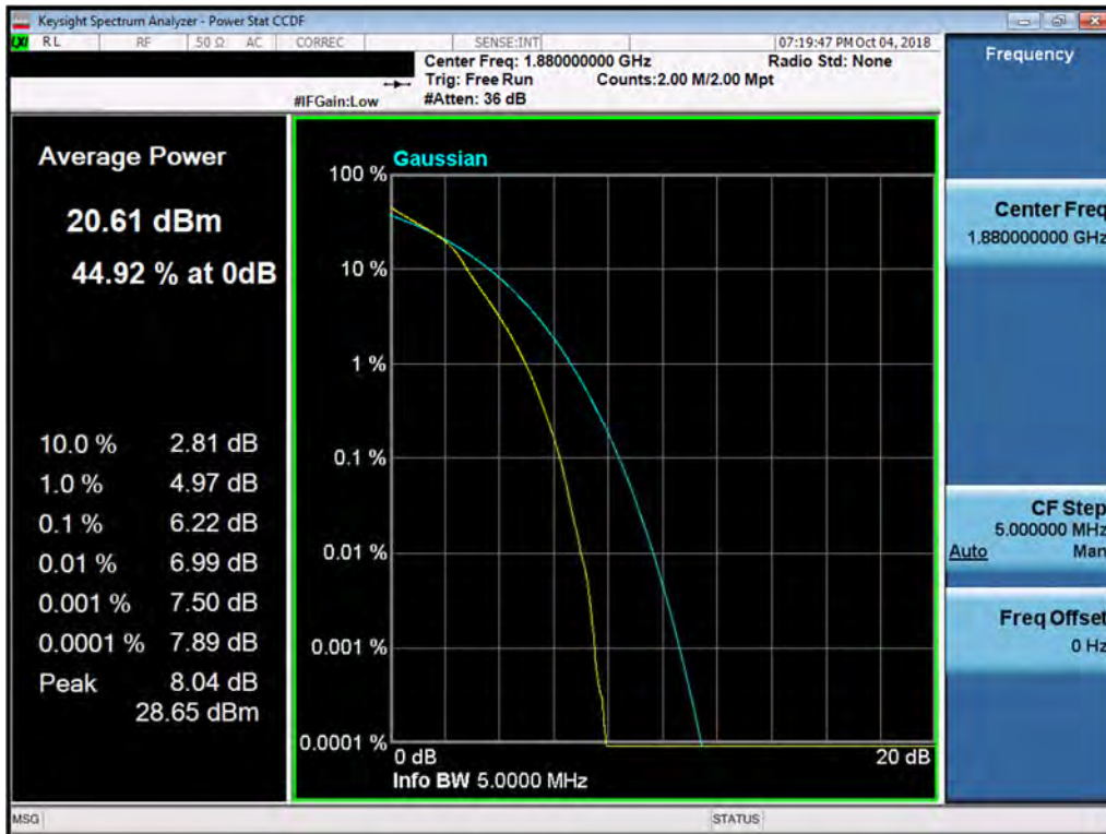
Plot 7-220. PAR Plot (Band 2 - 5.0MHz 16-QAM - Full RB Configuration)
