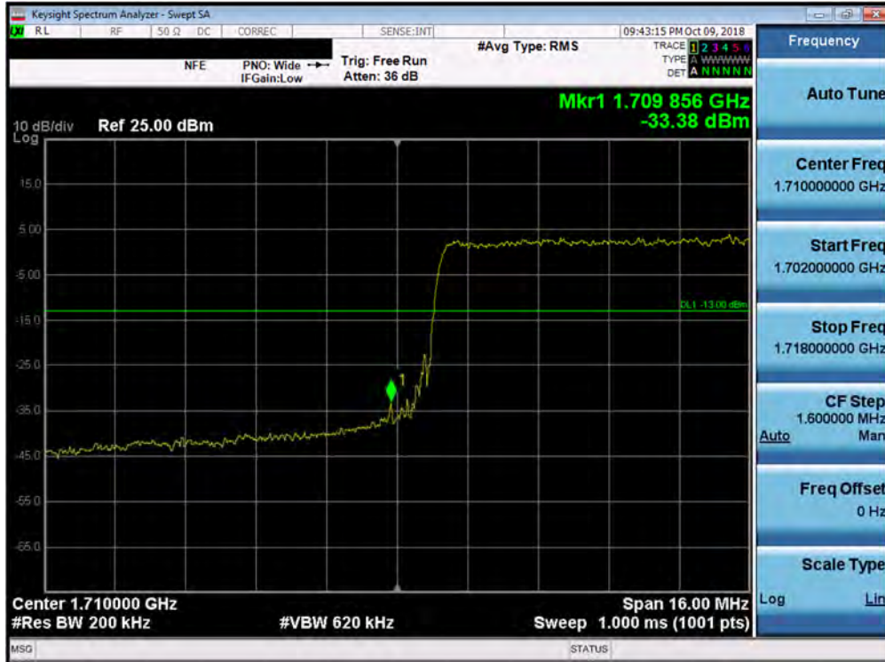
Plot 7-165. Lower Band Edge Plot (Band 66/4 - 20.0MHz QPSK - Full RB Configuration)
