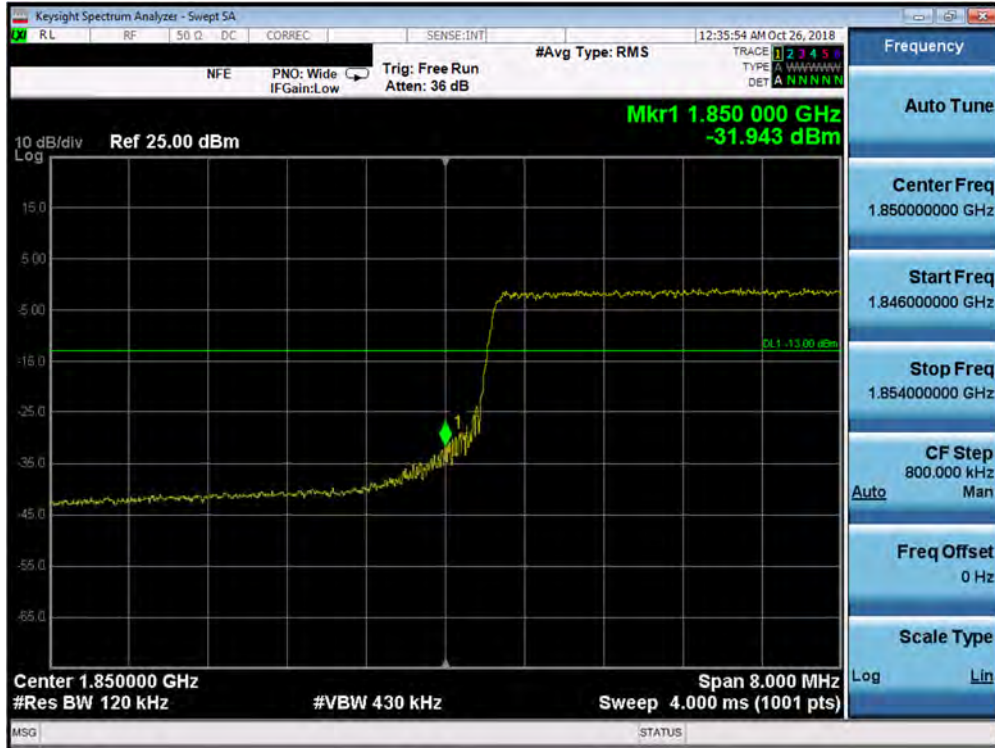
Plot 7-183. Lower Band Edge Plot (Band 2 –10.0MHz QPSK - Full RB Configuration)
