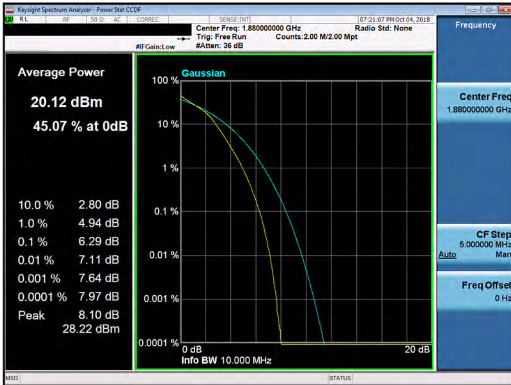
Plot 7-222. PAR Plot (Band 2 - 10.0MHz 16-QAM - Full RB Configuration)
