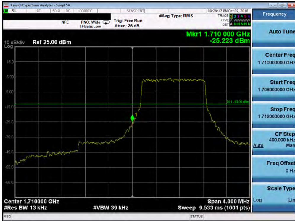
Plot 7-135. Lower Band Edge Plot (Band 66/4 - 1.4MHz QPSK - Full RB Configuration)
