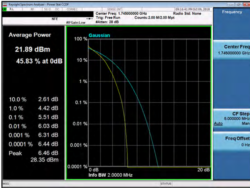
Plot 7-203. PAR Plot (Band 66/4 - 1.4MHz QPSK - Full RB Configuration)
