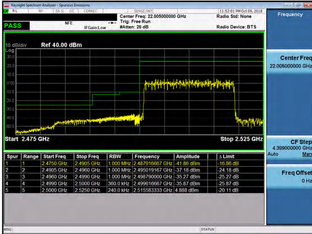
Plot 7-201. Lower ACP Plot (Band 7 - 20.0MHz QPSK - RB Size 100)
