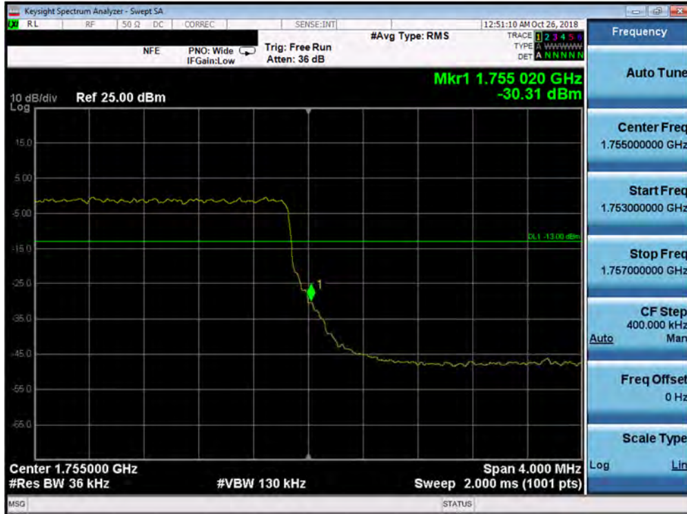
Plot 7-143. Upper Band Edge Plot (Band 4 - 3.0MHz QPSK - Full RB Configuration)
