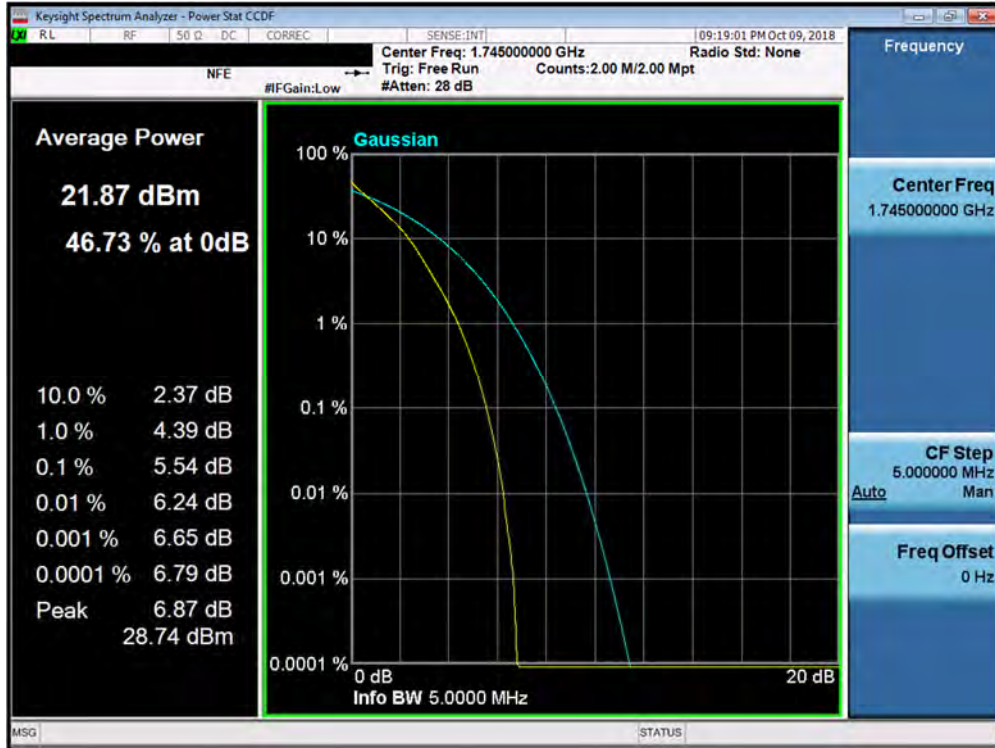
Plot 7-207. PAR Plot (Band 66/4 - 5.0MHz QPSK - Full RB Configuration)
