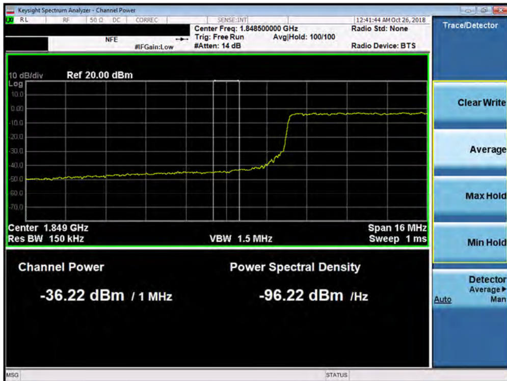
Plot 7-192. Lower Extended Band Edge Plot (Band 2 – 20.0MHz QPSK - Full RB Configuration)
