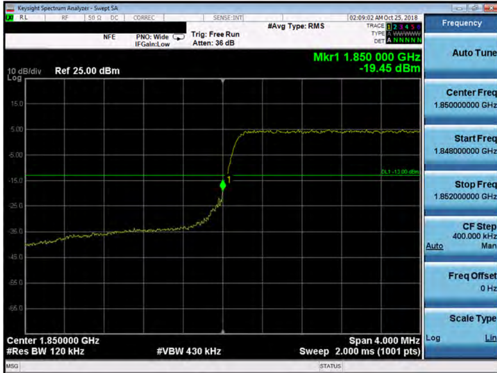
Plot 7-175. Lower Band Edge Plot (Band 2 –3.0MHz QPSK - Full RB Configuration)
