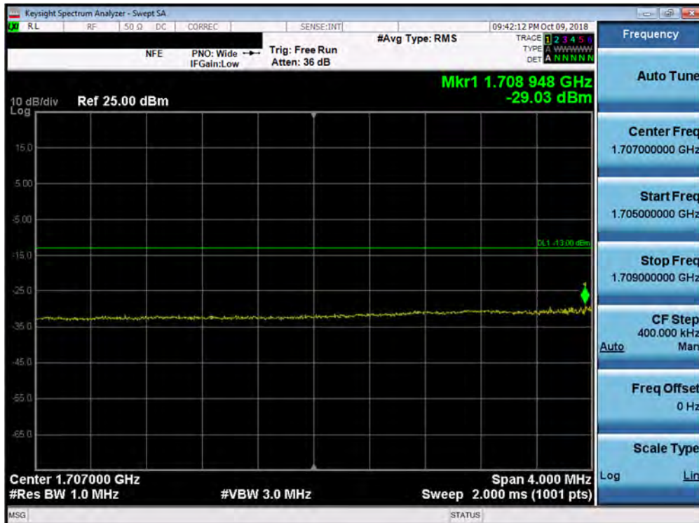
Plot 7-160. Lower Extended Band Edge Plot (Band 66/4 - 15.0MHz QPSK - Full RB Configuration)
