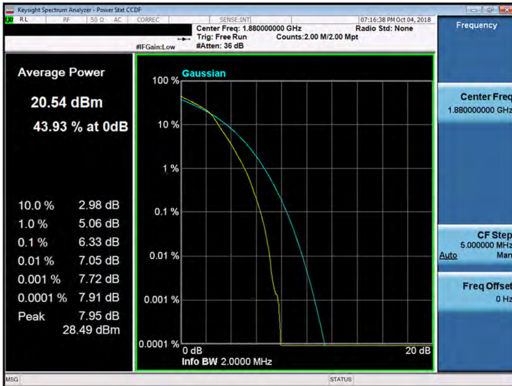
Plot 7-216. PAR Plot (Band 2 - 1.4MHz 16-QAM - Full RB Configuration)
