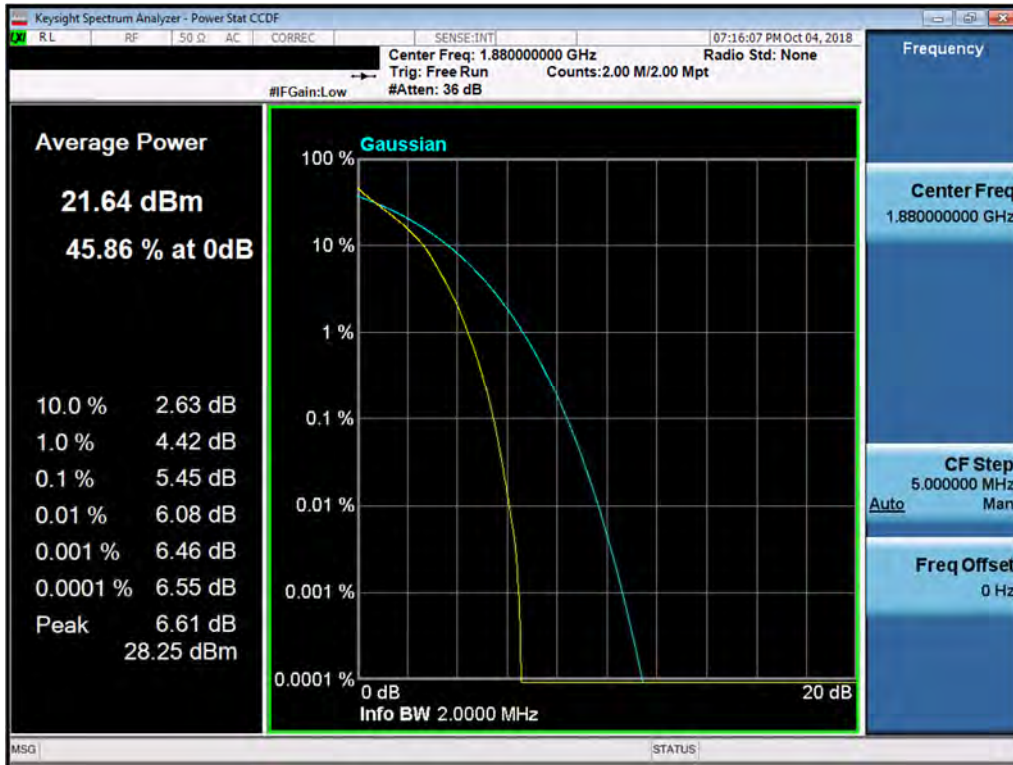
Plot 7-215. PAR Plot (Band 2 - 1.4MHz QPSK - Full RB Configuration)
