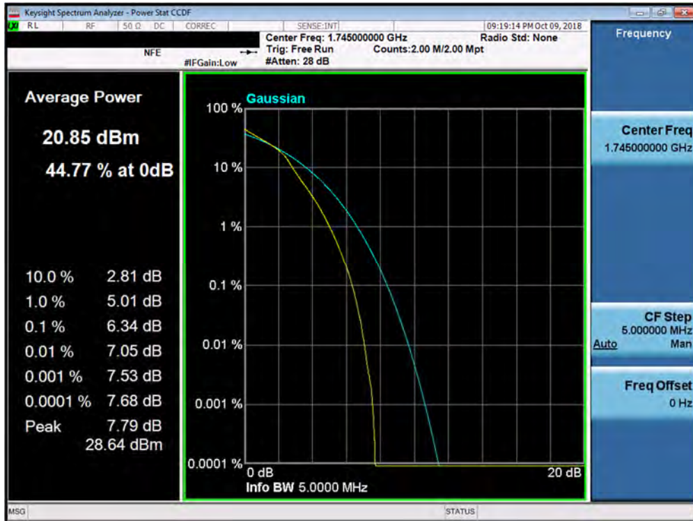
Plot 7-208. PAR Plot (Band 66/4 - 5.0MHz 16-QAM - Full RB Configuration)
