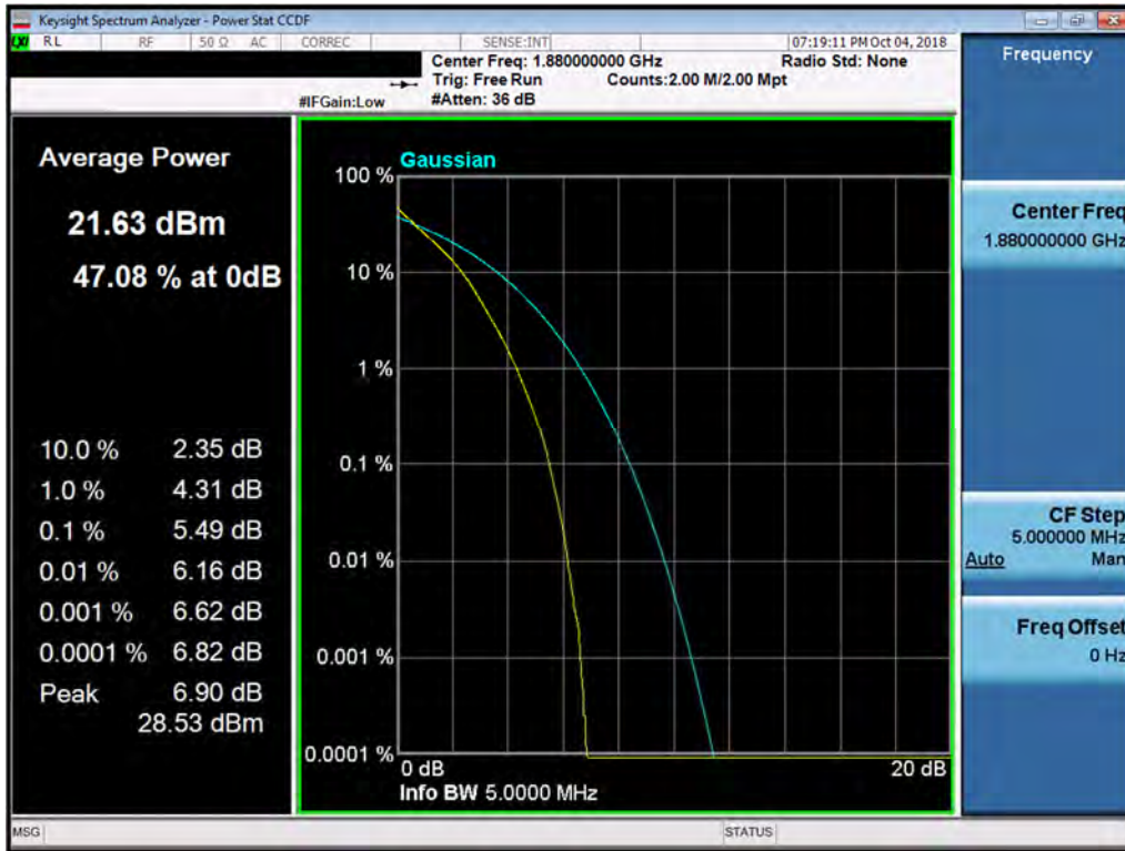
Plot 7-219. PAR Plot (Band 2 - 5.0MHz QPSK - Full RB Configuration)
