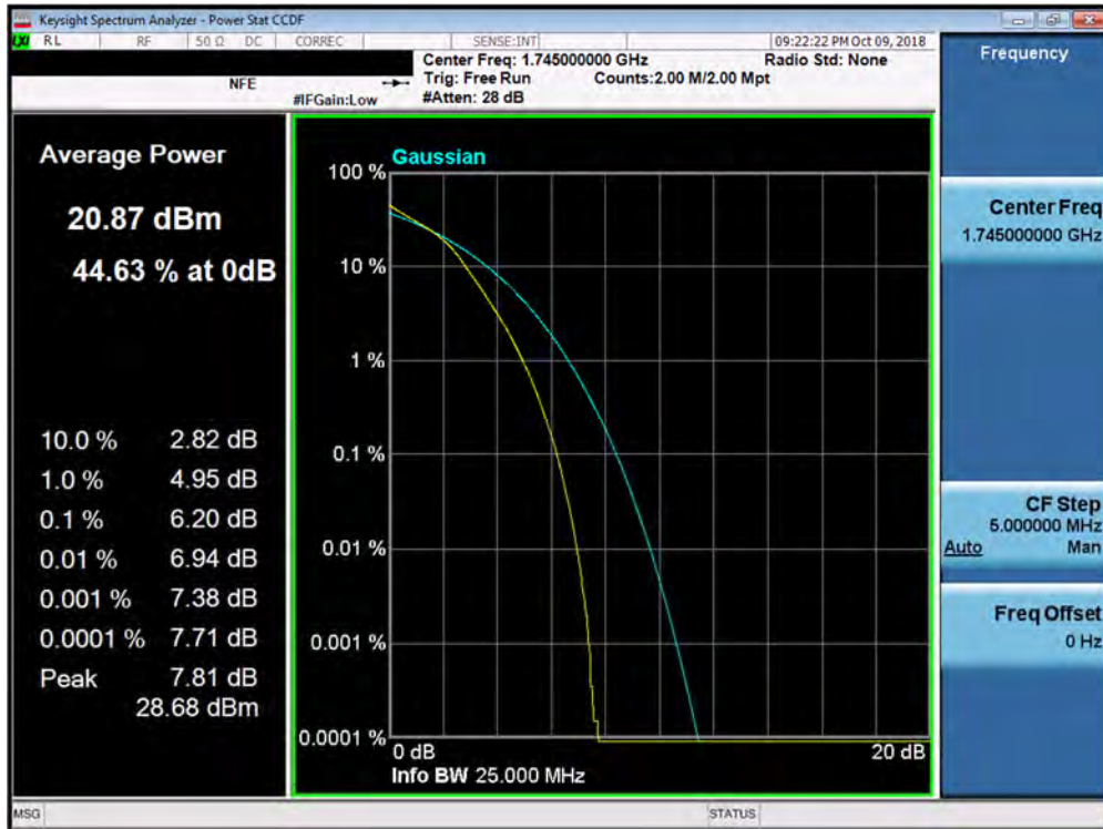
Plot 7-214. PAR Plot (Band 66/4 - 20.0MHz 16-QAM - Full RB Configuration)
