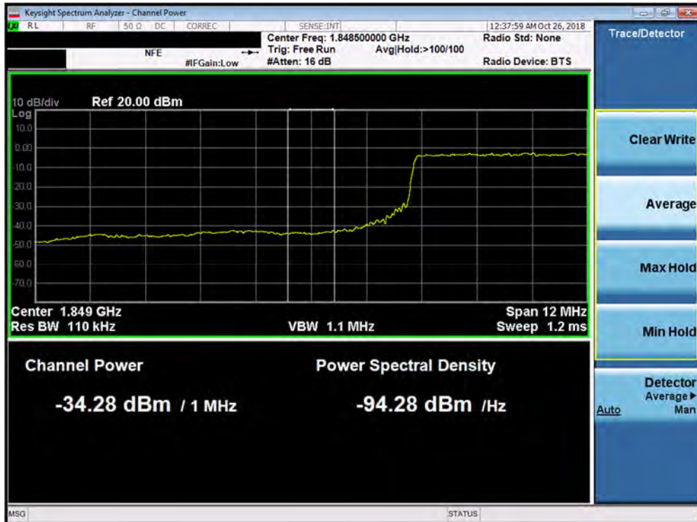
Plot 7-188. Lower Extended Band Edge Plot (Band 2 – 15.0MHz QPSK - Full RB Configuration)
