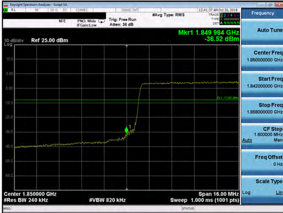
Plot 7-191. Lower Band Edge Plot (Band 2 – 20.0MHz QPSK - Full RB Configuration)
