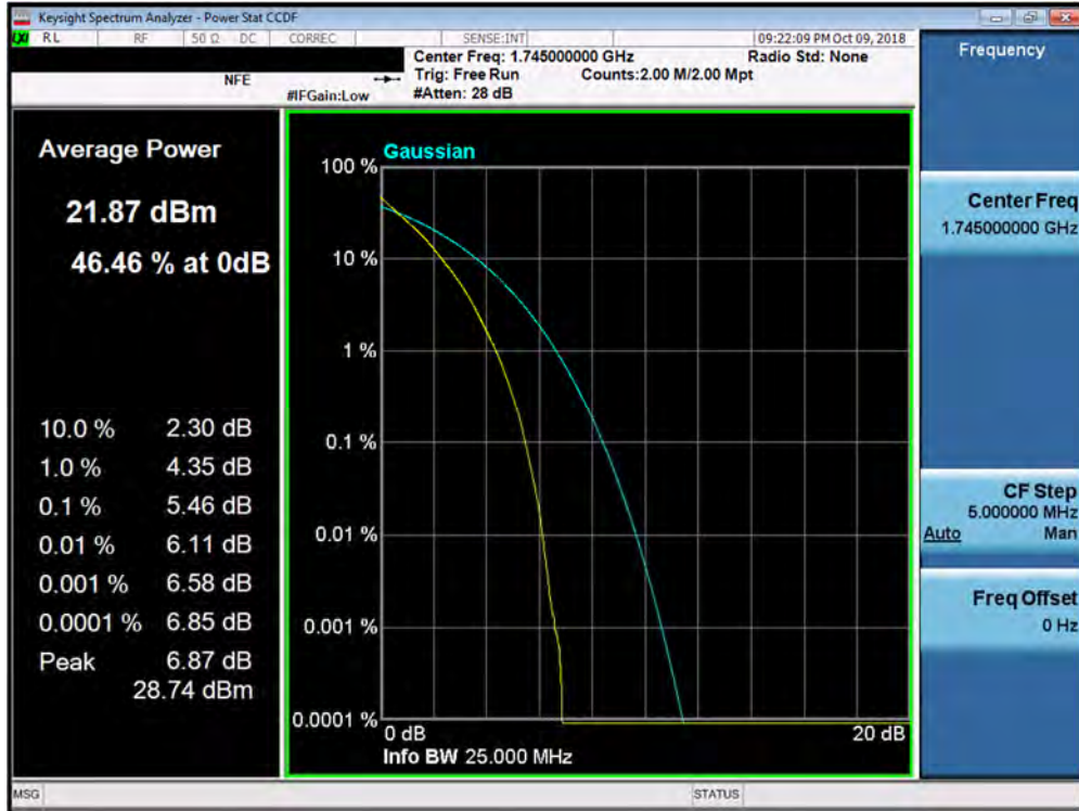
Plot 7-213. PAR Plot (Band 66/4 - 20.0MHz QPSK - Full RB Configuration)
