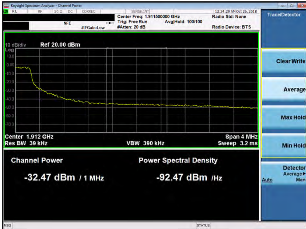
Plot 7-182. Upper Extended Band Edge Plot (Band 2 – 5.0MHz QPSK - Full RB Configuration)
