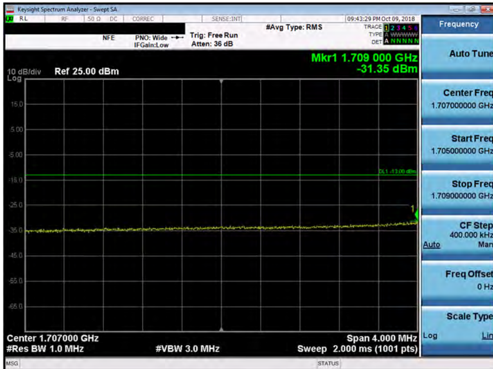
Plot 7-166. Lower Extended Band Edge Plot (Band 66/4 - 20.0MHz QPSK - Full RB Configuration)
