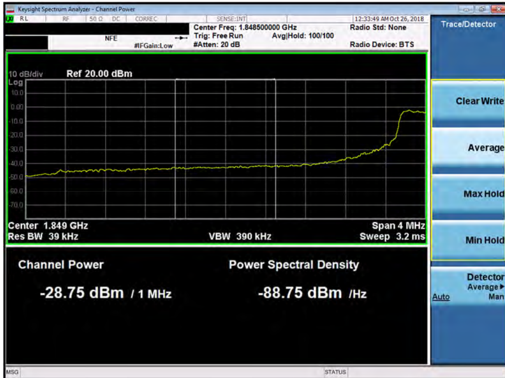
Plot 7-180. Lower Extended Band Edge Plot (Band 2 – 5.0MHz QPSK - Full RB Configuration)
