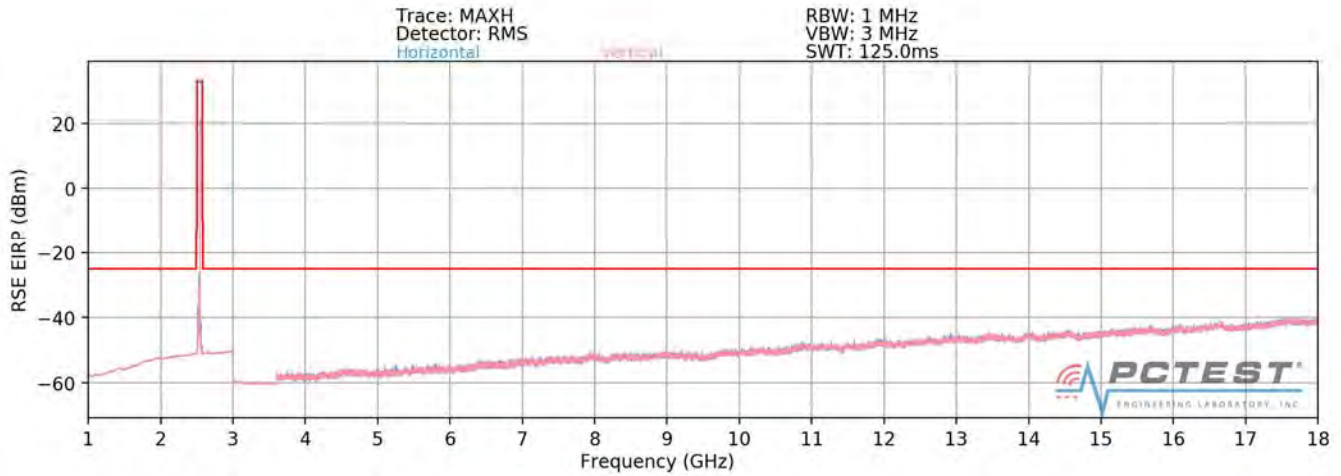
Plot 7-232. Radiated Spurious Plot above 1GHz (Band 7)
