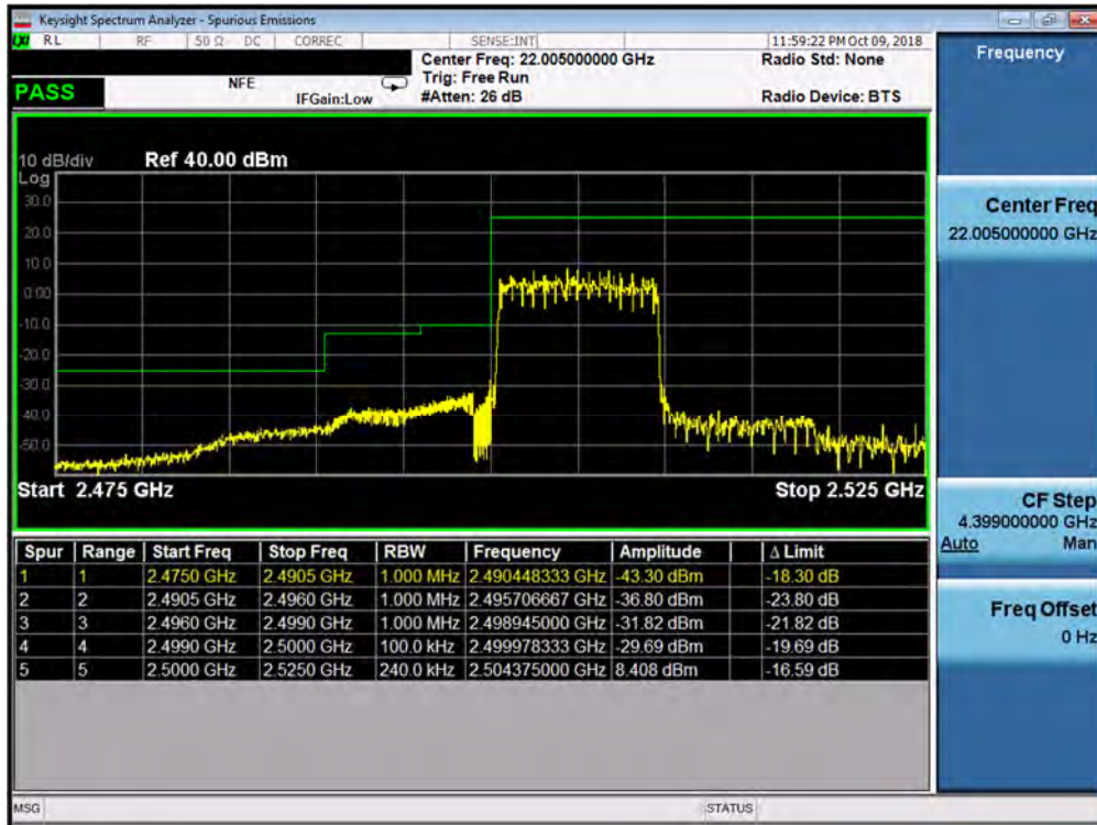
Plot 7-197. Lower ACP Plot (Band 7 - 10.0MHz QPSK - RB Size 50)
