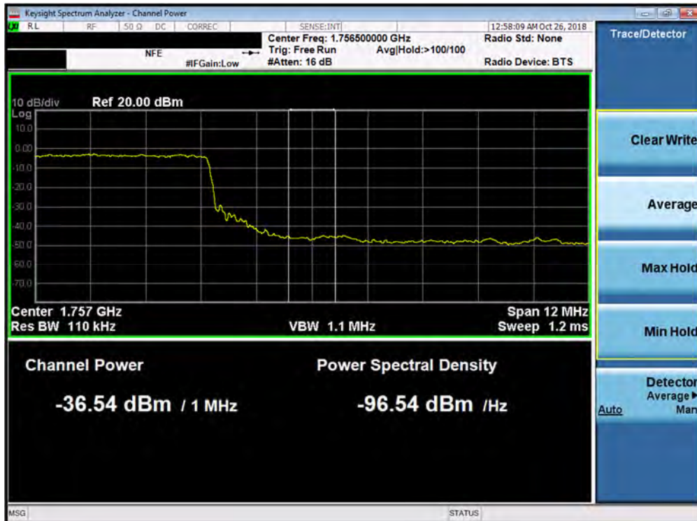
Plot 7-162. Upper Extended Band Edge Plot (Band 4 - 15.0MHz QPSK - Full RB Configuration)
