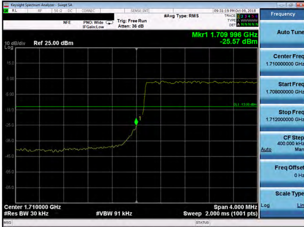
Plot 7-141. Lower Band Edge Plot (Band 66/4 - 3.0MHz QPSK - Full RB Configuration)
