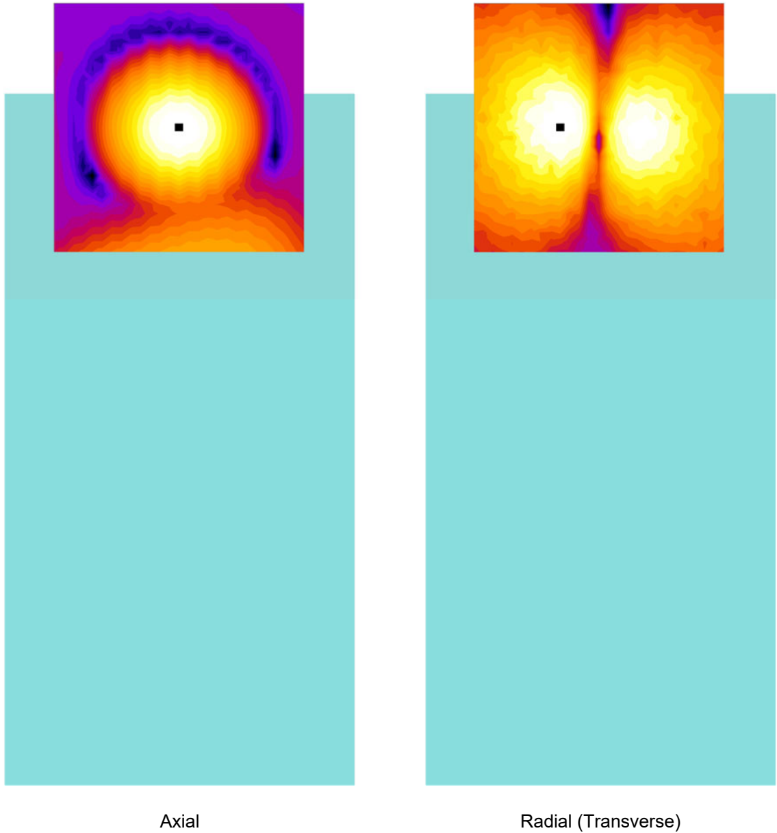
Axial Radial (Transverse) Figure 9-1 T-Coil Scan Overlay Magnetic Field Distributions
