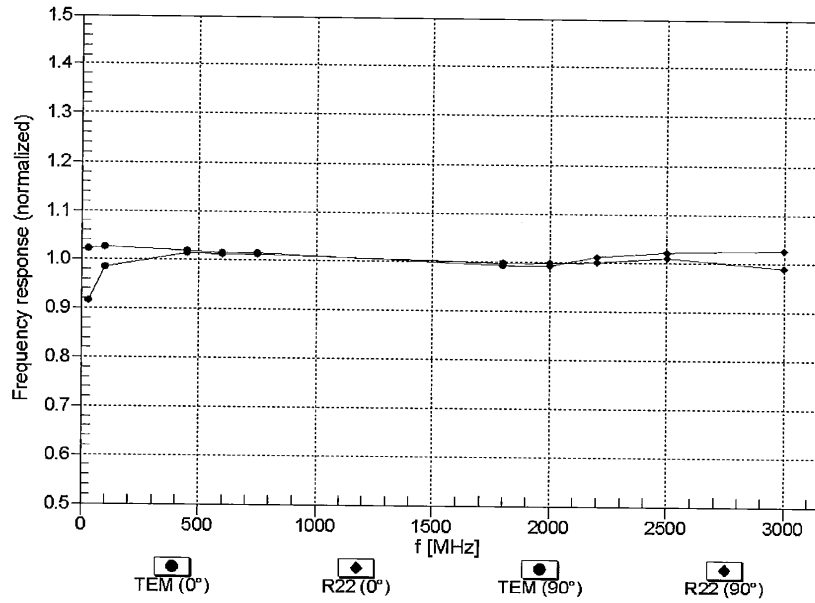
Uncertainty of Frequency Response of E-field: ± 6.3% (k=2)
