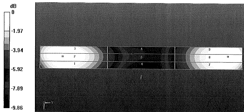
0 dB = 107.4 V/m = 40.62 dBV/m
