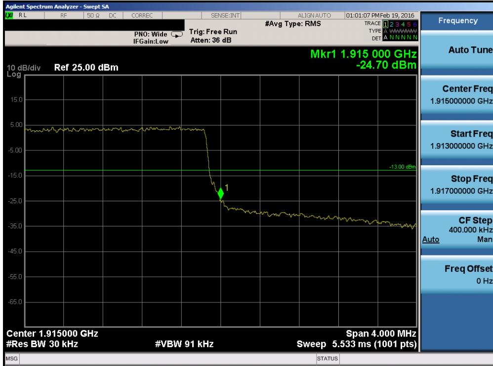
Plot 7-74. Upper Band Edge Plot (Band 25 – 3.0MHz QPSK – RB Size 15)
