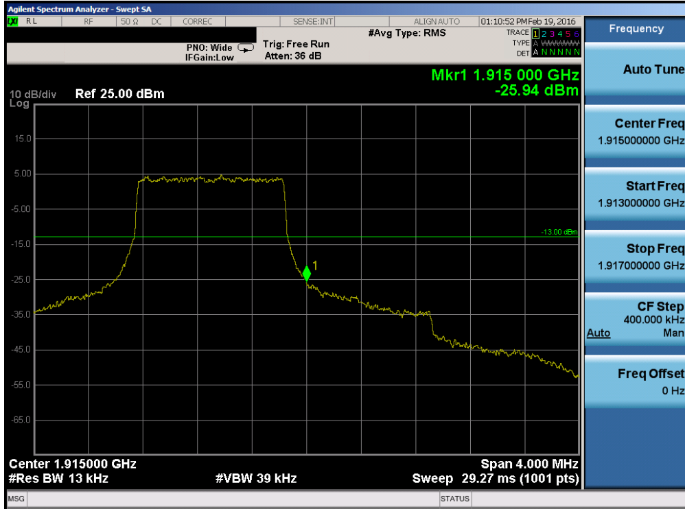
Plot 7-70. Upper Band Edge Plot (Band 25 – 1.4MHz QPSK – RB Size 6)
