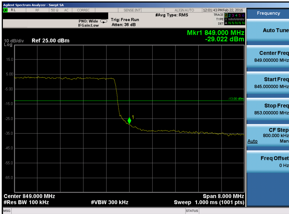
Plot 7-65. Upper Band Edge Plot (Band 26 – 10.0MHz QPSK – RB Size 50)
