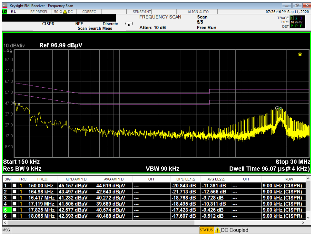
Plot 7-26. Line Conducted Plot with Bluetooth LE (N)
