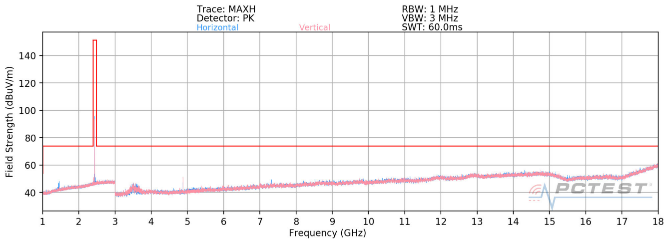
Plot 7-19. Radiated Spurious Plot above 1GHz (BT- Ch. 39)
