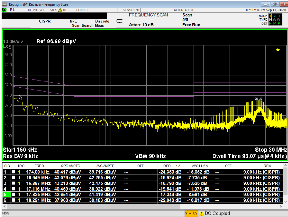
Plot 7-25. Line Conducted Plot with Bluetooth LE (L1)
