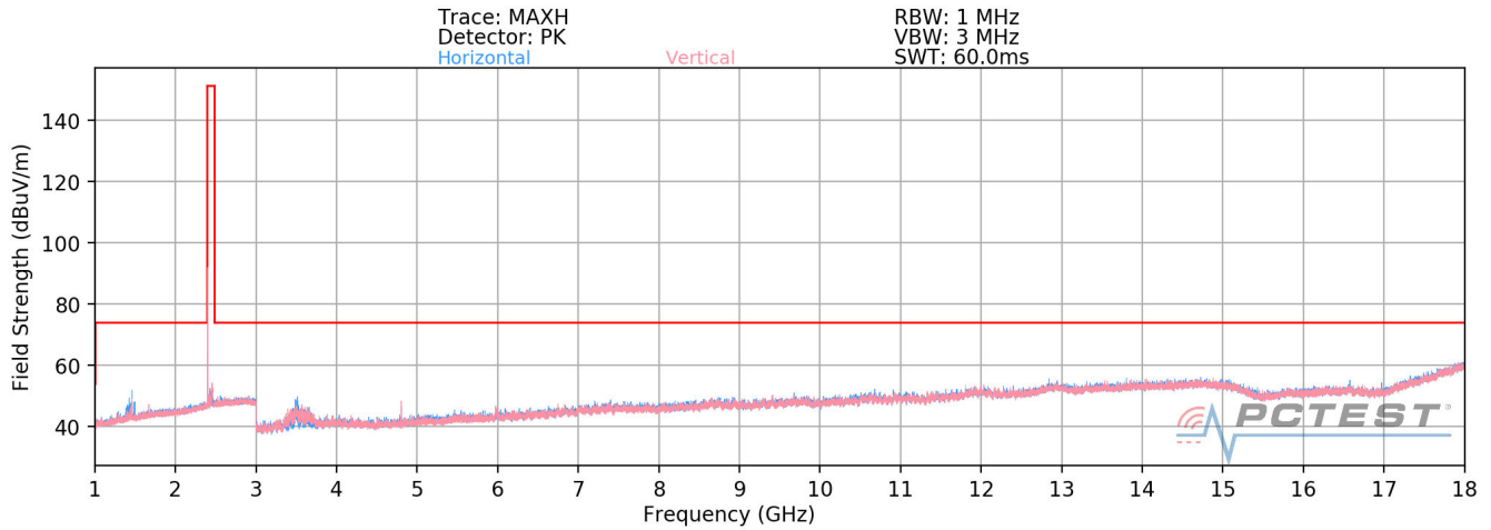
Plot 7-18. Radiated Spurious Plot above 1GHz (BT- Ch. 0)
