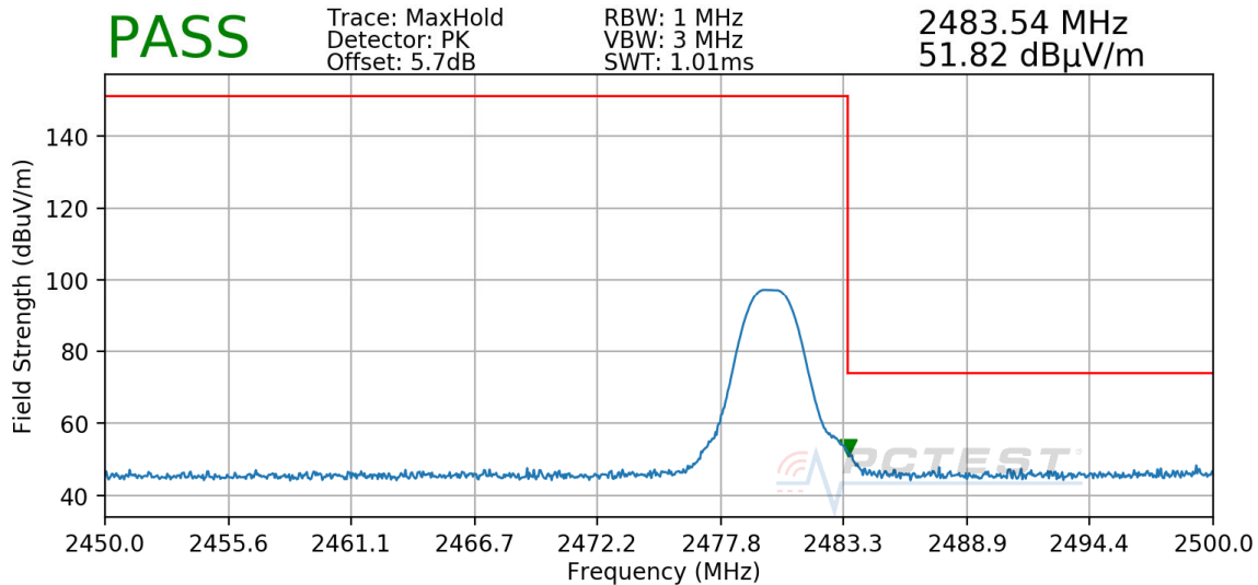
Plot 7-23. Radiated Restricted Upper Band Edge Measurement (Peak)
