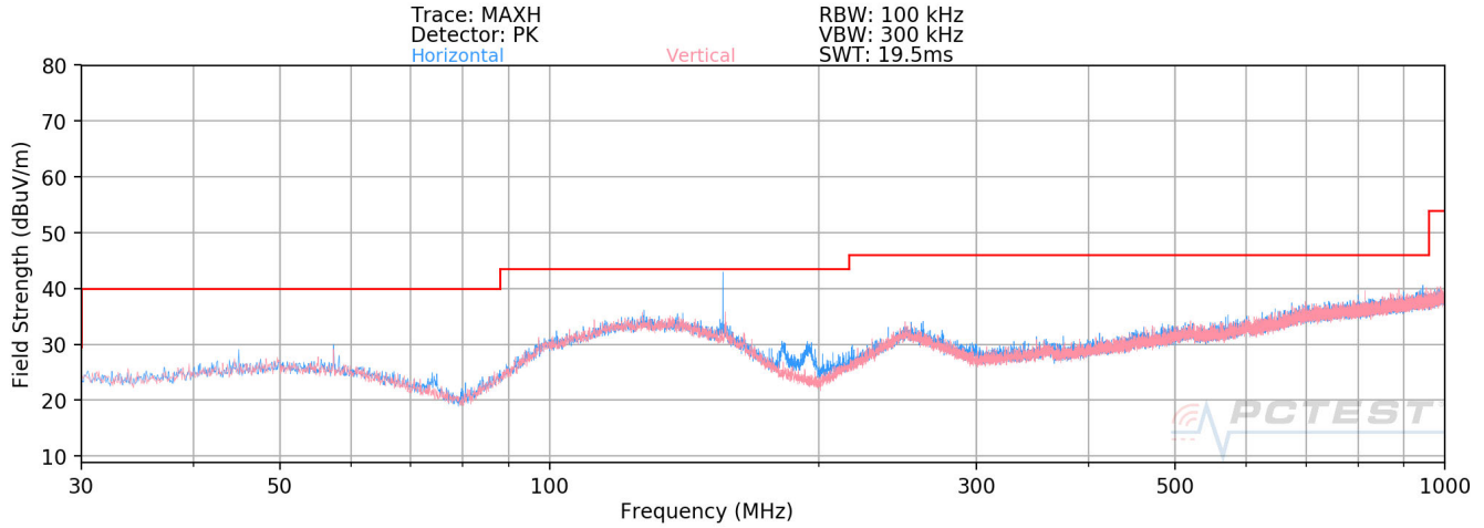
Plot 7-24. Radiated Spurious Plot below 1GHz
