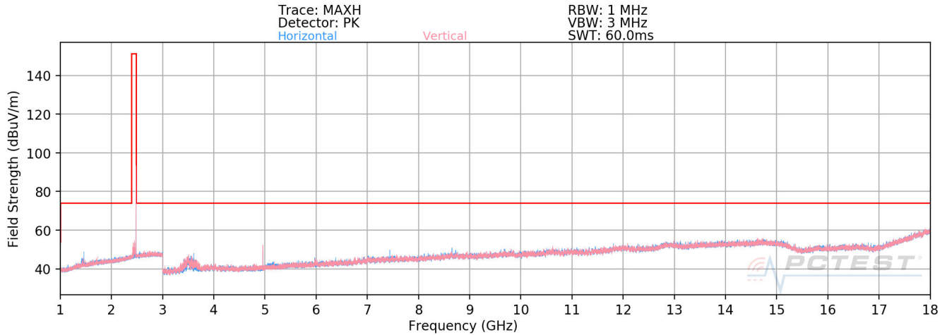
Plot 7-20. Radiated Spurious Plot above 1GHz (BT- Ch. 78)
