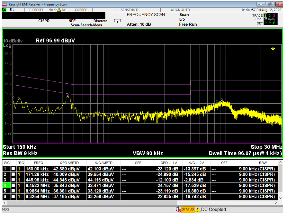
Plot 7-21. Line Conducted Plot with BluetoWoth LE (L1)
