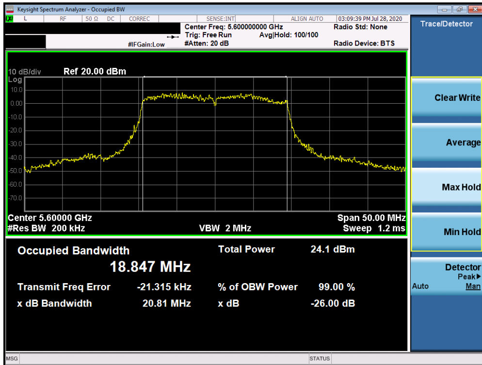
Plot 7-38. 26dB Bandwidth Plot ANT3 (20MHz BW 802.11ax (UNII Band 2C) – Ch. 120)
