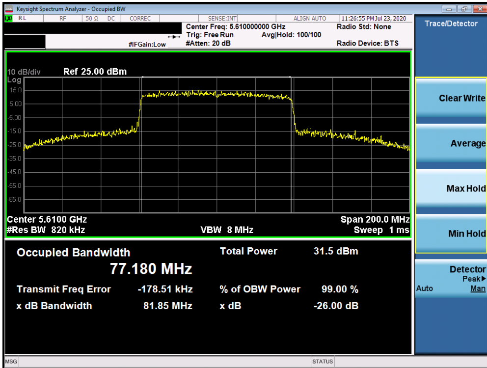
Plot 7-101. 26dB Bandwidth Plot ANT4 (80MHz BW 802.11ax (UNII Band 2C) – Ch. 122)
