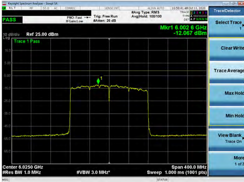
Plot 7-117. Power Spectral Density Plot MIMO ANT1 (160MHz BW 802.11ax (UNII Band 5) – Ch. 15)
