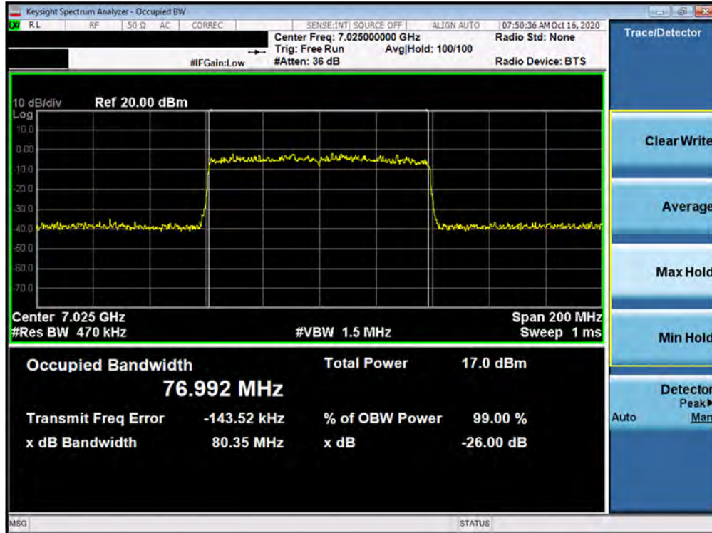
Plot 7-103. 26dB Bandwidth Plot MIMO ANT2 (80MHz BW 802.11ax (UNII Band 8) – Ch. 215)
