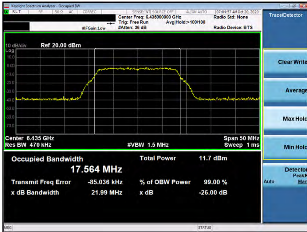
Plot 7-16. 26dB Bandwidth Plot MIMO ANT1 (802.11a (UNII Band 6) – Ch. 97)
