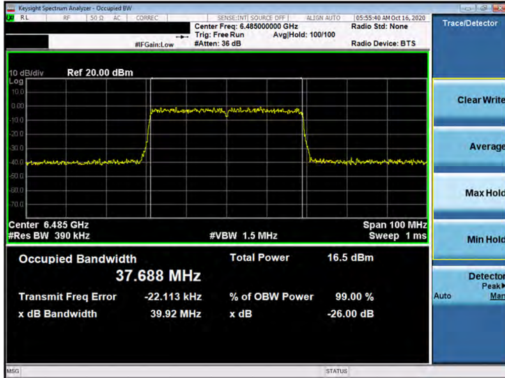
Plot 7-75. 26dB Bandwidth Plot MIMO ANT2 (40MHz BW 802.11ax (UNII Band 6) – Ch. 107)
