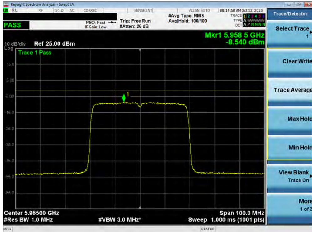
Plot 7-111. Power Spectral Density Plot MIMO ANT1 (40MHz BW 802.11ax (UNII Band 5) – Ch. 3)
