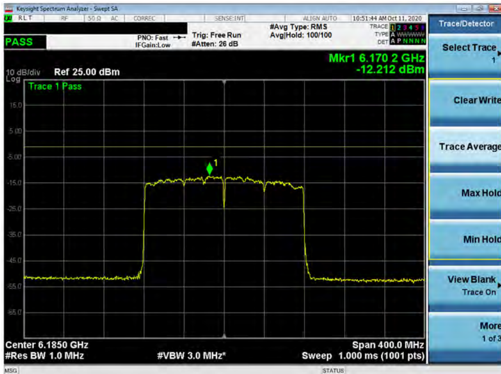
Plot 7-118. Power Spectral Density Plot MIMO ANT1 (160MHz BW 802.11ax (UNII Band 5) – Ch. 47)
