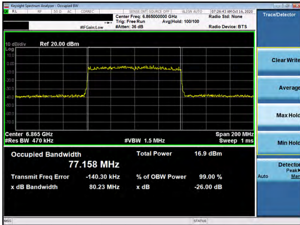
Plot 7-90. 26dB Bandwidth Plot MIMO ANT2 (80MHz BW 802.11ax (UNII Band 7) – Ch. 183)
