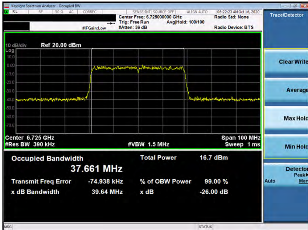
Plot 7-86. 26dB Bandwidth Plot MIMO ANT2 (40MHz BW 802.11ax (UNII Band 7) – Ch. 155)
