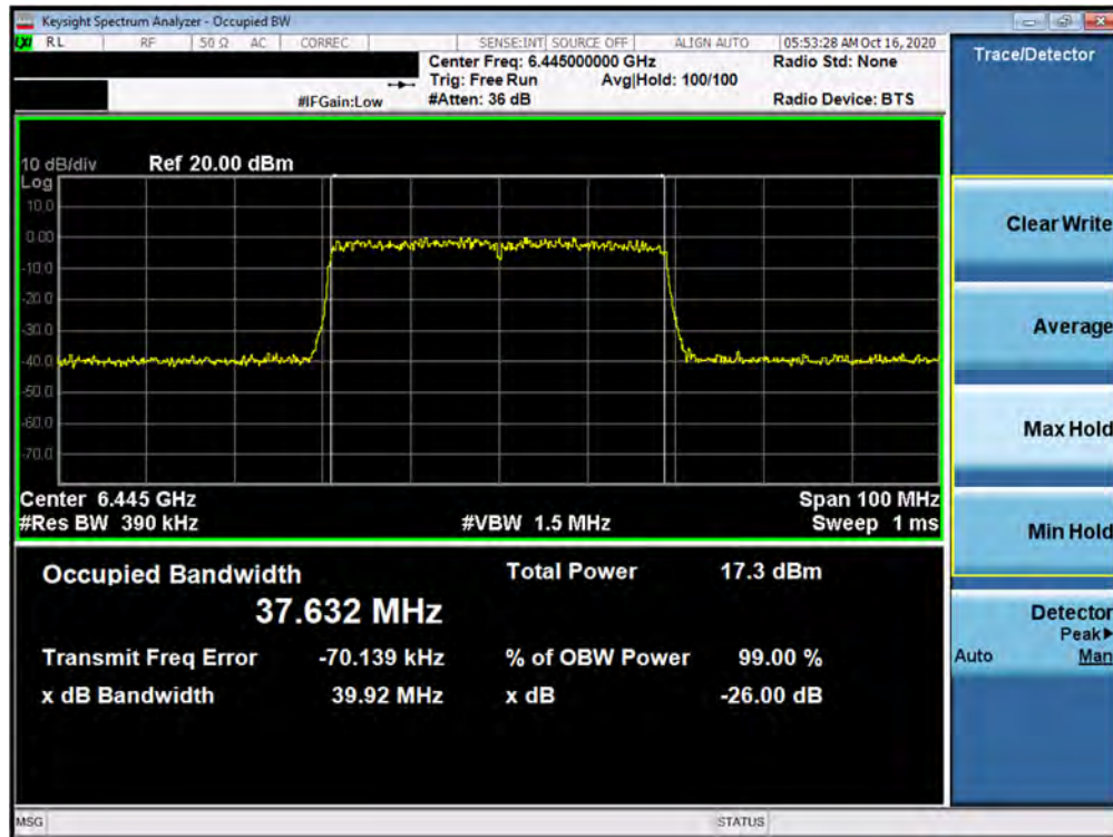
Plot 7-74. 26dB Bandwidth Plot MIMO ANT2 (40MHz BW 802.11ax (UNII Band 6) – Ch. 99)
