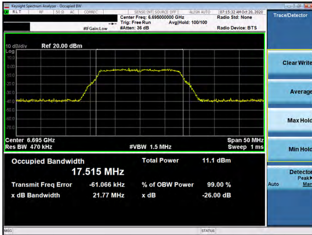
Plot 7-28. 26dB Bandwidth Plot MIMO ANT1 (802.11a (UNII Band 7) – Ch. 149)
