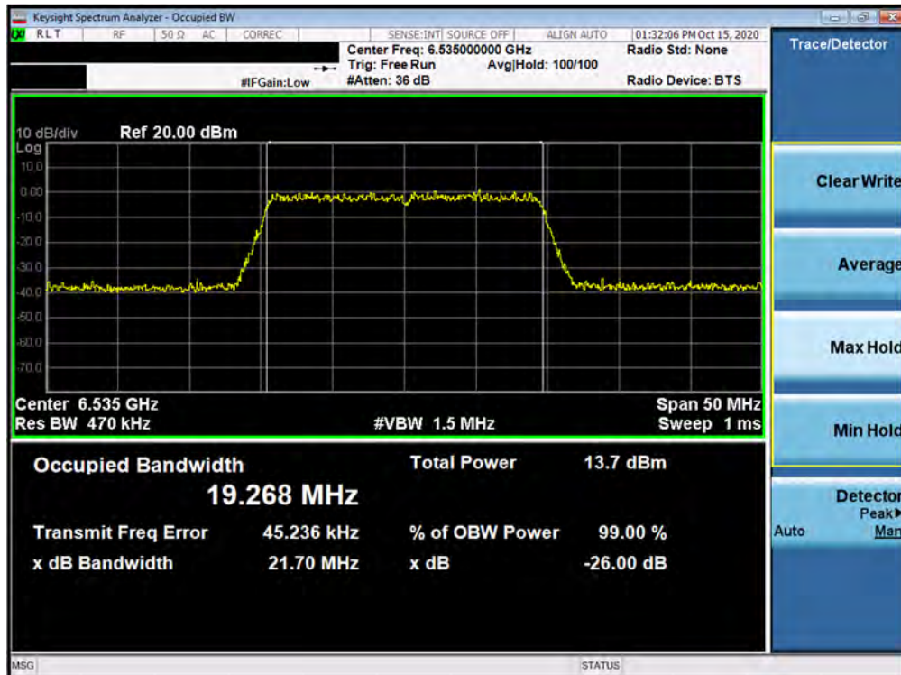
Plot 7-82. 26dB Bandwidth Plot MIMO ANT2 (20MHz BW 802.11ax (UNII Band 7) – Ch. 117)
