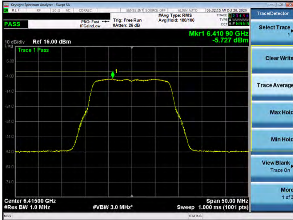
Plot 7-107. Power Spectral Density Plot MIMO ANT1 (802.11a (UNII Band 5) – Ch. 93)
