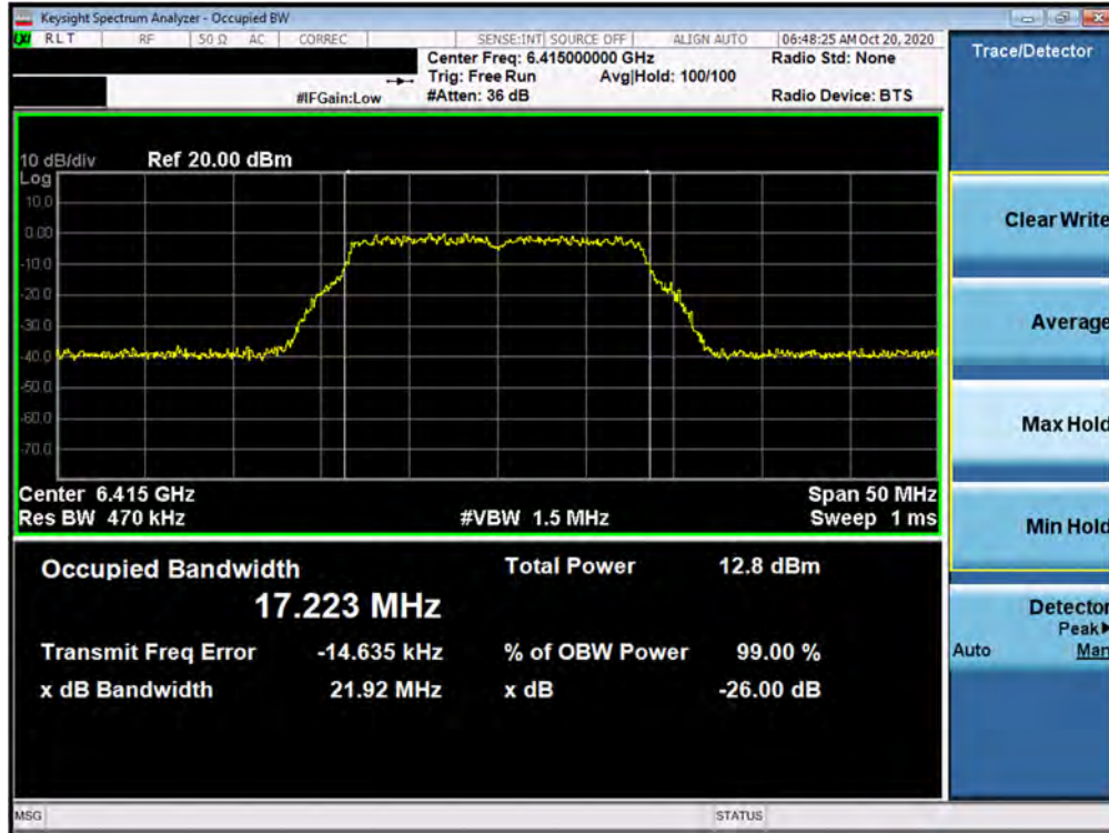
Plot 7-55. 26dB Bandwidth Plot MIMO ANT2 (802.11a (UNII Band 5) – Ch. 93)
