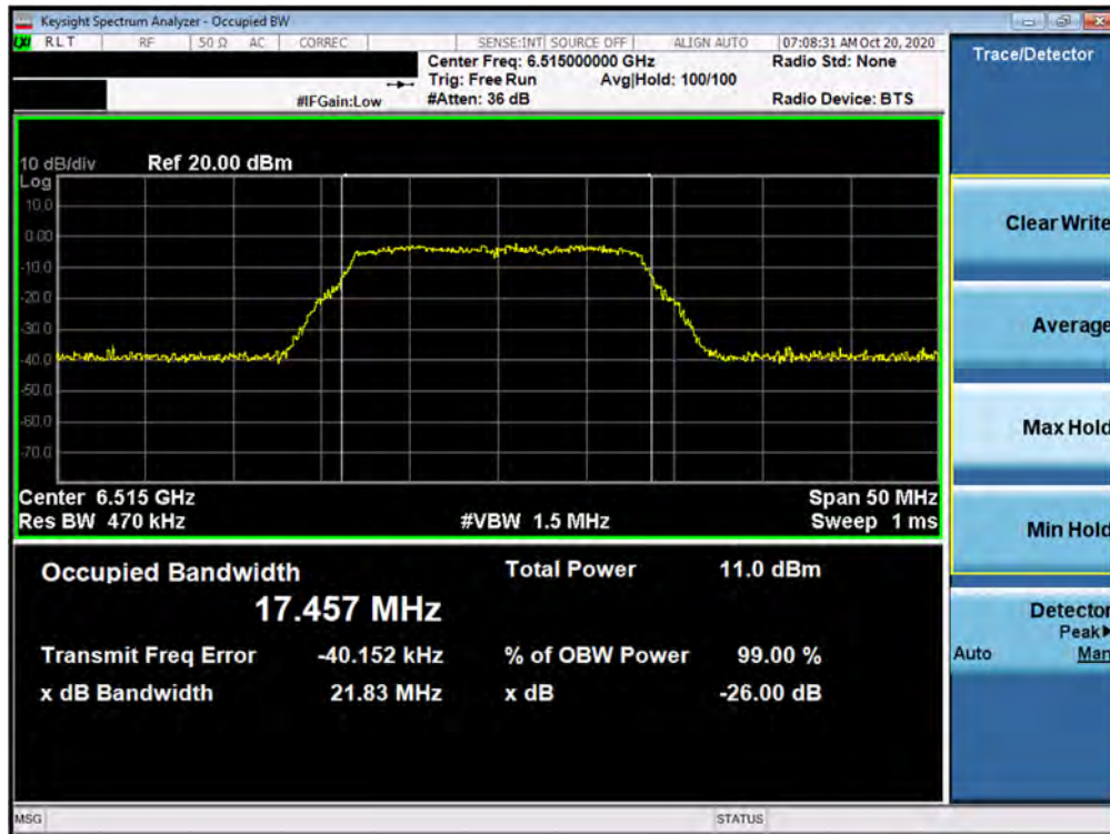
Plot 7-18. 26dB Bandwidth Plot MIMO ANT1 (802.11a (UNII Band 6) – Ch. 113)
