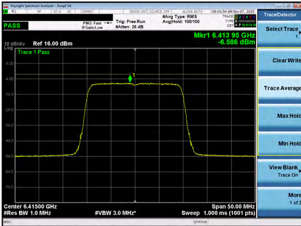
Plot 7-110. Power Spectral Density Plot MIMO ANT1 (20MHz BW 802.11ax (UNII Band 5) – Ch. 93)
