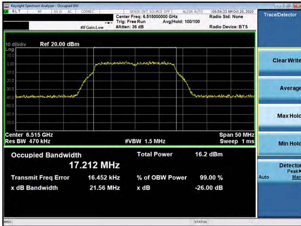
Plot 7-70. 26dB Bandwidth Plot MIMO ANT2 (802.11a (UNII Band 6) – Ch. 113)
