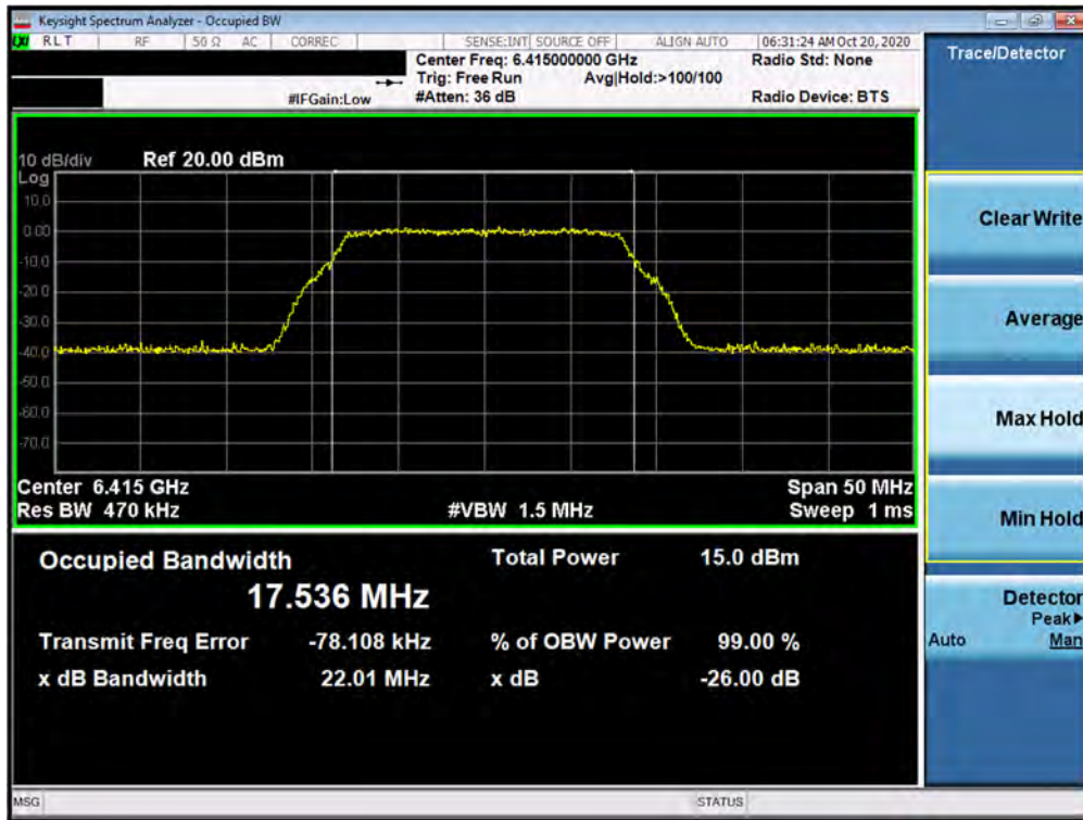
Plot 7-3. 26dB Bandwidth Plot MIMO ANT1 (802.11a (UNII Band 5) – Ch. 93)
