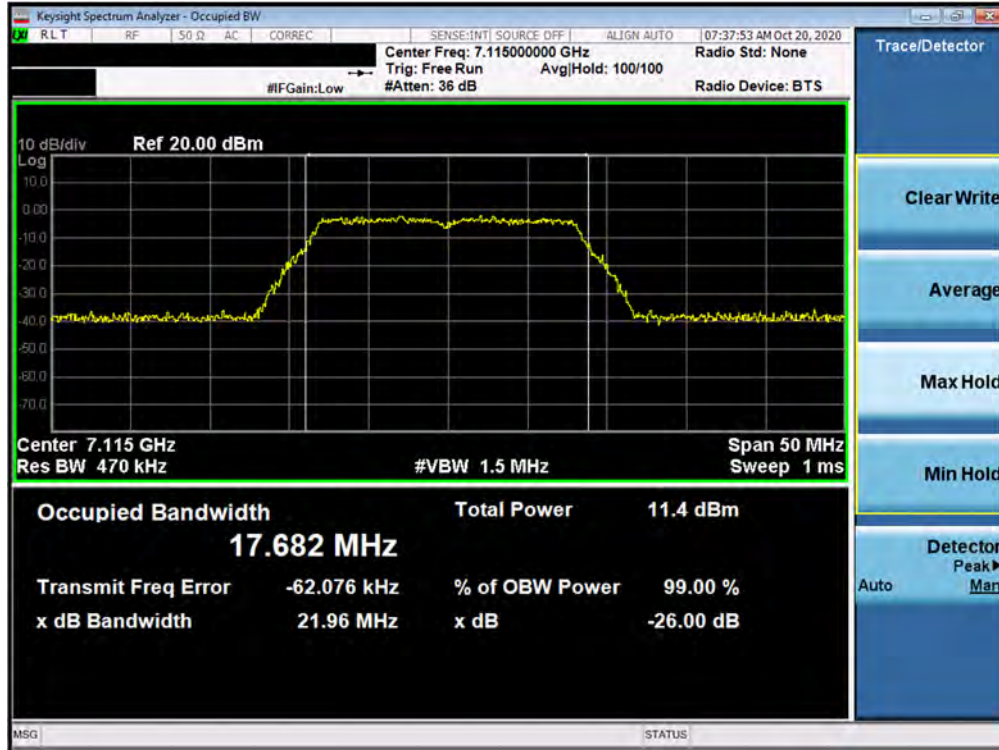
Plot 7-43. 26dB Bandwidth Plot MIMO ANT1 (802.11a (UNII Band 8) – Ch. 233)
