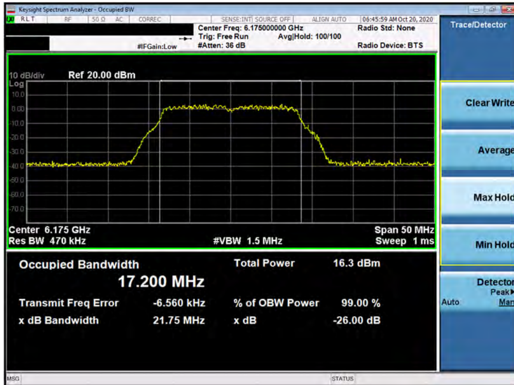
Plot 7-54. 26dB Bandwidth Plot MIMO ANT2 (802.11a (UNII Band 5) – Ch. 45)
