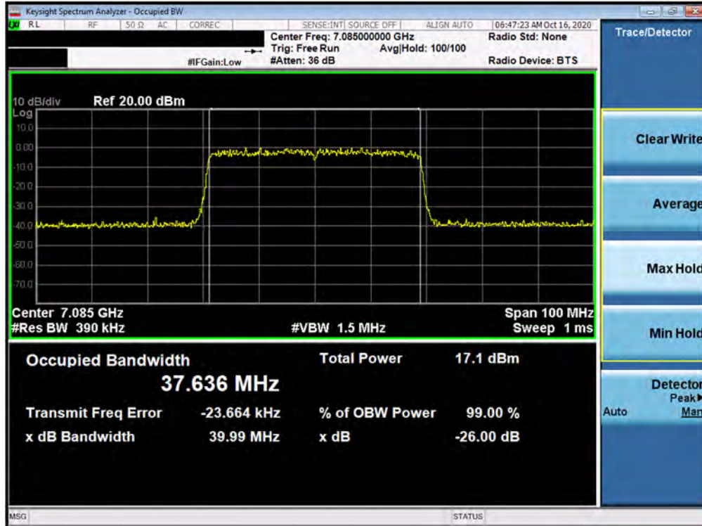
Plot 7-101. 26dB Bandwidth Plot MIMO ANT2 (40MHz BW 802.11ax (UNII Band 8) – Ch. 227)
