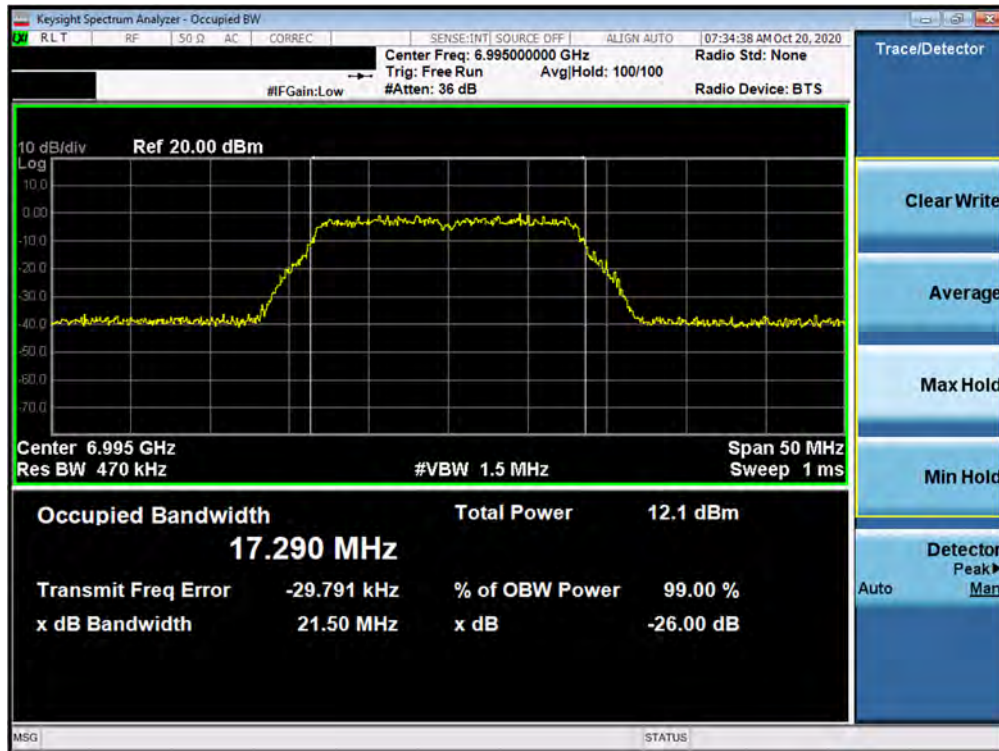
Plot 7-94. 26dB Bandwidth Plot MIMO ANT2 (802.11a (UNII Band 8) – Ch. 209)
