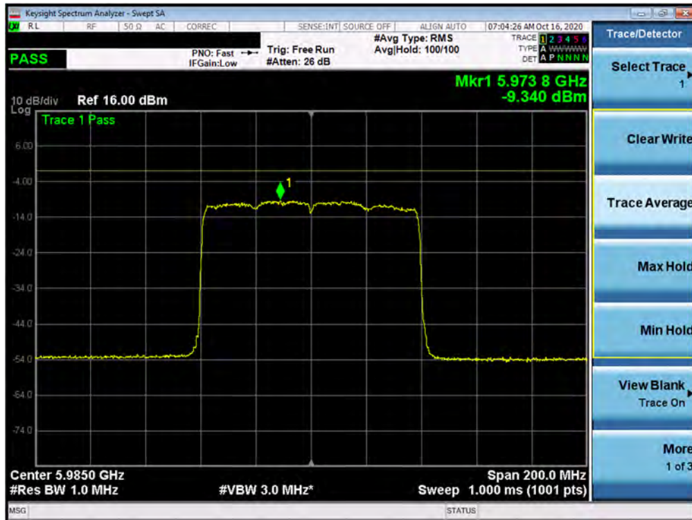
Plot 7-114. Power Spectral Density Plot MIMO ANT1 (80MHz BW 802.11ax (UNII Band 5) – Ch. 7)
