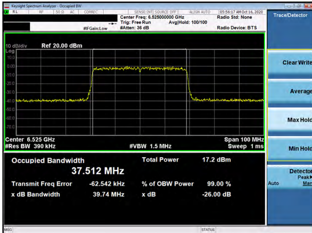
Plot 7-76. 26dB Bandwidth Plot MIMO ANT2 (40MHz BW 802.11ax (UNII Band 6) – Ch. 115)
