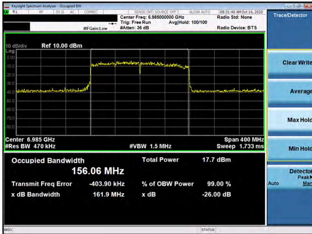
Plot 7-104. 26dB Bandwidth Plot MIMO ANT2 (160MHz BW 802.11ax (UNII Band 8) – Ch. 207)
