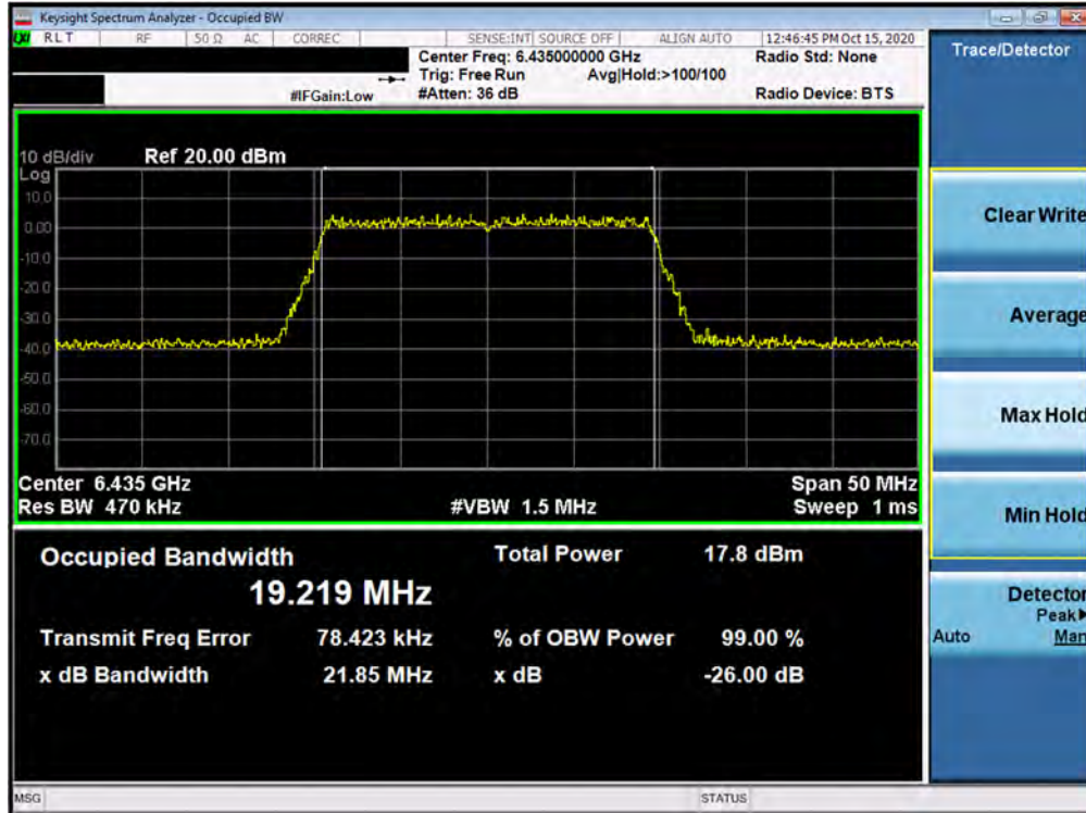
Plot 7-71. 26dB Bandwidth Plot MIMO ANT2 (20MHz BW 802.11ax (UNII Band 6) – Ch. 97)
