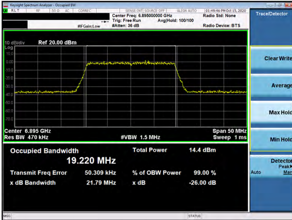
Plot 7-96. 26dB Bandwidth Plot MIMO ANT2 (20MHz BW 802.11ax (UNII Band 8) – Ch. 189)
