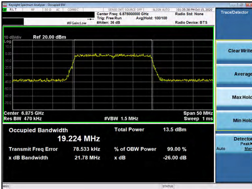
Plot 7-84. 26dB Bandwidth Plot MIMO ANT2 (20MHz BW 802.11ax (UNII Band 7) – Ch. 185)
