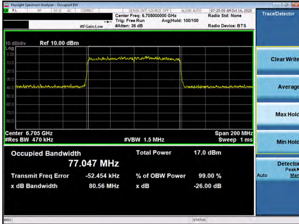
Plot 7-89. 26dB Bandwidth Plot MIMO ANT2 (80MHz BW 802.11ax (UNII Band 7) – Ch. 151)
