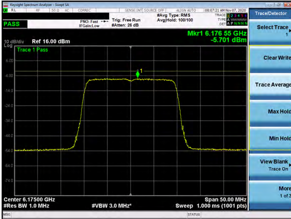
Plot 7-109. Power Spectral Density Plot MIMO ANT1 (20MHz BW 802.11ax (UNII Band 5) – Ch. 45)
