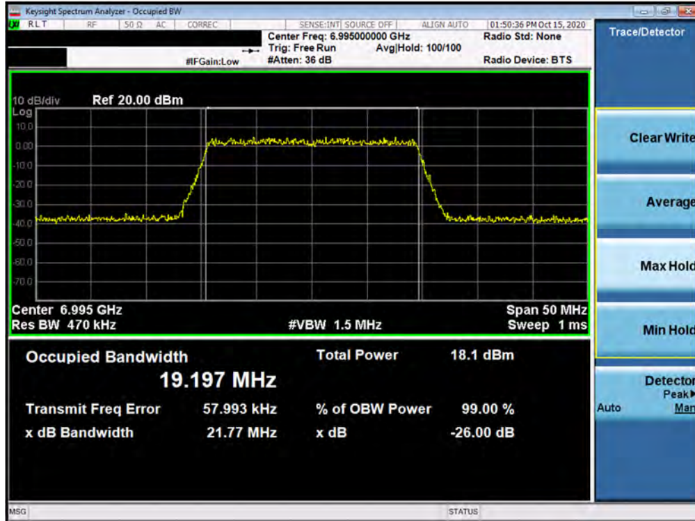
Plot 7-97. 26dB Bandwidth Plot MIMO ANT2 (20MHz BW 802.11ax (UNII Band 8) – Ch. 209)
