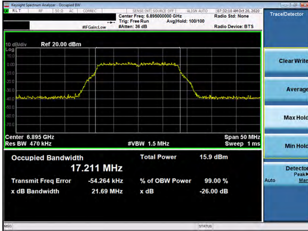
Plot 7-93. 26dB Bandwidth Plot MIMO ANT2 (802.11a (UNII Band 8) – Ch. 189)
