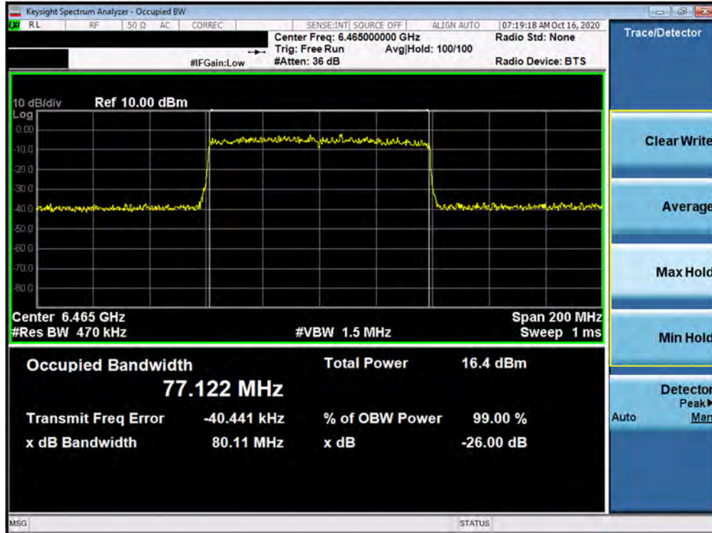
Plot 7-77. 26dB Bandwidth Plot MIMO ANT2 (80MHz BW 802.11ax (UNII Band 6) – Ch. 103)
