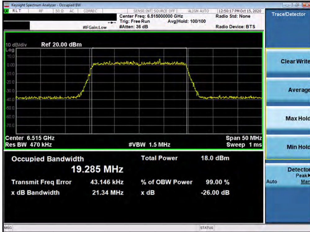
Plot 7-73. 26dB Bandwidth Plot MIMO ANT2 (20MHz BW 802.11ax (UNII Band 6) – Ch. 113)
