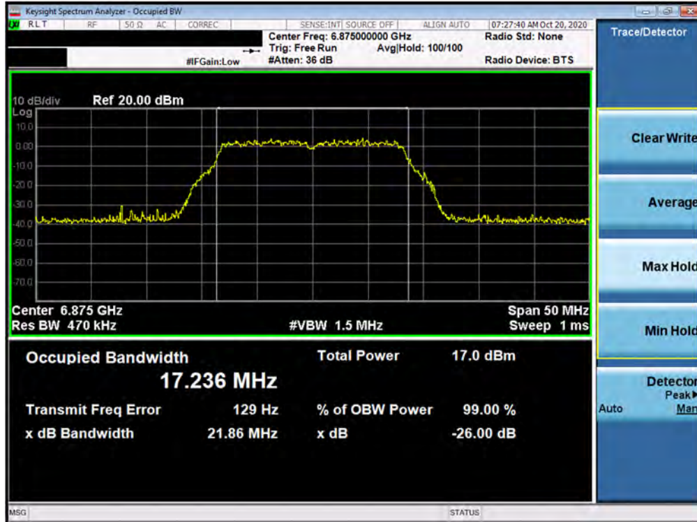
Plot 7-81. 26dB Bandwidth Plot MIMO ANT2 (802.11a (UNII Band 7) – Ch. 185)
