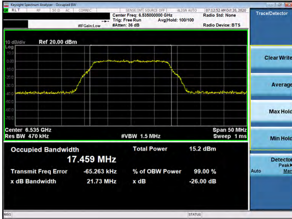
Plot 7-27. 26dB Bandwidth Plot MIMO ANT1 (802.11a (UNII Band 7) – Ch. 117)
