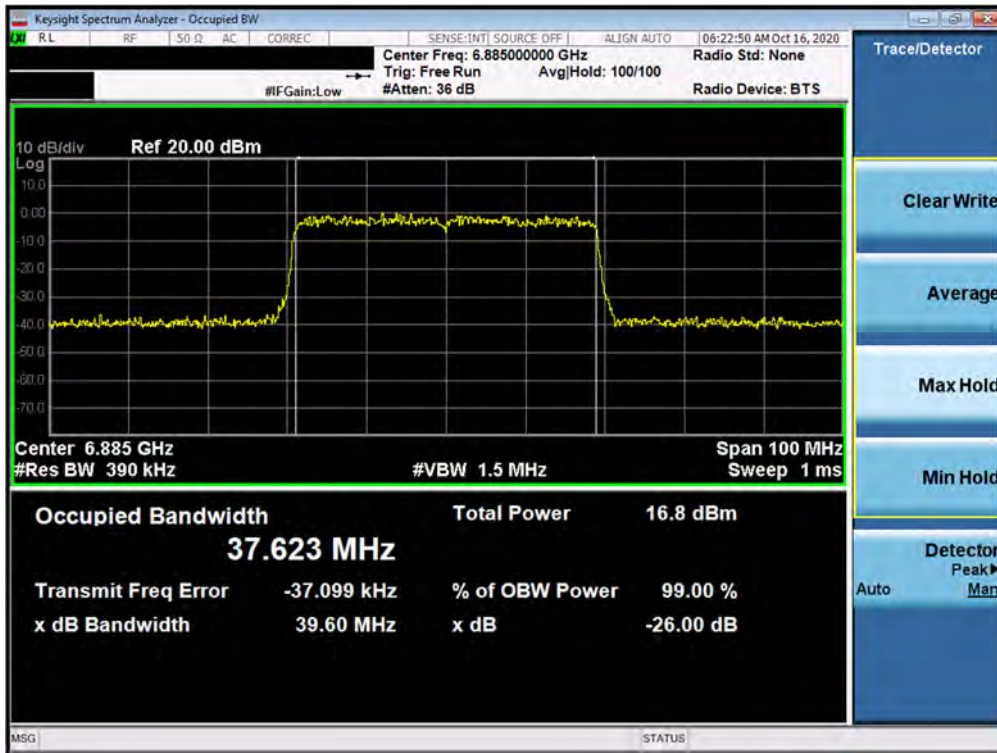
Plot 7-99. 26dB Bandwidth Plot MIMO ANT2 (40MHz BW 802.11ax (UNII Band 8) – Ch. 187)
