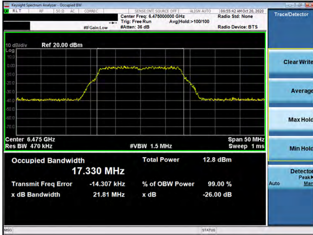
Plot 7-69. 26dB Bandwidth Plot MIMO ANT2 (802.11a (UNII Band 6) – Ch. 105)
