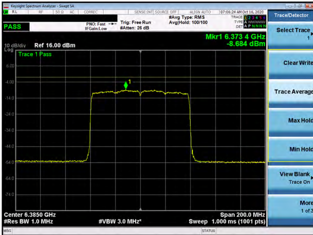
Plot 7-116. Power Spectral Density Plot MIMO ANT1 (80MHz BW 802.11ax (UNII Band 5) – Ch. 87)
