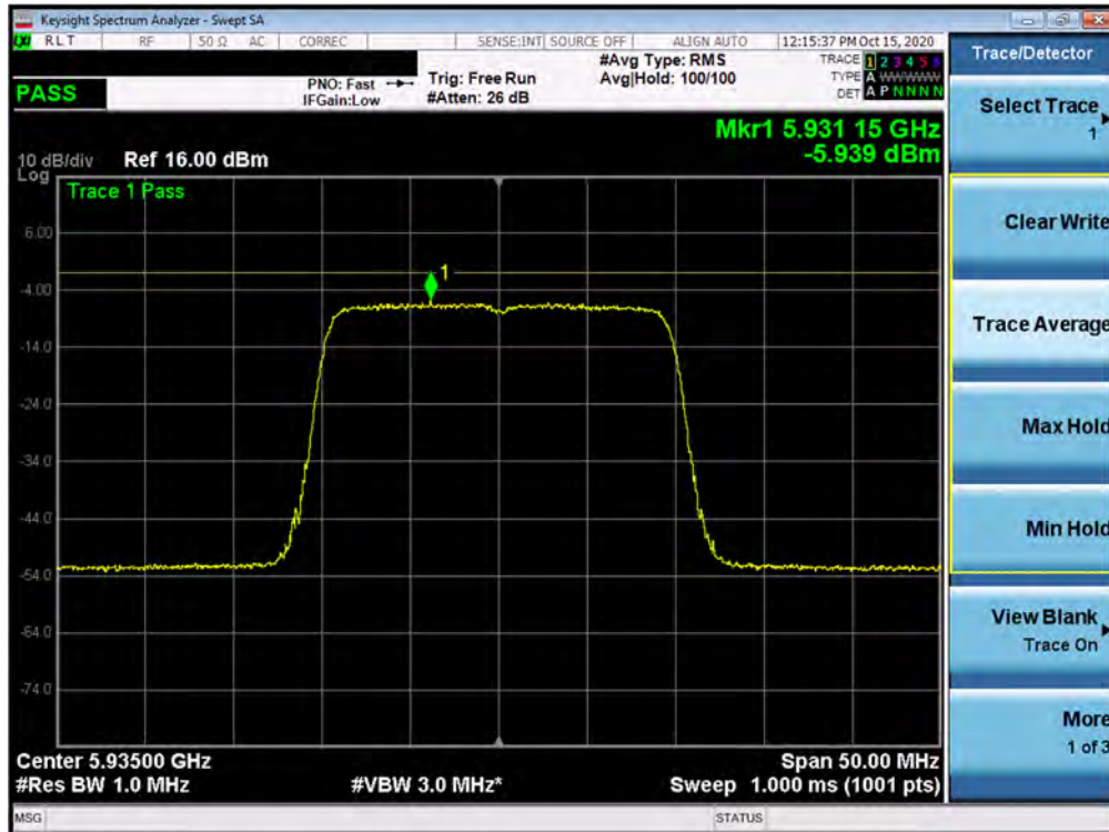
Plot 7-108. Power Spectral Density Plot MIMO ANT1 (20MHz BW 802.11ax (UNII Band 5) – Ch. 2)
