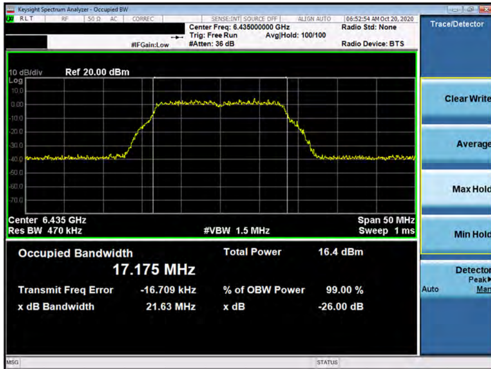
Plot 7-68. 26dB Bandwidth Plot MIMO ANT2 (802.11a (UNII Band 6) – Ch. 97)
