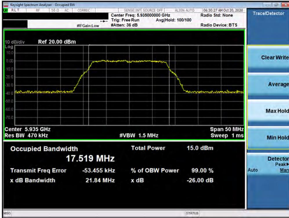
Plot 7-1. 26dB Bandwidth Plot MIMO ANT1 (802.11a (UNII Band 5) – Ch. 2)
