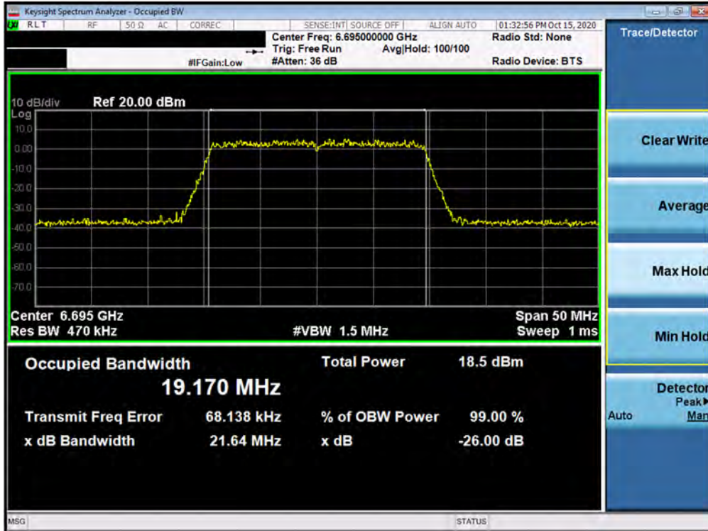
Plot 7-83. 26dB Bandwidth Plot MIMO ANT2 (20MHz BW 802.11ax (UNII Band 7) – Ch. 149)
