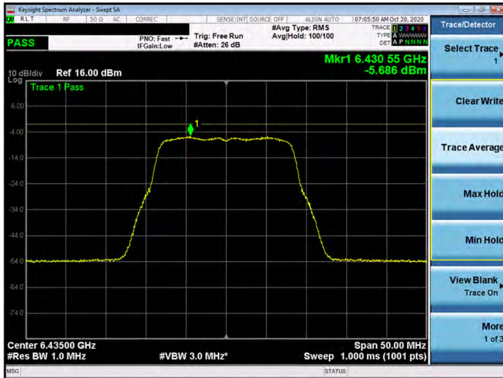
Plot 7-120. Power Spectral Density Plot MIMO ANT1 (802.11a (UNII Band 6) – Ch. 97)
