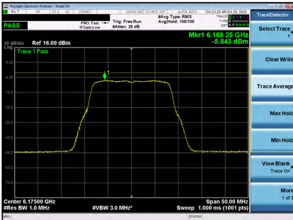
Plot 7-106. Power Spectral Density Plot MIMO ANT1 (802.11a (UNII Band 5) – Ch. 45)
