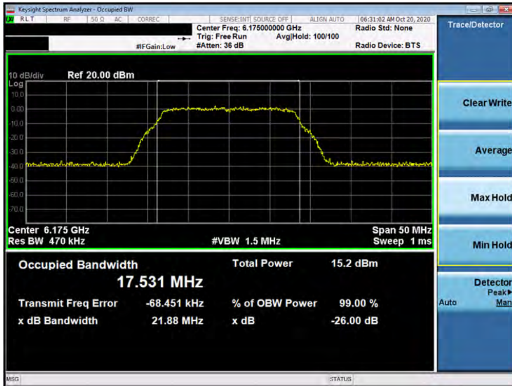
Plot 7-2. 26dB Bandwidth Plot MIMO ANT1 (802.11a (UNII Band 5) – Ch. 45)
