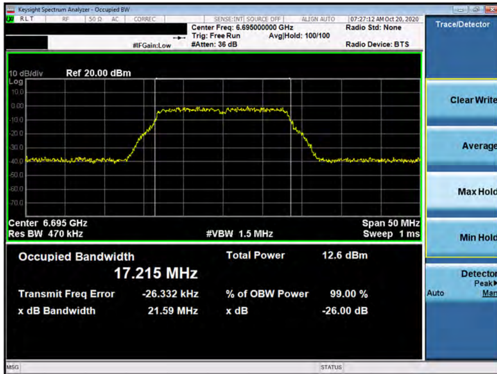
Plot 7-80. 26dB Bandwidth Plot MIMO ANT2 (802.11a (UNII Band 7) – Ch. 149)
