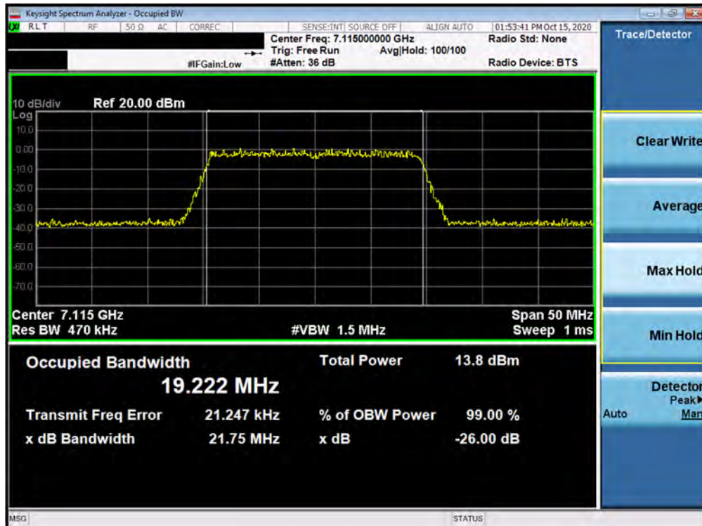
Plot 7-98. 26dB Bandwidth Plot MIMO ANT2 (20MHz BW 802.11ax (UNII Band 8) – Ch. 233)
