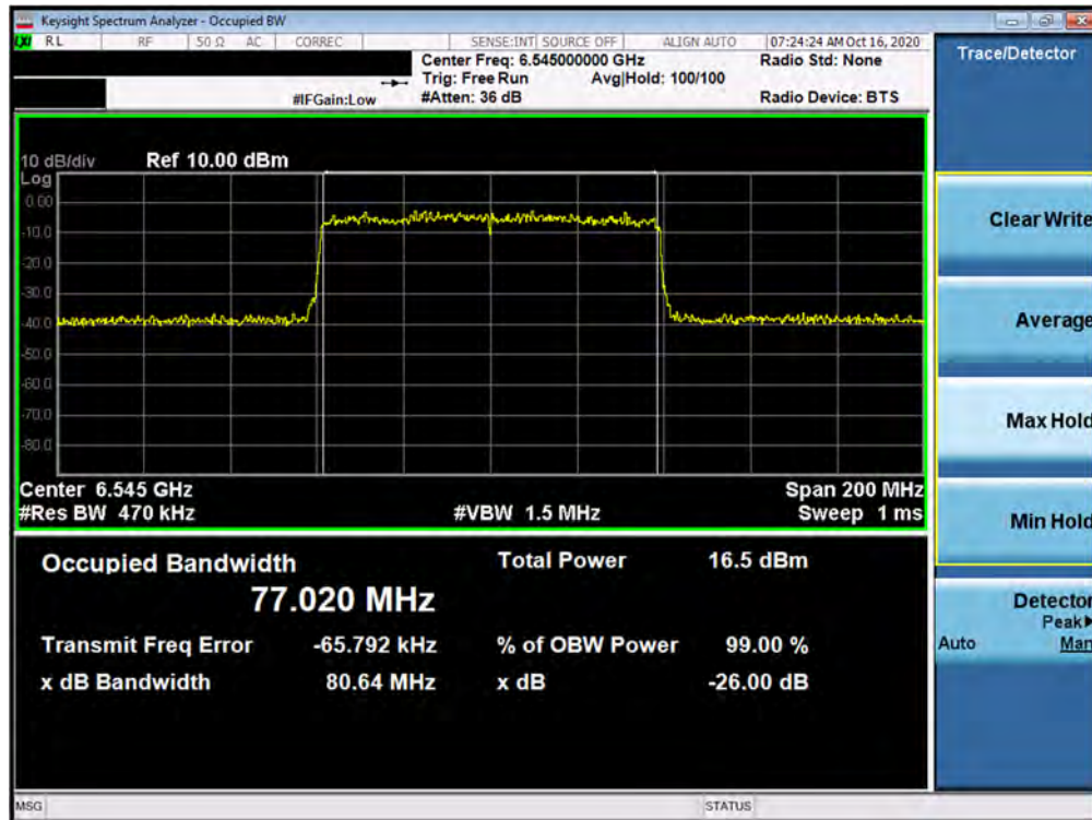
Plot 7-88. 26dB Bandwidth Plot MIMO ANT2 (80MHz BW 802.11ax (UNII Band 7) – Ch. 119)
