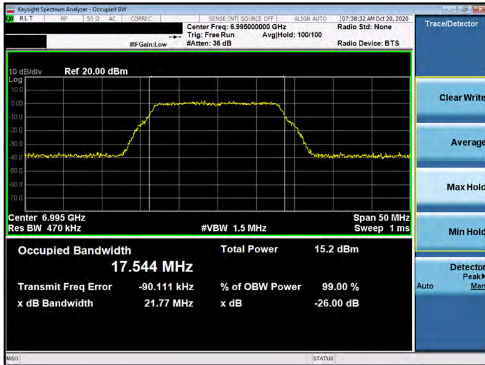
Plot 7-42. 26dB Bandwidth Plot MIMO ANT1 (802.11a (UNII Band 8) – Ch. 209)
