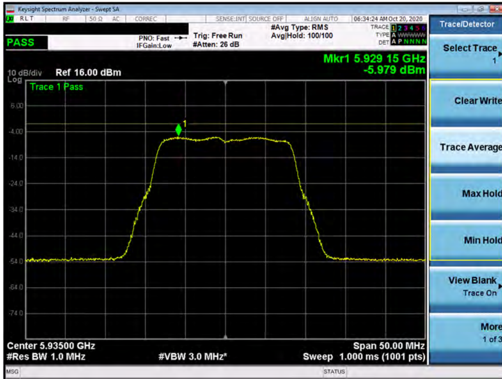
Plot 7-105. Power Spectral Density Plot MIMO ANT1 (802.11a (UNII Band 5) – Ch. 2)
