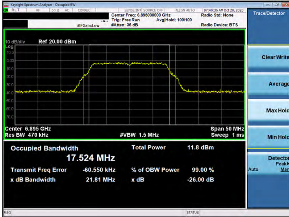
Plot 7-41. 26dB Bandwidth Plot MIMO ANT1 (802.11a (UNII Band 8) – Ch. 189)
