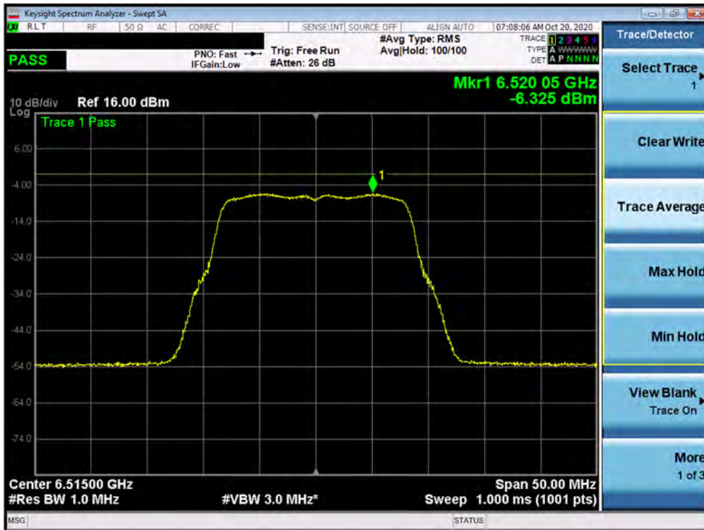
Plot 7-122. Power Spectral Density Plot MIMO ANT1 (802.11a (UNII Band 6) – Ch. 113)
