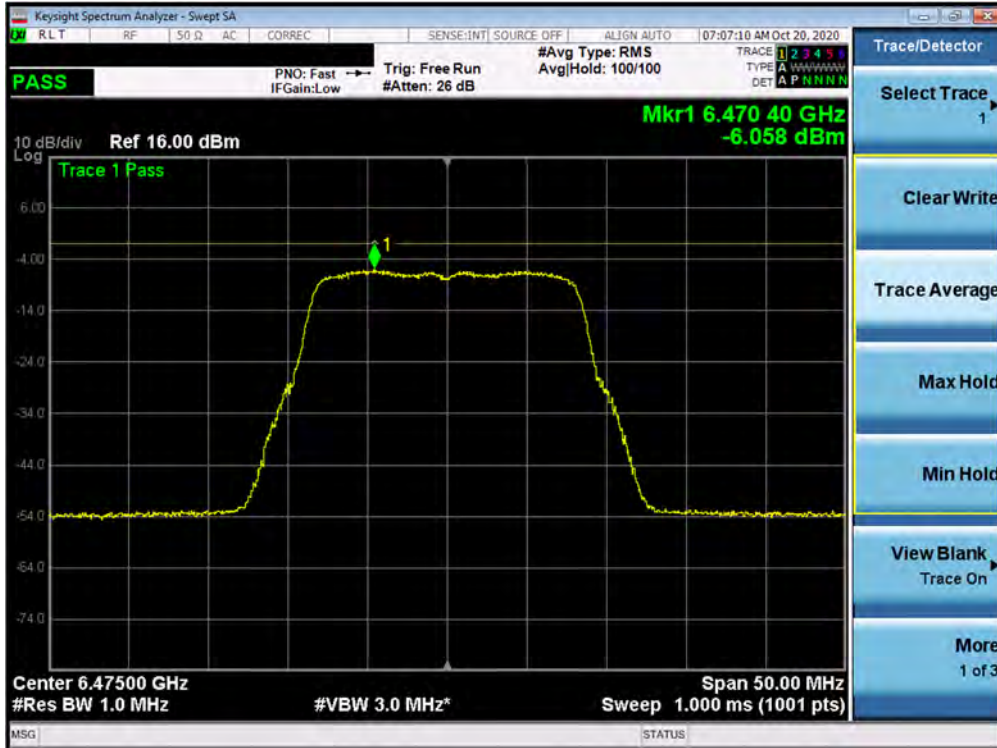
Plot 7-121. Power Spectral Density Plot MIMO ANT1 (802.11a (UNII Band 6) – Ch. 105)
