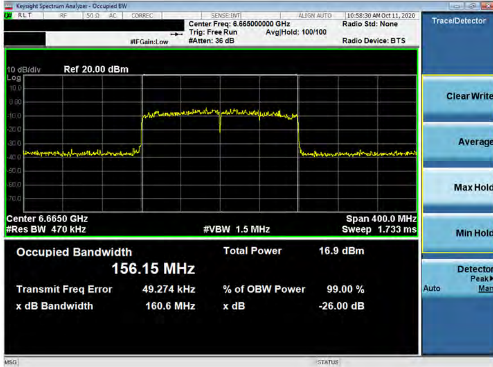
Plot 7-91. 26dB Bandwidth Plot MIMO ANT2 (160MHz BW 802.11ax (UNII Band 7) – Ch. 143)
