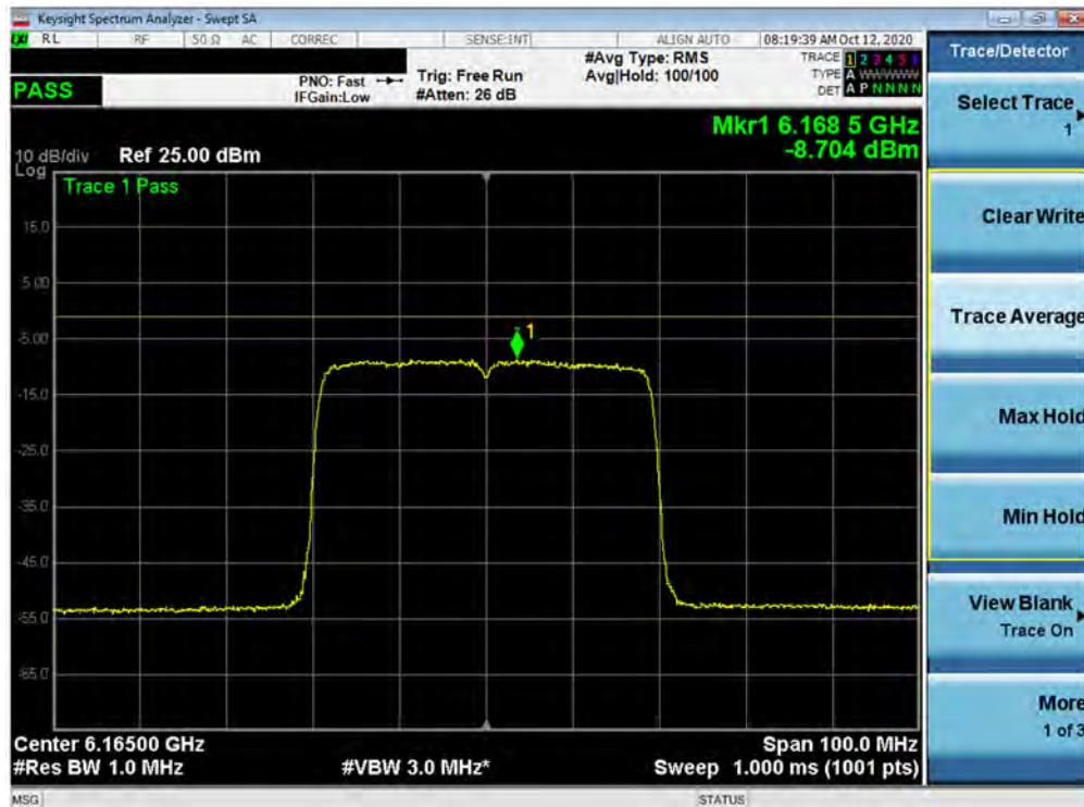
Plot 7-112. Power Spectral Density Plot MIMO ANT1 (40MHz BW 802.11ax (UNII Band 5) – Ch. 43)
