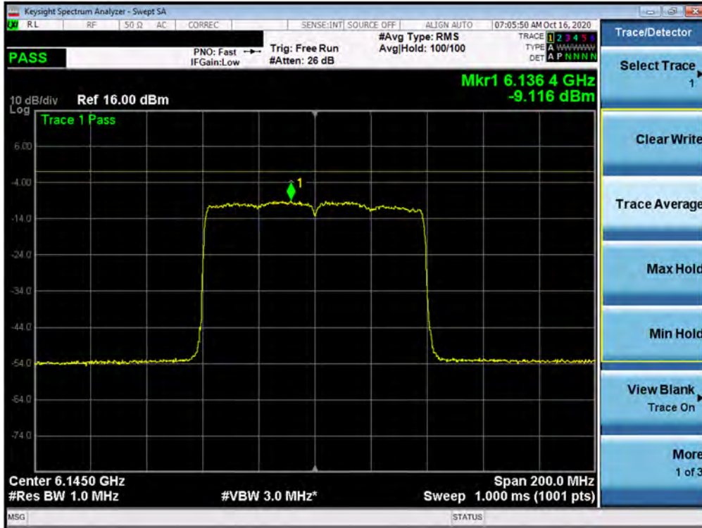
Plot 7-115. Power Spectral Density Plot MIMO ANT1 (80MHz BW 802.11ax (UNII Band 5) – Ch. 39)
