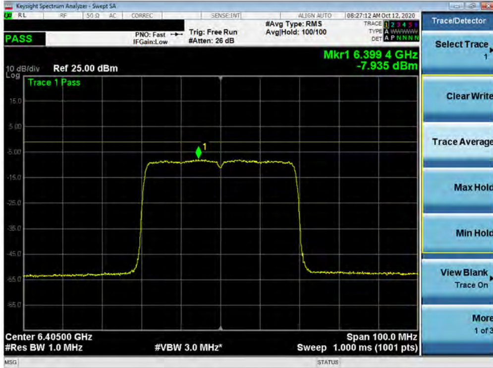
Plot 7-113. Power Spectral Density Plot MIMO ANT1 (40MHz BW 802.11ax (UNII Band 5) – Ch. 91)
