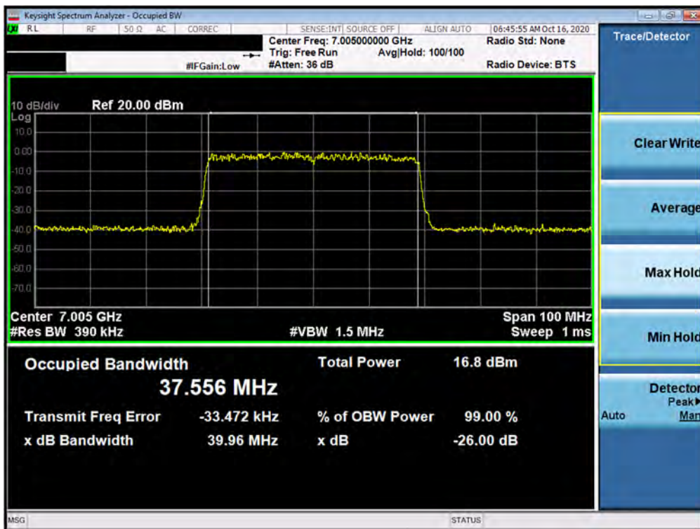
Plot 7-100. 26dB Bandwidth Plot MIMO ANT2 (40MHz BW 802.11ax (UNII Band 8) – Ch. 211)
