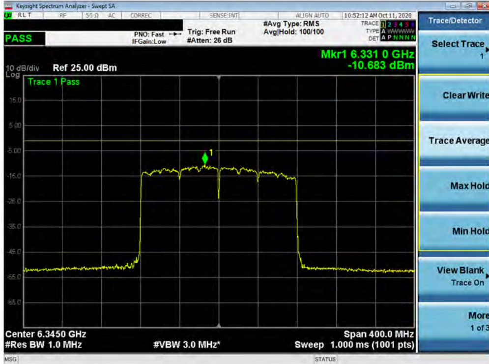
Plot 7-119. Power Spectral Density Plot MIMO ANT1 (160MHz BW 802.11ax (UNII Band 5) – Ch. 79)
