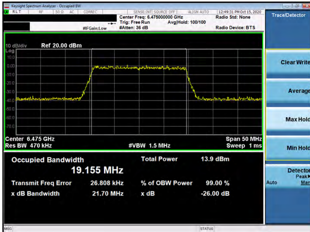
Plot 7-72. 26dB Bandwidth Plot MIMO ANT2 (20MHz BW 802.11ax (UNII Band 6) – Ch. 105)
