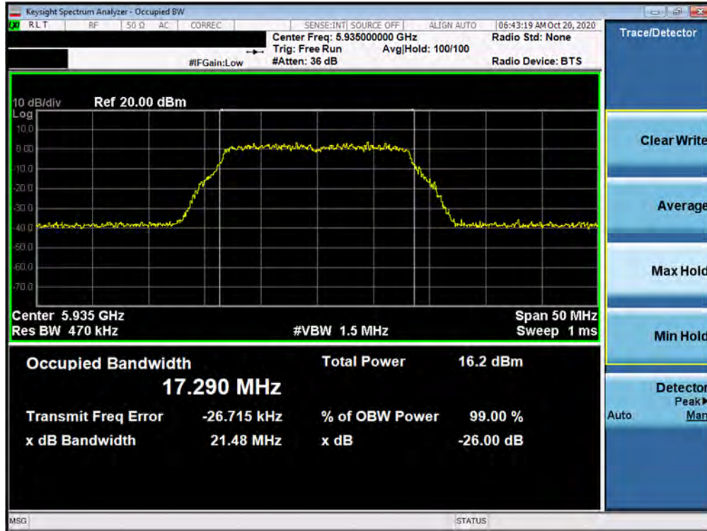
Plot 7-53. 26dB Bandwidth Plot MIMO ANT2 (802.11a (UNII Band 5) – Ch. 2)
