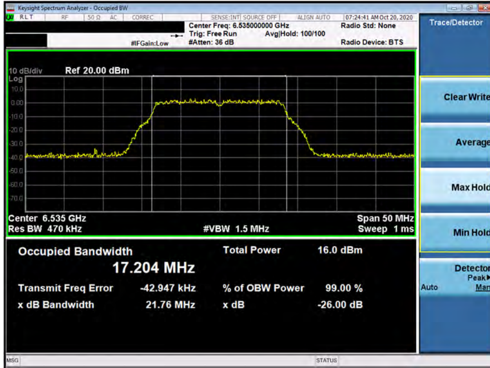
Plot 7-79. 26dB Bandwidth Plot MIMO ANT2 (802.11a (UNII Band 7) – Ch. 117)
