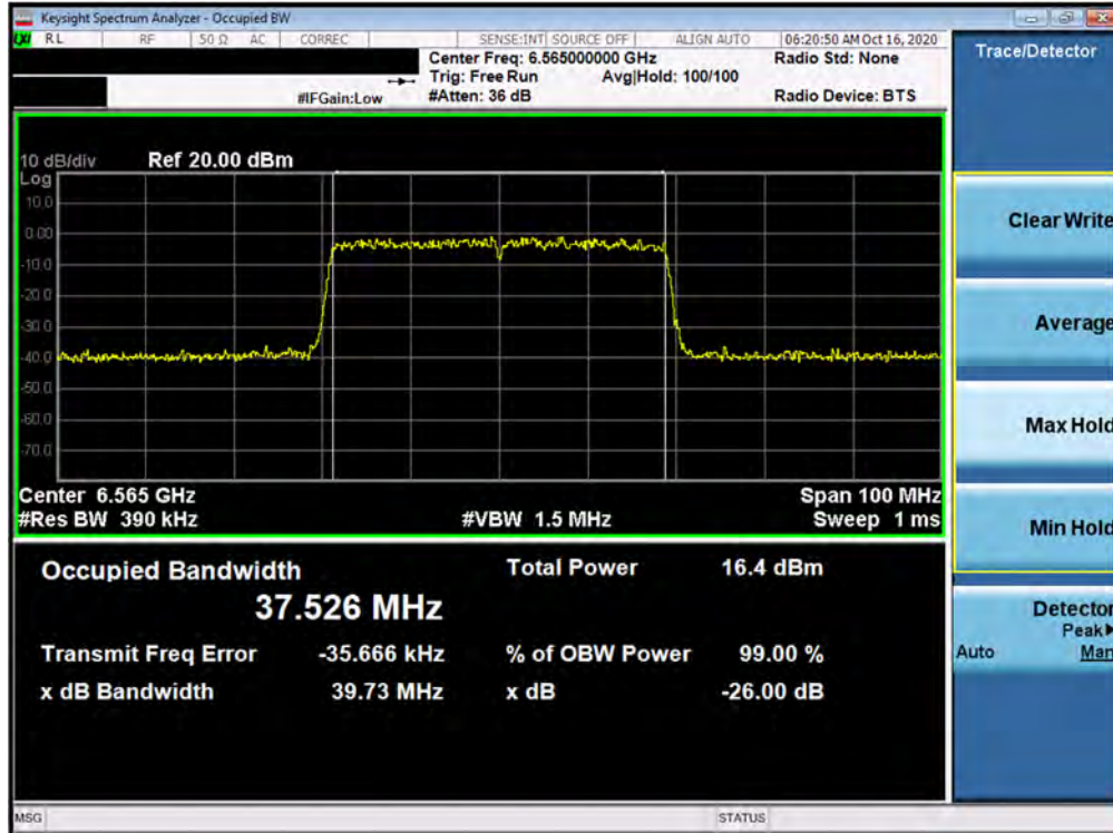
Plot 7-85. 26dB Bandwidth Plot MIMO ANT2 (40MHz BW 802.11ax (UNII Band 7) – Ch. 123)
