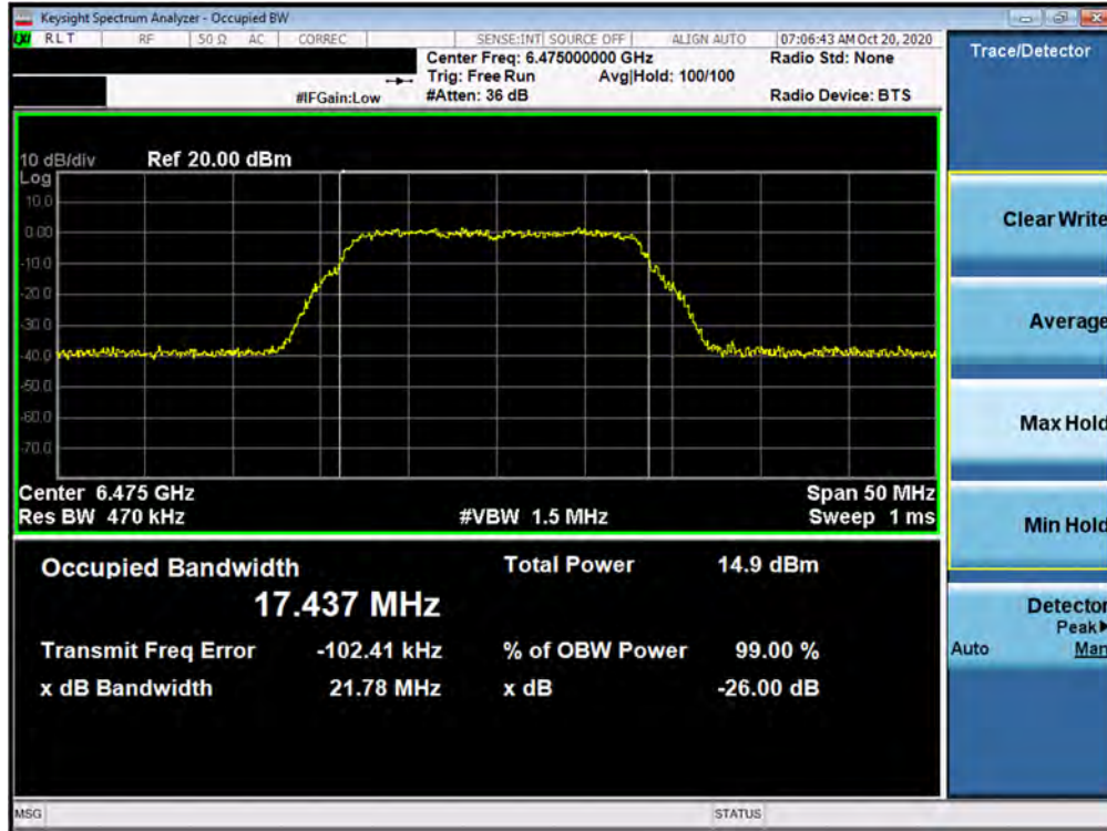
Plot 7-17. 26dB Bandwidth Plot MIMO ANT1 (802.11a (UNII Band 6) – Ch. 105)
