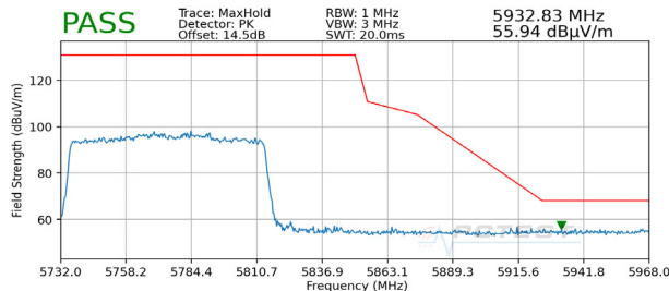
Plot 7-249. Radiated Upper Band Edge Plot MIMO (Peak – UNII Band 3 – 996 Tones)
