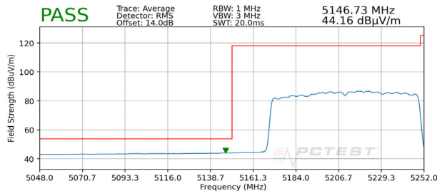
Plot 7-243. Radiated Lower Band Edge Plot MIMO (Average – UNII Band 1 – 996 Tones)
