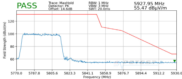
Plot 7-242. Radiated Upper Band Edge Plot MIMO (Peak – UNII Band 3 – 484 Tones)
