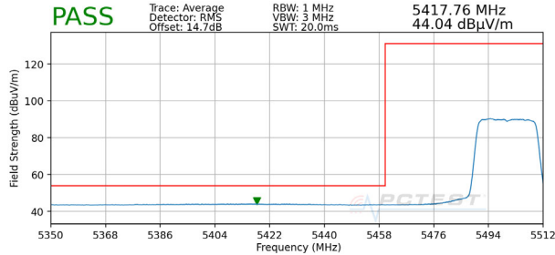
Plot 7-233. Radiated Lower Band Edge Plot MIMO (Average – UNII Band 2C – 242 Tones)
