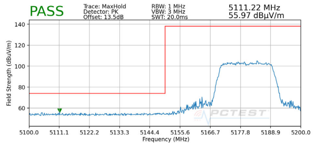
Plot 7-230. Radiated Lower Band Edge Plot MIMO (Peak – UNII Band 1 – 242 Tones)
