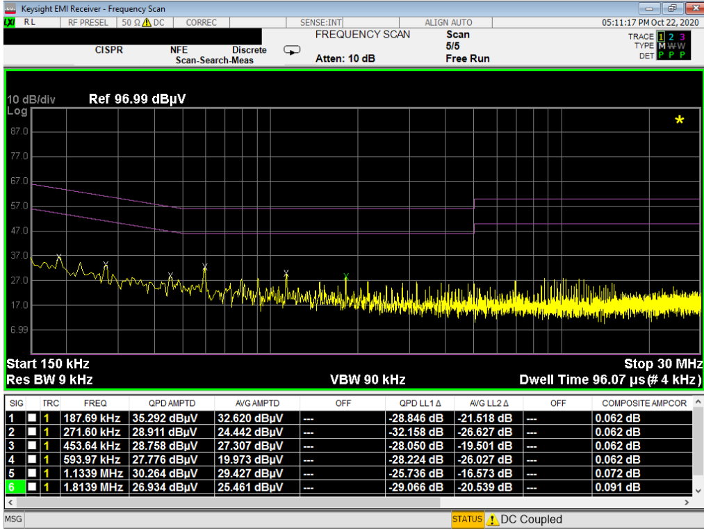
Plot 7-14. Line-Conducted Test Plot (L1) – Digitizer – Click
