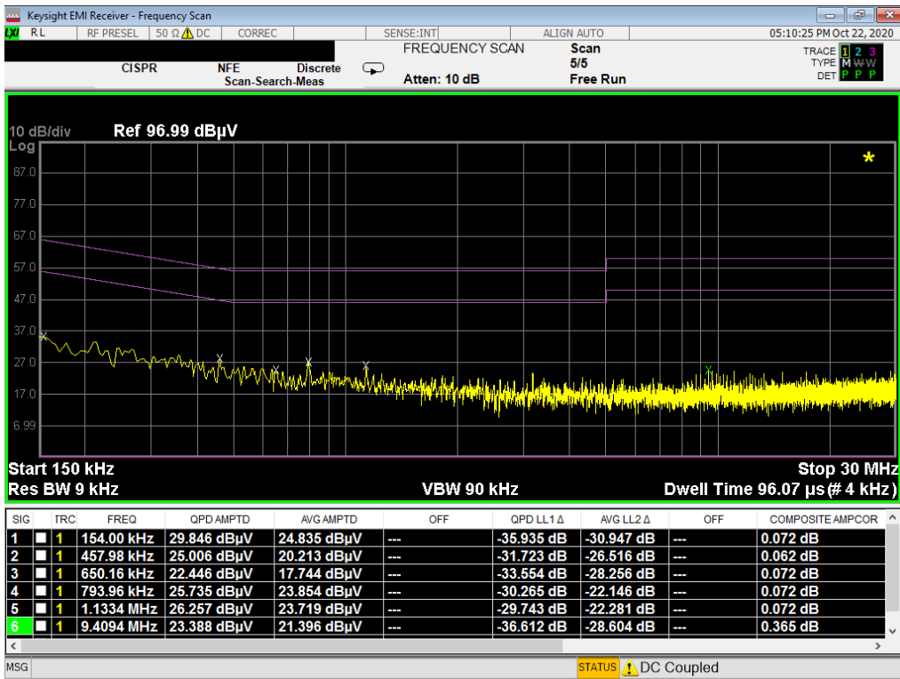
Plot 7-15. Line-Conducted Test Plot (N) – Digitizer – Click
