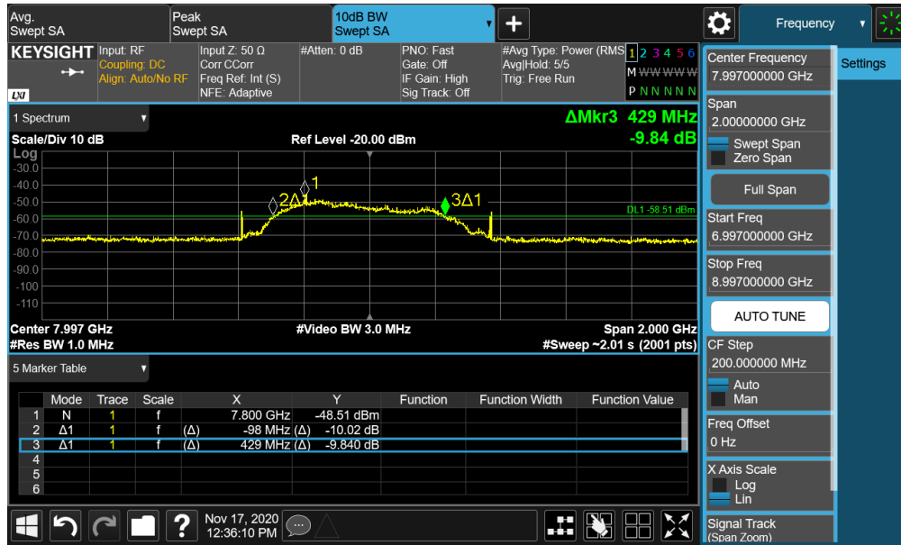
Plot 7-111. BANDWIDTH Plot – ANT1 - CH.9 – SP3 – Preamble 27
