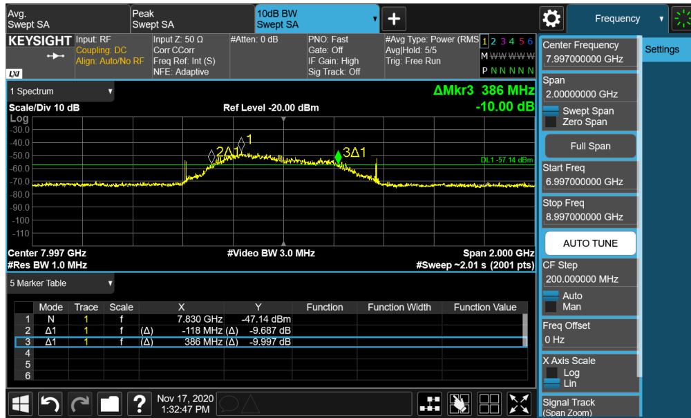
Plot 7-139. BANDWIDTH Plot – ANT1 - CH.9 - SP0 – Preamble 32
