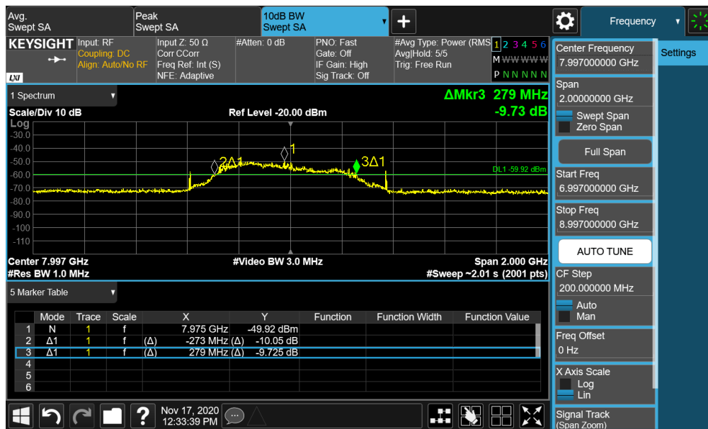
Plot 7-110. BANDWIDTH Plot – ANT1 - CH.9 – SP1 – Preamble 27
