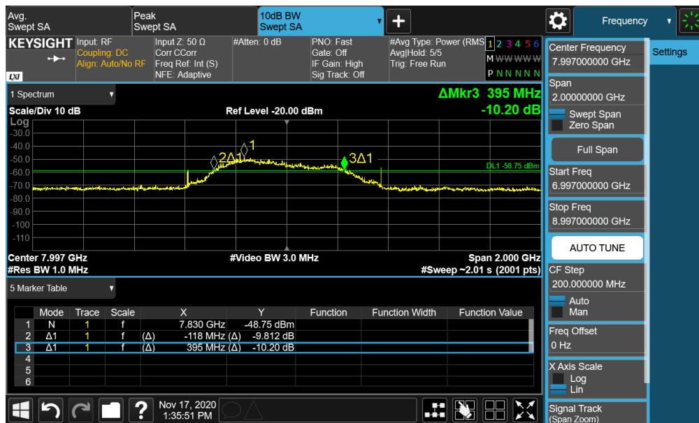
Plot 7-140. BANDWIDTH Plot – ANT1 - CH.9 – SP1 – Preamble 32
