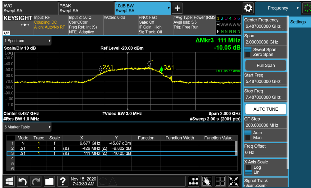
Plot 7-45. BANDWIDTH Plot – ANT1 - CH.5 – SP3 – Preamble 28
