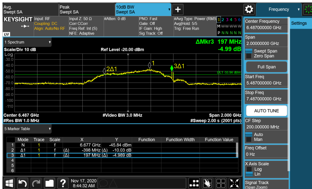
Plot 7-66. BANDWIDTH Plot – ANT2 - CH.5 – SP3 – Preamble 31
