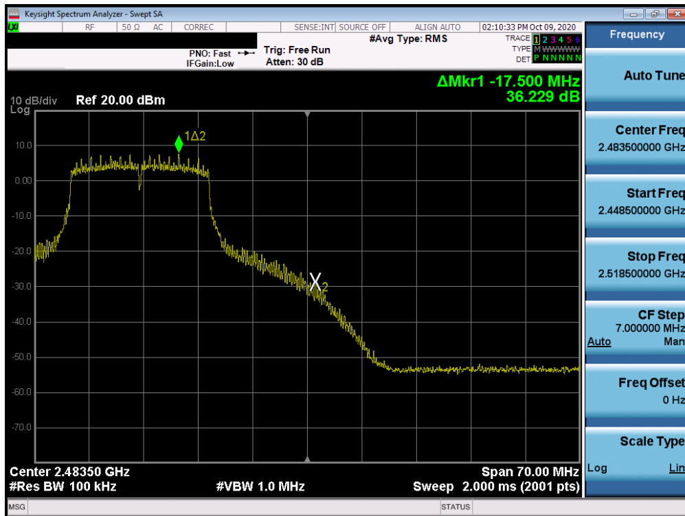
Plot 7-54. Band Edge Plot MIMO ANT2 (802.11n – Ch. 11)
