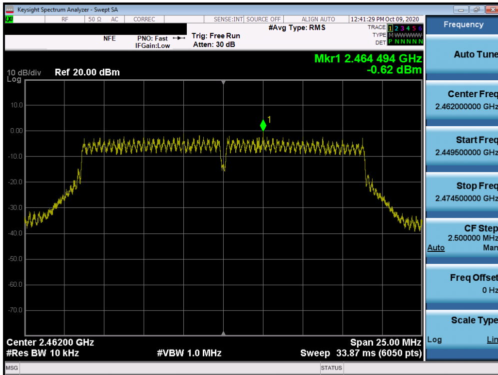
Plot 7-30. Power Spectral Density Plot MIMO ANT1 (802.11n – Ch. 11)
