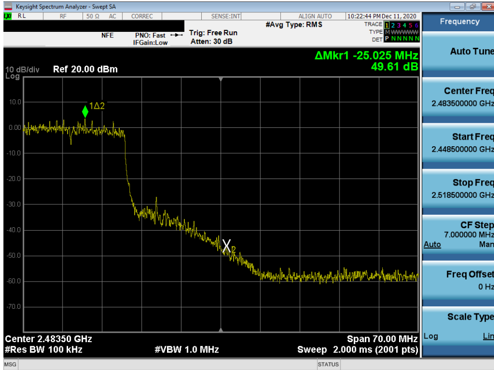
Plot 7-51. Band Edge Plot MIMO ANT1 (802.11ax – Ch. 10)
