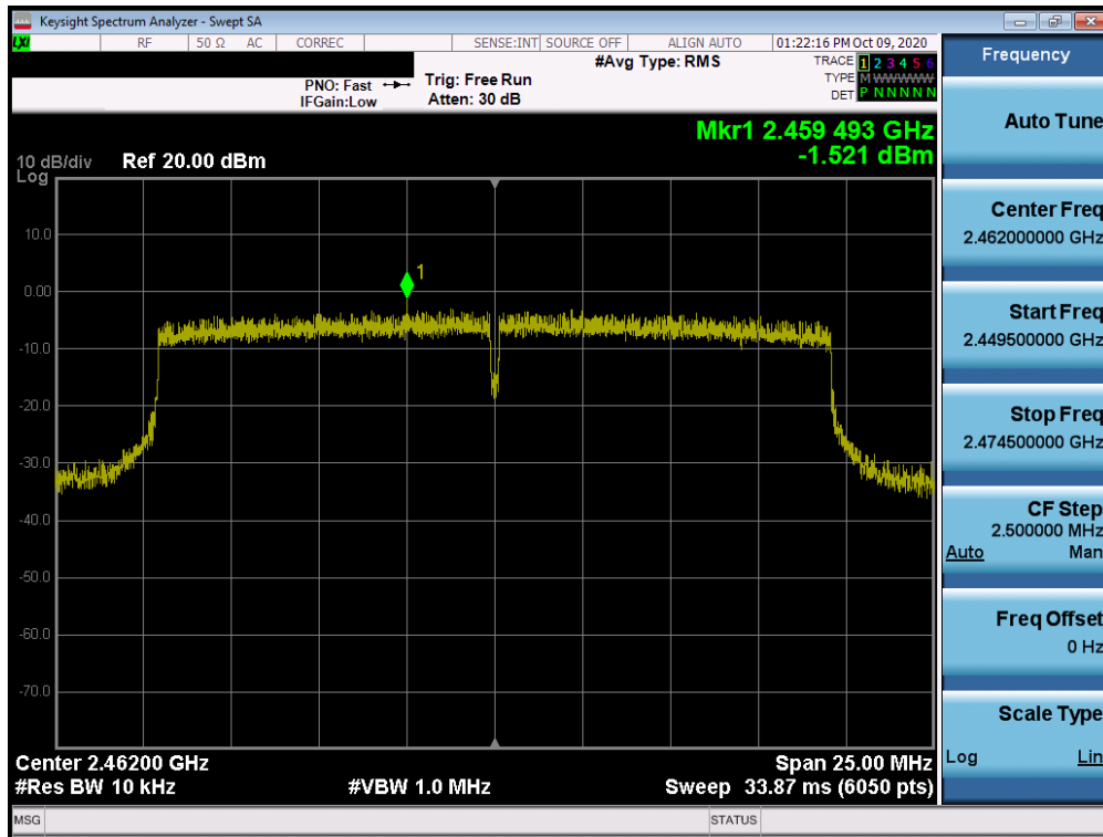
Plot 7-42. Power Spectral Density Plot MIMO ANT2 (802.11ax – Ch. 11)
