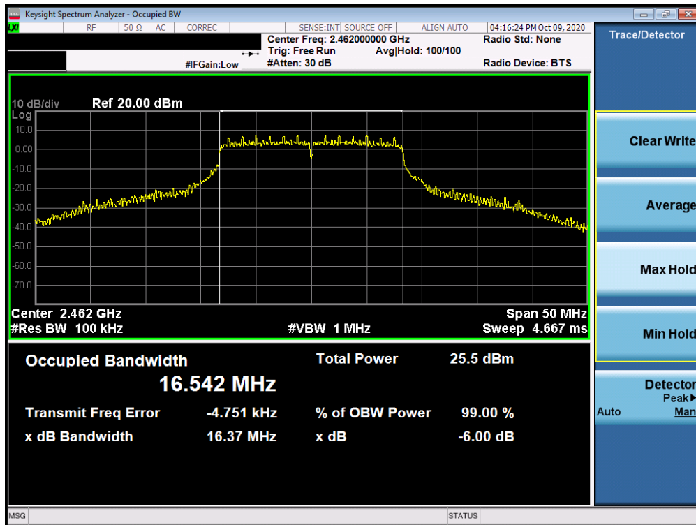
Plot 7-15. 6dB Bandwidth Plot MIMO ANT2 (802.11g – Ch. 11)
