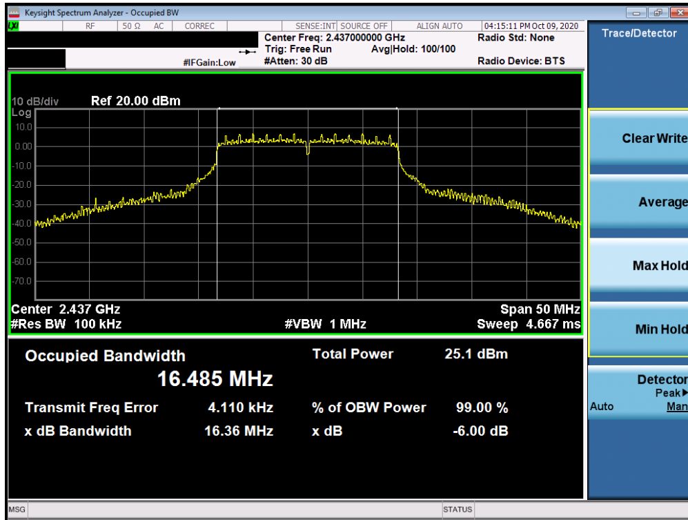
Plot 7-14. 6dB Bandwidth Plot MIMO ANT2 (802.11g – Ch. 6)
