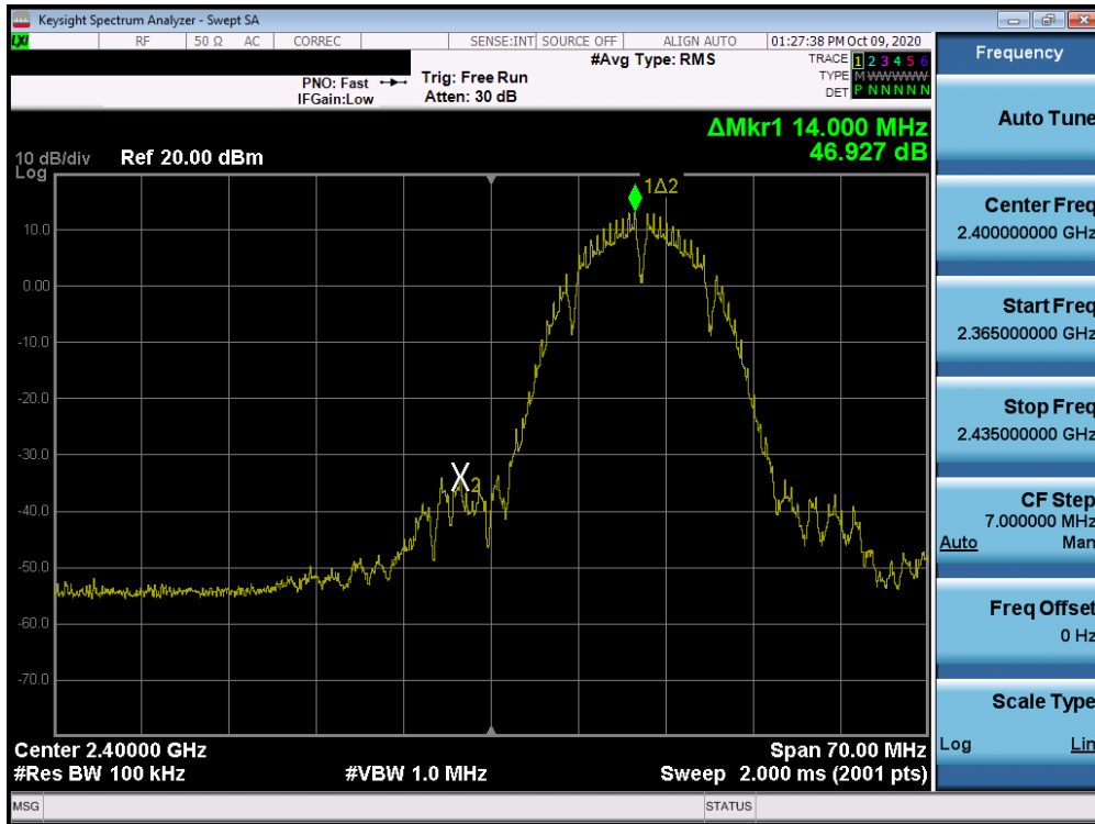
Plot 7-45. Band Edge Plot SISO ANT2 (802.11b – Ch. 1)
