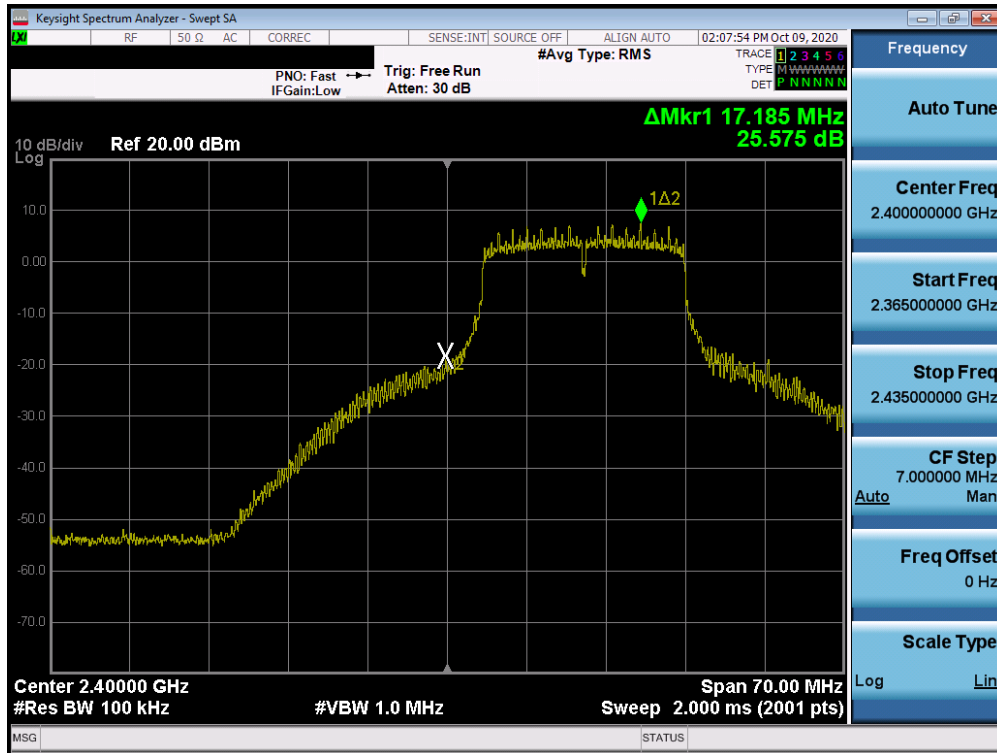
Plot 7-53. Band Edge Plot MIMO ANT2 (802.11n – Ch. 1)
