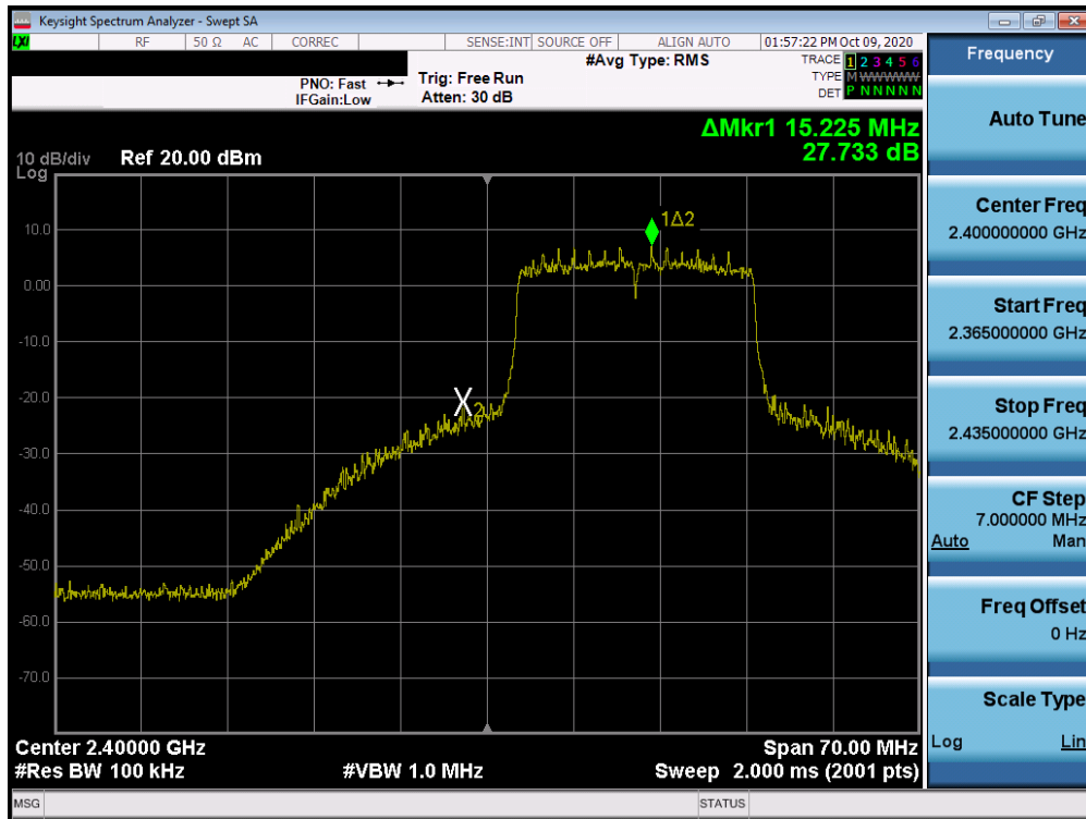
Plot 7-49. Band Edge Plot MIMO ANT1 (802.11ax – Ch. 1)
