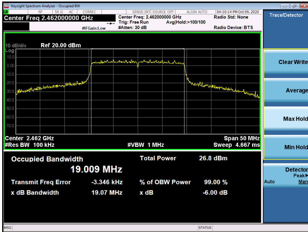
Plot 7-12. 6dB Bandwidth Plot MIMO ANT1 (802.11ax – Ch. 11)
