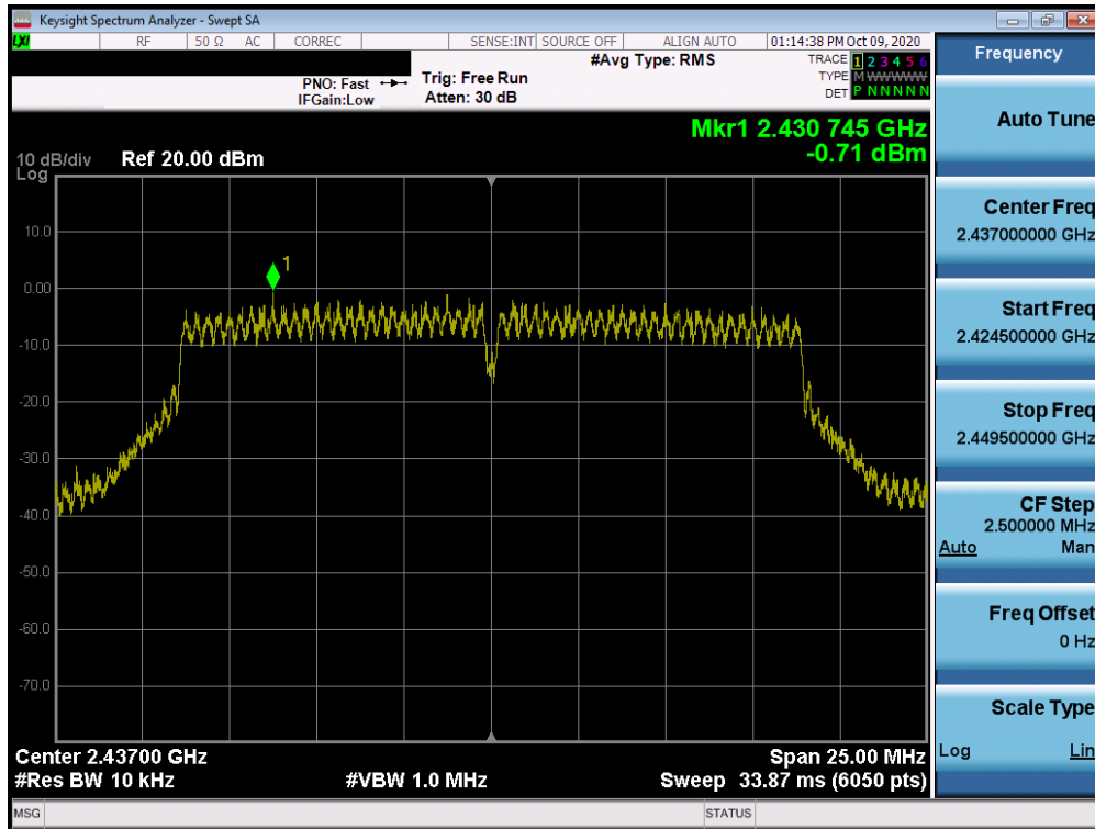
Plot 7-38. Power Spectral Density Plot MIMO ANT2 (802.11n – Ch. 6)
