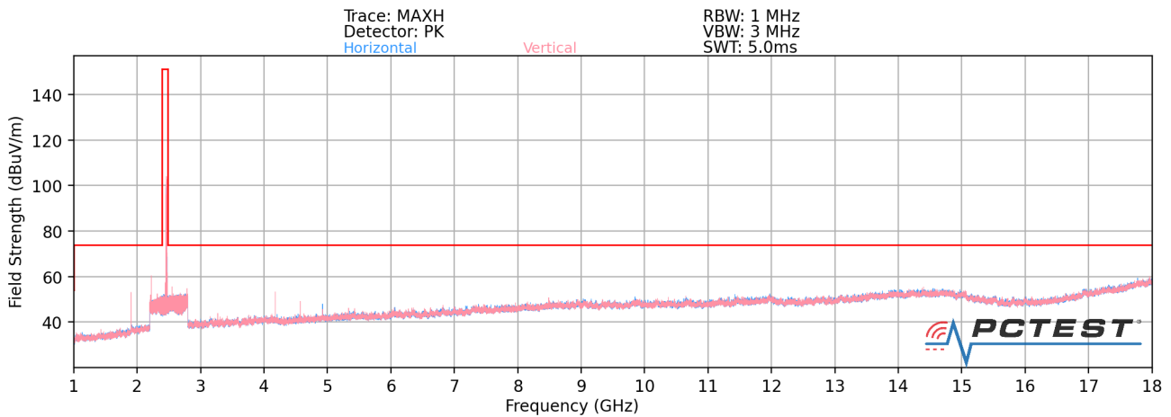
Plot 7-73. Radiated Spurious Plot above 1GHz SISO ANT1 (802.11b – Ch. 11)
