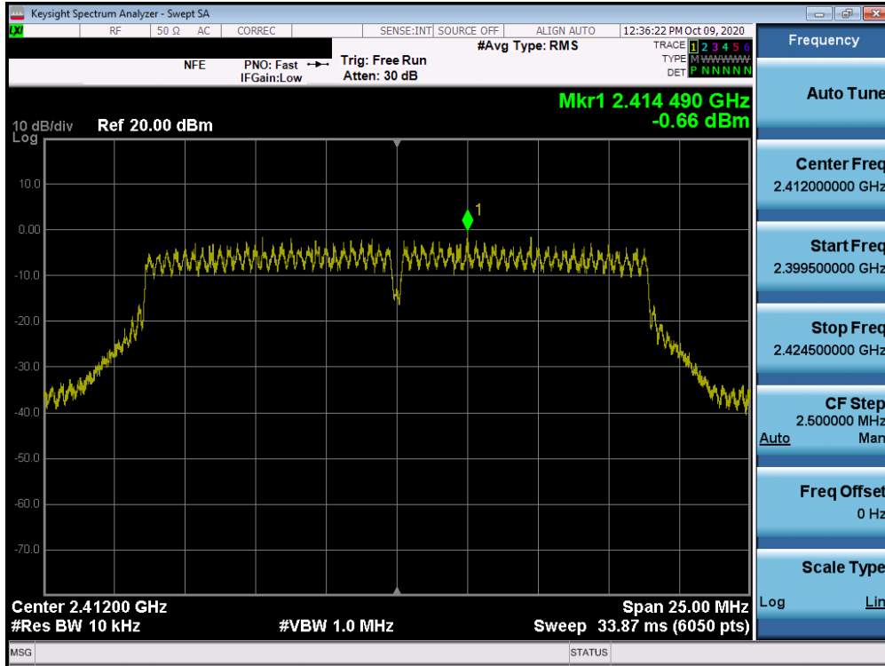
Plot 7-28. Power Spectral Density Plot MIMO ANT1 (802.11n – Ch. 1)
