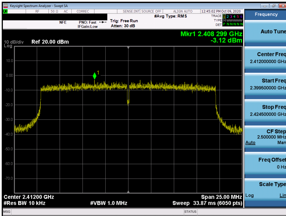
Plot 7-31. Power Spectral Density Plot MIMO ANT1 (802.11ax – Ch. 1)
