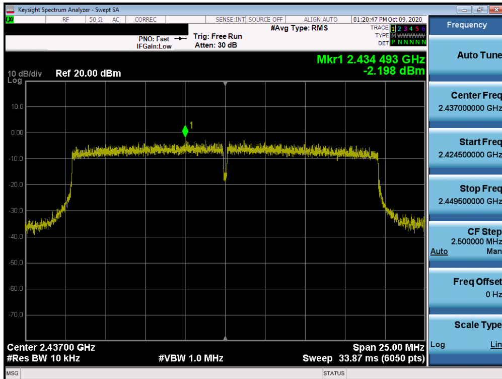
Plot 7-41. Power Spectral Density Plot MIMO ANT2 (802.11ax – Ch. 6)
