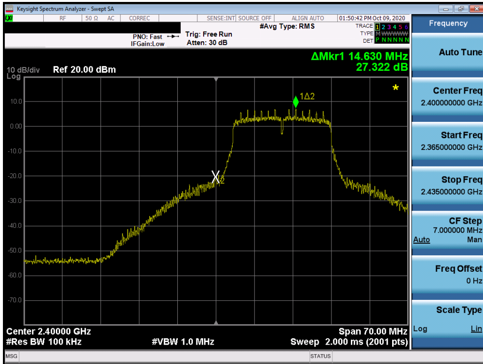
Plot 7-47. Band Edge Plot MIMO ANT1 (802.11n – Ch. 1)
