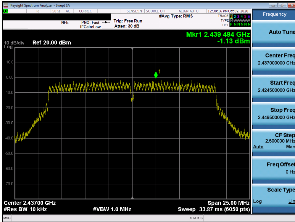
Plot 7-29. Power Spectral Density Plot MIMO ANT1 (802.11n – Ch. 6)
