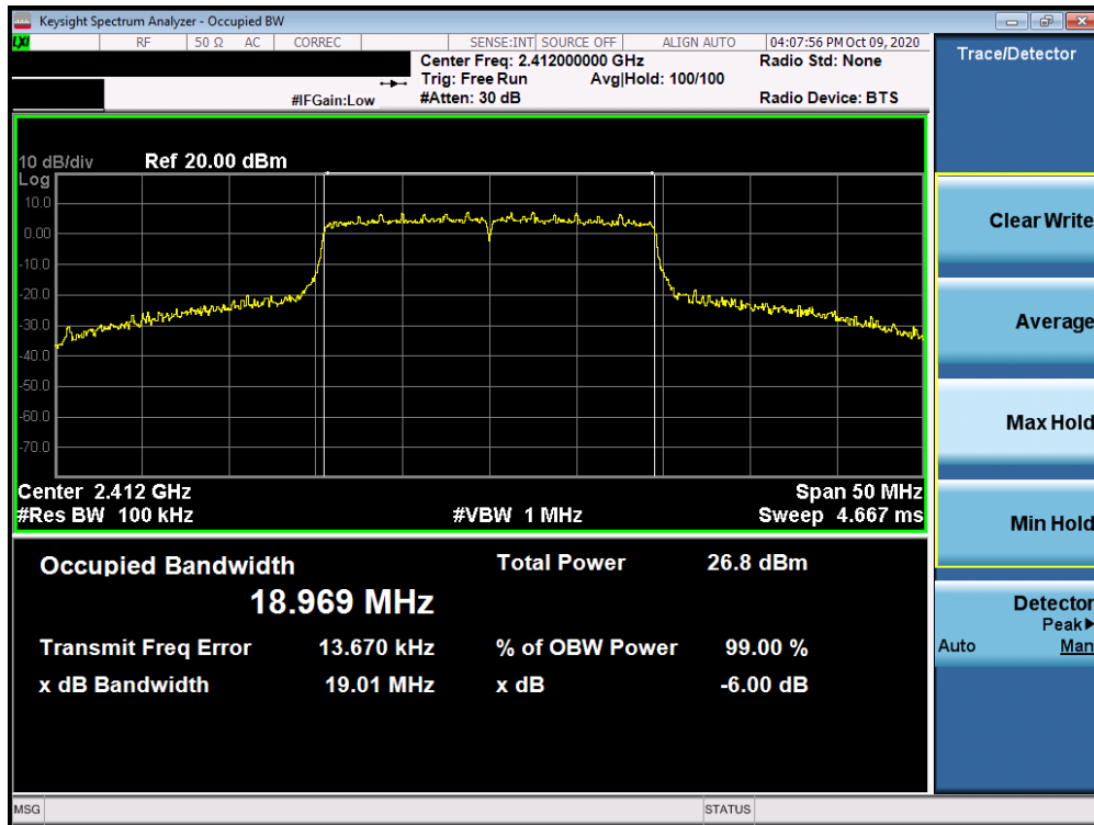
Plot 7-10. 6dB Bandwidth Plot MIMO ANT1 (802.11ax – Ch. 1)
