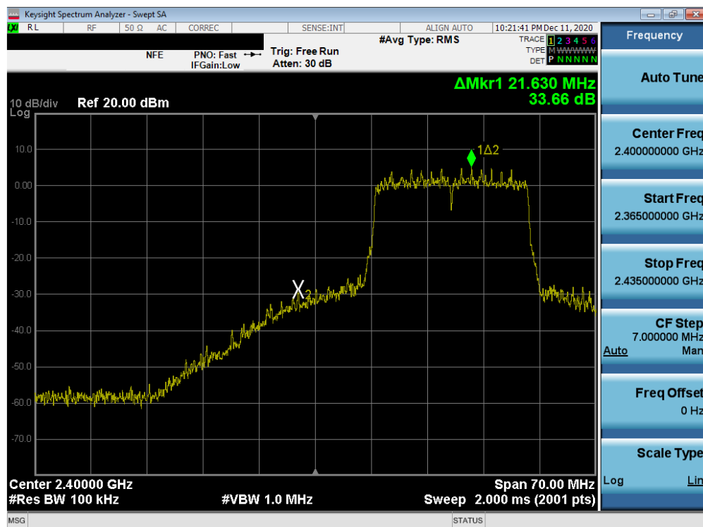
Plot 7-50. Band Edge Plot MIMO ANT1 (802.11ax – Ch. 2)
