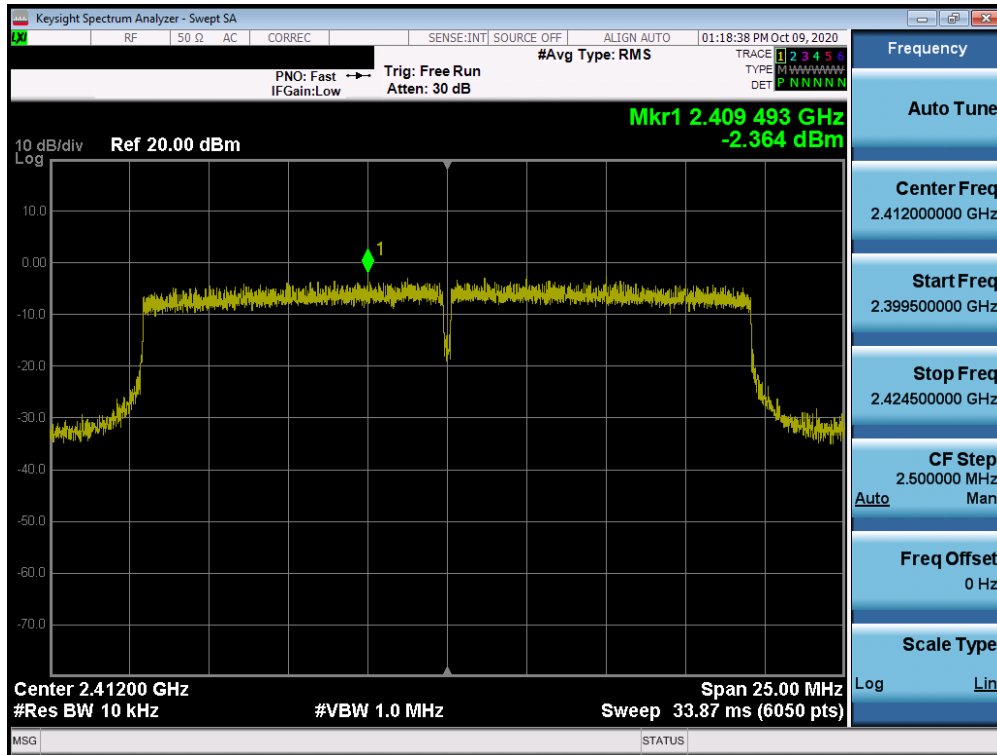
Plot 7-40. Power Spectral Density Plot MIMO ANT2 (802.11ax – Ch. 1)
