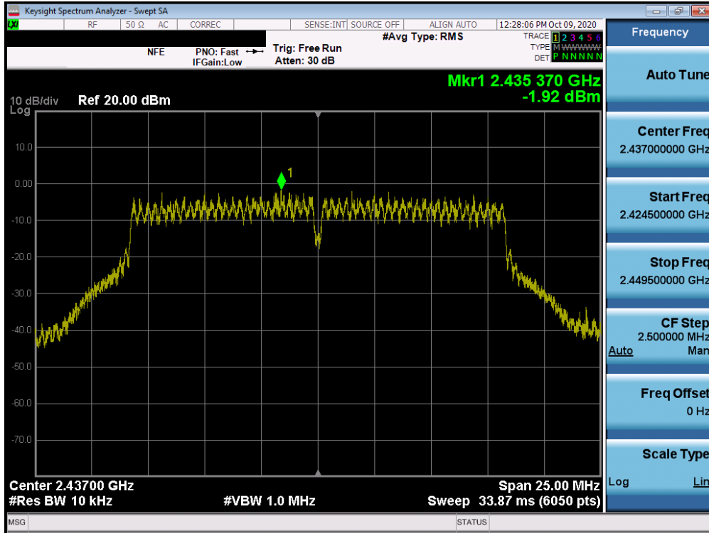
Plot 7-26. Power Spectral Density Plot MIMO ANT1 (802.11g – Ch. 6)
