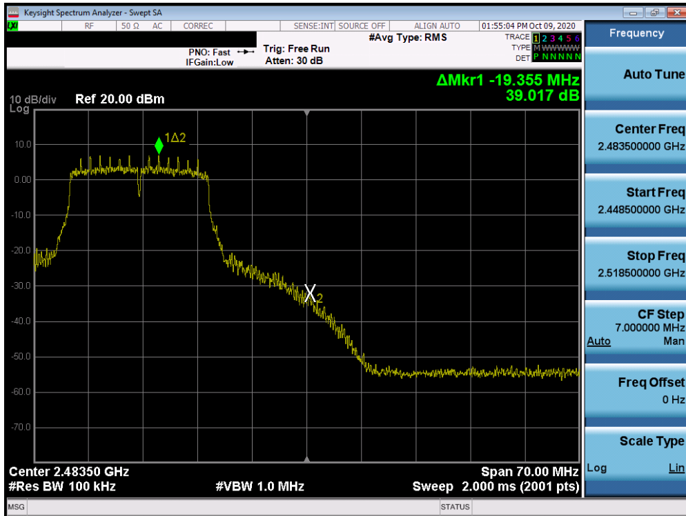
Plot 7-48. Band Edge Plot MIMO ANT1 (802.11n – Ch. 11)
