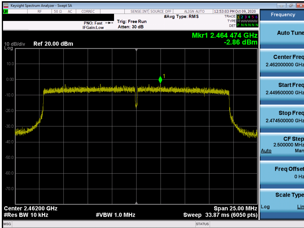
Plot 7-33. Power Spectral Density Plot MIMO ANT1 (802.11ax – Ch. 11)
