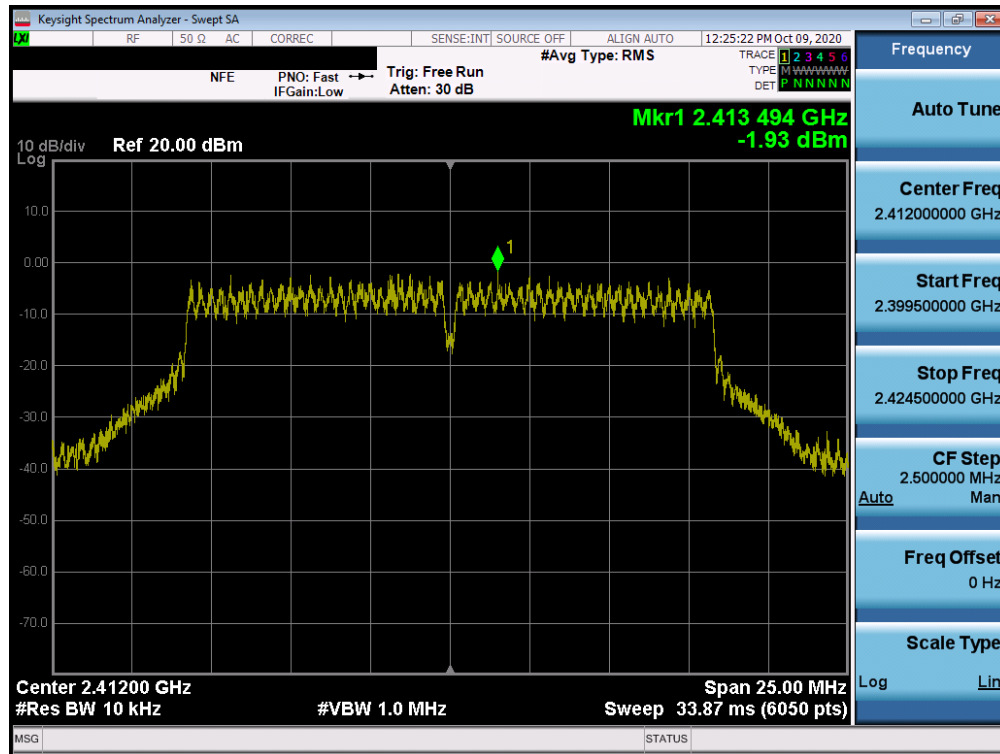
Plot 7-25. Power Spectral Density Plot MIMO ANT1 (802.11g – Ch. 1)
