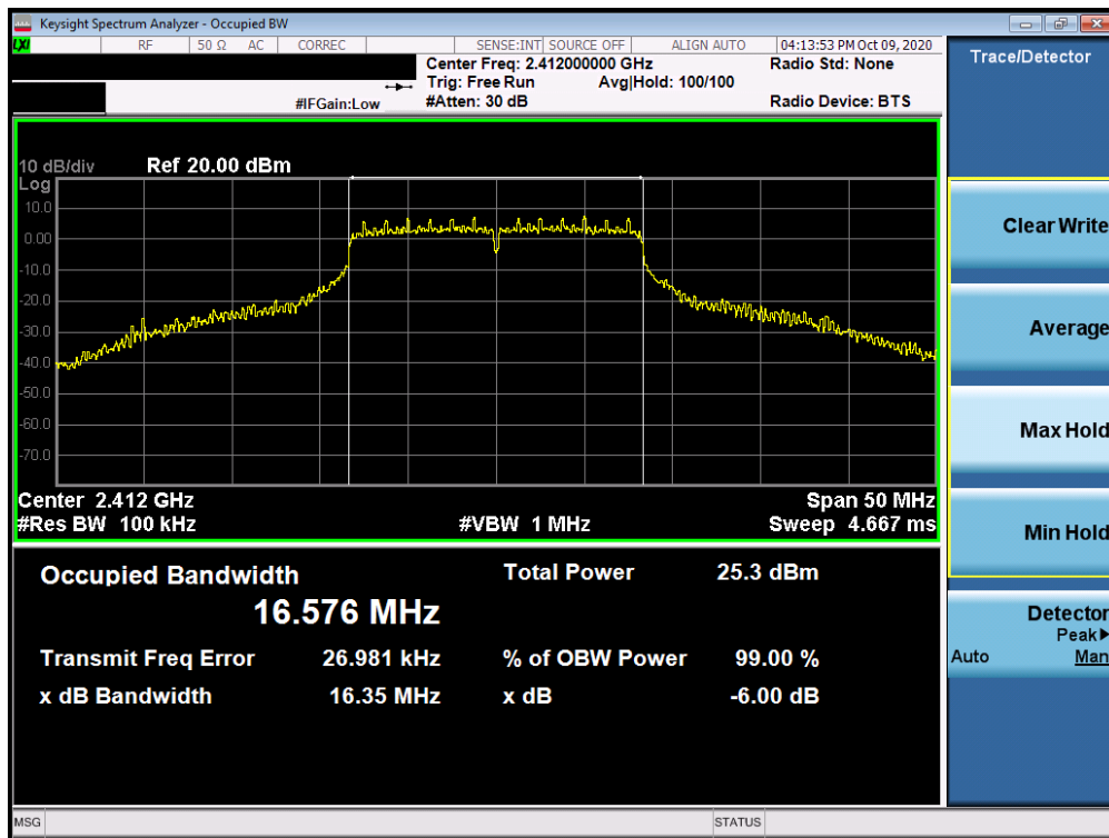
Plot 7-13. 6dB Bandwidth Plot MIMO ANT2 (802.11g – Ch. 1)
