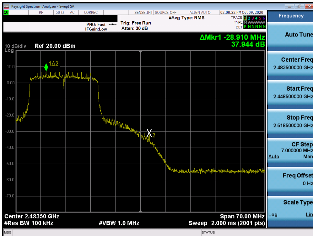
Plot 7-52. Band Edge Plot MIMO ANT1 (802.11ax – Ch. 11)
