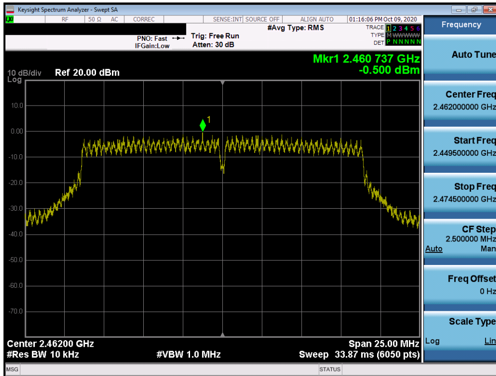
Plot 7-39. Power Spectral Density Plot MIMO ANT2 (802.11n – Ch. 11)
