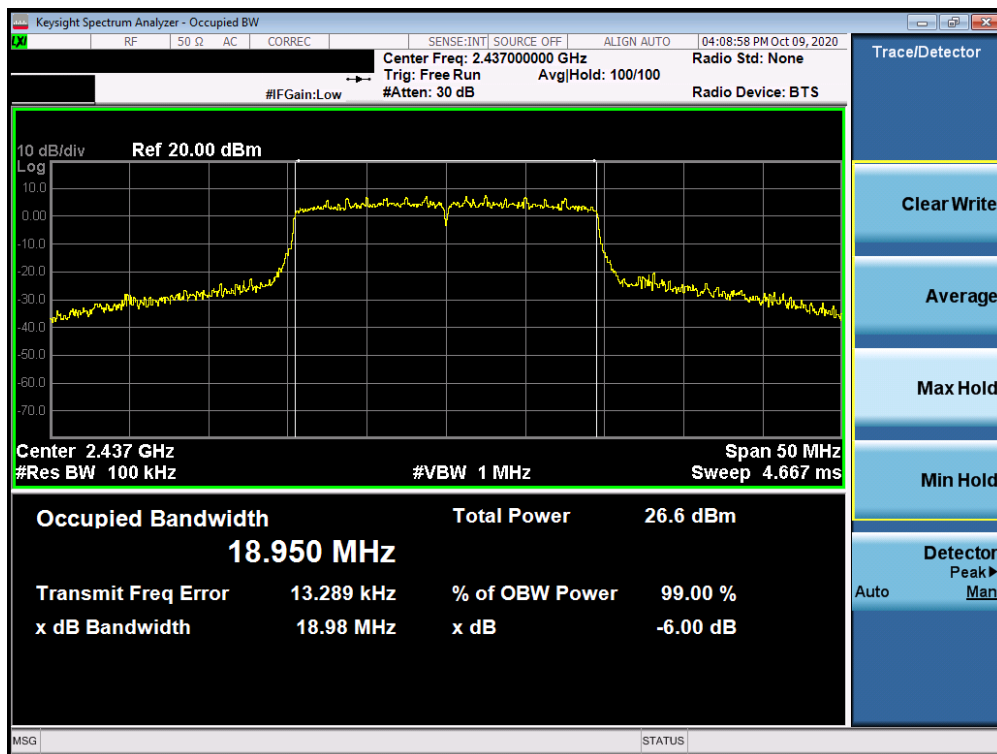
Plot 7-11. 6dB Bandwidth Plot MIMO ANT1 (802.11ax – Ch. 6)
