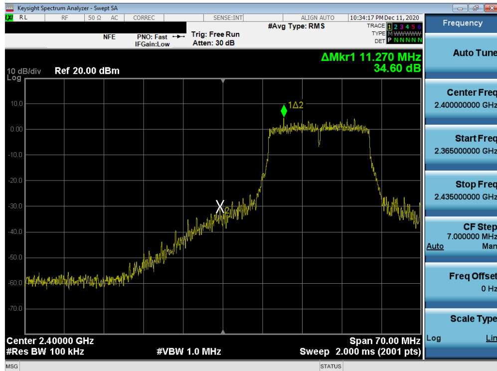
Plot 7-56. Band Edge Plot MIMO ANT2 (802.11ax – Ch. 2)
