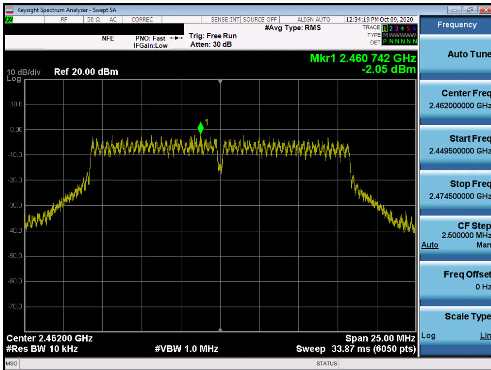
Plot 7-27. Power Spectral Density Plot MIMO ANT1 (802.11g – Ch. 11)
