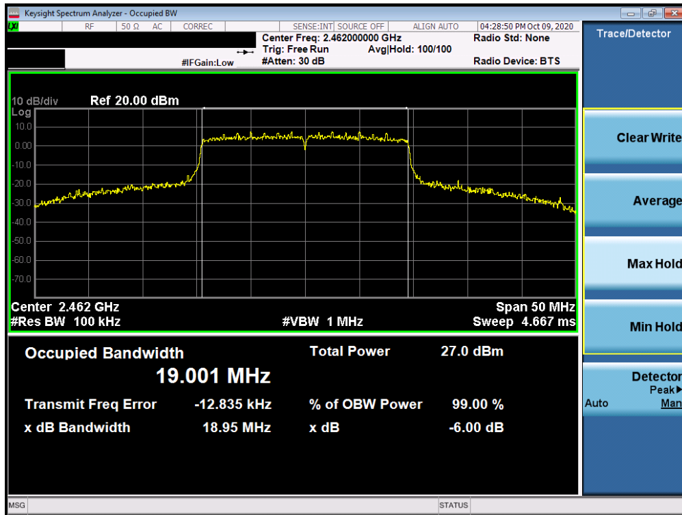
Plot 7-18. 6dB Bandwidth Plot MIMO ANT2 (802.11ax – Ch. 11)
