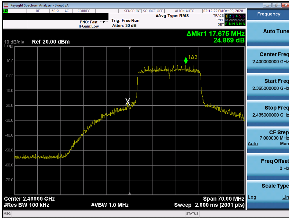
Plot 7-55. Band Edge Plot MIMO ANT2 (802.11ax – Ch. 1)
