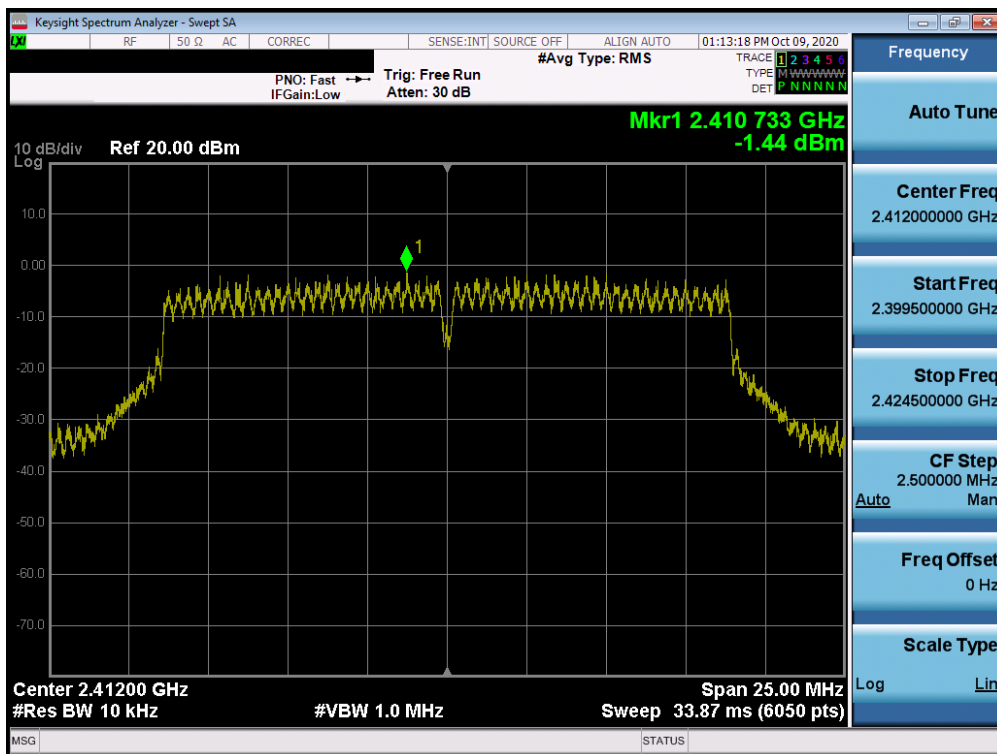
Plot 7-37. Power Spectral Density Plot MIMO ANT2 (802.11n – Ch. 1)
