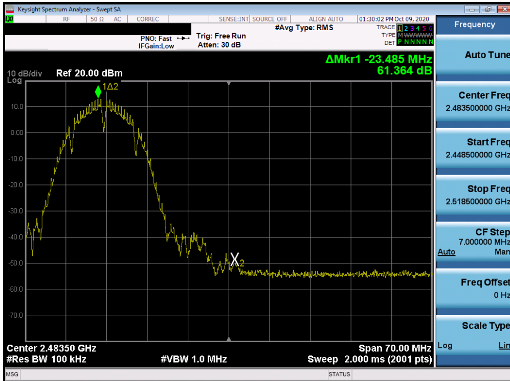
Plot 7-46. Band Edge Plot SISO ANT2 (802.11b – Ch. 11)
