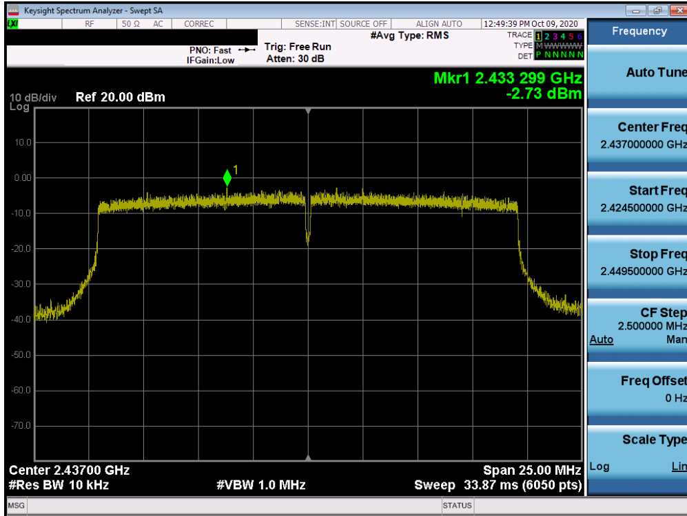
Plot 7-32. Power Spectral Density Plot MIMO ANT1 (802.11ax – Ch. 6)
