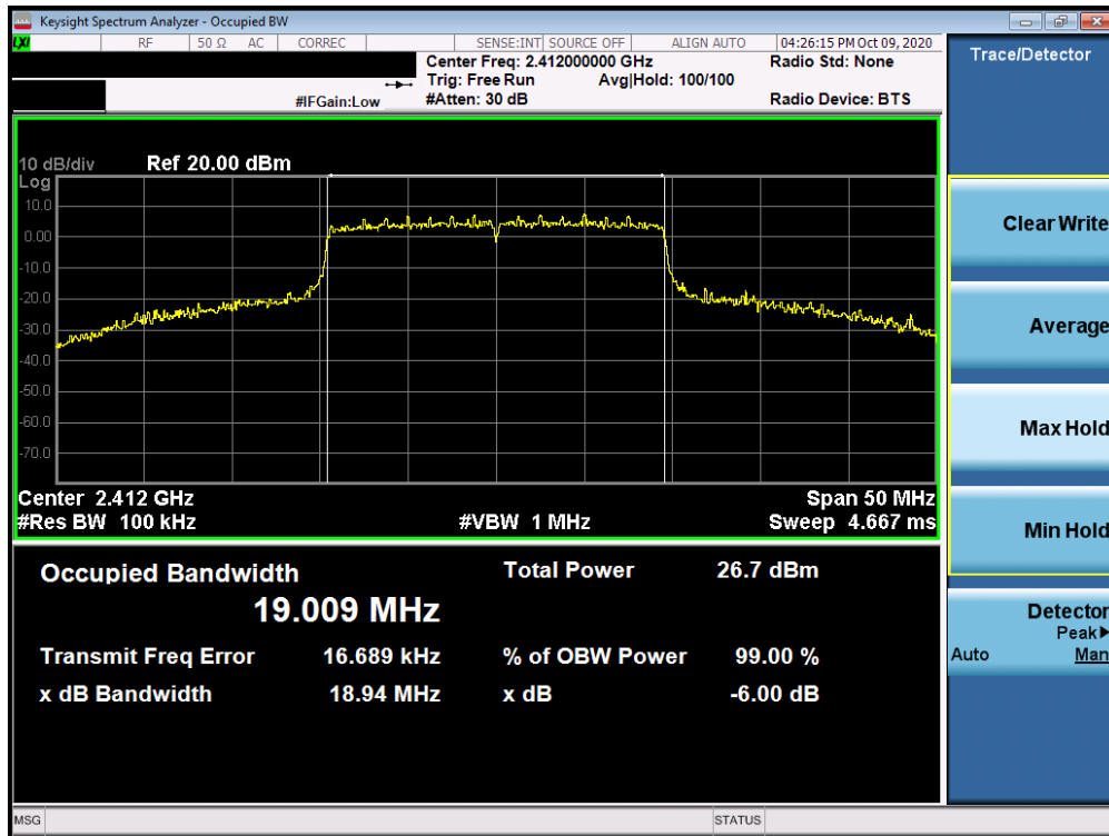
Plot 7-16. 6dB Bandwidth Plot MIMO ANT2 (802.11ax – Ch. 1)
