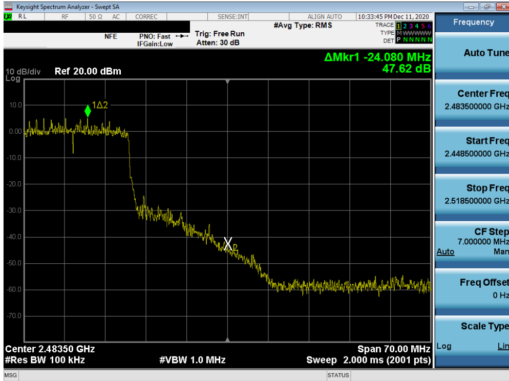
Plot 7-57. Band Edge Plot MIMO ANT2 (802.11ax – Ch. 10)
