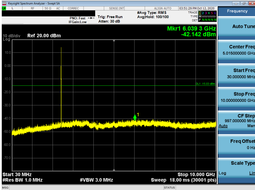
Plot 7-39. Conducted Spurious Plot MIMO ANT1 (802.11ax OFDMA – 26 Tones – Ch. 6)
