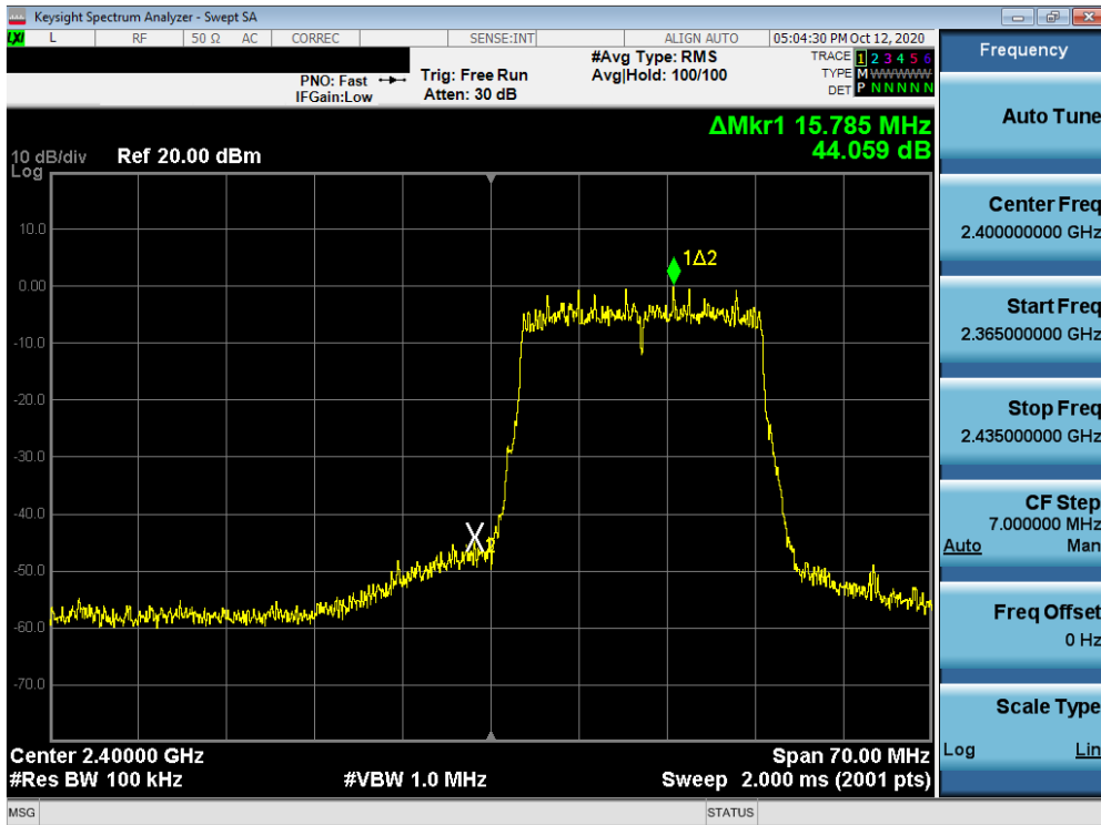
Plot 7-33. Band Edge Plot MIMO ANT2 (802.11ax OFDMA – 242 Tones – Ch. 1)
