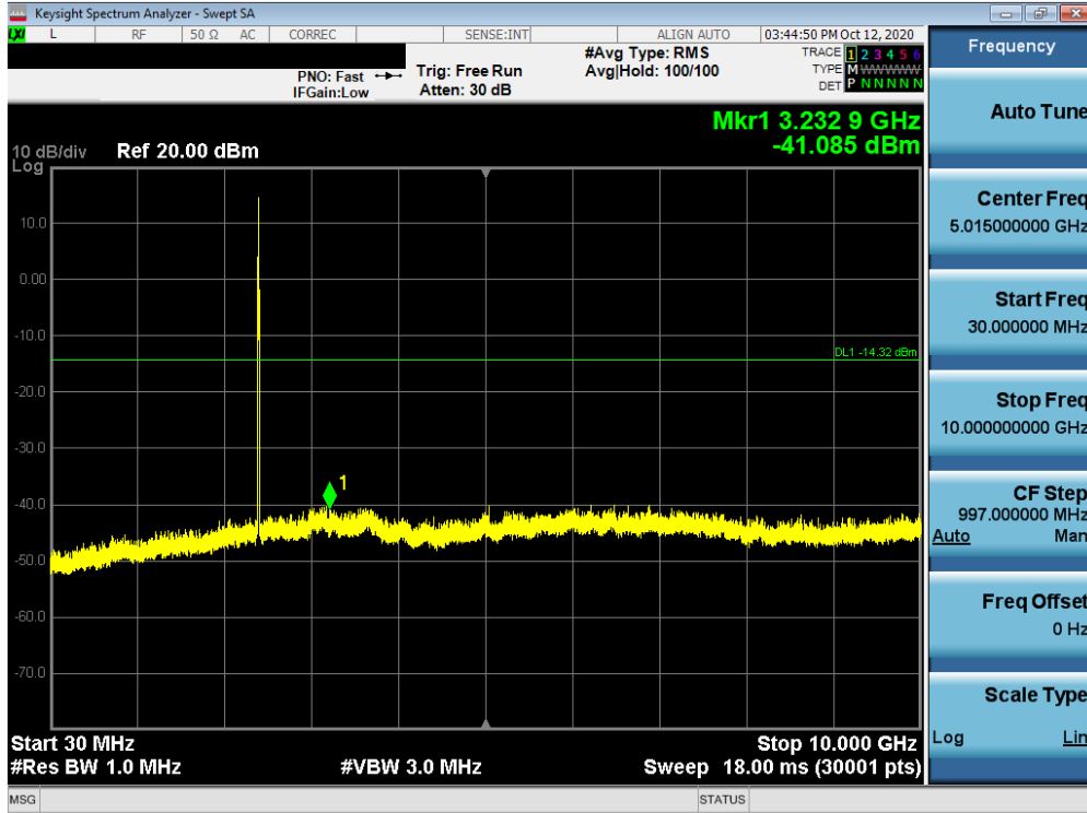
Plot 7-37. Conducted Spurious Plot MIMO ANT1 (802.11ax OFDMA – 26 Tones – Ch. 1)
