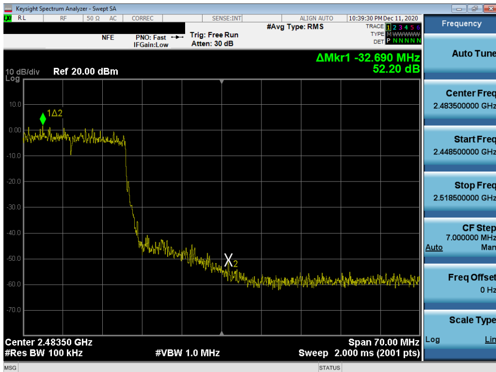
Plot 7-29. Band Edge Plot MIMO ANT1 (802.11ax OFDMA – 242 Tones – Ch. 10)
