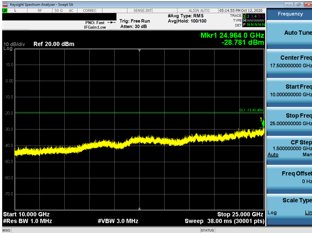
Plot 7-60. Conducted Spurious Plot MIMO ANT2 (802.11ax OFDMA – 242 Tones – Ch. 11)
