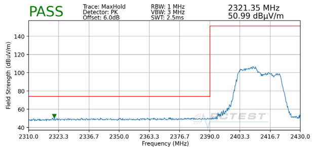
Plot 7-70. Radiated Restricted Lower Band Edge Measurement MIMO (Peak – 106 Tones)
