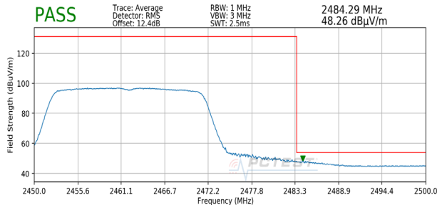
Plot 7-79. Radiated Restricted Upper Band Edge Measurement MIMO (Average – 242 Tones)
