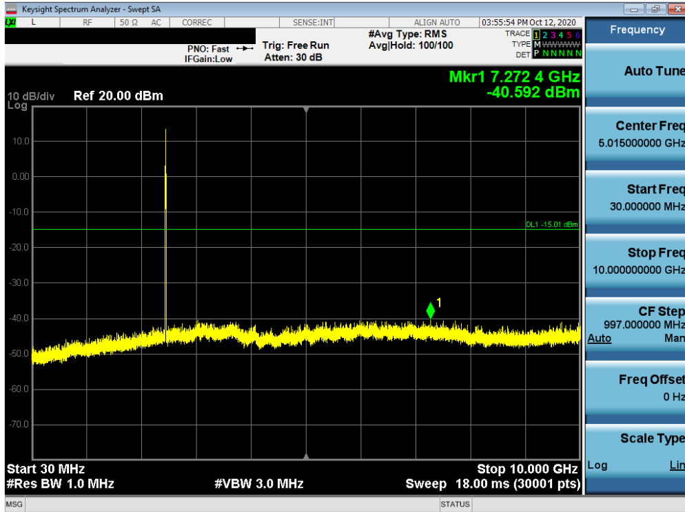
Plot 7-41. Conducted Spurious Plot MIMO ANT1 (802.11ax OFDMA – 26 Tones – Ch. 11)
