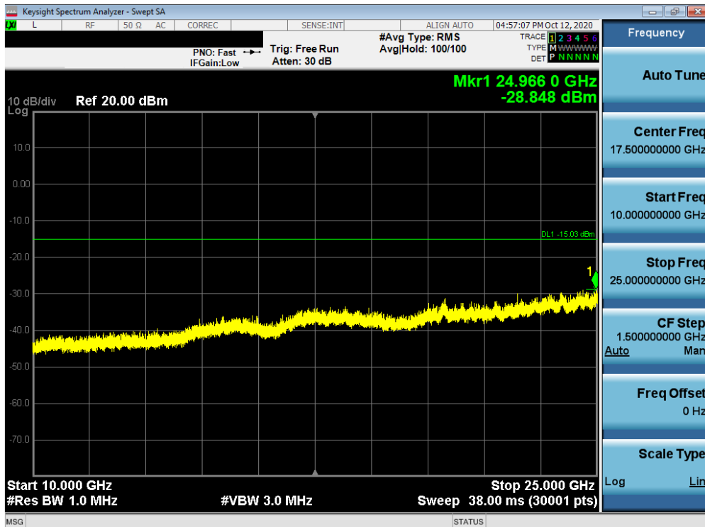
Plot 7-52. Conducted Spurious Plot MIMO ANT2 (802.11ax OFDMA – 26 Tones – Ch. 6)
