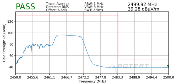
Plot 7-71. Radiated Restricted Upper Band Edge Measurement MIMO (Average – 106 Tones)
