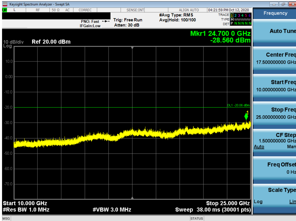
Plot 7-48. Conducted Spurious Plot MIMO ANT1 (802.11ax OFDMA – 242 Tones – Ch. 11)
