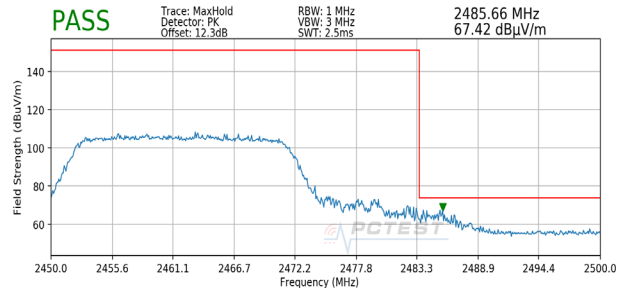
Plot 7-80. Radiated Restricted Upper Band Edge Measurement MIMO (Peak – 242 Tones)
