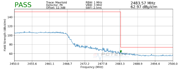
Plot 7-78. Radiated Restricted Upper Band Edge Measurement MIMO (Peak – 242 Tones)
