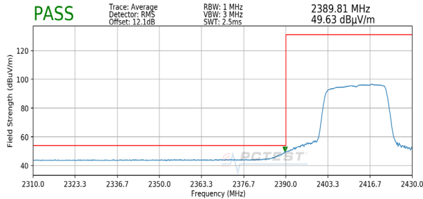
Plot 7-73. Radiated Restricted Lower Band Edge Measurement MIMO (Average – 242 Tones)
