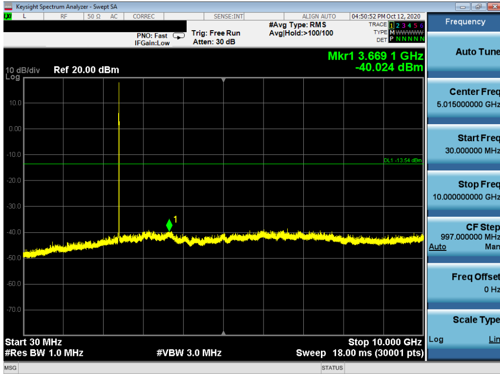
Plot 7-49. Conducted Spurious Plot MIMO ANT2 (802.11ax OFDMA – 26 Tones – Ch. 1)
