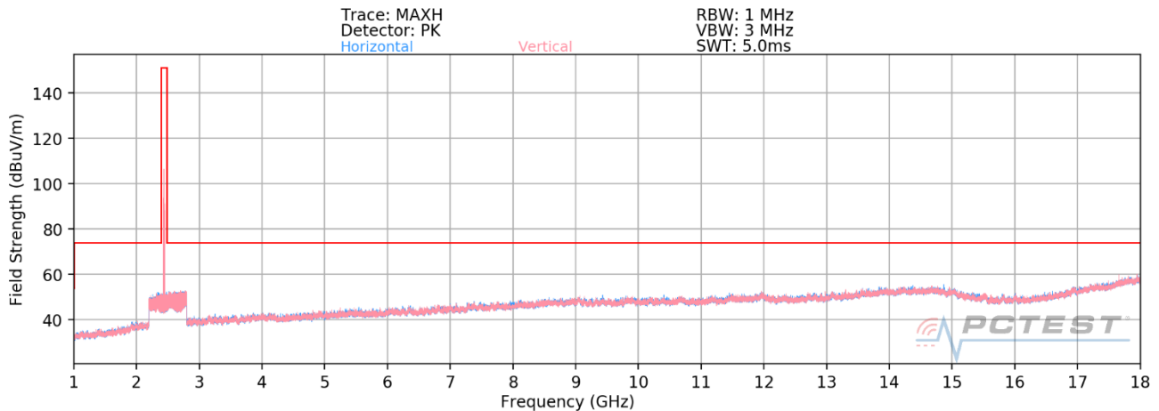
Plot 7-62. Radiated Spurious Plot above 1GHz MIMO (802.11ax OFDMA – 106 Tones – Ch. 6)
