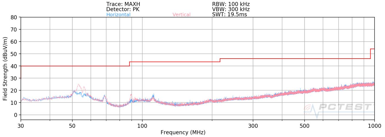
Plot 7-81. Radiated Spurious Plot below 1GHz (106 Tones)
