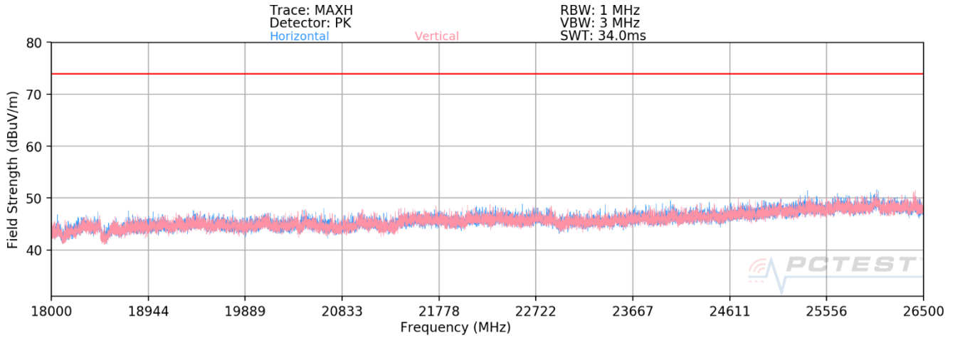
Plot 7-67. Radiated Spurious Plot above 18GHz MIMO (802.11ax OFDMA – 106 Tones)
