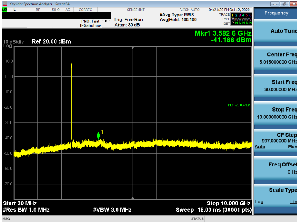
Plot 7-47. Conducted Spurious Plot MIMO ANT1 (802.11ax OFDMA – 242 Tones – Ch. 11)
