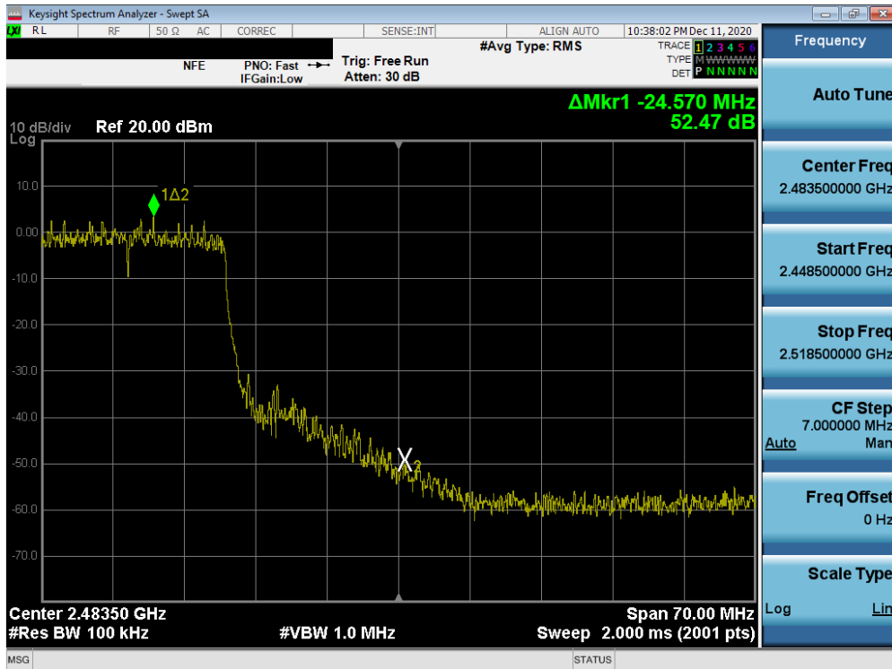
Plot 7-35. Band Edge Plot MIMO ANT2 (802.11ax OFDMA – 242 Tones – Ch. 10)
