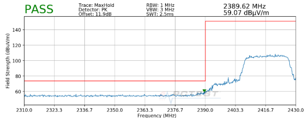
Plot 7-76. Radiated Restricted Lower Band Edge Measurement MIMO (Peak – 242 Tones)
