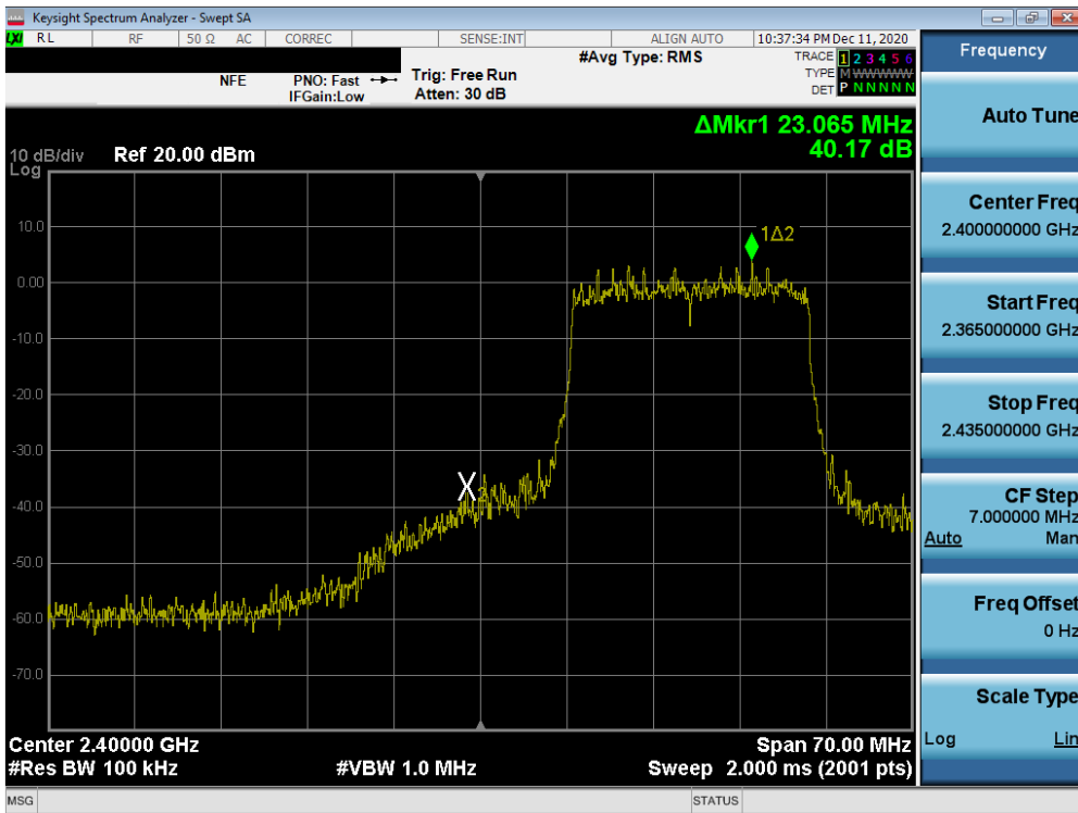
Plot 7-34. Band Edge Plot MIMO ANT2 (802.11ax OFDMA – 242 Tones – Ch. 2)
