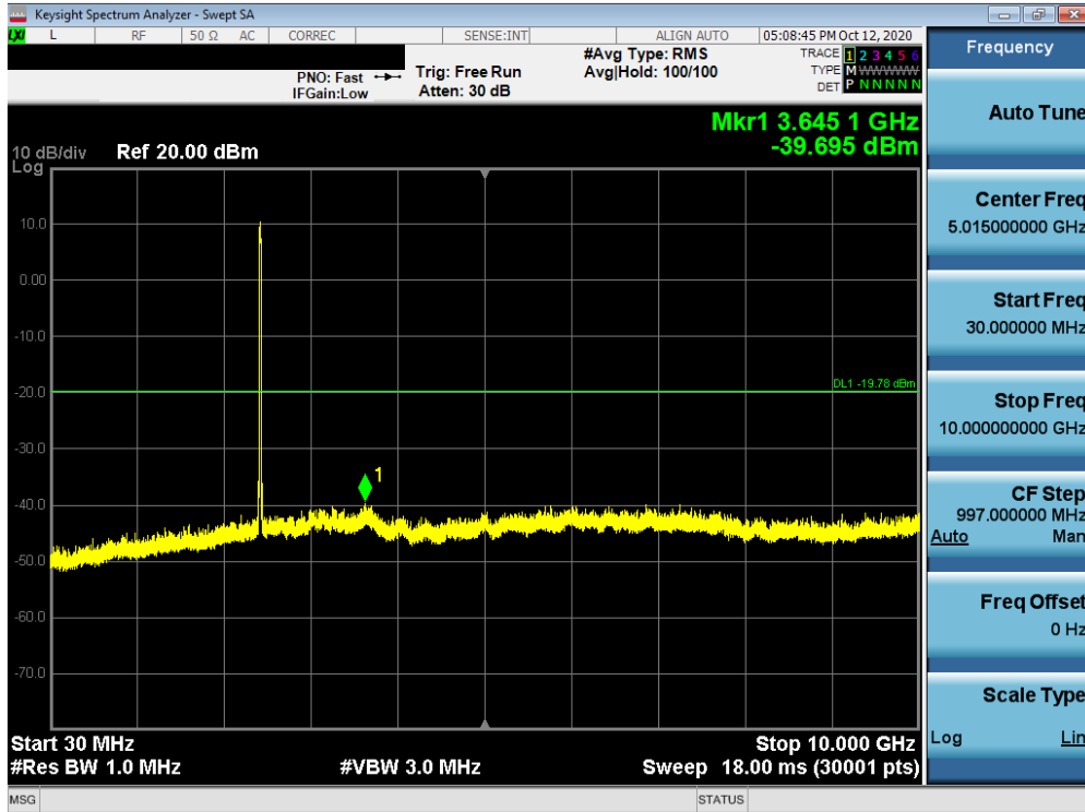
Plot 7-57. Conducted Spurious Plot MIMO ANT2 (802.11ax OFDMA – 242 Tones – Ch. 6)
