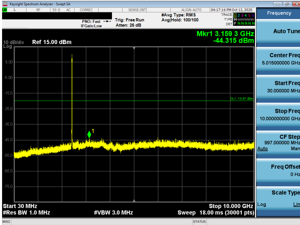
Plot 7-45. Conducted Spurious Plot MIMO ANT1 (802.11ax OFDMA – 242 Tones – Ch. 6)
