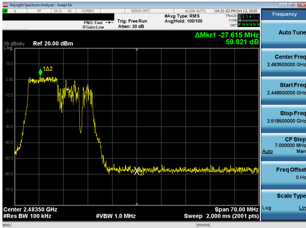
Plot 7-32. Band Edge Plot MIMO ANT2 (802.11ax OFDMA – 106 Tones – Ch. 11)
