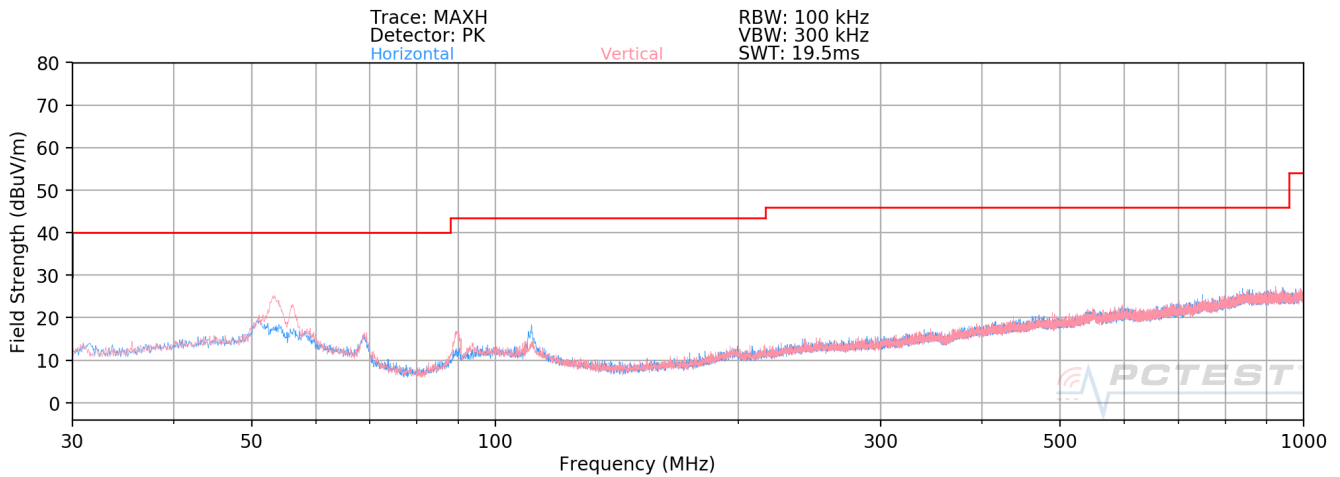
Plot 7-82. Radiated Spurious Plot below 1GHz (242 Tones)
