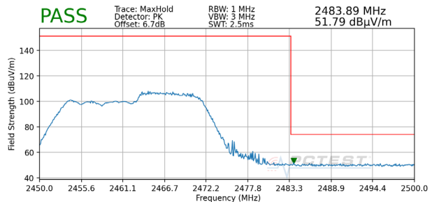
Plot 7-72. Radiated Restricted Upper Band Edge Measurement MIMO (Peak – 106 Tones)
