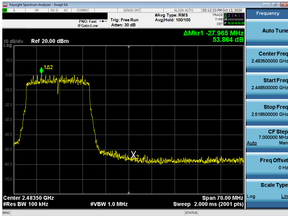
Plot 7-36. Band Edge Plot MIMO ANT2 (802.11ax OFDMA – 242 Tones – Ch. 11)
