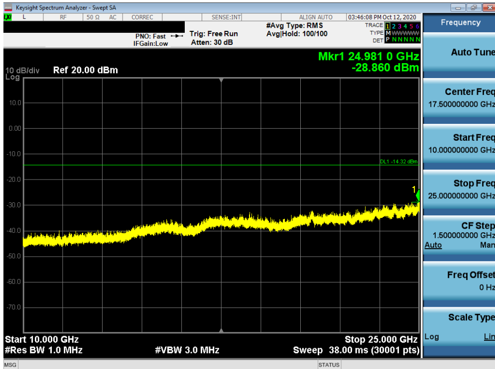
Plot 7-38. Conducted Spurious Plot MIMO ANT1 (802.11ax OFDMA – 26 Tones – Ch. 1)
