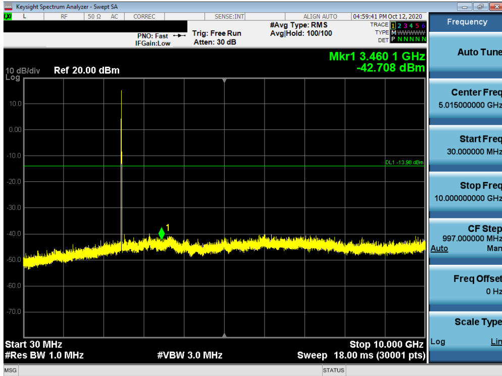
Plot 7-53. Conducted Spurious Plot MIMO ANT2 (802.11ax OFDMA – 26 Tones – Ch. 11)
