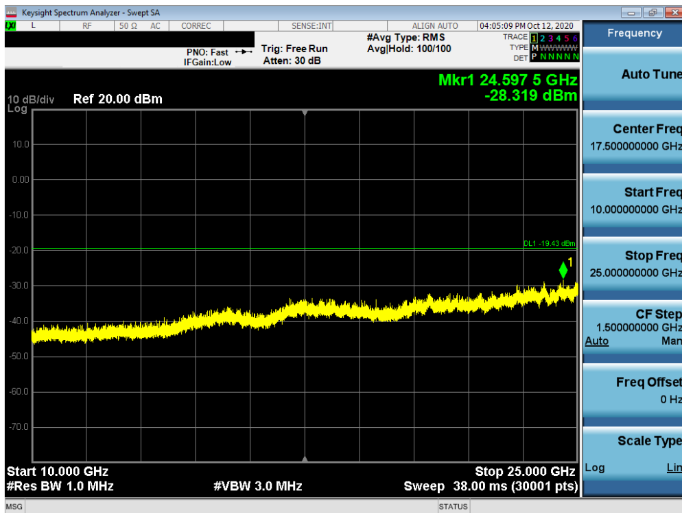
Plot 7-44. Conducted Spurious Plot MIMO ANT1 (802.11ax OFDMA – 242 Tones – Ch. 1)
