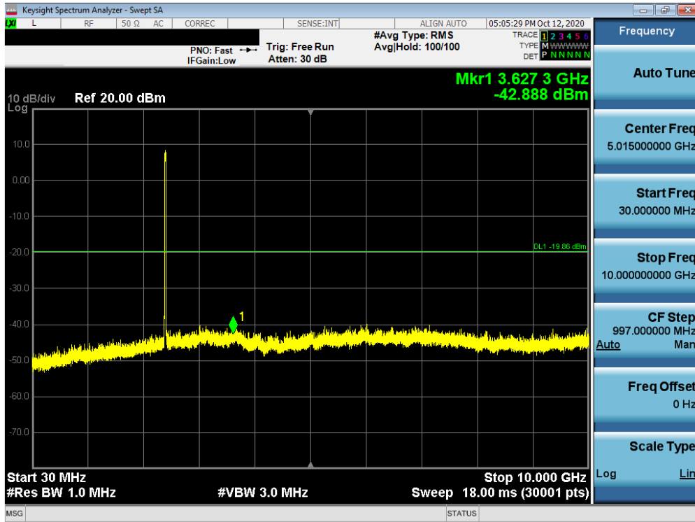
Plot 7-55. Conducted Spurious Plot MIMO ANT2 (802.11ax OFDMA – 242 Tones – Ch. 1)
