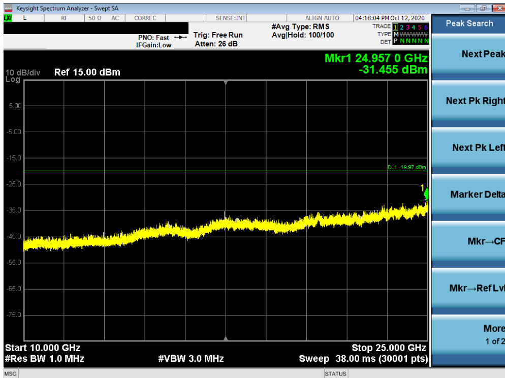
Plot 7-46. Conducted Spurious Plot MIMO ANT1 (802.11ax OFDMA – 242 Tones – Ch. 6)
