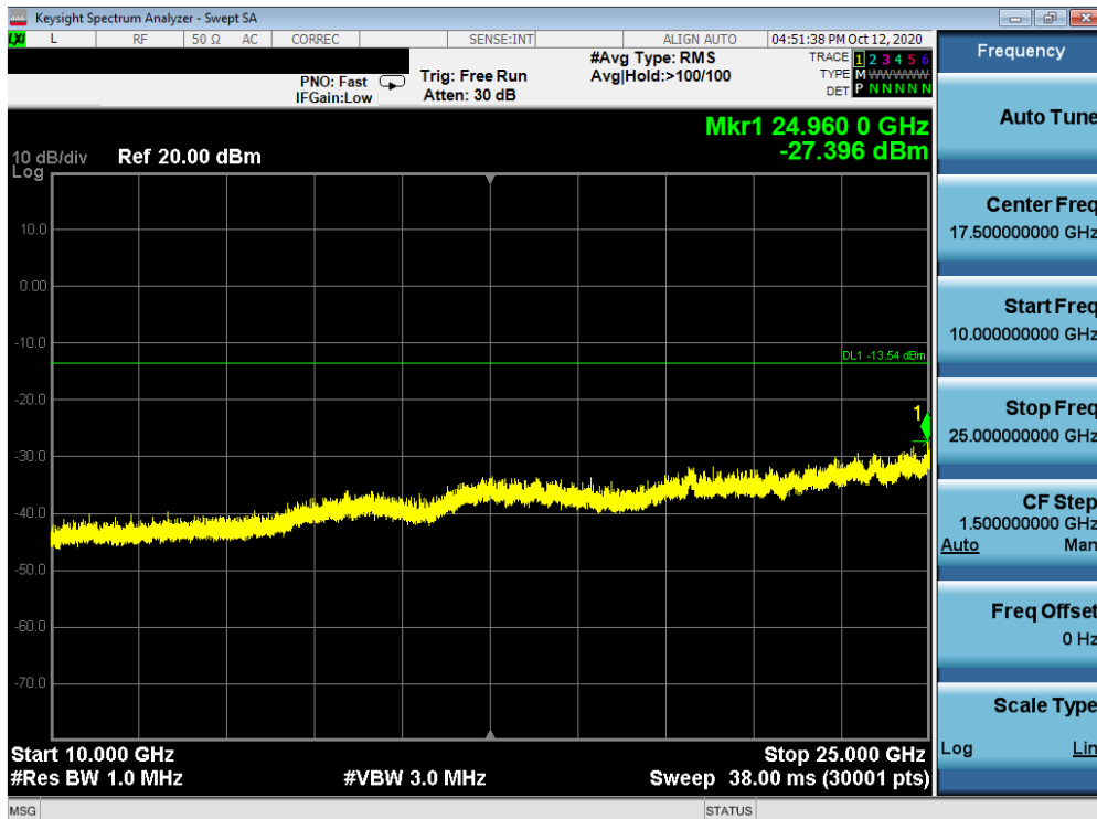
Plot 7-50. Conducted Spurious Plot MIMO ANT2 (802.11ax OFDMA – 26 Tones – Ch. 1)
