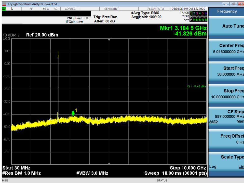
Plot 7-43. Conducted Spurious Plot MIMO ANT1 (802.11ax OFDMA – 242 Tones – Ch. 1)
