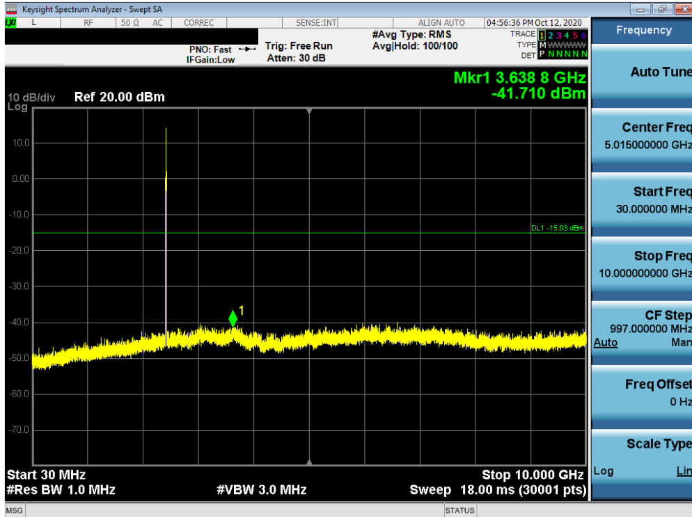
Plot 7-51. Conducted Spurious Plot MIMO ANT2 (802.11ax OFDMA – 26 Tones – Ch. 6)
