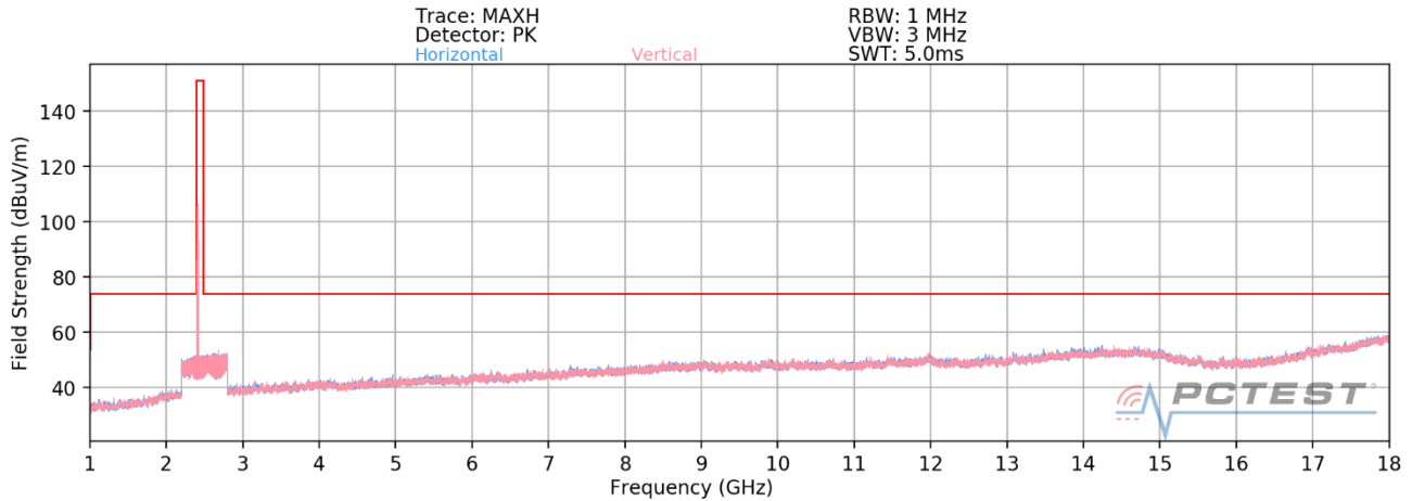
Plot 7-61. Radiated Spurious Plot above 1GHz MIMO (802.11ax OFDMA – 106 Tones – Ch. 1)
