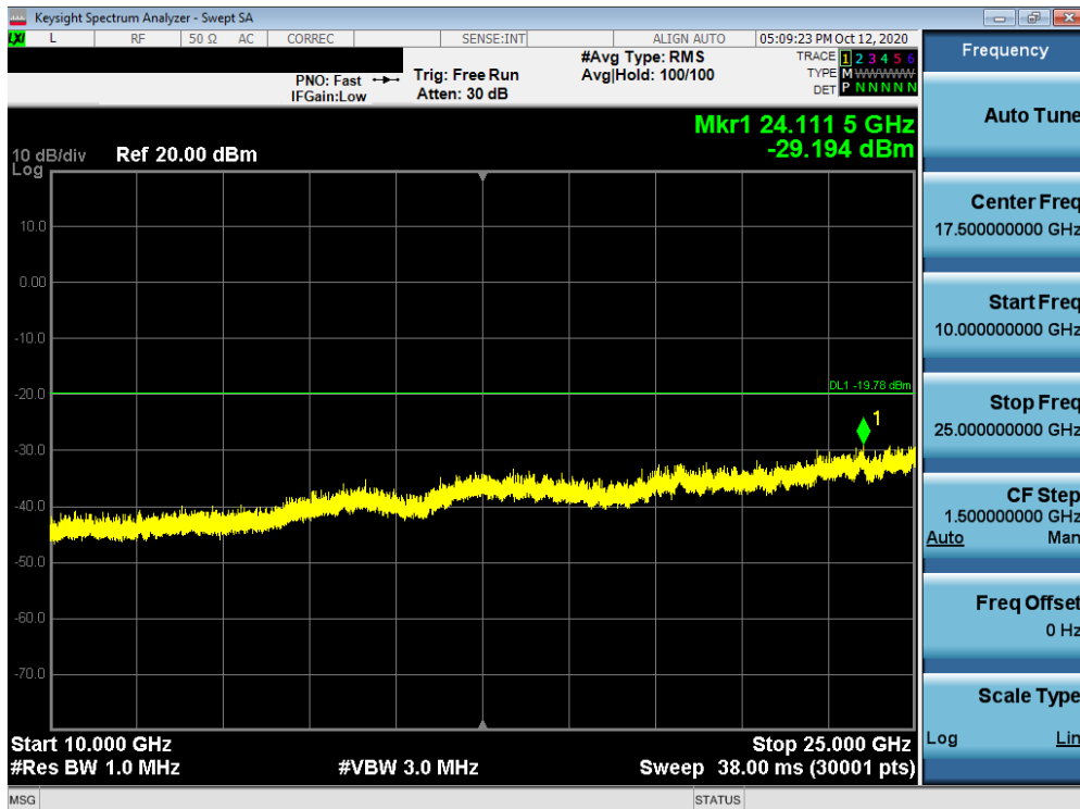
Plot 7-58. Conducted Spurious Plot MIMO ANT2 (802.11ax OFDMA – 242 Tones – Ch. 6)
