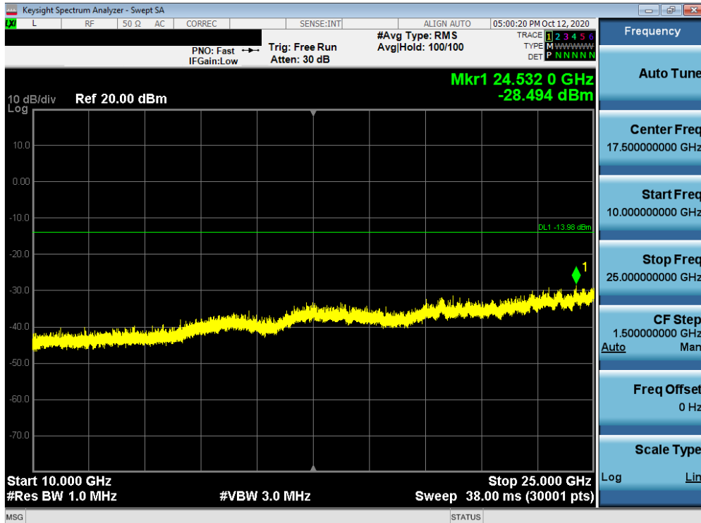
Plot 7-54. Conducted Spurious Plot MIMO ANT2 (802.11ax OFDMA – 26 Tones – Ch. 11)
