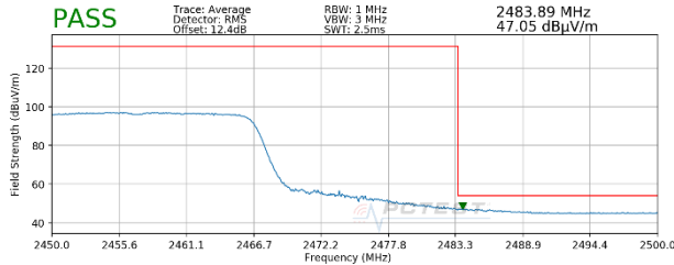
Plot 7-77. Radiated Restricted Upper Band Edge Measurement MIMO (Average – 242 Tones)
