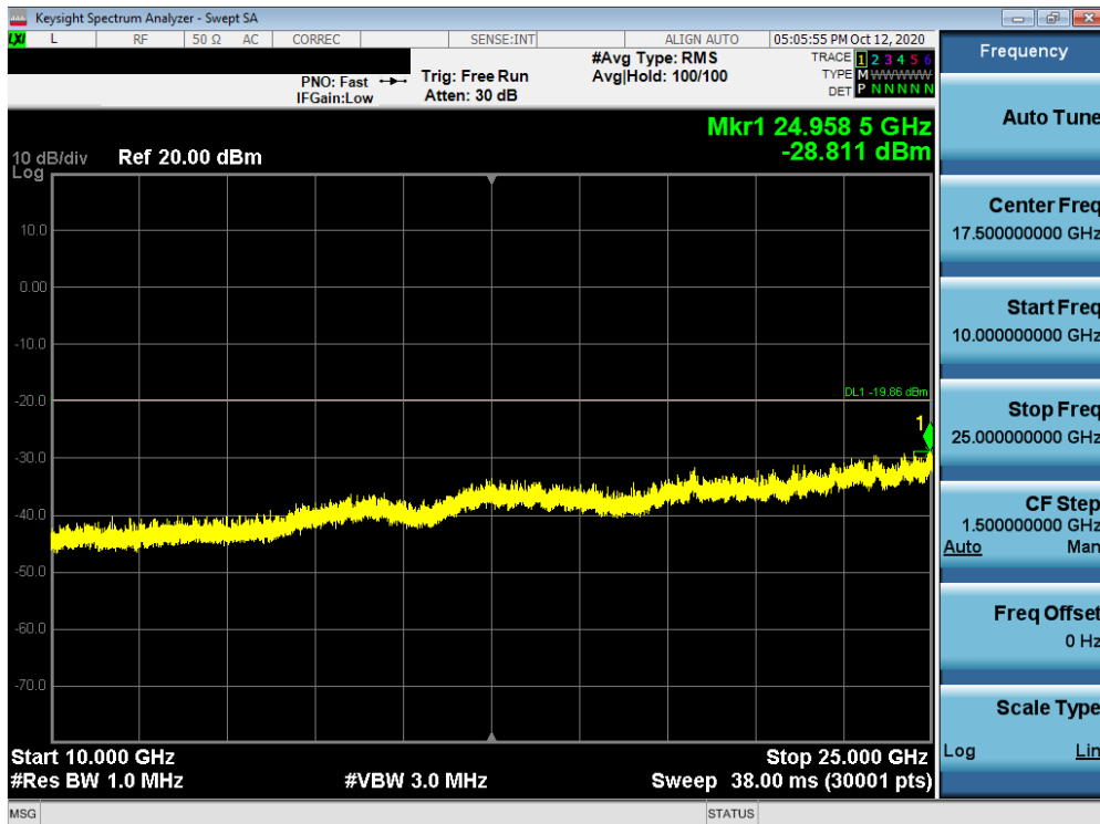
Plot 7-56. Conducted Spurious Plot MIMO ANT2 (802.11ax OFDMA – 242 Tones – Ch. 1)
