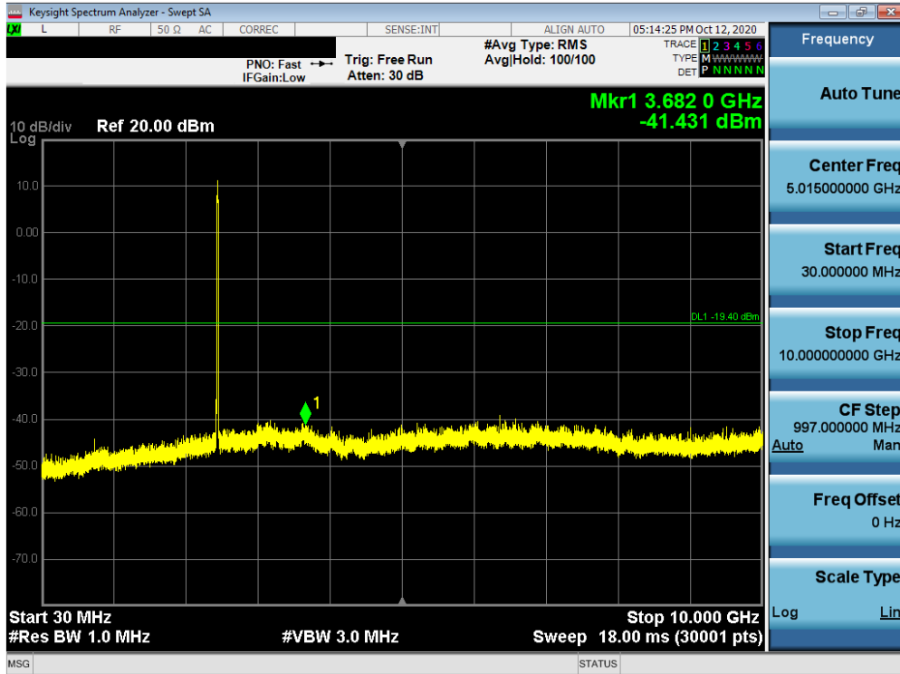
Plot 7-59. Conducted Spurious Plot MIMO ANT2 (802.11ax OFDMA – 242 Tones – Ch. 11)
