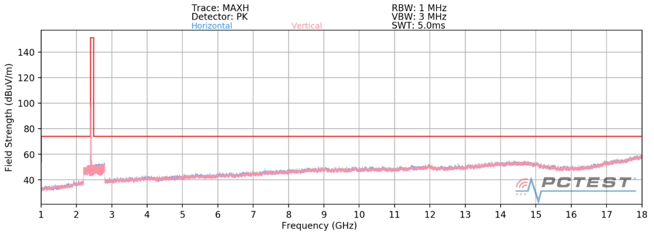
Plot 7-64. Radiated Spurious Plot above 1GHz MIMO (802.11ax OFDMA – 242 Tones – Ch. 1)
