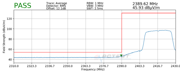
Plot 7-75. Radiated Restricted Lower Band Edge Measurement MIMO (Average – 242 Tones)
