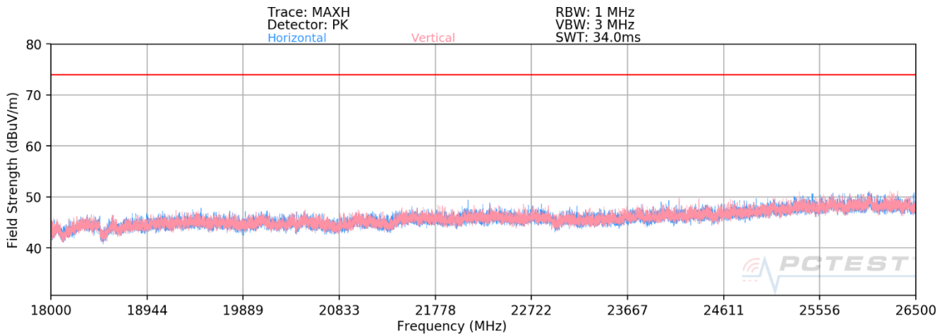
Plot 7-68. Radiated Spurious Plot above 18GHz MIMO (802.11ax OFDMA – 242 Tones)
