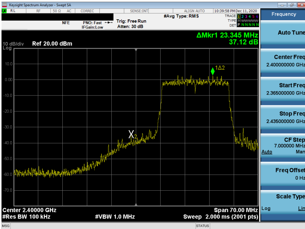
Plot 7-28. Band Edge Plot MIMO ANT1 (802.11ax OFDMA – 242 Tones – Ch. 2)
