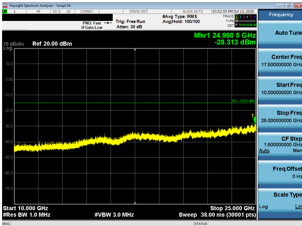
Plot 7-40. Conducted Spurious Plot MIMO ANT1 (802.11ax OFDMA – 26 Tones – Ch. 6)
