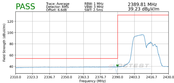
Plot 7-69. Radiated Restricted Lower Band Edge Measurement MIMO (Average – 106 Tones)
