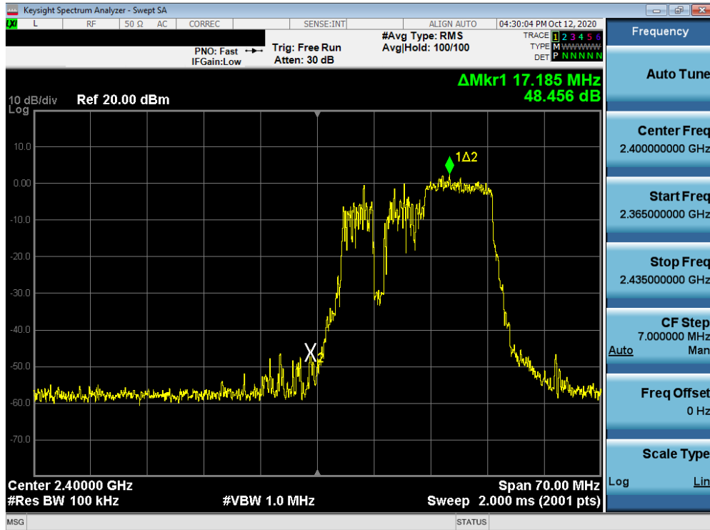
Plot 7-31. Band Edge Plot MIMO ANT2 (802.11ax OFDMA – 106 Tones – Ch. 1)
