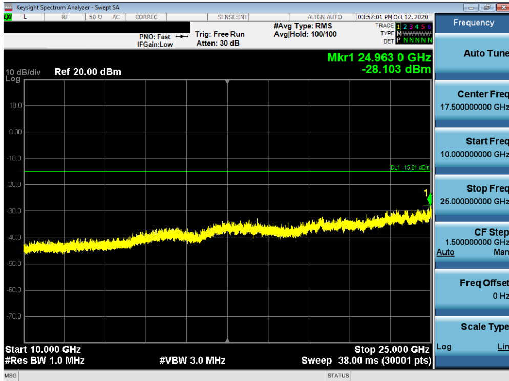
Plot 7-42. Conducted Spurious Plot MIMO ANT1 (802.11ax OFDMA – 26 Tones – Ch. 11)
