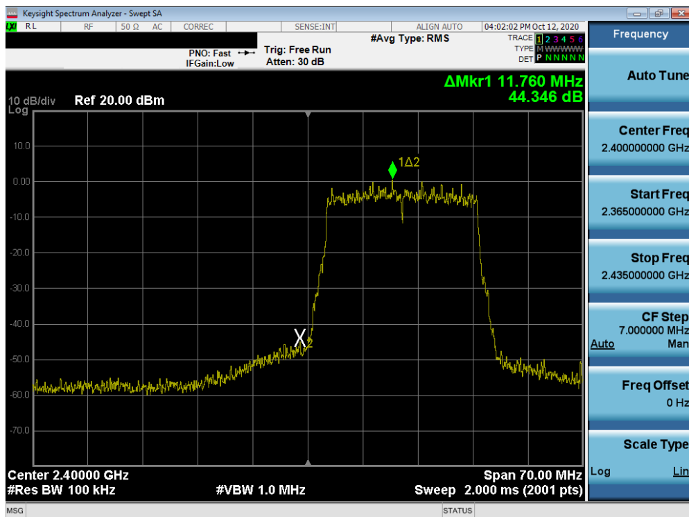
Plot 7-28. Band Edge Plot MIMO ANT1 (802.11ax OFDMA – 242 Tones – Ch. 1)
