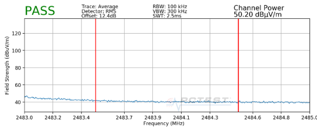
Plot 7-87. Radiated Restricted Upper Band Edge Measurement MIMO (Average – 242 Tones)
