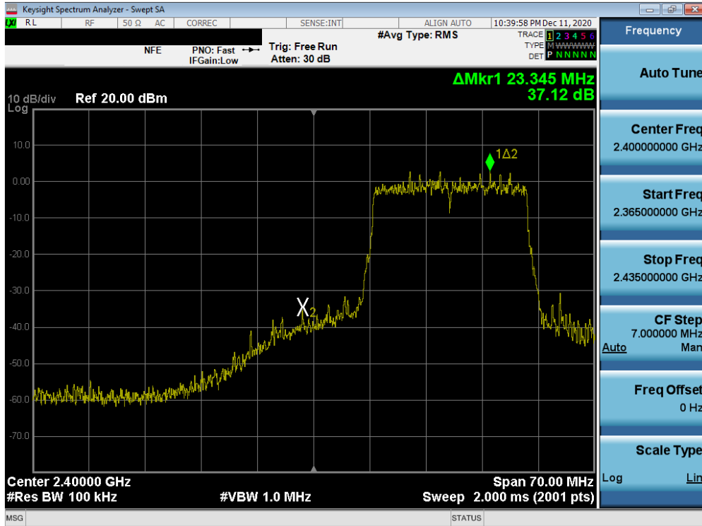
Plot 7-29. Band Edge Plot MIMO ANT1 (802.11ax OFDMA – 242 Tones – Ch. 2)
