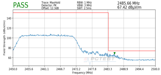
Plot 7-86. Radiated Restricted Upper Band Edge Measurement MIMO (Peak – 242 Tones)
