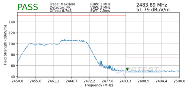
Plot 7-76. Radiated Restricted Upper Band Edge Measurement MIMO (Peak – 106 Tones)
