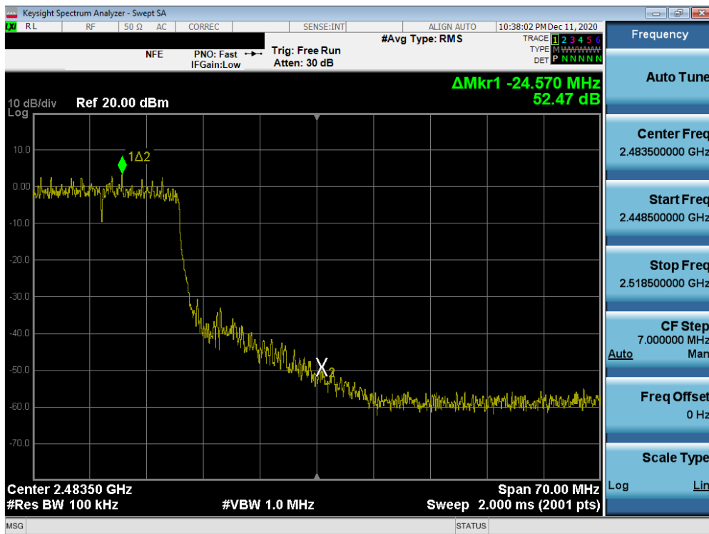
Plot 7-38. Band Edge Plot MIMO ANT2 (802.11ax OFDMA – 242 Tones – Ch. 10)
