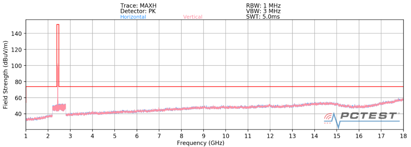
Plot 7-69. Radiated Spurious Plot above 1GHz MIMO (802.11ax OFDMA – 242 Tones – Ch. 6)
