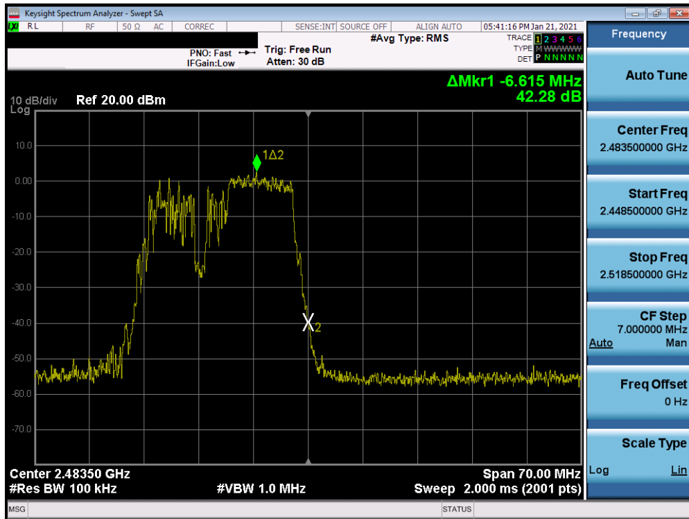
Plot 7-27. Band Edge Plot MIMO ANT1 (802.11ax OFDMA – 106 Tones – Ch. 13)
