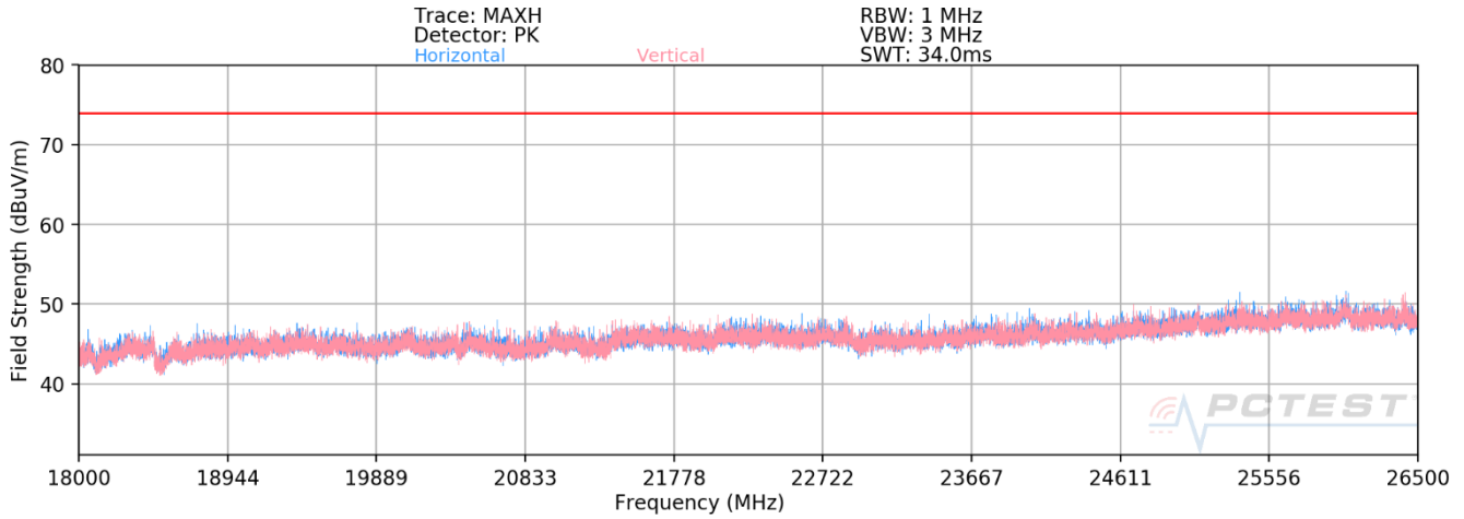
Plot 7-71. Radiated Spurious Plot above 18GHz MIMO (802.11ax OFDMA – 106 Tones)
