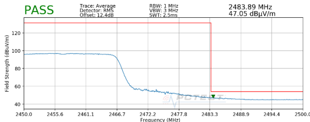
Plot 7-83. Radiated Restricted Upper Band Edge Measurement MIMO (Average – 242 Tones)
