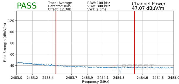
Plot 7-77. Radiated Restricted Upper Band Edge Measurement MIMO (Average – 106 Tones)
