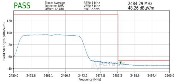
Plot 7-85. Radiated Restricted Upper Band Edge Measurement MIMO (Average – 242 Tones)
