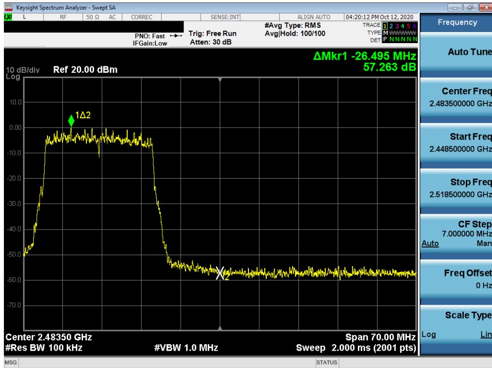
Plot 7-31. Band Edge Plot MIMO ANT1 (802.11ax OFDMA – 242 Tones – Ch. 11)
