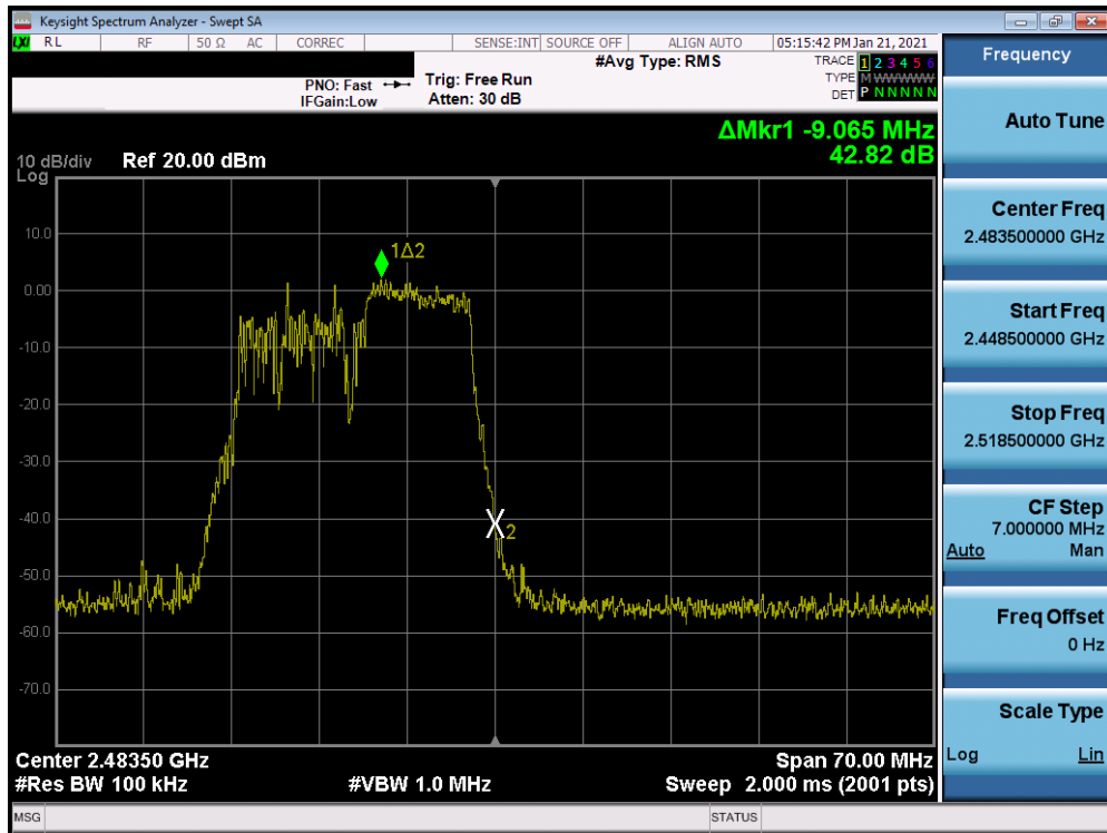
Plot 7-35. Band Edge Plot MIMO ANT2 (802.11ax OFDMA – 106 Tones – Ch. 13)
