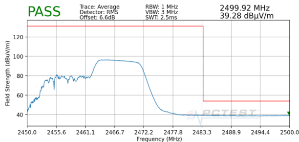
Plot 7-75. Radiated Restricted Upper Band Edge Measurement MIMO (Average – 106 Tones)
