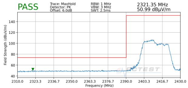
Plot 7-74. Radiated Restricted Lower Band Edge Measurement MIMO (Peak – 106 Tones)
