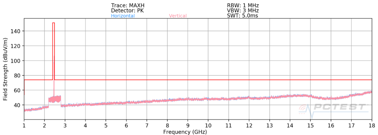
Plot 7-67. Radiated Spurious Plot above 1GHz MIMO (802.11ax OFDMA – 106 Tones – Ch. 11)
