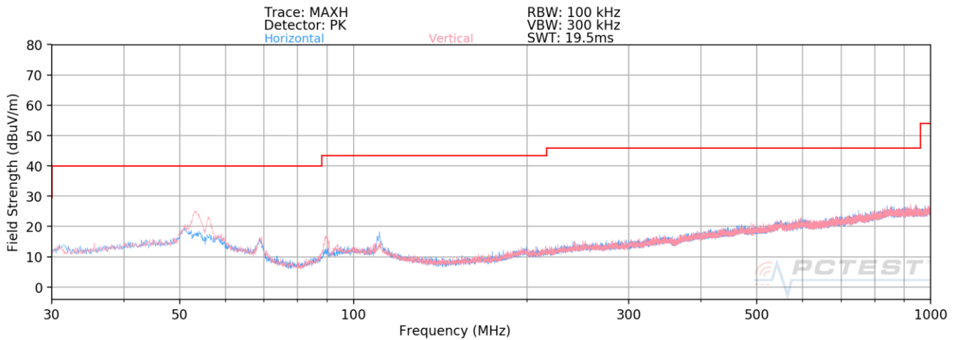
Plot 7-90. Radiated Spurious Plot below 1GHz (242 Tones)
