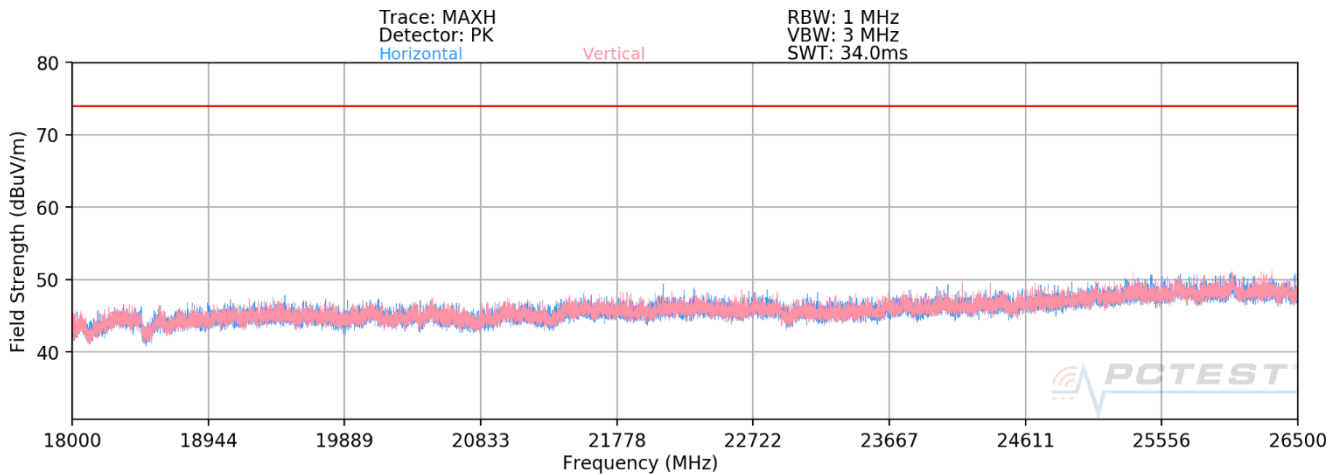
Plot 7-72. Radiated Spurious Plot above 18GHz MIMO (802.11ax OFDMA – 242 Tones)
