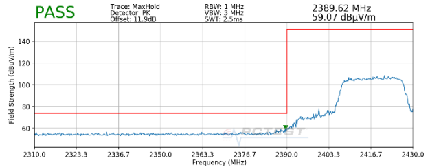
Plot 7-82. Radiated Restricted Lower Band Edge Measurement MIMO (Peak – 242 Tones)
