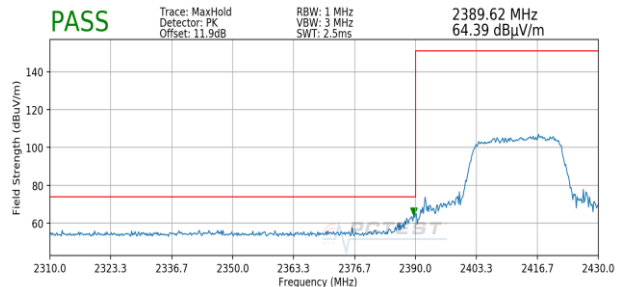
Plot 7-80. Radiated Restricted Lower Band Edge Measurement MIMO (Peak – 242 Tones)
