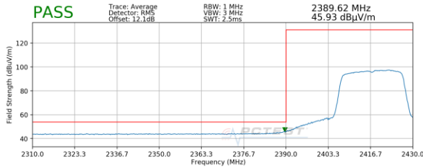
Plot 7-81. Radiated Restricted Lower Band Edge Measurement MIMO (Average – 242 Tones)
