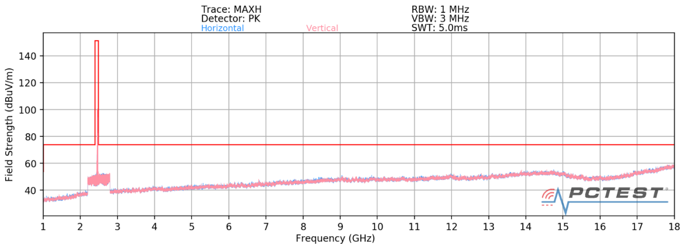
Plot 7-70. Radiated Spurious Plot above 1GHz MIMO (802.11ax OFDMA – 242 Tones – Ch. 11)
