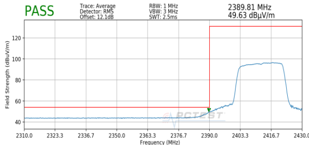
Plot 7-79. Radiated Restricted Lower Band Edge Measurement MIMO (Average – 242 Tones)
