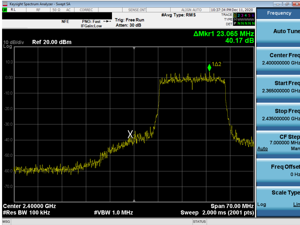
Plot 7-37. Band Edge Plot MIMO ANT2 (802.11ax OFDMA – 242 Tones – Ch. 2)
