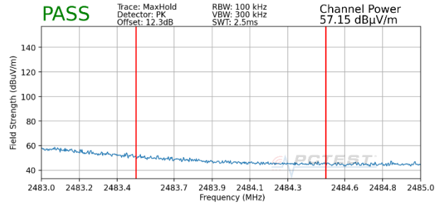
Plot 7-78. Radiated Restricted Upper Band Edge Measurement MIMO (Peak – 106 Tones)
