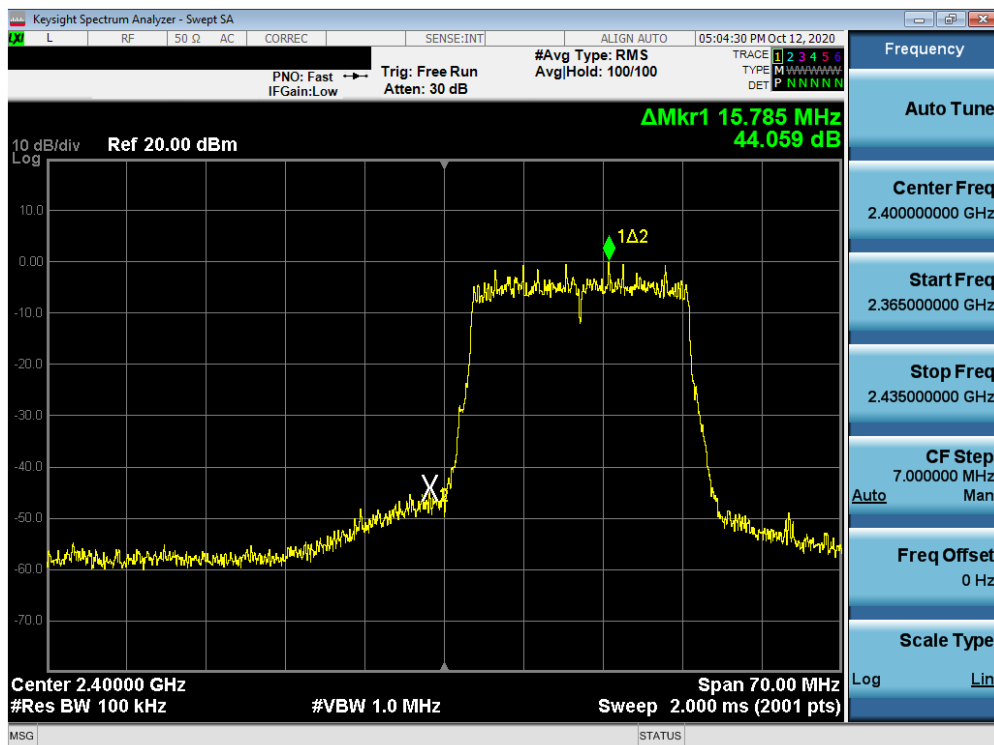
Plot 7-36. Band Edge Plot MIMO ANT2 (802.11ax OFDMA – 242 Tones – Ch. 1)
