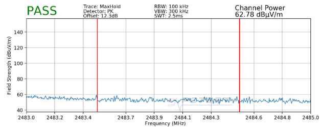
Plot 7-88. Radiated Restricted Upper Band Edge Measurement MIMO (Peak – 242 Tones)
