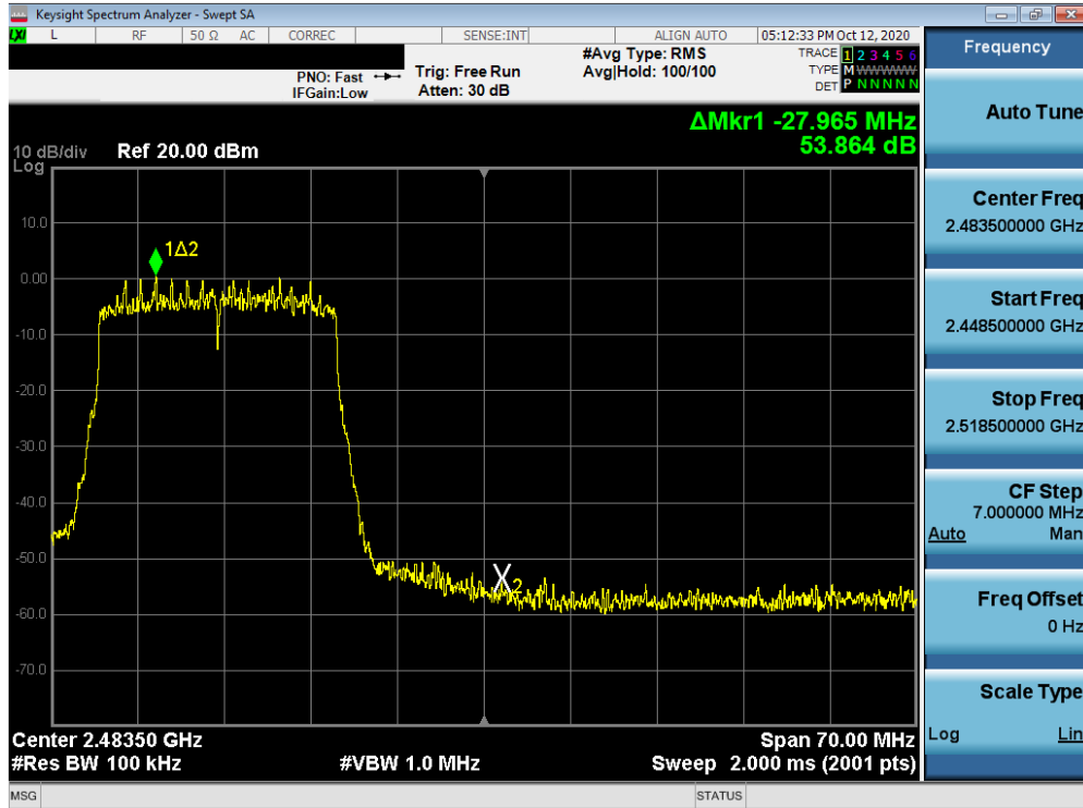
Plot 7-39. Band Edge Plot MIMO ANT2 (802.11ax OFDMA – 242 Tones – Ch. 11)
