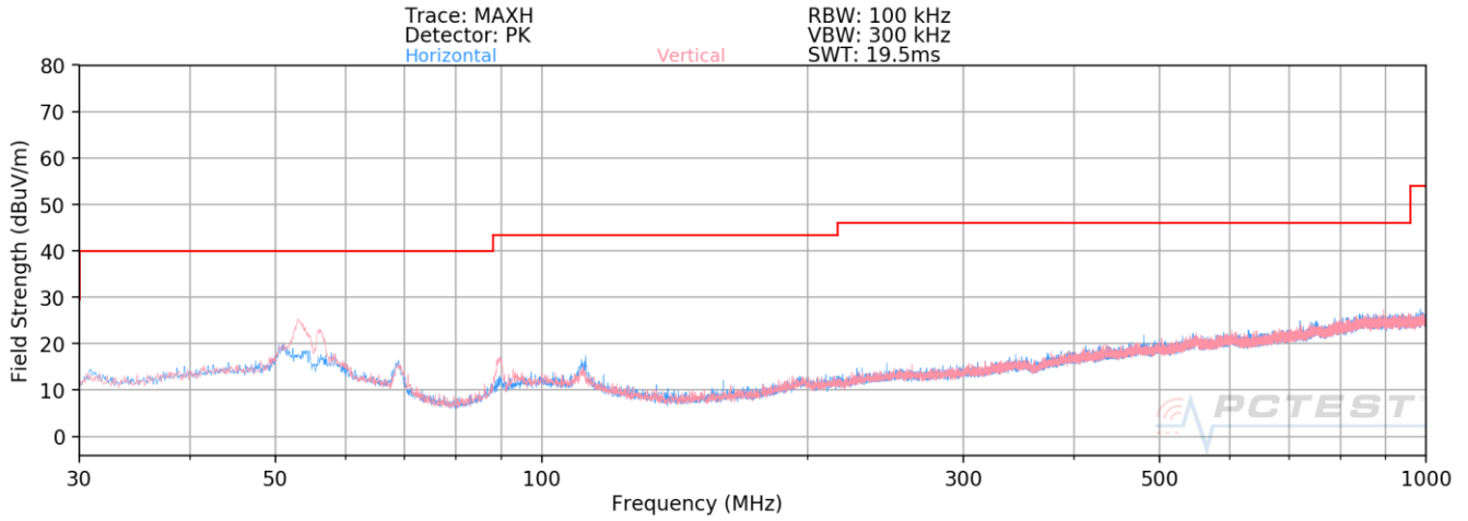
Plot 7-89. Radiated Spurious Plot below 1GHz (106 Tones)
