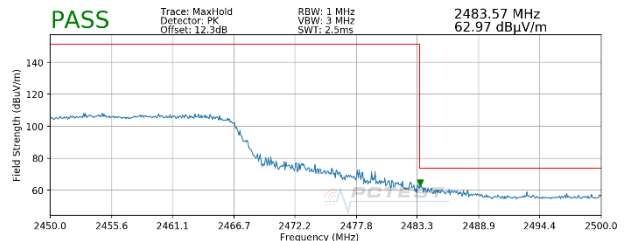
Plot 7-84. Radiated Restricted Upper Band Edge Measurement MIMO (Peak – 242 Tones)
