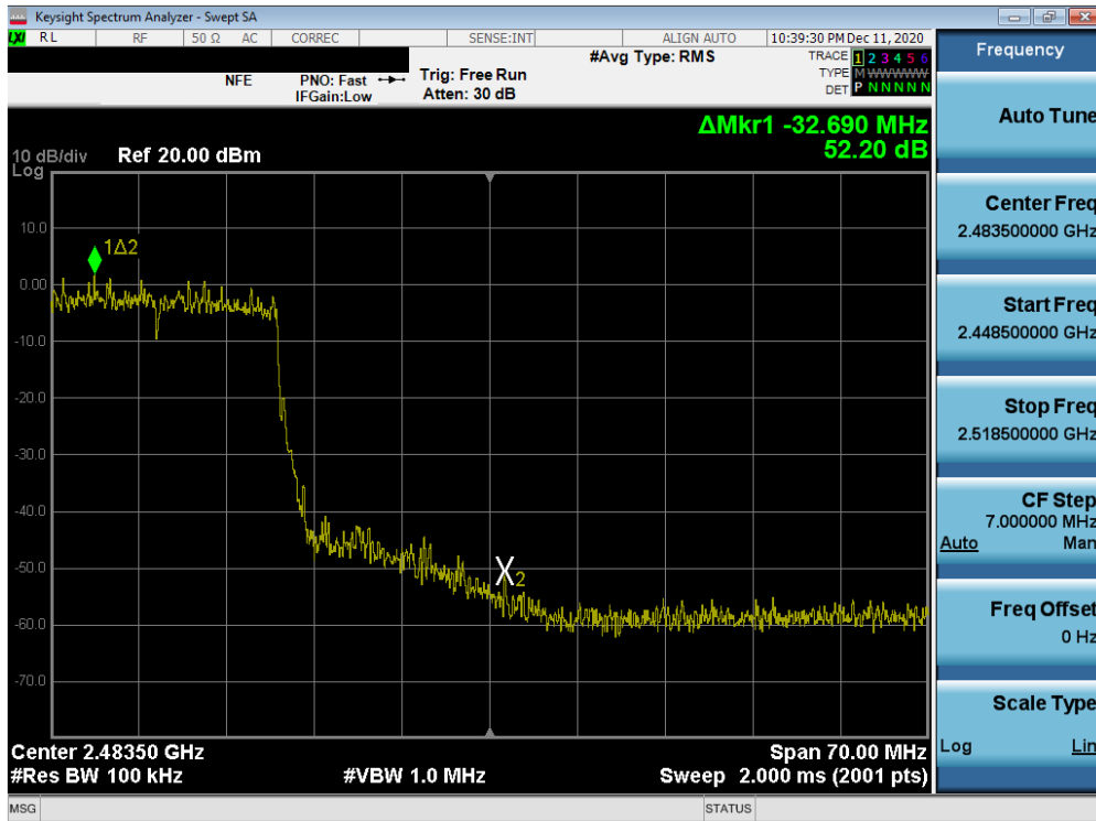
Plot 7-30. Band Edge Plot MIMO ANT1 (802.11ax OFDMA – 242 Tones – Ch. 10)
