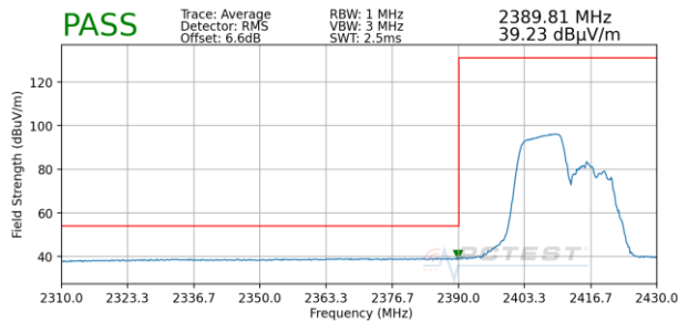
Plot 7-73. Radiated Restricted Lower Band Edge Measurement MIMO (Average – 106 Tones)
