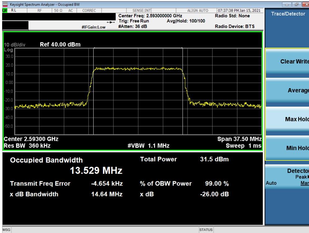
Plot 7-6. Occupied Bandwidth Plot (LTE Band 41(PCI3) - 15MHz 64-QAM - Full RB)
