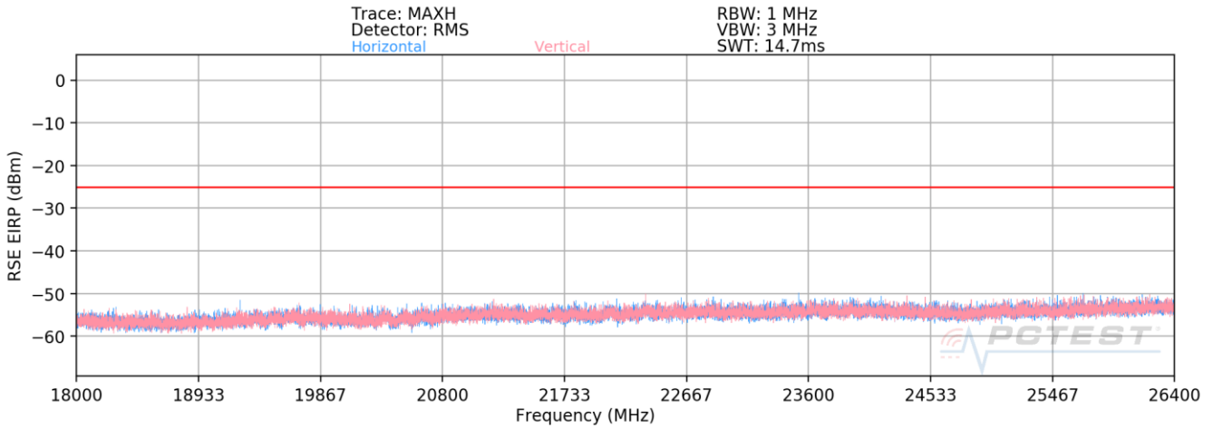
Plot 7-31. Radiated Spurious Plot >18GHz (LTE Band 41(PC3))
