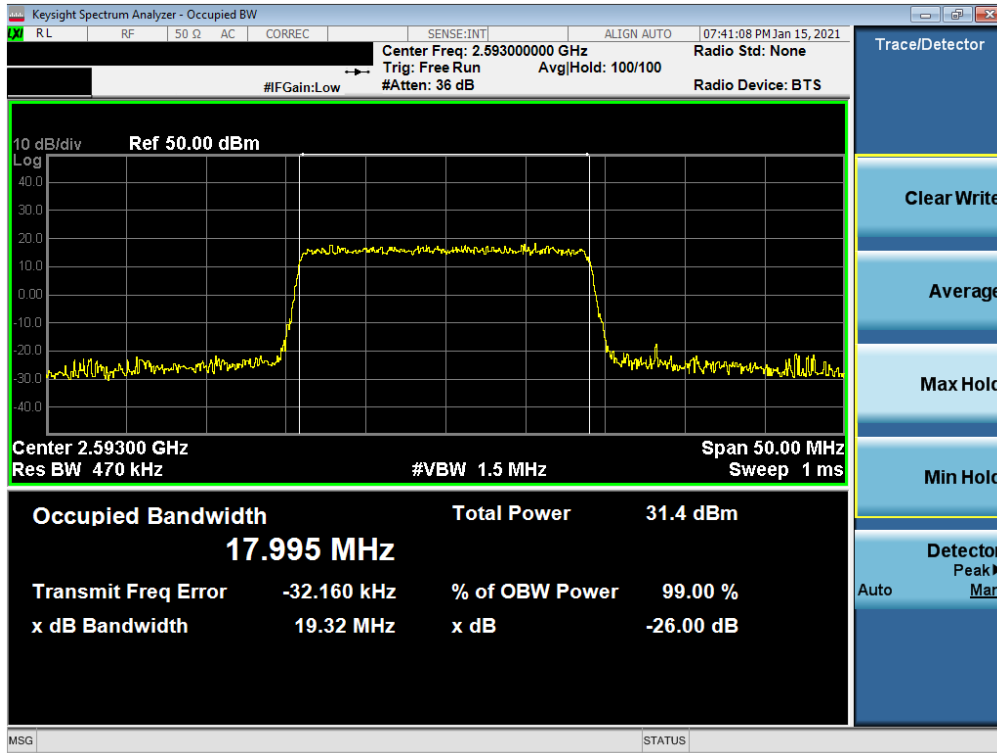
Plot 7-3. Occupied Bandwidth Plot (LTE Band 41(PC3) - 20MHz 64-QAM - Full RB)
