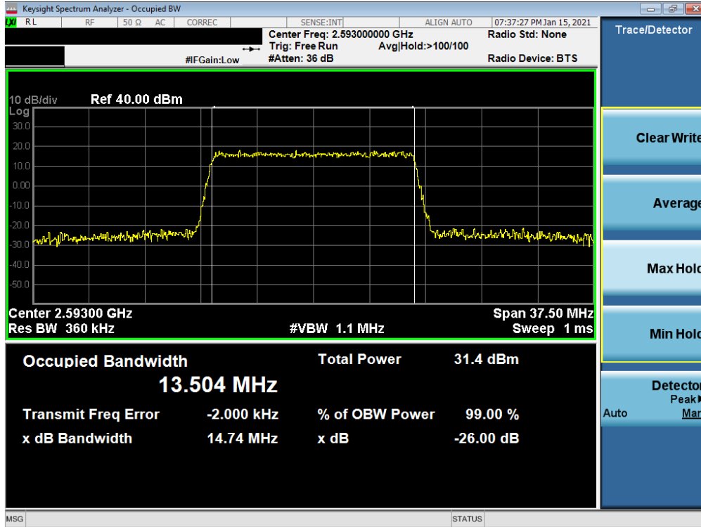
Plot 7-5. Occupied Bandwidth Plot (LTE Band 41(PCI3) - 15MHz 16-QAM - Full RB)
