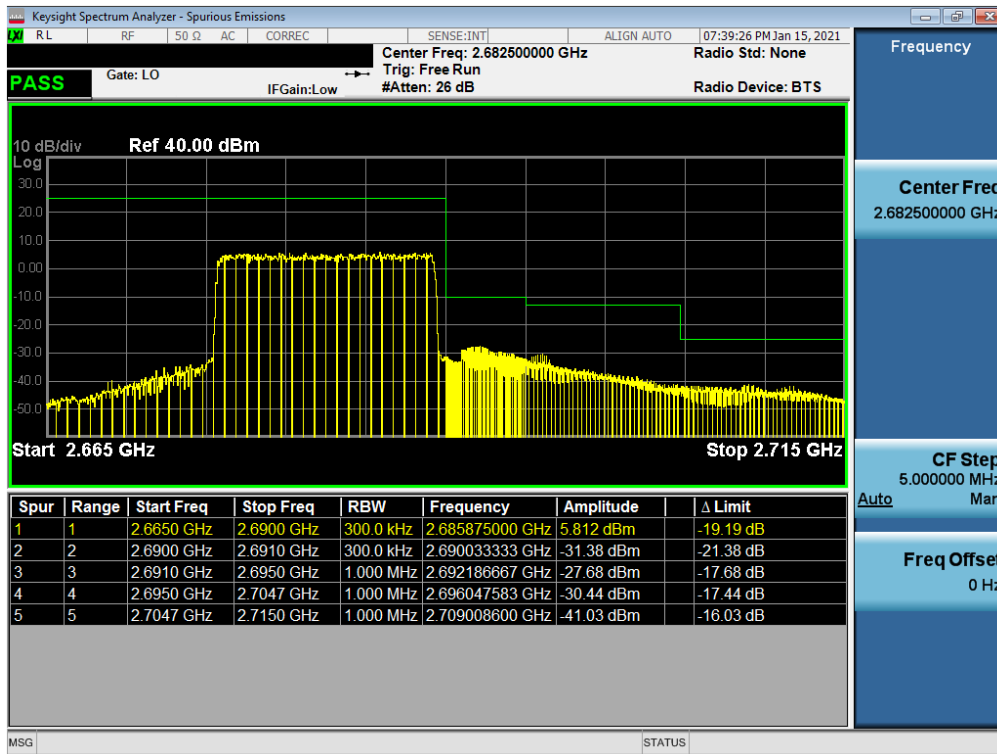
Plot 7-25. Upper ACP Plot (LTE Band 41(PC3) - 15MHz QPSK – Full RB)
