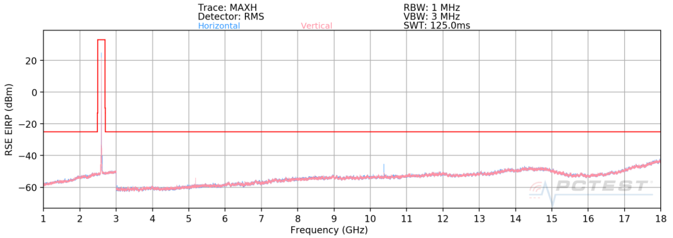
Plot 7-30. Radiated Spurious Plot <18GHz (LTE Band 41(PC3))
