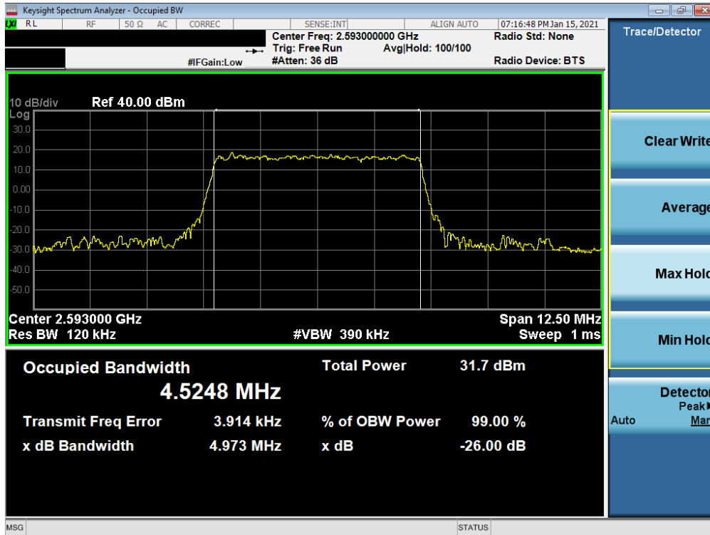
Plot 7-10. Occupied Bandwidth Plot (LTE Band 41(PC3) - 5MHz QPSK - Full RB)
