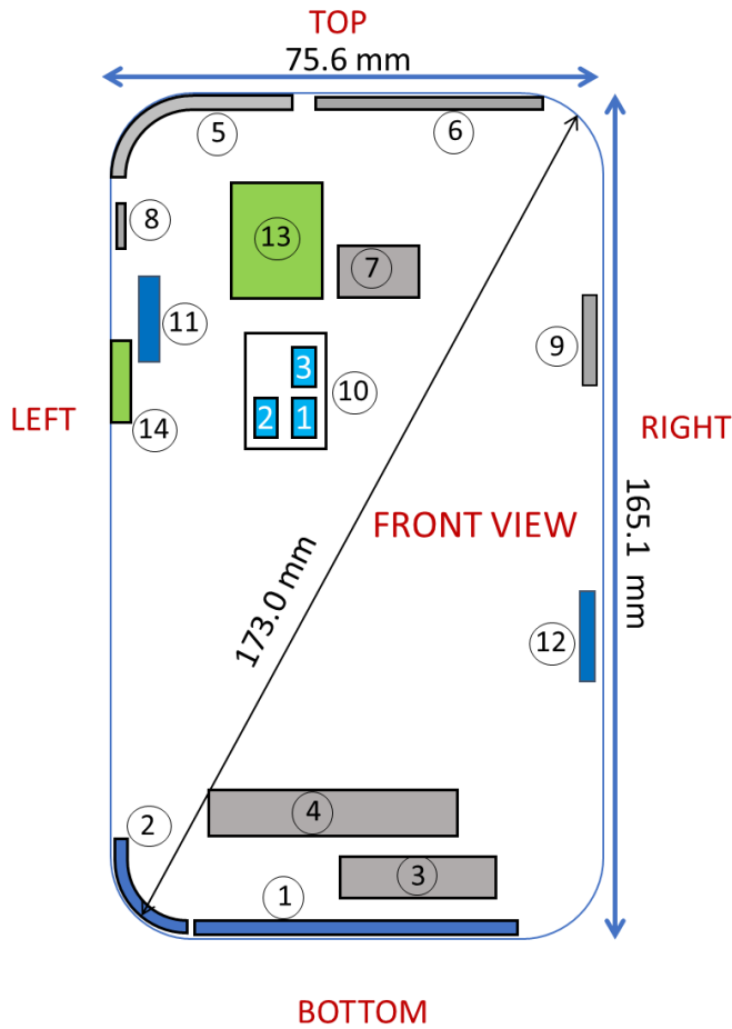
Figure E-1 DUT Antenna Locations
