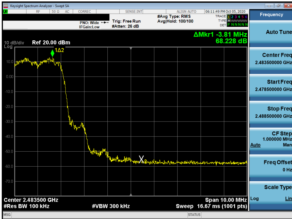
Plot 7-98. Band Edge Plot (Bluetooth with Hopping Enabled, ANT2 - 3 Mbps)
