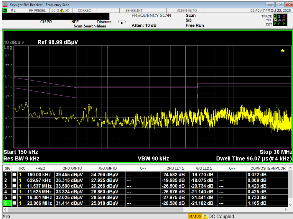
Plot 7-127. Line Conducted Plot with 802.11b with WCP (N)
