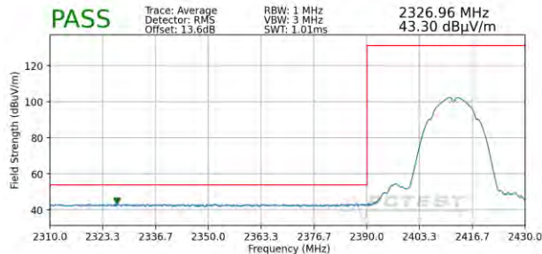
Plot 7-93. Radiated Restricted Lower Band Edge Measurement SISO ANT1 (Average)
