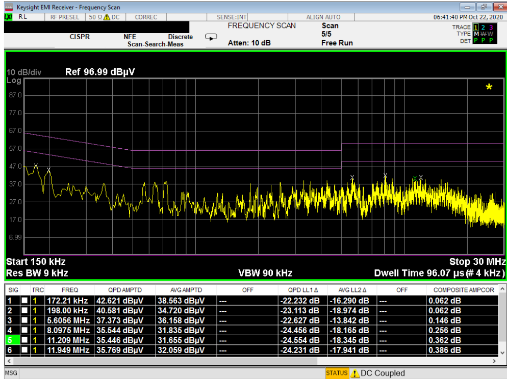
Plot 7-126. Line Conducted Plot with 802.11b with WCP (L1)
