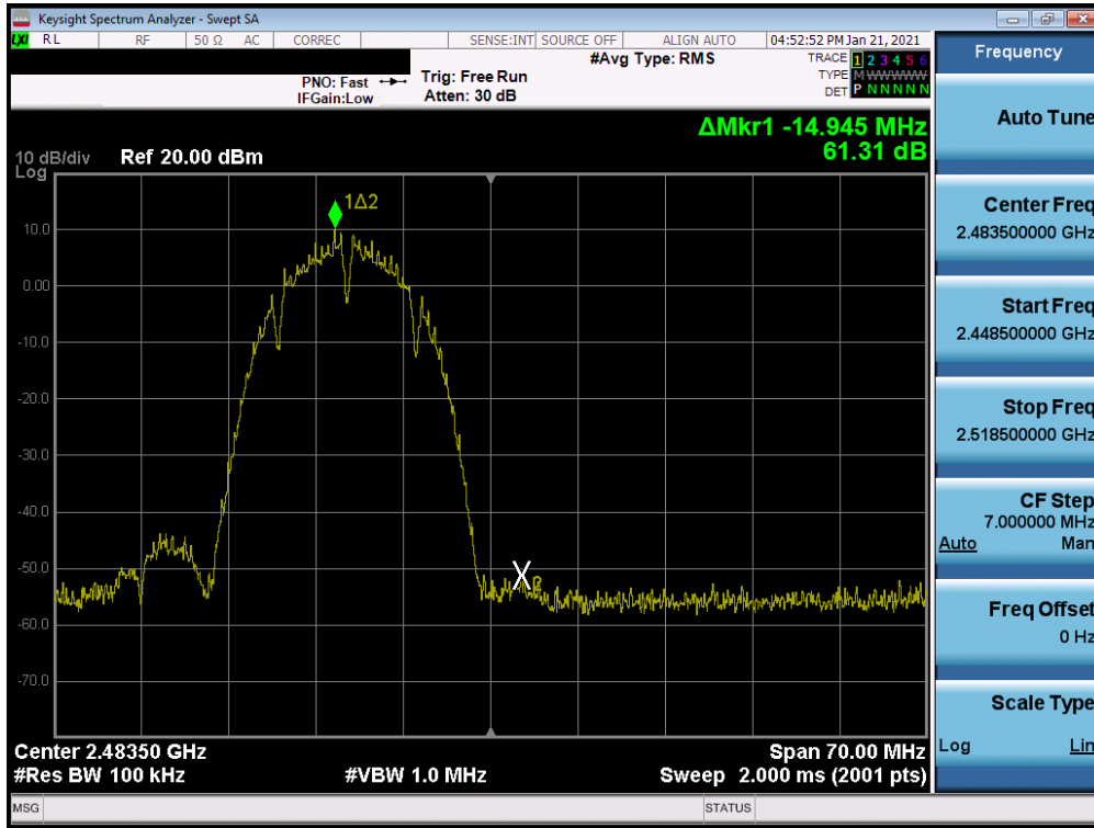
Plot 7-45. Band Edge Plot SISO ANT1 (802.11b – Ch. 13)
