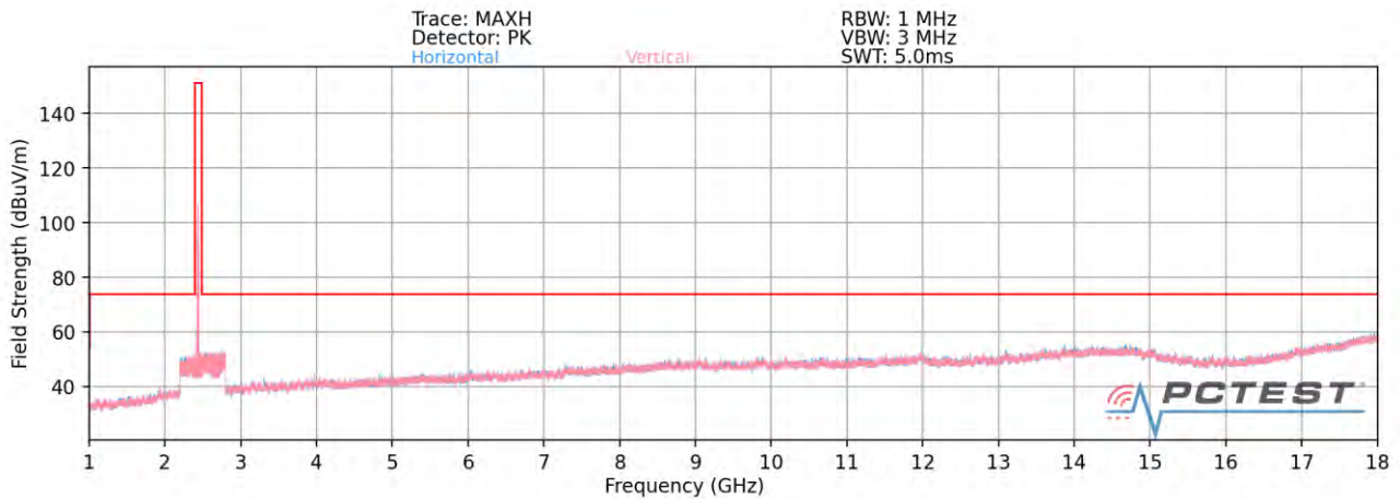
Plot 7-86. Radiated Spurious Plot above 1GHz SISO ANT2 (802.11b – Ch. 6)
