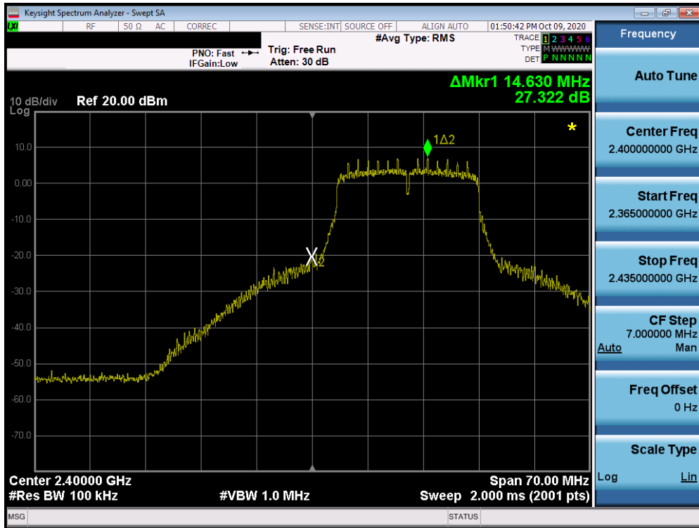
Plot 7-49. Band Edge Plot MIMO ANT1 (802.11n – Ch. 1)
