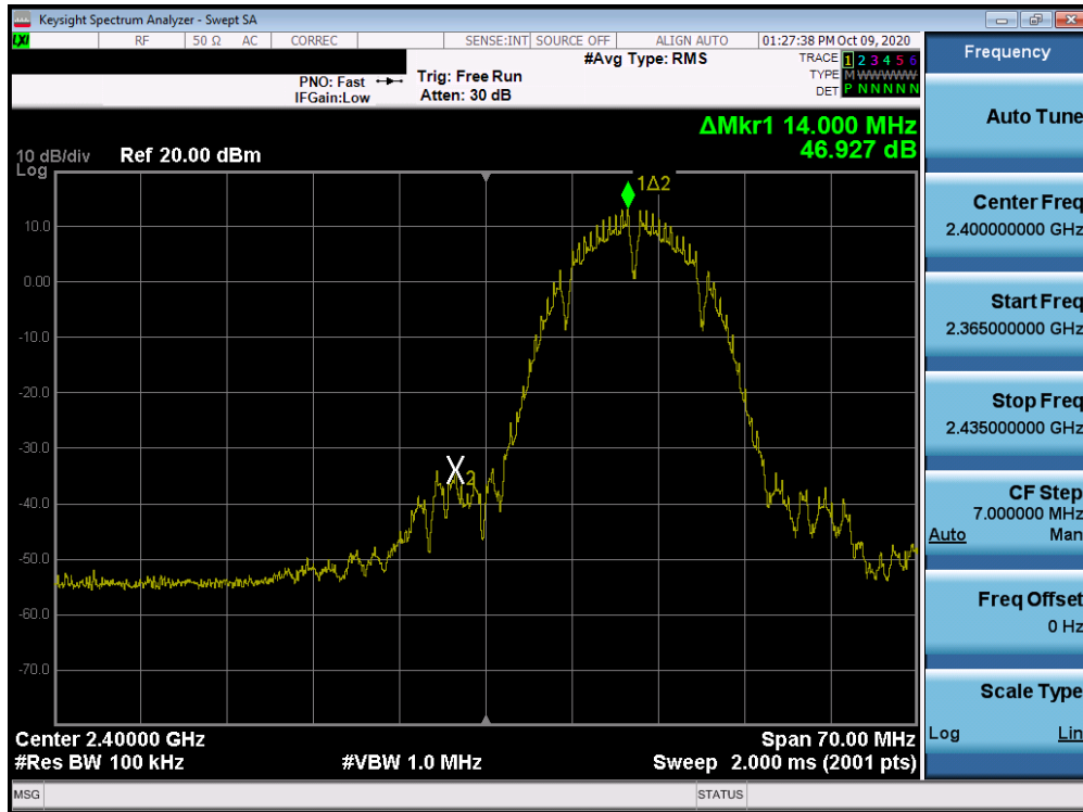
Plot 7-46. Band Edge Plot SISO ANT2 (802.11b – Ch. 1)
