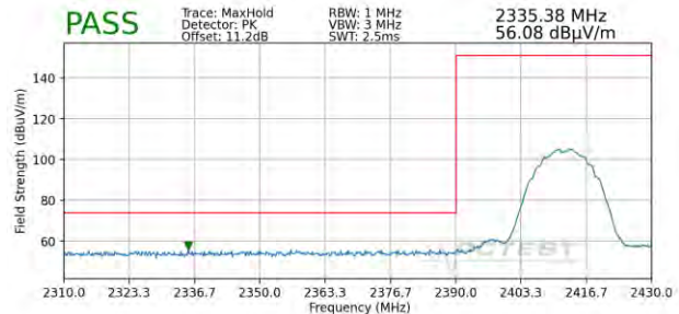
Plot 7-94. Radiated Restricted Lower Band Edge Measurement SISO ANT1 (Peak)
