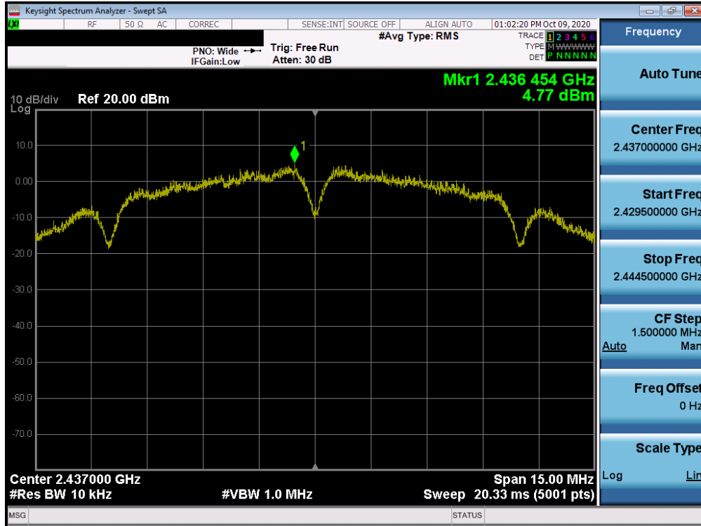
Plot 7-23. Power Spectral Density Plot SISO ANT2 (802.11b – Ch. 6)
