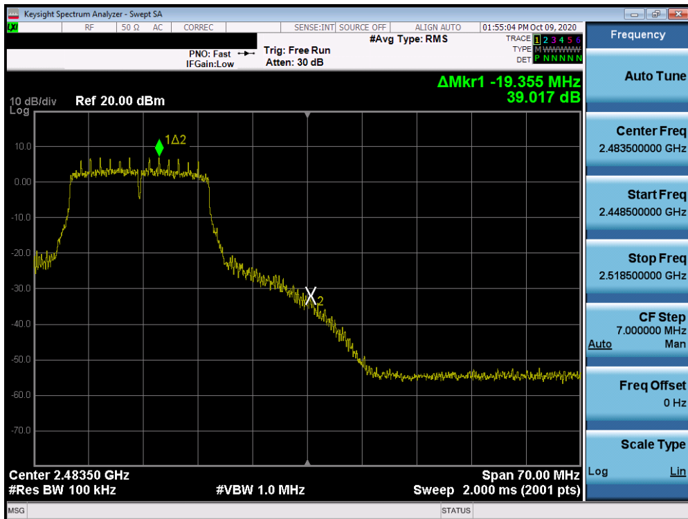
Plot 7-50. Band Edge Plot MIMO ANT1 (802.11n – Ch. 11)
