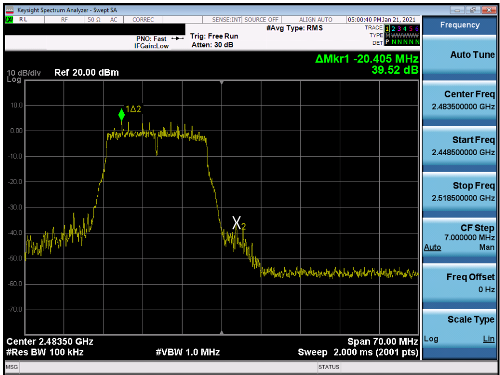
Plot 7-52. Band Edge Plot MIMO ANT1 (802.11n – Ch. 13)
