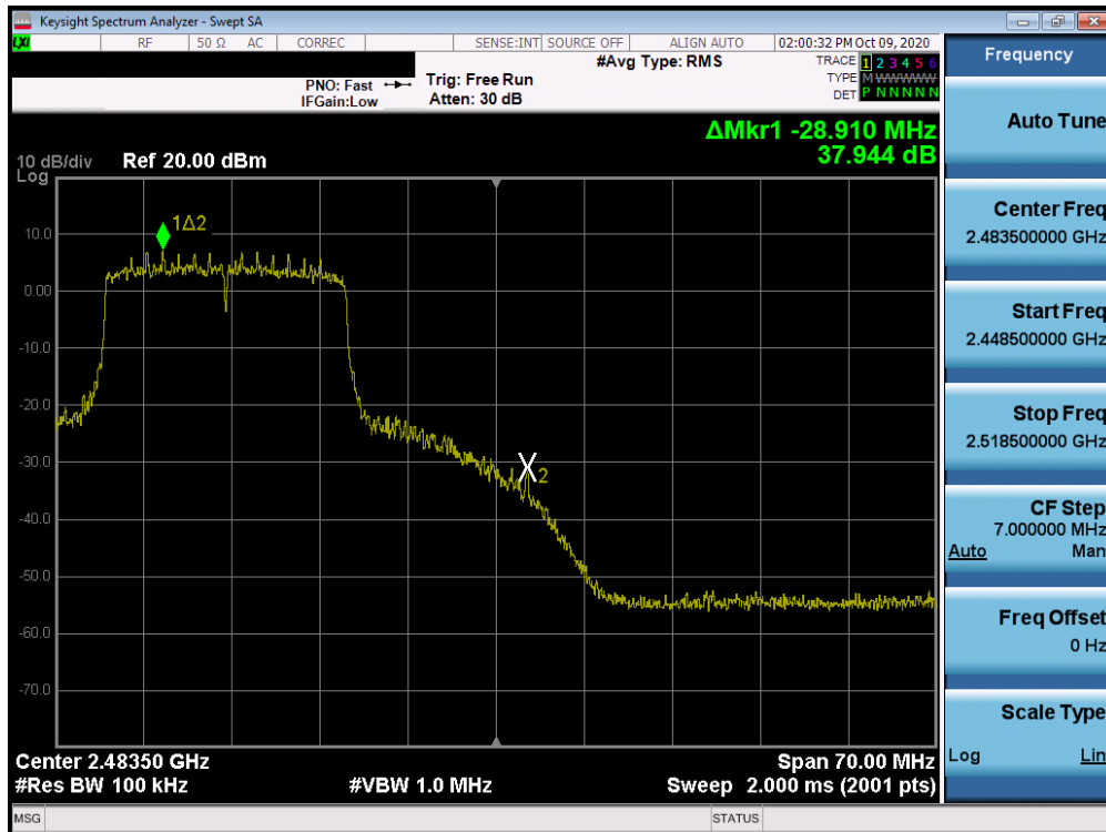
Plot 7-56. Band Edge Plot MIMO ANT1 (802.11ax – Ch. 11)
