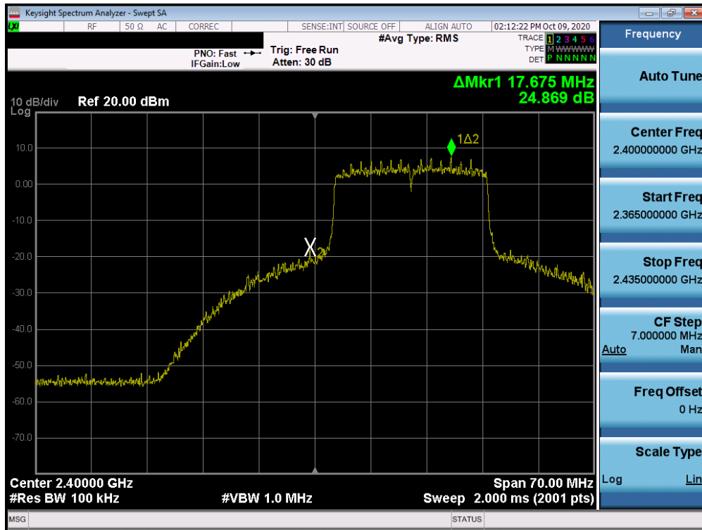
Plot 7-63. Band Edge Plot MIMO ANT2 (802.11ax – Ch. 1)
