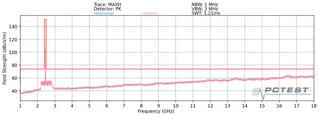
Plot 7-91. Radiated Spurious Plot above 1GHz MIMO/CDD (802.11g – Ch. 11)
