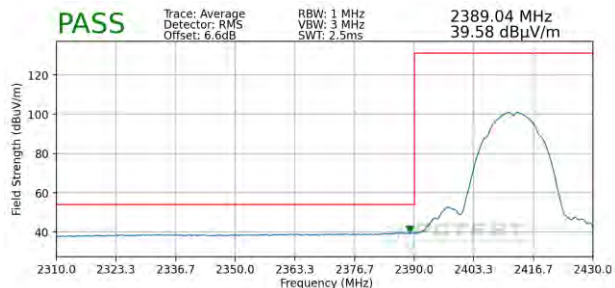
Plot 7-99. Radiated Restricted Band Edge Measurement SISO ANT1 with WCP (Average)
