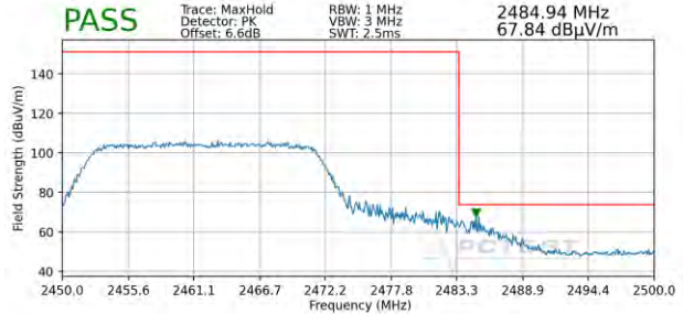
Plot 7-122. Radiated Restricted Band Edge Measurement MIMO with WCP (Peak)
