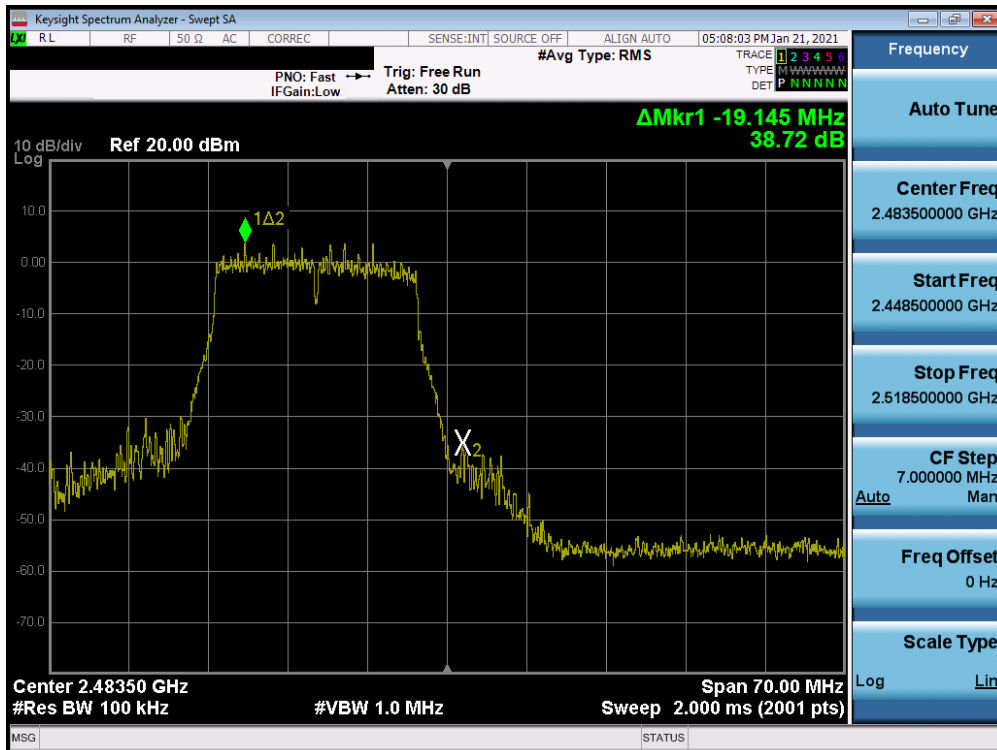
Plot 7-62. Band Edge Plot MIMO ANT2 (802.11n – Ch. 13)
