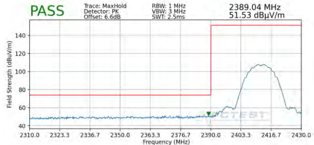
Plot 7-102. Radiated Restricted Lower Band Edge Measurement SISO ANT2 (Peak)
