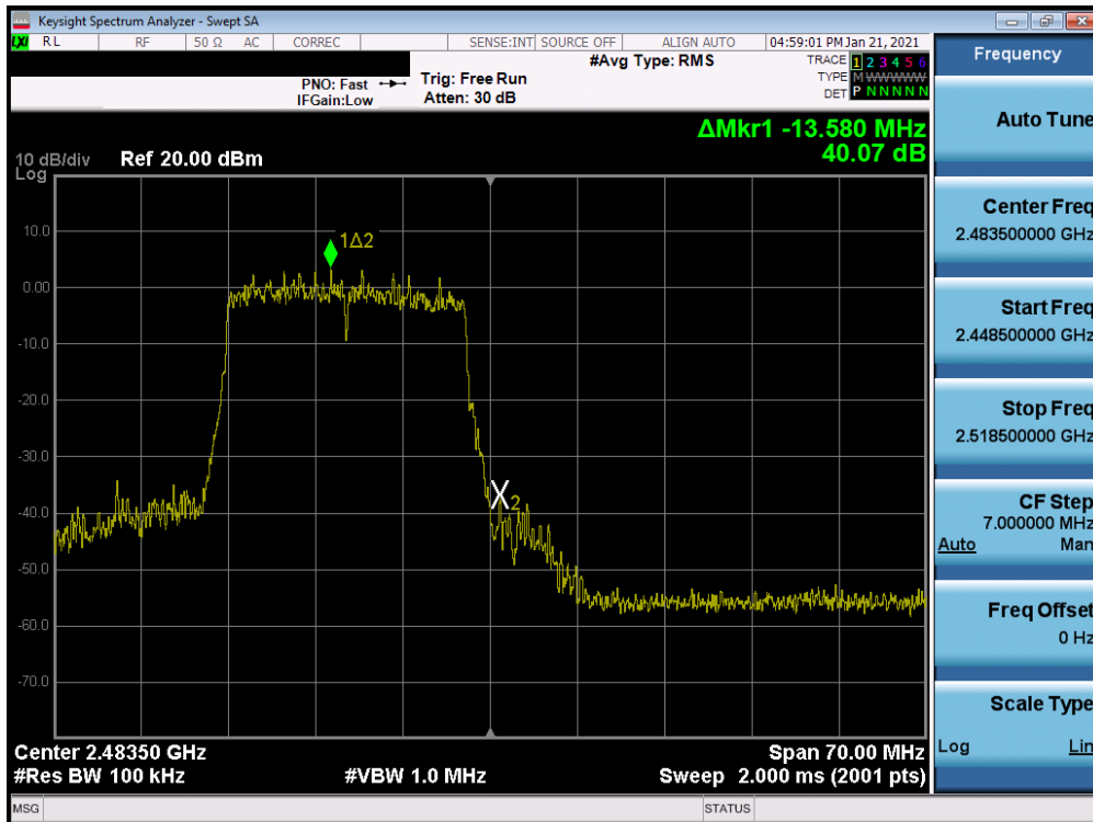
Plot 7-58. Band Edge Plot MIMO ANT1 (802.11ax – Ch. 13)
