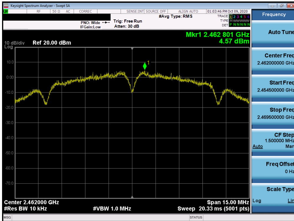
Plot 7-24. Power Spectral Density Plot SISO ANT2 (802.11b – Ch. 11)
