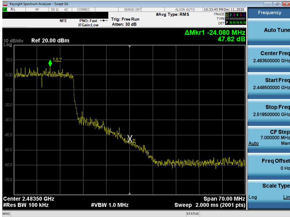
Plot 7-65. Band Edge Plot MIMO ANT2 (802.11ax – Ch. 10)
