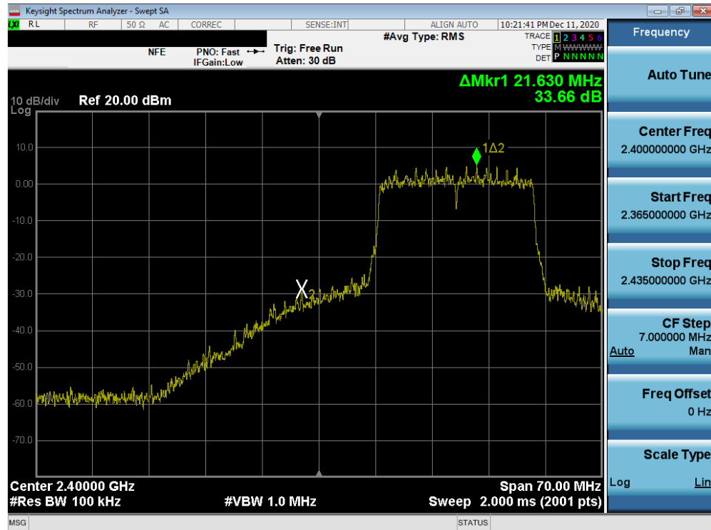
Plot 7-54. Band Edge Plot MIMO ANT1 (802.11ax – Ch. 2)
