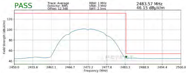
Plot 7-105. Radiated Restricted Band Edge Measurement SISO ANT2 (Average)
