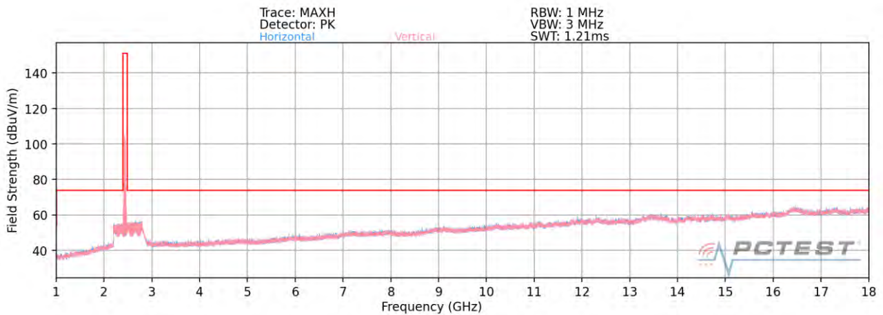
Plot 7-90. Radiated Spurious Plot above 1GHz MIMO/CDD (802.11g – Ch. 6)
