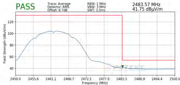
Plot 7-107. Radiated Restricted Band Edge Measurement SISO ANT2 with WCP (Average)
