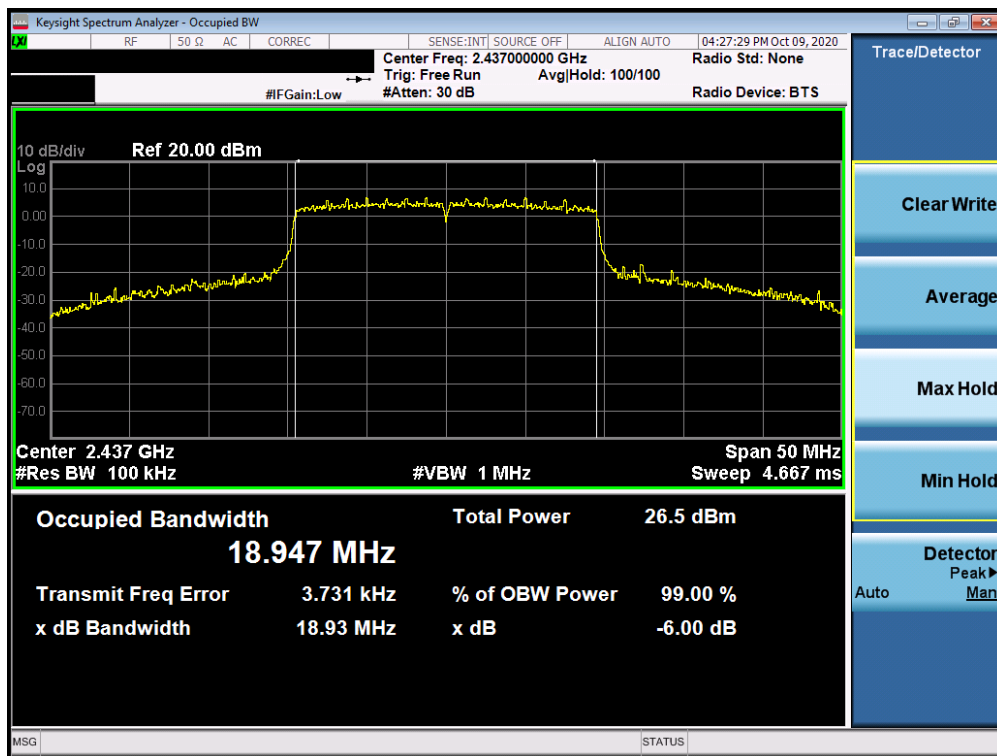
Plot 7-17. 6dB Bandwidth Plot MIMO ANT2 (802.11ax – Ch. 6)
