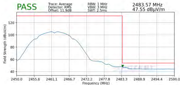
Plot 7-103. Radiated Restricted Upper Band Edge Measurement SISO ANT2 (Average)
