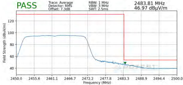
Plot 7-121. Radiated Restricted Band Edge Measurement MIMO with WCP (Average)
