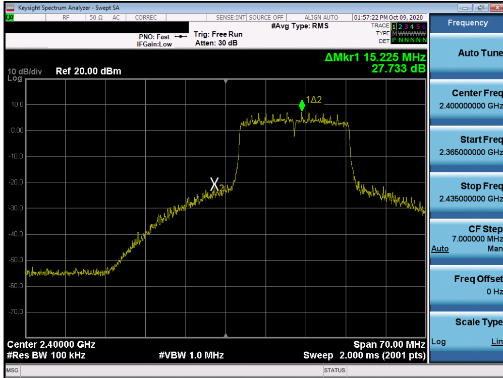
Plot 7-53. Band Edge Plot MIMO ANT1 (802.11ax – Ch. 1)
