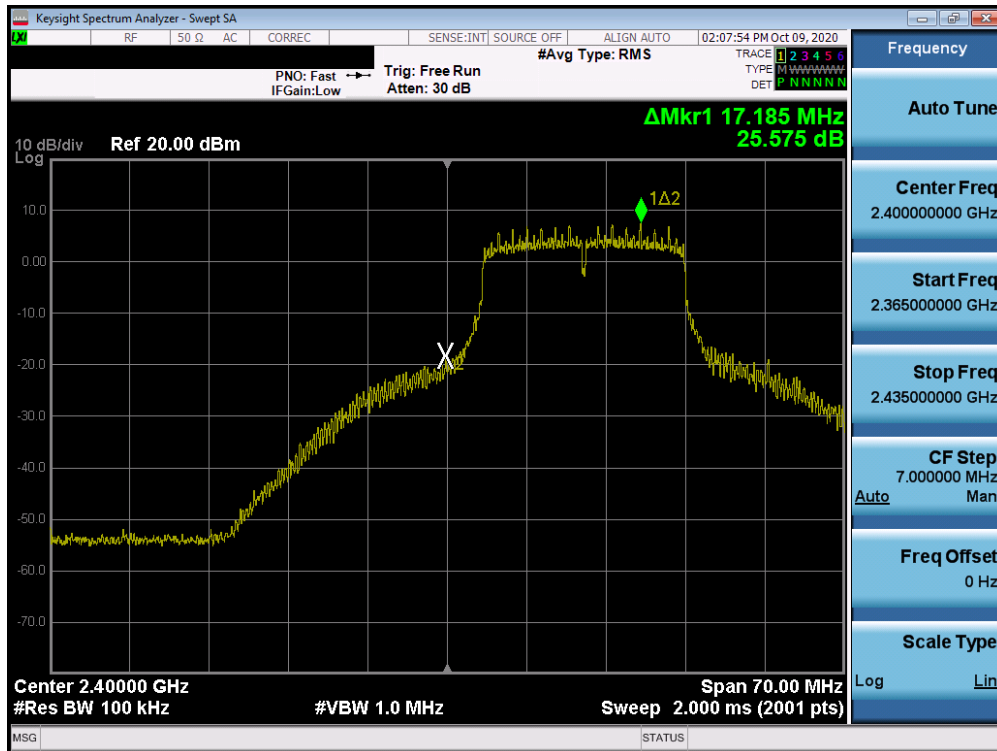
Plot 7-59. Band Edge Plot MIMO ANT2 (802.11n – Ch. 1)
