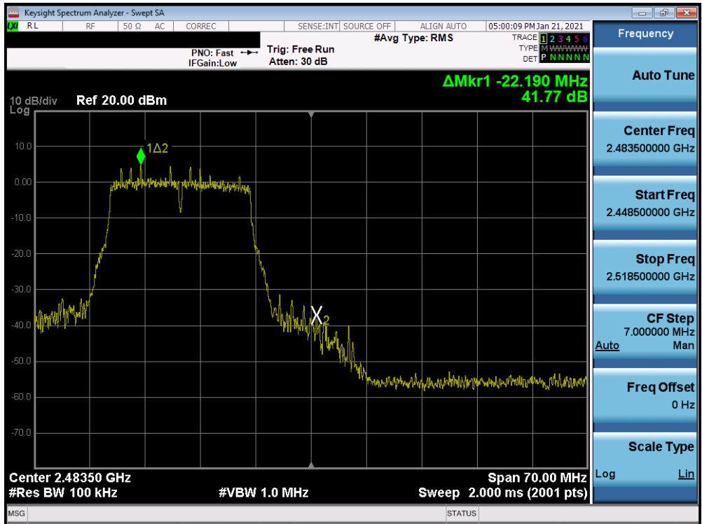
Plot 7-51. Band Edge Plot MIMO ANT1 (802.11n – Ch. 12)
