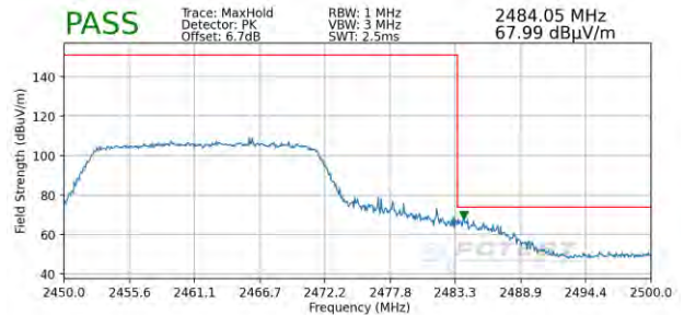
Plot 7-116. Radiated Restricted Upper Band Edge Measurement MIMO (Peak)
