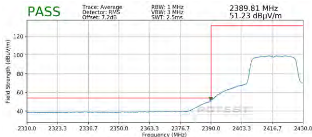
Plot 7-111. Radiated Restricted Lower Band Edge Measurement MIMO (Average)
