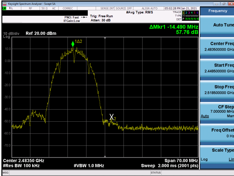
Plot 7-48. Band Edge Plot SISO ANT2 (802.11b – Ch. 13)
