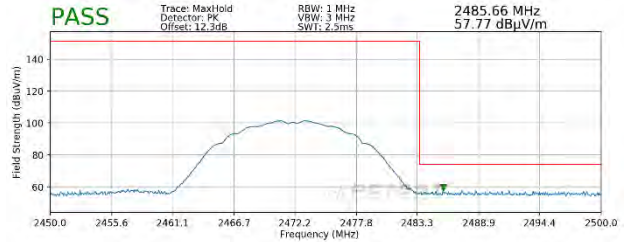
Plot 7-98. Radiated Restricted Band Edge Measurement SISO ANT1 (Peak)
