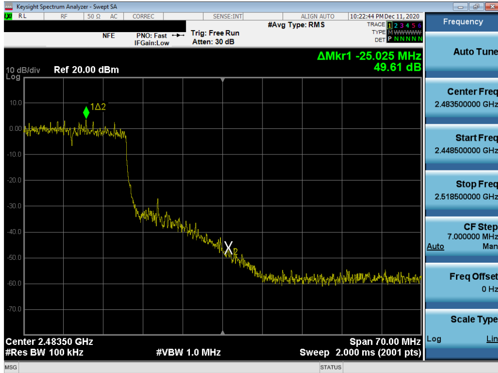
Plot 7-55. Band Edge Plot MIMO ANT1 (802.11ax – Ch. 10)
