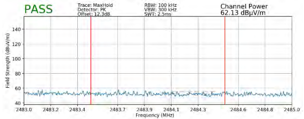
Plot 7-118. Radiated Restricted Band Edge Measurement MIMO (Peak)
