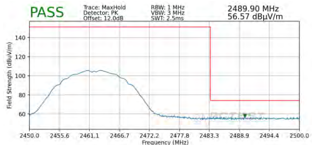
Plot 7-96. Radiated Restricted Upper Band Edge Measurement SISO ANT1 (Peak)
