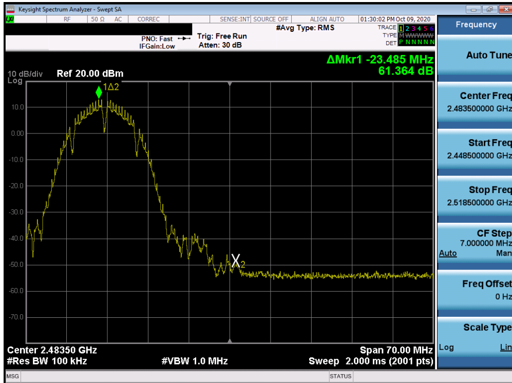
Plot 7-47. Band Edge Plot SISO ANT2 (802.11b – Ch. 11)
