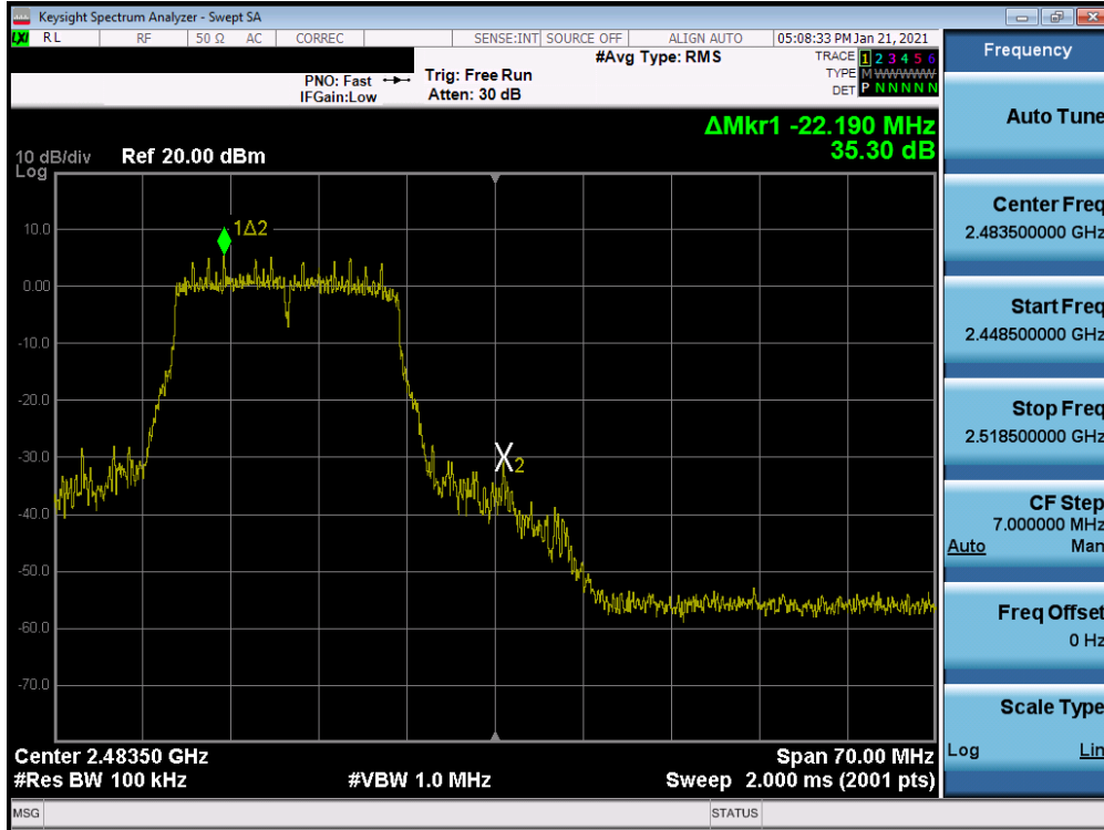
Plot 7-61. Band Edge Plot MIMO ANT2 (802.11n – Ch. 12)
