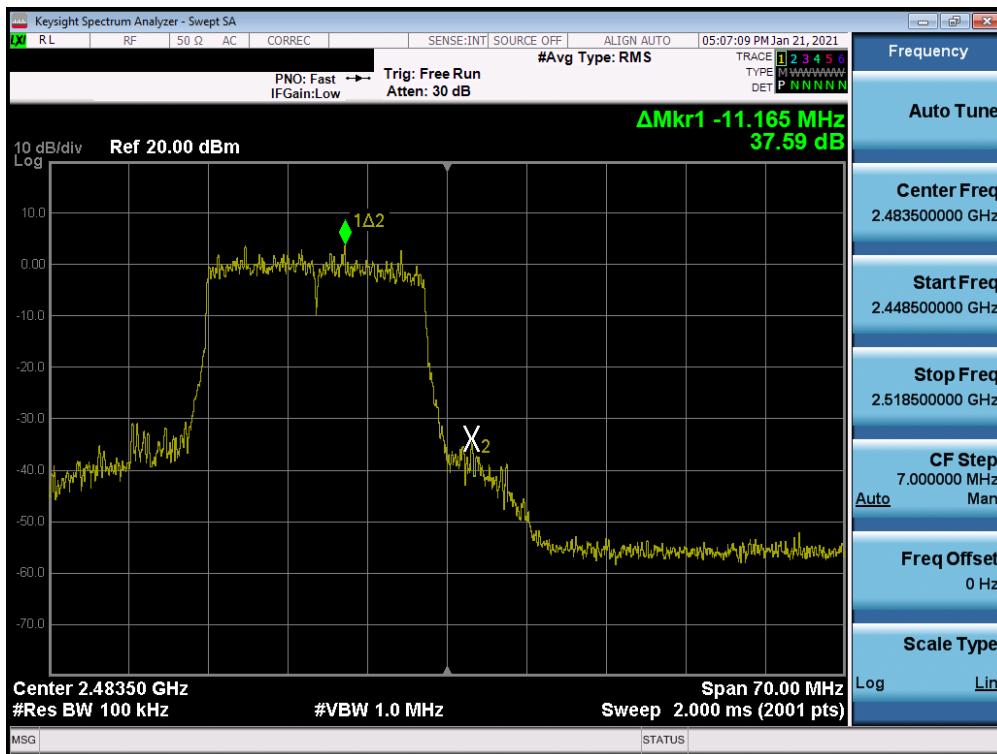
Plot 7-68. Band Edge Plot MIMO ANT2 (802.11ax – Ch. 13)
