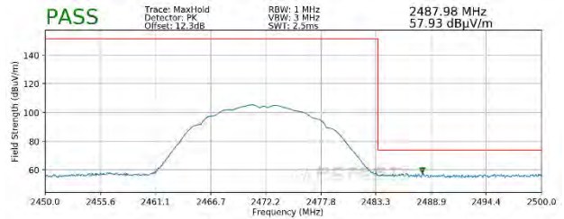
Plot 7-106. Radiated Restricted Band Edge Measurement SISO ANT2 (Peak)
