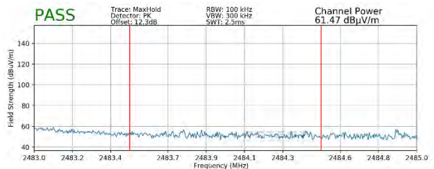
Plot 7-120. Radiated Restricted Band Edge Measurement MIMO (Peak)
