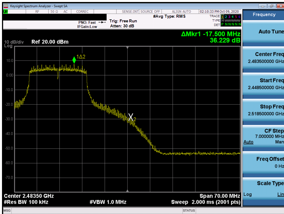
Plot 7-60. Band Edge Plot MIMO ANT2 (802.11n – Ch. 11)
