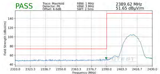
Plot 7-100. Radiated Restricted Band Edge Measurement SISO ANT1 with WCP (Peak)
