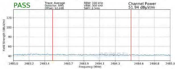
Plot 7-117. Radiated Restricted Band Edge Measurement MIMO (Average)
