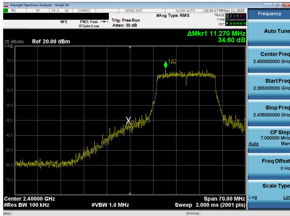
Plot 7-64. Band Edge Plot MIMO ANT2 (802.11ax – Ch. 2)
