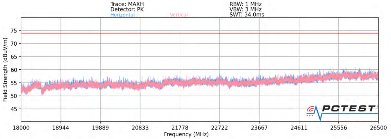
Plot 7-92. Radiated Spurious Plot above 18GHz MIMO/CDD
