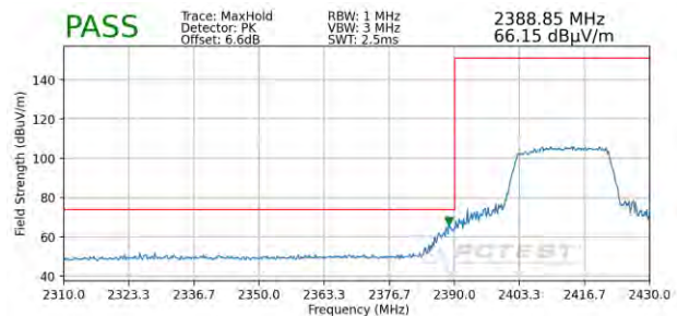
Plot 7-110. Radiated Restricted Lower Band Edge Measurement MIMO (Peak)
