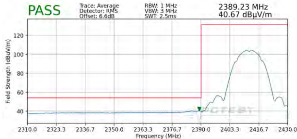
Plot 7-101. Radiated Restricted Lower Band Edge Measurement SISO ANT2 (Average)
