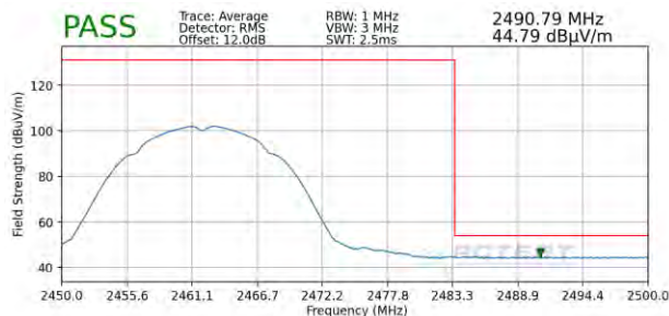
Plot 7-95. Radiated Restricted Upper Band Edge Measurement SISO ANT1 (Average)
