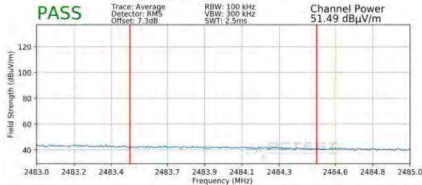
Plot 7-113. Radiated Restricted Upper Band Edge Measurement MIMO (Average)
