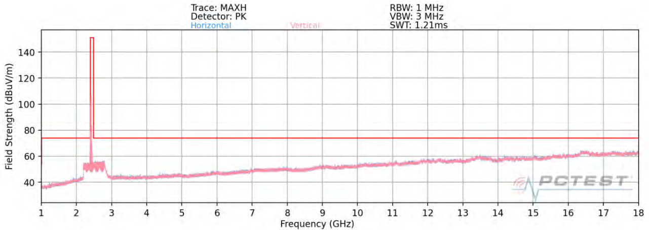
Plot 7-89. Radiated Spurious Plot above 1GHz MIMO/CDD (802.11g – Ch. 1)
