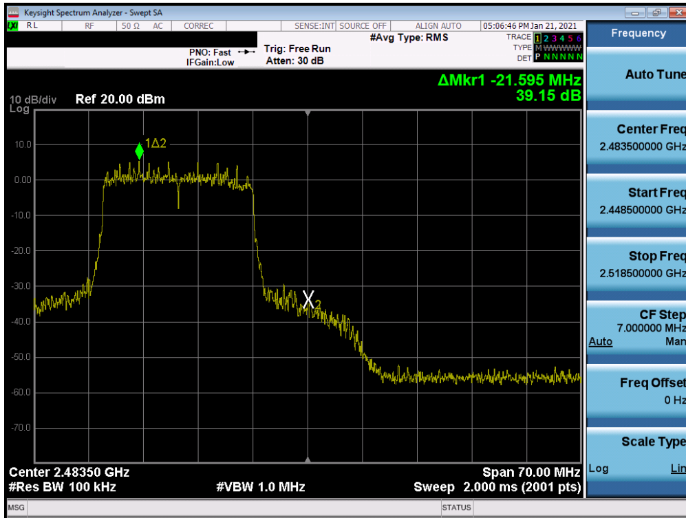
Plot 7-67. Band Edge Plot MIMO ANT2 (802.11ax – Ch. 12)
