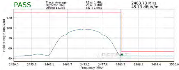
Plot 7-97. Radiated Restricted Band Edge Measurement SISO ANT1 (Average)
