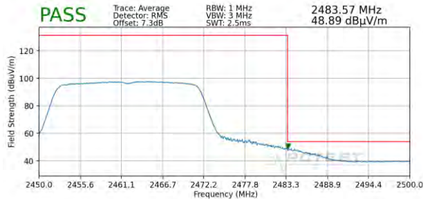
Plot 7-115. Radiated Restricted Upper Band Edge Measurement MIMO (Average)
