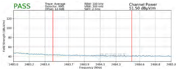
Plot 7-119. Radiated Restricted Band Edge Measurement MIMO (Average)
