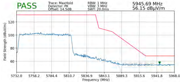
Plot 7-311. Radiated Upper Band Edge Plot MIMO (Peak – UNII Band 3)
