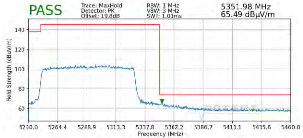
Plot 7-308. Radiated Upper Band Edge Plot MIMO (Peak – UNII Band 2A)
