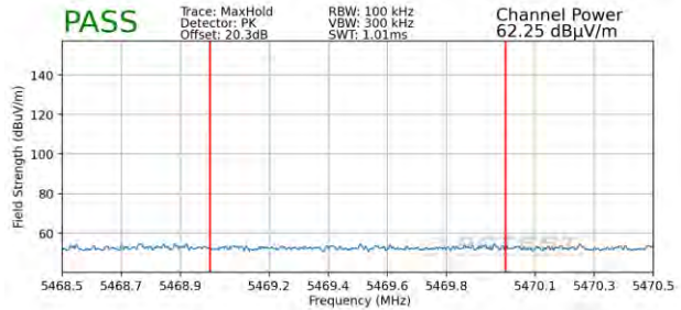
Plot 7-310. Radiated Lower Band Edge Plot MIMO (Peak – UNII Band 2C)
