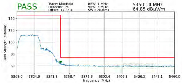
Plot 7-290. Radiated Upper Band Edge Plot MIMO (Peak – UNII Band 2A)
