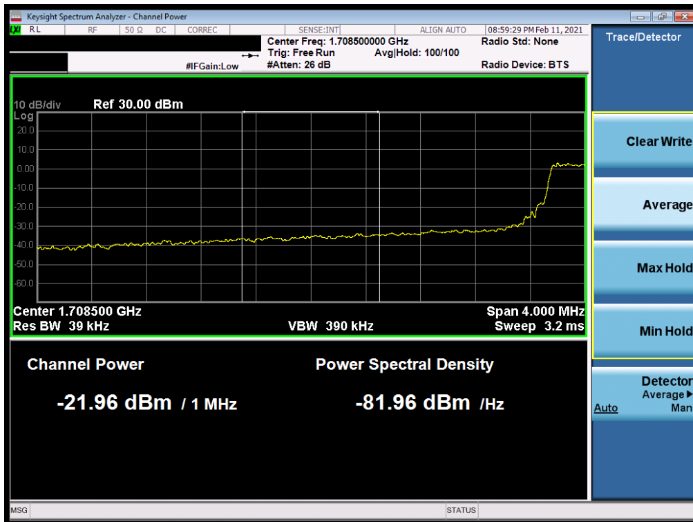
Plot 7-71. Lower Extended Band Edge Plot (LTE Band 4 - 5MHz QPSK – Full RB)
