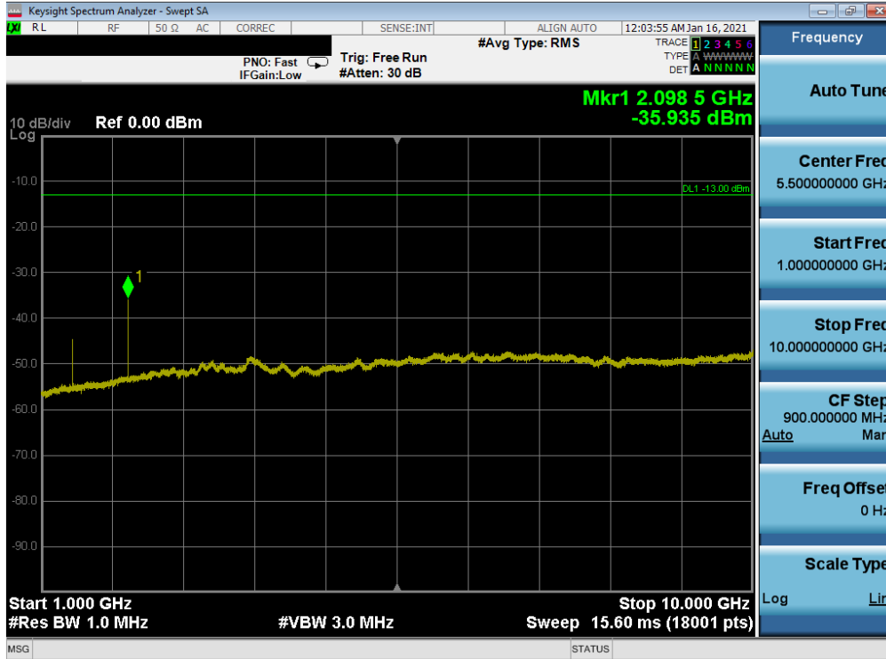
Plot 7-48. Conducted Spurious Plot (LTE Band 12 - 10MHz QPSK - RB Size 1, RB Offset 0 - Low Channel)
