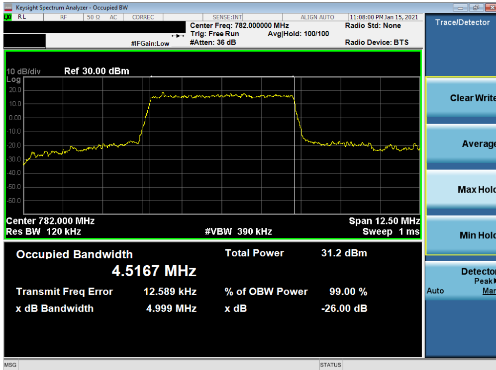
Plot 7-34. Occupied Bandwidth Plot (LTE Band 13 - 5MHz QPSK - Full RB)
