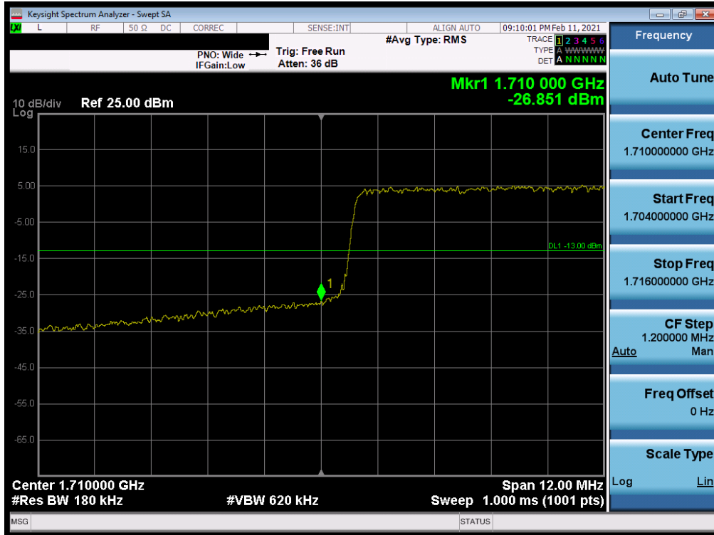
Plot 7-62. Lower Band Edge Plot (LTE Band 4 - 15MHz QPSK – Full RB)
