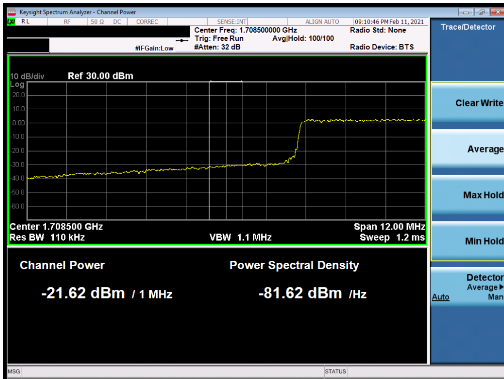
Plot 7-63. Lower Extended Band Edge Plot (LTE Band 4 - 15MHz QPSK – Full RB)
