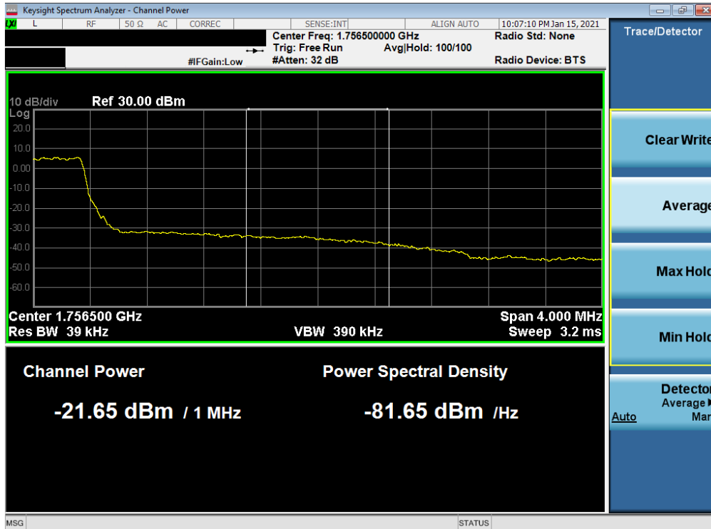
Plot 7-77. Upper Extended Band Edge Plot (LTE Band 4 - 3MHz QPSK – Full RB)
