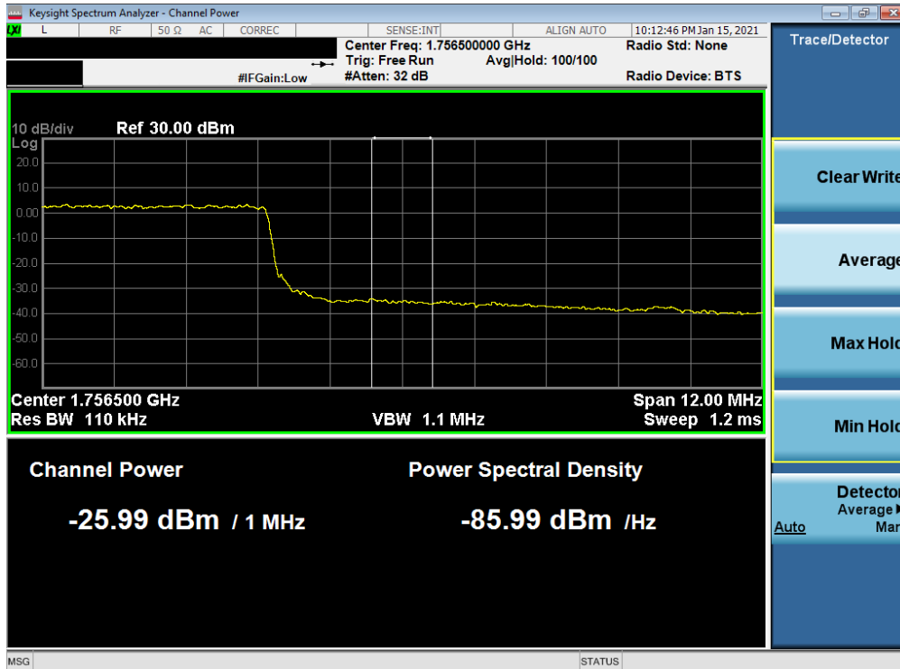
Plot 7-65. Upper Extended Band Edge Plot (LTE Band 4 - 15MHz QPSK – Full RB)
