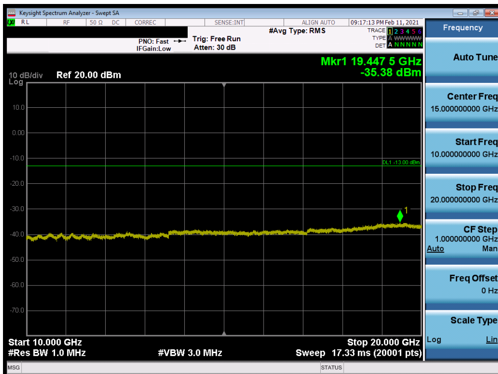
Plot 7-42. Conducted Spurious Plot (LTE Band 4 - 20MHz QPSK - RB Size 1, RB Offset 0 - Mid Channel)
