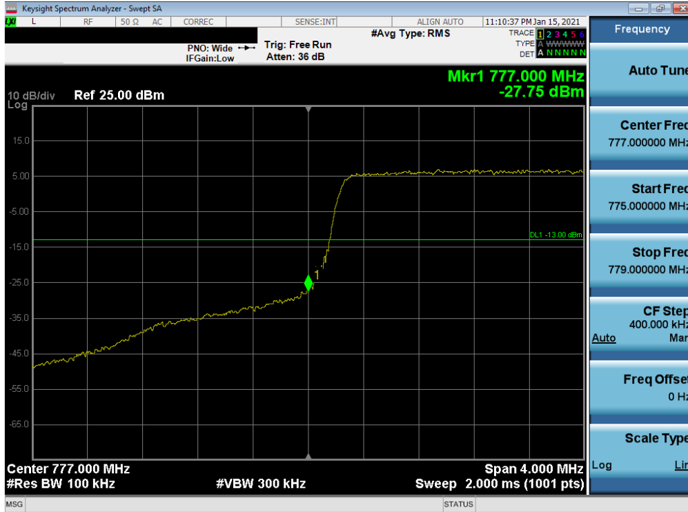
Plot 7-94. Lower Band Edge Plot (LTE Band 13 - 5MHz QPSK – Full RB)
