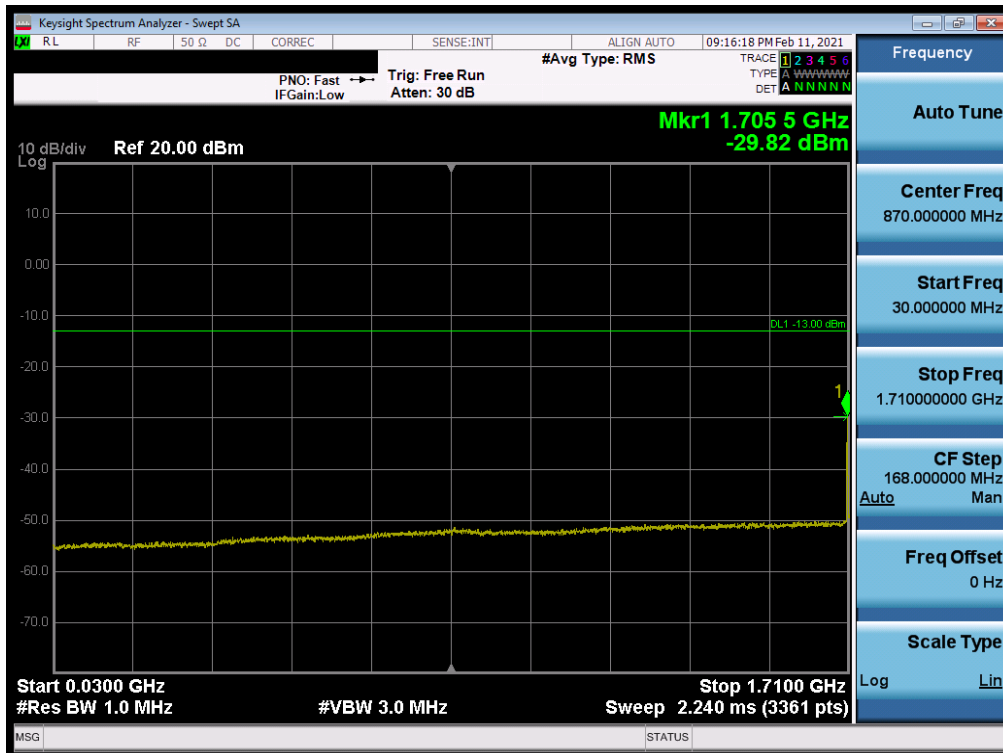
Plot 7-40. Conducted Spurious Plot (LTE Band 4 - 20MHz QPSK - RB Size 1, RB Offset 0 - Mid Channel)
