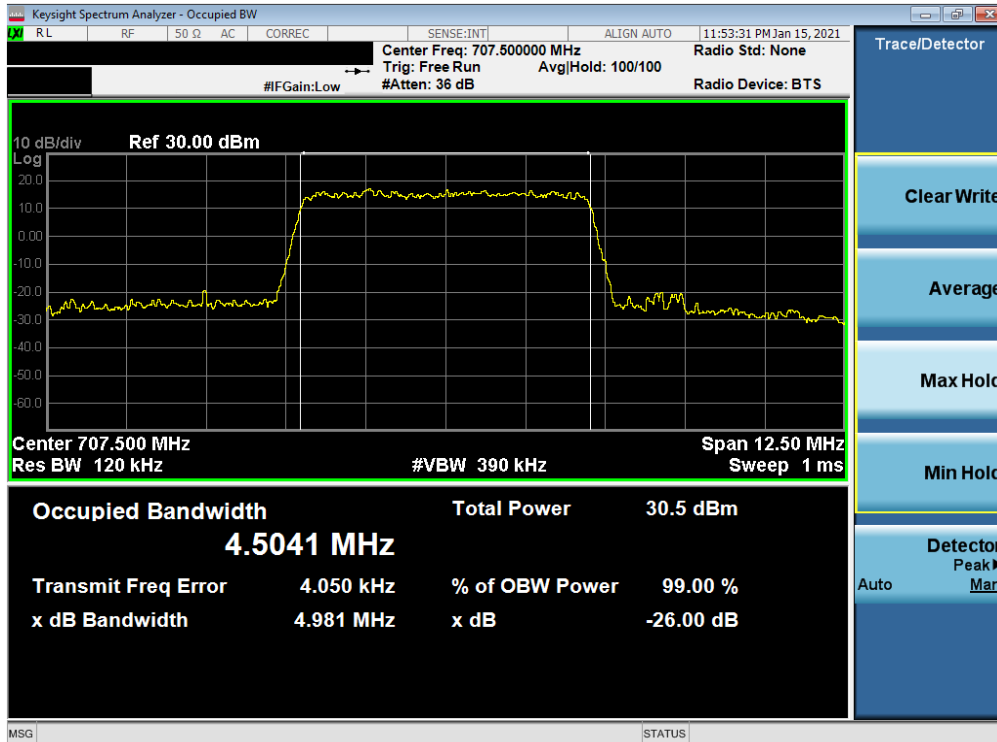
Plot 7-24. Occupied Bandwidth Plot (LTE Band 12 - 5MHz 64-QAM - Full RB)
