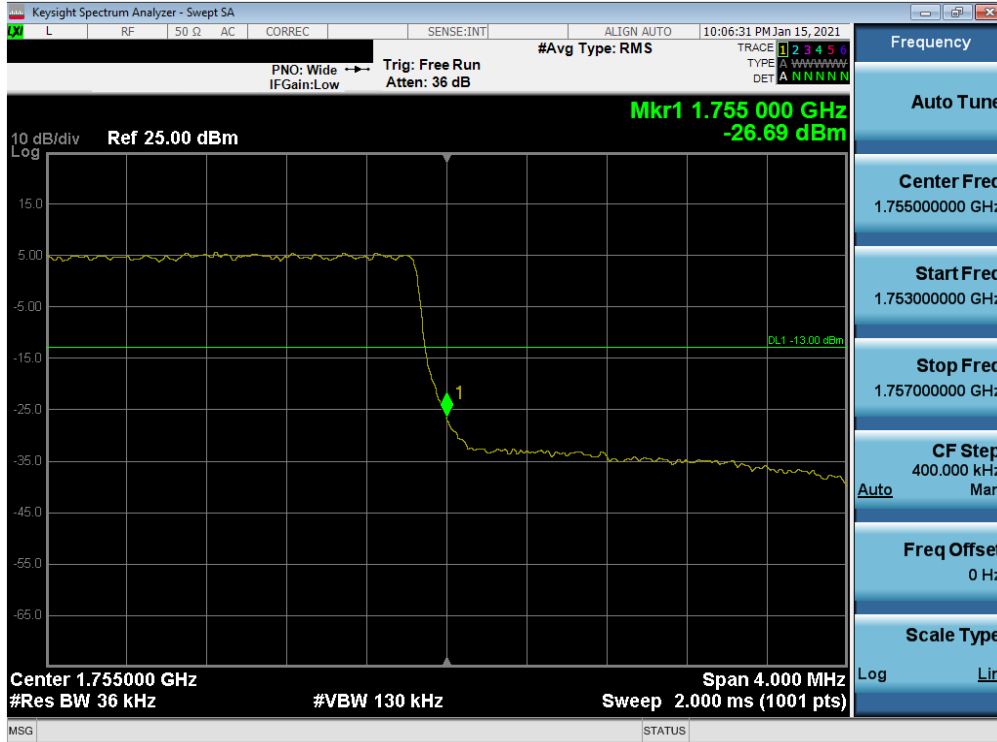
Plot 7-76. Upper Band Edge Plot (LTE Band 4 - 3MHz QPSK – Full RB)
