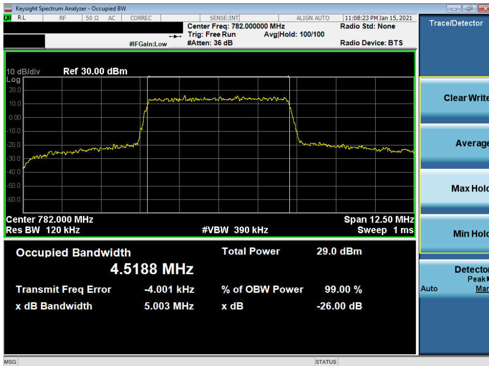
Plot 7-36. Occupied Bandwidth Plot (LTE Band 13 - 5MHz 64-QAM - Full RB)
