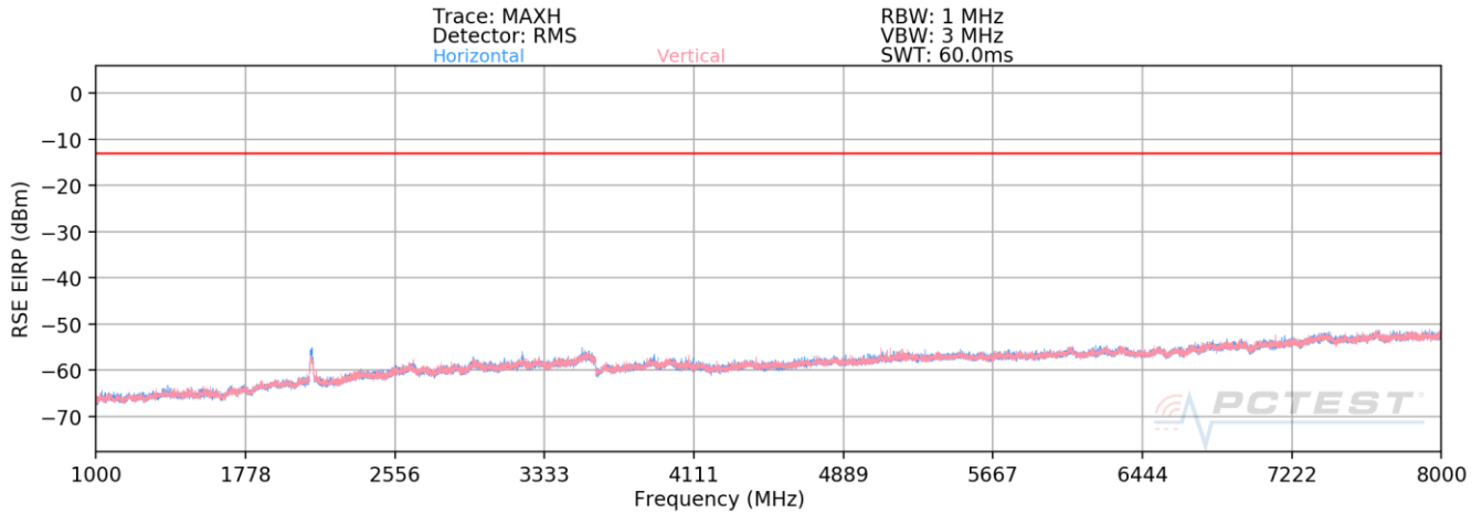
Plot 7-99. Radiated Spurious Plot (LTE Band 12)
