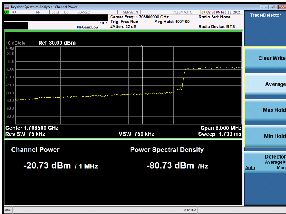
Plot 7-67. Lower Extended Band Edge Plot (LTE Band 4 - 10MHz QPSK – Full RB)
