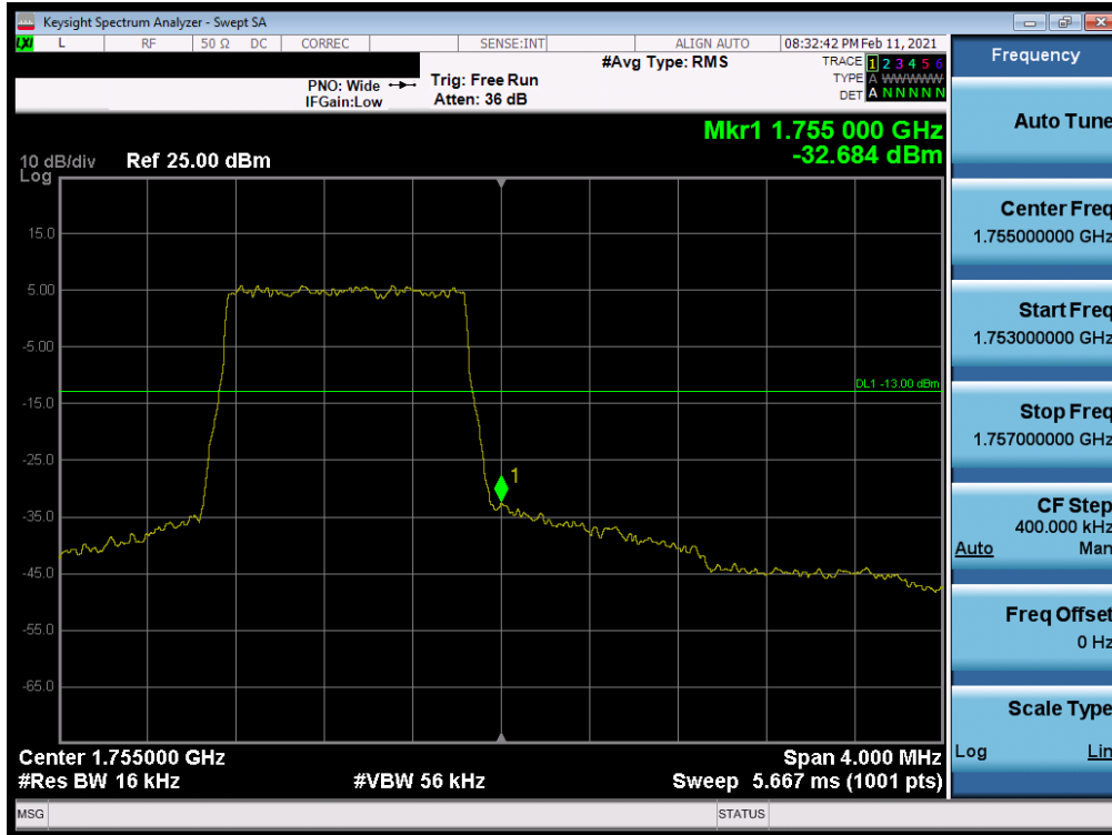
Plot 7-80. Upper Band Edge Plot (LTE Band 4 – 1.4MHz QPSK – Full RB)
