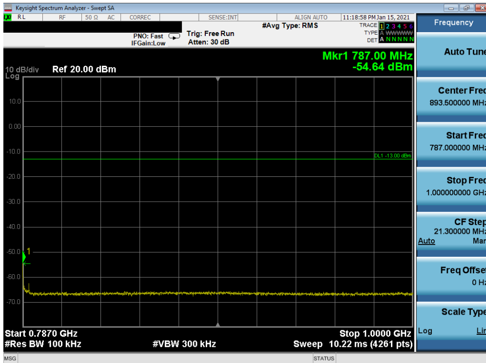
Plot 7-56. Conducted Spurious Plot (LTE Band 13 - 10MHz QPSK - RB Size 1, RB Offset 0)
