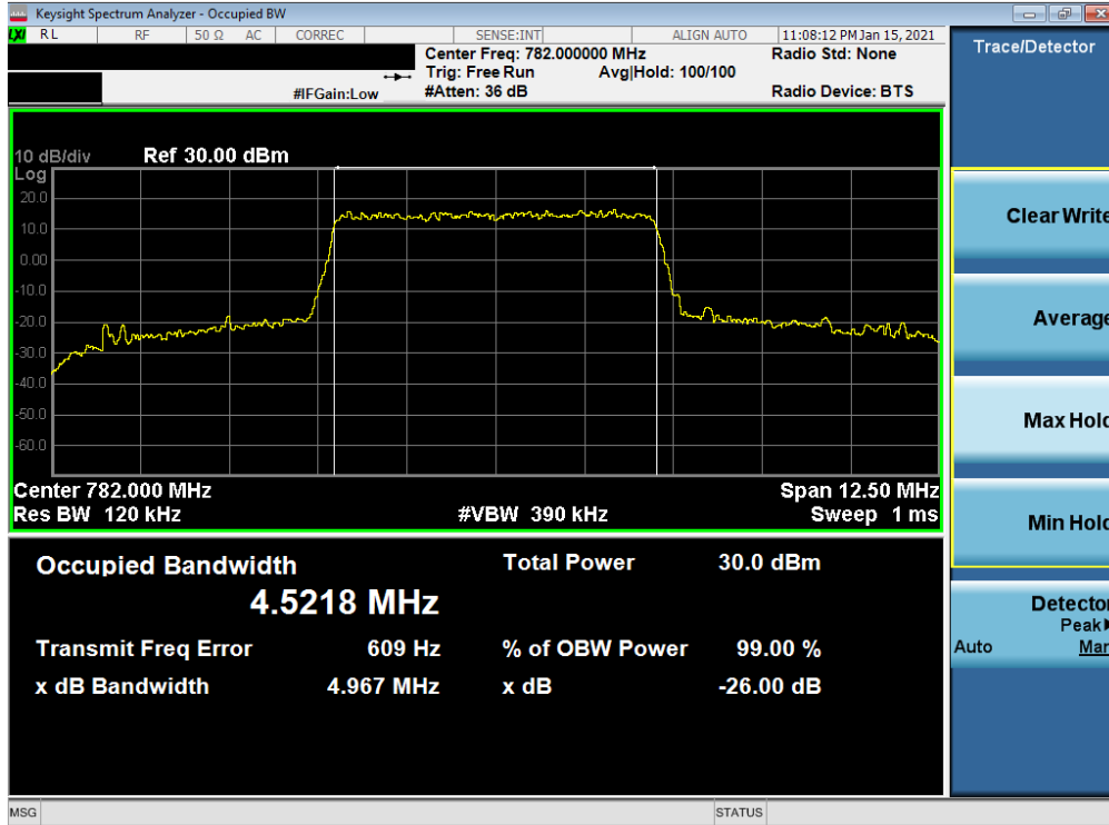
Plot 7-35. Occupied Bandwidth Plot (LTE Band 13 - 5MHz 16-QAM - Full RB)
