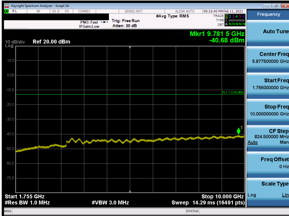
Plot 7-41. Conducted Spurious Plot (LTE Band 4 - 20MHz QPSK - RB Size 1, RB Offset 0 - Mid Channel)
