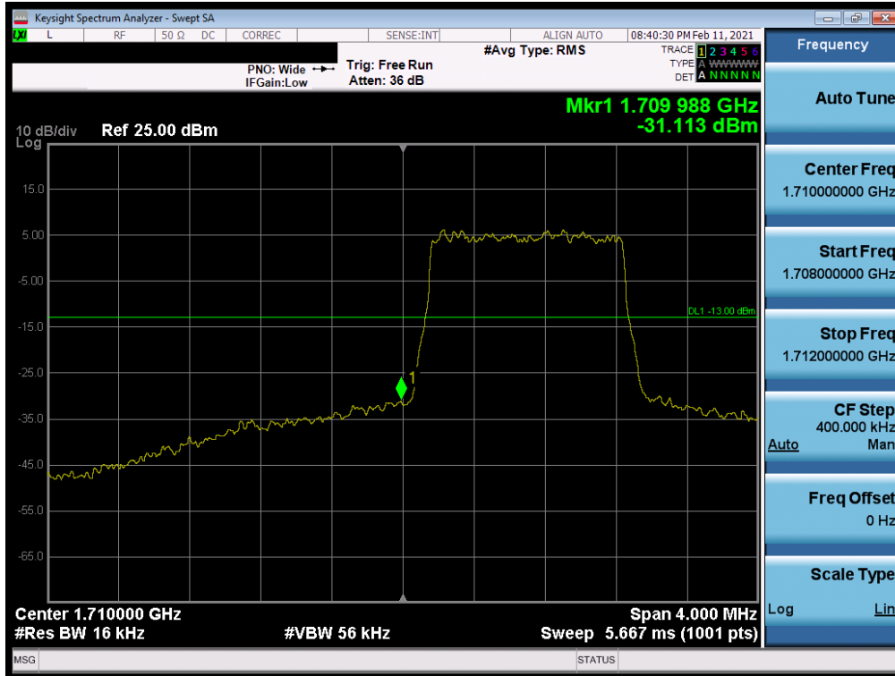
Plot 7-78. Lower Band Edge Plot (LTE Band 4 – 1.4MHz QPSK – Full RB)
