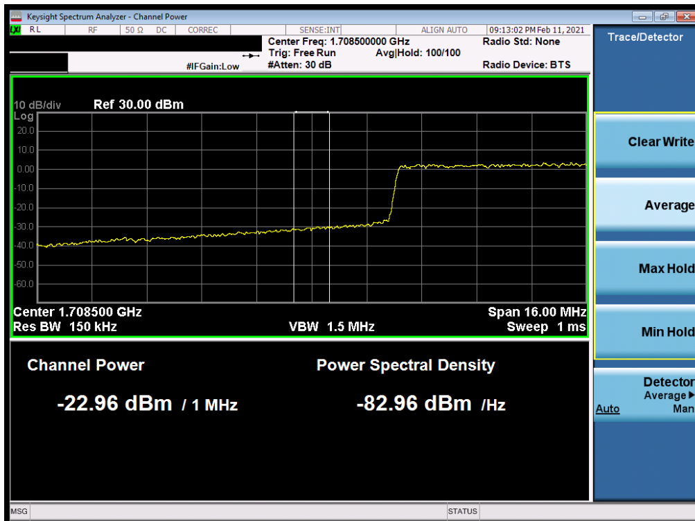
Plot 7-59. Lower Extended Band Edge Plot (LTE Band 4 - 20MHz QPSK – Full RB)
