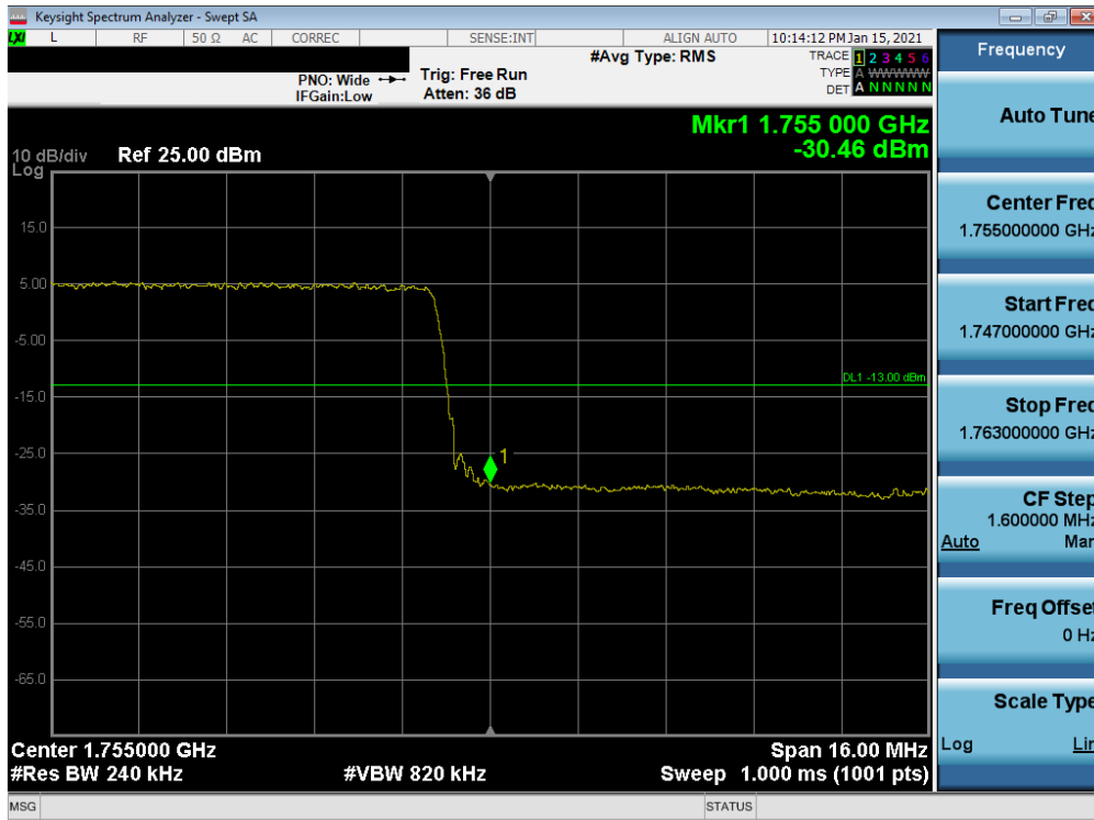
Plot 7-60. Upper Band Edge Plot (LTE Band 4 - 20MHz QPSK – Full RB)
