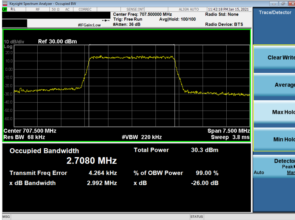
Plot 7-27. Occupied Bandwidth Plot (LTE Band 12 - 3MHz 64-QAM - Full RB)
