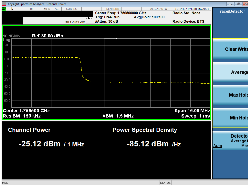
Plot 7-61. Upper Extended Band Edge Plot (LTE Band 4 - 20MHz QPSK – Full RB)
