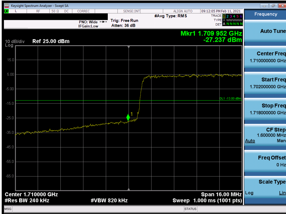
Plot 7-58. Lower Band Edge Plot (LTE Band 4 - 20MHz QPSK – Full RB)
