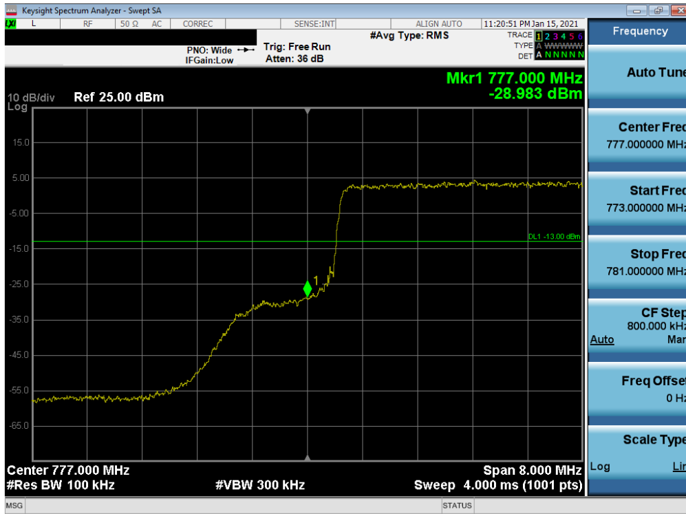
Plot 7-90. Lower Band Edge Plot (LTE Band 13 - 10MHz QPSK – Full RB)
