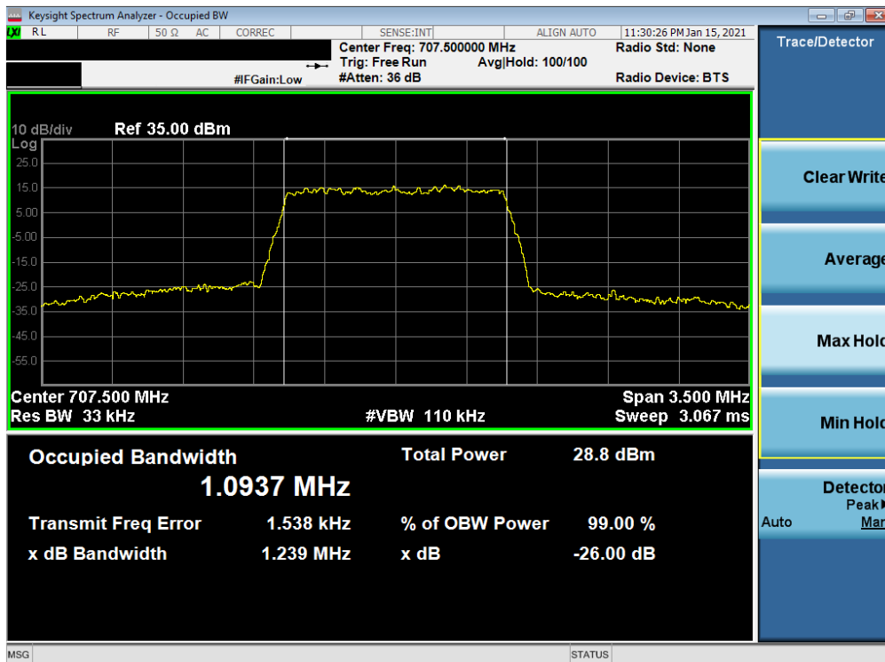
Plot 7-30. Occupied Bandwidth Plot (LTE Band 12 – 1.4MHz 64-QAM - Full RB)
