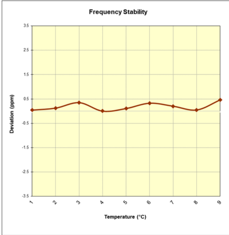
Plot 7-102. LTE Band 12 Frequency Stability Chart
