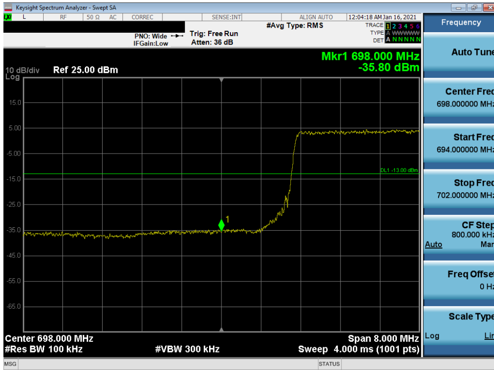
Plot 7-82. Lower Band Edge Plot (LTE Band 12 - 10MHz QPSK – Full RB)
