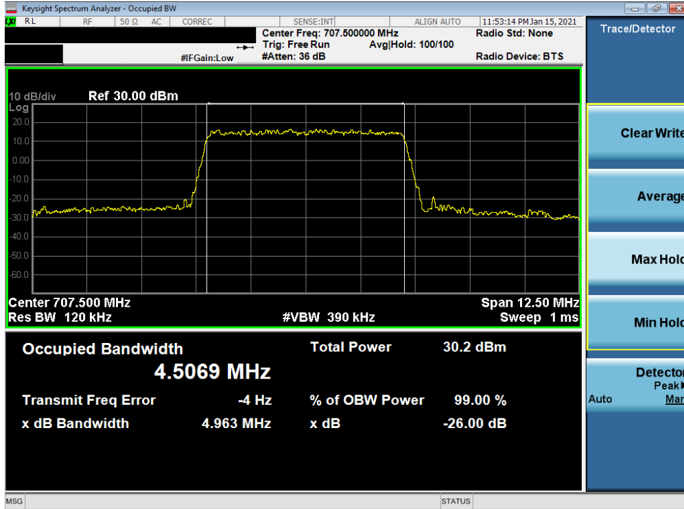
Plot 7-23. Occupied Bandwidth Plot (LTE Band 12 - 5MHz 16-QAM - Full RB)
