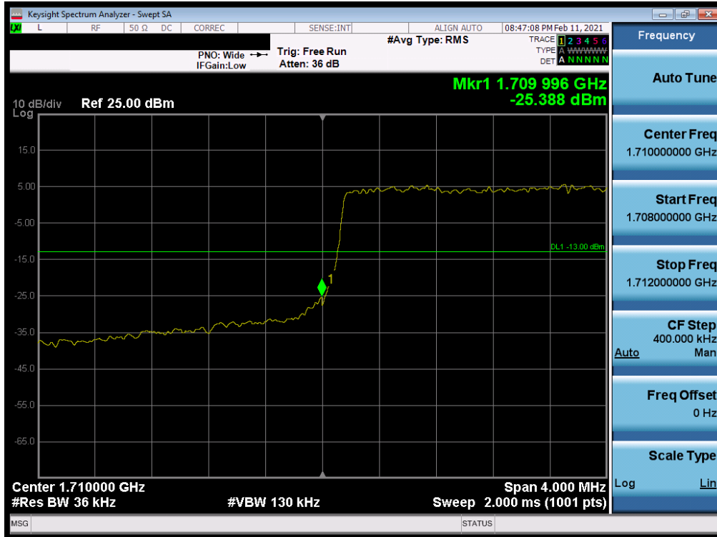
Plot 7-74. Lower Band Edge Plot (LTE Band 4 - 3MHz QPSK – Full RB)
