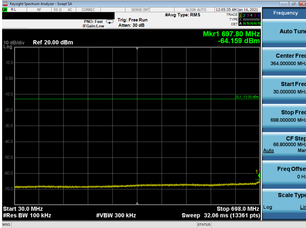
Plot 7-52. Conducted Spurious Plot (LTE Band 12 - 10MHz QPSK - RB Size 1, RB Offset 0 - High Channel)
