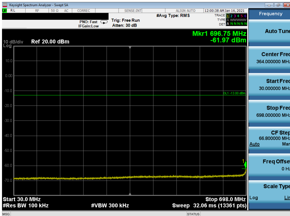
Plot 7-49. Conducted Spurious Plot (LTE Band 12 - 10MHz QPSK - RB Size 1, RB Offset 0 - Mid Channel)
