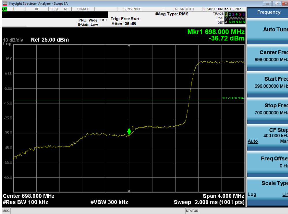
Plot 7-88. Lower Band Edge Plot (LTE Band 12 – 1.4MHz QPSK – Full RB)
