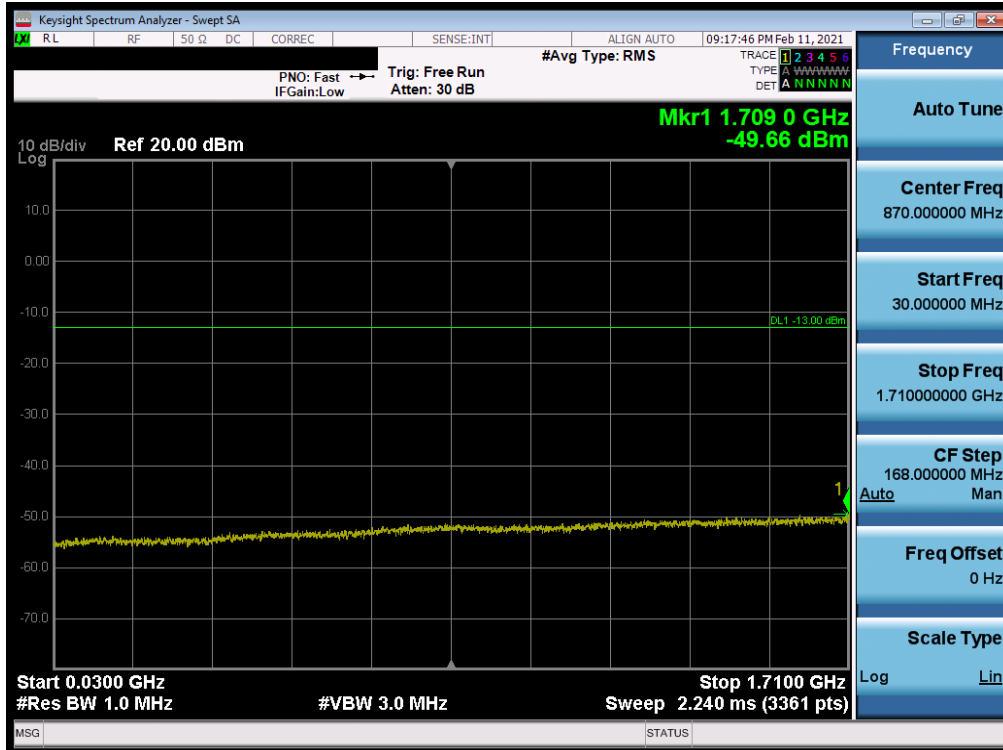
Plot 7-43. Conducted Spurious Plot (LTE Band 4 - 20MHz QPSK - RB Size 1, RB Offset 0 - High Channel)
