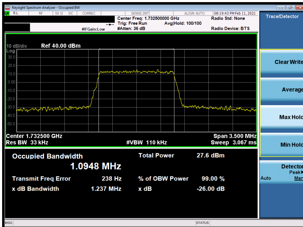
Plot 7-18. Occupied Bandwidth Plot (LTE Band 4 - 1.4MHz 64-QAM - Full RB Configuration)
