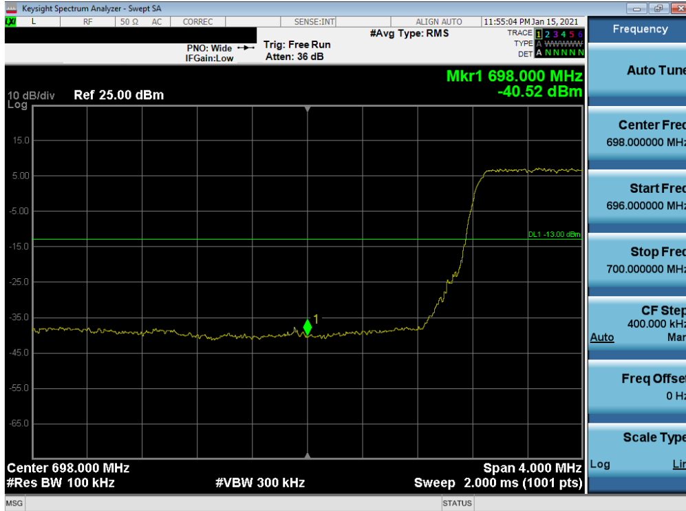
Plot 7-84. Lower Band Edge Plot (LTE Band 12 - 5MHz QPSK – Full RB)
