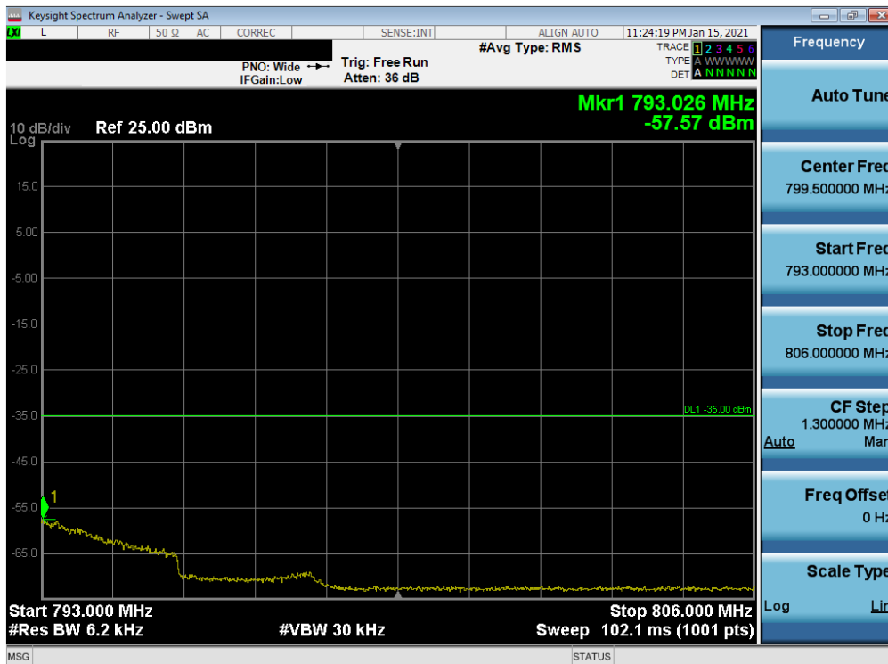
Plot 7-93. Upper Emission Mask Plot (LTE Band 13 - 10MHz QPSK – Full RB)
