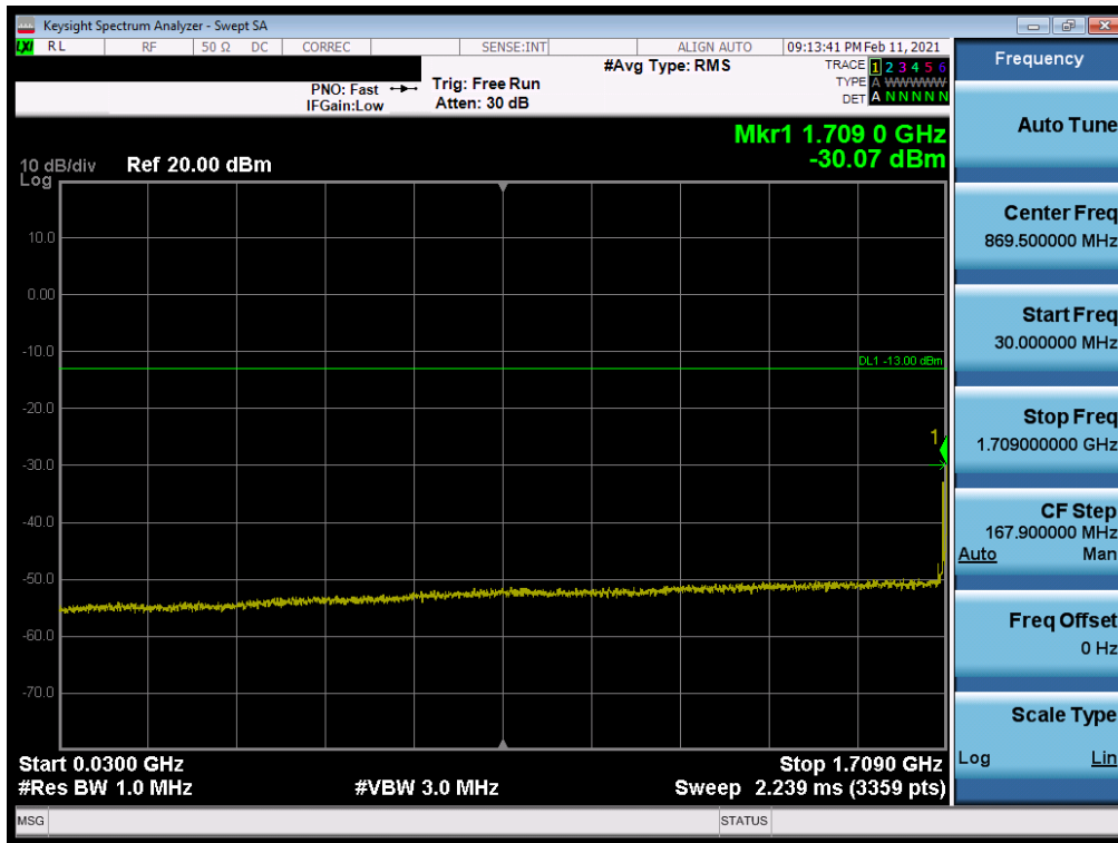
Plot 7-37. Conducted Spurious Plot (LTE Band 4 - 20MHz QPSK - RB Size 1, RB Offset 0-Low Channel)
