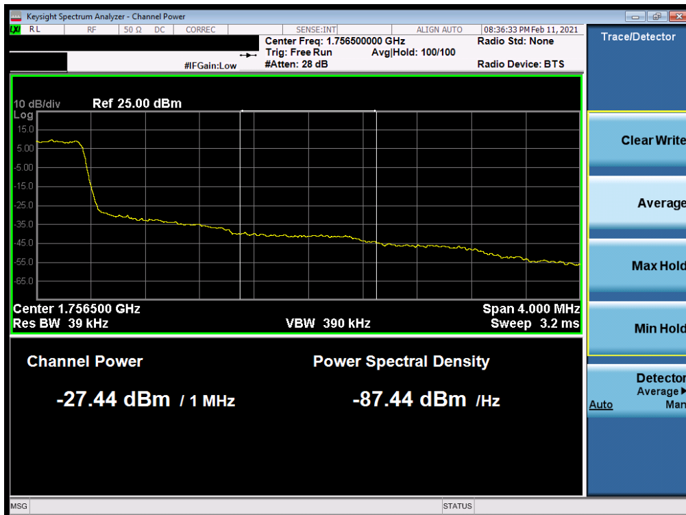
Plot 7-81. Upper Extended Band Edge Plot (LTE Band 4 – 1.4MHz QPSK – Full RB)
