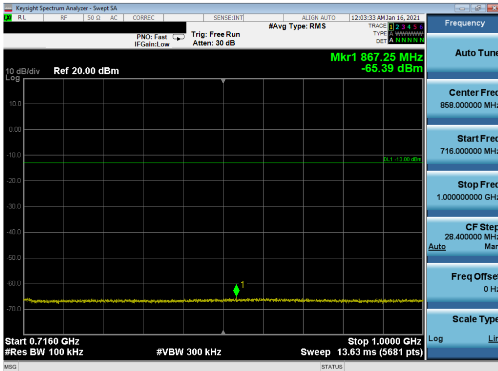
Plot 7-47. Conducted Spurious Plot (LTE Band 12 - 10MHz QPSK - RB Size 1, RB Offset 0 - Low Channel)
