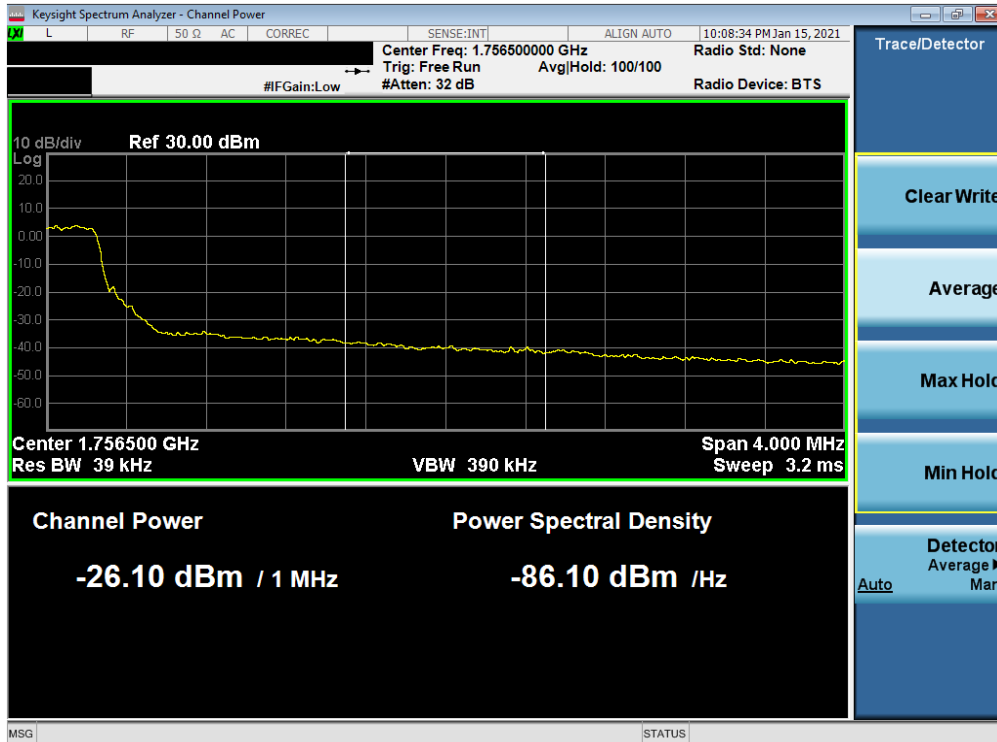
Plot 7-73. Upper Extended Band Edge Plot (LTE Band 4 - 5MHz QPSK – Full RB)
