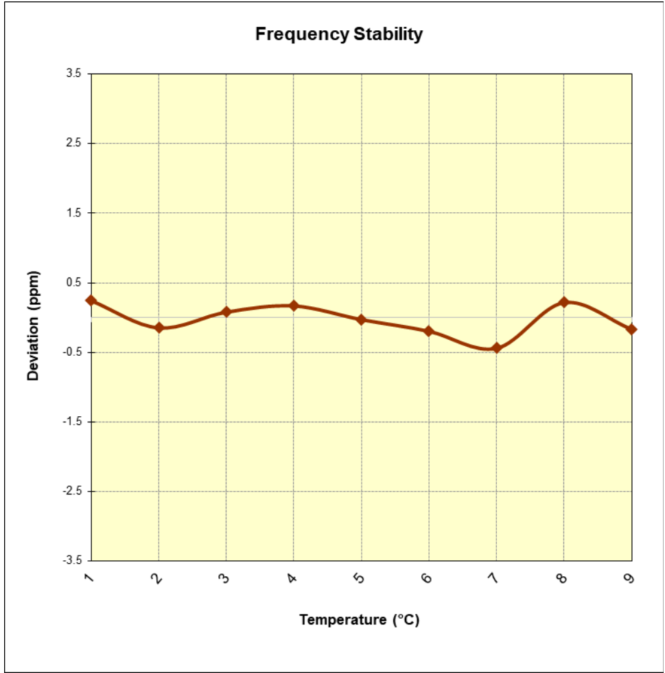
Plot 7-103. LTE Band 13 Frequency Stability Chart
