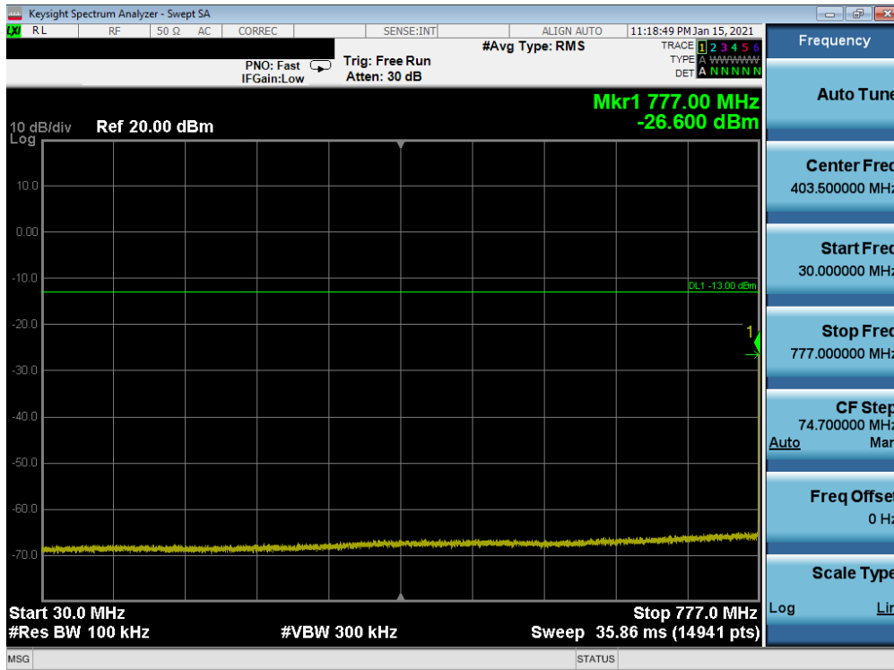
Plot 7-55. Conducted Spurious Plot (LTE Band 13 - 10MHz QPSK - RB Size 1, RB Offset 0)
