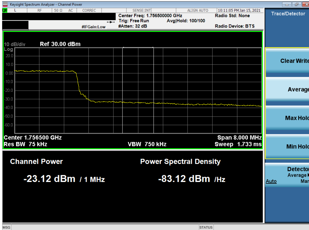
Plot 7-69. Upper Extended Band Edge Plot (LTE Band 4 - 10MHz QPSK – Full RB)
