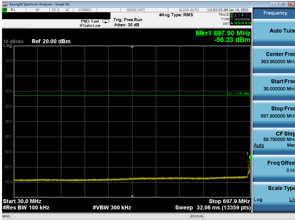
Plot 7-46. Conducted Spurious Plot (LTE Band 12 - 10MHz QPSK - RB Size 1, RB Offset 0 - Low Channel)
