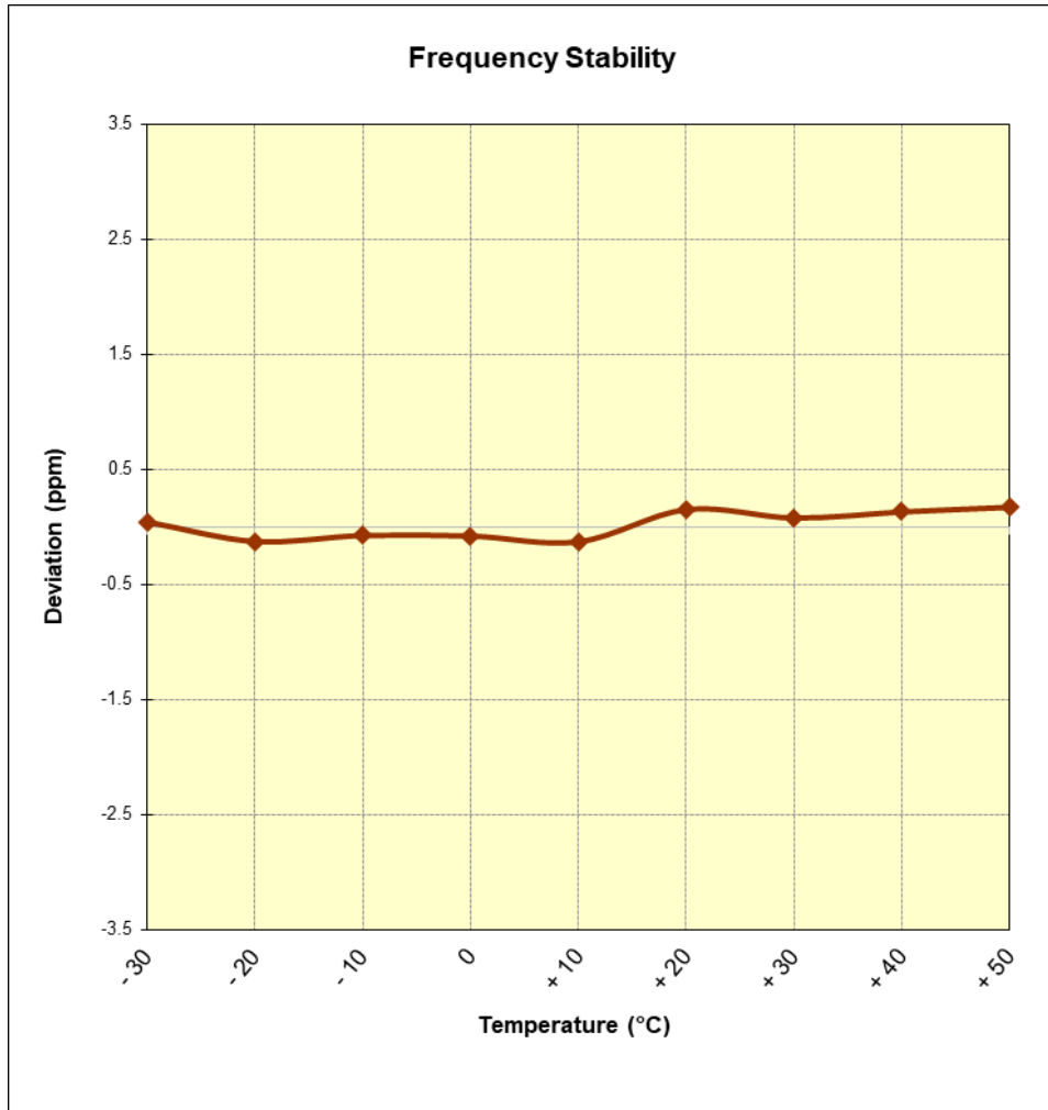
Plot 7-101. LTE Band 4 Frequency Stability Chart
