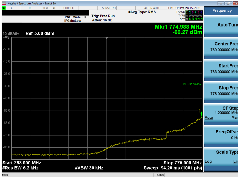
Plot 7-95. Lower Emission Mask Plot (LTE Band 13 - 5MHz QPSK – Full RB)
