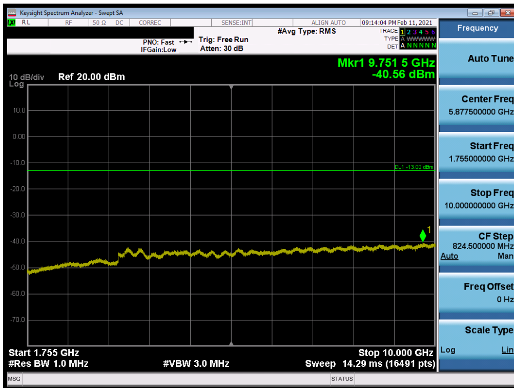
Plot 7-38. Conducted Spurious Plot (LTE Band 4 - 20MHz QPSK - RB Size 1, RB Offset 0 - Low Channel)
