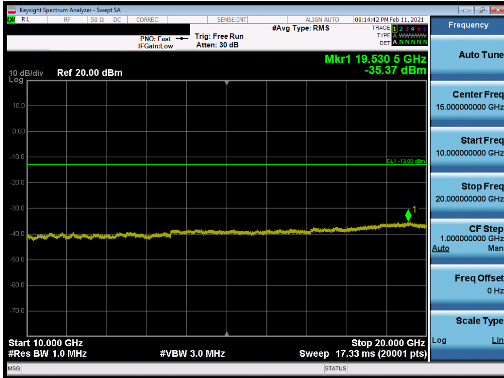
Plot 7-39. Conducted Spurious Plot (LTE Band 4 - 20MHz QPSK - RB Size 1, RB Offset 0 - Low Channel)
