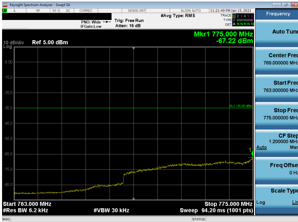
Plot 7-91. Lower Emission Mask Plot (LTE Band 13 - 10MHz QPSK – Full RB)
