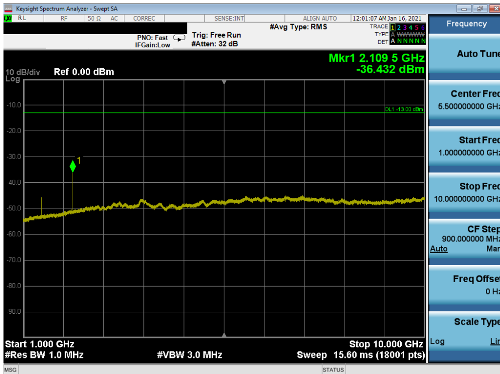
Plot 7-51. Conducted Spurious Plot (LTE Band 12 - 10MHz QPSK - RB Size 1, RB Offset 0 - Mid Channel)
