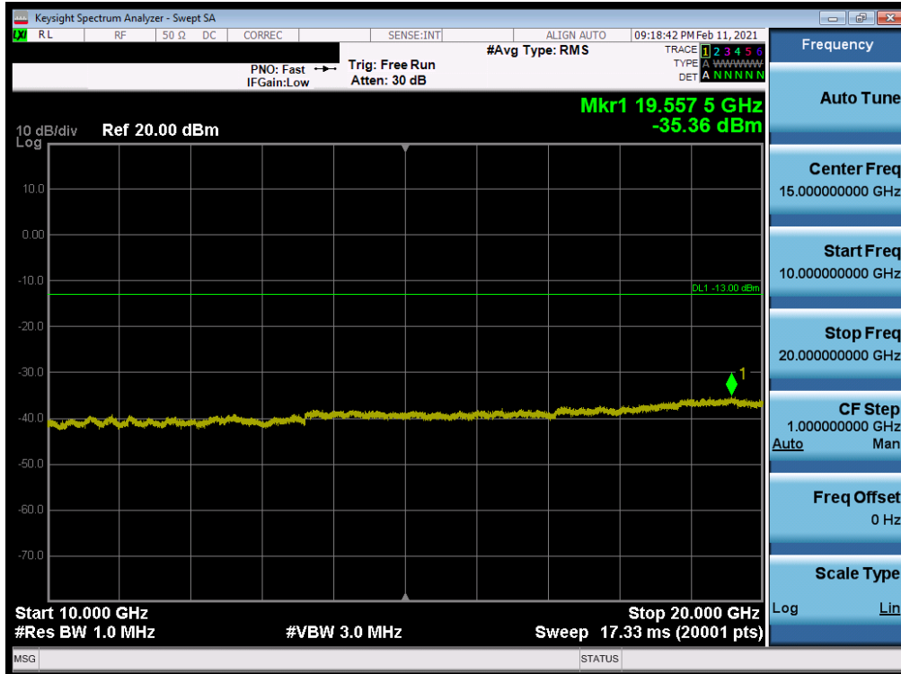
Plot 7-45. Conducted Spurious Plot (LTE Band 4 - 20MHz QPSK - RB Size 1, RB Offset 0 - High Channel)
