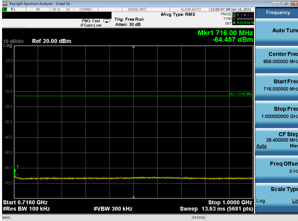
Plot 7-50. Conducted Spurious Plot (LTE Band 12 - 10MHz QPSK - RB Size 1, RB Offset 0 - Mid Channel)
