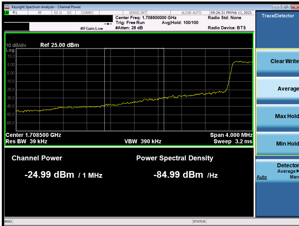
Plot 7-79. Lower Extended Band Edge Plot (LTE Band 4 – 1.4MHz QPSK – Full RB)
