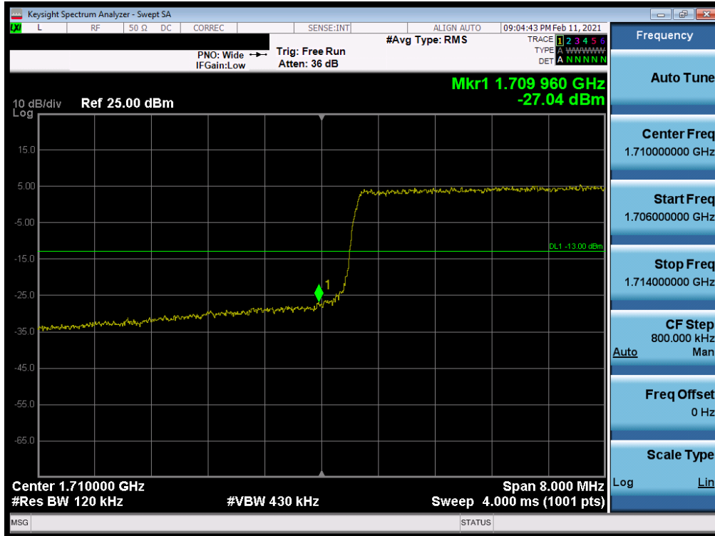
Plot 7-66. Lower Band Edge Plot (LTE Band 4 - 10MHz QPSK – Full RB)
