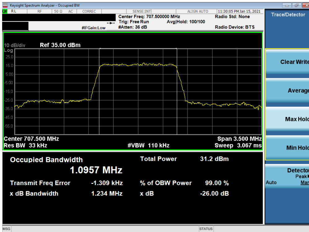
Plot 7-28. Occupied Bandwidth Plot (LTE Band 12 - 1.4MHz QPSK - Full RB)
