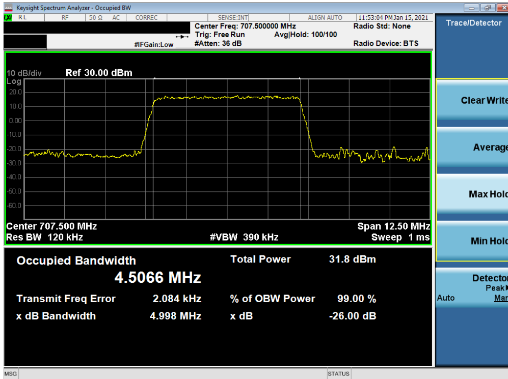
Plot 7-22. Occupied Bandwidth Plot (LTE Band 12 - 5MHz QPSK - Full RB)
