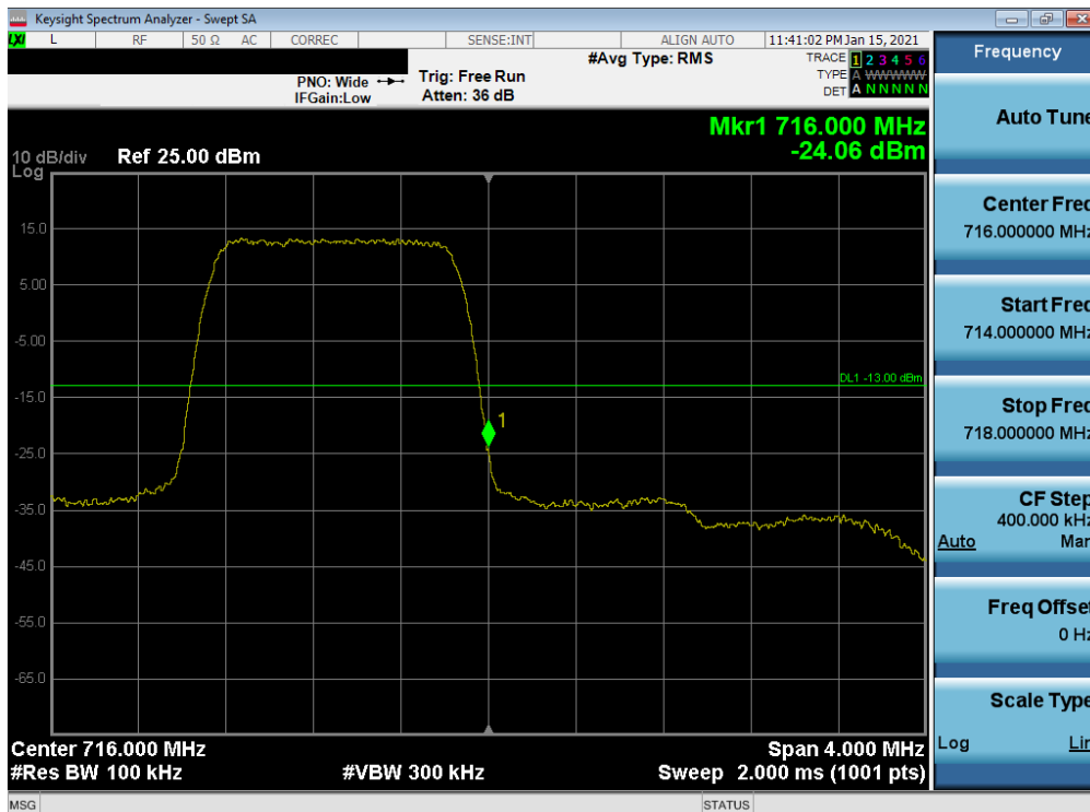
Plot 7-89. Upper Band Edge Plot (LTE Band 12 – 1.4MHz QPSK – Full RB)
