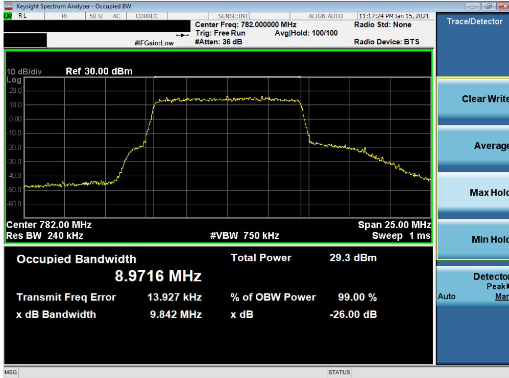
Plot 7-33. Occupied Bandwidth Plot (LTE Band 13 - 10MHz 64-QAM - Full RB)
