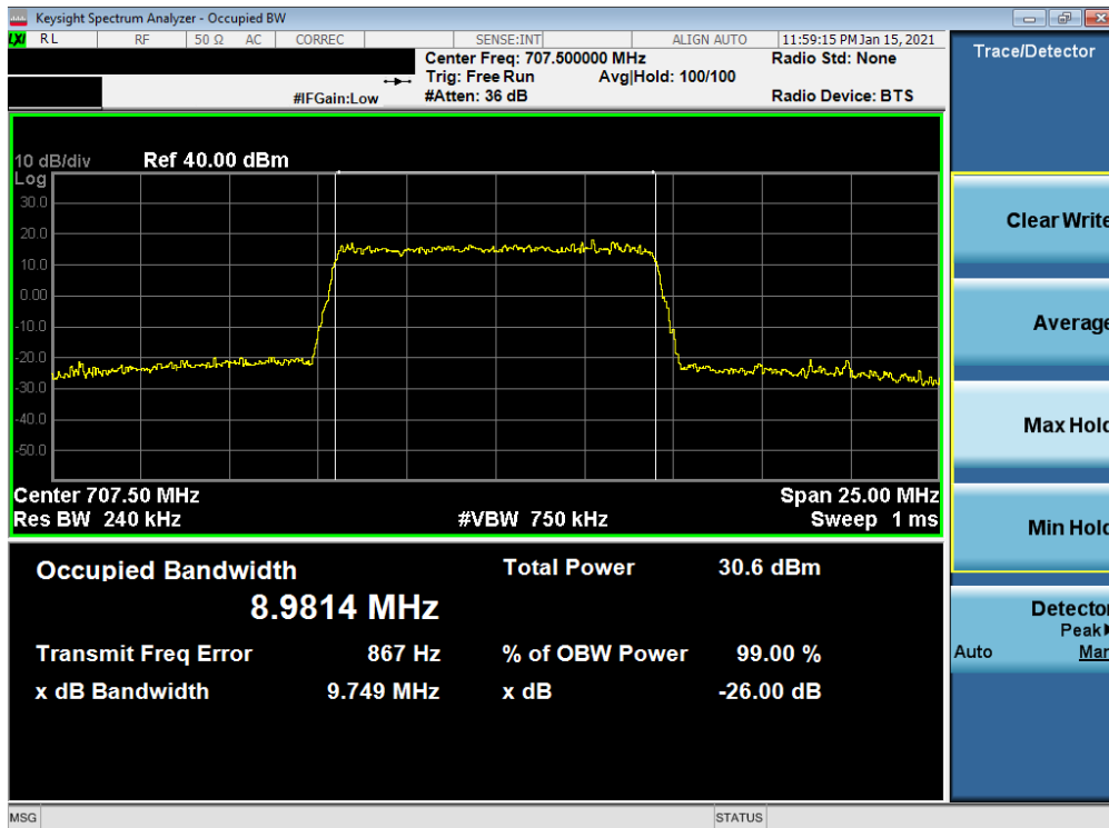
Plot 7-20. Occupied Bandwidth Plot (LTE Band 12 - 10MHz 16-QAM - Full RB)
