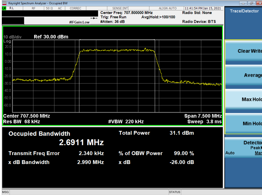
Plot 7-25. Occupied Bandwidth Plot (LTE Band 12 - 3MHz QPSK - Full RB)
