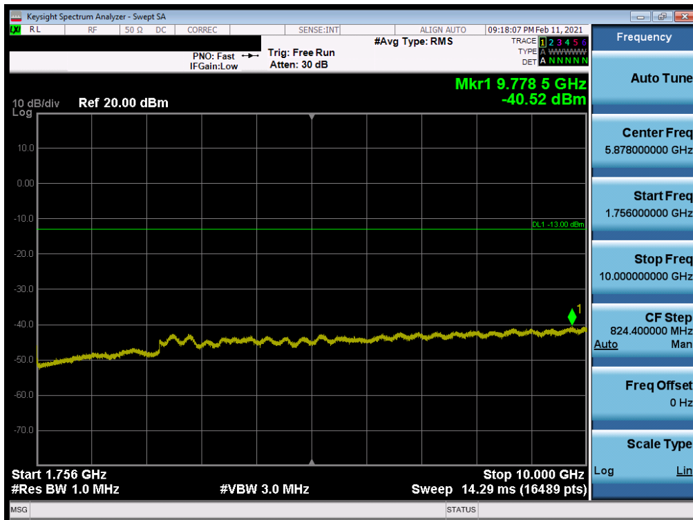
Plot 7-44. Conducted Spurious Plot (LTE Band 4 - 20MHz QPSK - RB Size 1, RB Offset 0 - High Channel)
