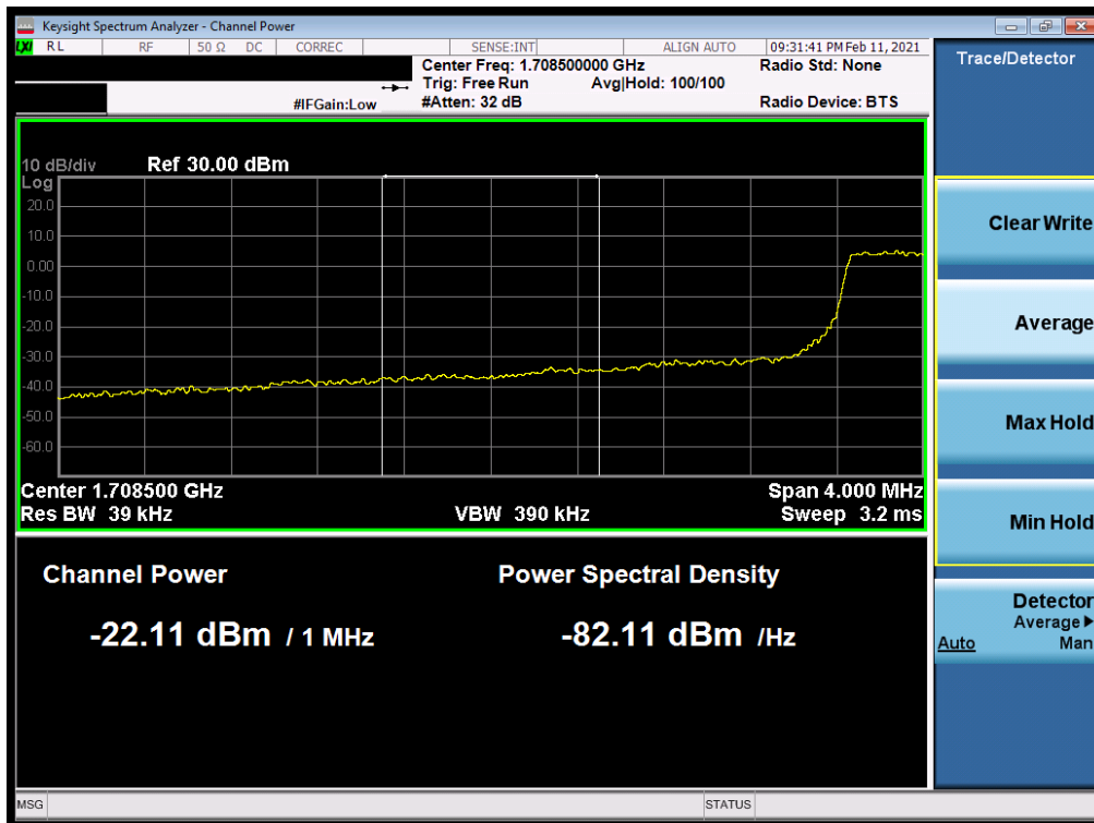
Plot 7-75. Lower Extended Band Edge Plot (LTE Band 4 - 3MHz QPSK – Full RB)
