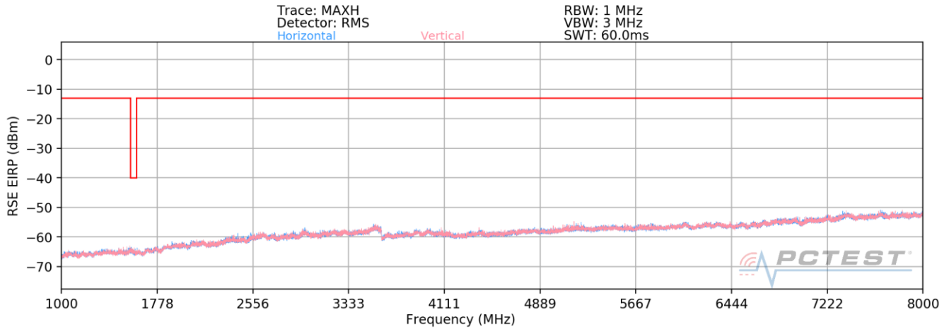
Plot 7-100. Radiated Spurious Plot (LTE Band 13)
