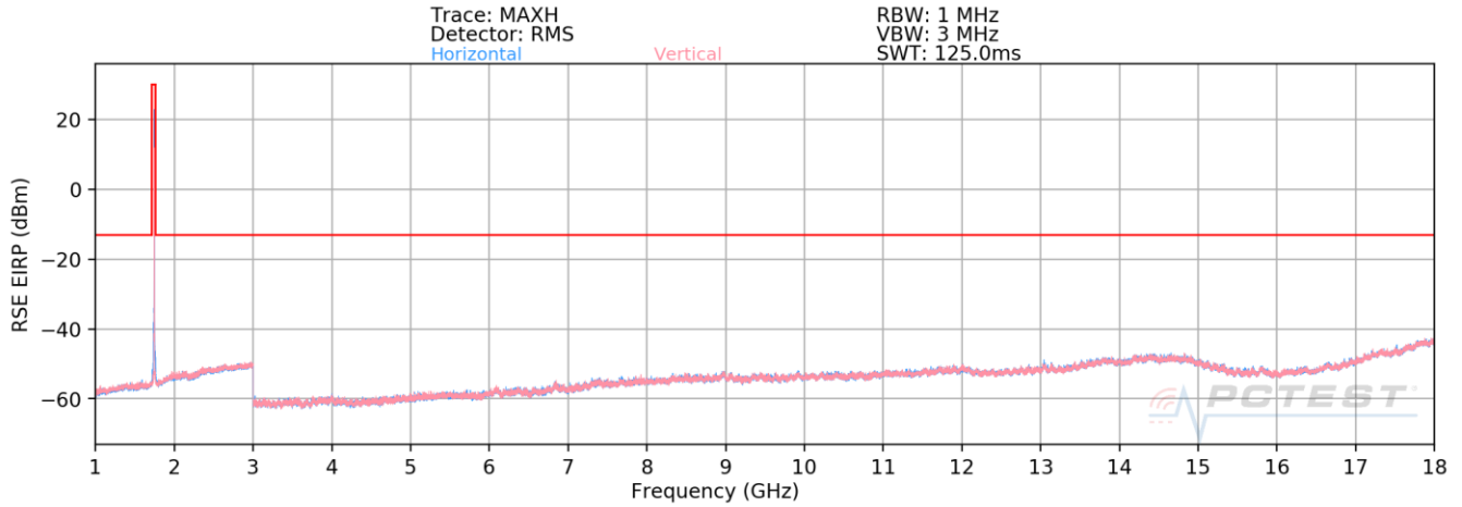
Plot 7-98. Radiated Spurious Plot (LTE Band 4)
