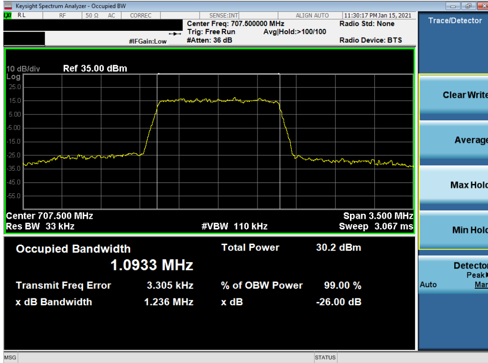
Plot 7-29. Occupied Bandwidth Plot (LTE Band 12 – 1.4MHz 16-QAM - Full RB)
