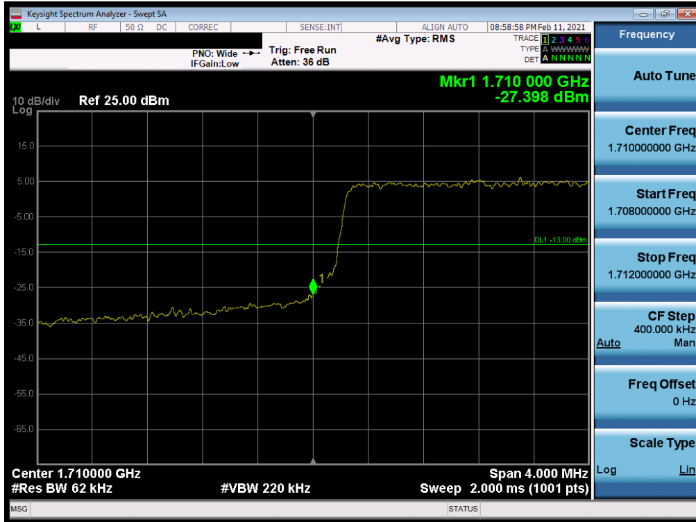
Plot 7-70. Lower Band Edge Plot (LTE Band 4 - 5MHz QPSK – Full RB)
