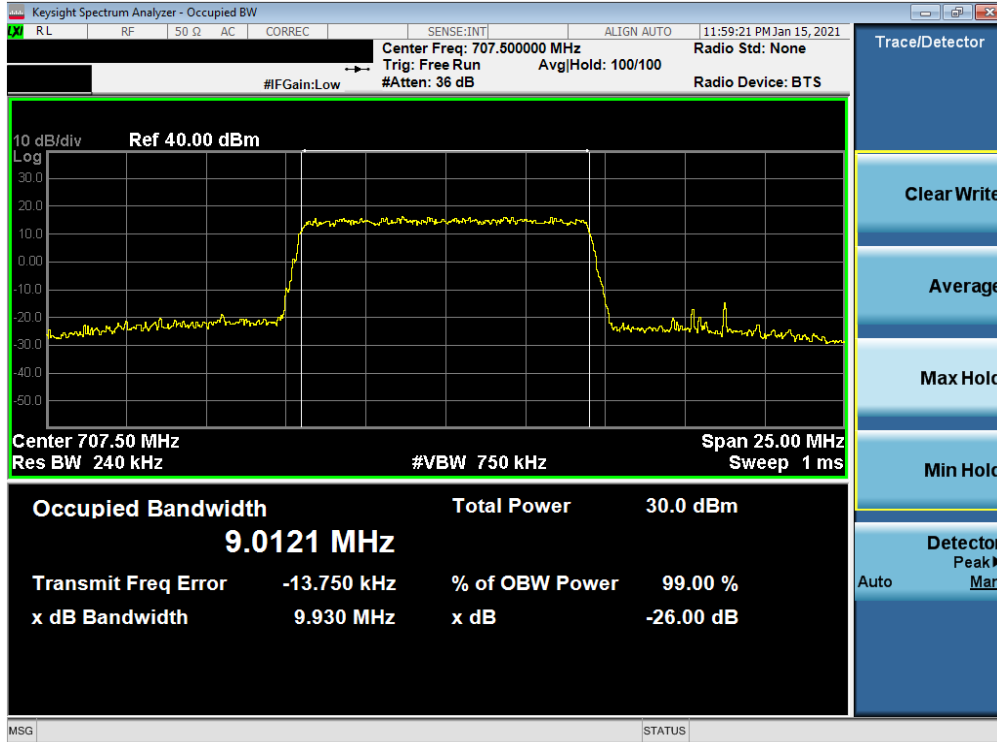
Plot 7-21. Occupied Bandwidth Plot (LTE Band 12 - 10MHz 64-QAM - Full RB)
