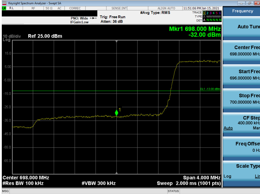
Plot 7-86. Lower Band Edge Plot (LTE Band 12 - 3MHz QPSK – Full RB)
