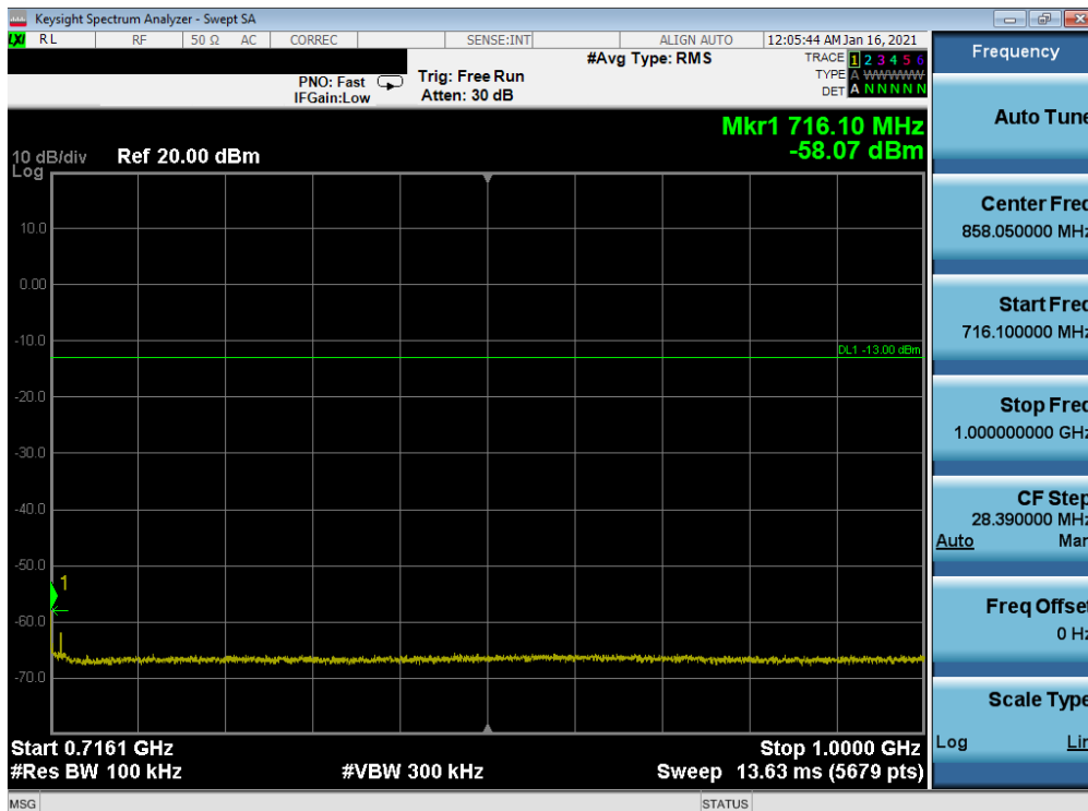
Plot 7-53. Conducted Spurious Plot (LTE Band 12 - 10MHz QPSK - RB Size 1, RB Offset 0 - High Channel)
