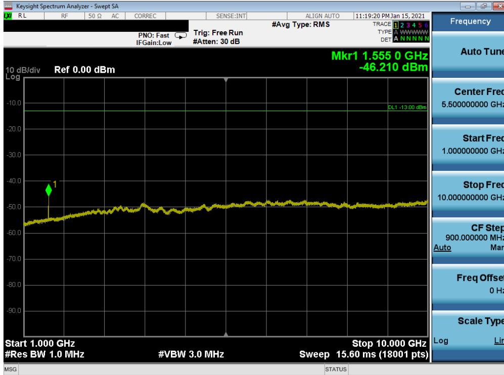
Plot 7-57. Conducted Spurious Plot (LTE Band 13 - 10MHz QPSK - RB Size 1, RB Offset 0)
