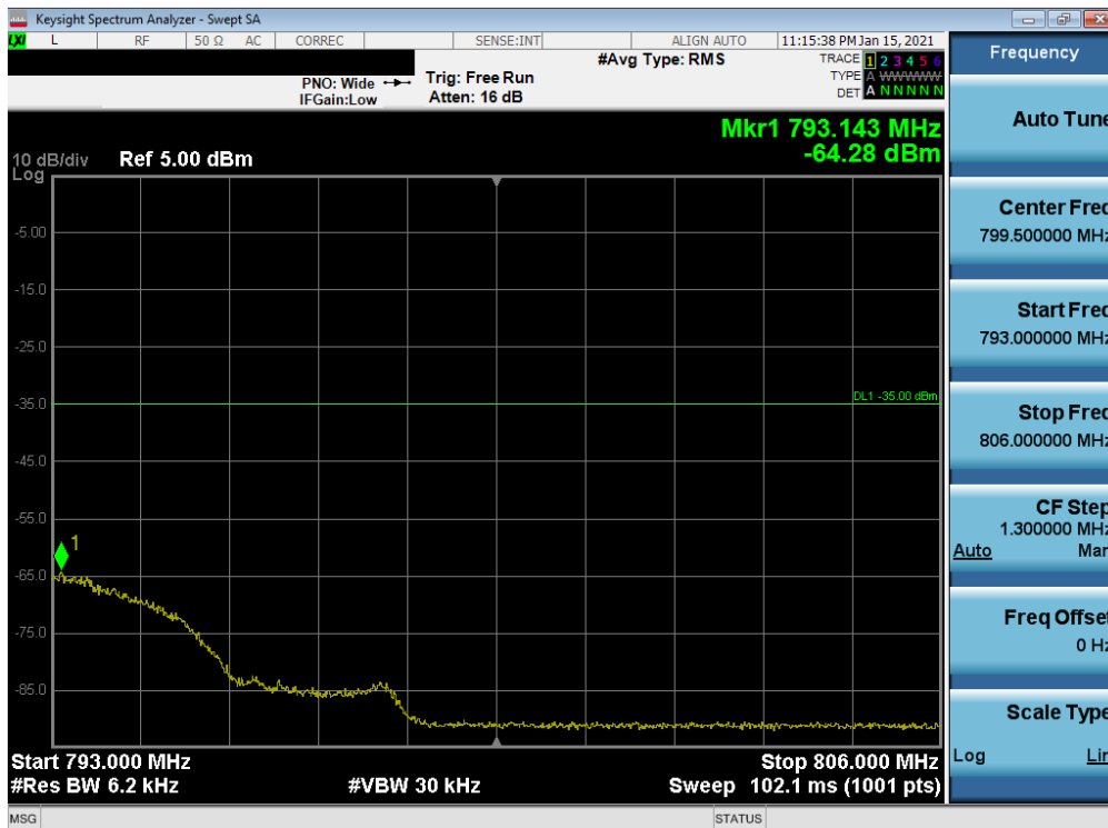
Plot 7-97. Upper Emission Mask Plot (LTE Band 13 - 5MHz QPSK – Full RB)
