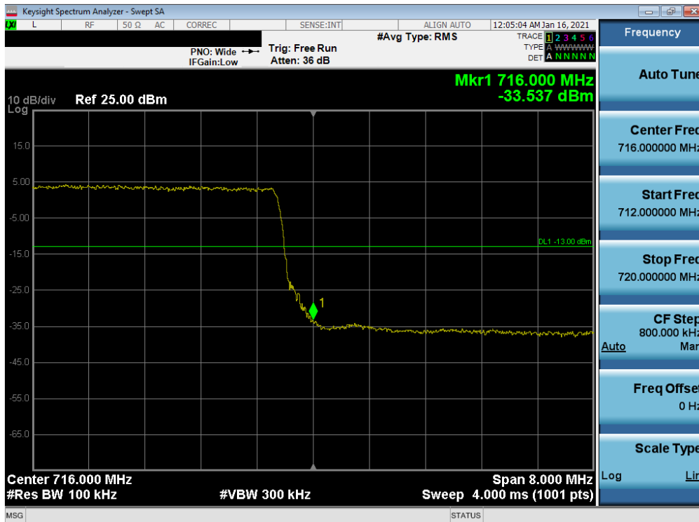
Plot 7-83. Upper Band Edge Plot (LTE Band 12 - 10MHz QPSK – Full RB)
