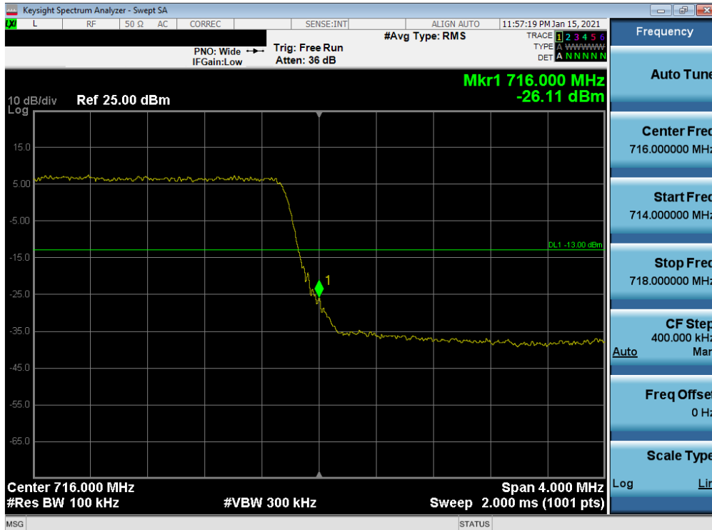
Plot 7-85. Upper Band Edge Plot (LTE Band 12 - 5MHz QPSK – Full RB)
