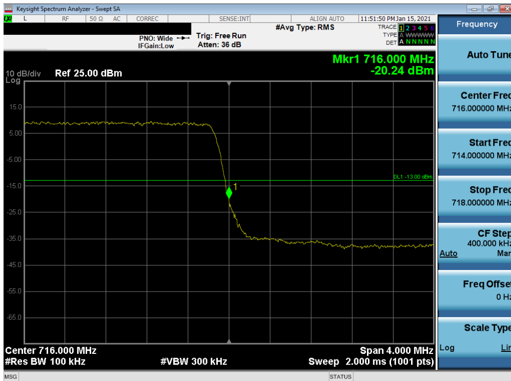
Plot 7-87. Upper Band Edge Plot (LTE Band 12 - 3MHz QPSK – Full RB)
