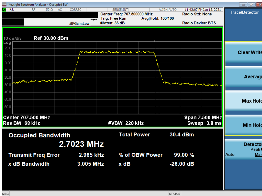
Plot 7-26. Occupied Bandwidth Plot (LTE Band 12 - 3MHz 16-QAM - Full RB)
