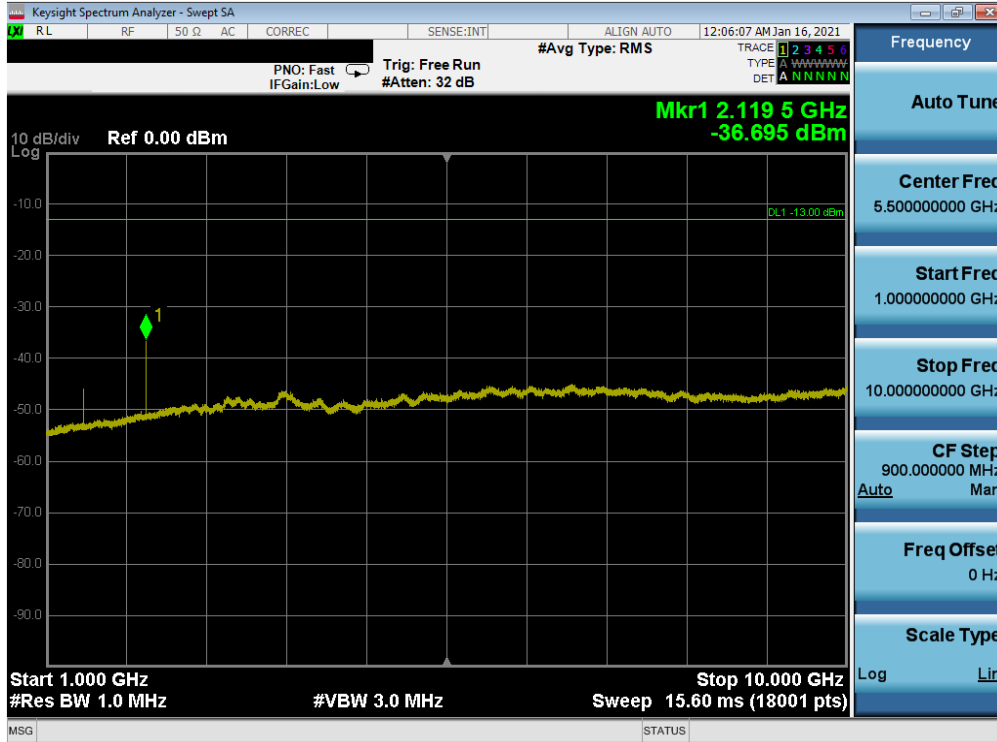
Plot 7-54. Conducted Spurious Plot (LTE Band 12 - 10MHz QPSK - RB Size 1, RB Offset 0 - High Channel)
