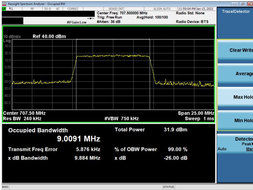
Plot 7-19. Occupied Bandwidth Plot (LTE Band 12 - 10MHz QPSK - Full RB)
