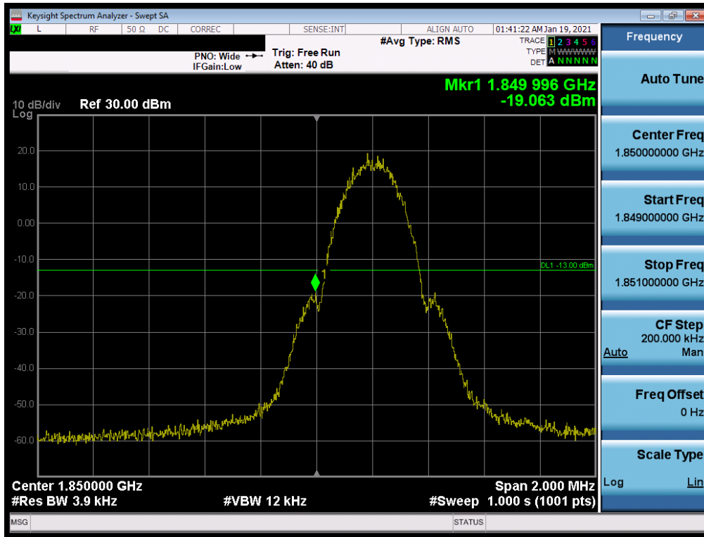
Plot 7-12. Lower Band Edge Plot (GPRS PCS – Ch. 512)
