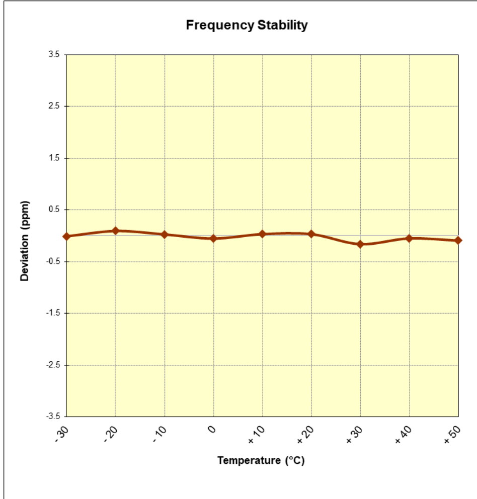
Plot 7-17. GSM/GPRS PCS Frequency Stability Chart
