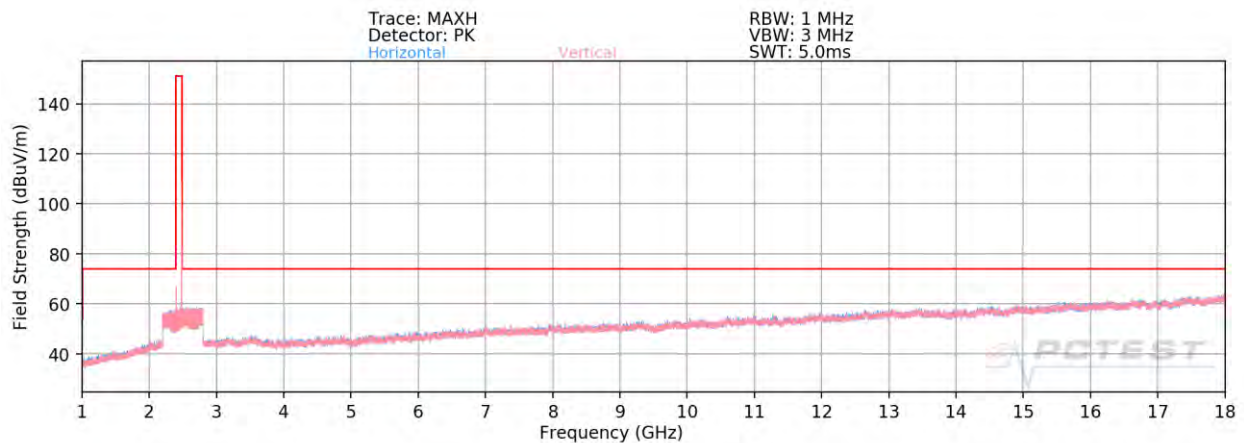
Plot 7-124. Radiated Spurious Plot above 1GHz Ant-1 (BT- Ch. 78)
