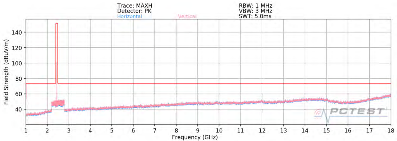
Plot 7-120. Radiated Spurious Plot above 1GHz Ant-1 (BT - Ch. 39)
