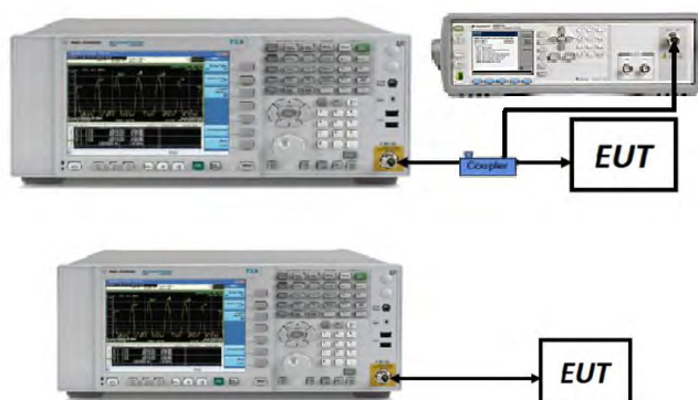
Figure 7-5. Test Instrument & Measurement Setup
