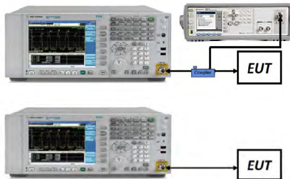
Figure 7-6. Test Instrument & Measurement Setup
