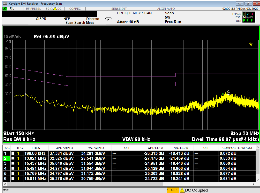
Plot 7-143. Line-Conducted Test Plot (N)-ANT 2
