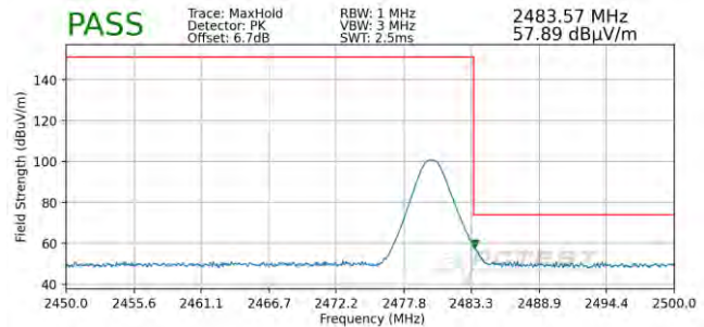
Plot 7-140. Radiated Restricted Upper Band Edge Measurement with WCP (Peak)- Dual BT
