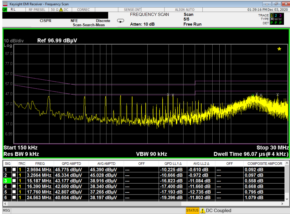
Plot 7-144. Line-Conducted Test Plot (L1) with WCP-ANT 2
