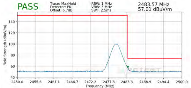
Plot 7-138. Radiated Restricted Upper Band Edge Measurement with WCP (Peak)-ANT 2
