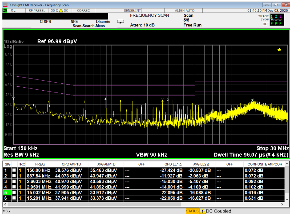
Plot 7-145. Line-Conducted Test Plot (N) with WCP-ANT 2
