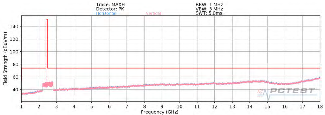
Plot 7-126. Radiated Spurious Plot above 1GHz Dual BT, Ant-1 + Ant-2 (BT - Ch. 39)
