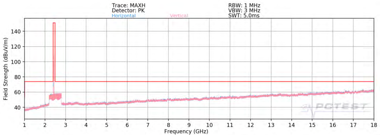
Plot 7-123. Radiated Spurious Plot above 1GHz Ant21 (BT - Ch. 39)
