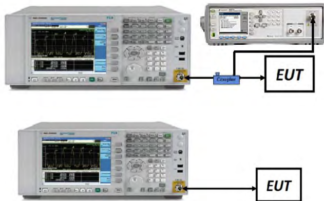
Figure 7-4. Test Instrument & Measurement Setup
