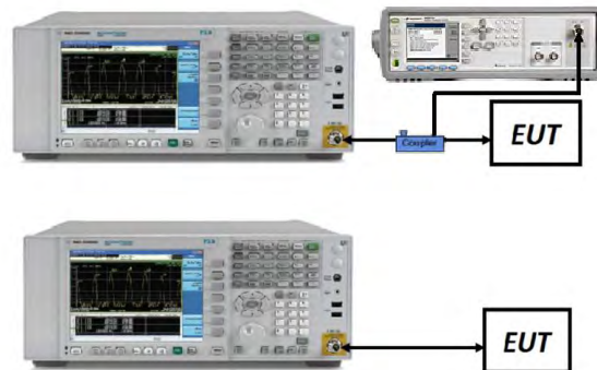
Figure 7-7. Test Instrument & Measurement Setup
