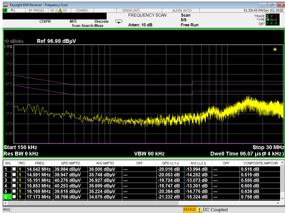
Plot 7-142. Line-Conducted Test Plot (L1)-ANT 2
