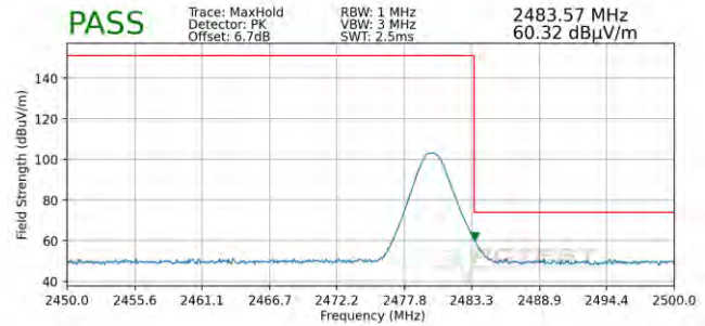
Plot 7-134. Radiated Restricted Upper Band Edge Measurement (Peak)-ANT 2
