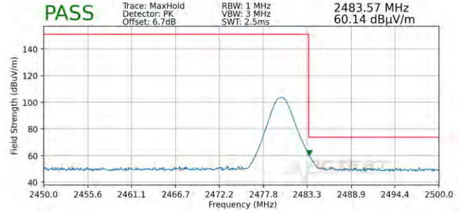
Plot 7-132. Radiated Restricted Upper Band Edge Measurement with WCP (Peak)-ANT 1
