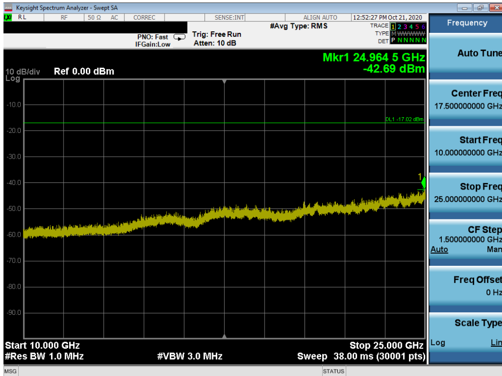
Plot 7-48. Conducted Spurious Plot ANT1 (802.11ax OFDMA – 26 Tones – Ch. 6)
