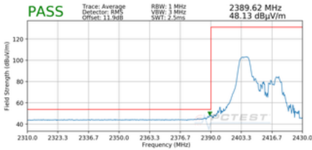
Plot 7-85. Radiated Restricted Lower Band Edge Measurement MIMO (Average – 52 Tones)
