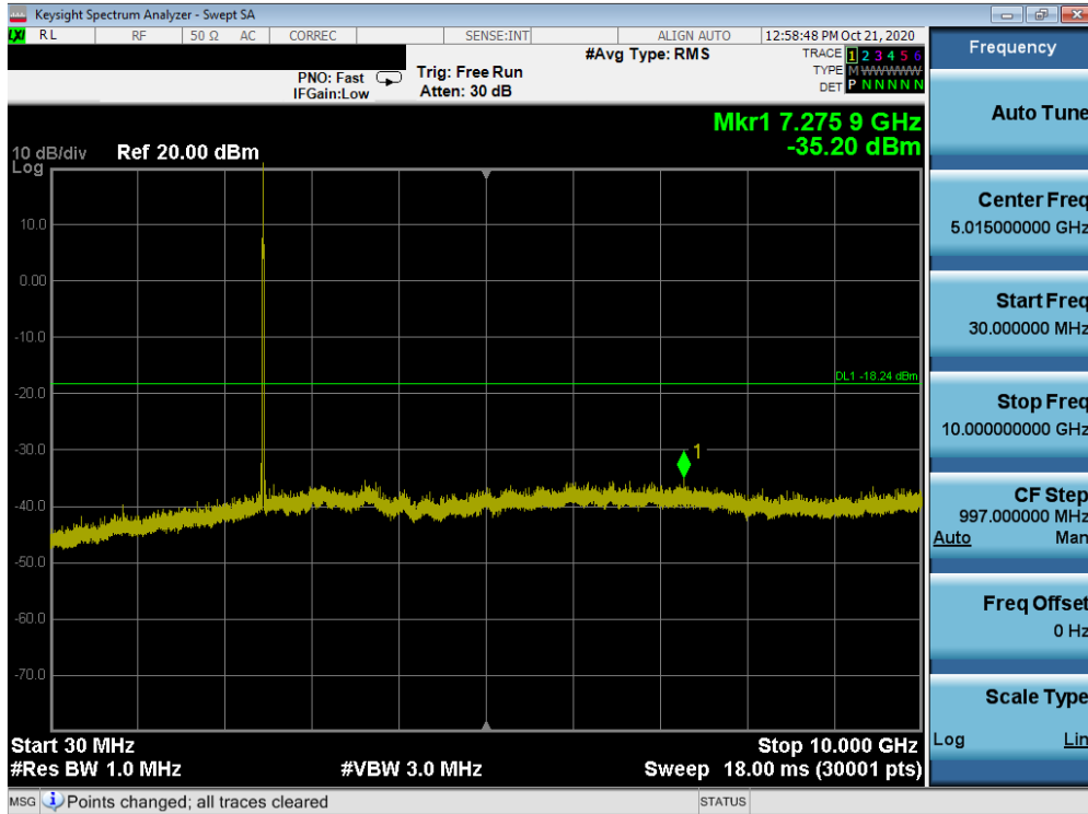
Plot 7-49. Conducted Spurious Plot ANT1 (802.11ax OFDMA – 26 Tones – Ch. 11)
