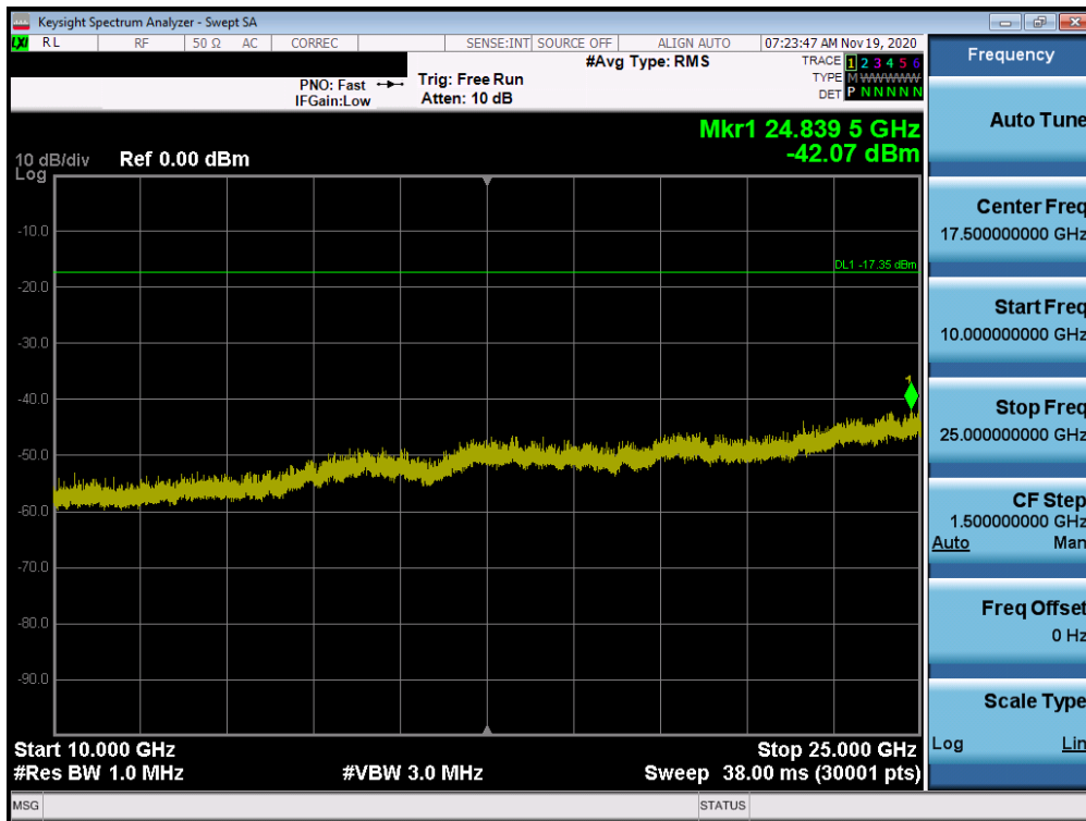
Plot 7-60. Conducted Spurious Plot ANT2 (802.11ax OFDMA – 26 Tones – Ch. 6)
