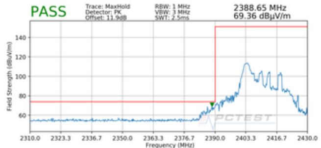
Plot 7-78. Radiated Restricted Lower Band Edge Measurement MIMO (Peak – 26Tones)
