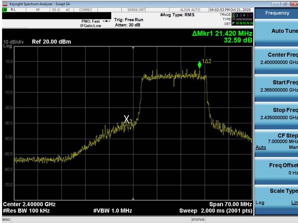
Plot 7-39. Band Edge Plot ANT2 (802.11ax OFDMA – 242 Tones – Ch. 1)
