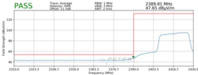
Plot 7-103. Radiated Restricted Lower Band Edge Measurement MIMO (Average – 242 Tones)
