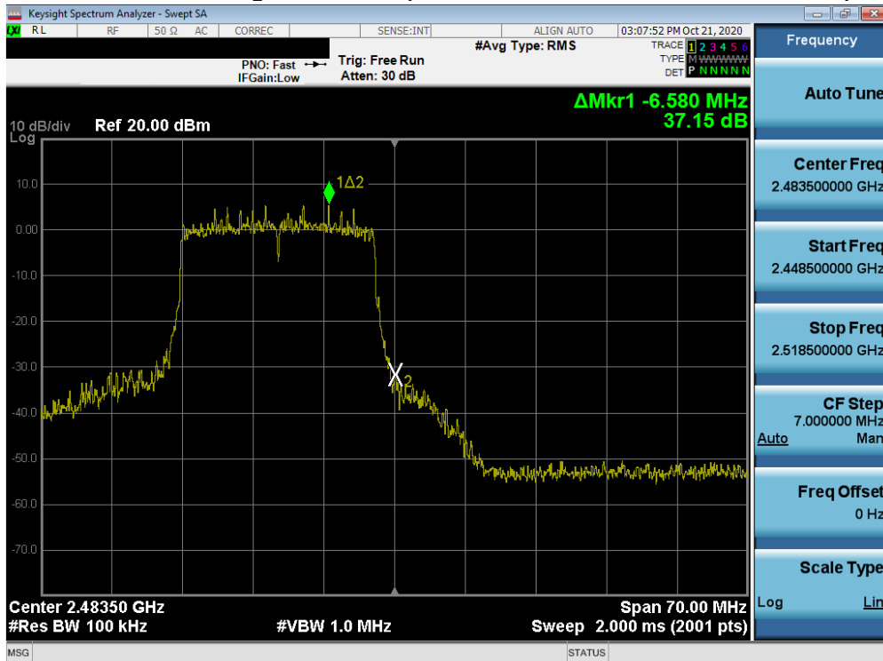
Plot 7-44. Band Edge Plot ANT2 (802.11ax OFDMA – 242 Tones – Ch. 13)
