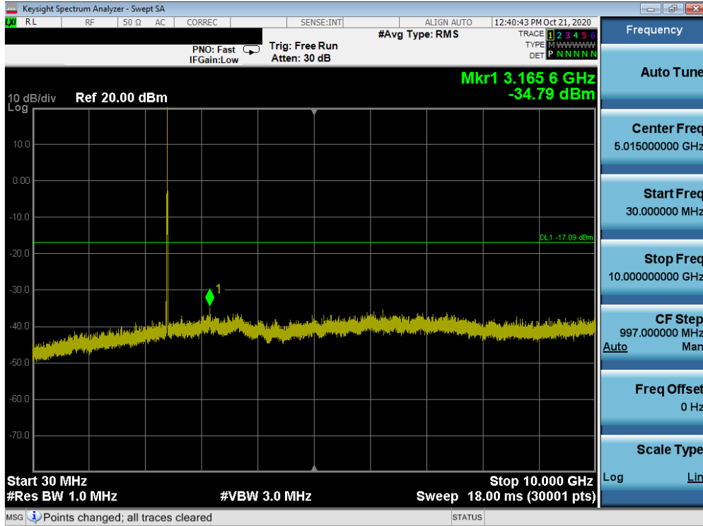
Plot 7-45. Conducted Spurious Plot ANT1 (802.11ax OFDMA – 26 Tones – Ch. 1)
