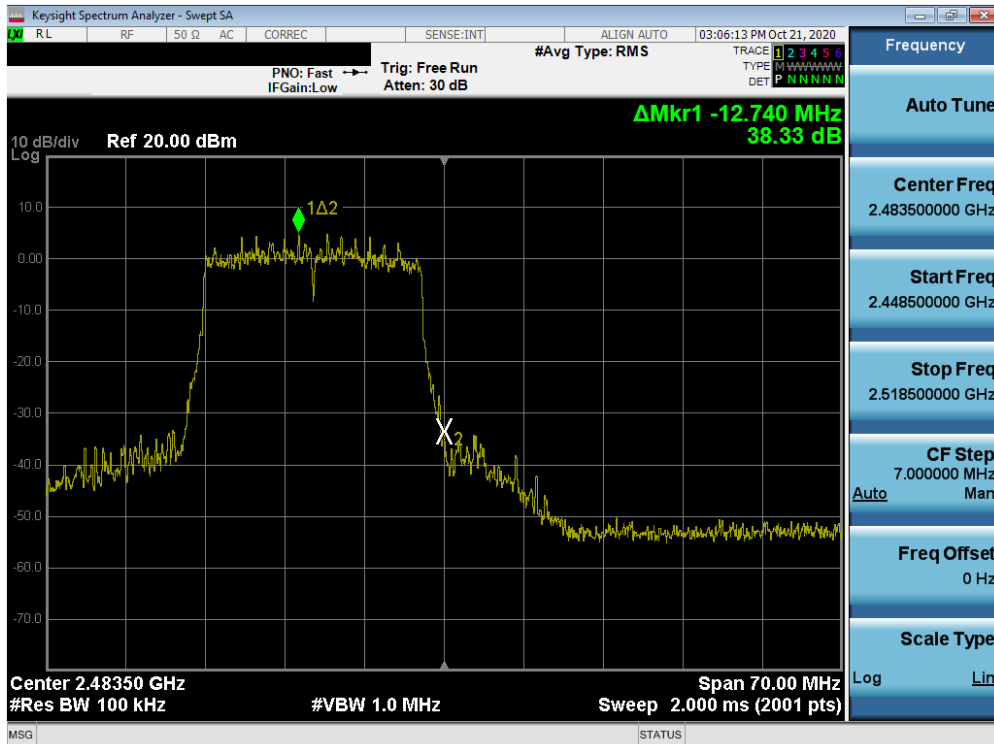
Plot 7-34. Band Edge Plot ANT1 (802.11ax OFDMA – 242 Tones – Ch. 13)
