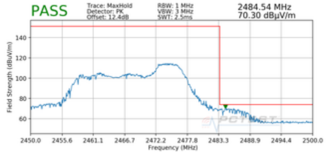
Plot 7-90. Radiated Restricted Upper Band Edge Measurement MIMO (Peak – 52 Tones)
