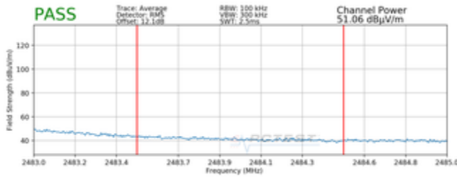
Plot 7-111. Radiated Restricted Upper Band Edge Measurement MIMO (Average – 242 Tones)
