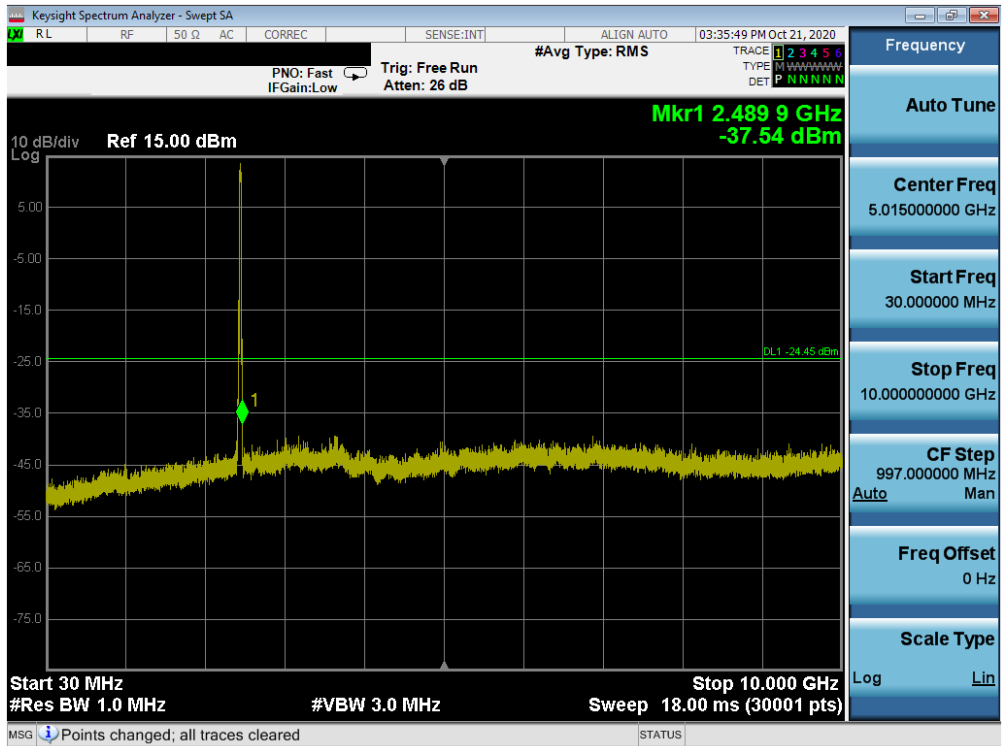
Plot 7-67. Conducted Spurious Plot ANT2 (802.11ax OFDMA – 242 Tones – Ch. 11)
