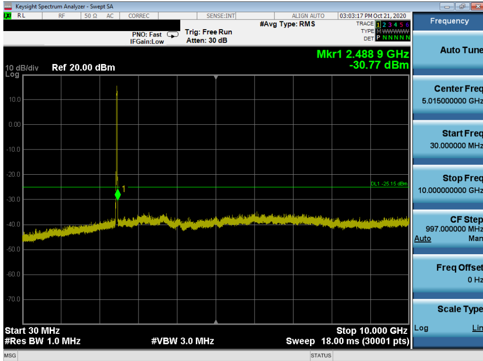
Plot 7-55. Conducted Spurious Plot ANT1 (802.11ax OFDMA – 242 Tones – Ch. 11)
