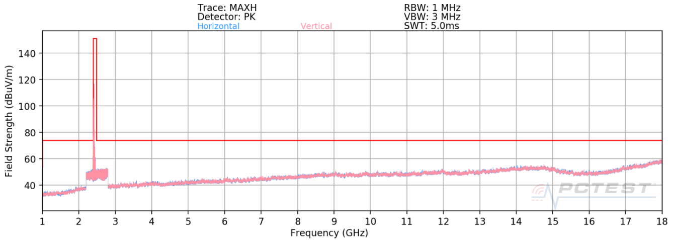
Plot 7-69. Radiated Spurious Plot above 1GHz MIMO (802.11ax OFDMA – 26 Tones – Ch. 1)
