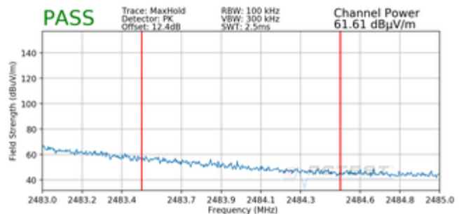
Plot 7-84. Radiated Restricted Upper Band Edge Measurement MIMO (Peak – 26Tones)
