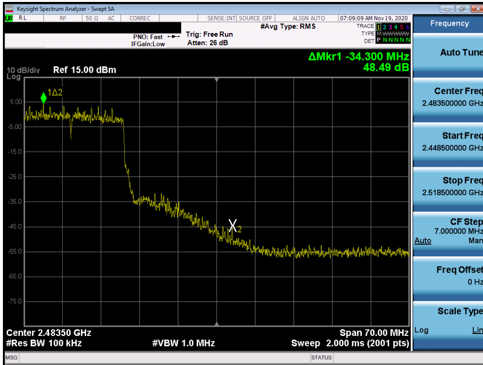
Plot 7-31. Band Edge Plot ANT1 (802.11ax OFDMA – 242 Tones – Ch. 10)
