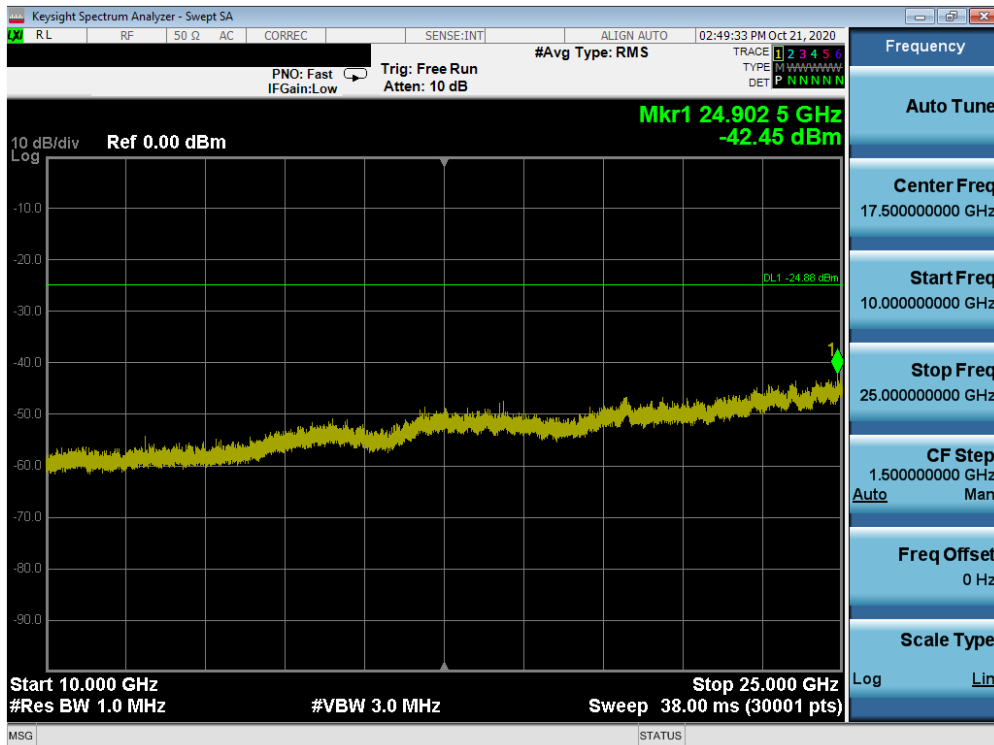
Plot 7-52. Conducted Spurious Plot ANT1 (802.11ax OFDMA – 242 Tones – Ch. 1)
