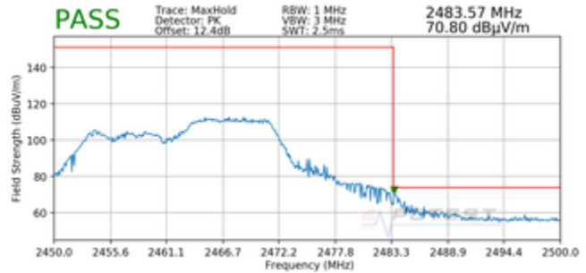
Plot 7-96. Radiated Restricted Upper Band Edge Measurement MIMO (Peak – 106 Tones)
