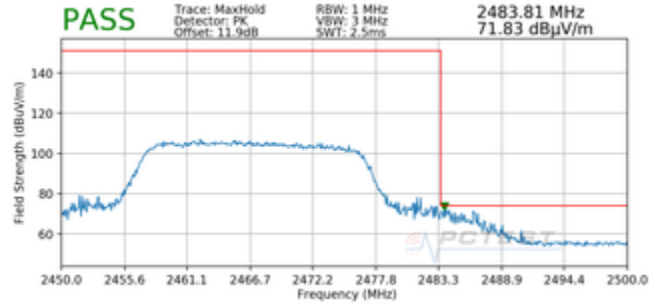
Plot 7-114. Radiated Restricted Upper Band Edge Measurement MIMO (Peak – 242 Tones) – WCP
