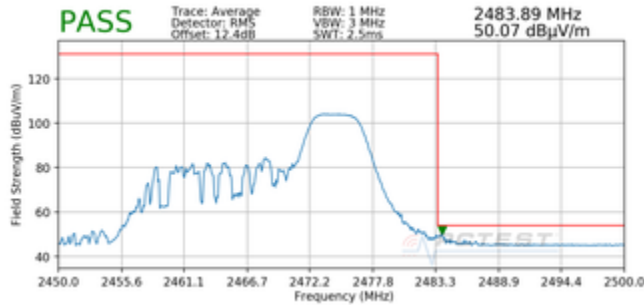
Plot 7-89. Radiated Restricted Upper Band Edge Measurement MIMO (Average – 52 Tones)
