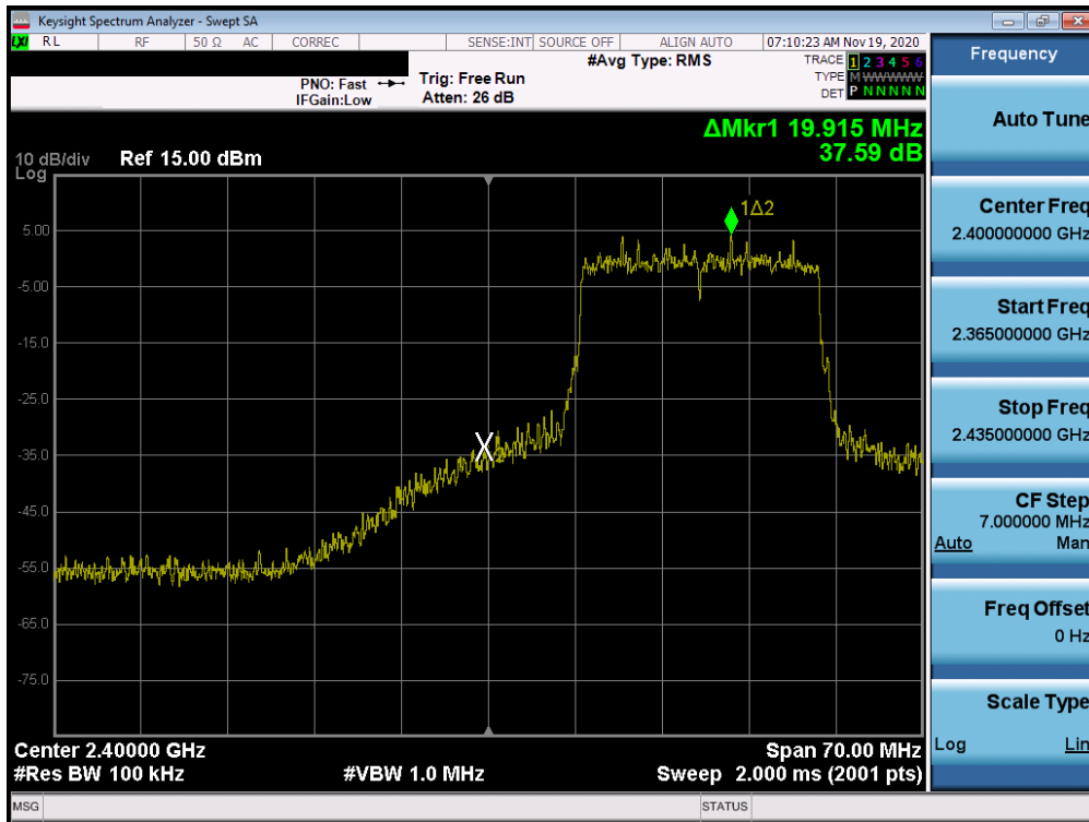
Plot 7-30. Band Edge Plot ANT1 (802.11ax OFDMA – 242 Tones – Ch. 2)
