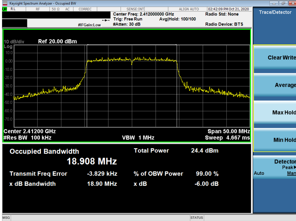
Plot 7-4. 6dB Bandwidth Plot ANT1 (802.11ax OFDMA – 242 Tones – Ch. 1)
