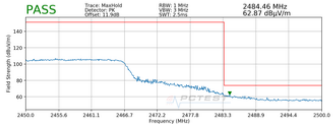
Plot 7-106. Radiated Restricted Upper Band Edge Measurement MIMO (Peak – 242 Tones)
