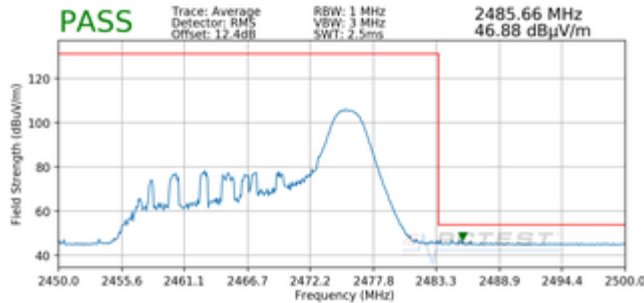
Plot 7-81. Radiated Restricted Upper Band Edge Measurement MIMO (Average – 26Tones)
