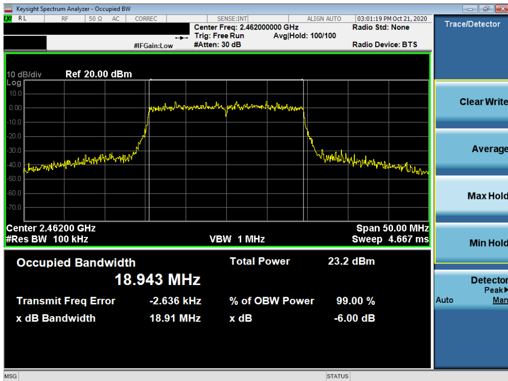
Plot 7-6. 6dB Bandwidth Plot ANT1 (802.11ax OFDMA – 242 Tones – Ch. 11)
