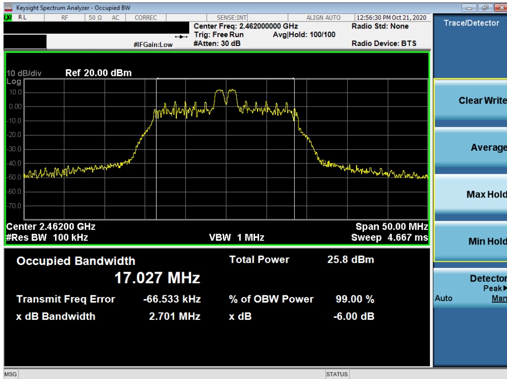
Plot 7-3. 6dB Bandwidth Plot ANT1 (802.11ax OFDMA – 26 Tones – Ch. 11)
