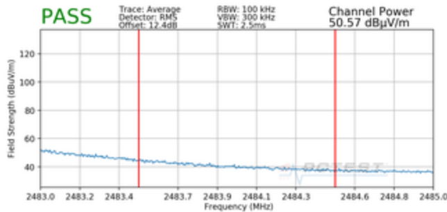
Plot 7-91. Radiated Restricted Upper Band Edge Measurement MIMO (Average – 52 Tones)
