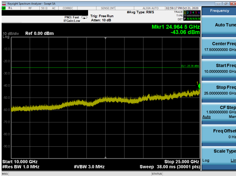
Plot 7-54. Conducted Spurious Plot ANT1 (802.11ax OFDMA – 242 Tones – Ch. 6)
