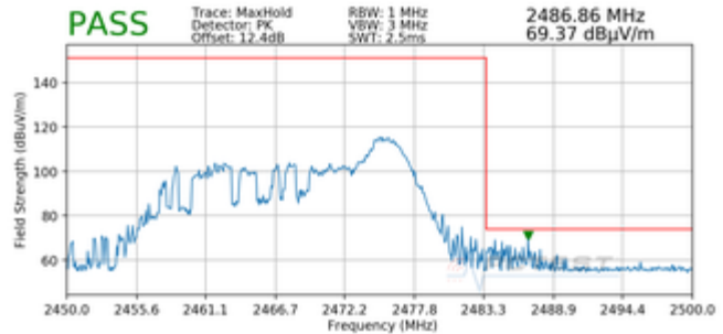
Plot 7-82. Radiated Restricted Upper Band Edge Measurement MIMO (Peak – 26Tones)
