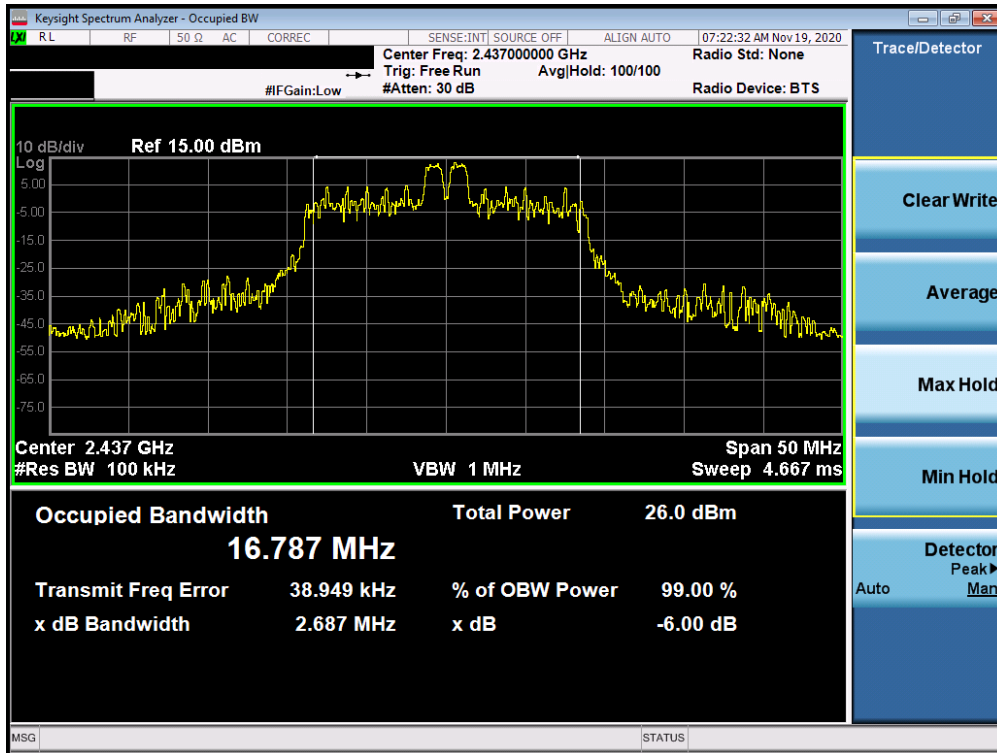
Plot 7-8. 6dB Bandwidth Plot ANT1 (802.11ax OFDMA – 26 Tones – Ch. 6)
