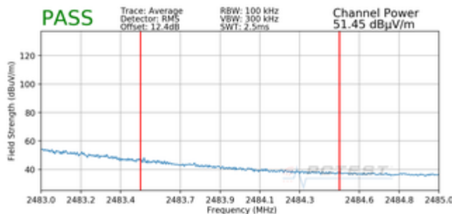
Plot 7-83. Radiated Restricted Upper Band Edge Measurement MIMO (Average – 26Tones)
