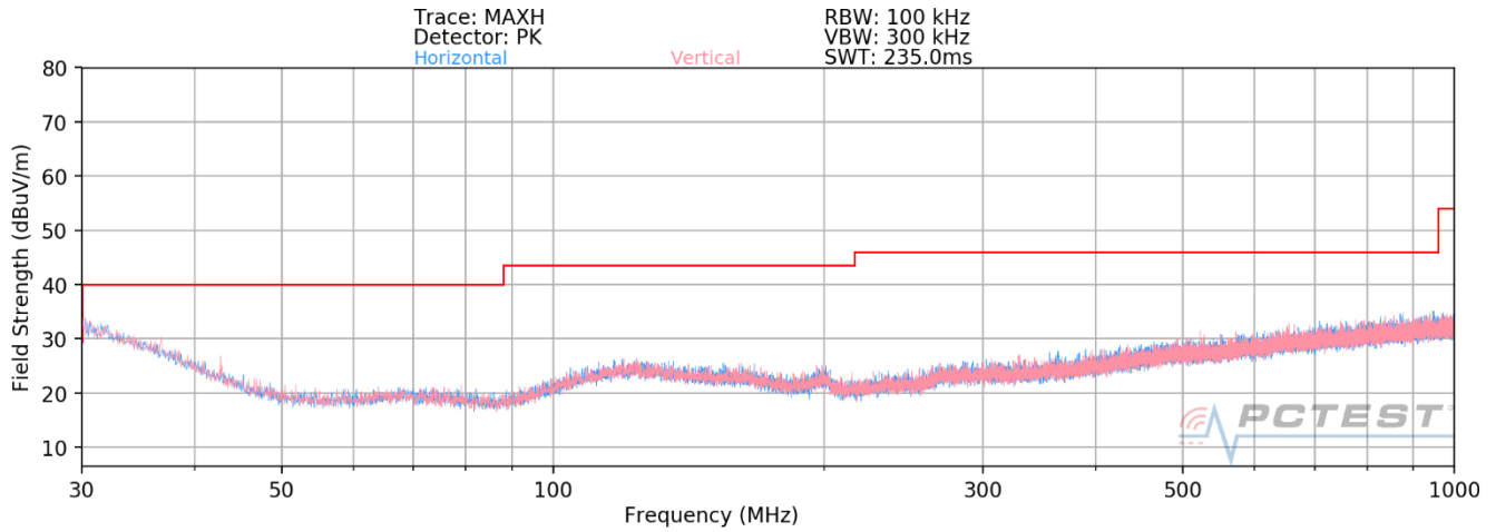
Plot 7-115. Radiated Spurious Plot below 1GHz MIMO (26 Tones)
