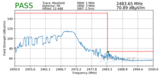
Plot 7-88. Radiated Restricted Upper Band Edge Measurement MIMO (Peak – 52 Tones)
