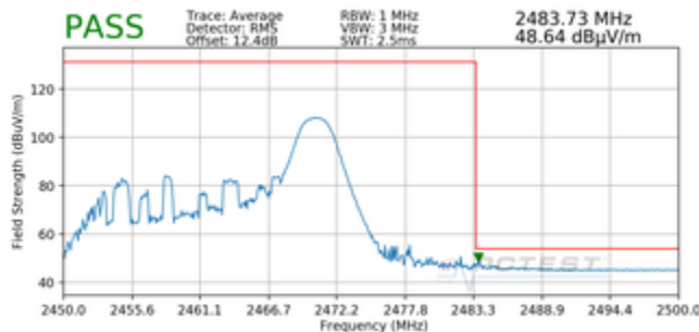
Plot 7-79. Radiated Restricted Upper Band Edge Measurement MIMO (Average – 26Tones)
