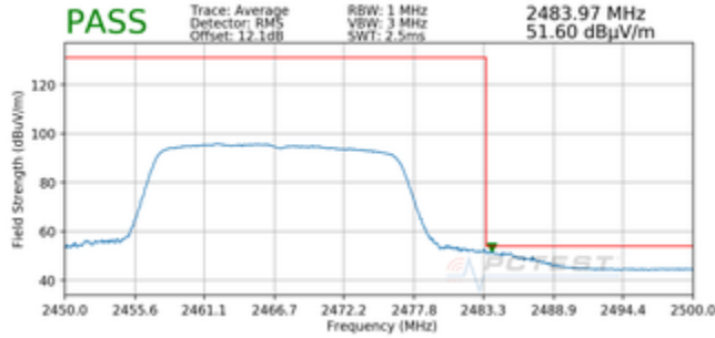
Plot 7-113. Radiated Restricted Upper Band Edge Measurement MIMO (Average – 242 Tones) – WCP
