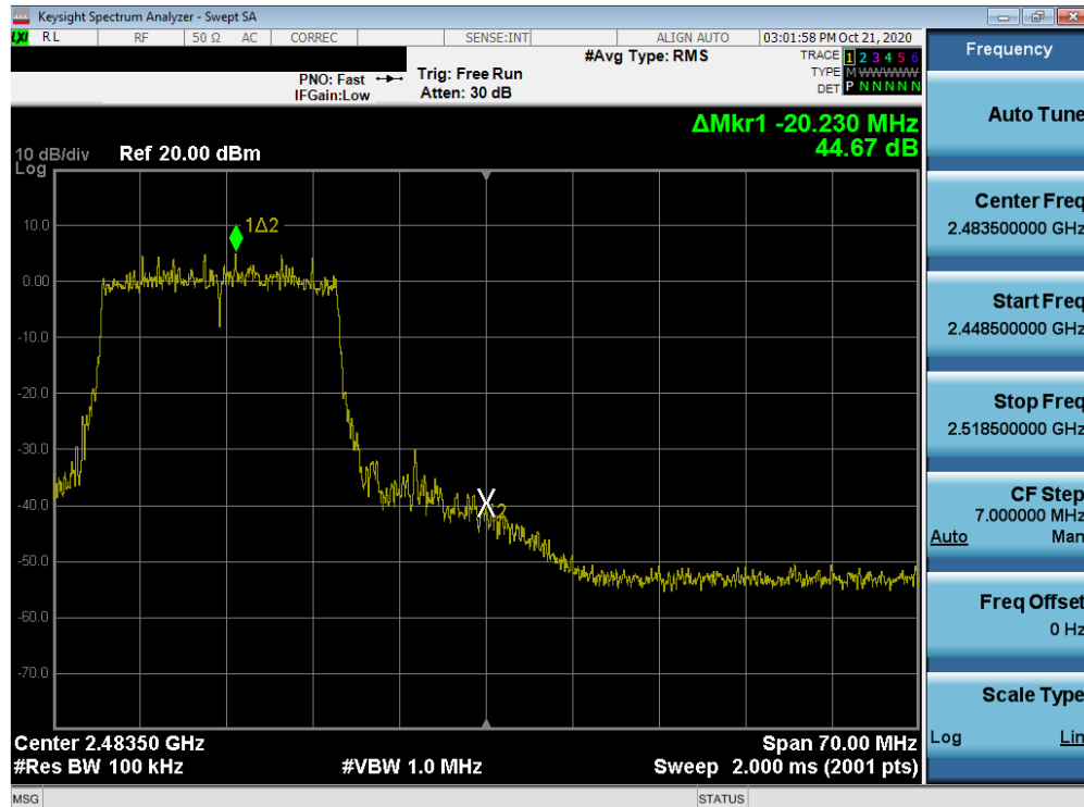
Plot 7-32. Band Edge Plot ANT1 (802.11ax OFDMA – 242 Tones – Ch. 11)
