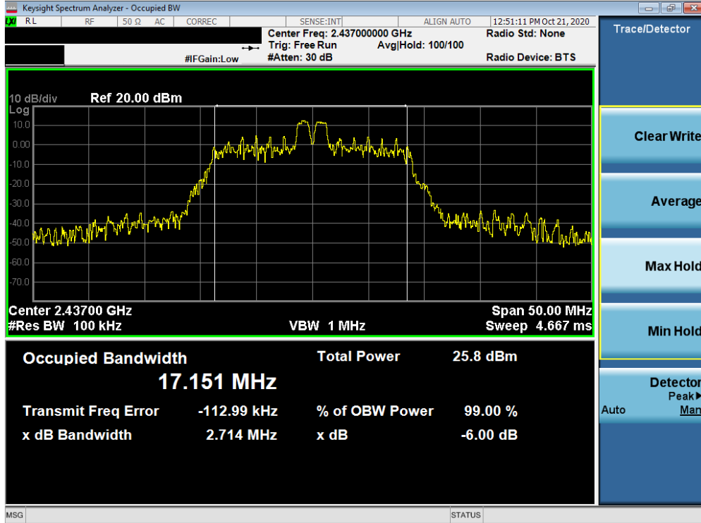
Plot 7-2. 6dB Bandwidth Plot ANT1 (802.11ax OFDMA – 26 Tones – Ch. 6)
