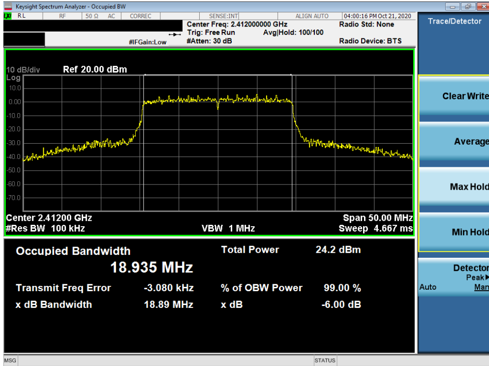
Plot 7-10. 6dB Bandwidth Plot ANT1 (802.11ax OFDMA – 242 Tones – Ch. 1)
