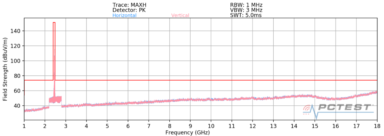
Plot 7-71. Radiated Spurious Plot above 1GHz MIMO (802.11ax OFDMA – 26 Tones – Ch. 11)
