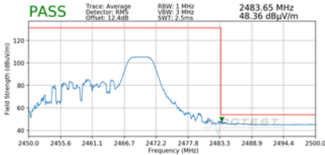
Plot 7-87. Radiated Restricted Upper Band Edge Measurement MIMO (Average – 52 Tones)
