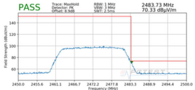
Plot 7-112. Radiated Restricted Upper Band Edge Measurement MIMO (Peak – 242 Tones)
