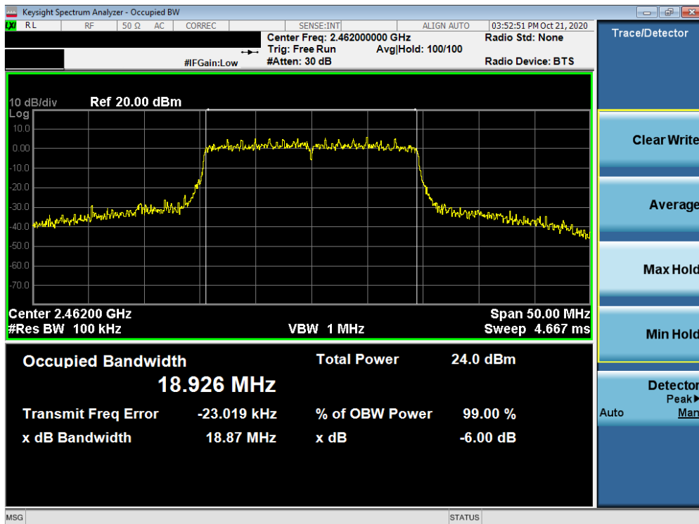
Plot 7-12. 6dB Bandwidth Plot ANT1 (802.11ax OFDMA – 242 Tones – Ch. 11)
