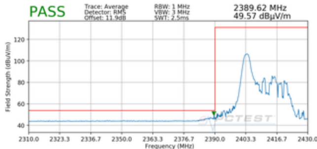
Plot 7-77. Radiated Restricted Lower Band Edge Measurement MIMO (Average – 26 Tones)
