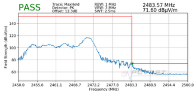
Plot 7-80. Radiated Restricted Upper Band Edge Measurement MIMO (Peak – 26Tones)
