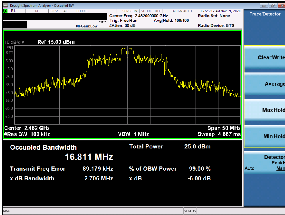
Plot 7-9. 6dB Bandwidth Plot ANT1 (802.11ax OFDMA – 26 Tones – Ch. 11)
