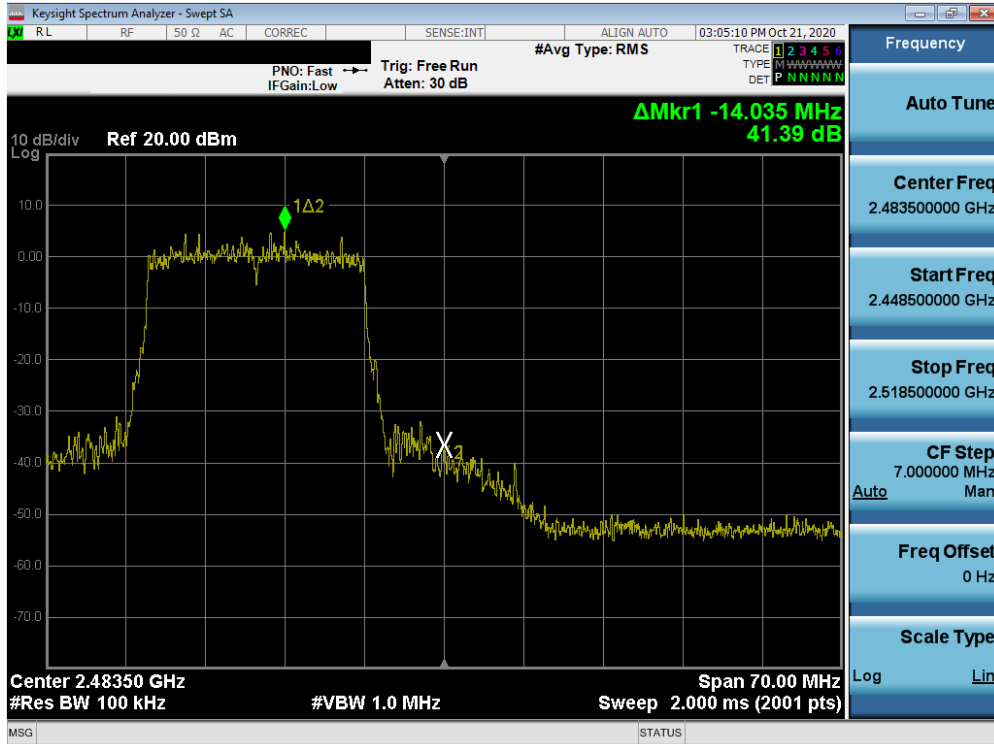
Plot 7-33. Band Edge Plot ANT1 (802.11ax OFDMA – 242 Tones – Ch. 12)
