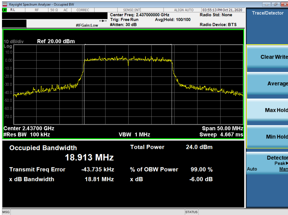
Plot 7-11. 6dB Bandwidth Plot ANT1 (802.11ax OFDMA – 242 Tones – Ch. 6)
