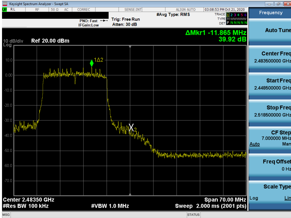
Plot 7-43. Band Edge Plot ANT2 (802.11ax OFDMA – 242 Tones – Ch. 12)
