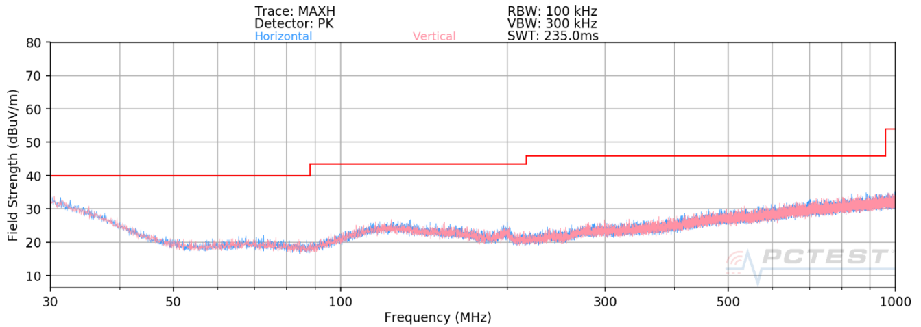
Plot 7-116. Radiated Spurious Plot below 1GHz MIMO (242 Tones)
