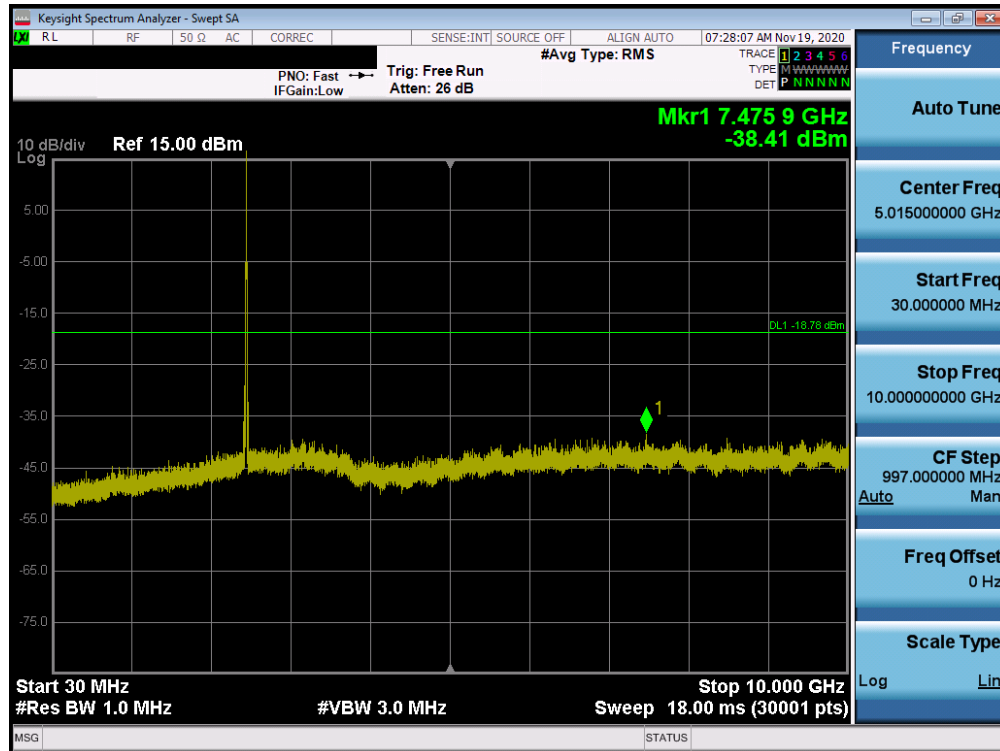
Plot 7-61. Conducted Spurious Plot ANT2 (802.11ax OFDMA – 26 Tones – Ch. 11)
