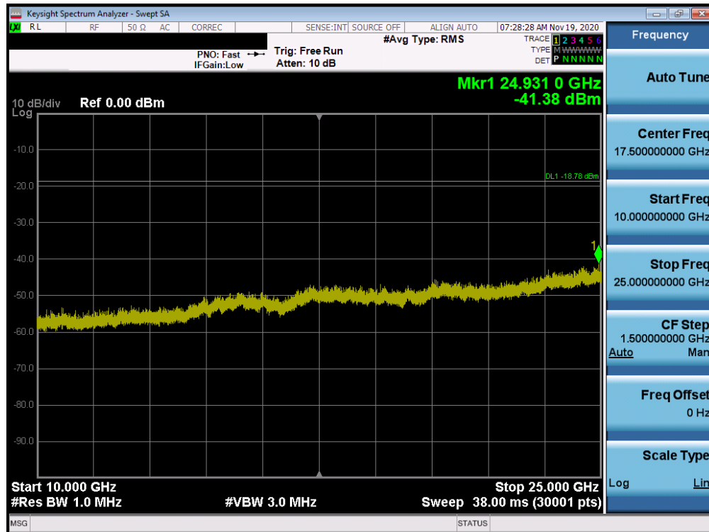
Plot 7-62. Conducted Spurious Plot ANT2 (802.11ax OFDMA – 26 Tones – Ch. 11)
