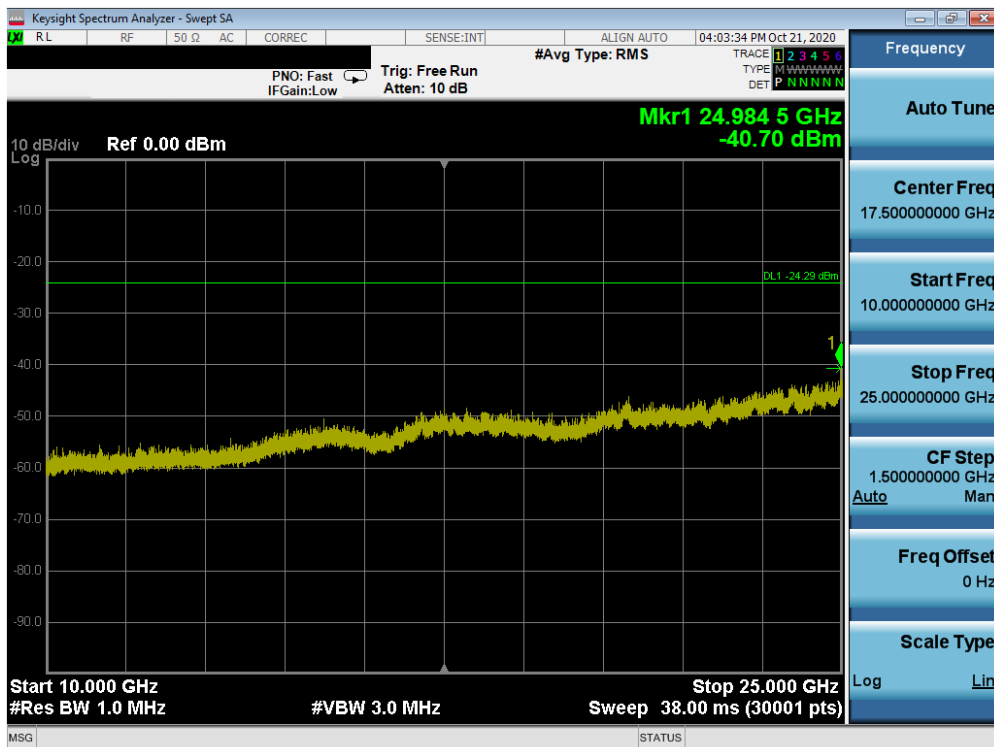
Plot 7-64. Conducted Spurious Plot ANT2 (802.11ax OFDMA – 242 Tones – Ch. 1)
