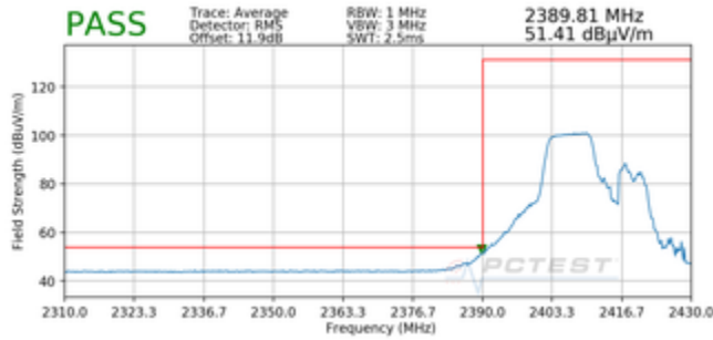
Plot 7-93. Radiated Restricted Lower Band Edge Measurement MIMO (Average – 106 Tones)
