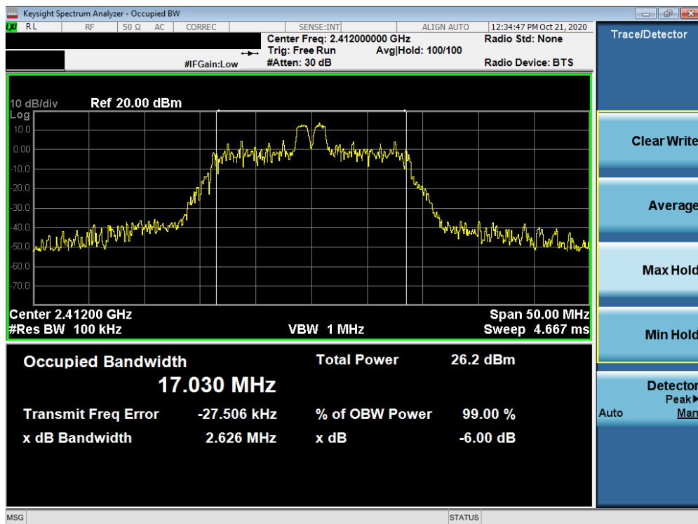
Plot 7-1. 6dB Bandwidth Plot ANT1 (802.11ax OFDMA – 26 Tones – Ch. 1)
