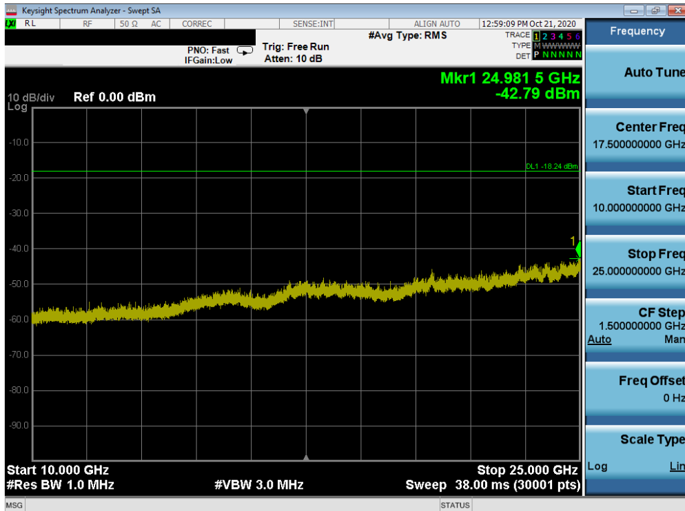
Plot 7-50. Conducted Spurious Plot ANT1 (802.11ax OFDMA – 26 Tones – Ch. 11)
