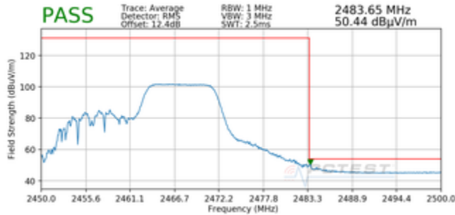
Plot 7-95. Radiated Restricted Upper Band Edge Measurement MIMO (Average – 106 Tones)
