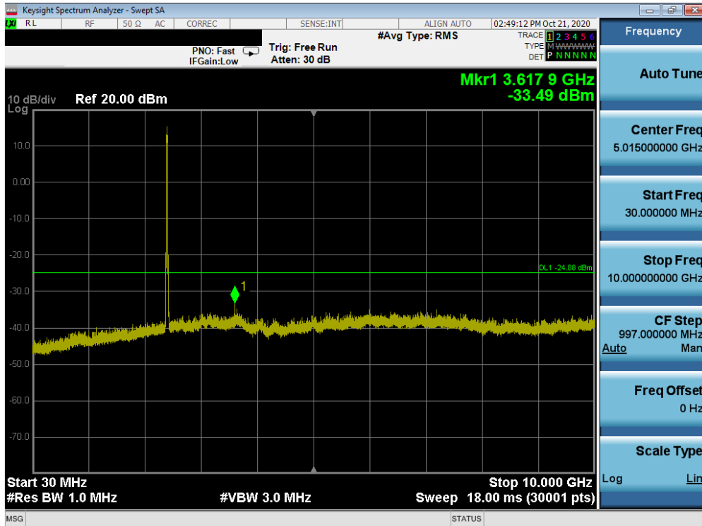
Plot 7-51. Conducted Spurious Plot ANT1 (802.11ax OFDMA – 242 Tones – Ch. 1)
