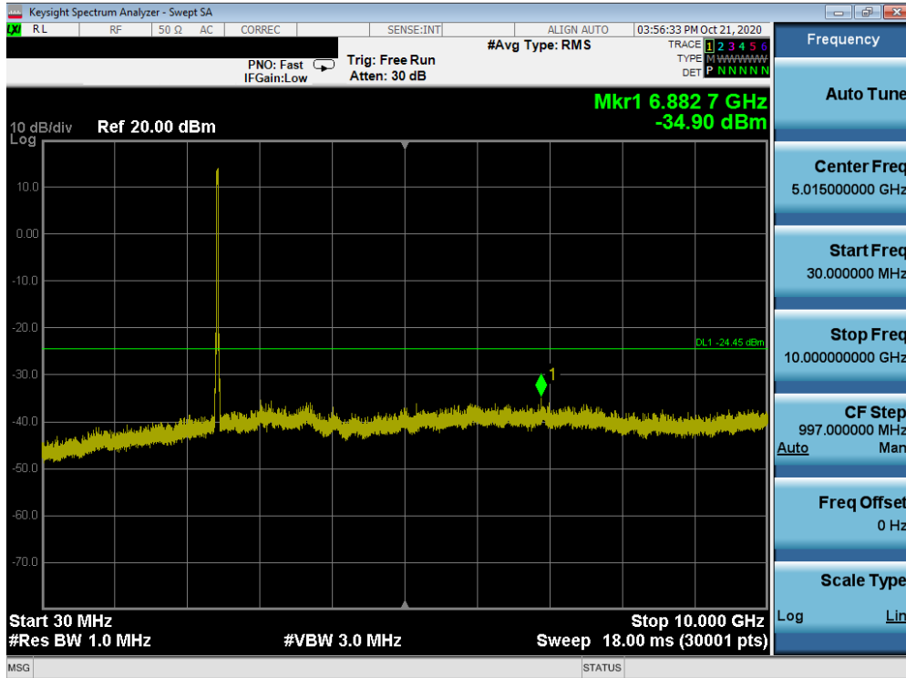
Plot 7-65. Conducted Spurious Plot ANT2 (802.11ax OFDMA – 242 Tones – Ch. 6)
