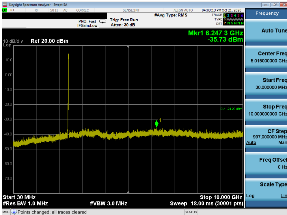
Plot 7-63. Conducted Spurious Plot ANT2 (802.11ax OFDMA – 242 Tones – Ch. 1)
