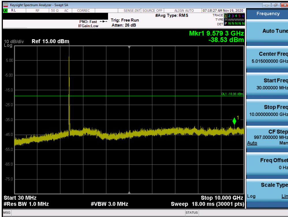
Plot 7-57. Conducted Spurious Plot ANT2 (802.11ax OFDMA – 26 Tones – Ch. 1)
