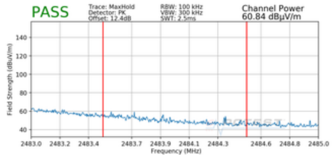
Plot 7-92. Radiated Restricted Upper Band Edge Measurement MIMO (Peak – 52 Tones)
