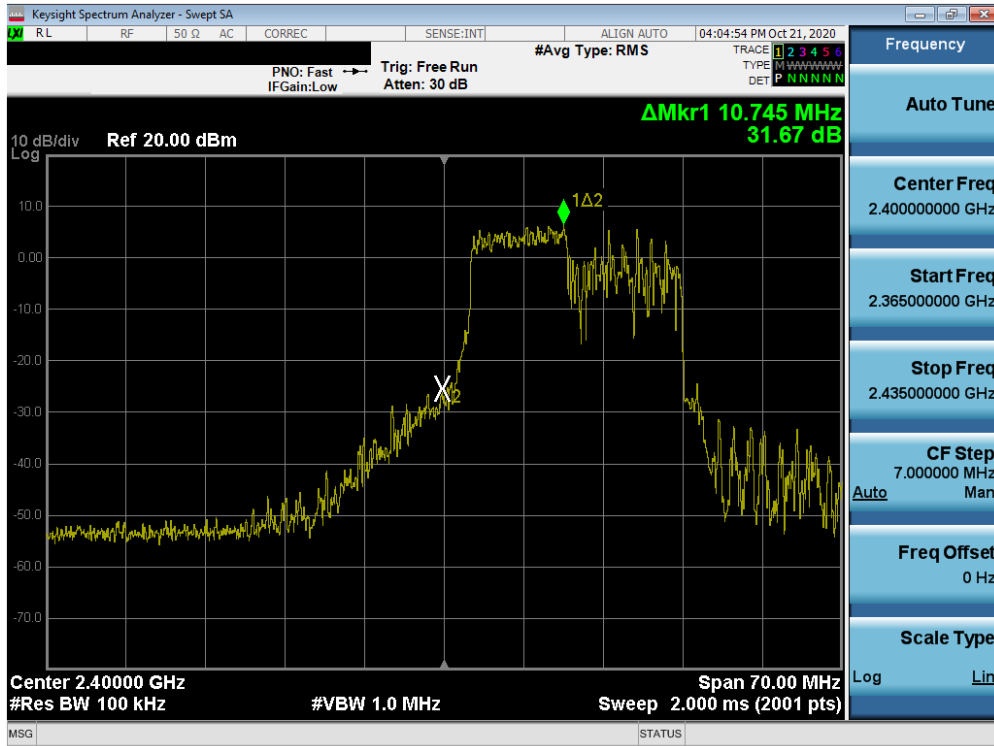
Plot 7-35. Band Edge Plot ANT2 (802.11ax OFDMA – 106 Tones – Ch. 1)
