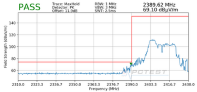
Plot 7-86. Radiated Restricted Lower Band Edge Measurement MIMO (Peak – 52 Tones)
