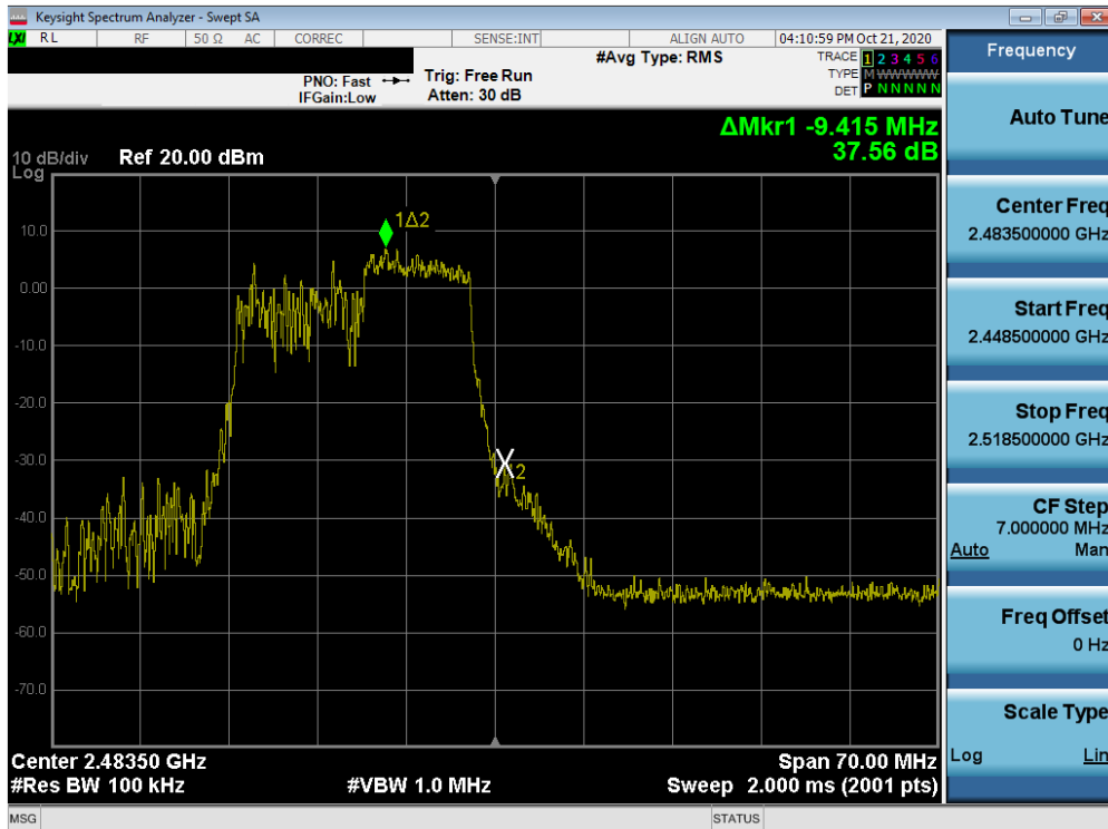
Plot 7-38. Band Edge Plot ANT2 (802.11ax OFDMA – 106 Tones – Ch. 13)
