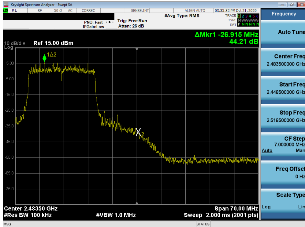
Plot 7-42. Band Edge Plot ANT2 (802.11ax OFDMA - 242 Tones - Ch. 11)
