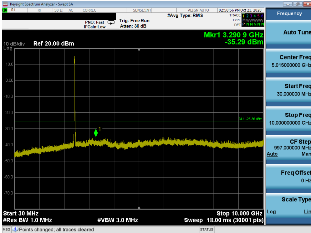
Plot 7-53. Conducted Spurious Plot ANT1 (802.11ax OFDMA – 242 Tones – Ch. 6)
