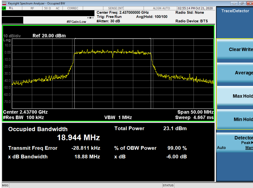
Plot 7-5. 6dB Bandwidth Plot ANT1 (802.11ax OFDMA – 242 Tones – Ch. 6)
