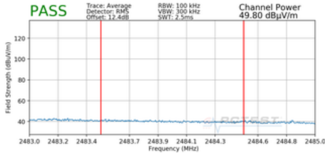
Plot 7-97. Radiated Restricted Upper Band Edge Measurement MIMO (Average – 106 Tones)
