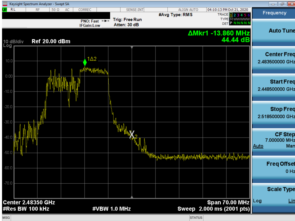
Plot 7-37. Band Edge Plot ANT2 (802.11ax OFDMA – 106 Tones – Ch. 12)
