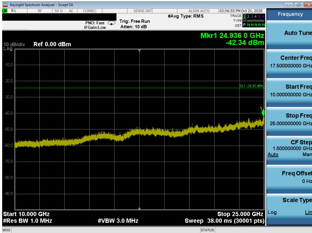
Plot 7-66. Conducted Spurious Plot ANT2 (802.11ax OFDMA – 242 Tones – Ch. 6)
