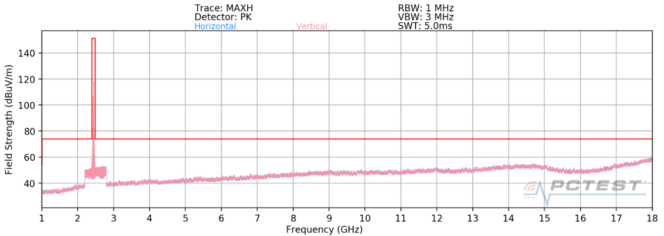
Plot 7-70. Radiated Spurious Plot above 1GHz MIMO (802.11ax OFDMA – 26 Tones – Ch. 6)
