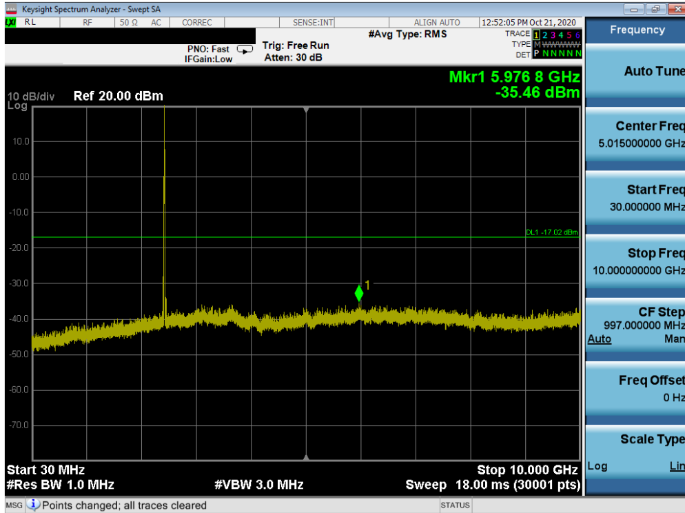
Plot 7-47. Conducted Spurious Plot ANT1 (802.11ax OFDMA – 26 Tones – Ch. 6)
