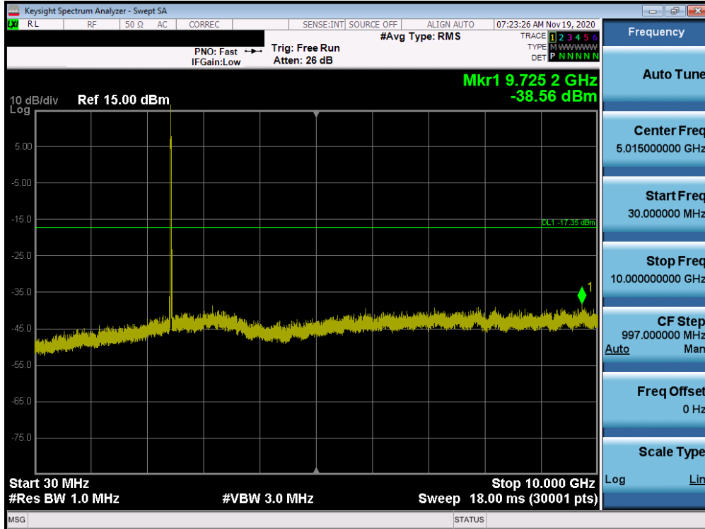
Plot 7-59. Conducted Spurious Plot ANT2 (802.11ax OFDMA – 26 Tones – Ch. 6)
