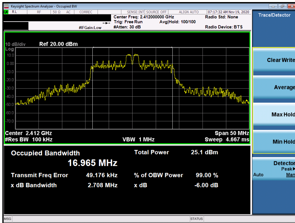
Plot 7-7. 6dB Bandwidth Plot ANT1 (802.11ax OFDMA – 26 Tones – Ch. 1)
