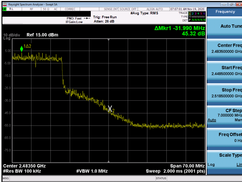
Plot 7-41. Band Edge Plot ANT2 (802.11ax OFDMA - 242 Tones - Ch. 10)
