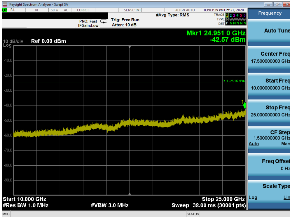
Plot 7-56. Conducted Spurious Plot ANT1 (802.11ax OFDMA – 242 Tones – Ch. 11)
