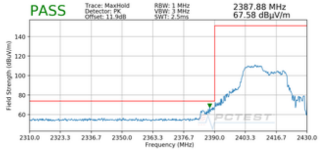
Plot 7-94. Radiated Restricted Lower Band Edge Measurement MIMO (Peak – 106 Tones)
