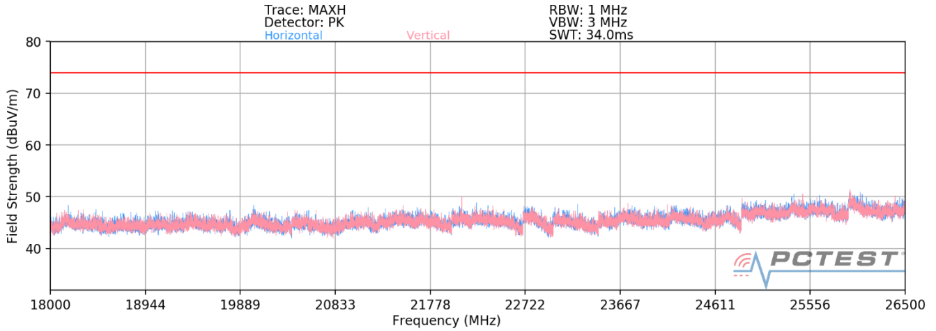
Plot 7-75. Radiated Spurious Plot above 18GHz MIMO (802.11ax OFDMA – 26 Tones)
