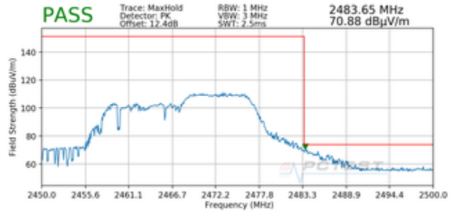
Plot 7-98. Radiated Restricted Upper Band Edge Measurement MIMO (Peak – 106 Tones)
