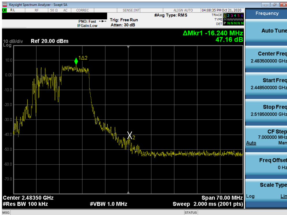
Plot 7-36. Band Edge Plot ANT2 (802.11ax OFDMA – 106 Tones – Ch. 11)
