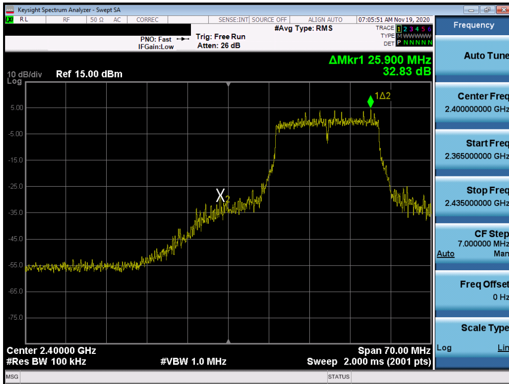
Plot 7-40. Band Edge Plot ANT2 (802.11ax OFDMA – 242 Tones – Ch. 2)
