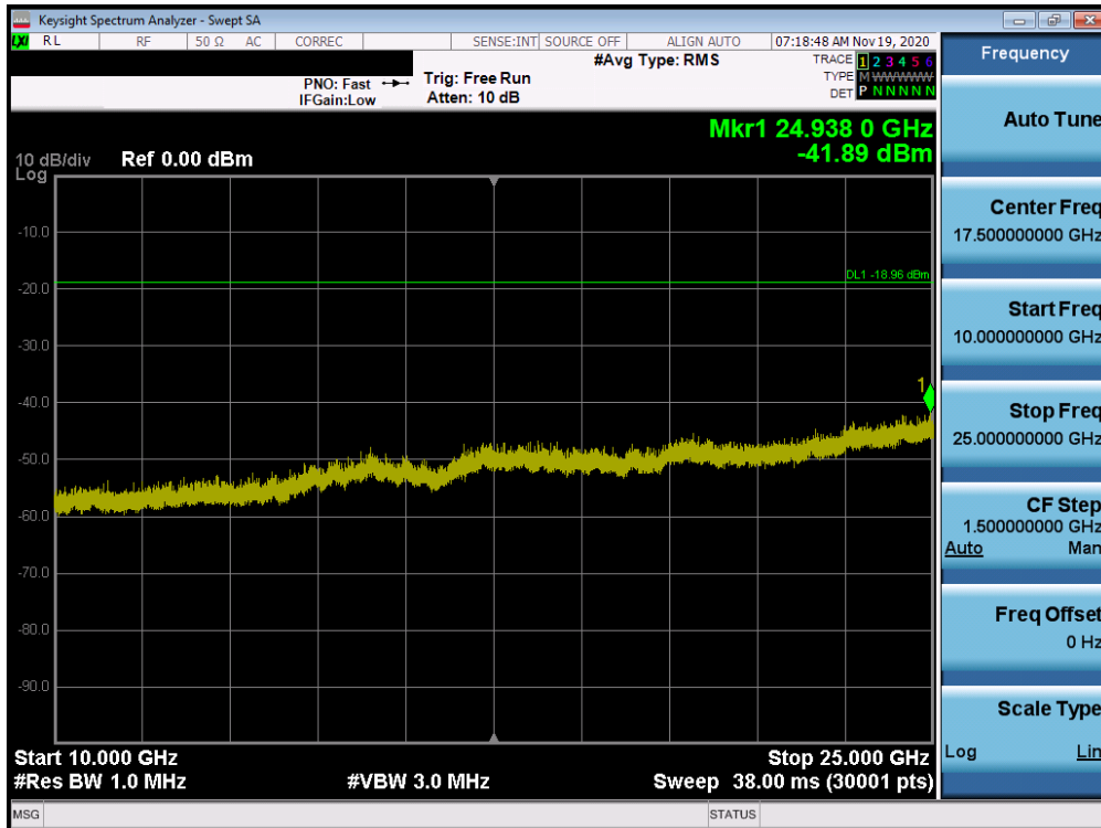
Plot 7-58. Conducted Spurious Plot ANT2 (802.11ax OFDMA – 26 Tones – Ch. 1)
