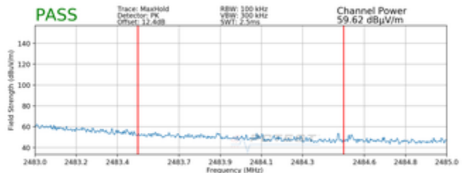
Plot 7-100. Radiated Restricted Upper Band Edge Measurement MIMO (Peak – 106 Tones)
