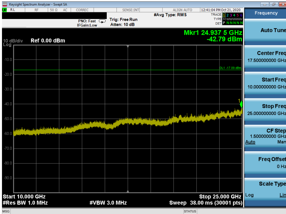
Plot 7-46. Conducted Spurious Plot ANT1 (802.11ax OFDMA – 26 Tones – Ch. 1)
