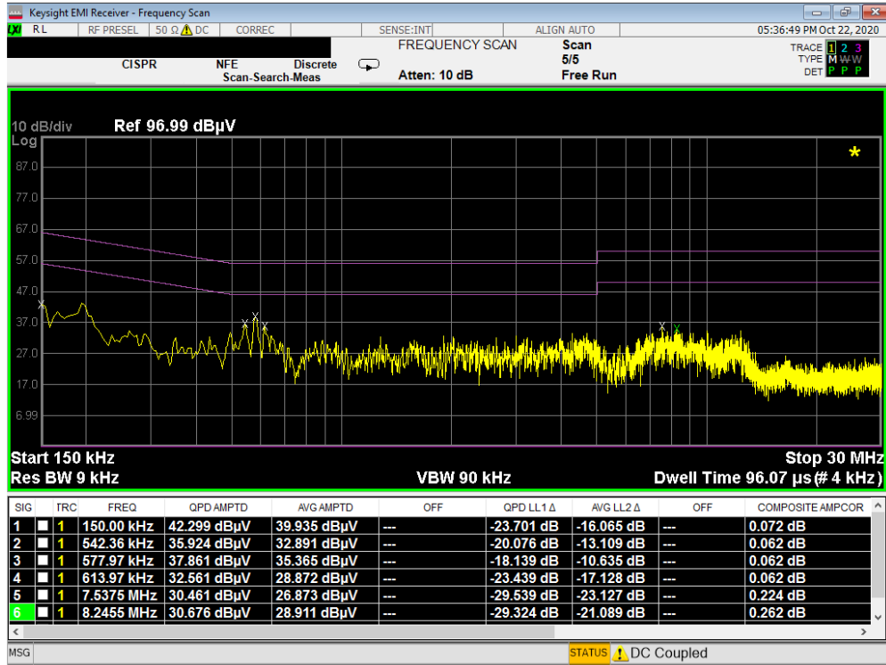
Plot 7-128. Line Conducted Plot with 802.11b (L1)
