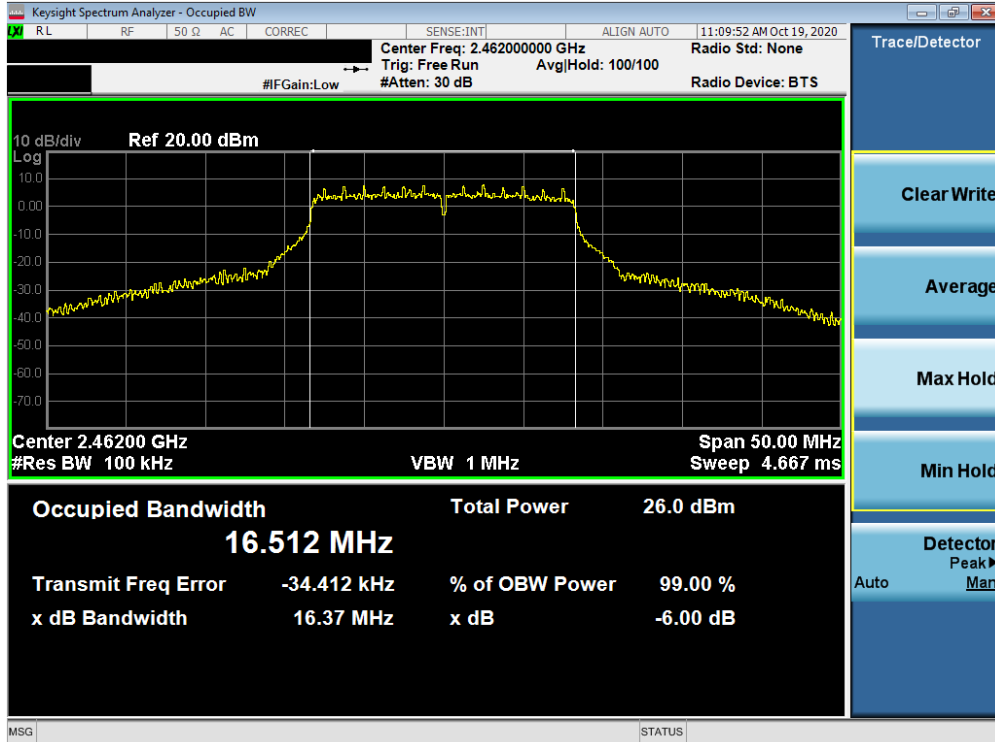
Plot 7-12. 6dB Bandwidth Plot MIMO ANT2 (802.11g – Ch. 11)
