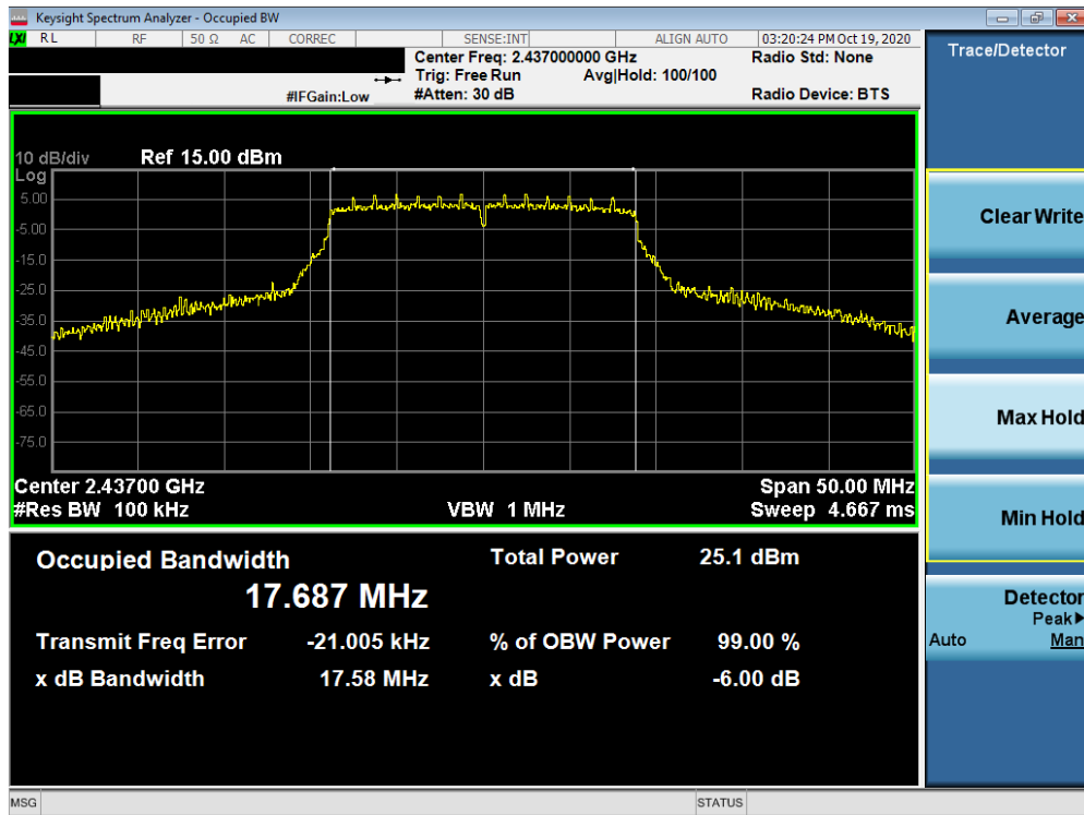
Plot 7-15. 6dB Bandwidth Plot MIMO ANT1 (802.11n (2.4GHz) – Ch. 6)
