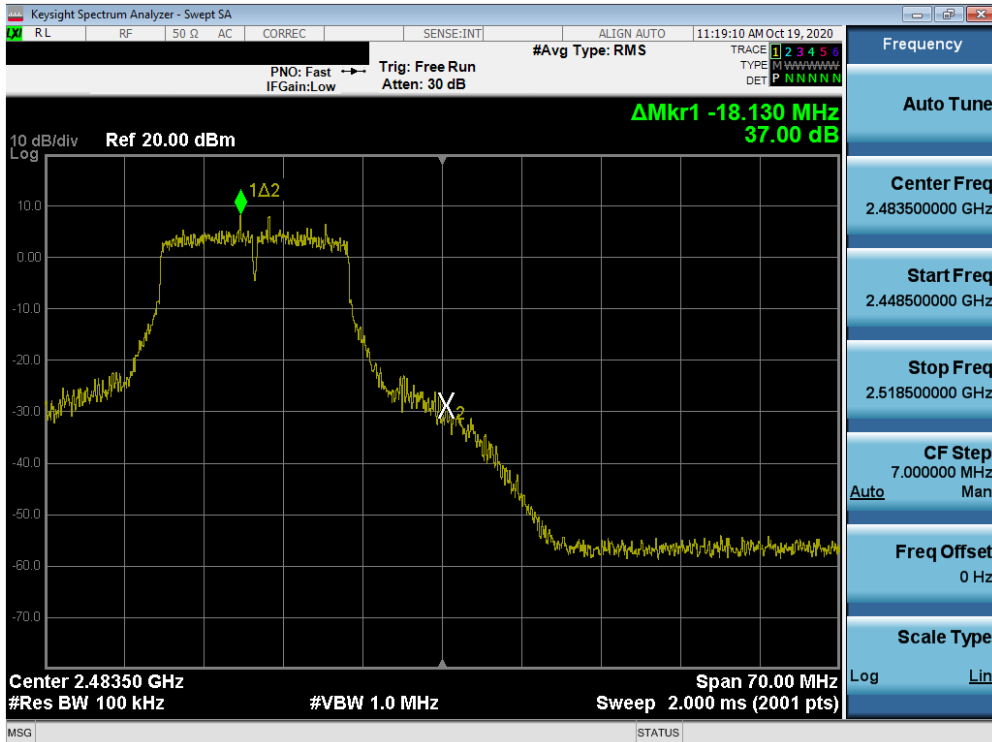
Plot 7-62. Band Edge Plot MIMO ANT2 (802.11g – Ch. 12)
