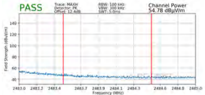
Plot 7-124. Radiated Restricted Band Edge Measurement MIMO (Peak)
