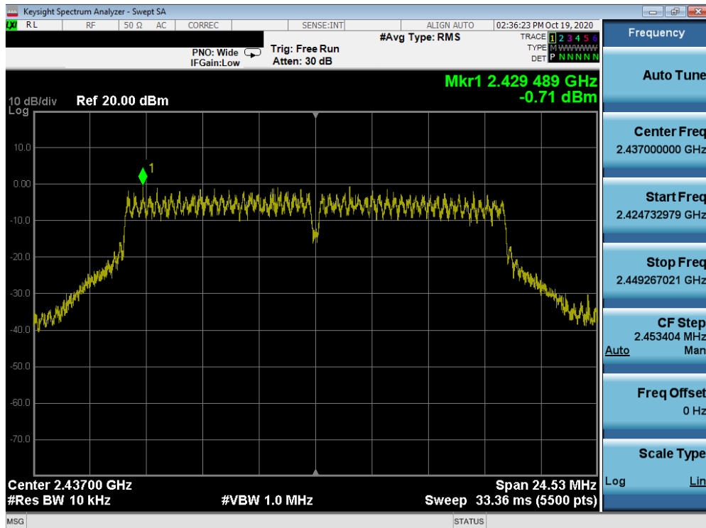
Plot 7-33. Power Spectral Density Plot MIMO ANT1 (802.11g – Ch. 6)
