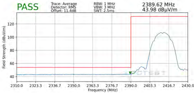
Plot 7-103. Radiated Restricted Lower Band Edge Measurement SISO ANT2 (Average)
