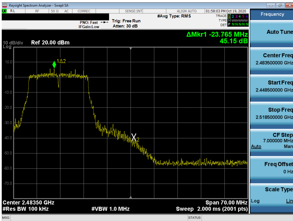
Plot 7-68. Band Edge Plot MIMO ANT2 (802.11n (2.4GHz) – Ch. 11)
