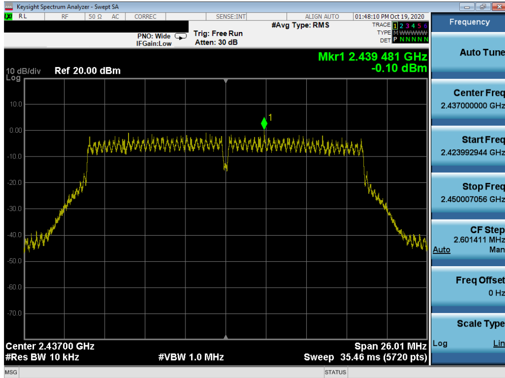
Plot 7-40. Power Spectral Density Plot MIMO ANT2 (802.11n (2.4GHz) – Ch. 6)
