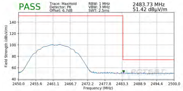
Plot 7-100. Radiated Restricted Upper Band Edge Measurement SISO ANT1 (Peak)
