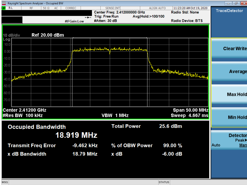
Plot 7-20. 6dB Bandwidth Plot MIMO ANT2 (802.11ax (2.4GHz) – Ch. 1)
