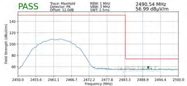
Plot 7-106. Radiated Restricted Upper Band Edge Measurement SISO ANT2 (Peak)
