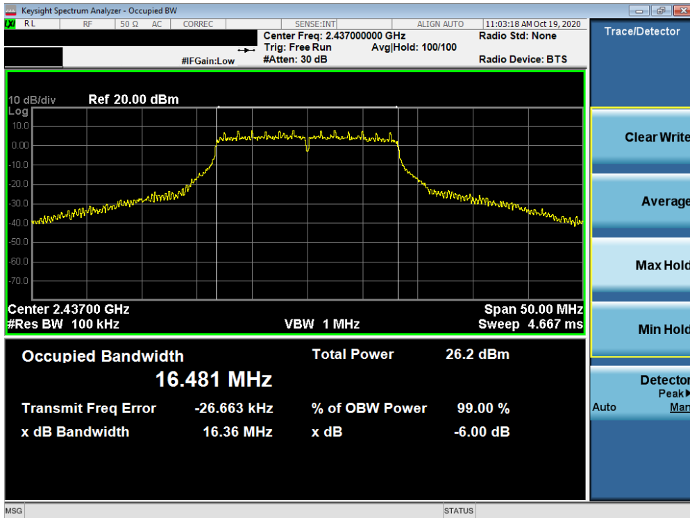
Plot 7-10. 6dB Bandwidth Plot MIMO ANT2 (802.11g – Ch. 6)
