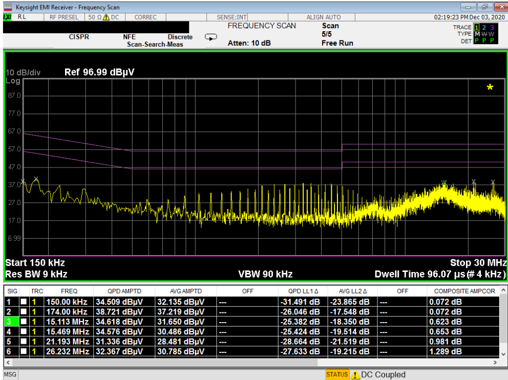
Plot 7-131. Line Conducted Plot with 802.11b with WCP (N)
