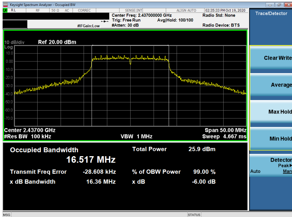
Plot 7-9. 6dB Bandwidth Plot MIMO ANT1 (802.11g – Ch. 6)
