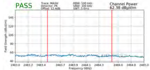
Plot 7-120. Radiated Restricted Upper Band Edge Measurement MIMO (Peak)
