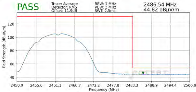
Plot 7-105. Radiated Restricted Upper Band Edge Measurement SISO ANT2 (Average)
