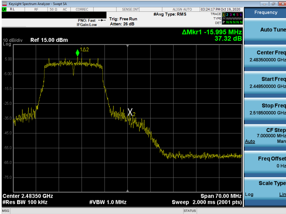
Plot 7-69. Band Edge Plot MIMO ANT1 (802.11n (2.4GHz) – Ch. 12)
