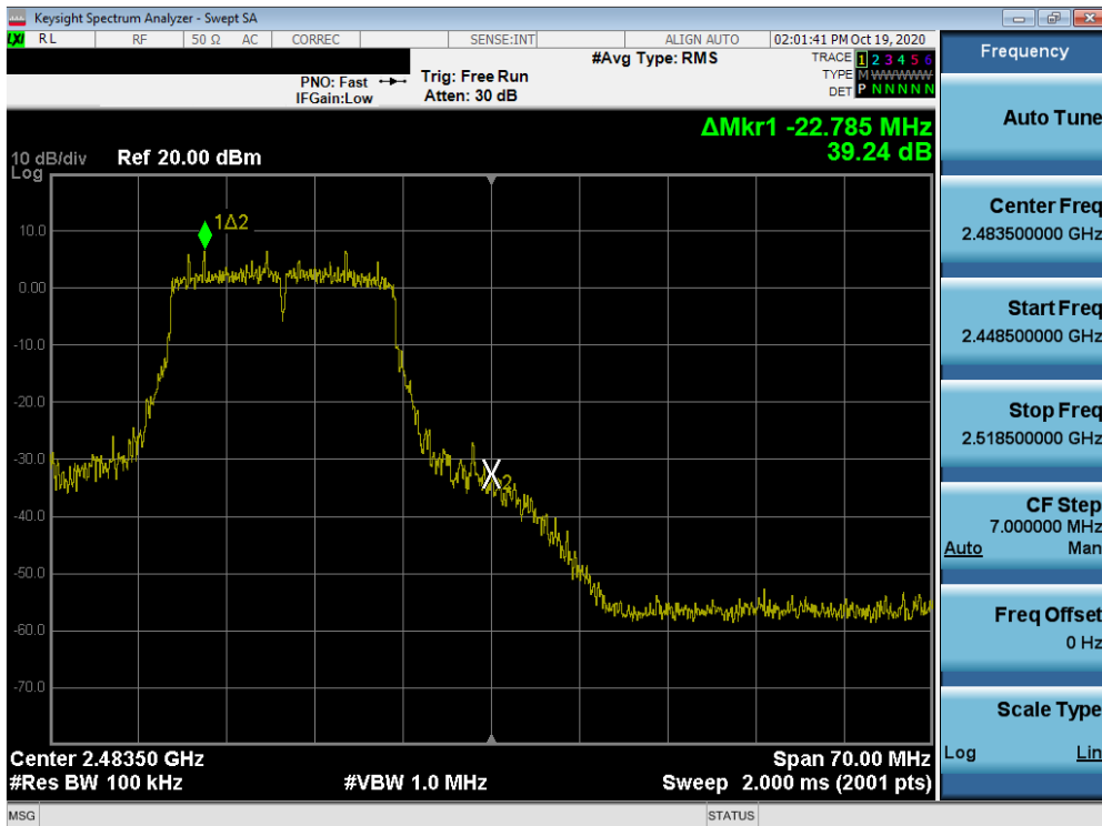
Plot 7-70. Band Edge Plot MIMO ANT2 (802.11n (2.4GHz) – Ch. 12)
