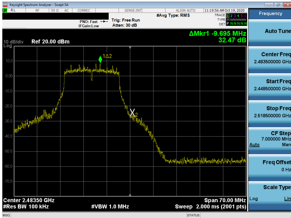
Plot 7-64. Band Edge Plot MIMO ANT2 (802.11g – Ch. 13)
