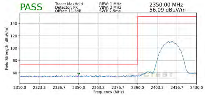
Plot 7-104. Radiated Restricted Lower Band Edge Measurement SISO ANT2 (Peak)
