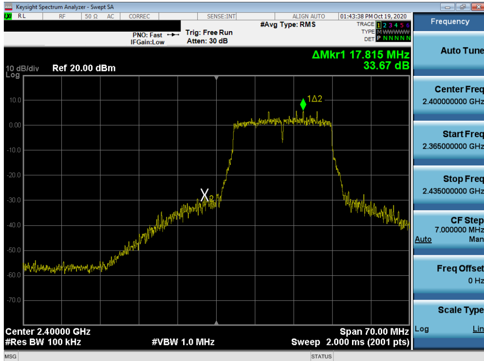
Plot 7-66. Band Edge Plot MIMO ANT2 (802.11n (2.4GHz) – Ch. 1)
