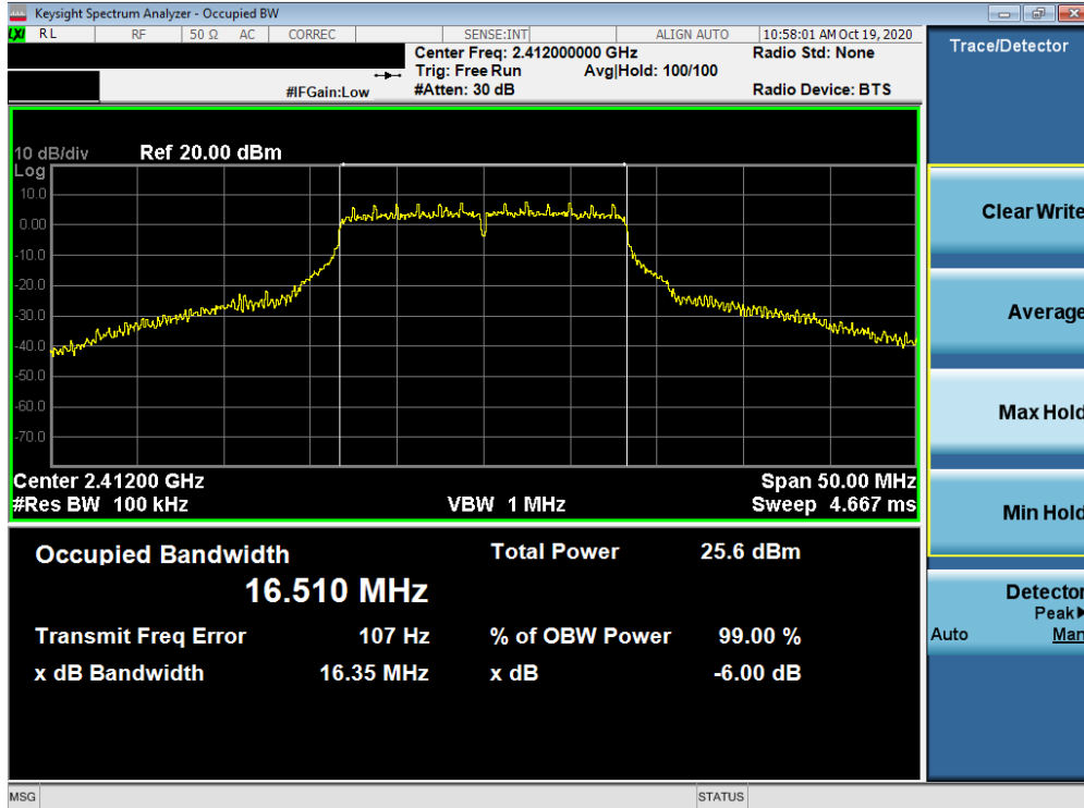
Plot 7-8. 6dB Bandwidth Plot MIMO ANT2 (802.11g – Ch. 1)
