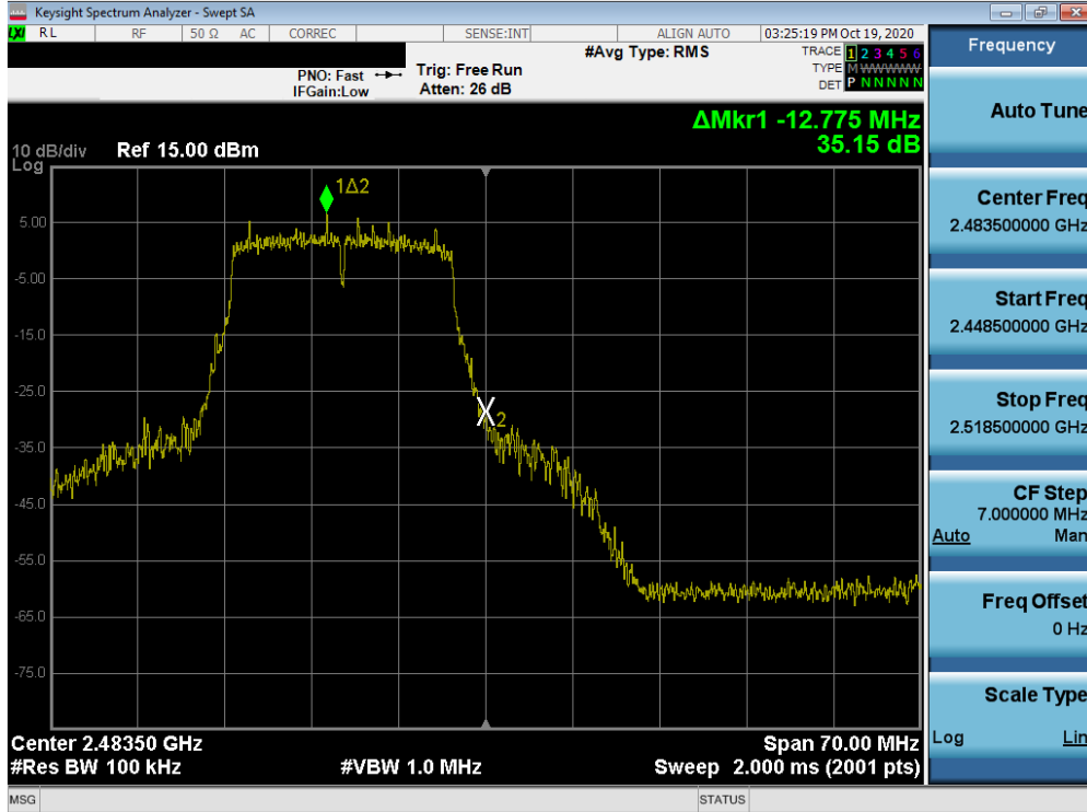
Plot 7-71. Band Edge Plot MIMO ANT1 (802.11n (2.4GHz) – Ch. 13)
