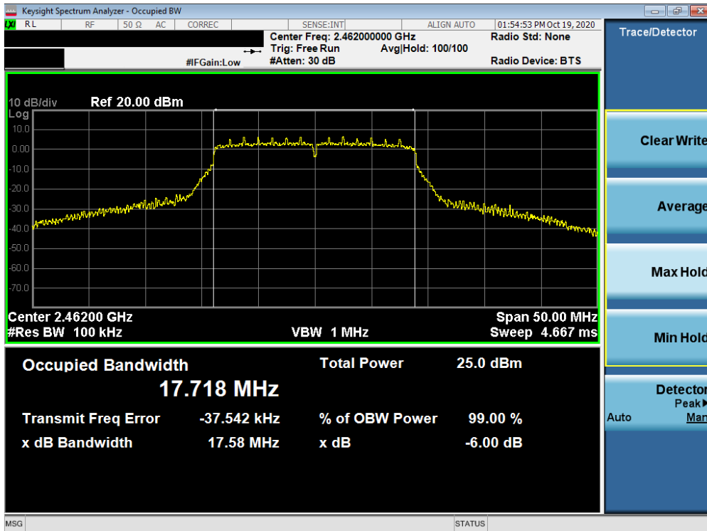
Plot 7-18. 6dB Bandwidth Plot MIMO ANT1 (802.11n (2.4GHz) – Ch. 11)
