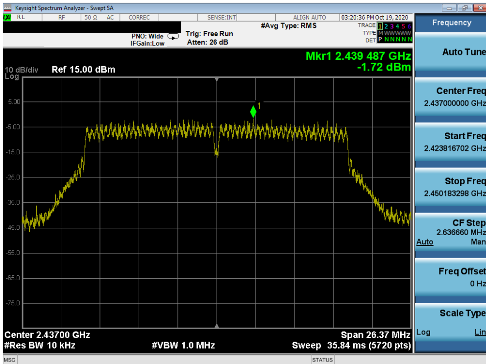
Plot 7-39. Power Spectral Density Plot MIMO ANT1 (802.11n (2.4GHz) – Ch. 6)
