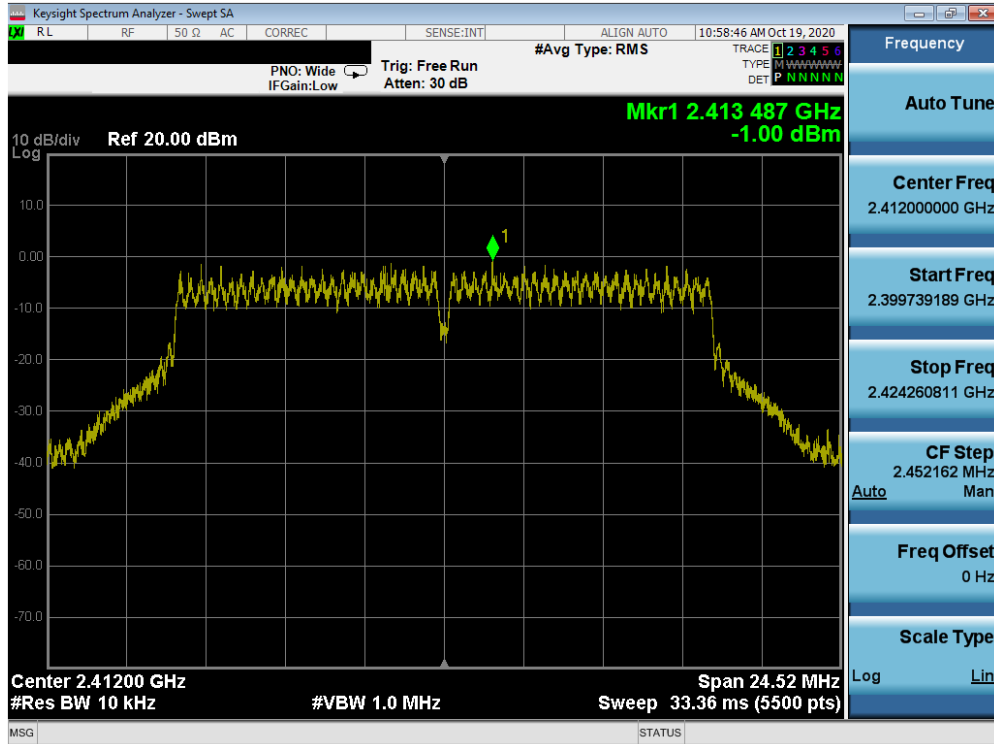
Plot 7-32. Power Spectral Density Plot MIMO ANT2 (802.11g – Ch. 1)
