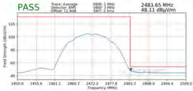
Plot 7-107. Radiated Restricted Band Edge Measurement SISO ANT2 (Average)
