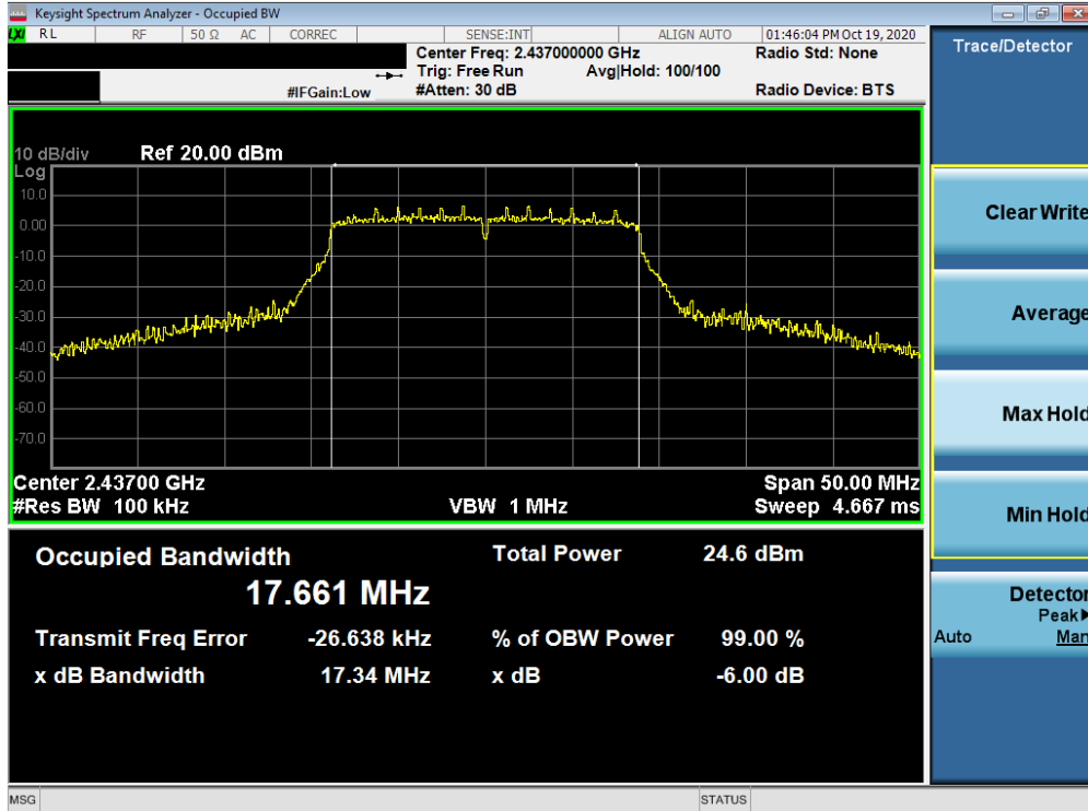
Plot 7-16. 6dB Bandwidth Plot MIMO ANT2 (802.11n) (2.4GHz) – Ch. 6)
