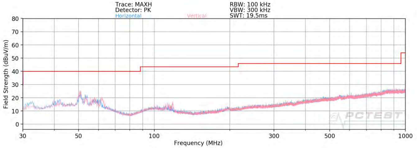
Plot 7-127. Radiated Spurious Plot below 1GHz
