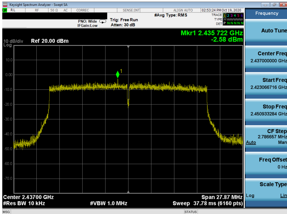
Plot 7-45. Power Spectral Density Plot MIMO ANT1 (802.11ax (2.4GHz) – Ch. 6)
