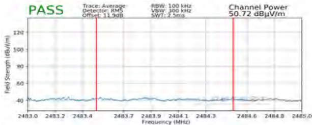
Plot 7-121. Radiated Restricted Band Edge Measurement MIMO (Average)
