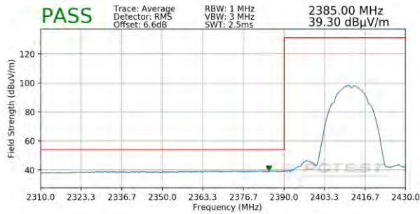
Plot 7-97. Radiated Restricted Lower Band Edge Measurement SISO ANT1 (Average)
