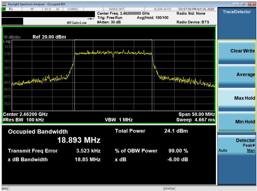
Plot 7-23. 6dB Bandwidth Plot MIMO ANT1 (802.11ax (2.4GHz) – Ch. 11)
