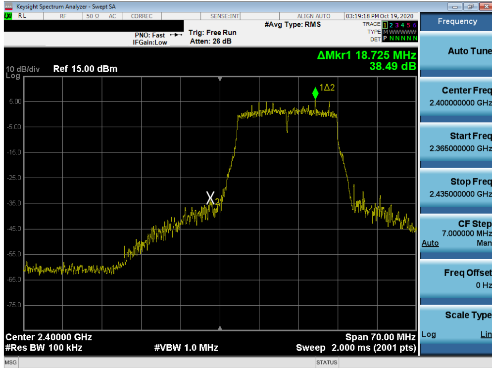
Plot 7-65. Band Edge Plot MIMO ANT1 (802.11n (2.4GHz) – Ch. 1)
