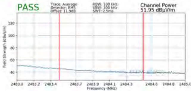
Plot 7-123. Radiated Restricted Band Edge Measurement MIMO (Average)
