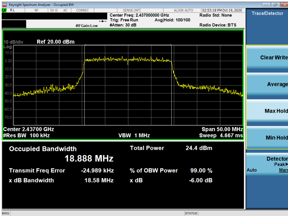
Plot 7-21. 6dB Bandwidth Plot MIMO ANT1 (802.11ax (2.4GHz) – Ch. 6)
