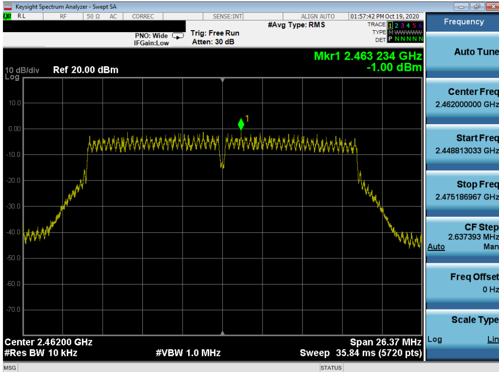
Plot 7-42. Power Spectral Density Plot MIMO ANT2 (802.11n (2.4GHz) – Ch. 11)
