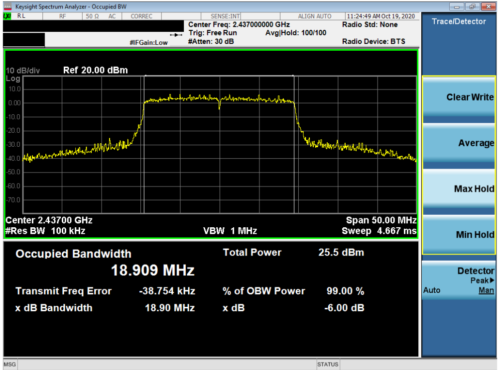
Plot 7-22. 6dB Bandwidth Plot MIMO ANT2 (802.11ax (2.4GHz) – Ch. 6)
