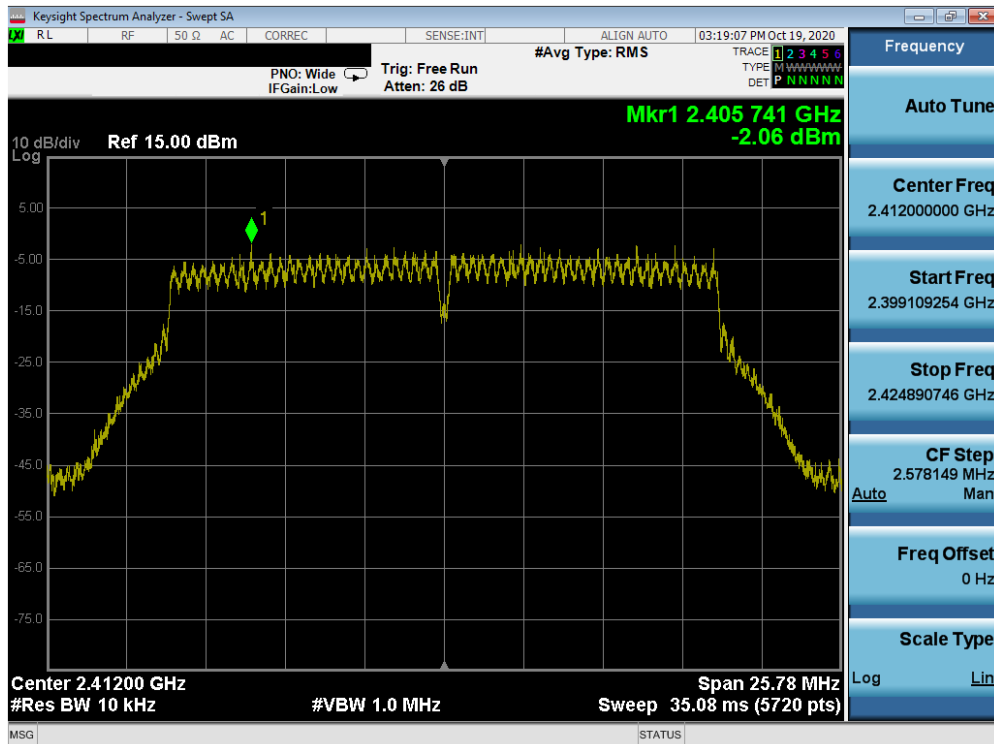
Plot 7-37. Power Spectral Density Plot MIMO ANT1 (802.11n (2.4GHz) – Ch. 1)
