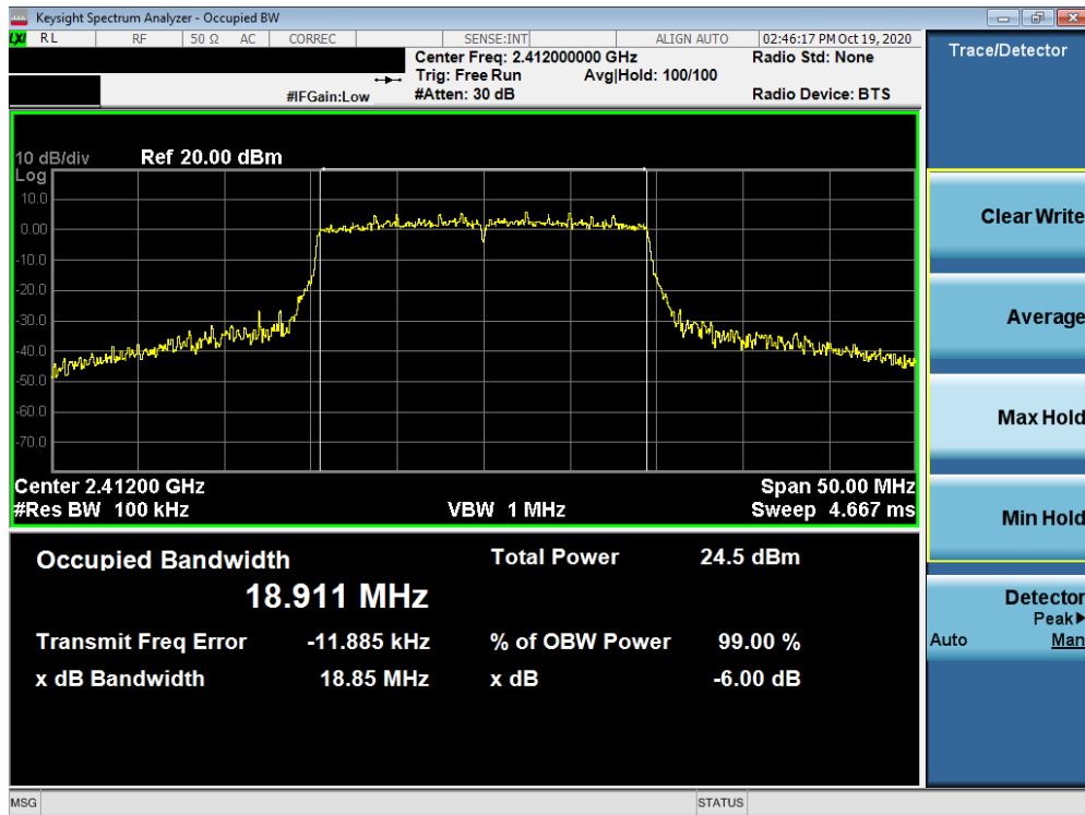
Plot 7-19. 6dB Bandwidth Plot MIMO ANT1 (802.11ax (2.4GHz) – Ch. 1)
