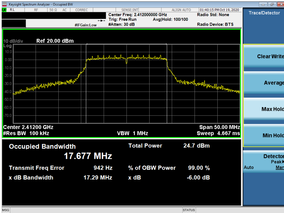
Plot 7-14. 6dB Bandwidth Plot MIMO ANT2 (802.11n (2.4GHz) – Ch. 1)
