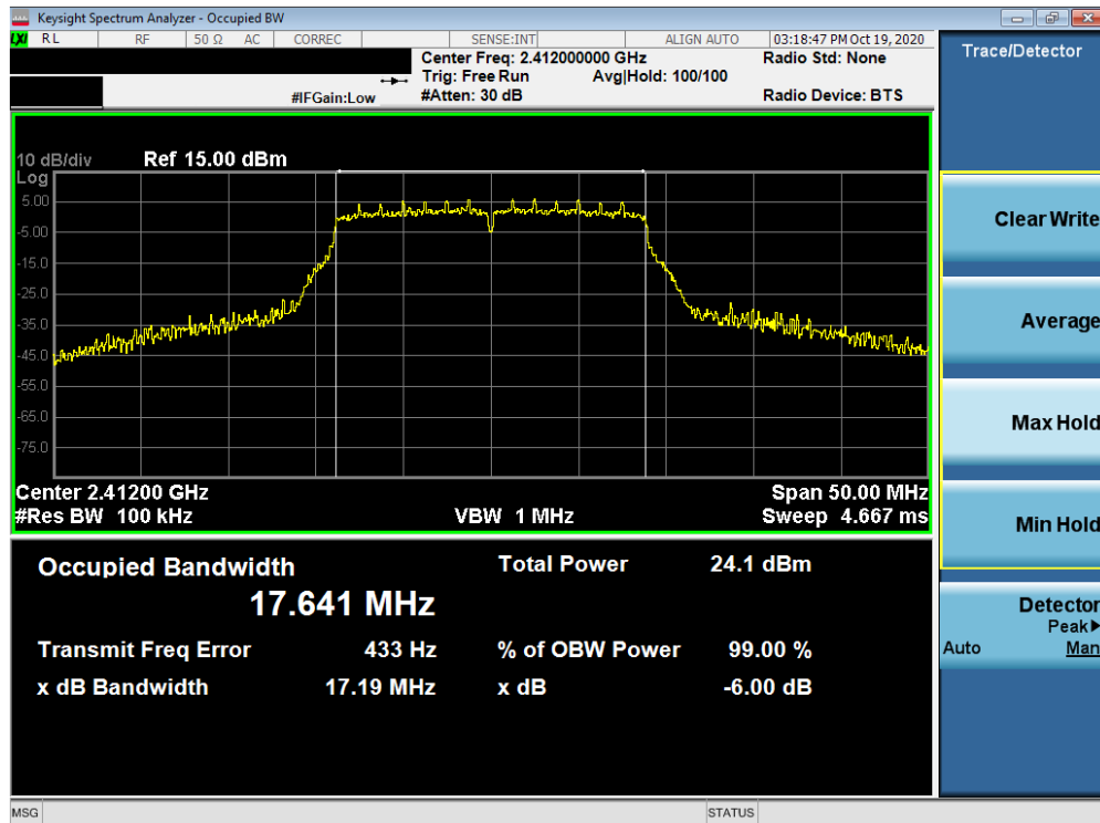
Plot 7-13. 6dB Bandwidth Plot MIMO ANT1 (802.11n (2.4GHz) – Ch. 1)
