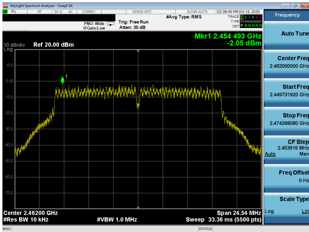
Plot 7-35. Power Spectral Density Plot MIMO ANT1 (802.11g – Ch. 11)
