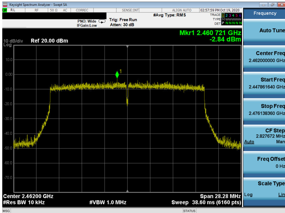
Plot 7-47. Power Spectral Density Plot MIMO ANT1 (802.11ax (2.4GHz) – Ch. 11)
