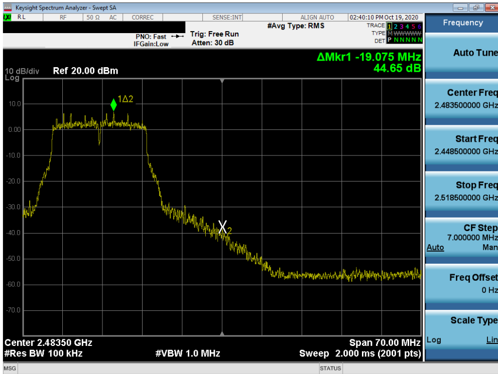
Plot 7-59. Band Edge Plot MIMO ANT1 (802.11g – Ch. 11)
