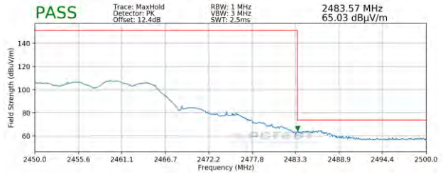
Plot 7-118. Radiated Restricted Upper Band Edge Measurement MIMO (Peak)
