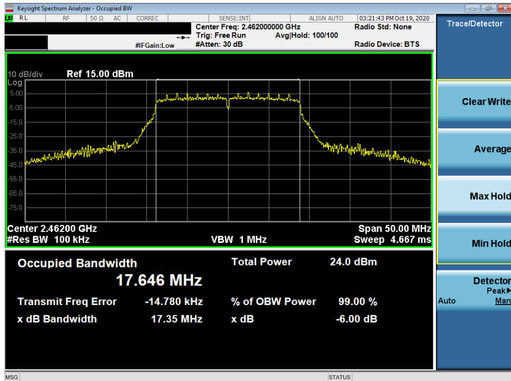
Plot 7-17. 6dB Bandwidth Plot MIMO ANT1 (802.11n) (2.4GHz) – Ch. 11)
