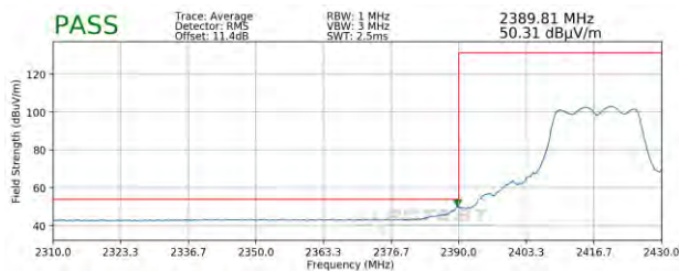
Plot 7-111. Radiated Restricted Lower Band Edge Measurement MIMO (Average)
