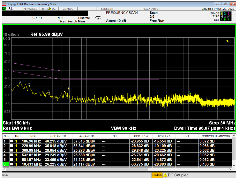
Plot 7-129. Line Conducted Plot with 802.11b (N)
