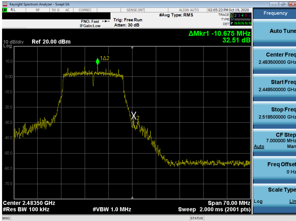
Plot 7-72. Band Edge Plot MIMO ANT2 (802.11n (2.4GHz) – Ch. 13)
