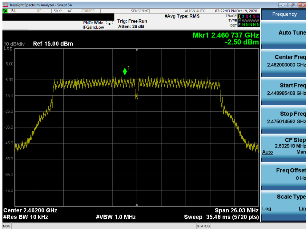
Plot 7-41. Power Spectral Density Plot MIMO ANT1 (802.11n (2.4GHz) – Ch. 11)
