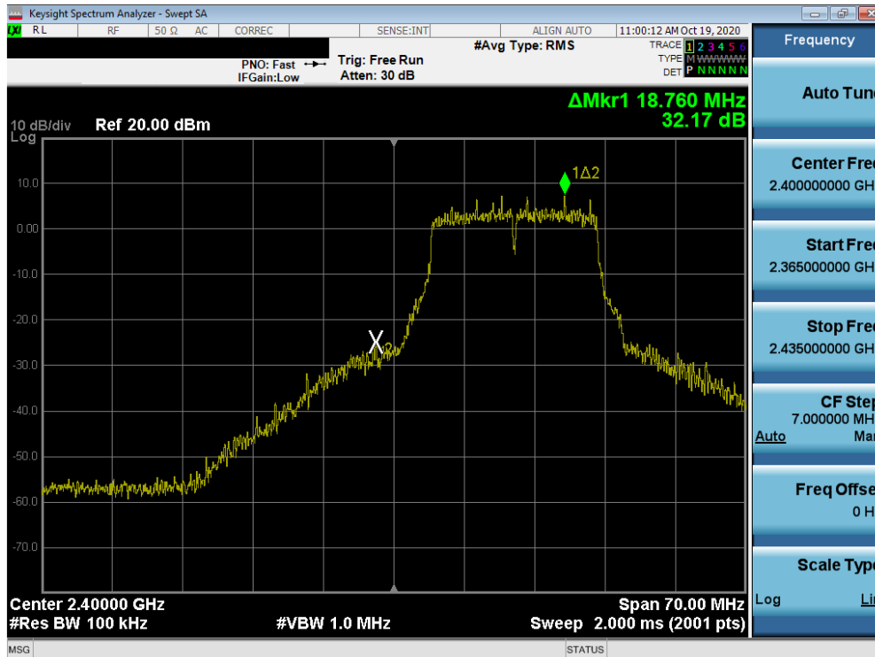
Plot 7-58. Band Edge Plot MIMO ANT2 (802.11g– Ch. 1)
