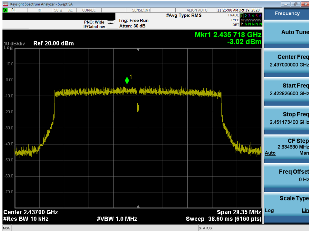
Plot 7-46. Power Spectral Density Plot MIMO ANT2 (802.11ax (2.4GHz) – Ch. 6)
