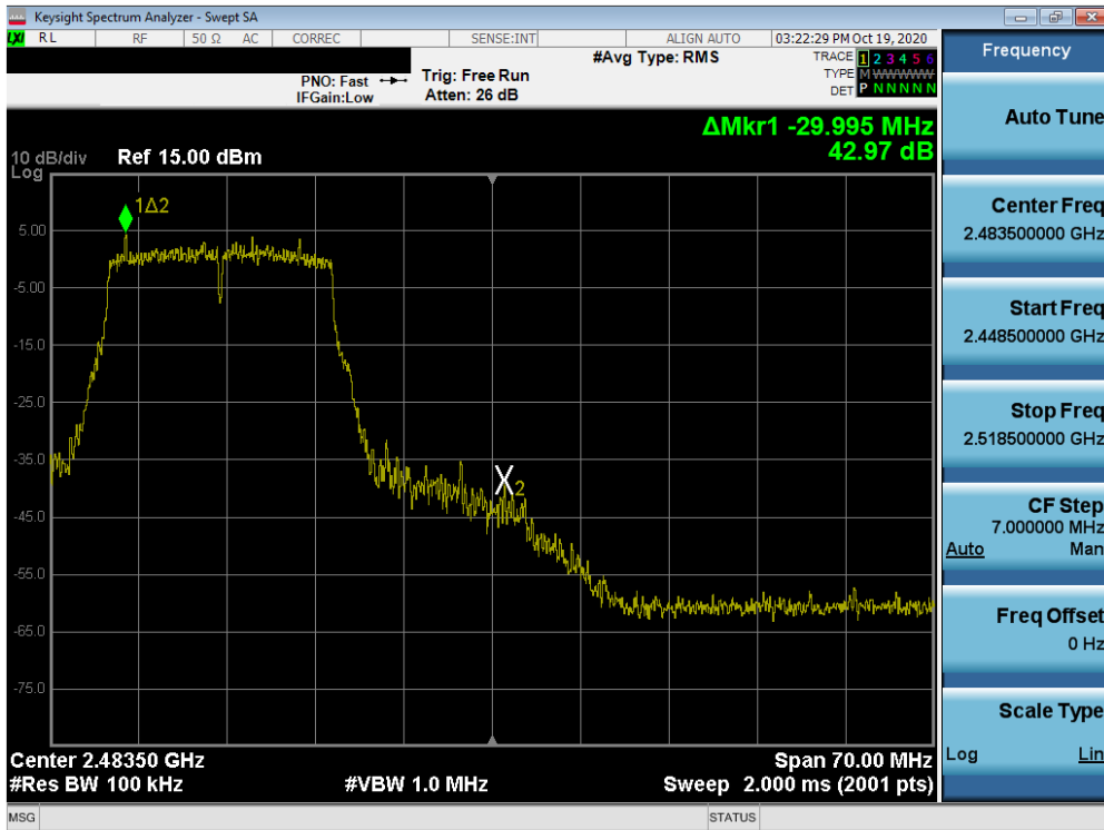
Plot 7-67. Band Edge Plot MIMO ANT1 (802.11n (2.4GHz) – Ch. 11)
