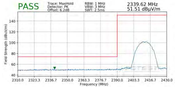
Plot 7-98. Radiated Restricted Lower Band Edge Measurement SISO ANT1 (Peak)
