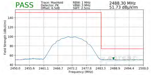
Plot 7-102. Radiated Restricted Band Edge Measurement SISO ANT1
