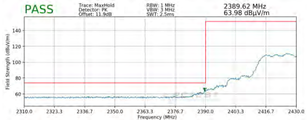
Plot 7-114. Radiated Restricted Lower Band Edge Measurement MIMO (Peak)
