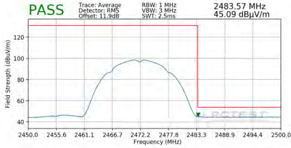
Plot 7-101. Radiated Restricted Band Edge Measurement SISO ANT1
