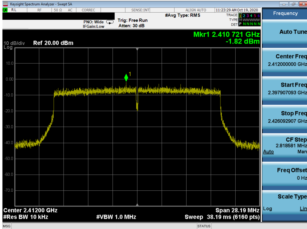
Plot 7-44. Power Spectral Density Plot MIMO ANT2 (802.11ax (2.4GHz) – Ch. 1)
