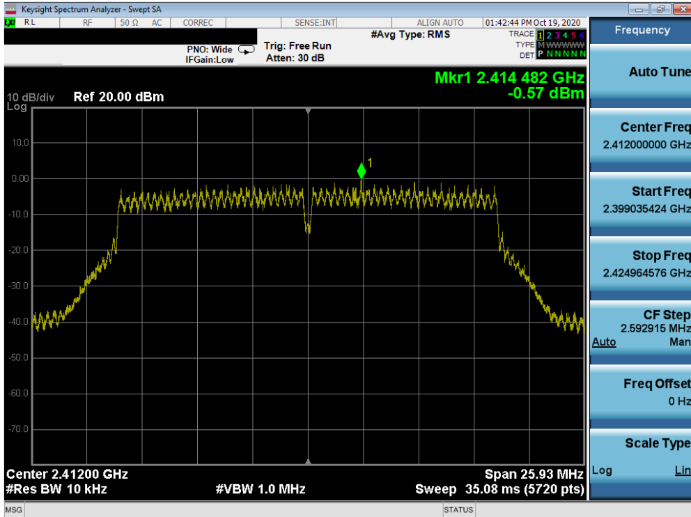
Plot 7-38. Power Spectral Density Plot MIMO ANT2 (802.11n (2.4GHz) – Ch. 1)
