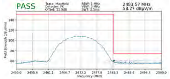
Plot 7-108. Radiated Restricted Band Edge Measurement SISO ANT2 (Peak)
