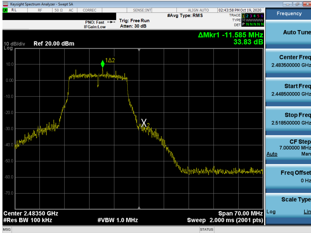
Plot 7-63. Band Edge Plot MIMO ANT1 (802.11g – Ch. 13)
