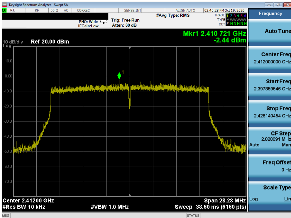
Plot 7-43. Power Spectral Density Plot MIMO ANT1 (802.11ax (2.4GHz) – Ch. 1)
