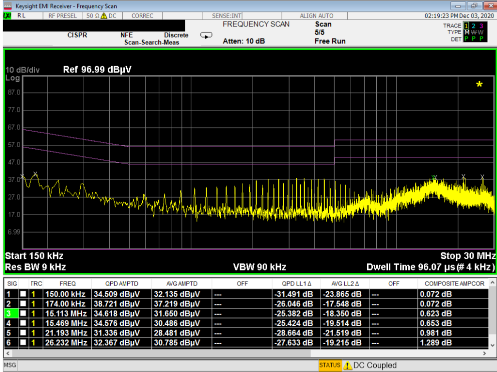
Plot 7-130. Line Conducted Plot with 802.11b with WCP (L1)
