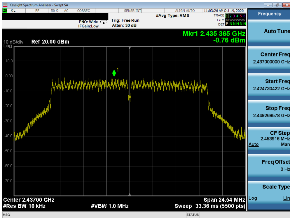
Plot 7-34. Power Spectral Density Plot MIMO ANT2 (802.11g – Ch. 6)
