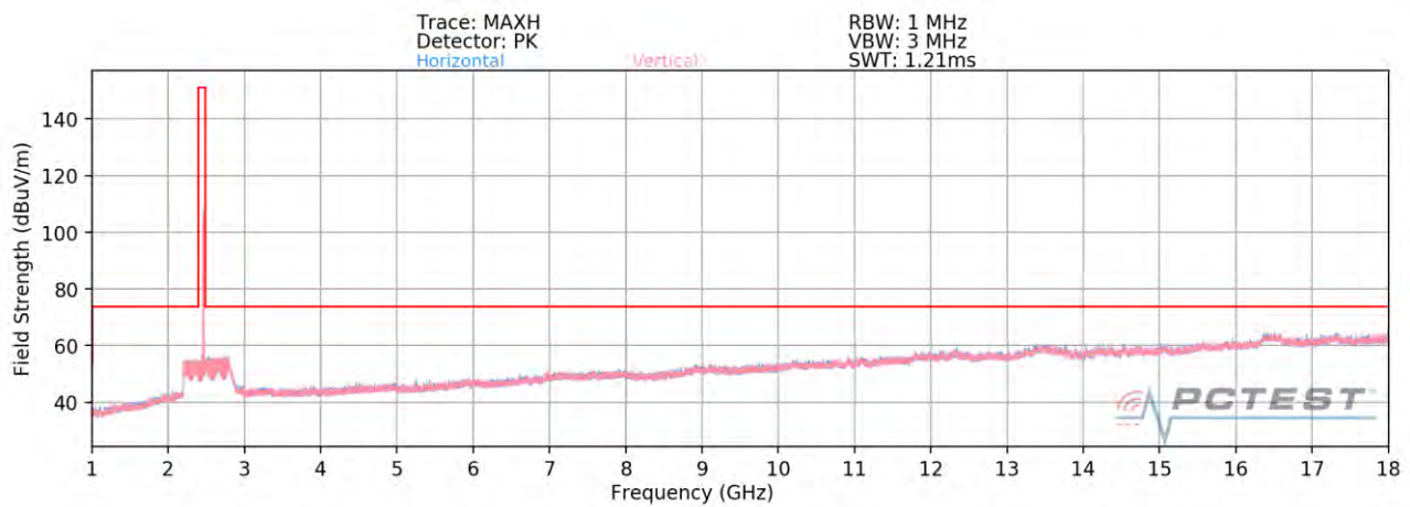
Plot 7-91. Radiated Spurious Plot above 1GHz SISO ANT2 (802.11b – Ch. 11)
