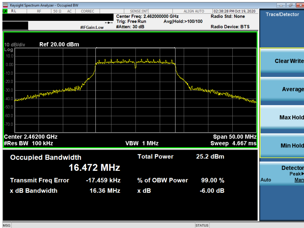
Plot 7-11. 6dB Bandwidth Plot MIMO ANT1 (802.11g – Ch. 11)
