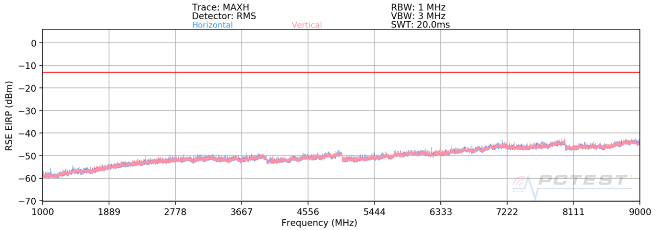
Plot 7-33. Radiated Spurious Plot (LTE Band 26)
