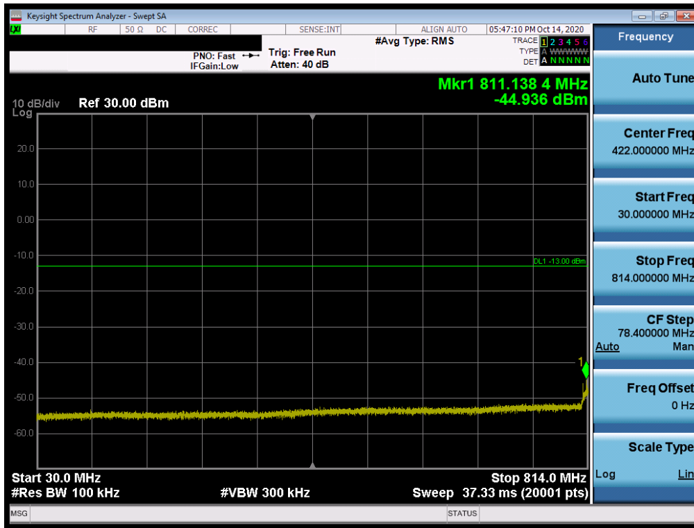
Plot 7-21. Conducted Spurious Plot (LTE Band 26 - 15MHz QPSK - RB Size 1, RB Offset 0)
