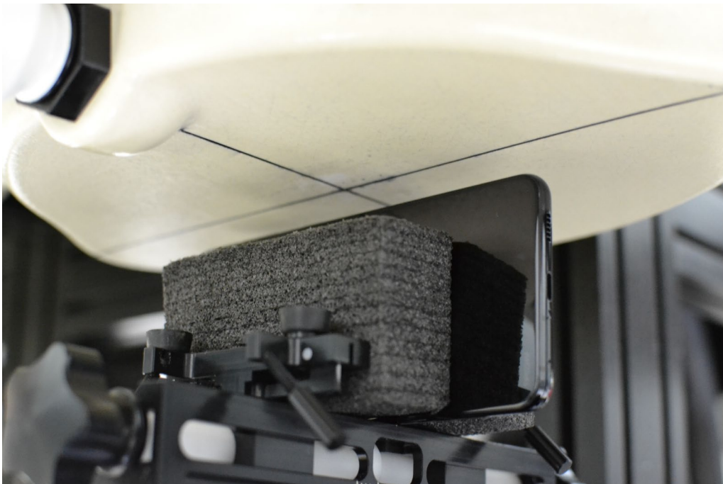
SAR Test Setup Photo 8 – Right Side at 10 mm
