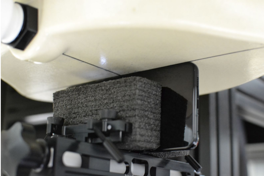
SAR Test Setup Photo 9 – Right Side at 0 mm
