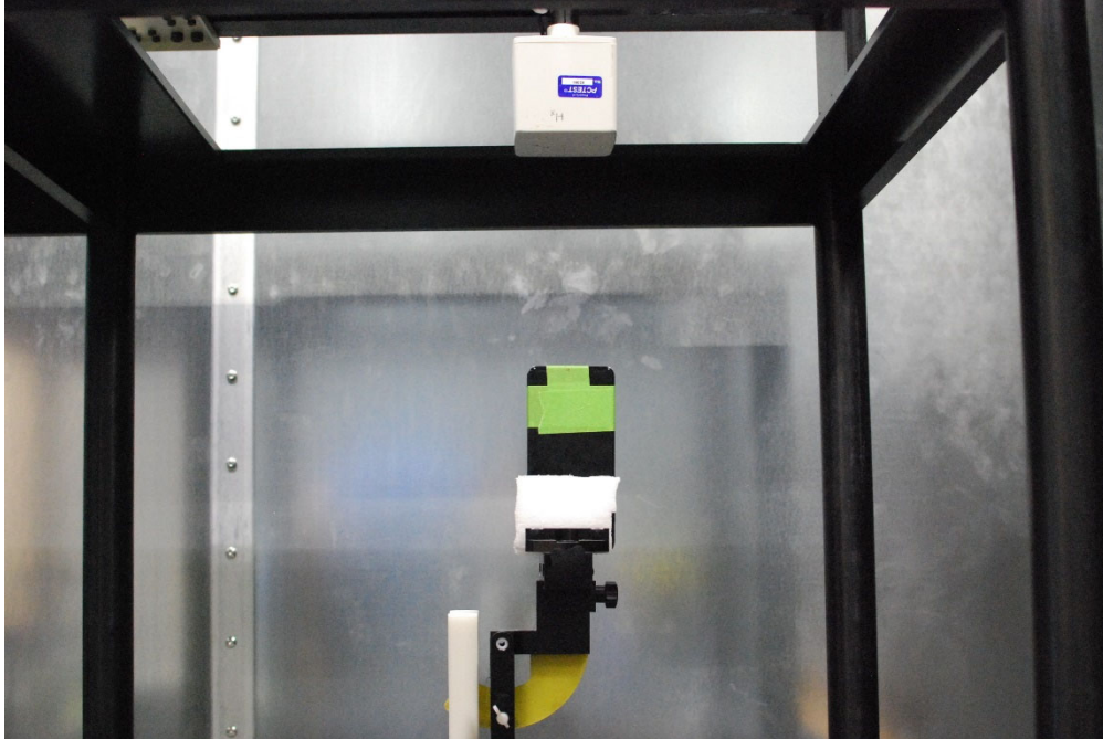
Photo 23. H-field 20cm
