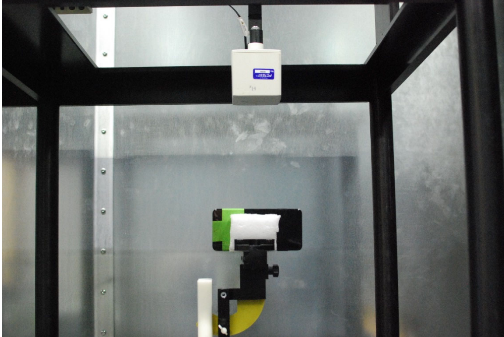
Photo 21. H-field 20cm
