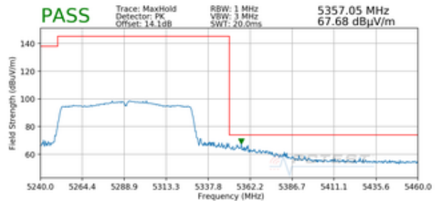
Plot 7-306. Radiated Upper Band Edge Plot SISO ANT1 (Peak – UNII Band 2A)
