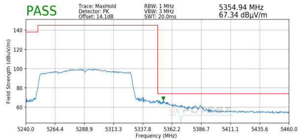
Plot 7-348. Radiated Upper Band Edge Plot MIMO (Peak – UNII Band 2A)
