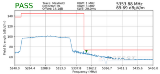
Plot 7-327. Radiated Upper Band Edge Plot SISO ANT2 (Peak – UNII Band 2A)
