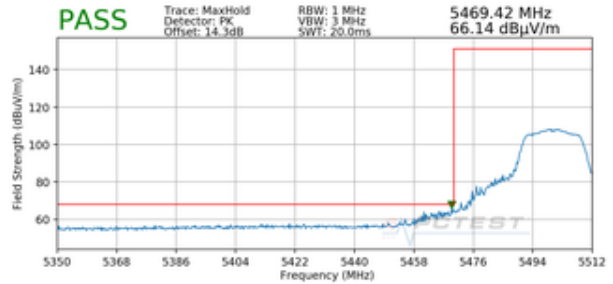
Plot 7-315. Radiated Lower Band Edge Plot SISO ANT2 (Peak – UNII Band 2C)
