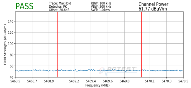
Plot 7-329. Radiated Lower Band Edge Plot SISO ANT2 (Peak – UNII Band 2C)
