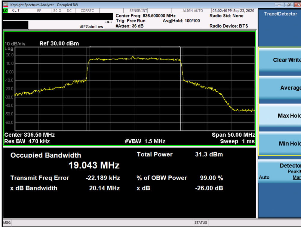
Plot 7-23. Occupied Bandwidth Plot (NR Band n5 - 20MHz 16-QAM - Full RB Configuration)
