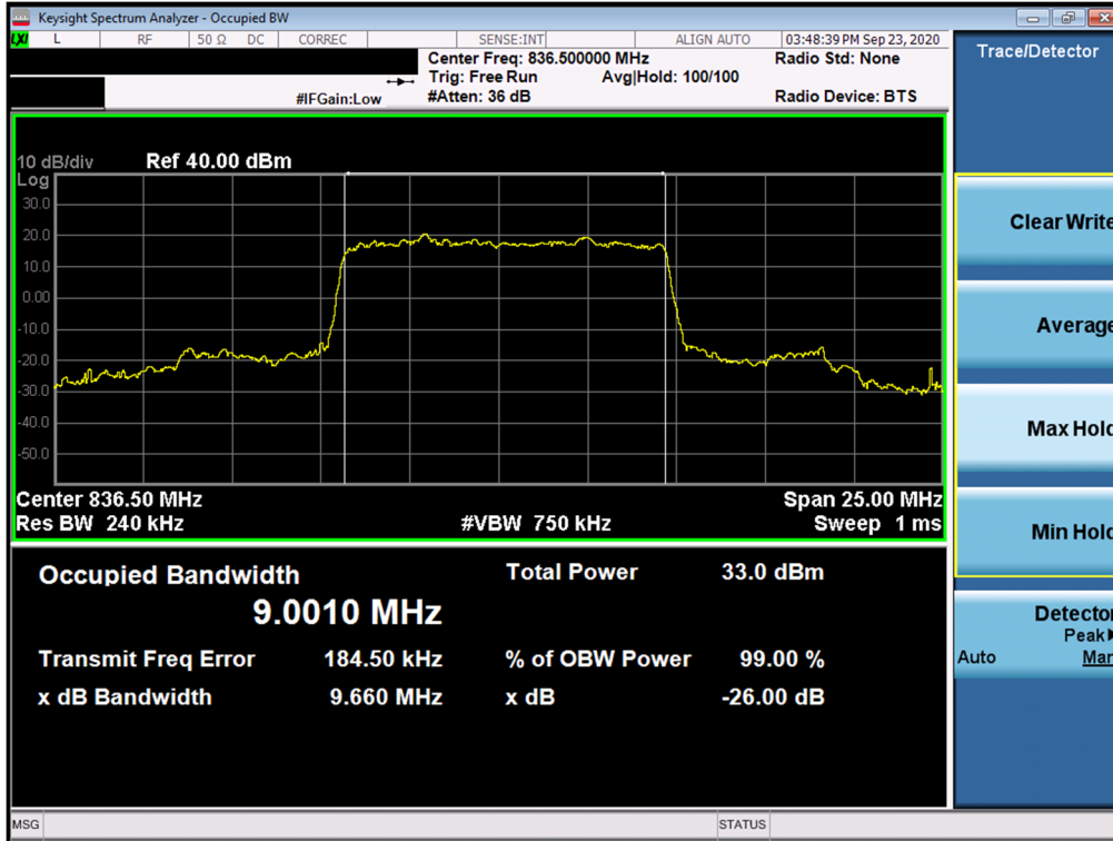
Plot 7-31. Occupied Bandwidth Plot (NR Band n5 - 10MHz \pi/2 BPSK - Full RB Configuration)
