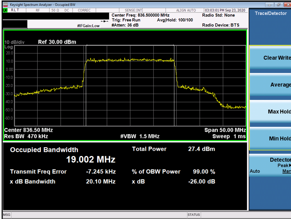
Plot 7-25. Occupied Bandwidth Plot (NR Band n5 - 20MHz 256-QAM - Full RB Configuration)
