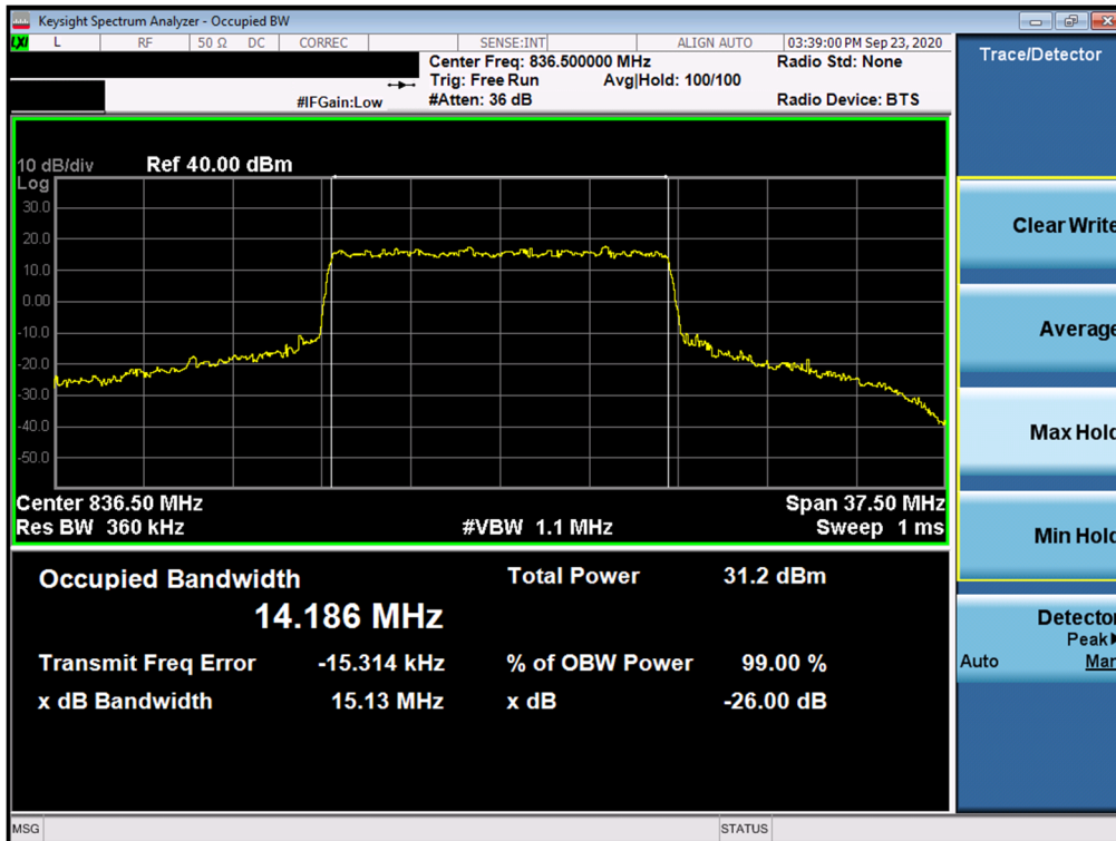
Plot 7-28. Occupied Bandwidth Plot (NR Band n5 - 15MHz 16-QAM - Full RB Configuration)
