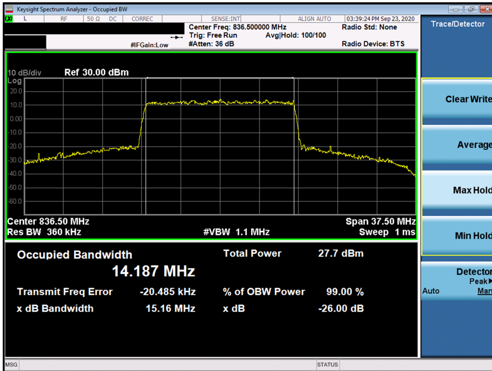
Plot 7-30. Occupied Bandwidth Plot (NR Band n5 - 15MHz 256-QAM - Full RB Configuration)
