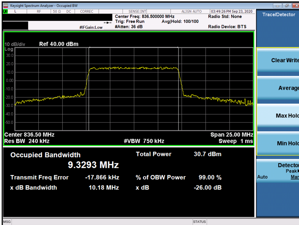
Plot 7-32. Occupied Bandwidth Plot (NR Band n5 - 10MHz QPSK - Full RB Configuration)
