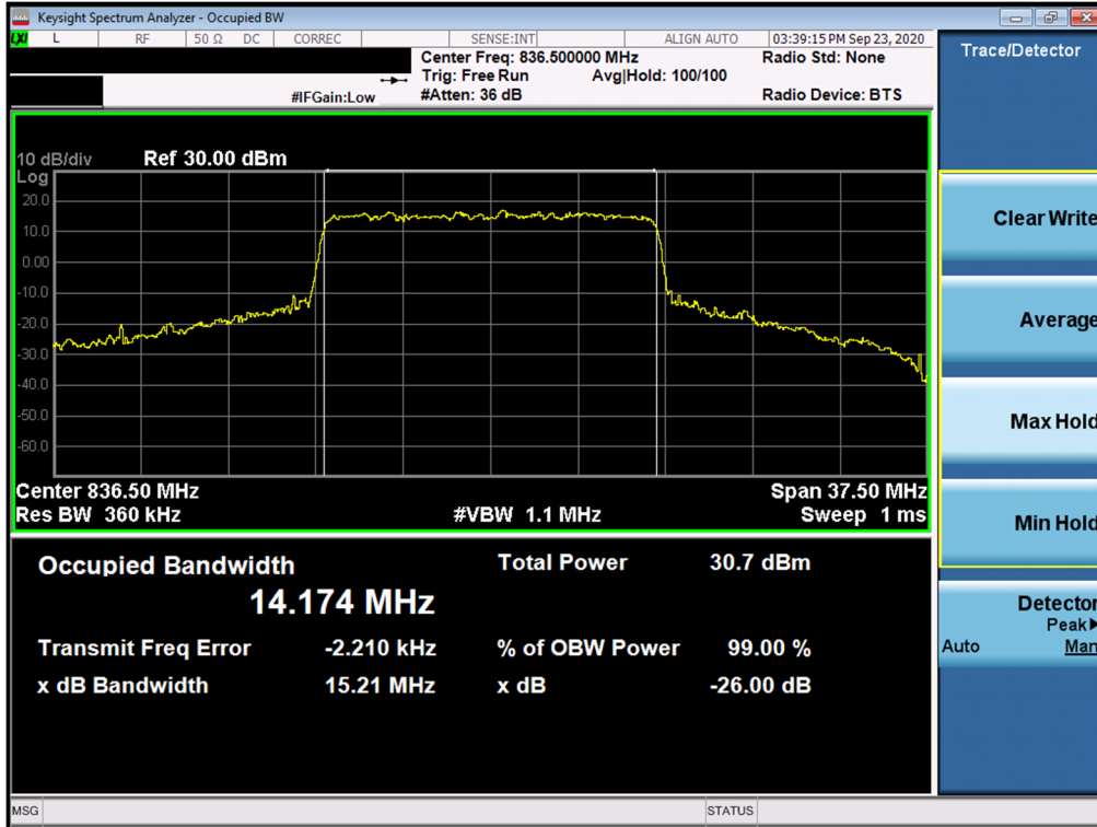
Plot 7-29. Occupied Bandwidth Plot (NR Band n5 - 15MHz 64-QAM - Full RB Configuration)
