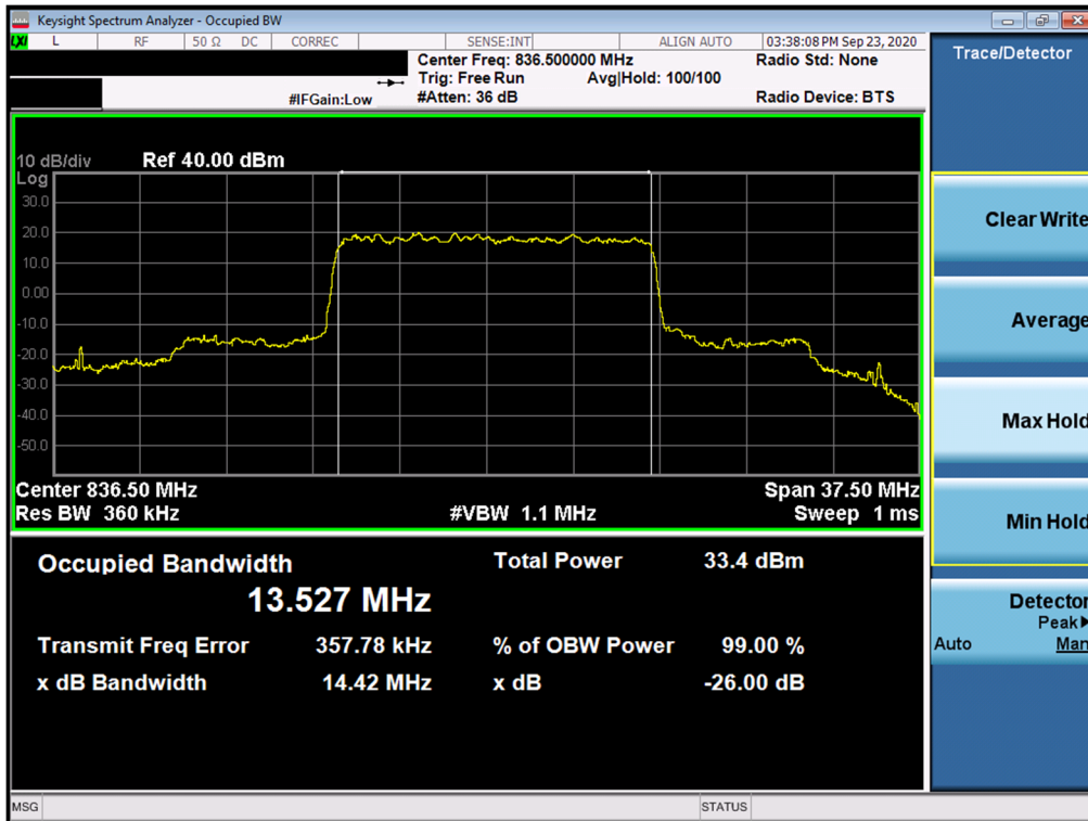
Plot 7-26. Occupied Bandwidth Plot (NR Band n5 - 15MHz \pi/2 BPSK - Full RB Configuration)
