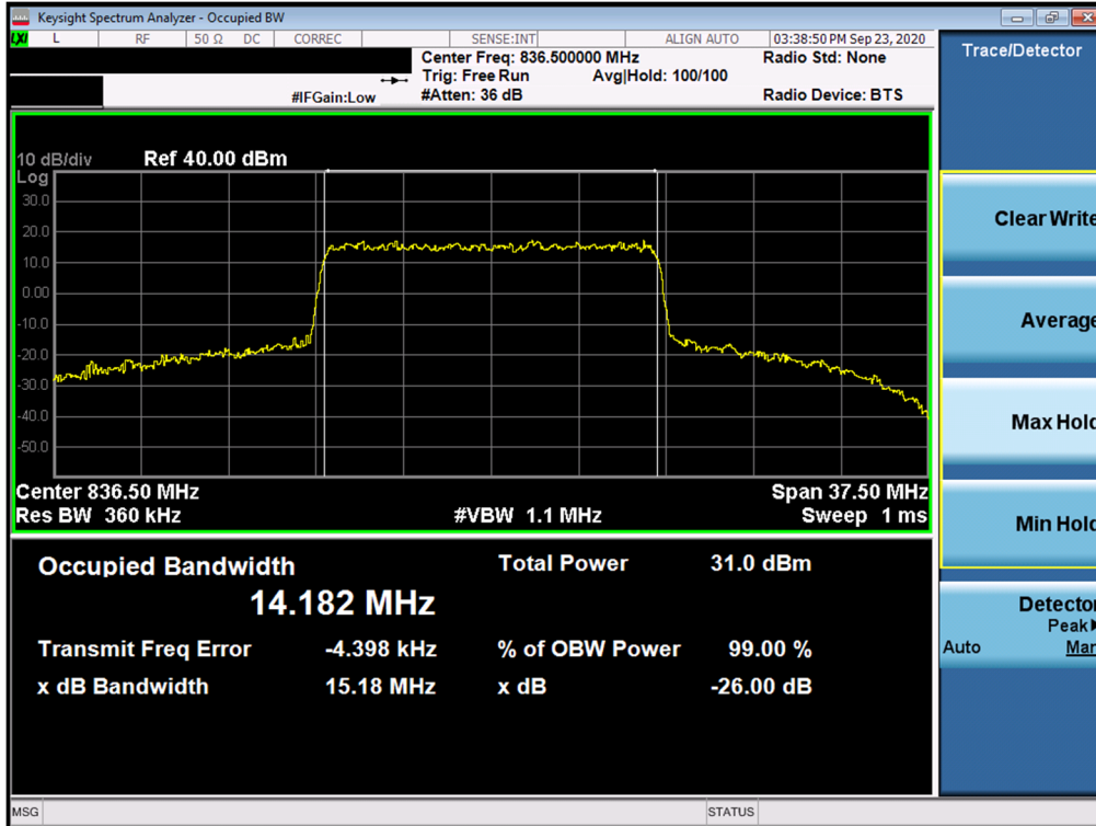
Plot 7-27. Occupied Bandwidth Plot (NR Band n5 - 15MHz QPSK - Full RB Configuration)
