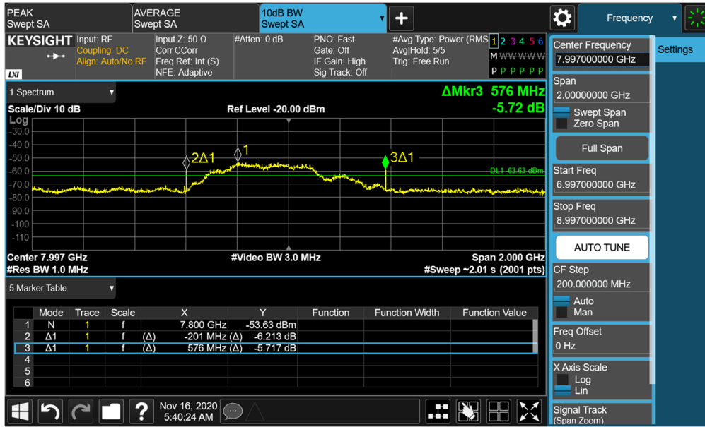
Plot 7-123. BANDWIDTH Plot – ANT1 - CH.9 – SP3 – Preamble 29
