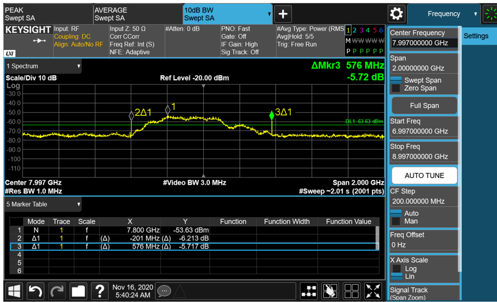
Plot 7-126. BANDWIDTH Plot – ANT2 - CH.9 – SP3 – Preamble 29
