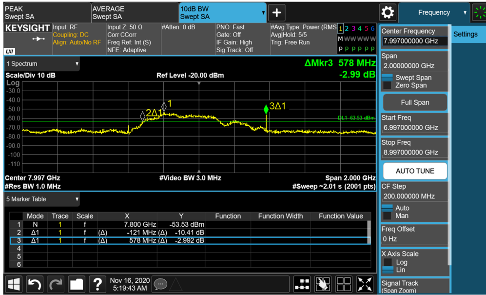
Plot 7-115. BANDWIDTH Plot – ANT1 - CH.9 - SP0 – Preamble 28
