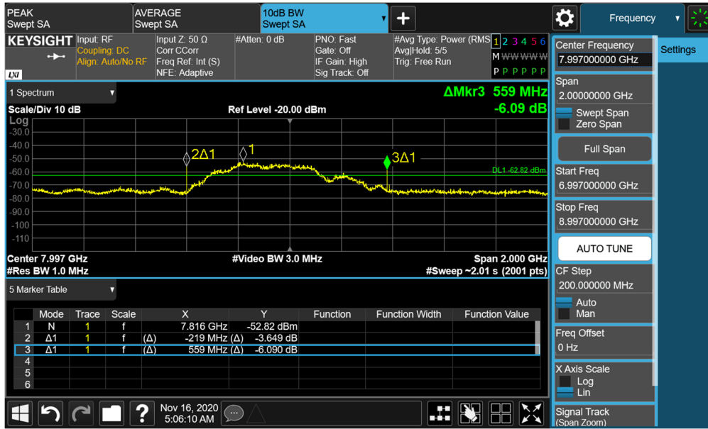
Plot 7-113. BANDWIDTH Plot – ANT2 - CH.9 – SP1 – Preamble 27
