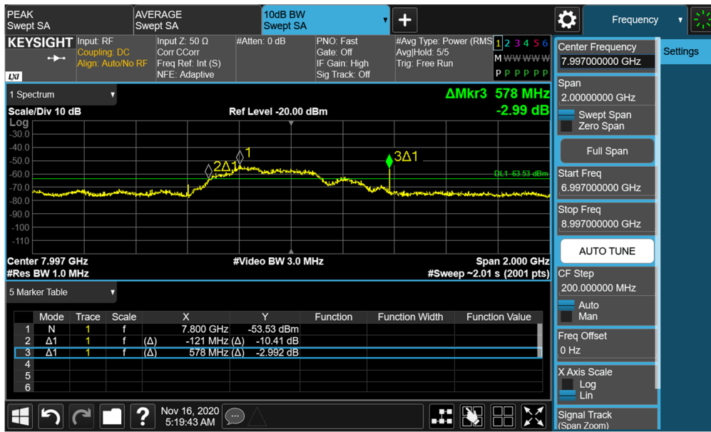
Plot 7-120. BANDWIDTH Plot – ANT2 - CH.9 – SP3 – Preamble 28
