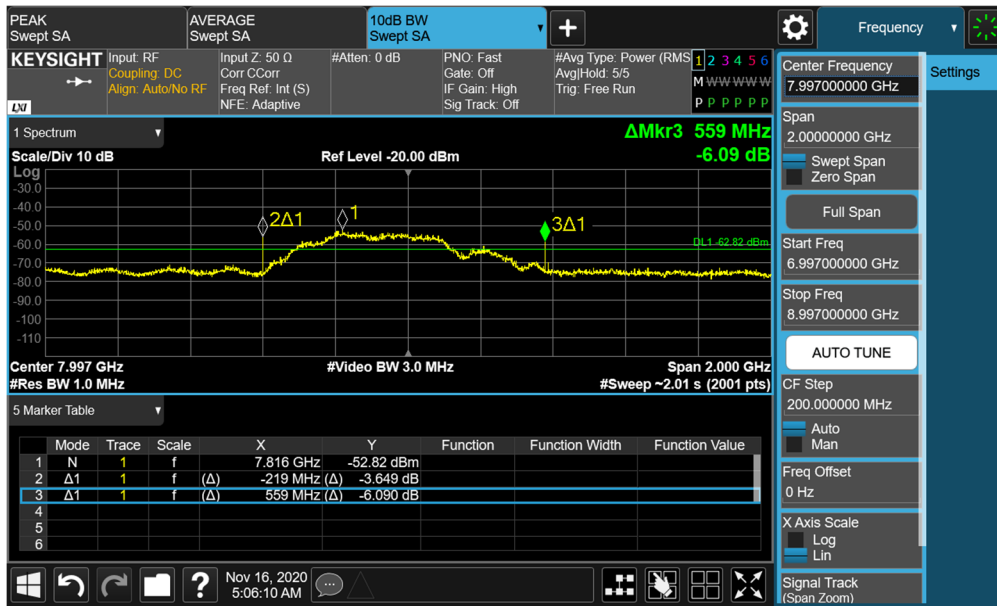
Plot 7-110. BANDWIDTH Plot – ANT1 - CH.9 – SP1 – Preamble 27
