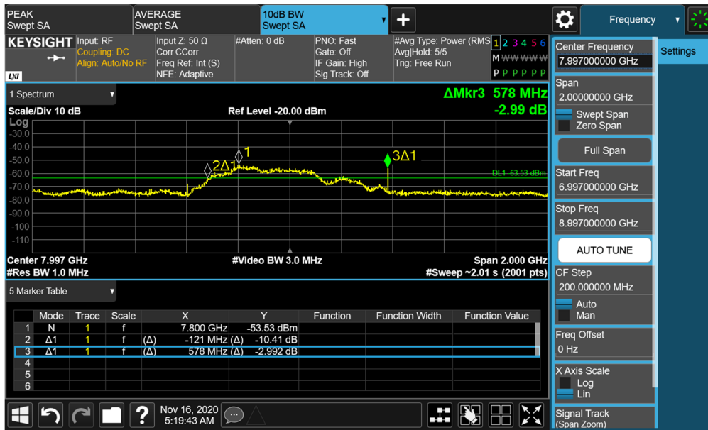
Plot 7-116. BANDWIDTH Plot – ANT1 - CH.9 – SP1 – Preamble 28
