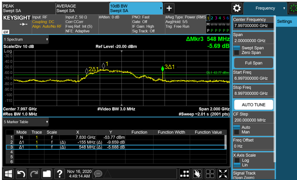
Plot 7-104. BANDWIDTH Plot – ANT1 - CH.9 – SP1 – Preamble 26
