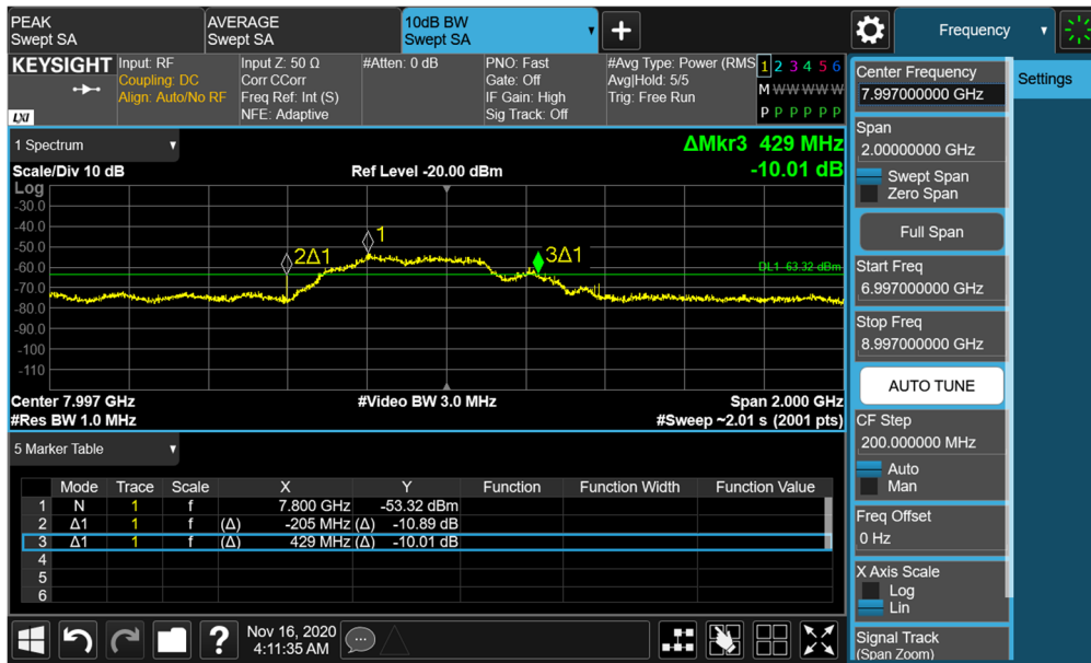
Plot 7-98. BANDWIDTH Plot – ANT1 - CH.9 – SP1 – Preamble 25
