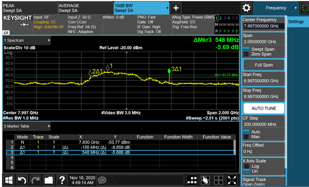
Plot 7-105. BANDWIDTH Plot – ANT1 - CH.9 – SP3 – Preamble 26
