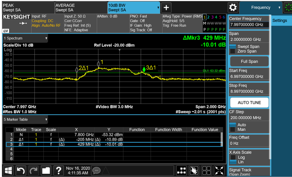
Plot 7-101. BANDWIDTH Plot – ANT2 - CH.9 – SP1 – Preamble 25
