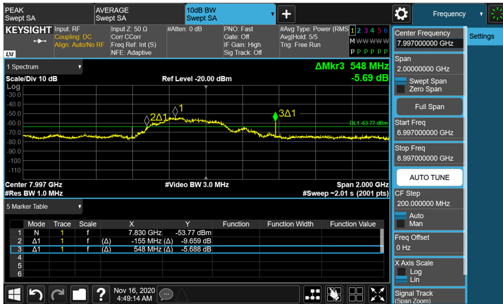
Plot 7-106. BANDWIDTH Plot – ANT2 - CH.9 - SP0 – Preamble 26
