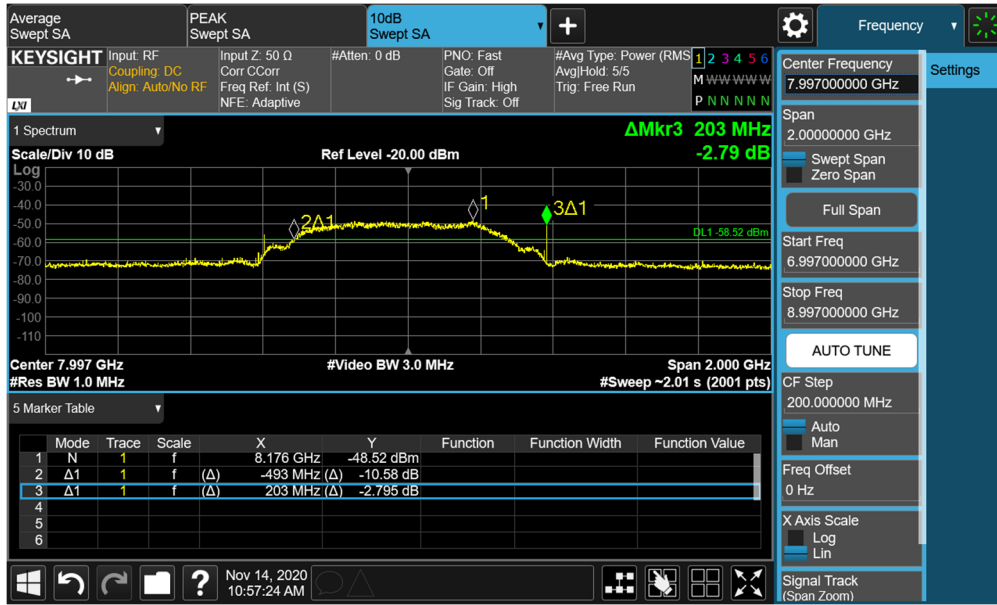
Plot 7-89. BANDWIDTH Plot – ANT2 - CH.9 – SP1 – Preamble 11
