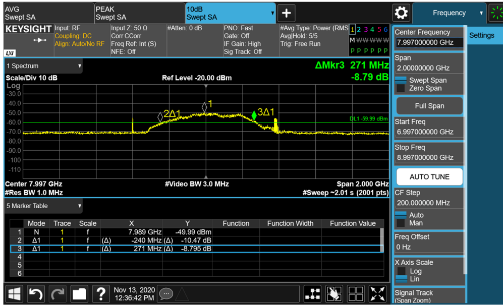
Plot 7-75. BANDWIDTH Plot – ANT1 - CH.9 – SP3 – Preamble 9
