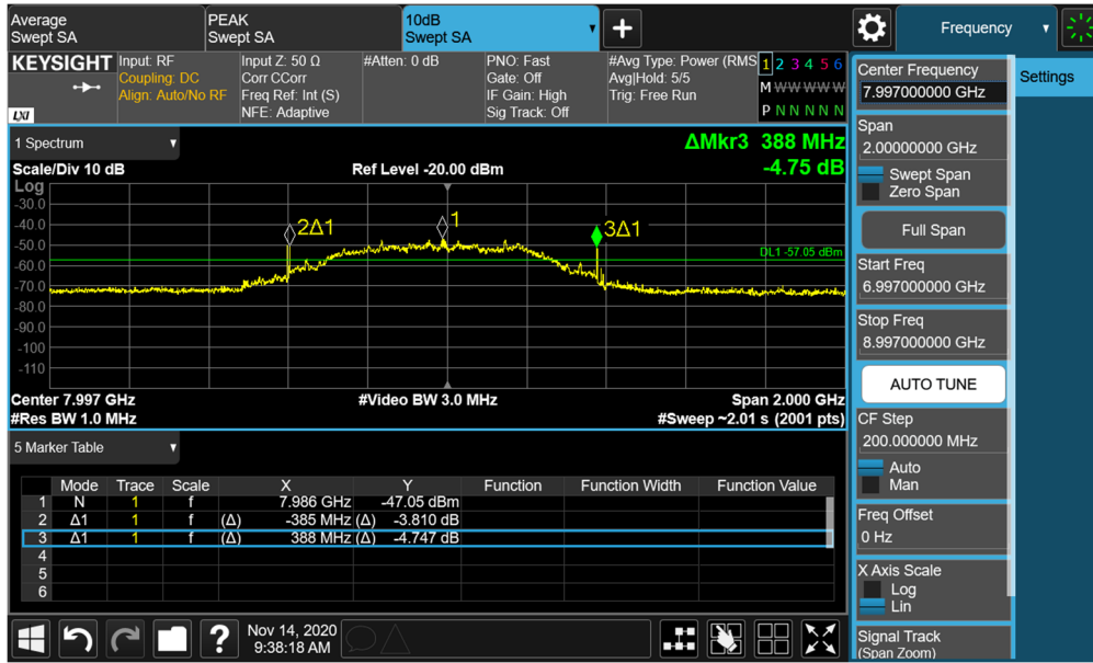
Plot 7-77. BANDWIDTH Plot – ANT2 - CH.9 – SP1 – Preamble 9
