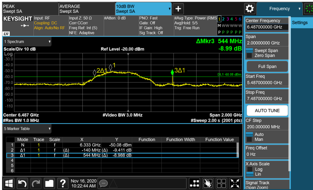
Plot 7-50. BANDWIDTH Plot – ANT1 - CH.5 – SP1 – Preamble 29
