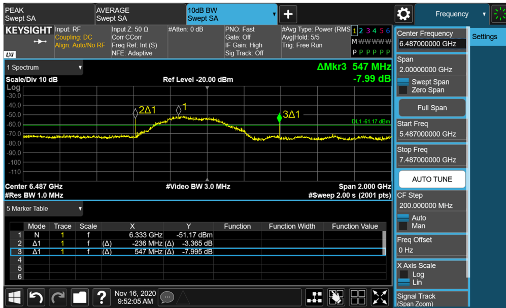
Plot 7-38. BANDWIDTH Plot – ANT1 - CH.5 – SP1 – Preamble 27
