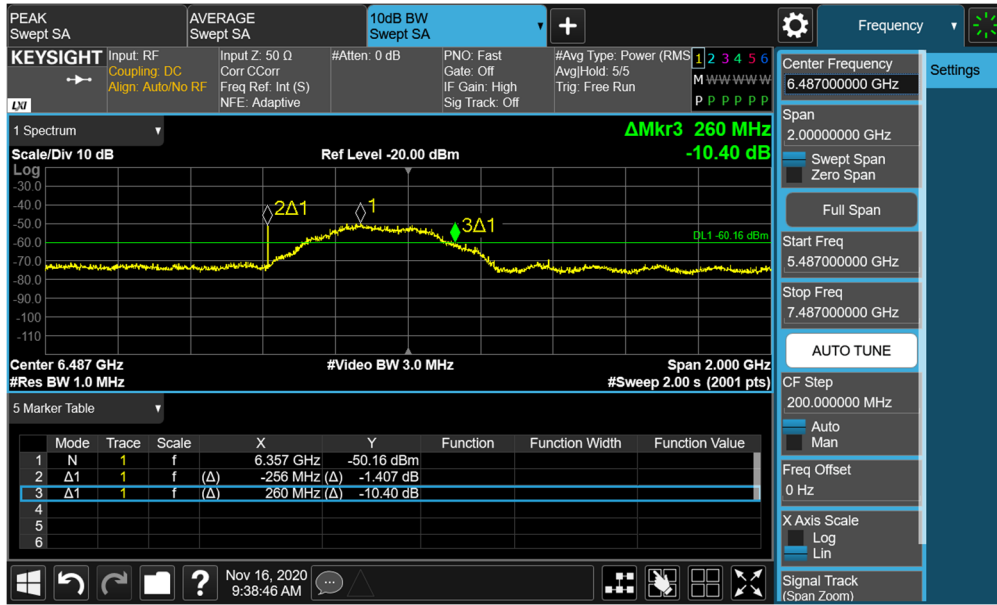
Plot 7-33. BANDWIDTH Plot – ANT1 - CH.5 – SP3 – Preamble 26
