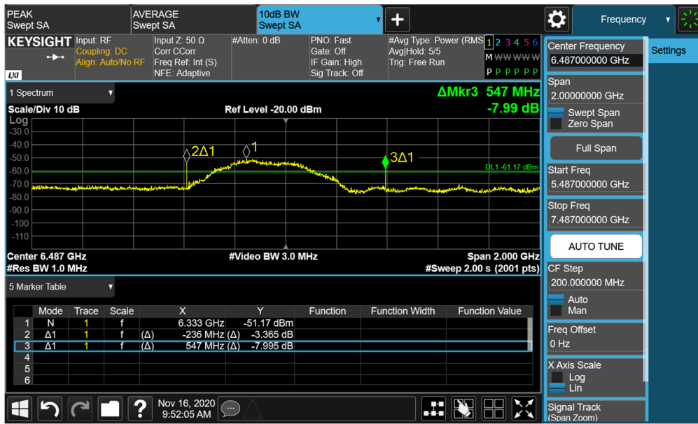
Plot 7-42. BANDWIDTH Plot – ANT2 - CH.5 – SP3 – Preamble 27
