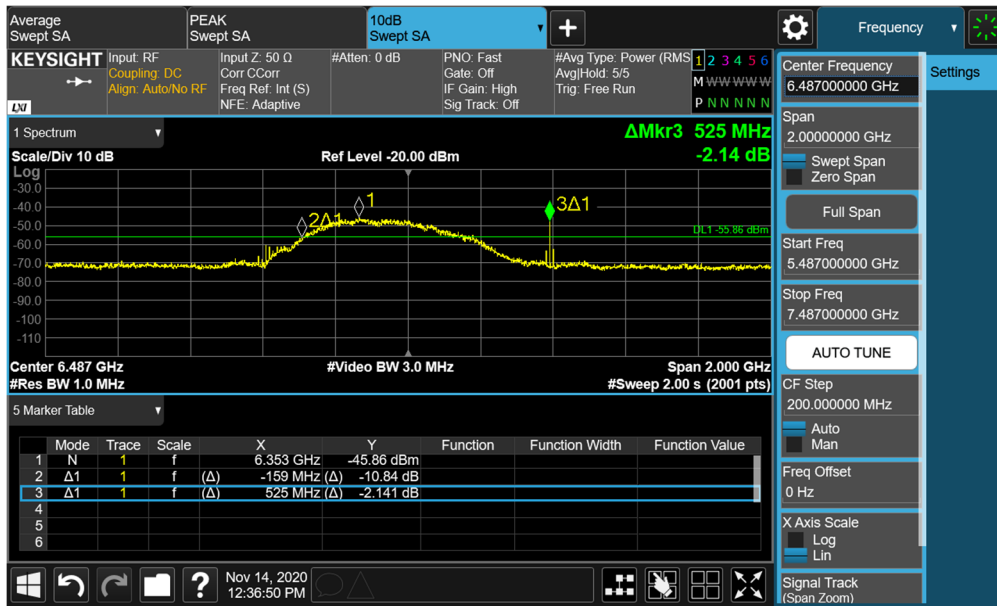
Plot 7-20. BANDWIDTH Plot – ANT1 - CH.5 – SP1 – Preamble 12
