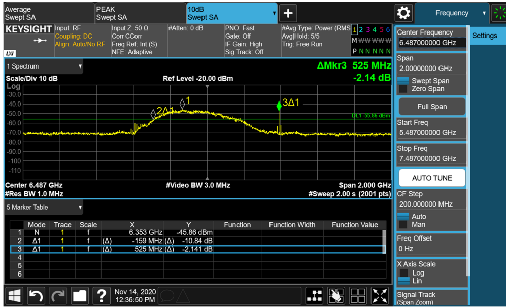
Plot 7-23. BANDWIDTH Plot – ANT2 - CH.5 – SP1 – Preamble 12
