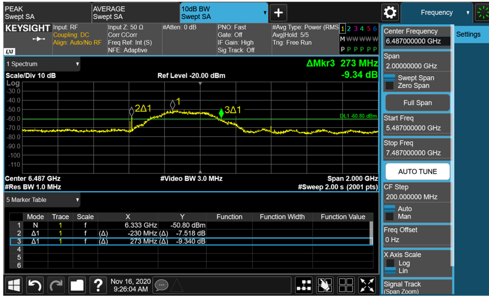
Plot 7-27. BANDWIDTH Plot – ANT1 - CH.5 – SP3 – Preamble 25
