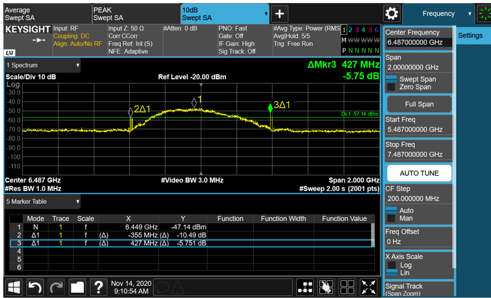
Plot 7-18. BANDWIDTH Plot – ANT2 - CH.5 – SP3 – Preamble 11
