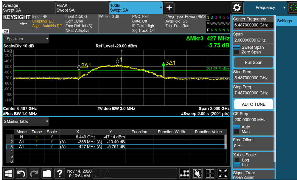
Plot 7-17. BANDWIDTH Plot – ANT2 - CH.5 – SP1 – Preamble 11
