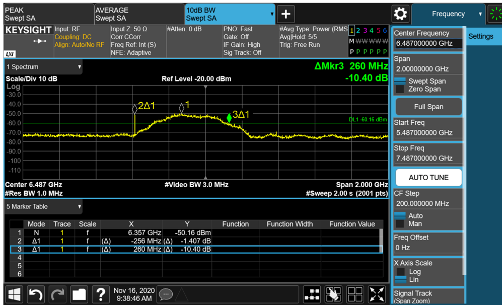
Plot 7-32. BANDWIDTH Plot – ANT1 - CH.5 – SP1 – Preamble 26
