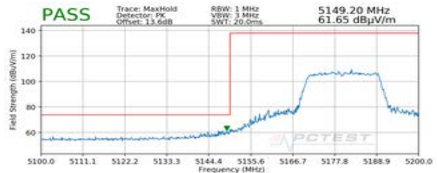
Plot 7-418. Radiated Lower Band Edge Plot MIMO (Peak – UNII Band 1 – 242 Tones)
