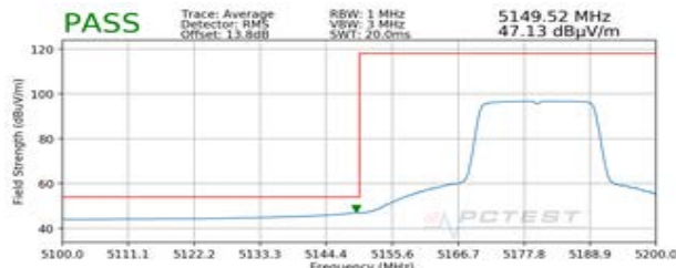
Plot 7-417. Radiated Lower Band Edge Plot MIMO (Average – UNII Band 1 – 242 Tones)
