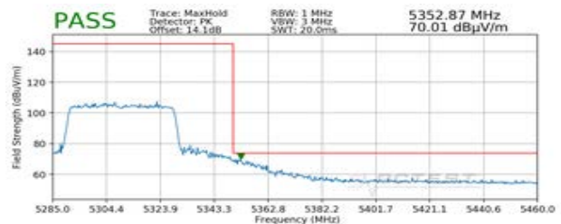
Plot 7-406. Radiated Upper Band Edge Plot SISO ANT2 (Peak – UNII Band 2A – 484 Tones)
