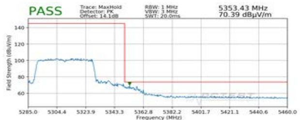
Plot 7-427. Radiated Upper Band Edge Plot MIMO (Peak – UNII Band 2A – 484 Tones)
