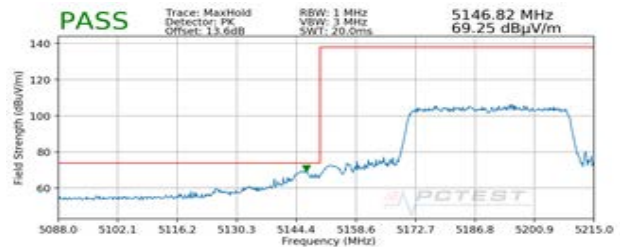
Plot 7-404. Radiated Lower Band Edge Plot SISO ANT2 (Peak – UNII Band 1 – 484 Tones)
