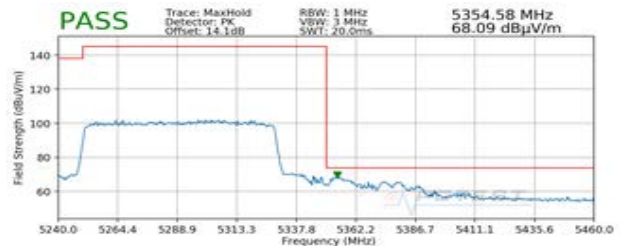
Plot 7-413. Radiated Upper Band Edge Plot SISO ANT2 (Peak – UNII Band 2A – 996 Tones)
