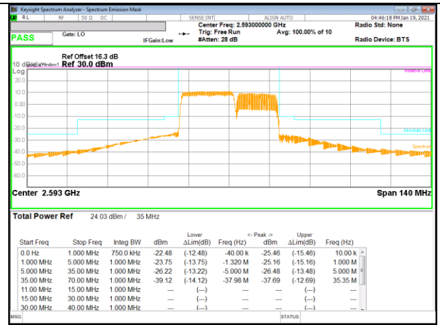
LTE B41 20MHz + 15MHz 16QAM Mid Ch RB100-0 + RB75-0
