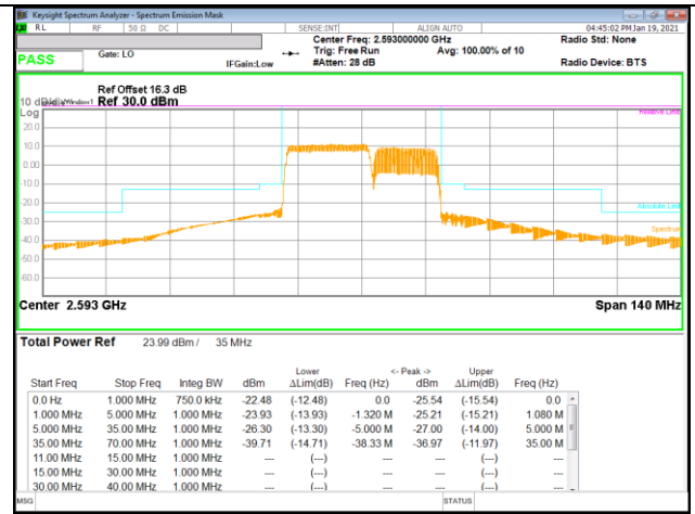
LTE B41 20MHz + 15MHz QPSK Mid Ch RB100-0 + RB75-0
