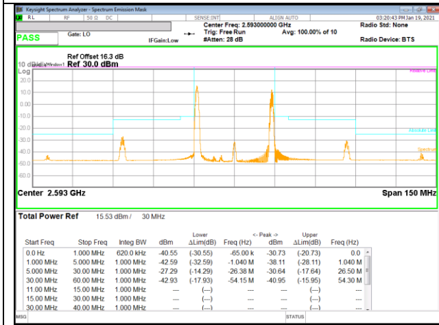
LTE B41 10MHz + 20MHz 16QAM Mid Ch RB1-0 + RB1-99
