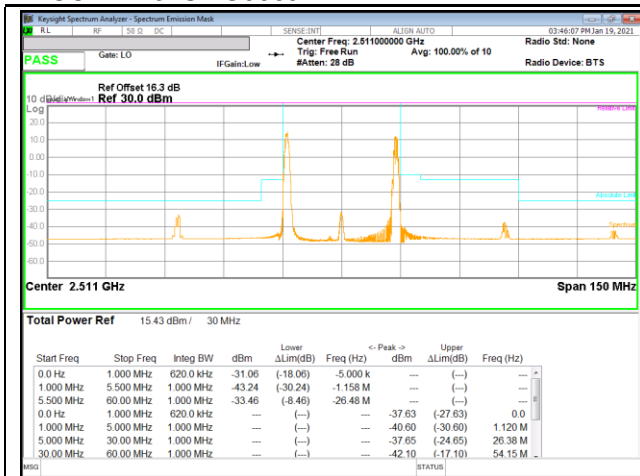
LTE B41 20MHz + 10MHz 16QAM Low Ch RB1-0 + RB1-49
