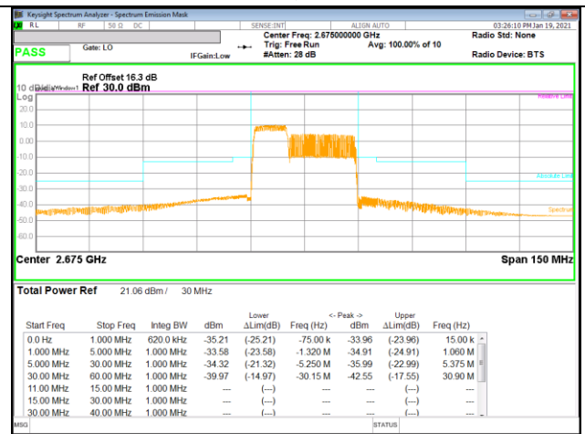
LTE B41 10MHz + 20MHz 16QAM High Ch RB50-0 + RB100-0
