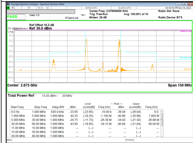
LTE B41 20MHz + 10MHz QPSK High Ch RB1-0 + RB1-49
