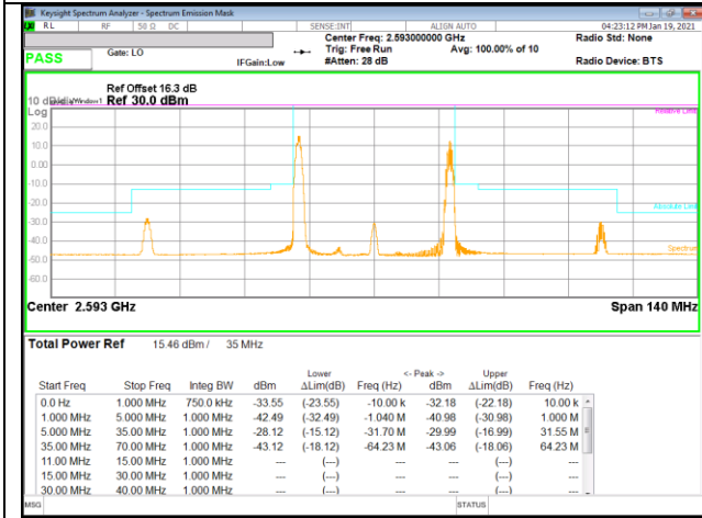
LTE B41 15MHz + 20MHz 16QAM Mid Ch RB1-0 + RB1-99
