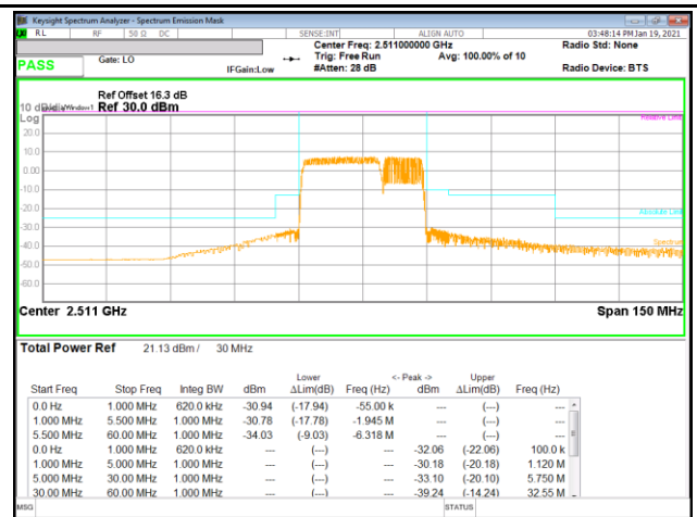
LTE B41 20MHz + 10MHz 16QAM Low Ch RB100-0 + RB50-0
