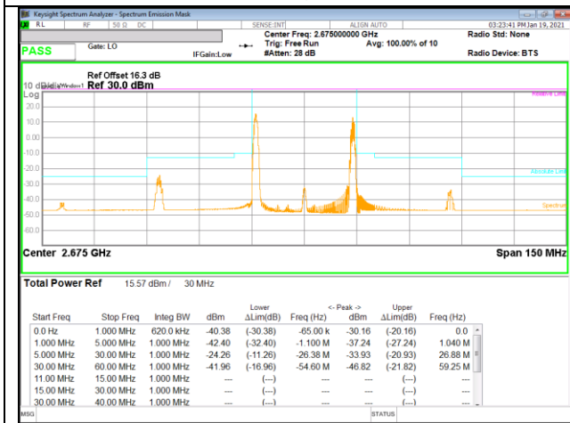
LTE B41 10MHz + 20MHz 16QAM High Ch RB1-0 + RB1-99
