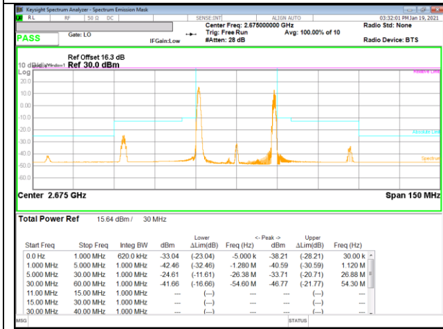
LTE B41 20MHz + 10MHz 16QAM High Ch RB1-0 + RB1-49
