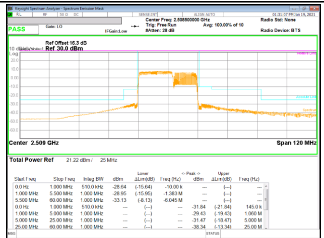
LTE B41 15MHz + 10MHz 16QAM Low Ch RB75-0 + RB50-0
