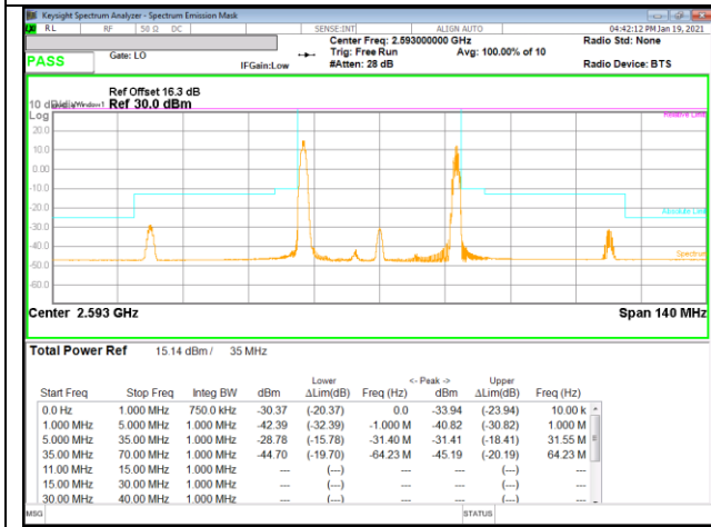
LTE B41 20MHz + 15MHz QPSK Mid Ch RB1-0 + RB1-74
