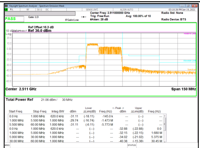
LTE B41 10MHz + 20MHz 16QAM Low Ch RB50-0 + RB100-0
