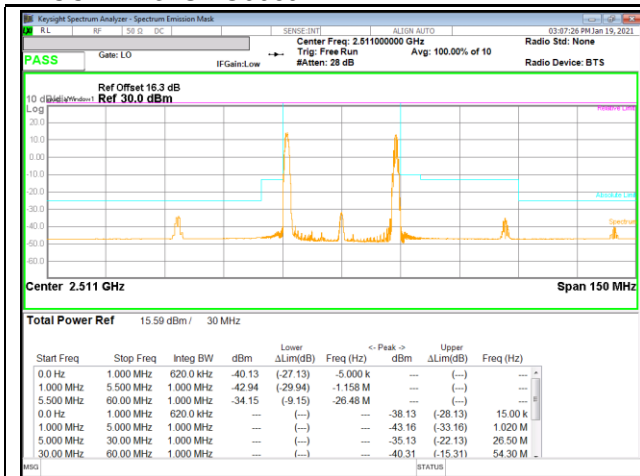
LTE B41 10MHz + 20MHz 16QAM Low Ch RB1-0 + RB1-99
