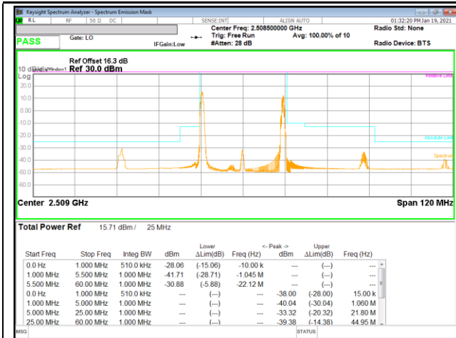
LTE B41 15MHz + 10MHz 16QAM Low Ch RB1-0 + RB1-49
