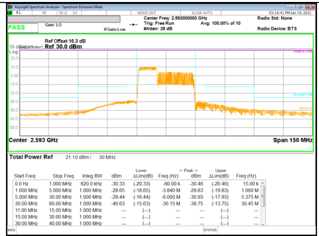
LTE B41 10MHz + 20MHz 16QAM Mid Ch RB50-0 + RB100-0
