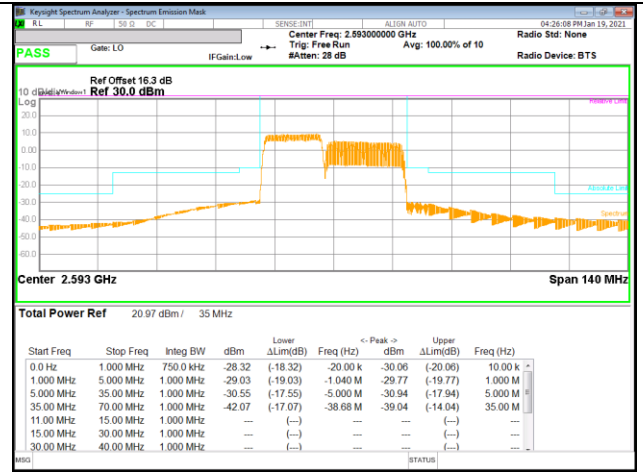
LTE B41 15MHz + 20MHz 16QAM Mid Ch RB75-0 + RB100-0
