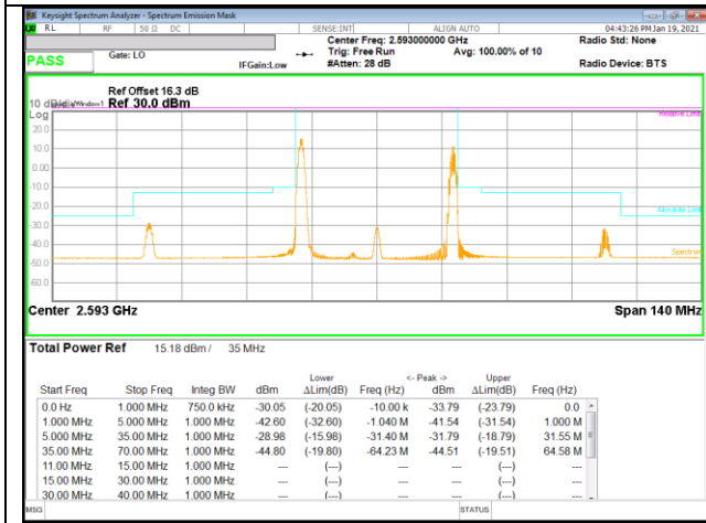
LTE B41 20MHz + 15MHz 16QAM Mid Ch RB1-0 + RB1-74
