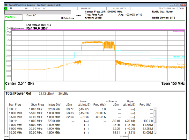
LTE B41 20MHz + 10MHz QPSK Low Ch RB100-0 + RB50-0
