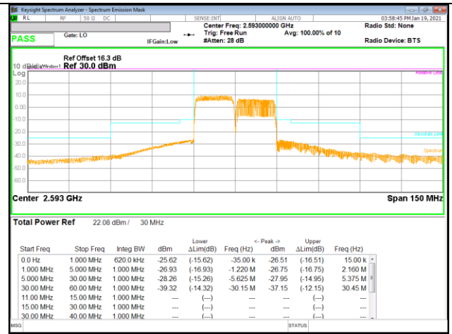
LTE B41 15MHz + 15MHz QPSK Mid Ch RB75-0 + RB75-0
