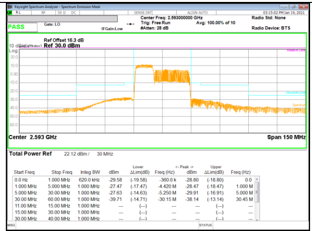
LTE B41 10MHz + 20MHz QPSK Mid Ch RB50-0 + RB100-0
