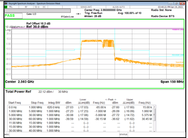
LTE B41 20MHz + 10MHz QPSK Mid Ch RB100-0 + RB50-0
