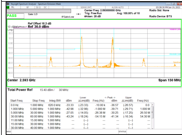
LTE B41 20MHz + 10MHz 16QAM Mid Ch RB1-0 + RB1-49
