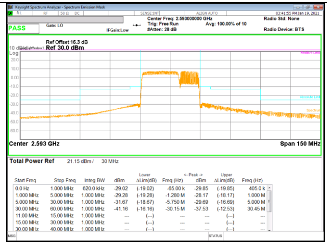
LTE B41 20MHz + 10MHz 16QAM Mid Ch RB100-0 + RB50-0
