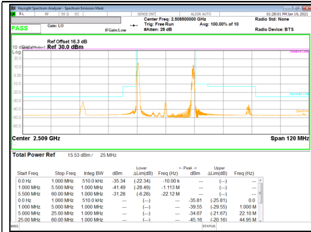
LTE B41 10MHz + 15MHz QPSK Low Ch RB1-0 + RB1-74
