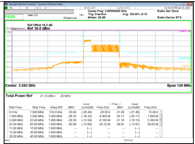
LTE B41 5MHz + 20MHz 16QAM Mid Ch RB25-0 + RB100-0
