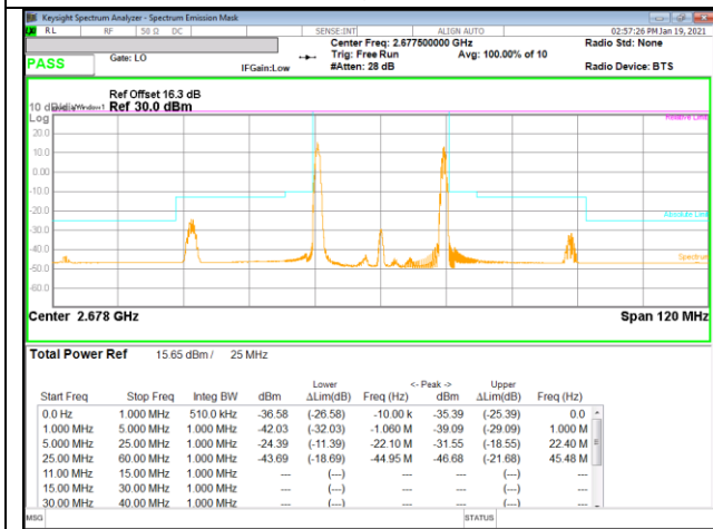
LTE B41 15MHz + 10MHz QPSK High Ch RB1-0 + RB1-49
