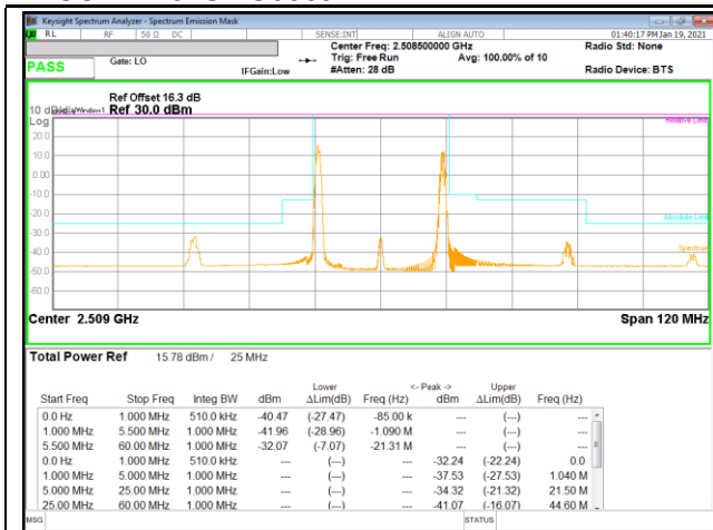
LTE B41 5MHz + 20MHz 16QAM Low Ch RB1-0 + RB1-99
