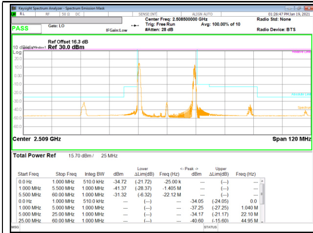
LTE B41 10MHz + 15MHz 16QAM Low Ch RB1-0 + RB1-74
