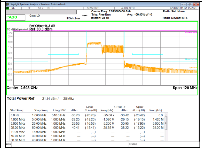
LTE B41 10MHz + 15MHz 16QAM Mid Ch RB50-0 + RB75-0
