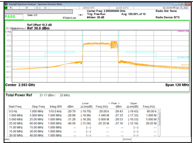
LTE B41 20MHz + 5MHz 16QAM Mid Ch RB100-0 + RB25-0
