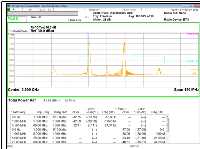
LTE B41 20MHz + 5MHz 16QAM Low Ch RB1-0 + RB1-24
