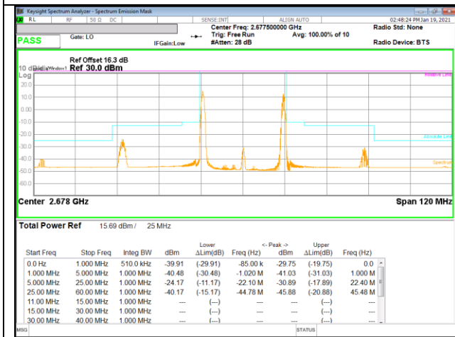
LTE B41 10MHz + 15MHz 16QAM High Ch RB1-0 + RB1-74
