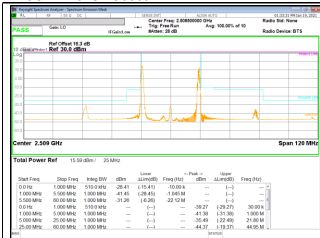
LTE B41 15MHz + 10MHz QPSK Low Ch RB1-0 + RB1-49
