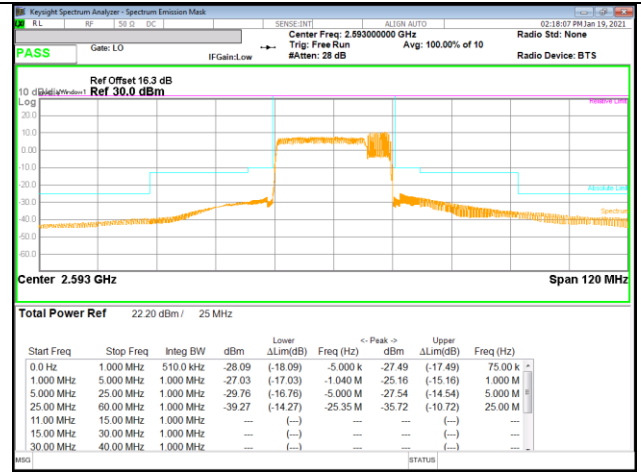
LTE B41 20MHz + 5MHz QPSK Mid Ch RB100-0 + RB25-0
