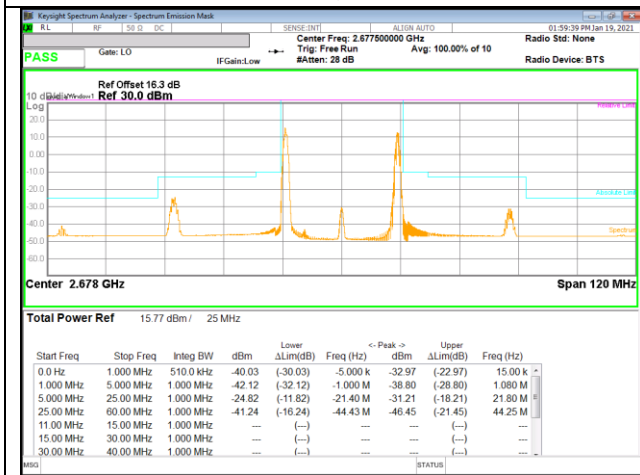
LTE B41 5MHz + 20MHz 16QAM High Ch RB1-0 + RB1-99
