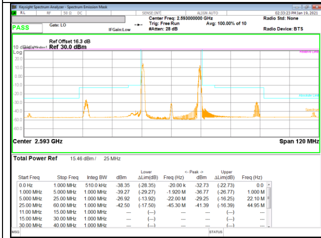
LTE B41 10MHz + 15MHz 16QAM Mid Ch RB1-0 + RB1-74
