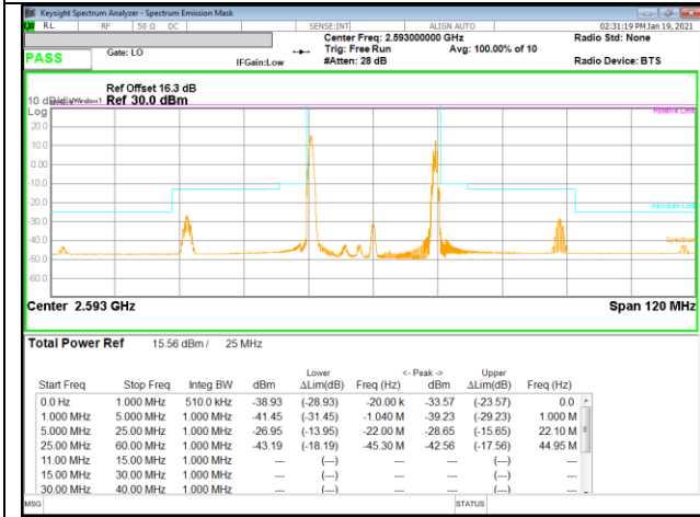
LTE B41 10MHz + 15MHz QPSK Mid Ch RB1-0 + RB1-74
