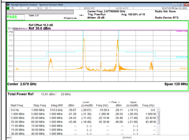
LTE B41 10MHz + 15MHz QPSK High Ch RB1-0 + RB1-74
