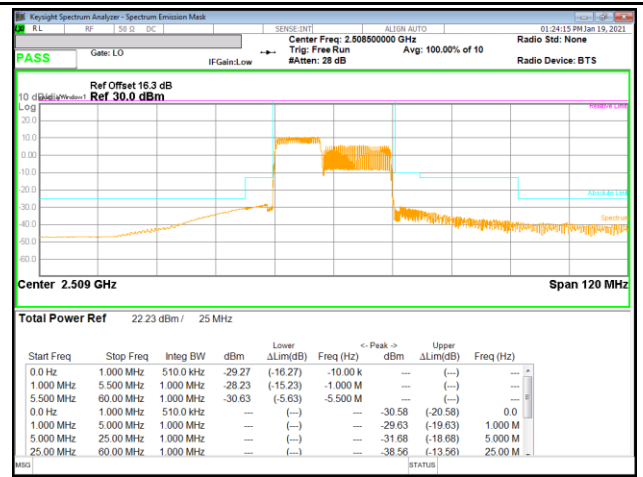
LTE B41 10MHz + 15MHz QPSK Low Ch RB50-0 + RB75-0
