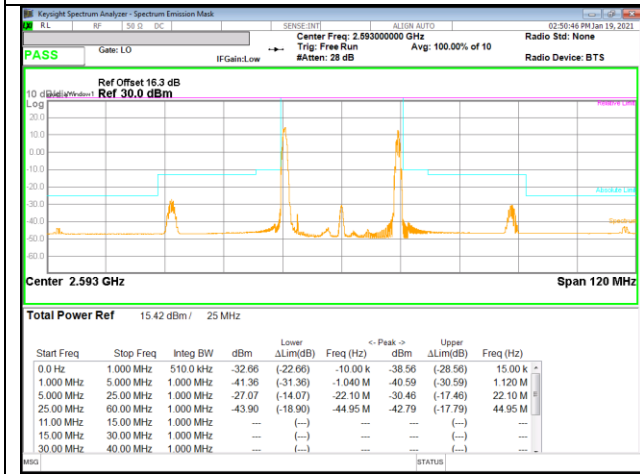
LTE B41 15MHz + 10MHz QPSK Mid Ch RB1-0 + RB1-49
