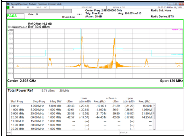
LTE B41 5MHz + 20MHz 16QAM Mid Ch RB1-0 + RB1-99
