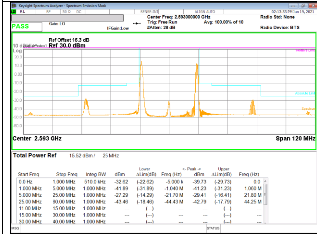
LTE B41 20MHz + 5MHz QPSK Mid Ch RB1-0 + RB1-24
