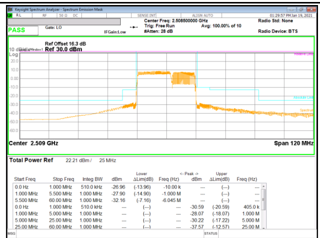
LTE B41 15MHz + 10MHz QPSK Low Ch RB75-0 + RB50-0
