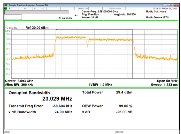
LTE B41 10MHz + 15MHz 16QMA RB50-0 + RB75-0
