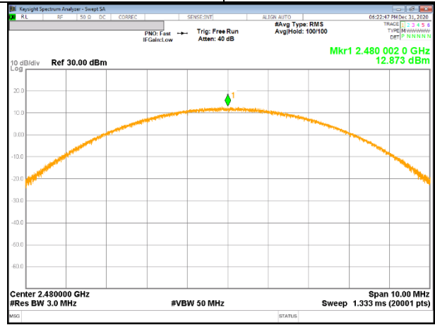
8PSK, 78 CHANNEL
