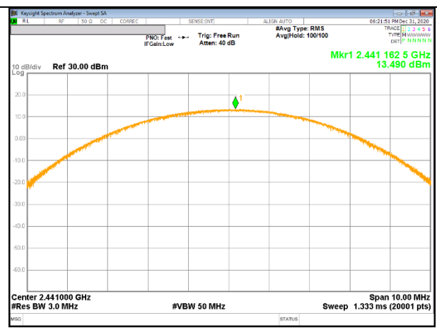
Pi/4-DPSK, 39 CHANNEL
