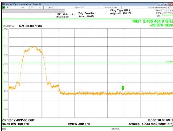
78 CHANNEL BANDEDGE
