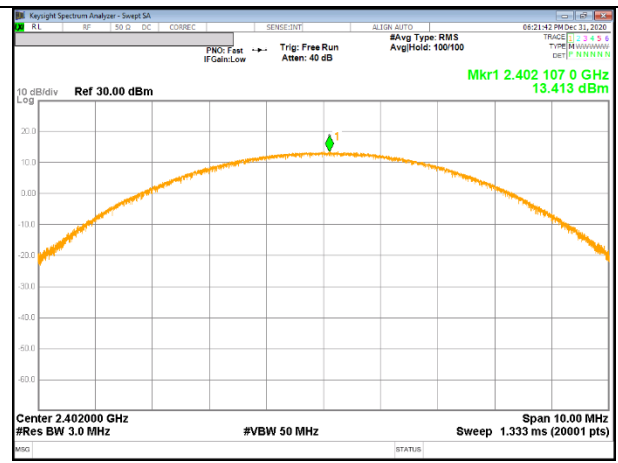
Pi/4-DPSK, 0 CHANNEL
