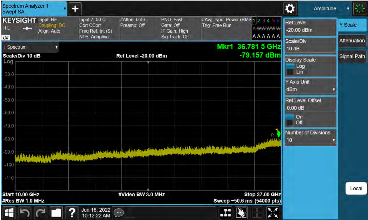
Sub6 n48. Conducted Spurious Plot 2 (20 MHz Ch. 646000 QPSK RB 1, Offset 1)
