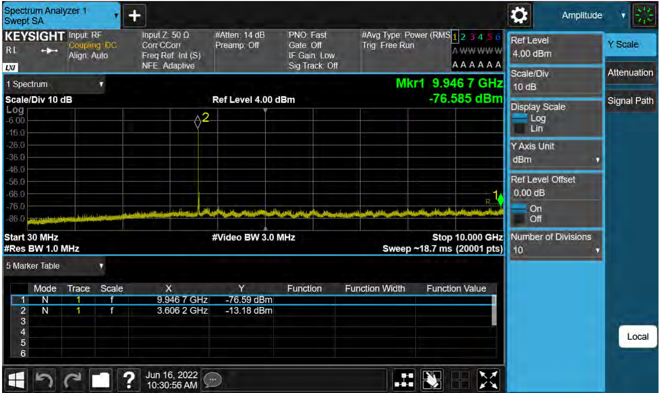
Sub6 n48. Conducted Spurious Plot 1 (40 MHz Ch. 641666 QPSK RB 1, Offset 1)
