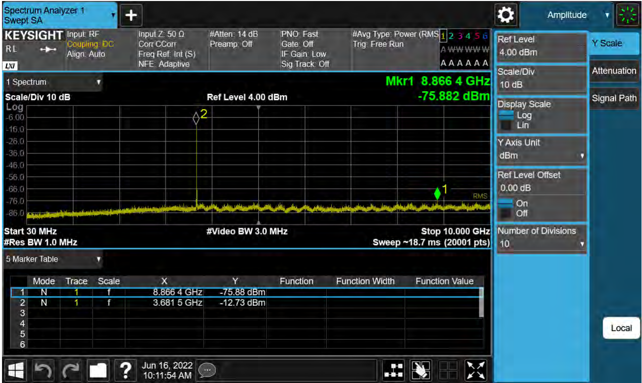
Sub6 n48. Conducted Spurious Plot 1 (20 MHz Ch. 646000 QPSK RB 1, Offset 1)
