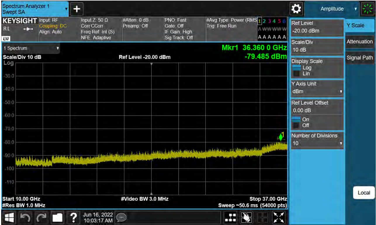
Sub6 n48. Conducted Spurious Plot 2 (20 MHz Ch. 641666 QPSK RB 1, Offset 1)
