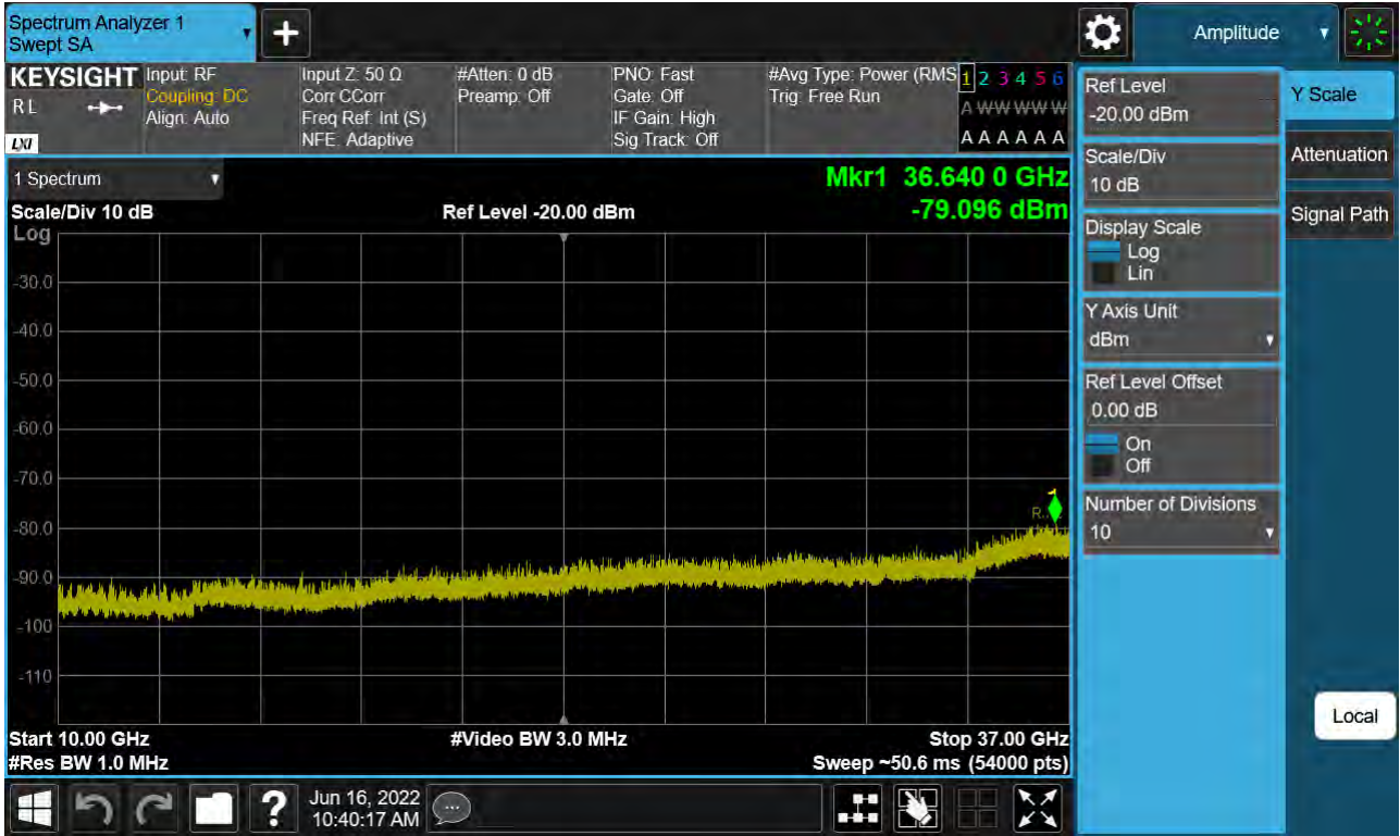
Sub6 n48. Conducted Spurious Plot 2 (40 MHz Ch. 645332 QPSK RB 1, Offset 1)
