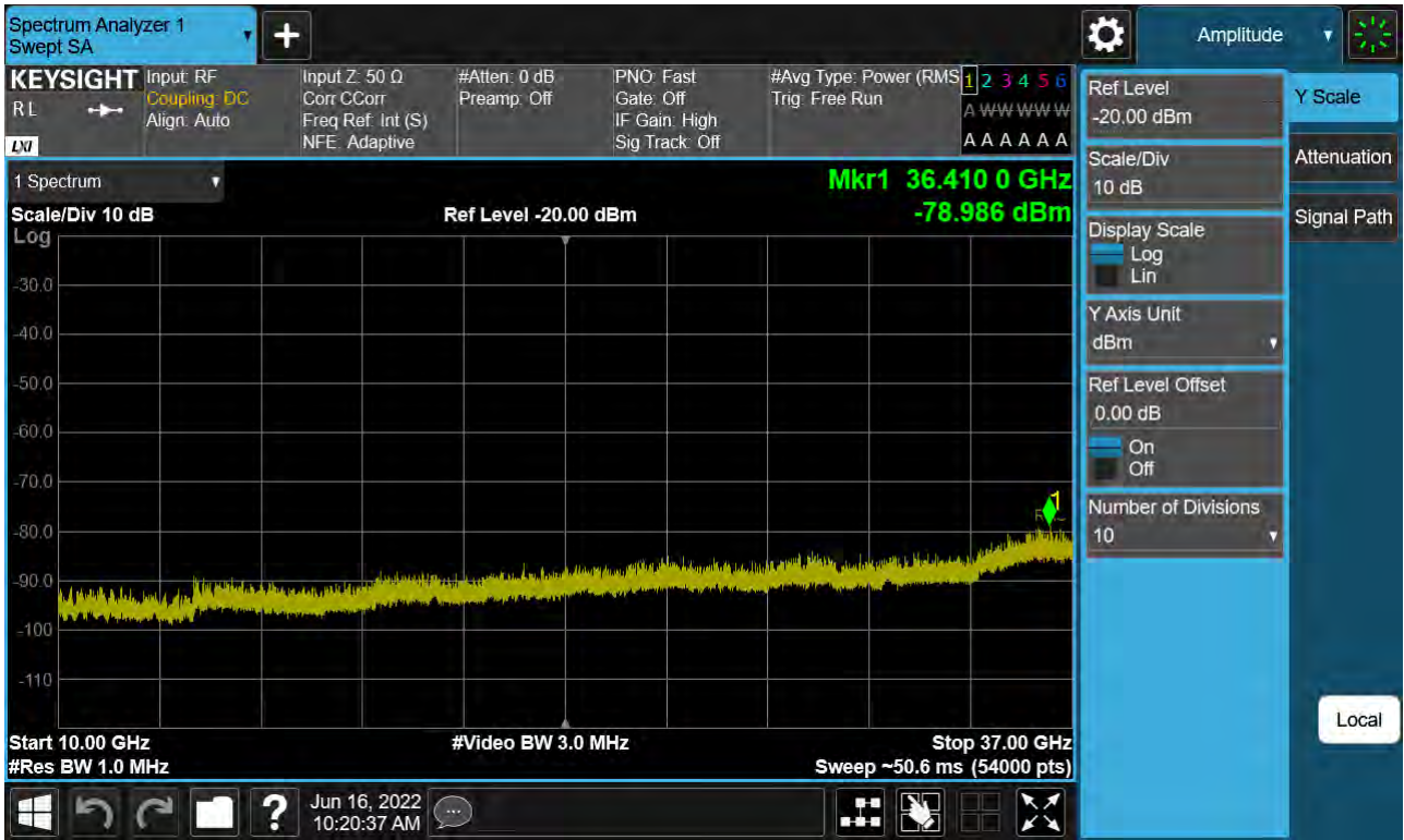
Sub6 n48. Conducted Spurious Plot 2 (40 MHz Ch. 638000 QPSK RB 1, Offset 1)
