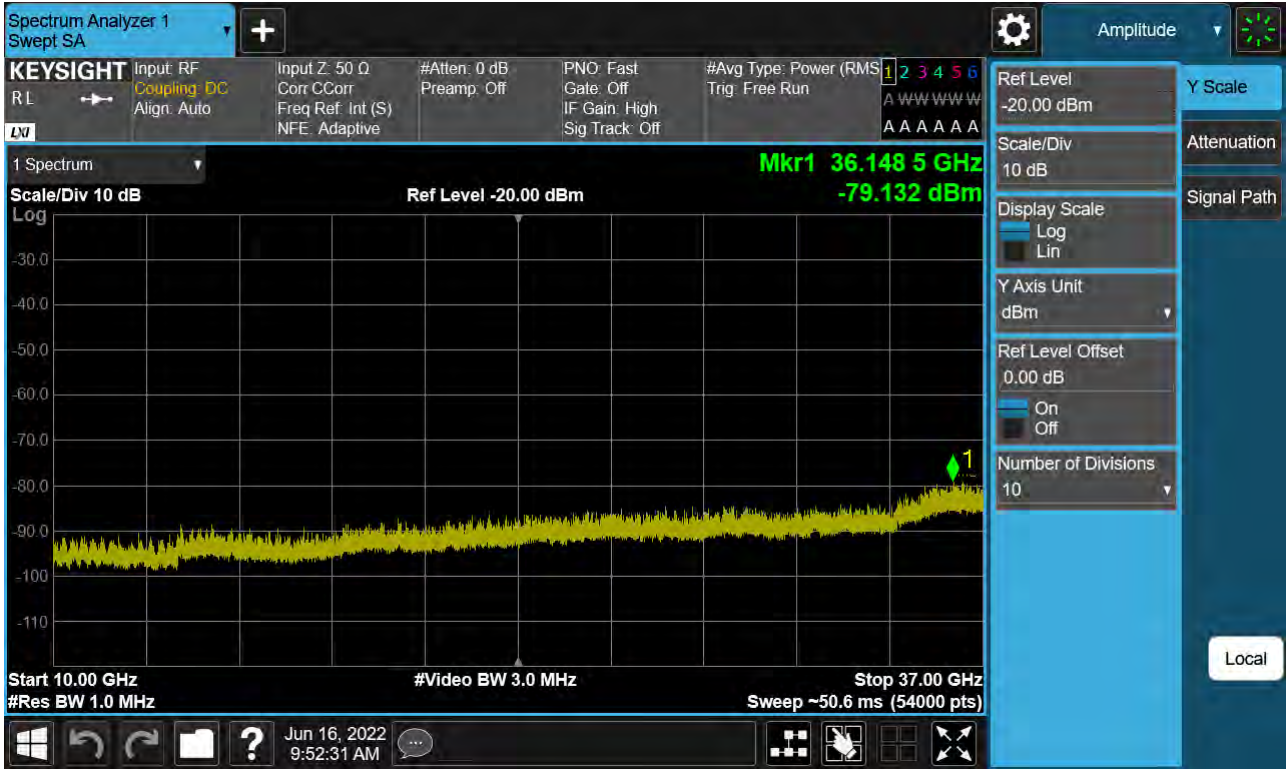
Sub6 n48. Conducted Spurious Plot 2 (20 MHz Ch. 637334 QPSK RB 1, Offset 1)
