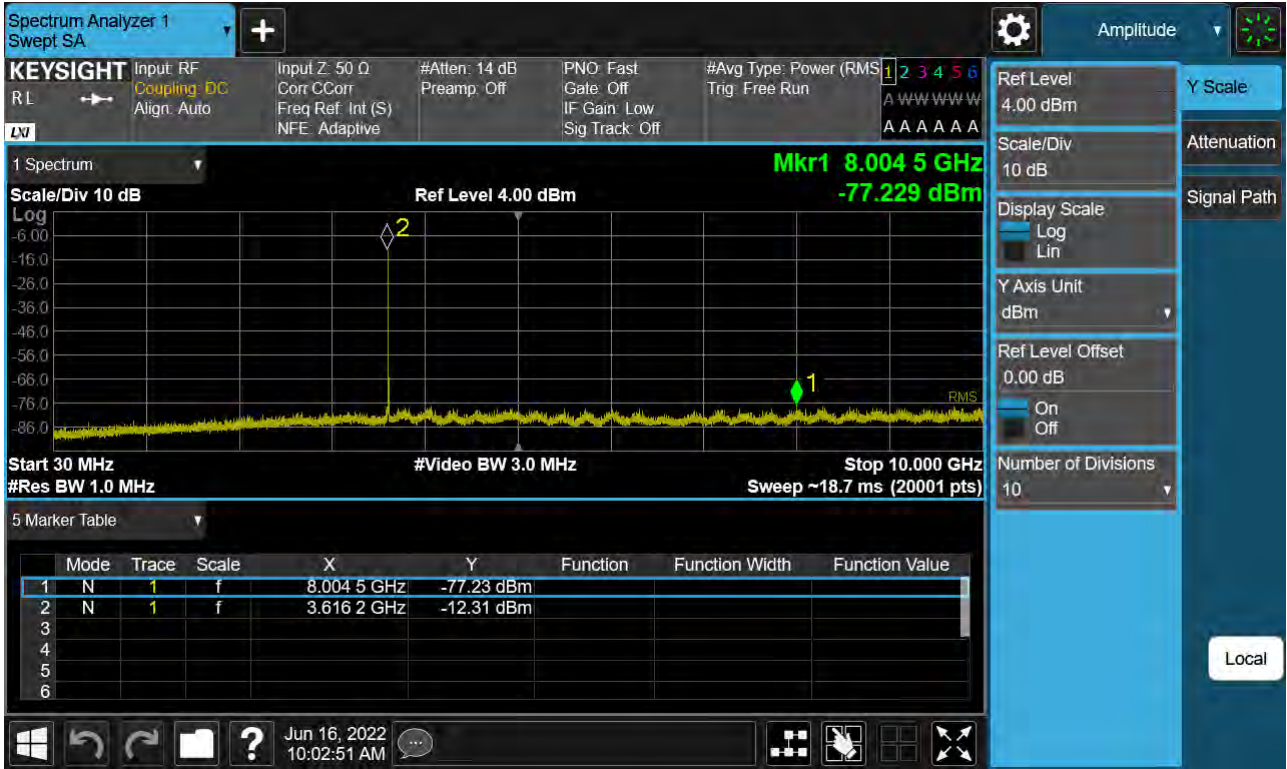
Sub6 n48. Conducted Spurious Plot 1 (20 MHz Ch. 641666 QPSK RB 1, Offset 1)
