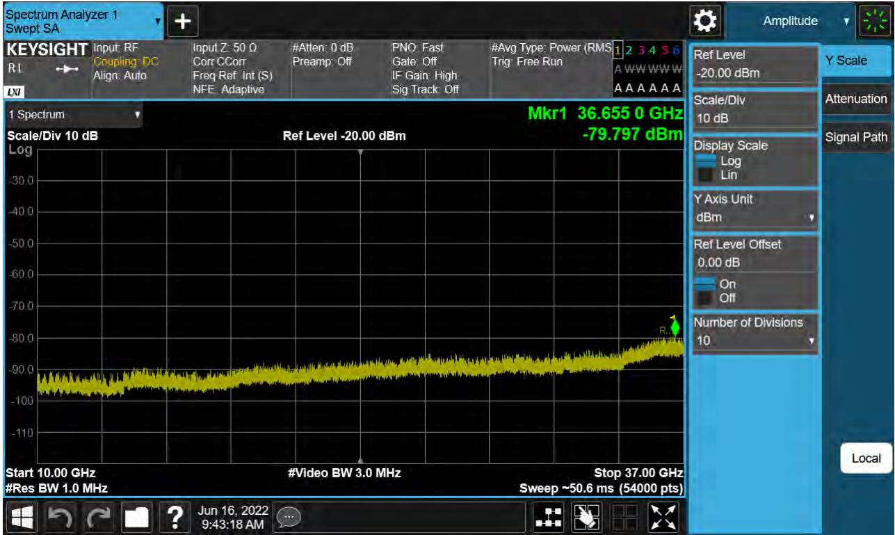
Sub6 n48. Conducted Spurious Plot 2 (10 MHz Ch. 646332 QPSK RB 1, Offset 1)
