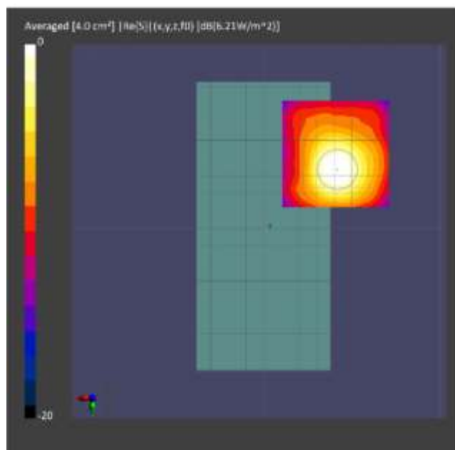
Figure 10-3: 4cm 2 -averaged power density distribution measured at input.power.limit of 11.1 dBm on the Rear surface for n260 beam 4
