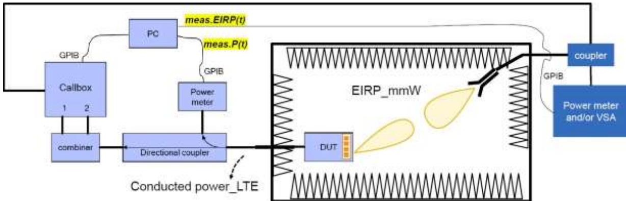
Figure 10-1 mmW NR radiated power measurement setup (see Appendix E for missing figures)
