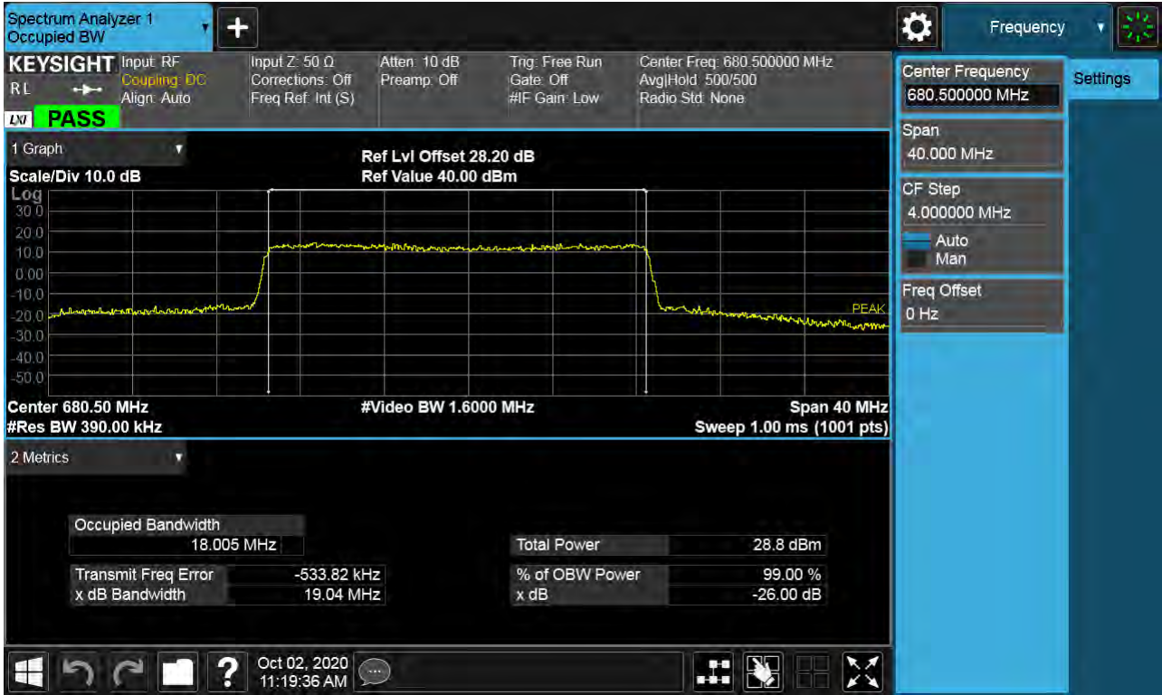
Sub6 n71. Occupied Bandwidth Plot (20M BW Ch.136100 256QAM_RB50_0)
