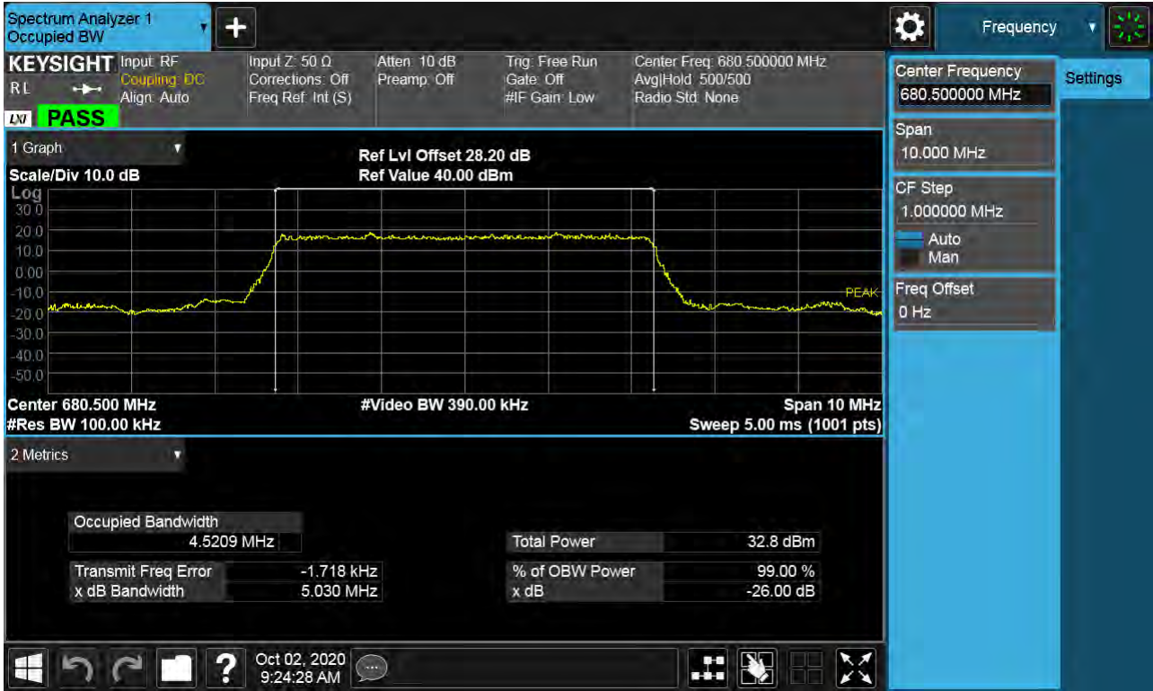
Sub6 n71. Occupied Bandwidth Plot (5M BW Ch.136100 BPSK_RB6_0)
