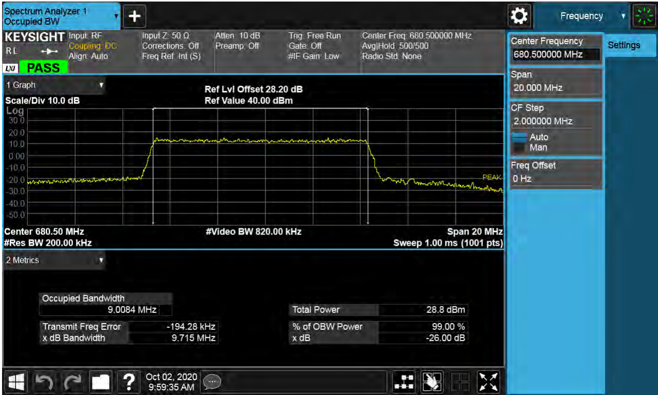
Sub6 n71. Occupied Bandwidth Plot (10M BW Ch.136100 256QAM_RB15_0)
