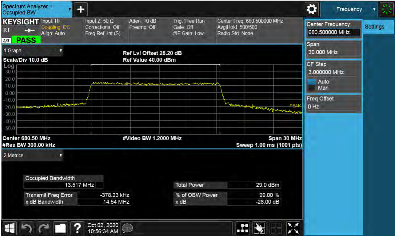
Sub6 n71. Occupied Bandwidth Plot (15M BW Ch.136100 256QAM_RB25_0)
