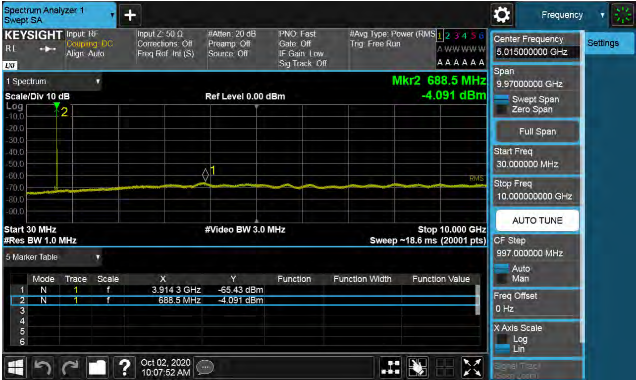
Sub6 n71. Conducted Spurious Plot _ (138600ch_10M Hz_BPSK_RB 1_1)
