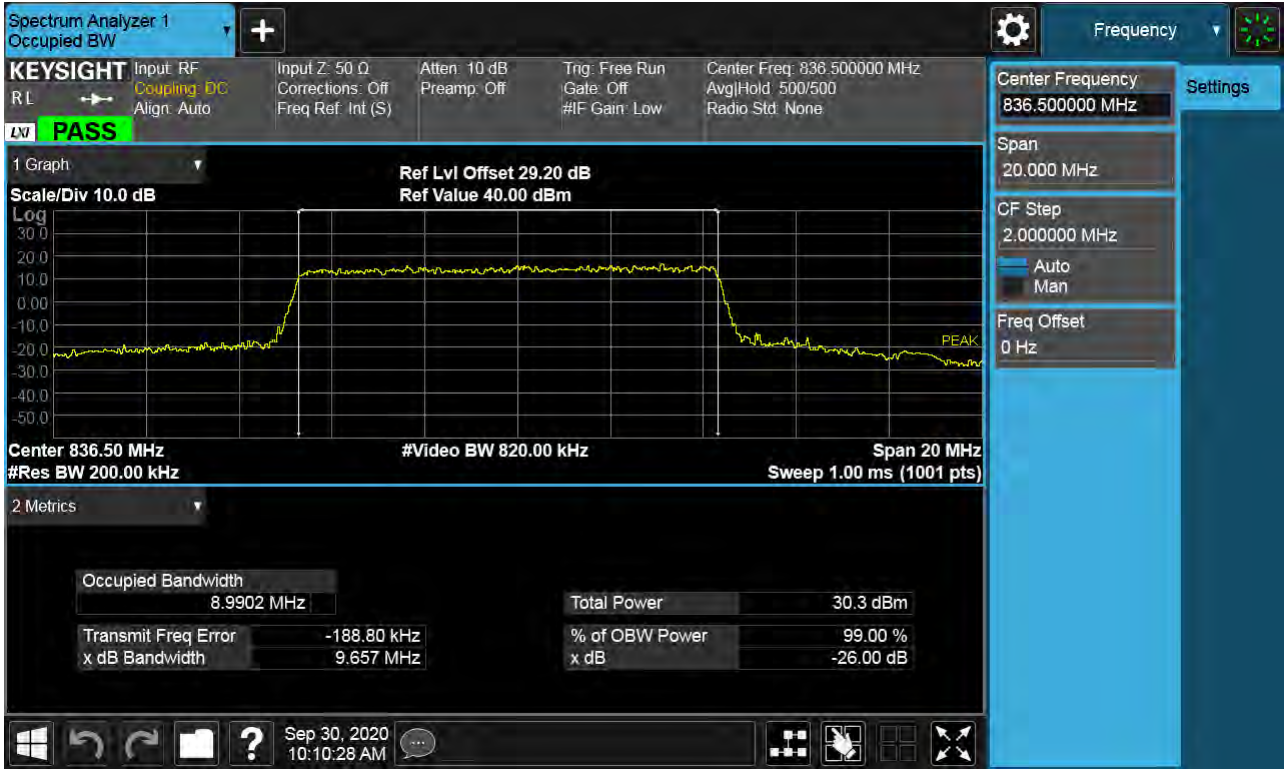
Sub6 n5. Occupied Bandwidth Plot (10M BW Ch.167300 64QAM_RB15_0)
