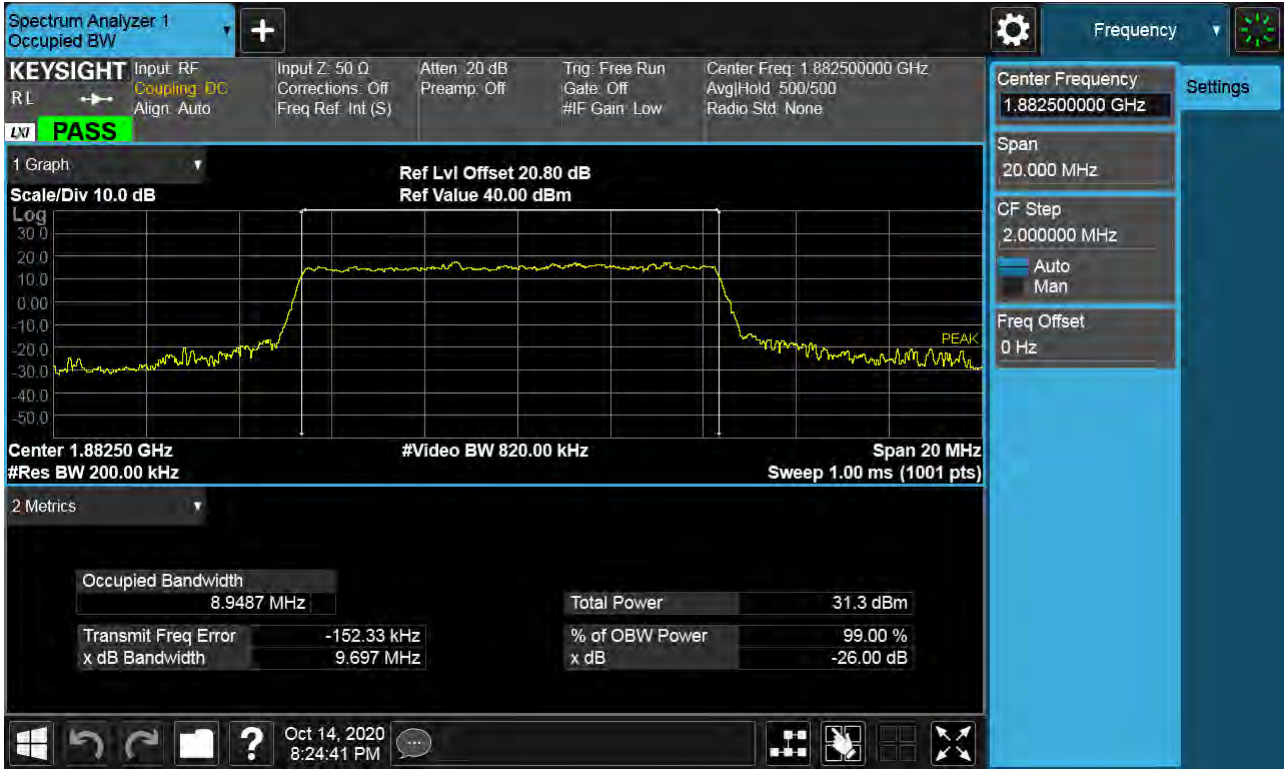
Sub6 n25(2). Occupied Bandwidth Plot (10M BW Ch.376500 QPSK RB 50_0)
