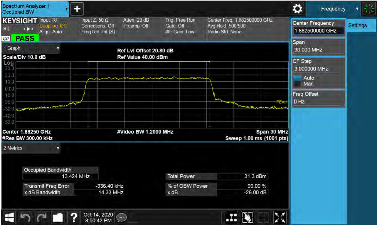
Sub6 n25(2). Occupied Bandwidth Plot (15M BW Ch.376500 QPSK RB 75_0)
