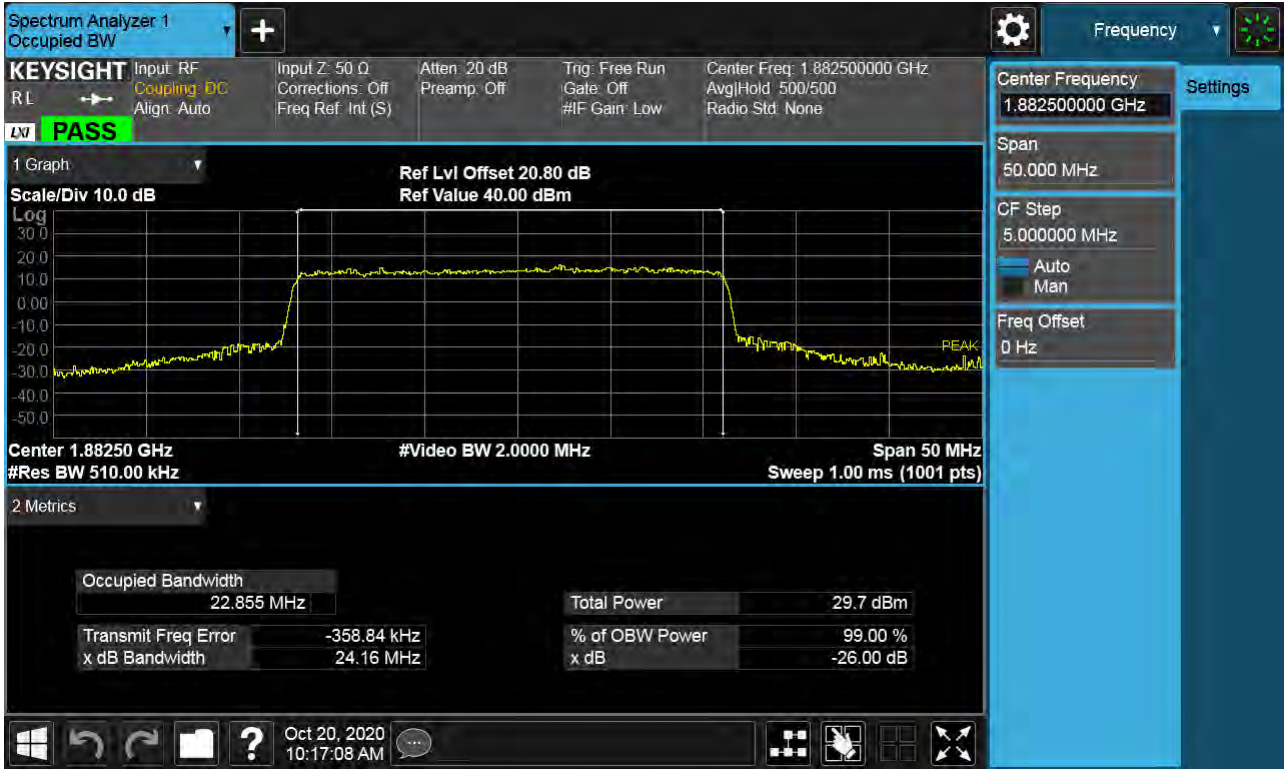
Sub6 n25(2). Occupied Bandwidth Plot (25M BW Ch.376500 64QAM)
