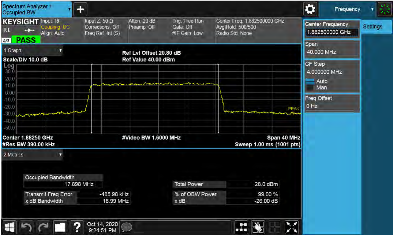
Sub6 n25(2). Occupied Bandwidth Plot (20M BW Ch.376500 256QAM RB 100_0)
