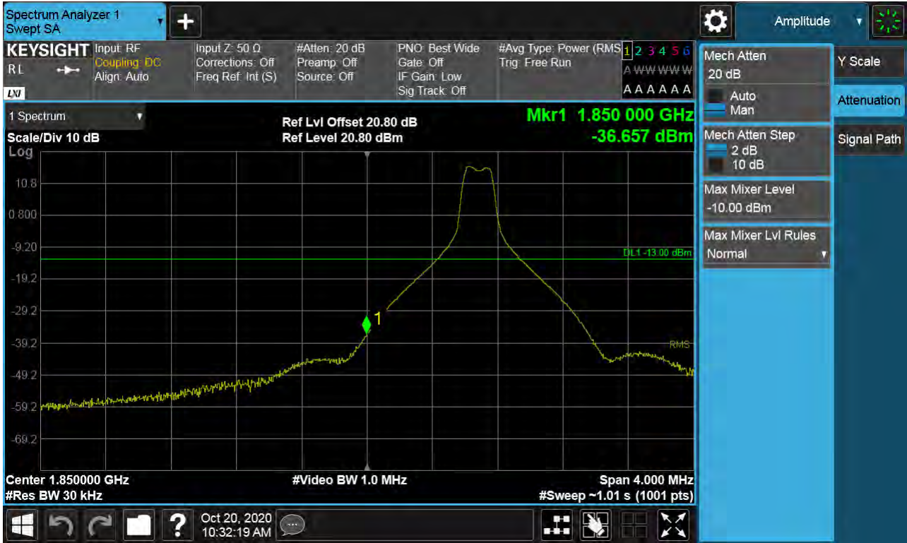
Sub6 n25(2). Lower Band Edge Plot (30M BW Ch.373000 BPSK_RB1_Offset 0)
