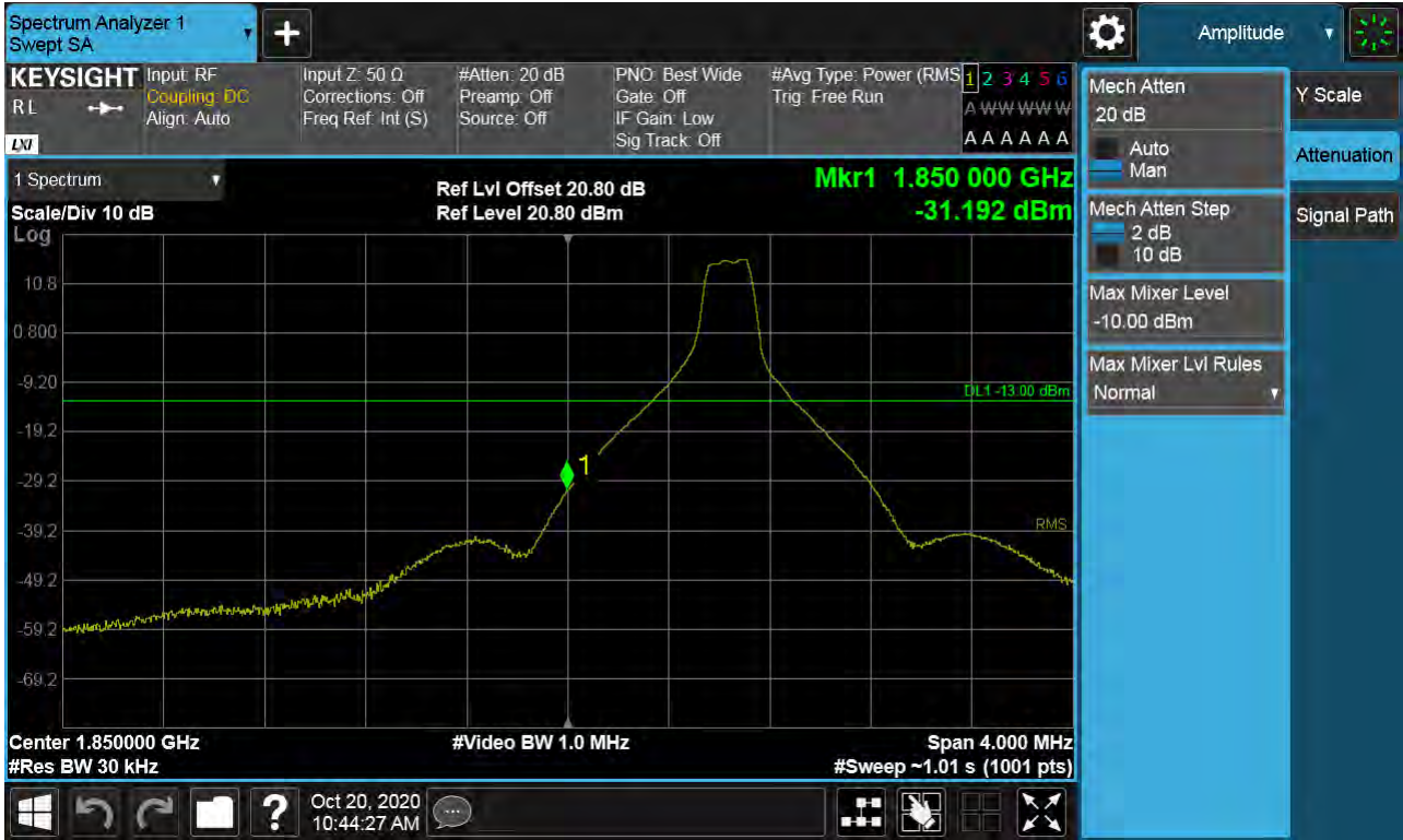
Sub6 n25(2). Lower Band Edge Plot (40M BW Ch.374000 BPSK_RB1_Offset 0)
