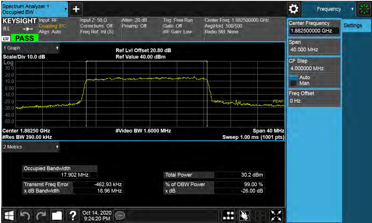
Sub6 n25(2). Occupied Bandwidth Plot (20M BW Ch.376500 64QAM RB 100_0)
