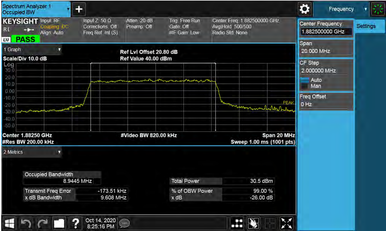
Sub6 n25(2). Occupied Bandwidth Plot (10M BW Ch.376500 16QAM RB 50_0)
