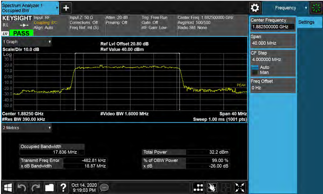
Sub6 n25(2). Occupied Bandwidth Plot (20M BW Ch.376500 BPSK RB 100_0)
