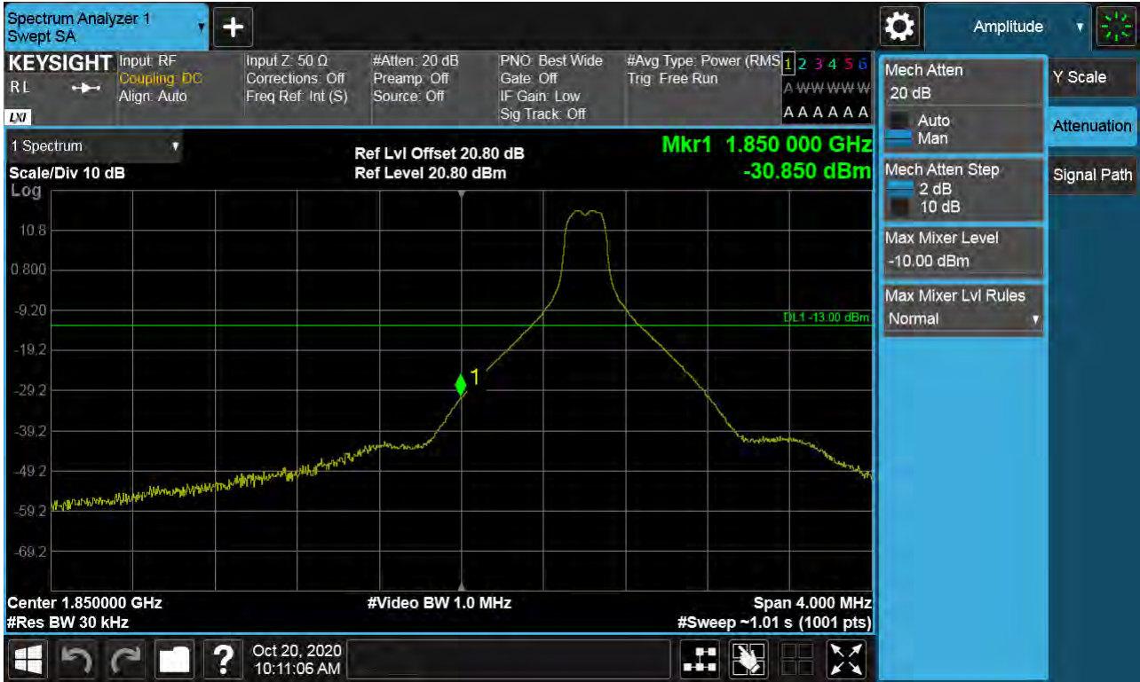
Sub6 n25(2). Lower Band Edge Plot (25M BW Ch.372500 BPSK_RB1_Offset 0)
