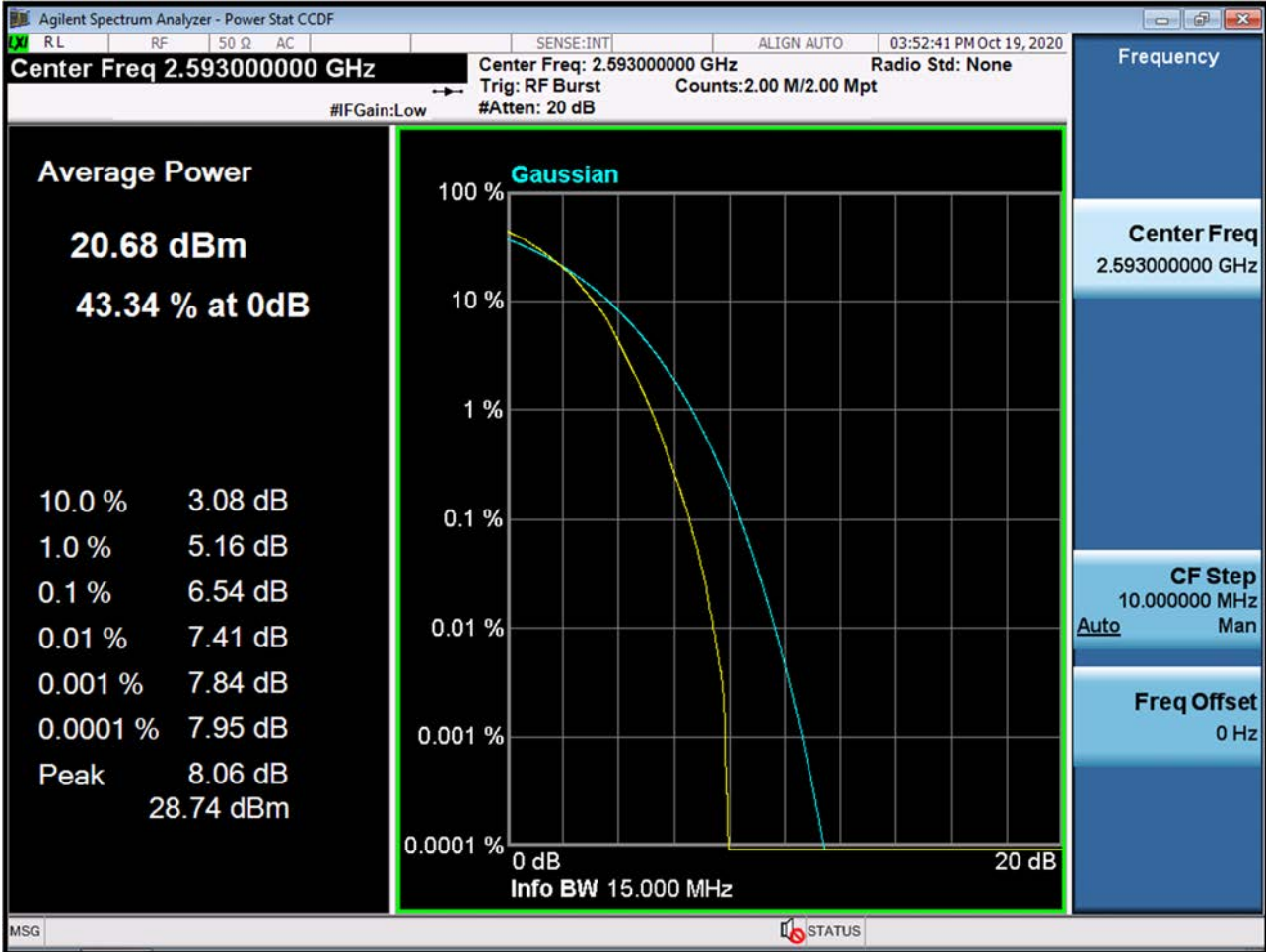
PAR Plot (15M BW_Ch.40620_64QAM_RB75_0) (POWER CLASS 3)
