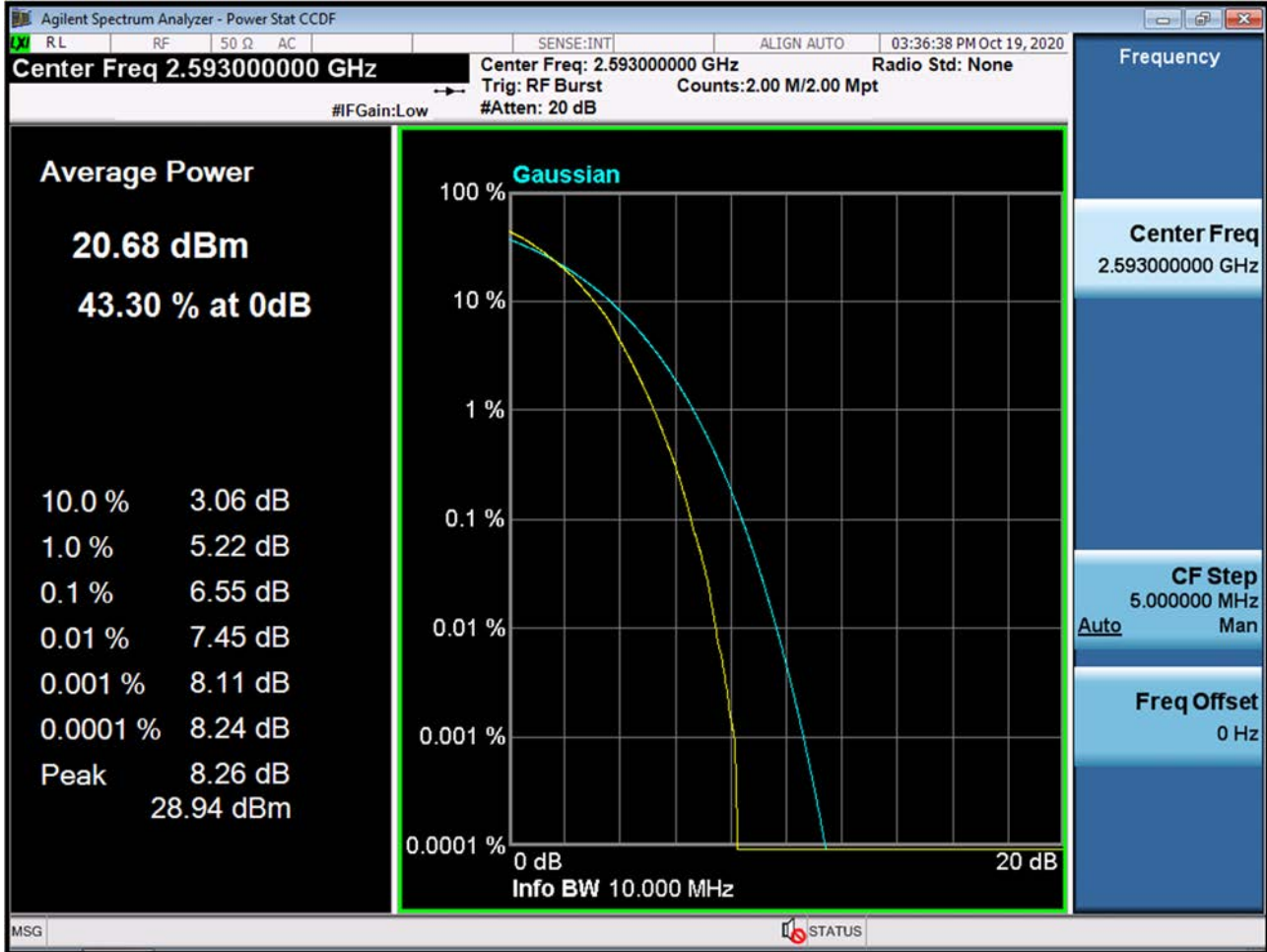
PAR Plot (10M BW_Ch.40620_64QAM_RB50_0) (POWER CLASS 3)
